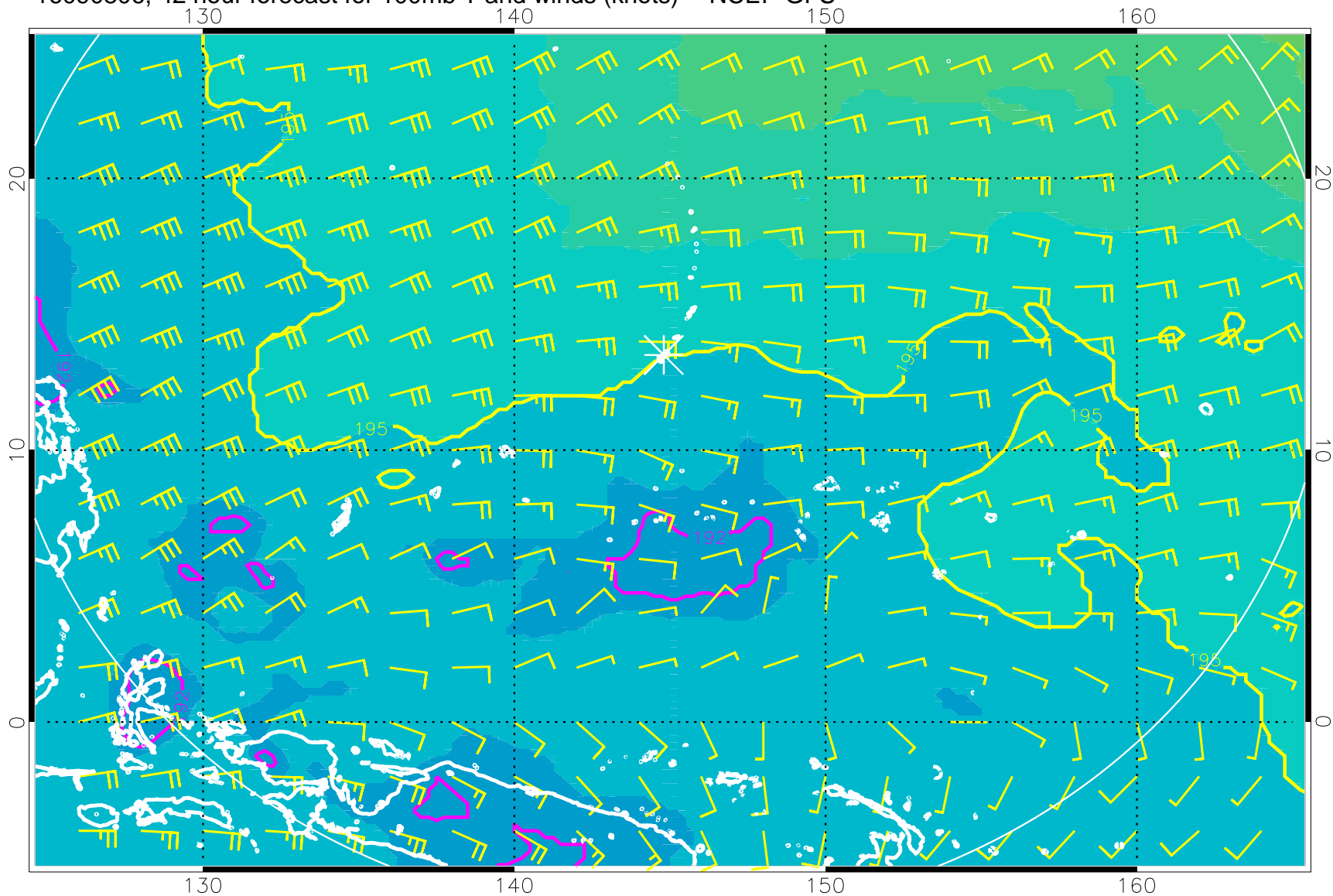
16090806, 42 hour forecast for 100mb T and winds (knots) -- NCEP GFS
