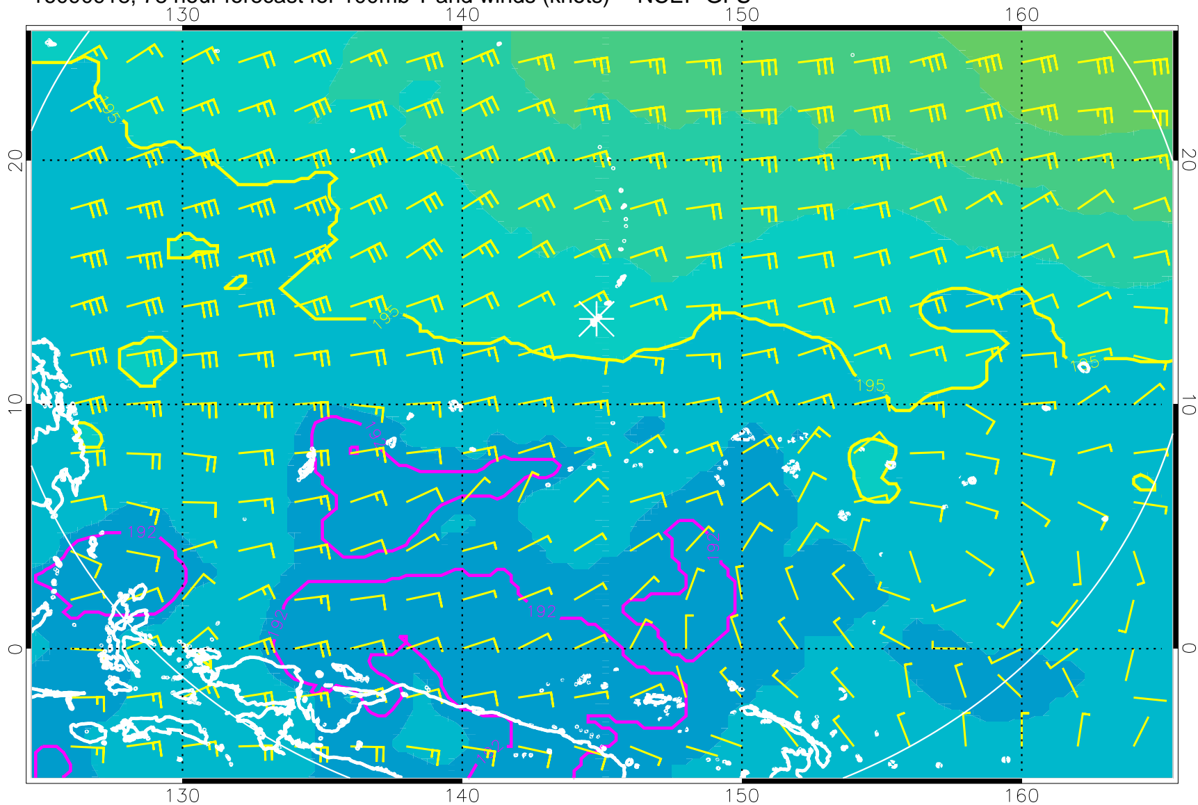
16090918, 78 hour forecast for 100mb T and winds (knots) -- NCEP GFS
