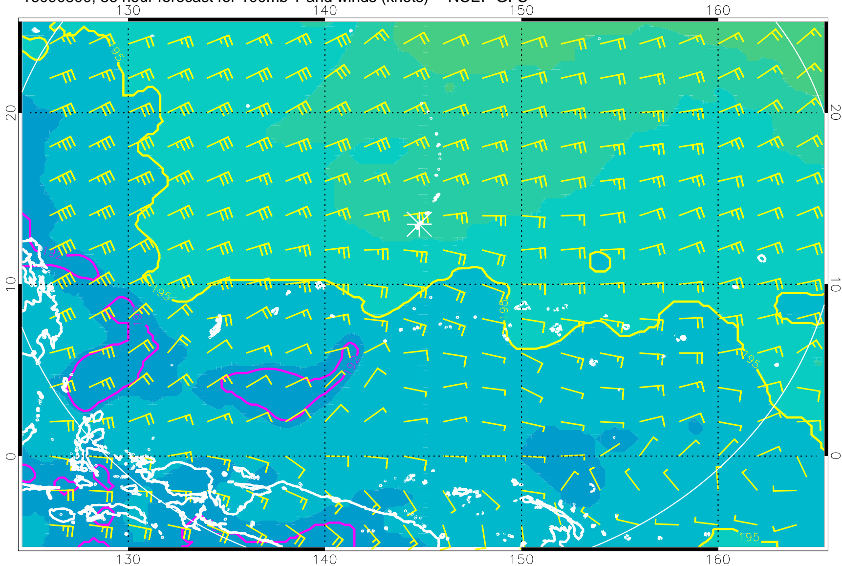
16090800, 36 hour forecast for 100mb T and winds (knots) -- NCEP GFS
