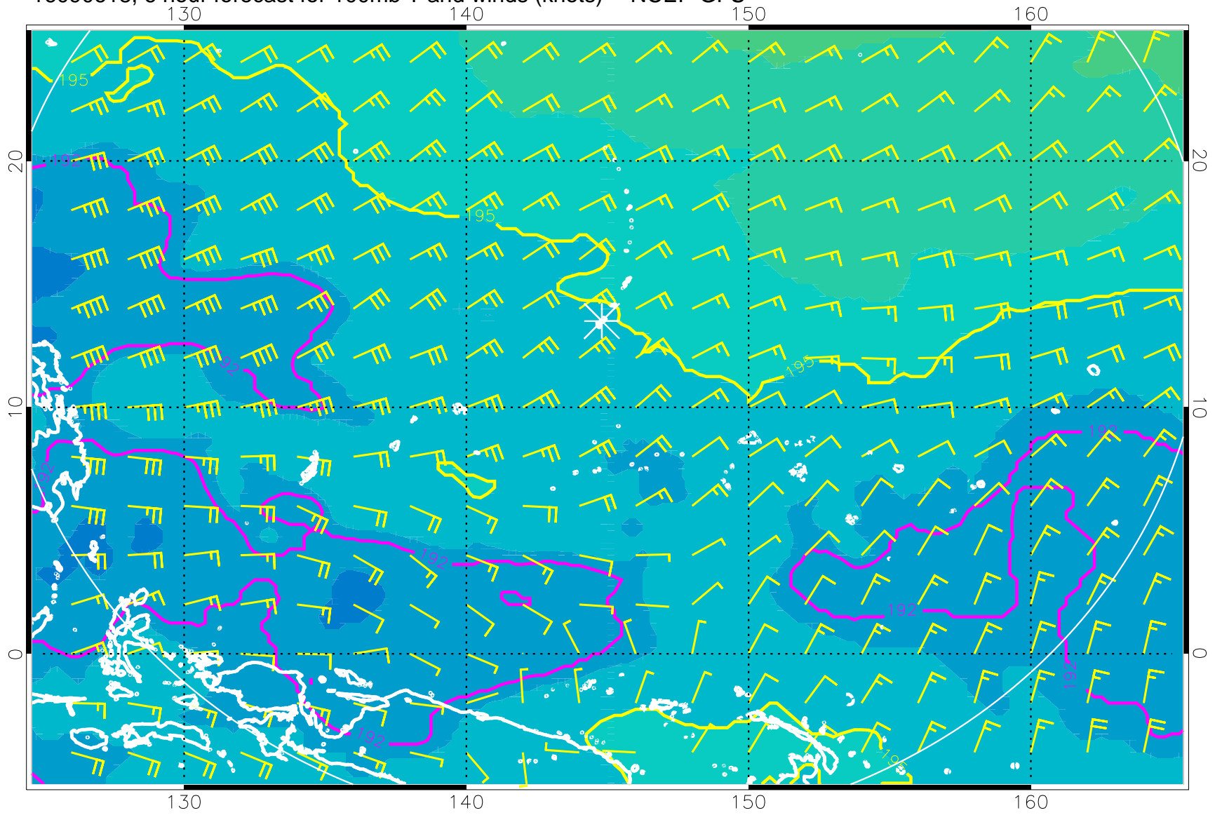
16090618, 6 hour forecast for 100mb T and winds (knots) -- NCEP GFS
