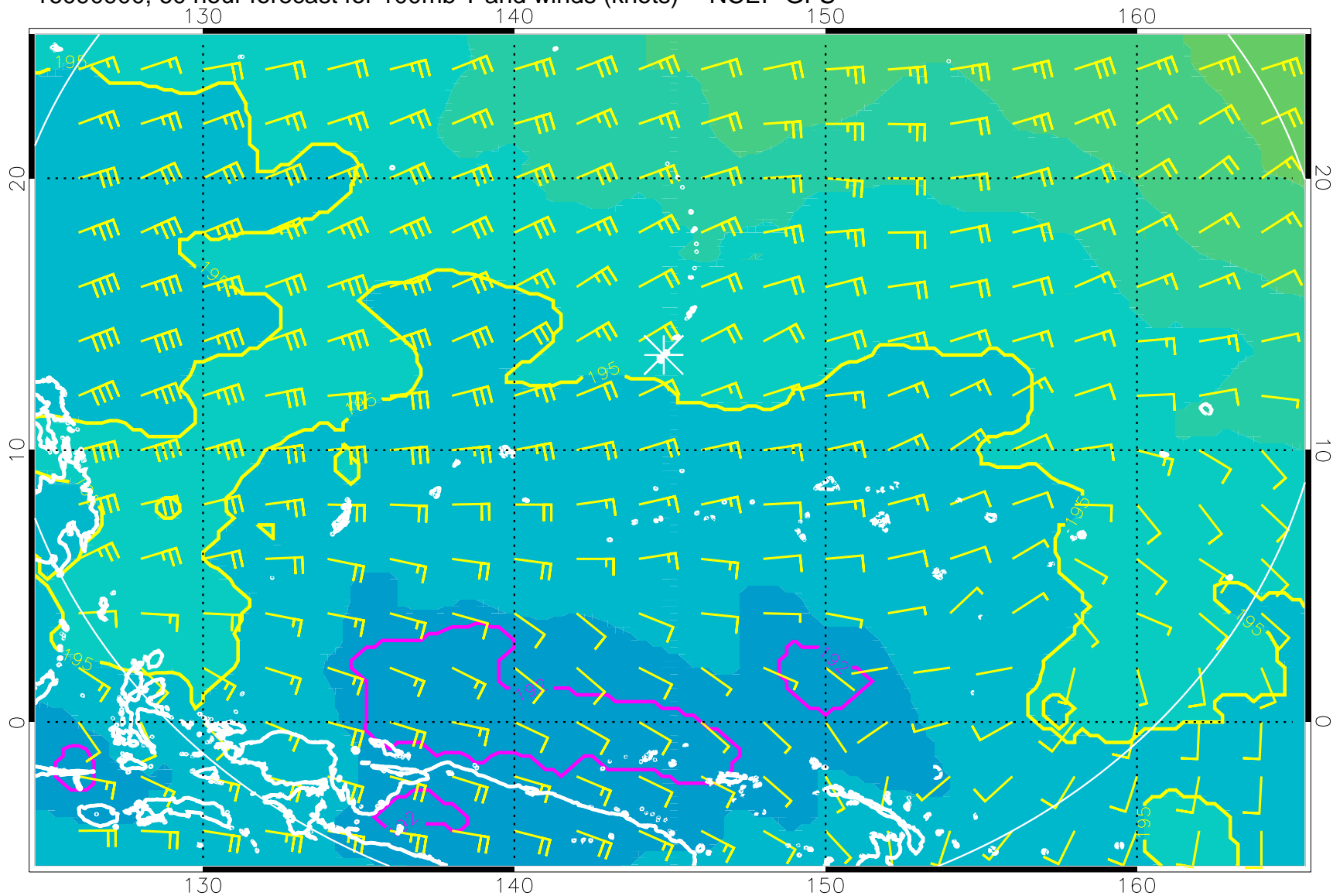
16090900, 60 hour forecast for 100mb T and winds (knots) -- NCEP GFS
