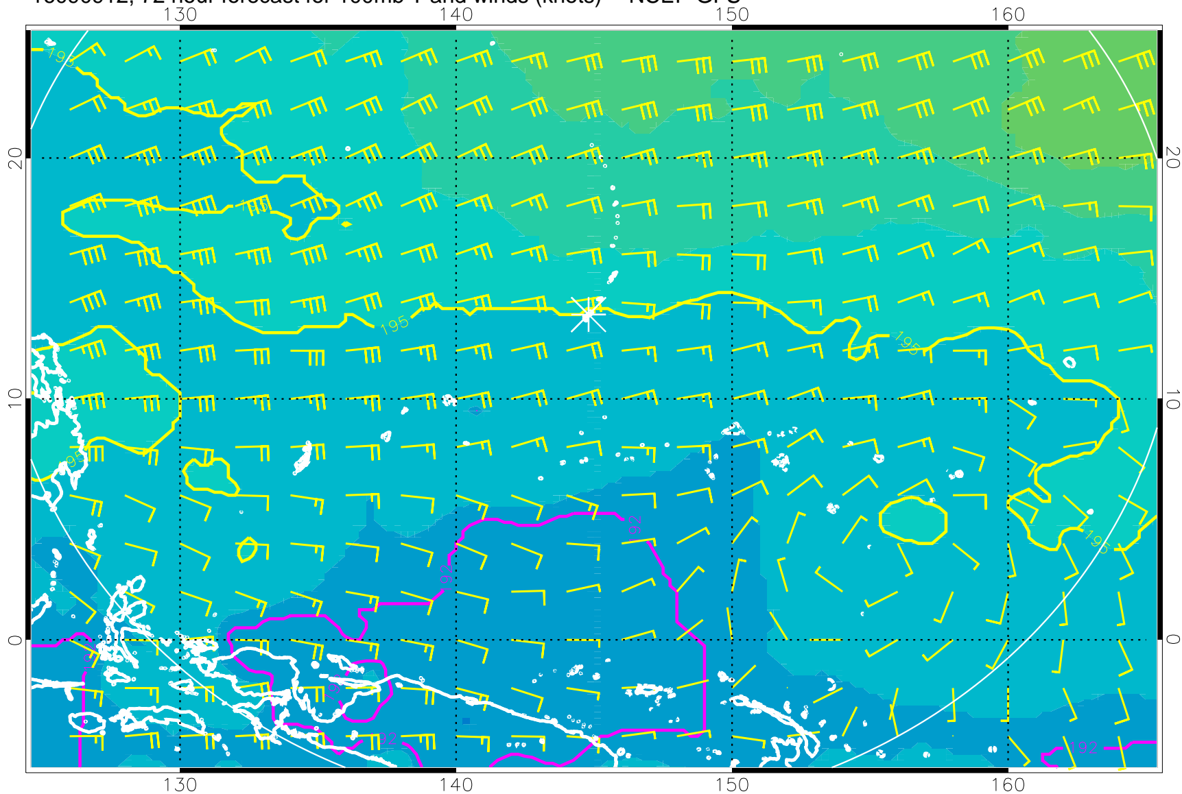
16090912, 72 hour forecast for 100mb T and winds (knots) -- NCEP GFS
