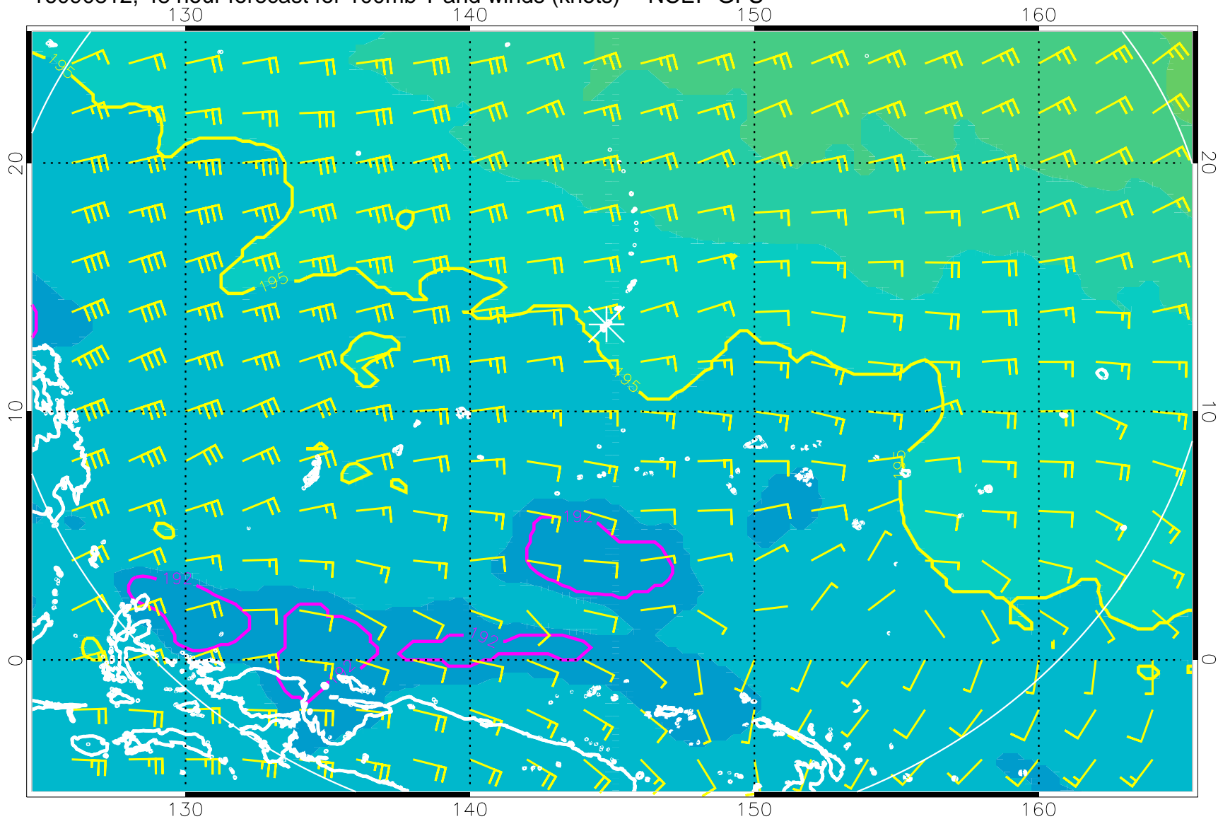
16090812, 48 hour forecast for 100mb T and winds (knots) -- NCEP GFS
