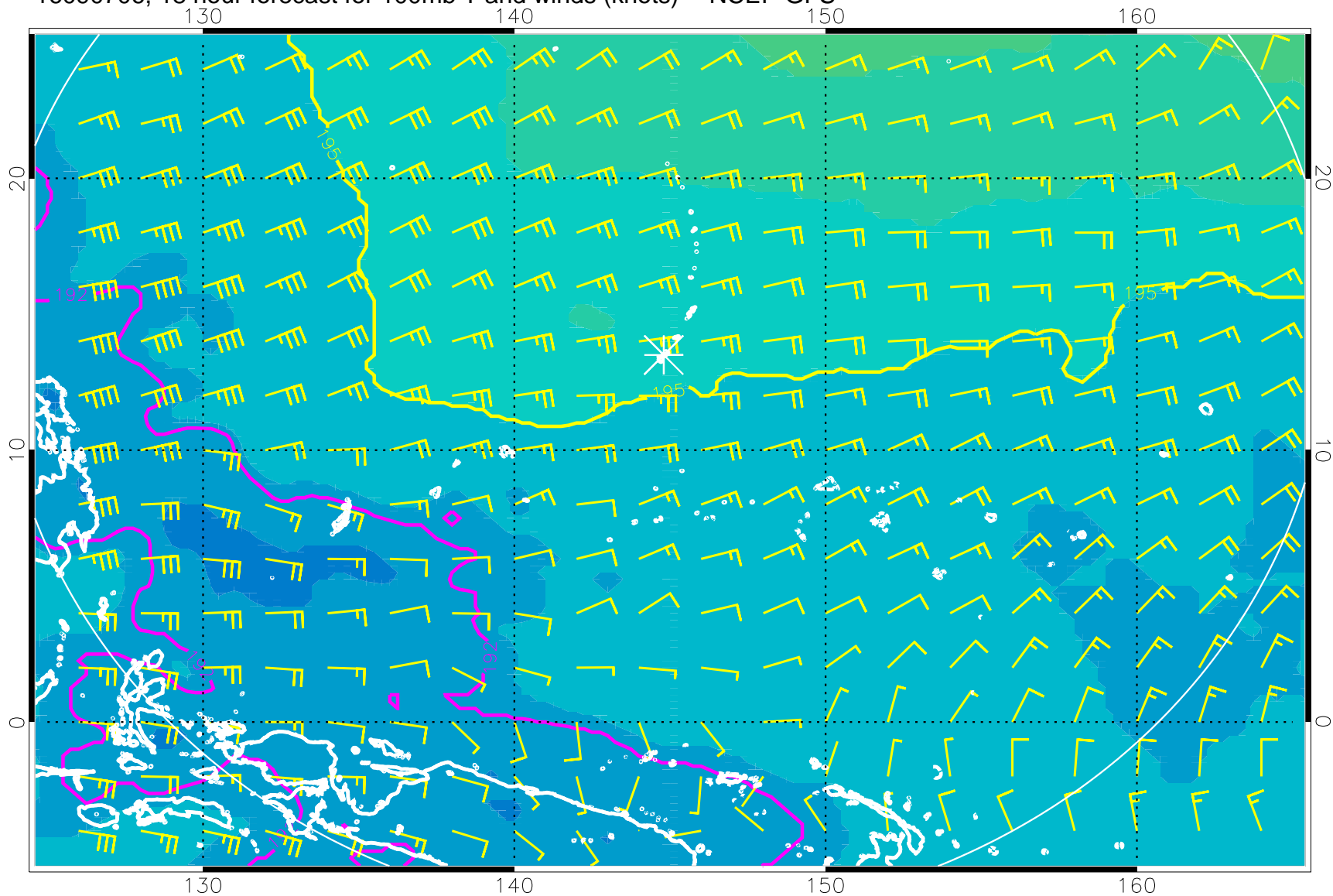
16090706, 18 hour forecast for 100mb T and winds (knots) -- NCEP GFS
