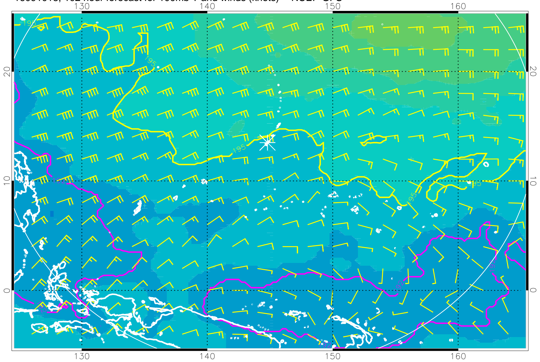
16091018, 102 hour forecast for 100mb T and winds (knots) -- NCEP GFS
