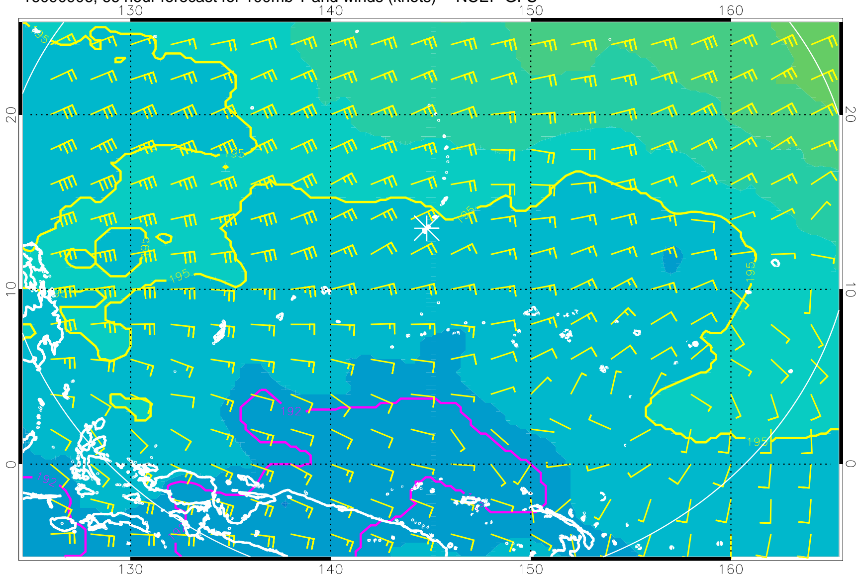
16090906, 66 hour forecast for 100mb T and winds (knots) -- NCEP GFS
