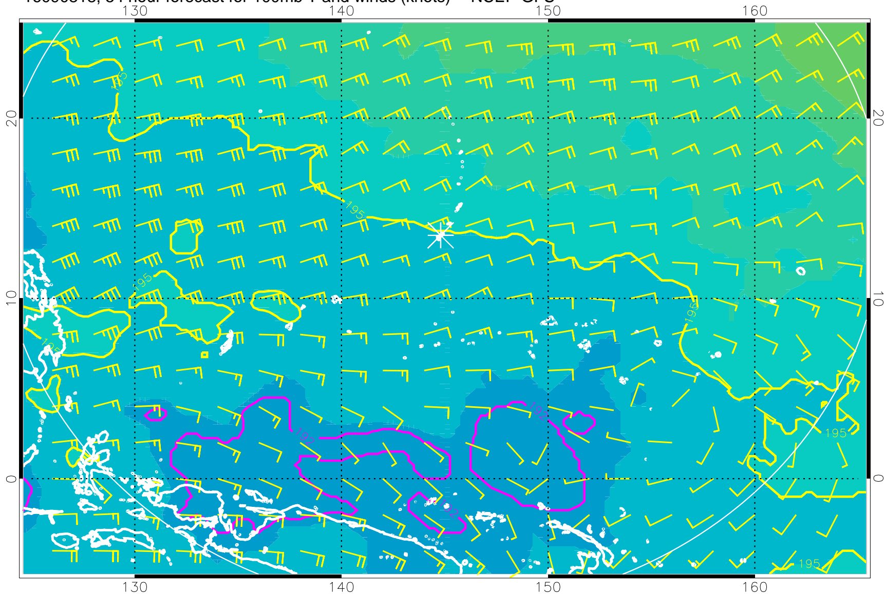
16090818, 54 hour forecast for 100mb T and winds (knots) -- NCEP GFS
