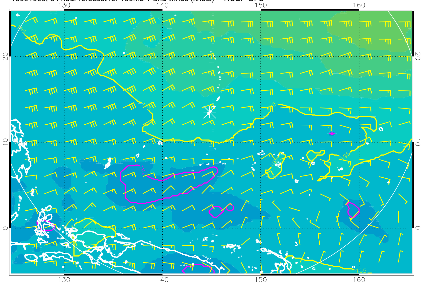
16091000, 84 hour forecast for 100mb T and winds (knots) -- NCEP GFS
