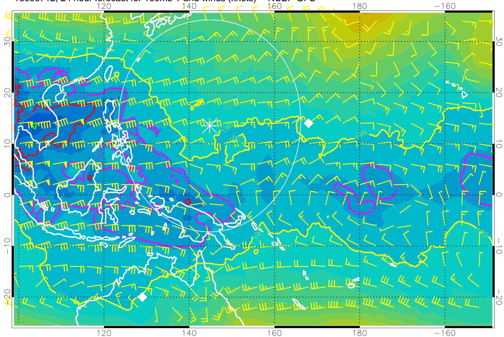
16090712, 24 hour forecast for 100mb T and winds (knots) -- NCEP GFS
