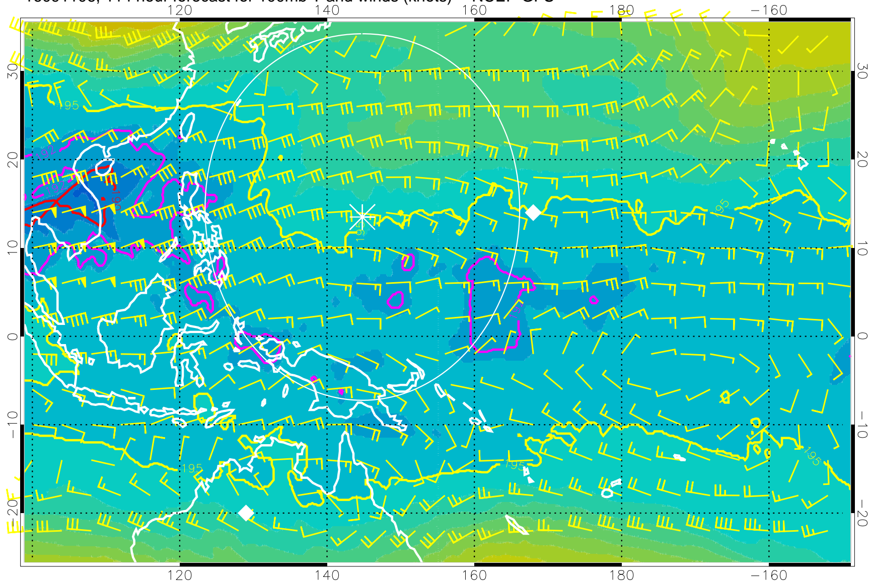
16091106, 114 hour forecast for 100mb T and winds (knots) -- NCEP GFS
