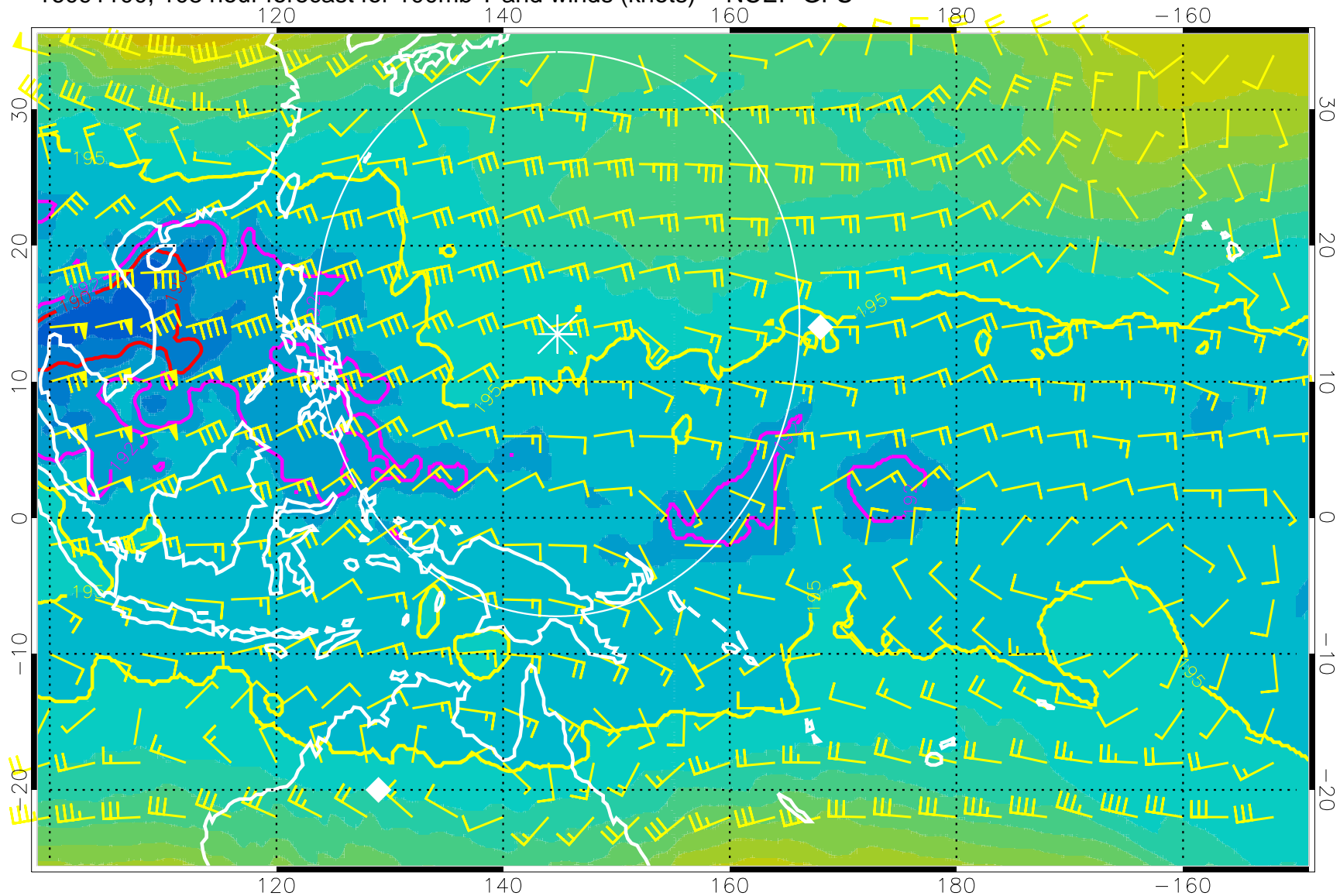
16091100, 108 hour forecast for 100mb T and winds (knots) -- NCEP GFS
