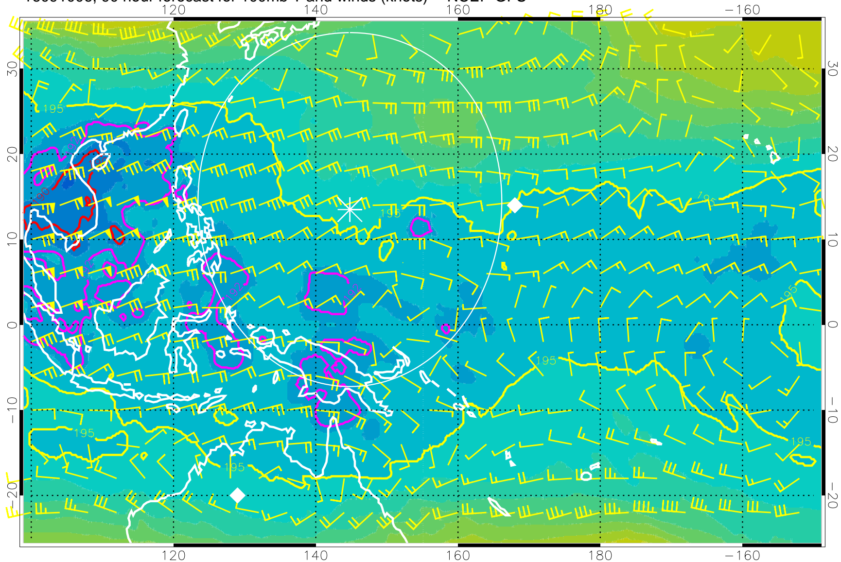
16091006, 90 hour forecast for 100mb T and winds (knots) -- NCEP GFS
