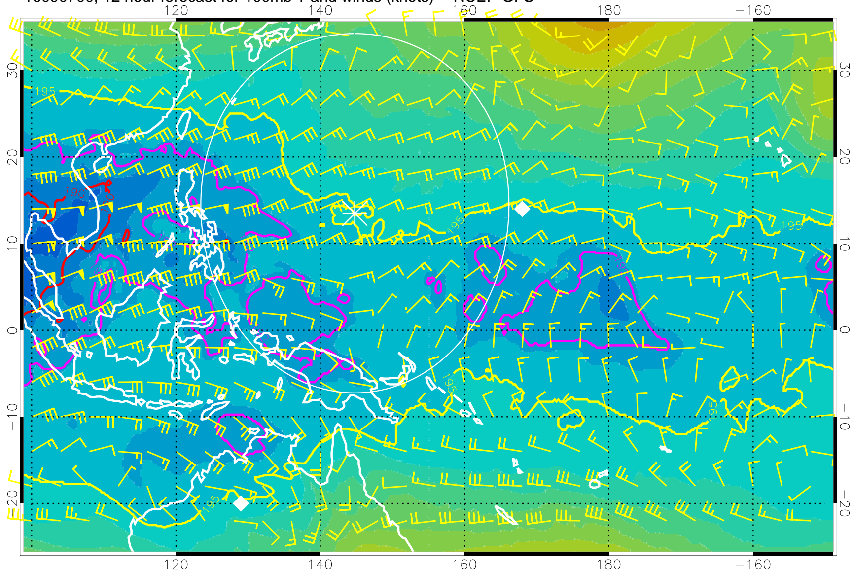
16090700, 12 hour forecast for 100mb T and winds (knots) -- NCEP GFS
