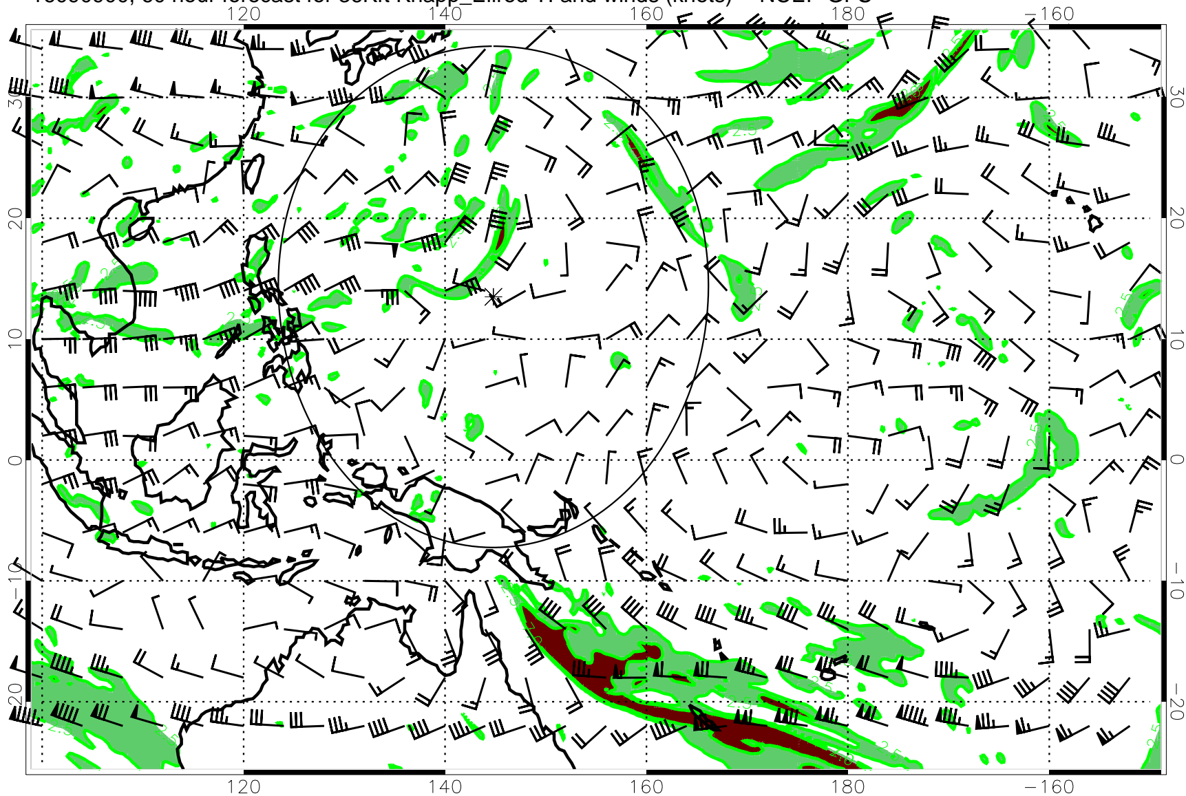
16090900, 60 hour forecast for 36Kft Knapp_Ellrod TI and winds (knots) -- NCEP GFS
