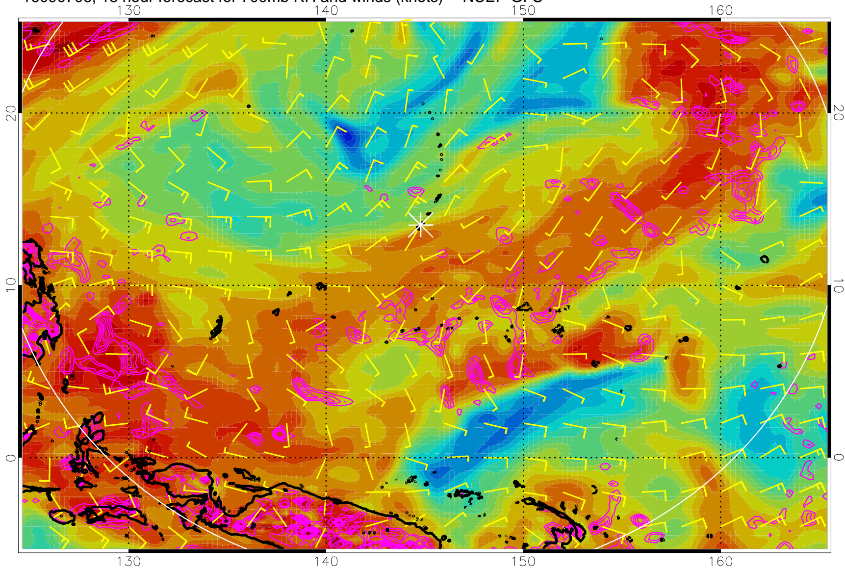
16090706, 18 hour forecast for 700mb RH and winds (knots) -- NCEP GFS
