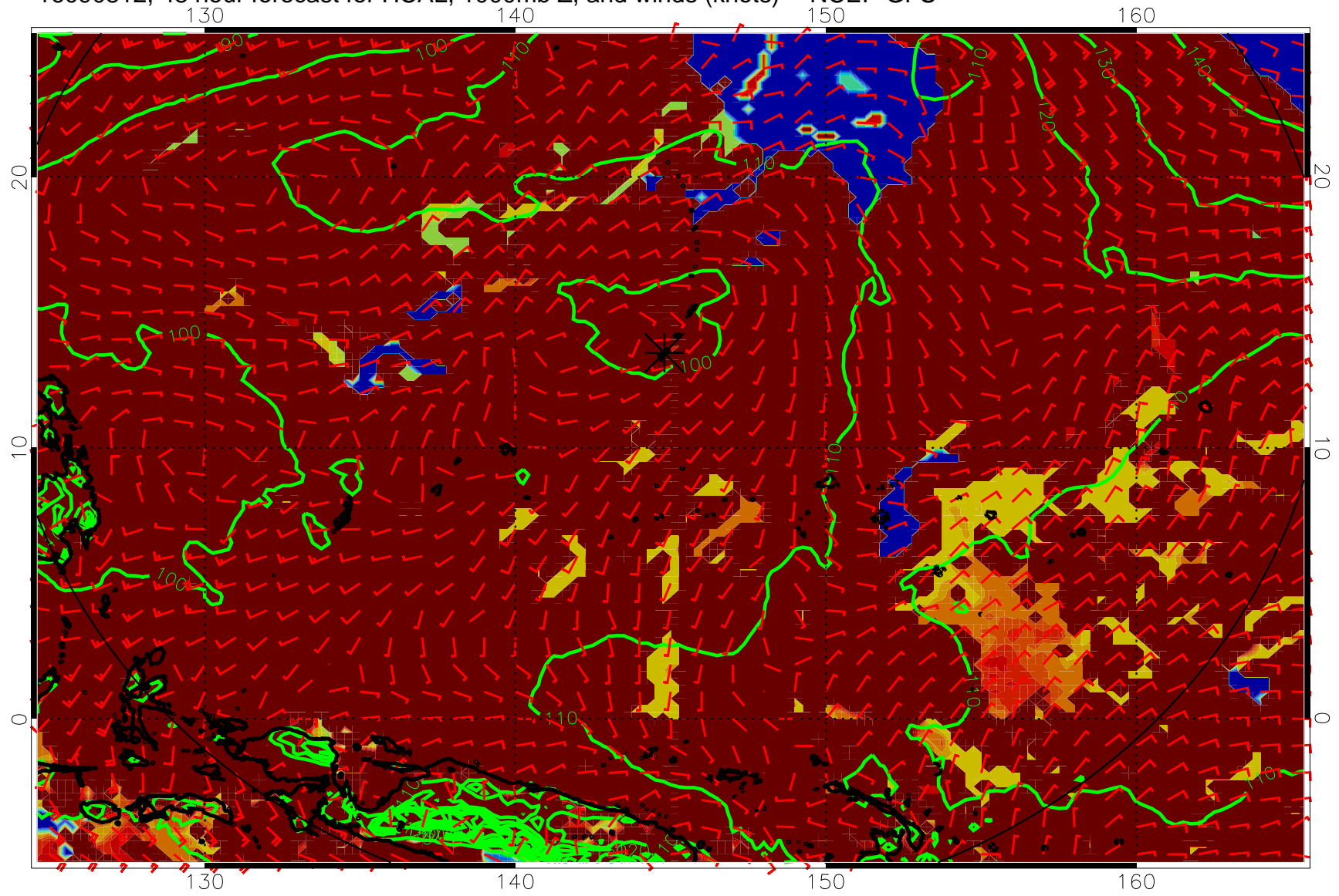
16090812, 48 hour forecast for HCAL, 1000mb Z, and winds (knots) -- NCEP GFS
