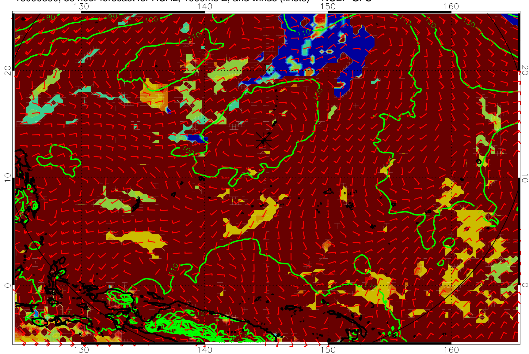
16090800, 36 hour forecast for HCAL, 1000mb Z, and winds (knots) -- NCEP GFS
