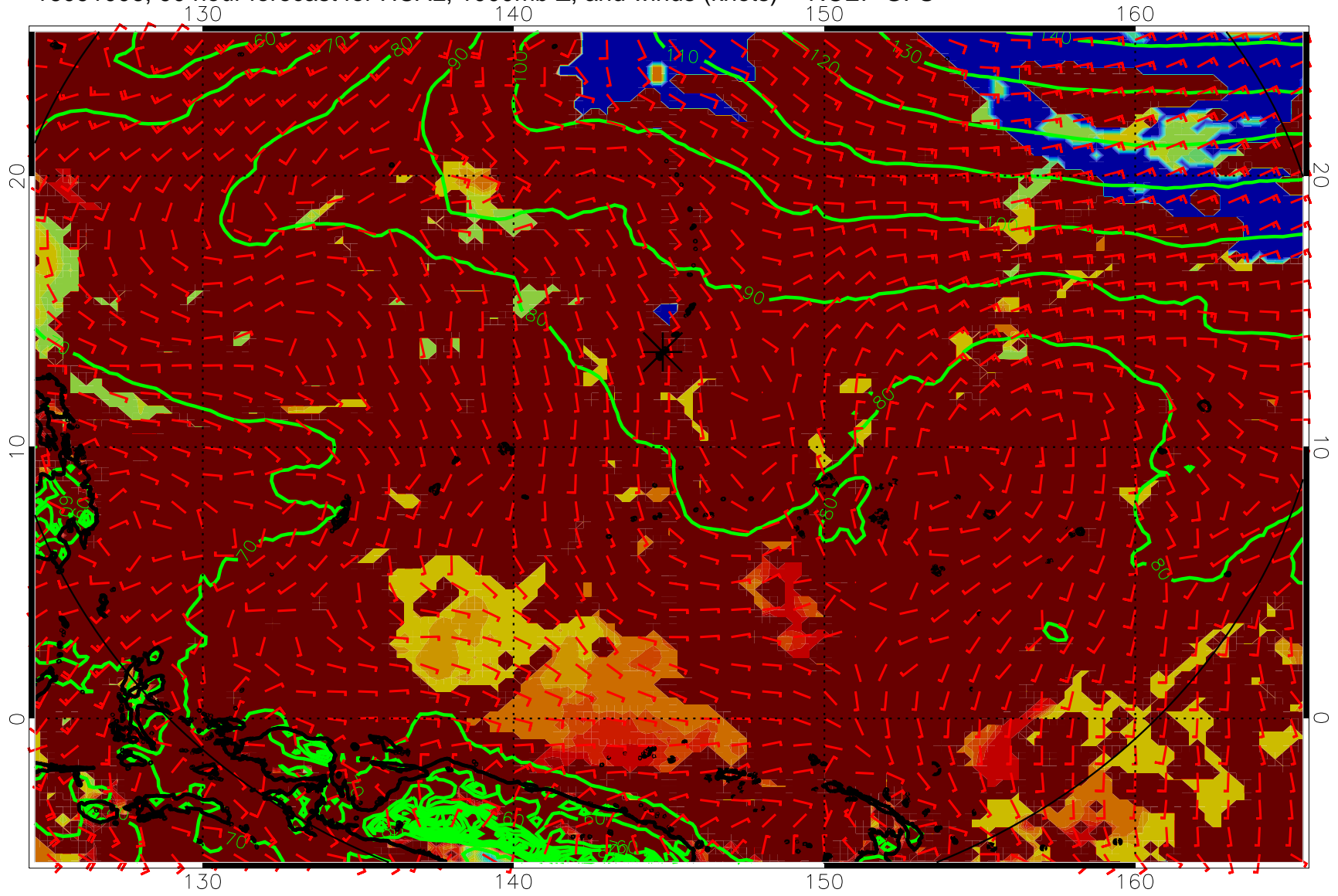
16091006, 90 hour forecast for HCAL, 1000mb Z, and winds (knots) -- NCEP GFS
