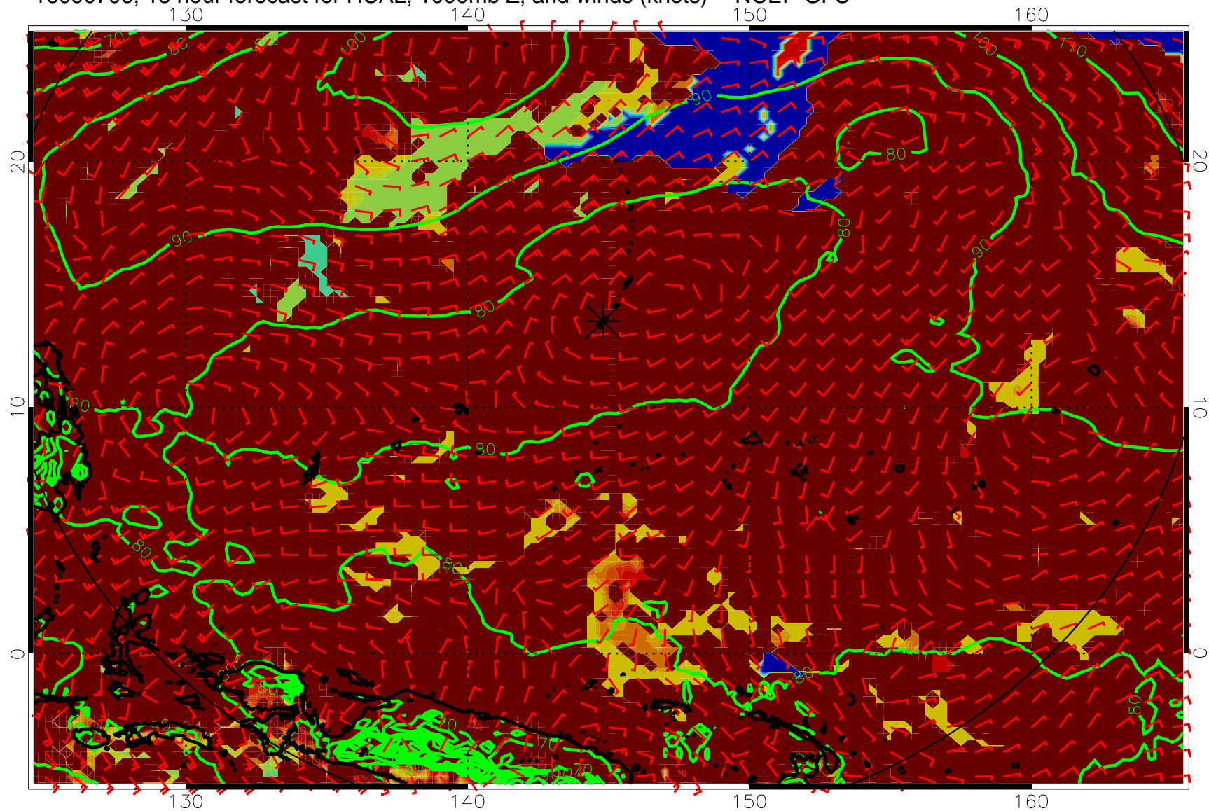
16090706, 18 hour forecast for HCAL, 1000mb Z, and winds (knots) -- NCEP GFS
