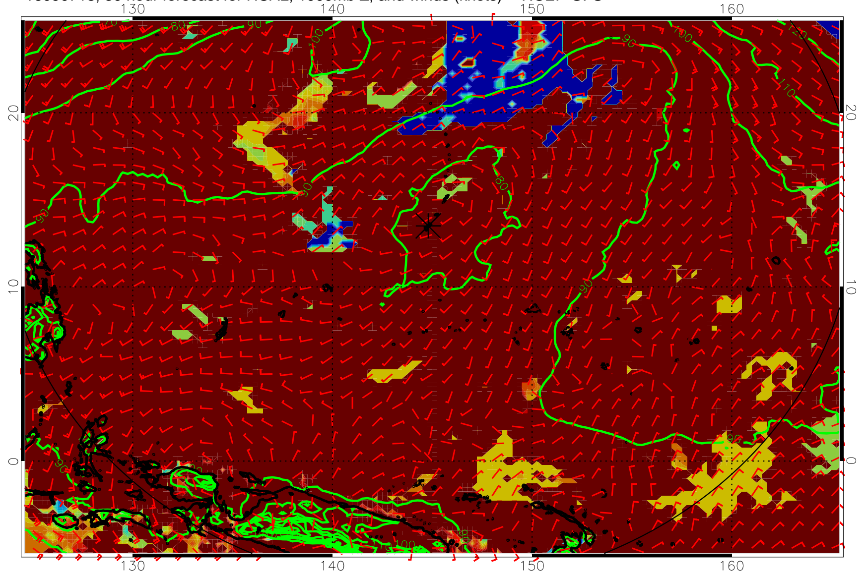
16090718, 30 hour forecast for HCAL, 1000mb Z, and winds (knots) -- NCEP GFS
