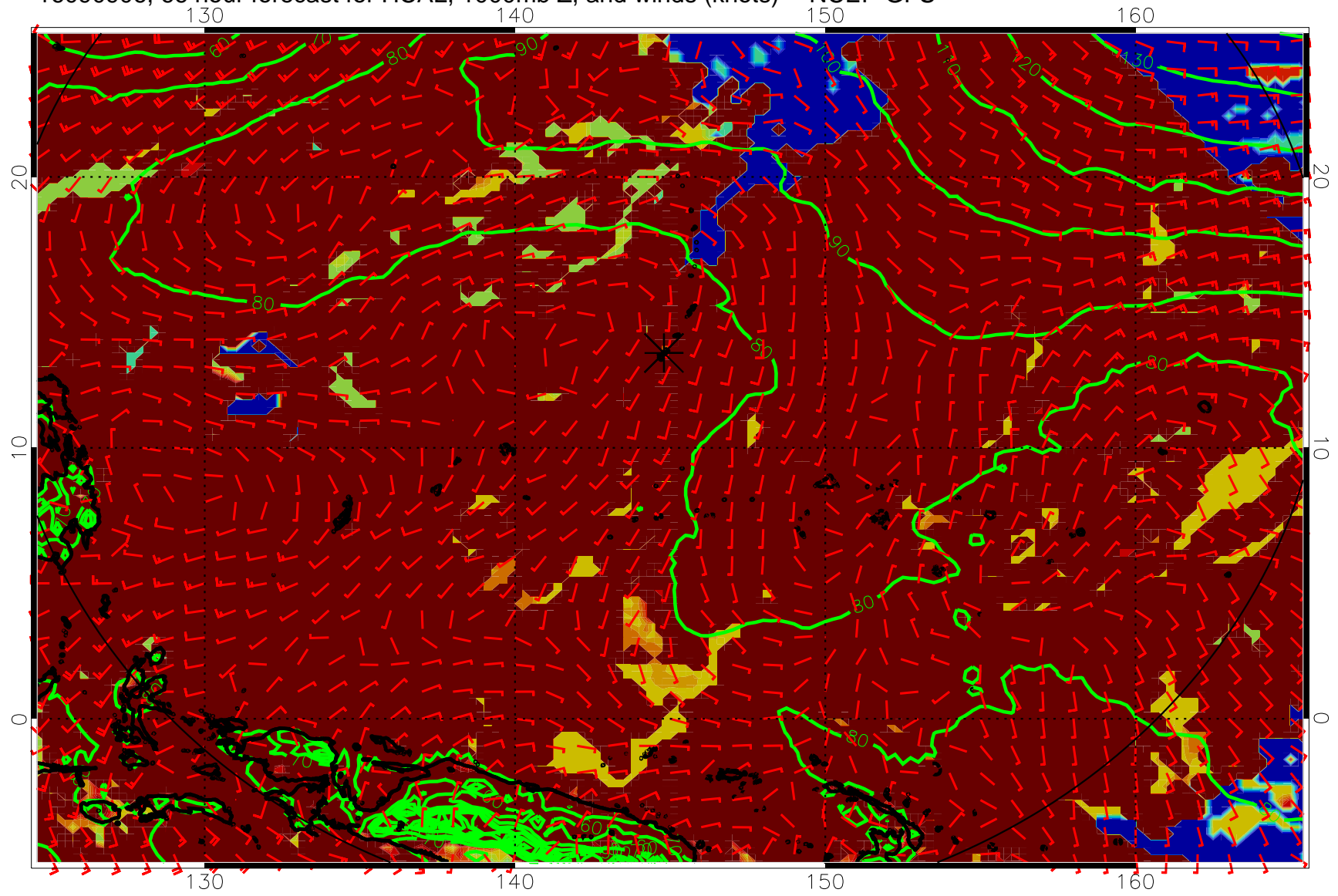
16090906, 66 hour forecast for HCAL, 1000mb Z, and winds (knots) -- NCEP GFS
