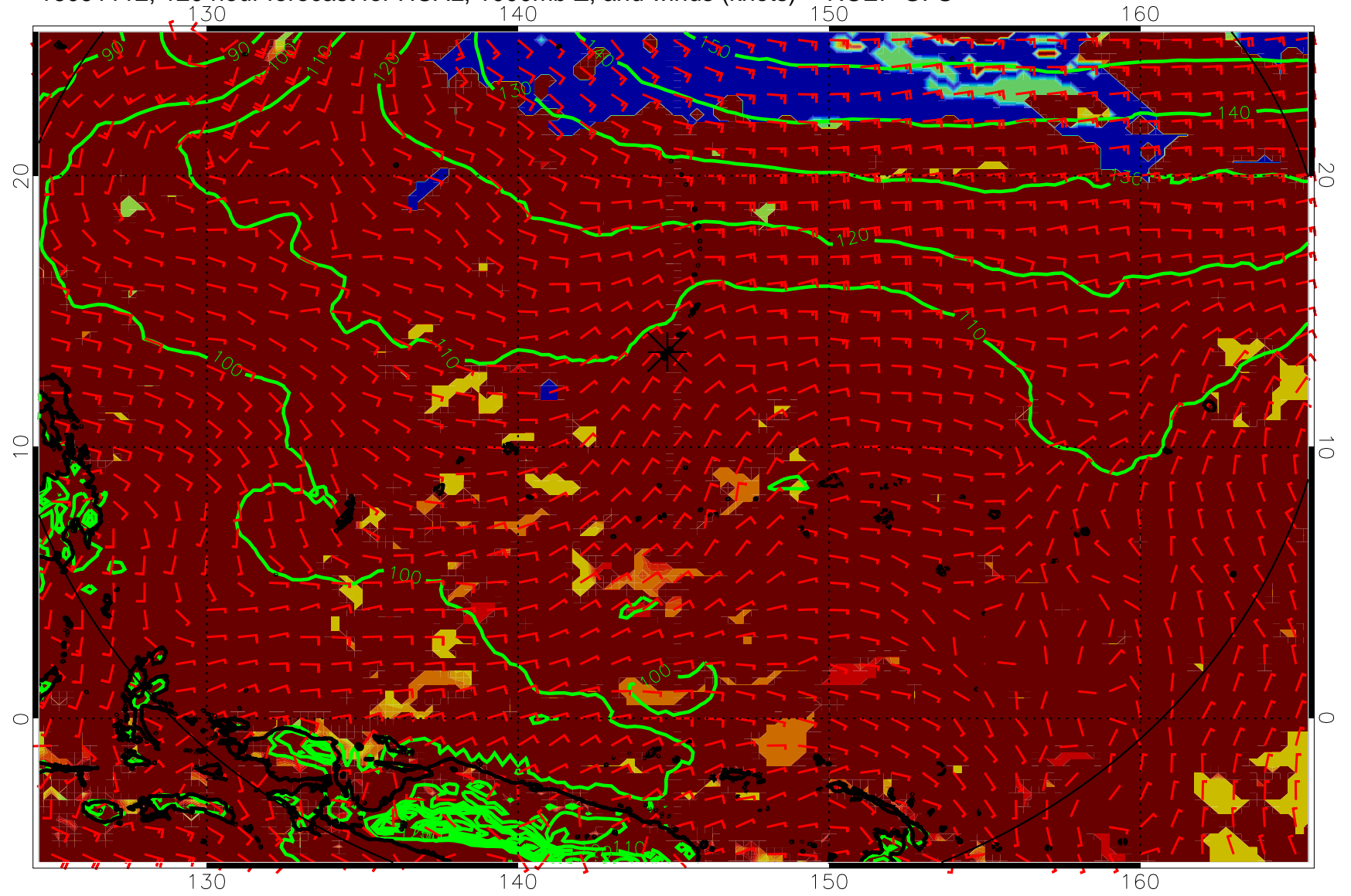
16091112, 120 hour forecast for HCAL, 1000mb Z, and winds (knots) -- NCEP GFS
