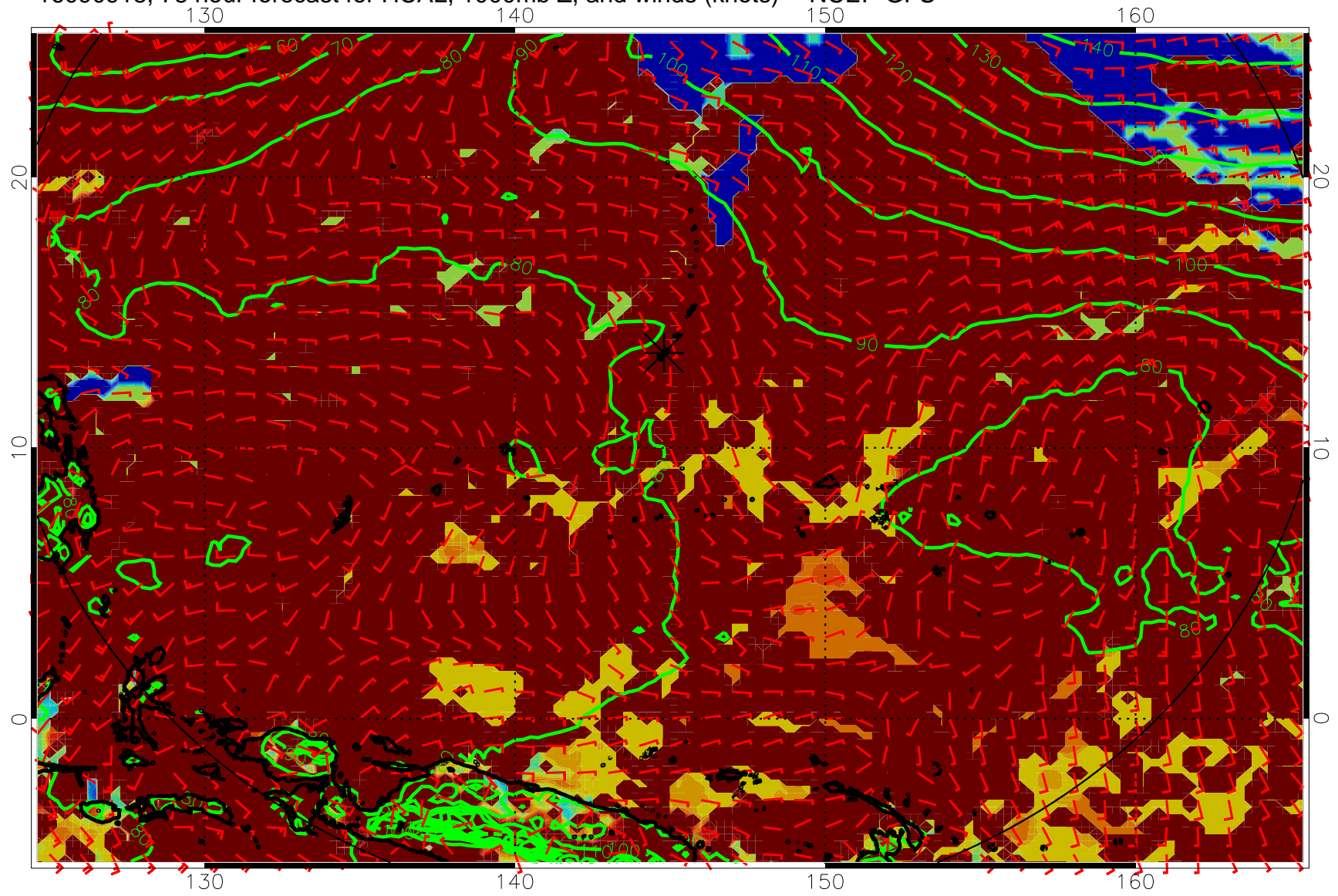
16090918, 78 hour forecast for HCAL, 1000mb Z, and winds (knots) -- NCEP GFS
