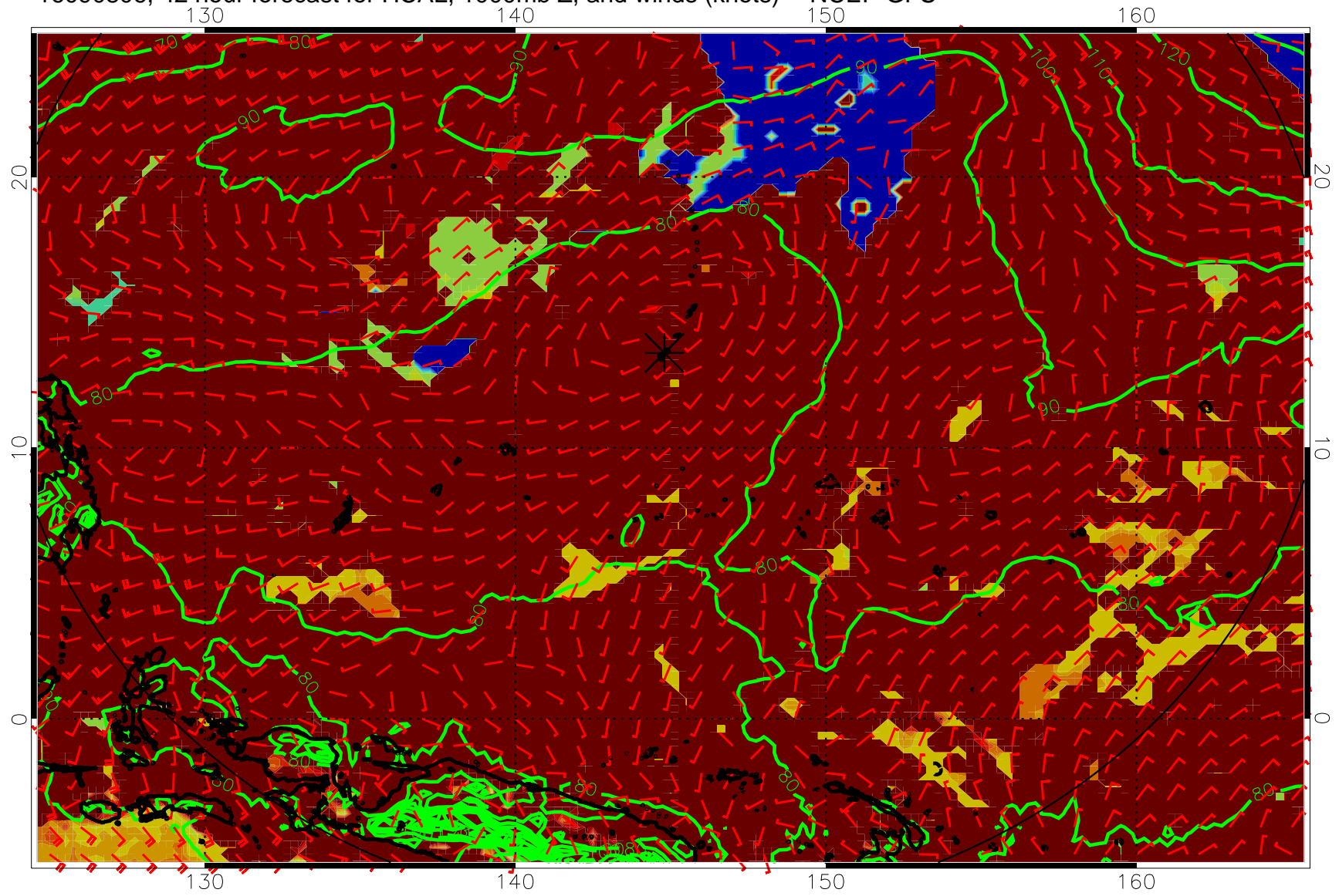
16090806, 42 hour forecast for HCAL, 1000mb Z, and winds (knots) -- NCEP GFS
