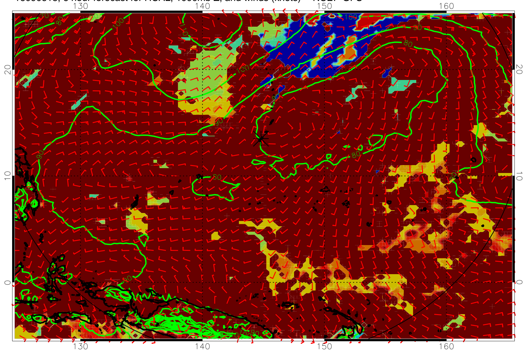
16090618, 6 hour forecast for HCAL, 1000mb Z, and winds (knots) -- NCEP GFS
