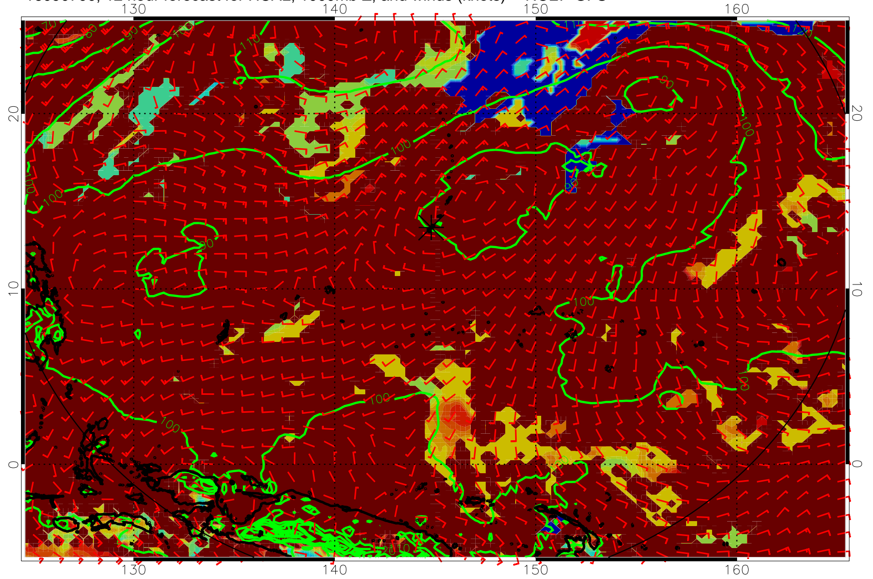
16090700, 12 hour forecast for HCAL, 1000mb Z, and winds (knots) -- NCEP GFS
