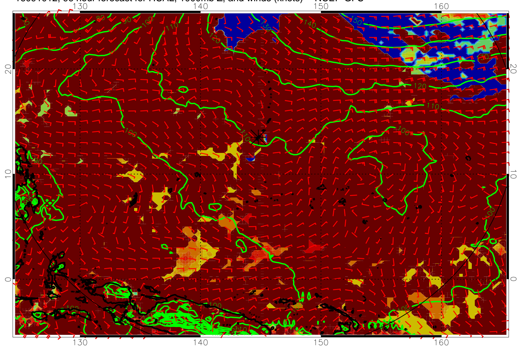
16091012, 96 hour forecast for HCAL, 1000mb Z, and winds (knots) -- NCEP GFS
