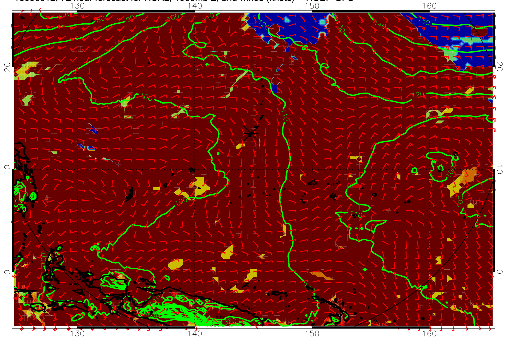
16090912, 72 hour forecast for HCAL, 1000mb Z, and winds (knots) -- NCEP GFS
