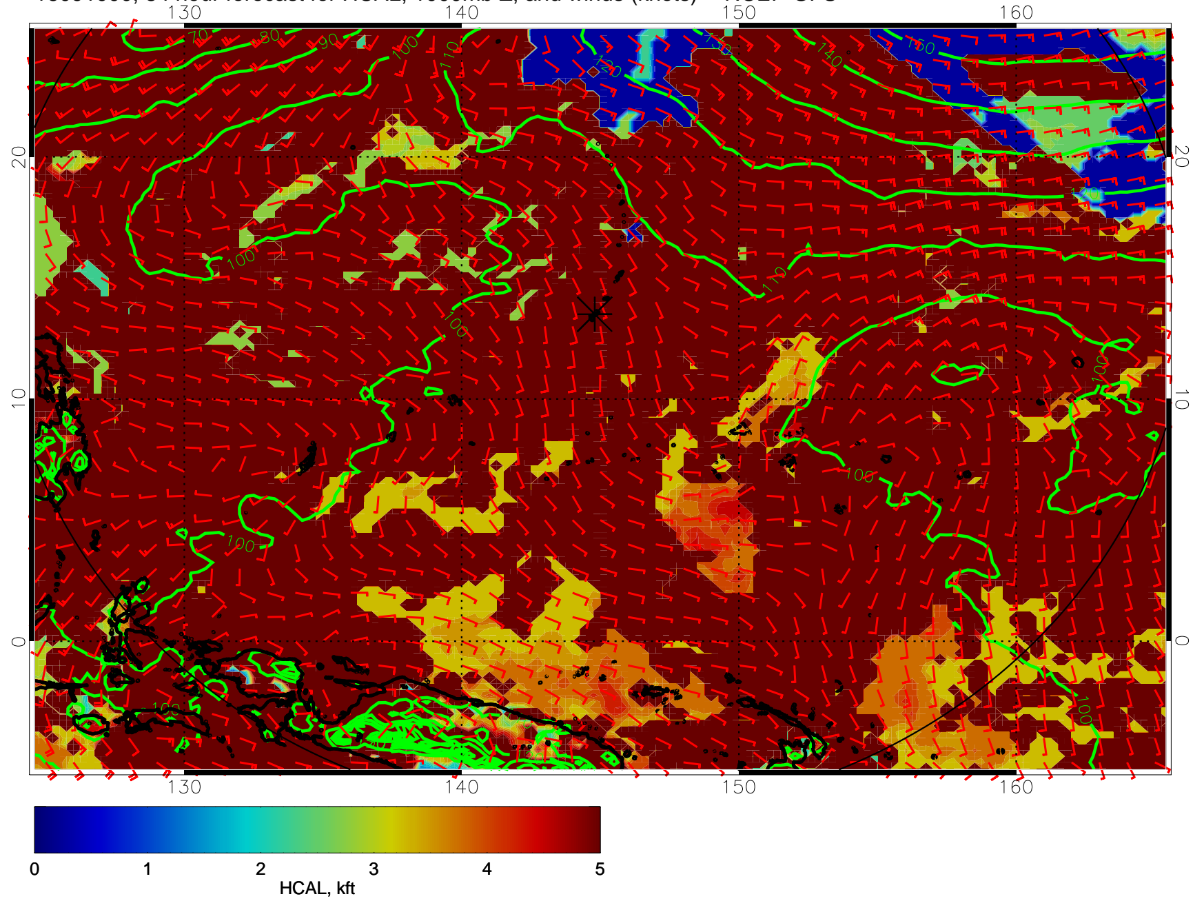
16091000, 84 hour forecast for HCAL, 1000mb Z, and winds (knots) -- NCEP GFS
