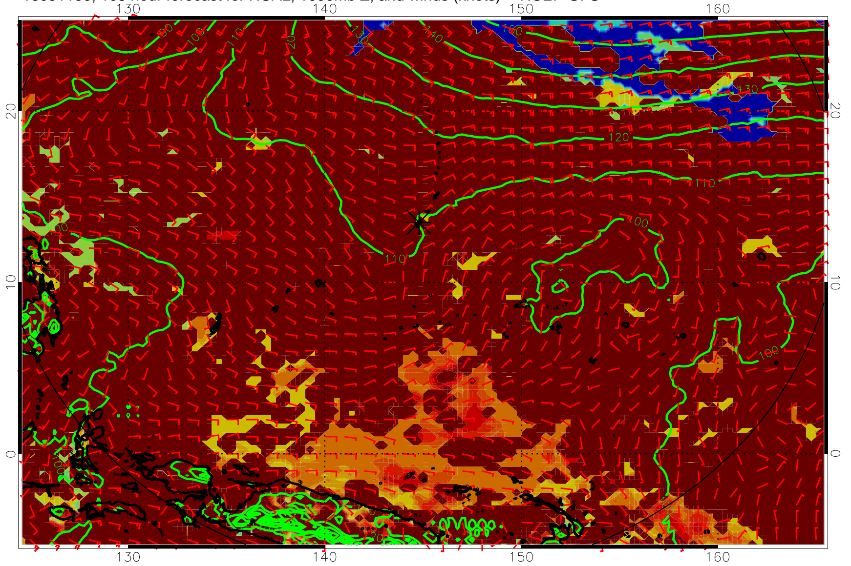
16091100, 108 hour forecast for HCAL, 1000mb Z, and winds (knots) -- NCEP GFS
