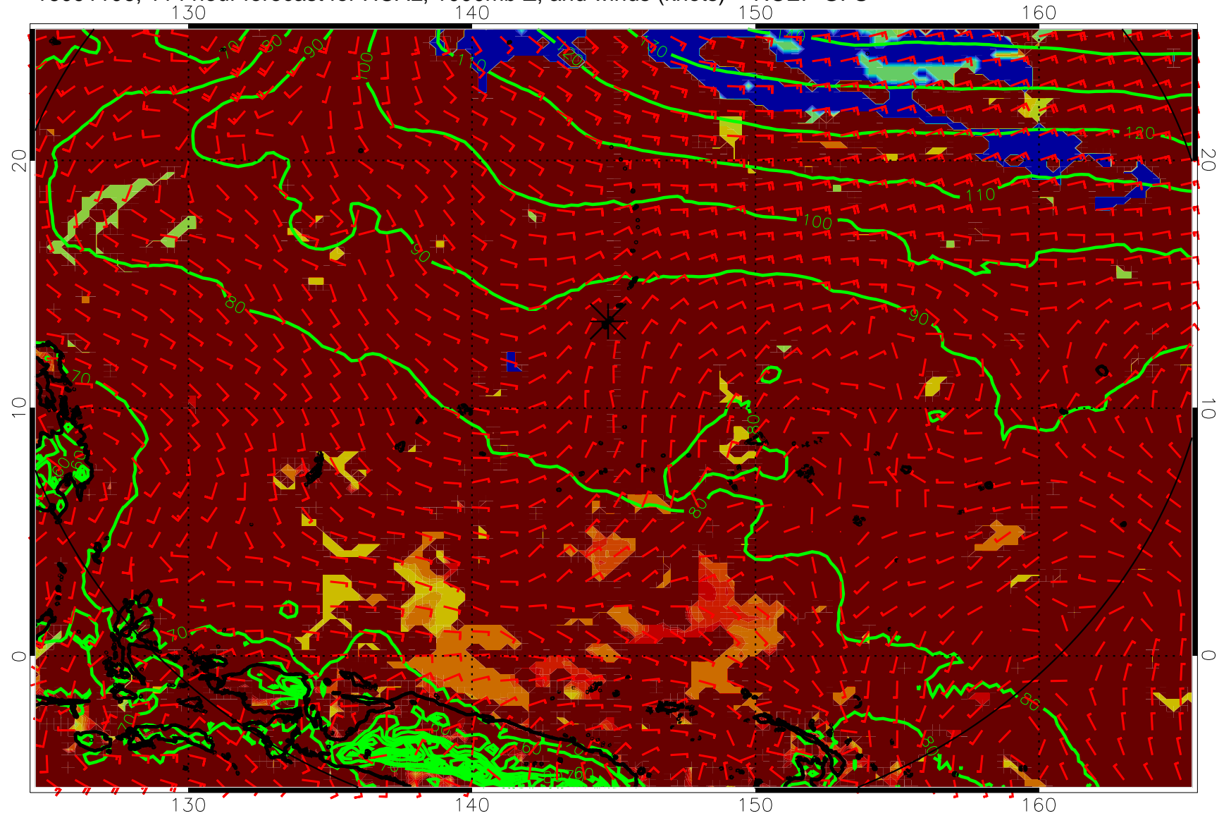
16091106, 114 hour forecast for HCAL, 1000mb Z, and winds (knots) -- NCEP GFS
