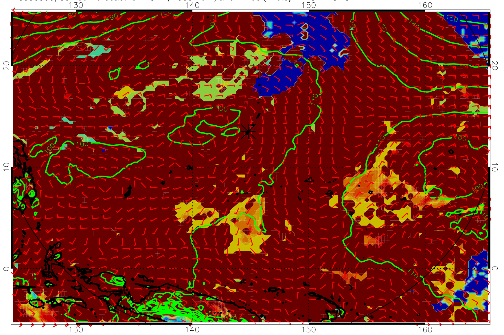
16090900, 60 hour forecast for HCAL, 1000mb Z, and winds (knots) -- NCEP GFS
