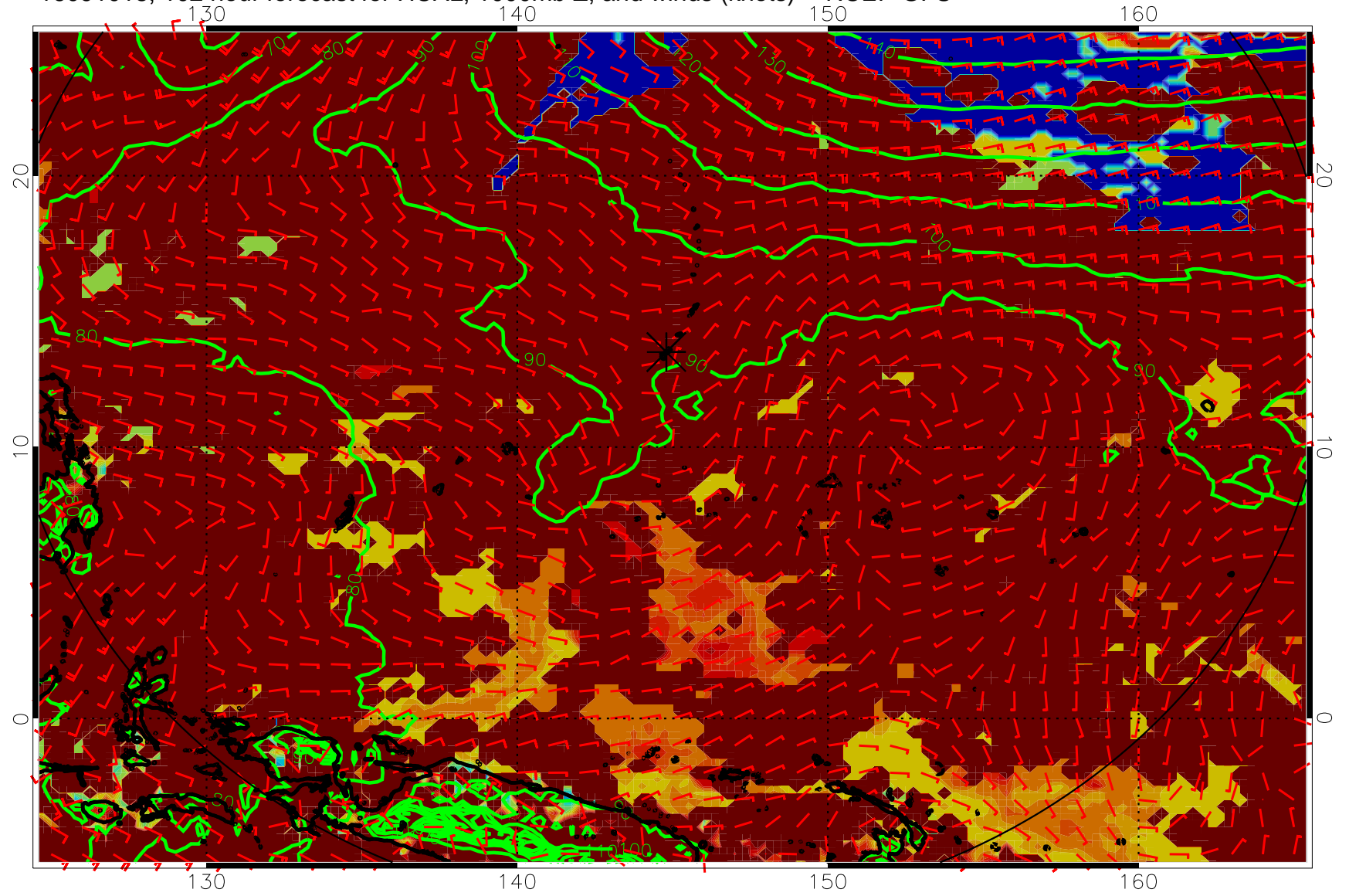
16091018, 102 hour forecast for HCAL, 1000mb Z, and winds (knots) -- NCEP GFS
