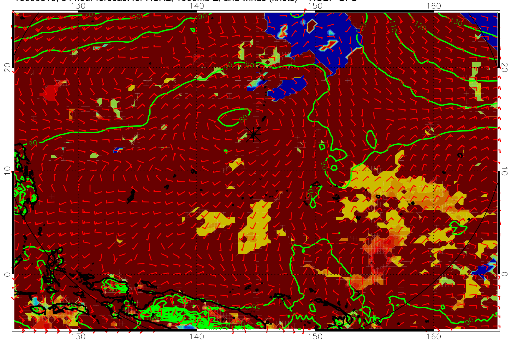
16090818, 54 hour forecast for HCAL, 1000mb Z, and winds (knots) -- NCEP GFS
