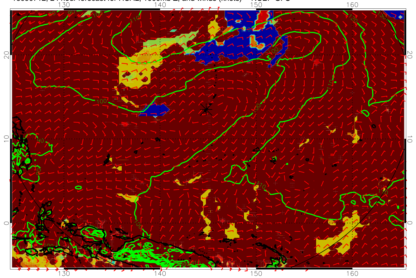
16090712, 24 hour forecast for HCAL, 1000mb Z, and winds (knots) -- NCEP GFS
