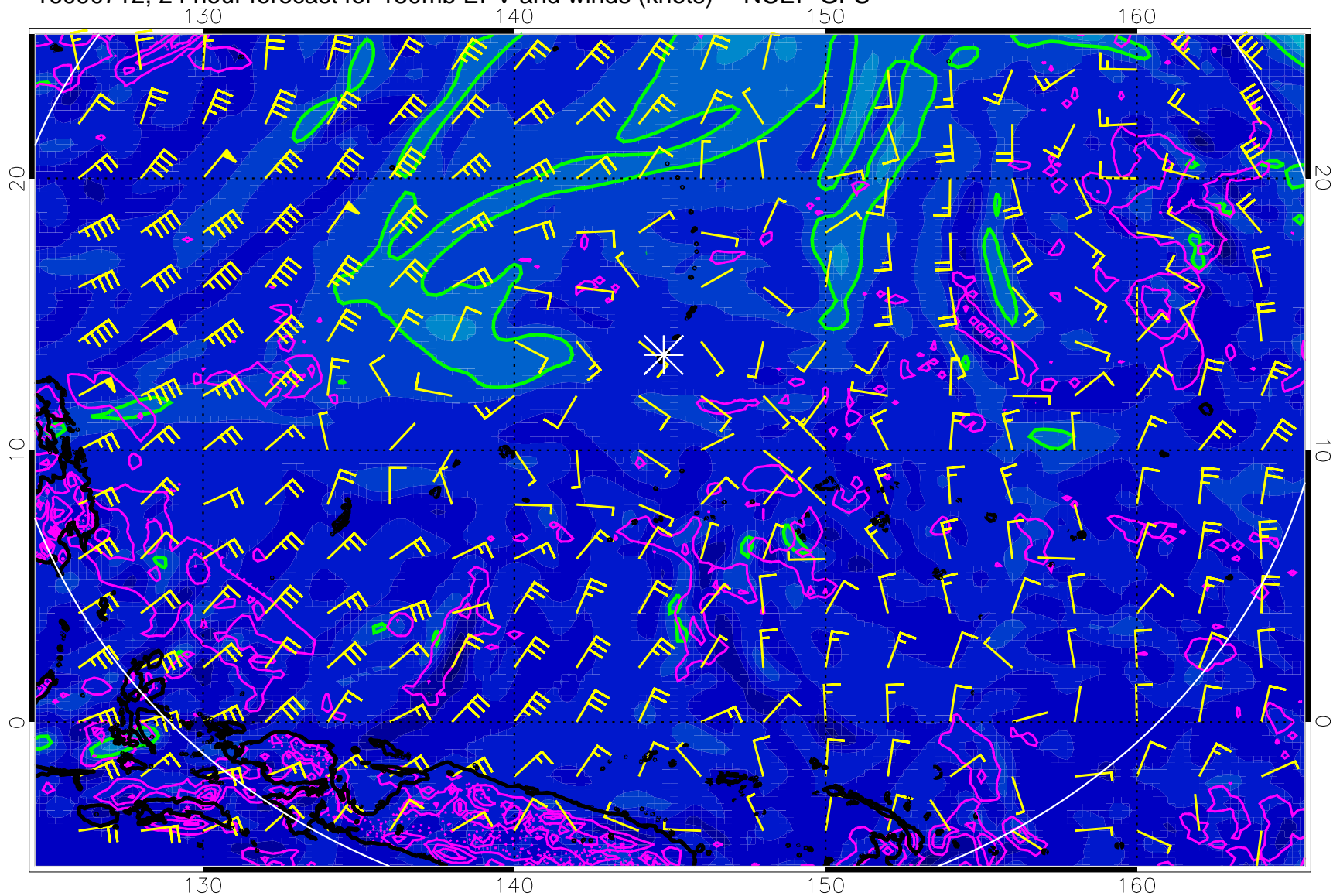
16090712, 24 hour forecast for 150mb EPV and winds (knots) -- NCEP GFS
