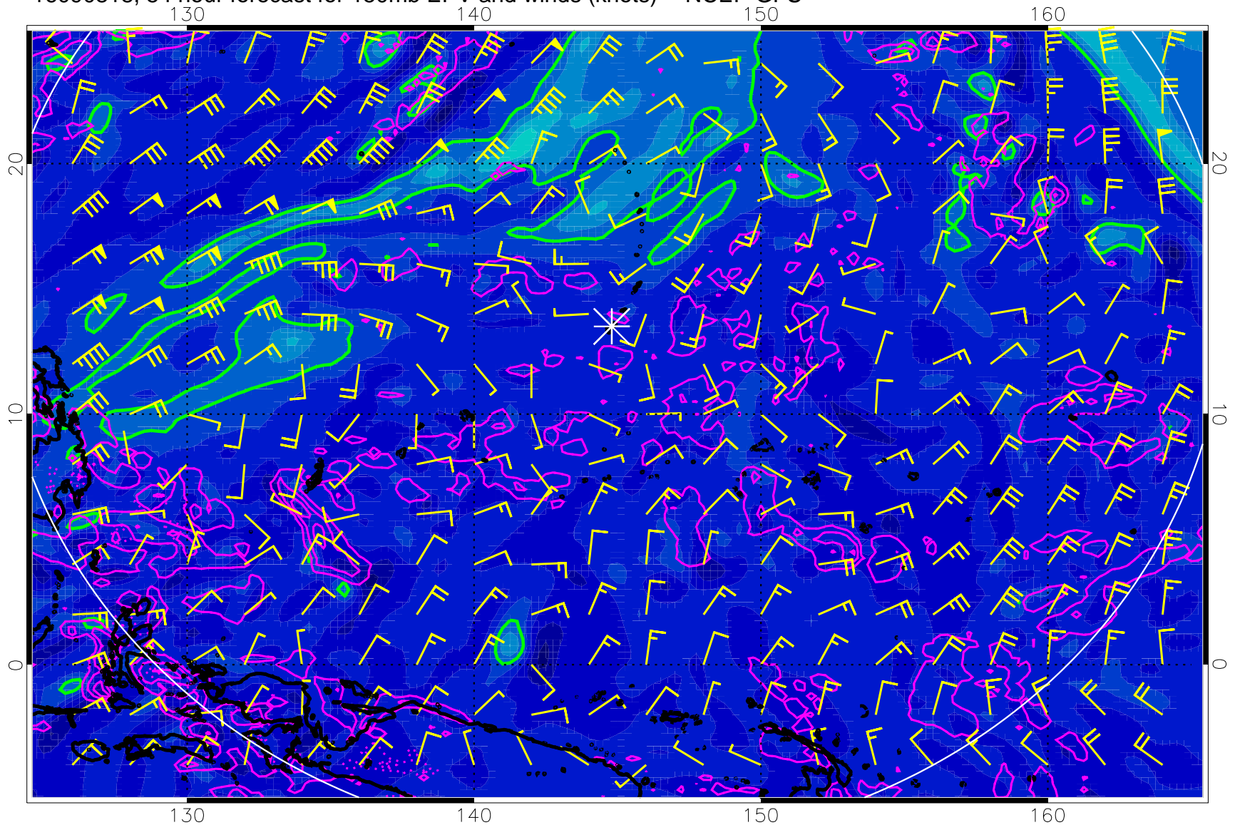
16090818, 54 hour forecast for 150mb EPV and winds (knots) -- NCEP GFS
