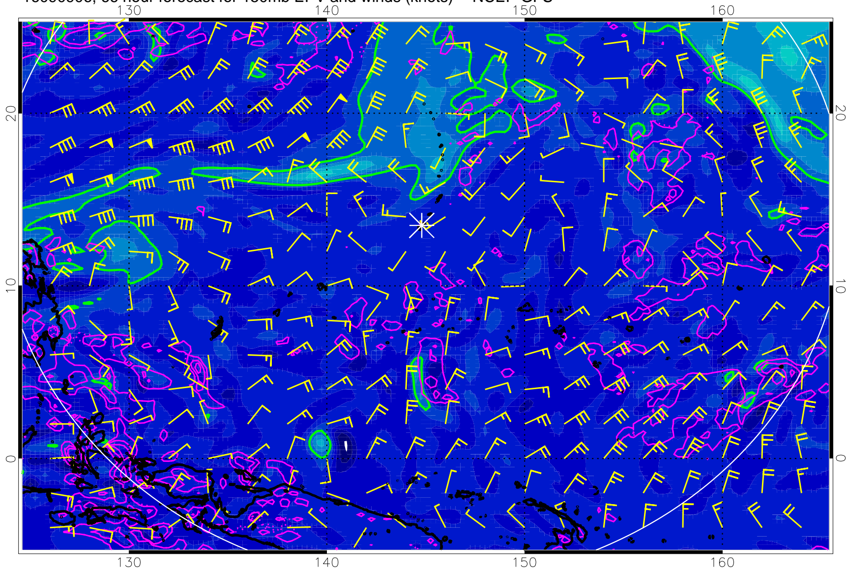
16090906, 66 hour forecast for 150mb EPV and winds (knots) -- NCEP GFS
