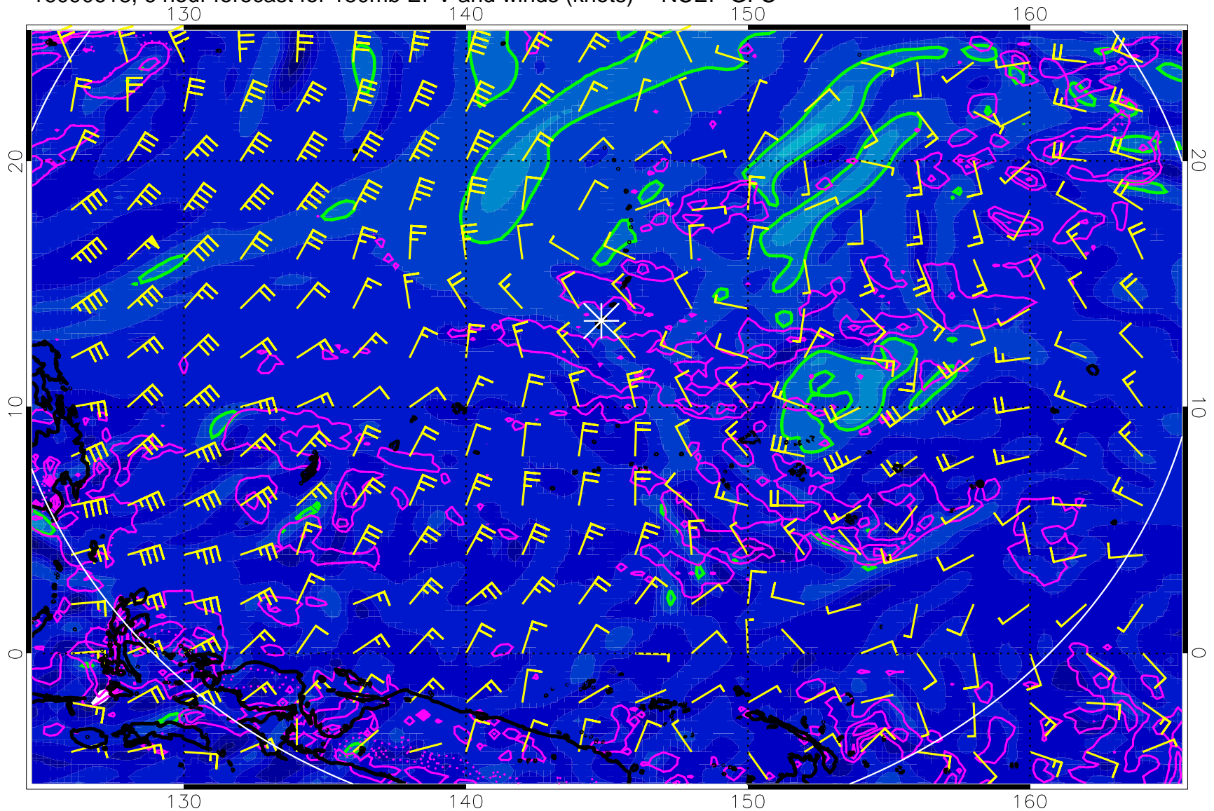
16090618, 6 hour forecast for 150mb EPV and winds (knots) -- NCEP GFS
