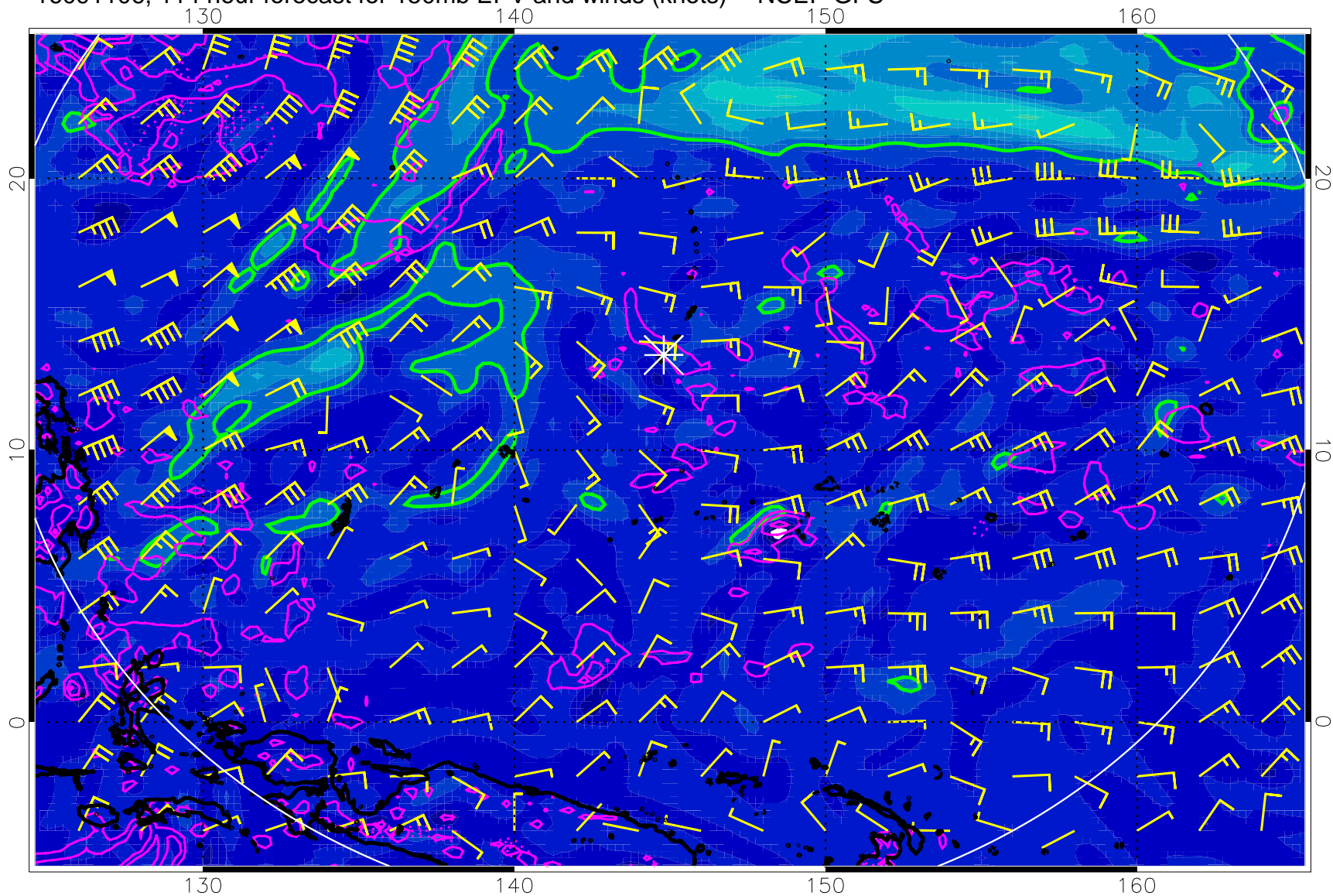
16091106, 114 hour forecast for 150mb EPV and winds (knots) -- NCEP GFS
