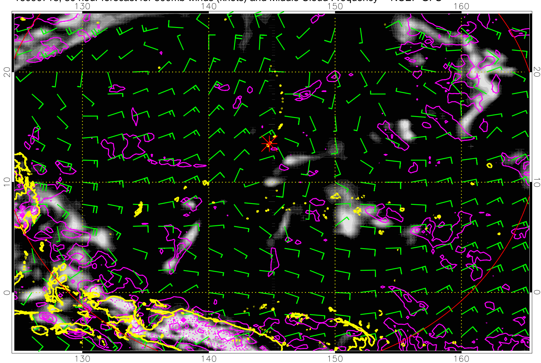
16090718, 30 hour forecast for 500mb winds (knots) and Middle Cloud Frequency -- NCEP GFS
