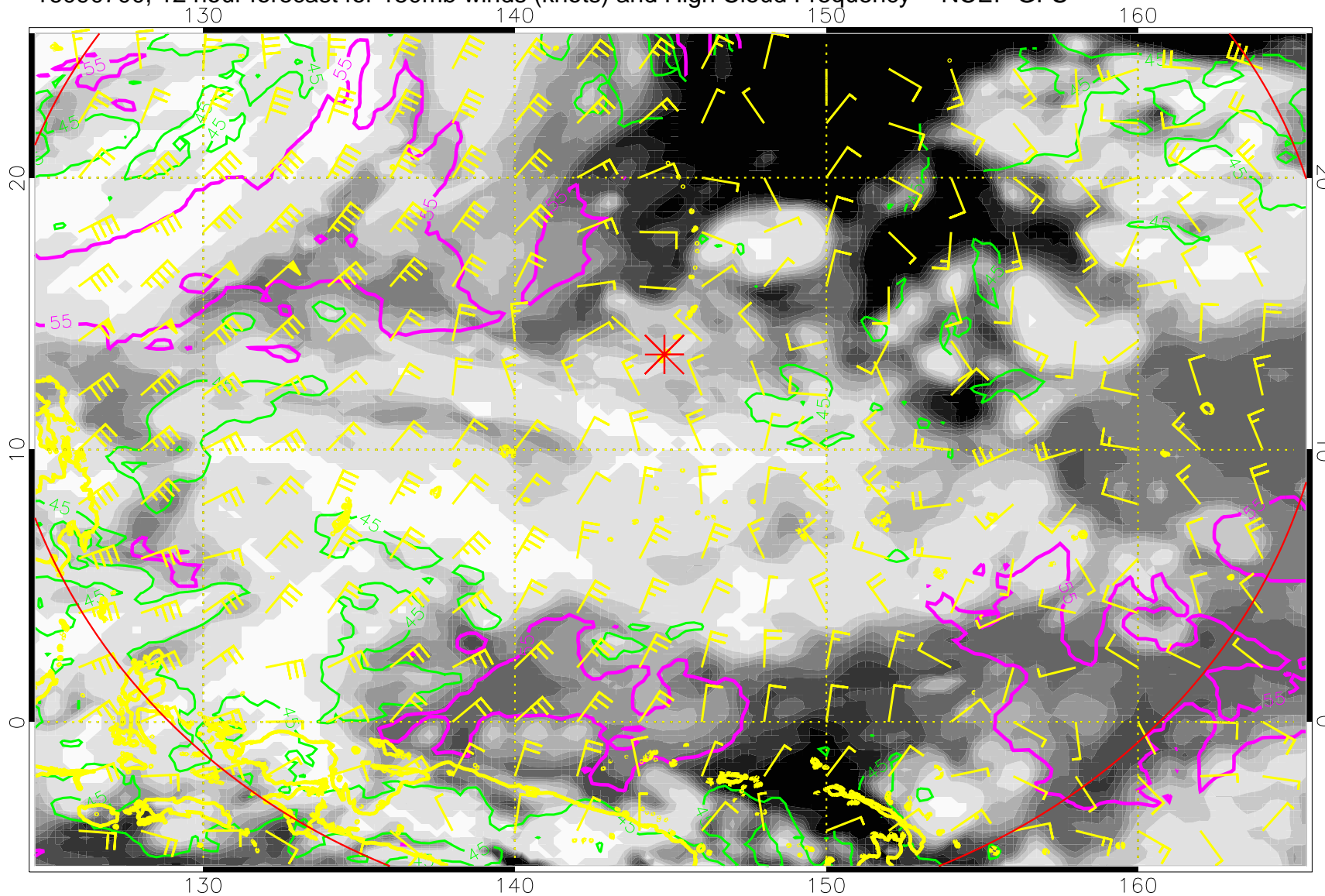
16090700, 12 hour forecast for 150mb winds (knots) and High Cloud Frequency -- NCEP GFS
