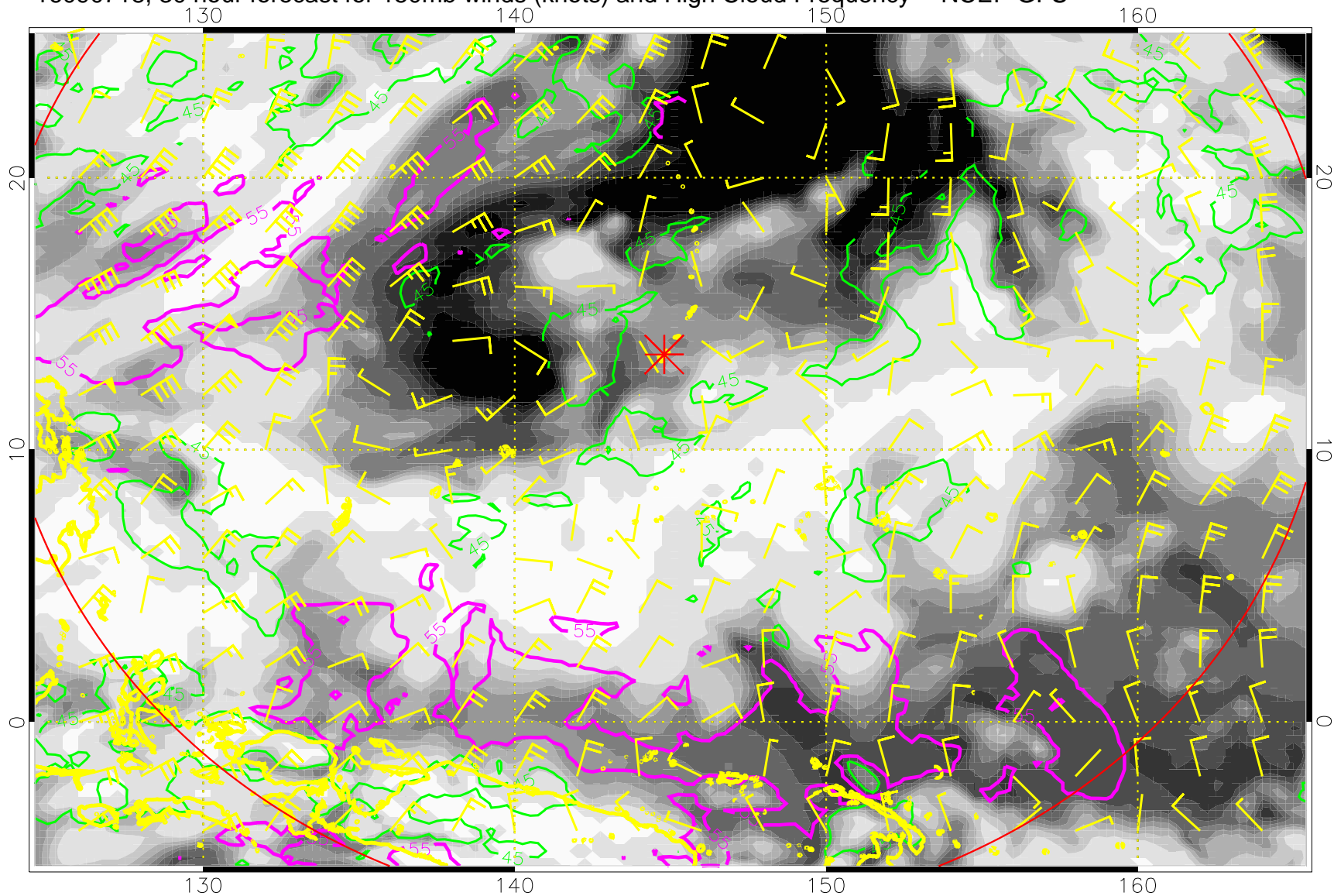
16090718, 30 hour forecast for 150mb winds (knots) and High Cloud Frequency -- NCEP GFS
