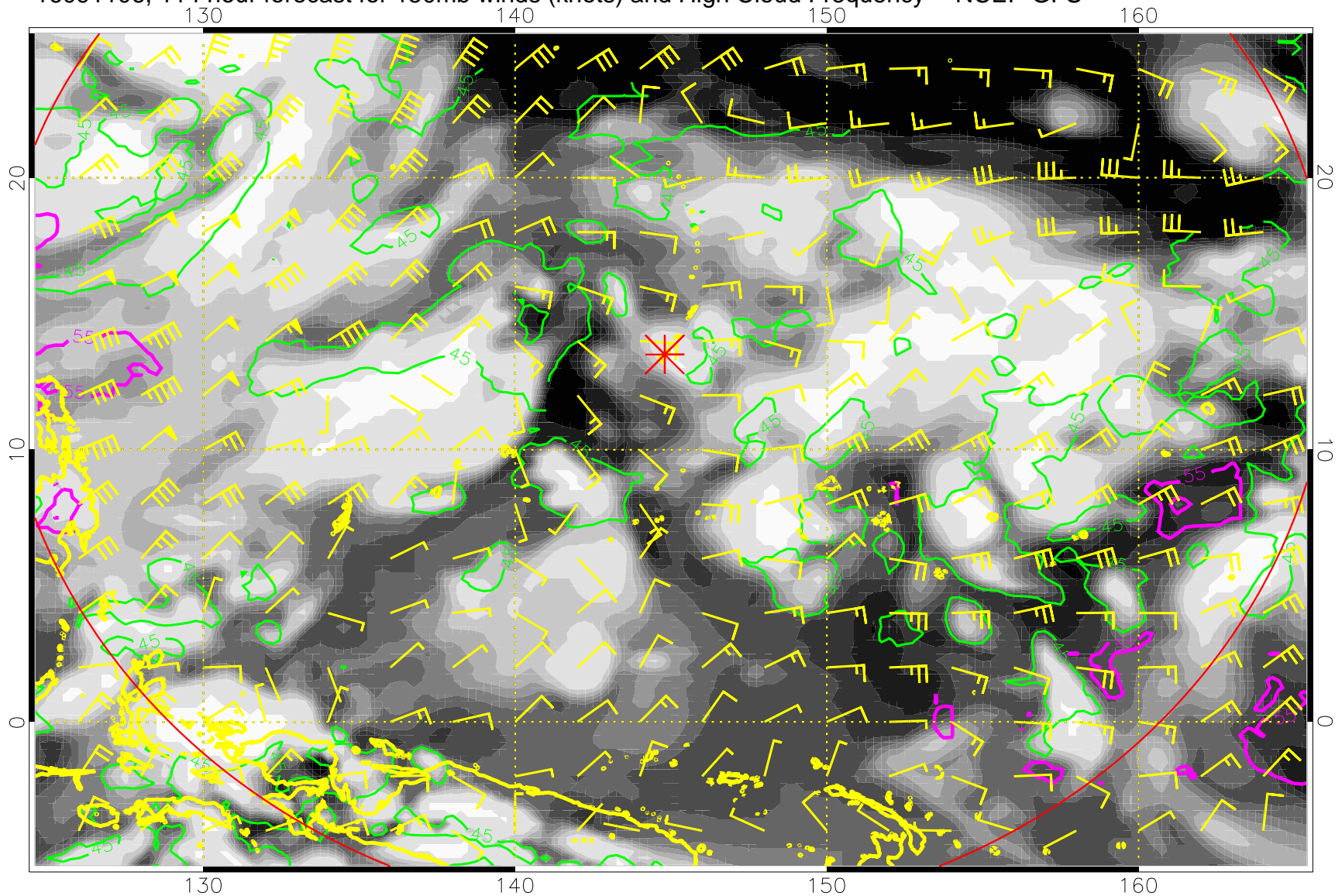
16091106, 114 hour forecast for 150mb winds (knots) and High Cloud Frequency -- NCEP GFS
