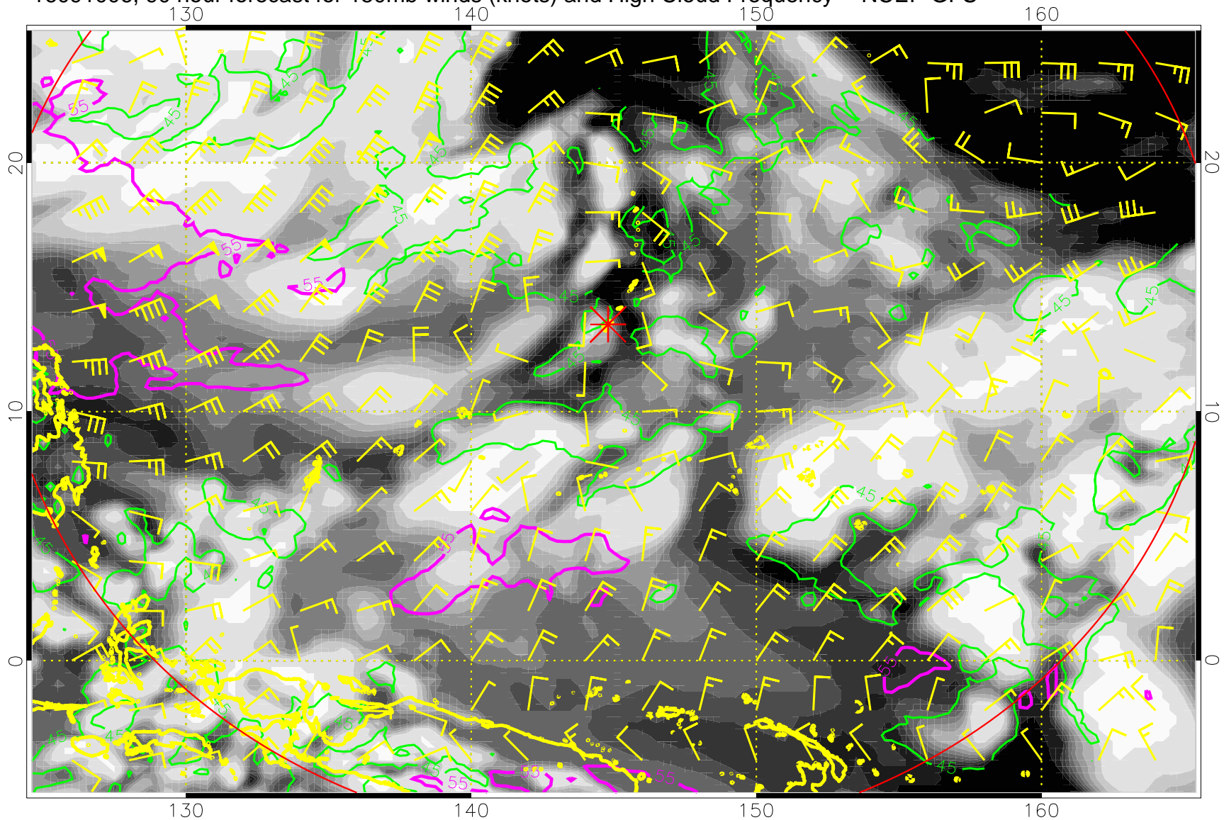
16091006, 90 hour forecast for 150mb winds (knots) and High Cloud Frequency -- NCEP GFS
