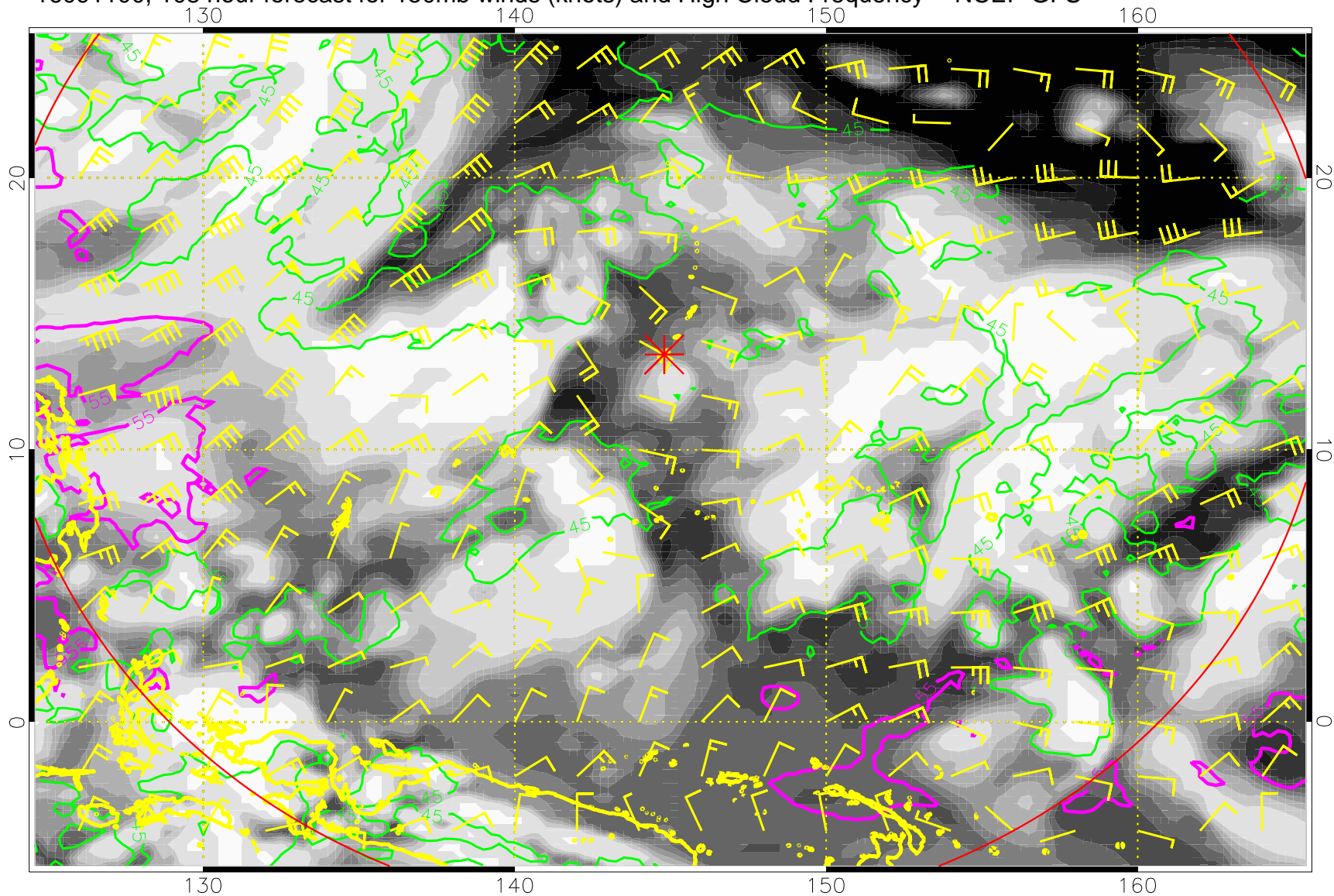
16091100, 108 hour forecast for 150mb winds (knots) and High Cloud Frequency -- NCEP GFS
