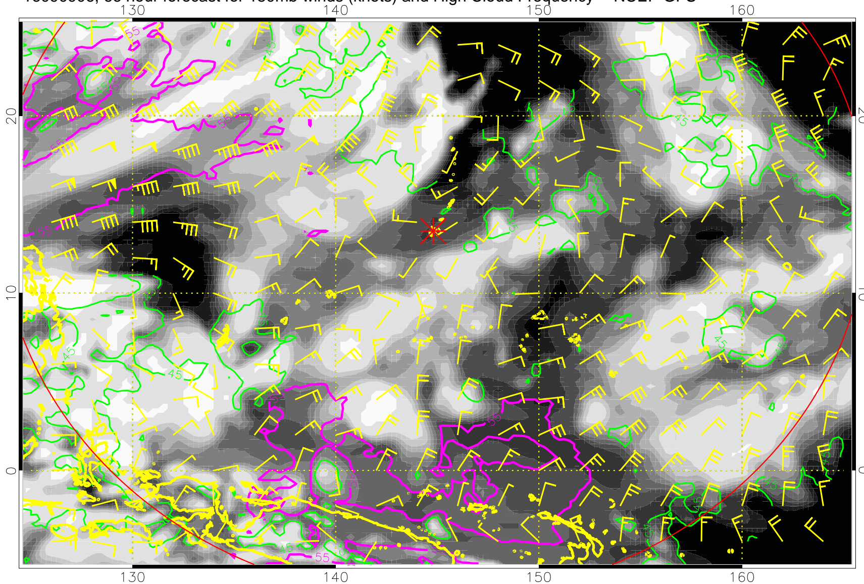
16090906, 66 hour forecast for 150mb winds (knots) and High Cloud Frequency -- NCEP GFS
