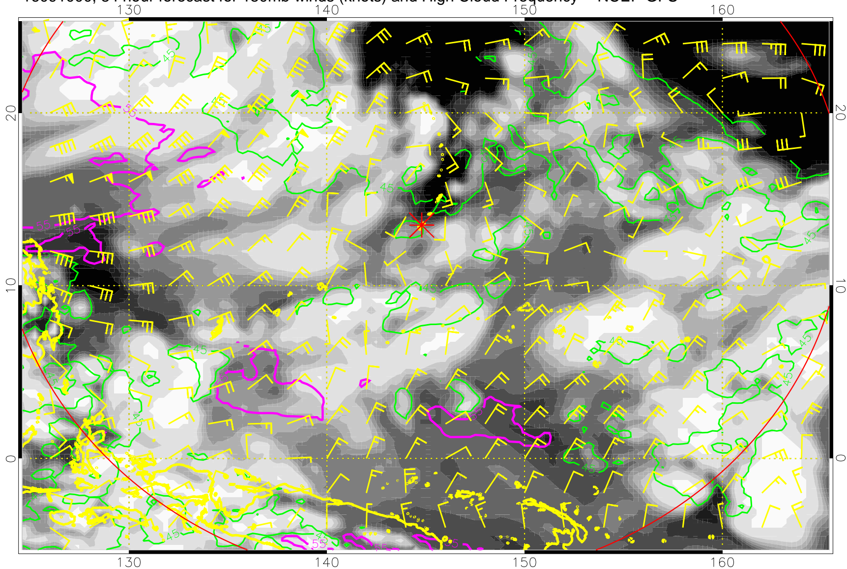
16091000, 84 hour forecast for 150mb winds (knots) and High Cloud Frequency -- NCEP GFS
