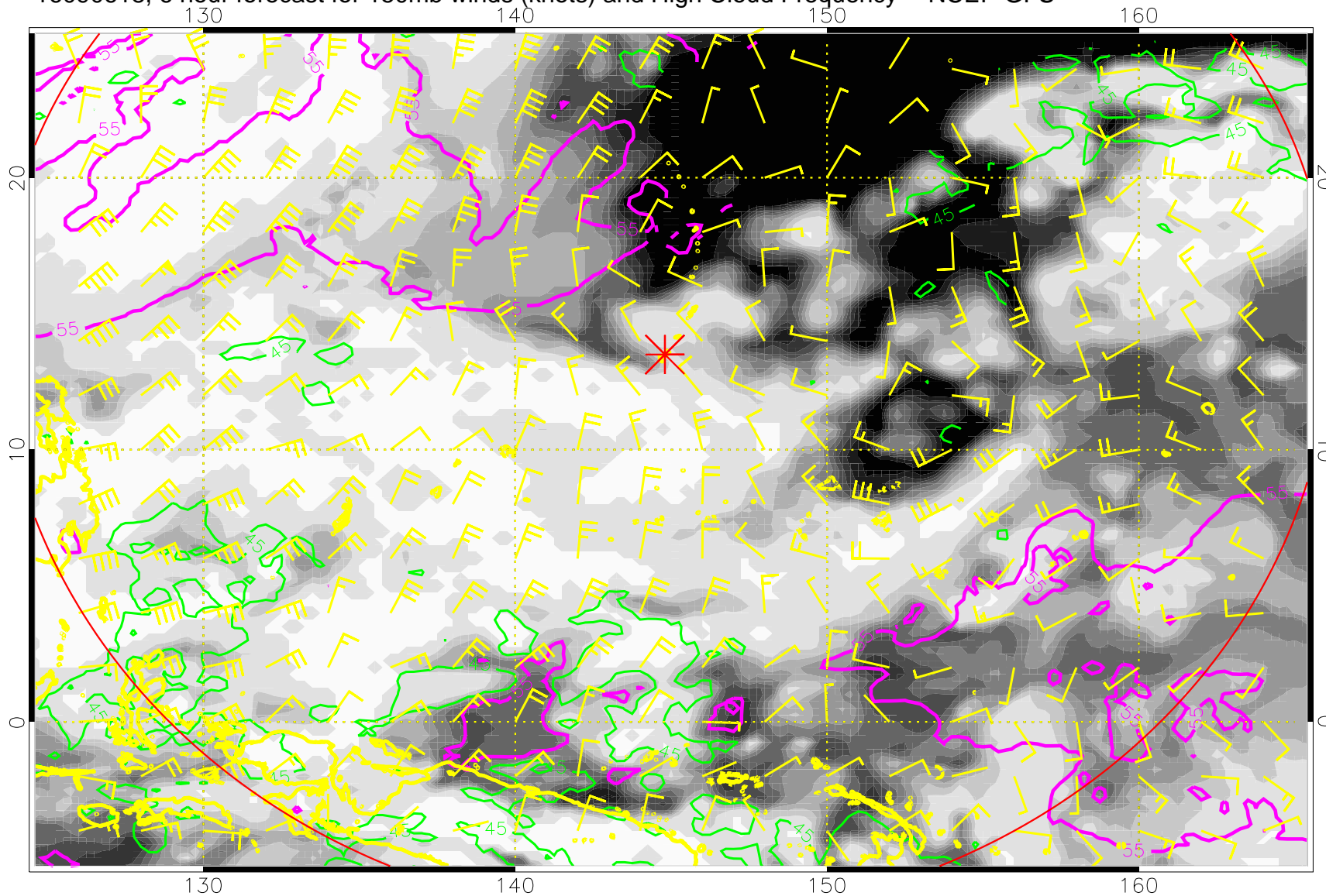
16090618, 6 hour forecast for 150mb winds (knots) and High Cloud Frequency -- NCEP GFS
