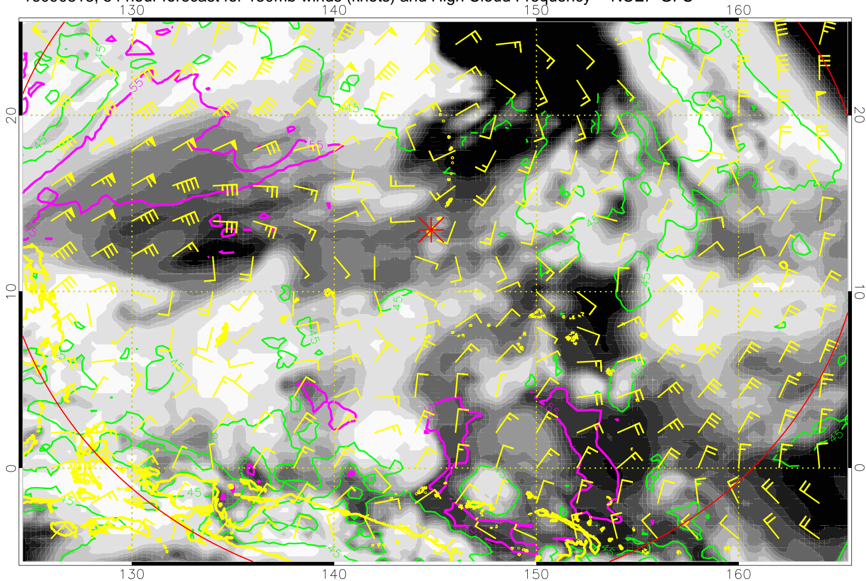
16090818, 54 hour forecast for 150mb winds (knots) and High Cloud Frequency -- NCEP GFS
