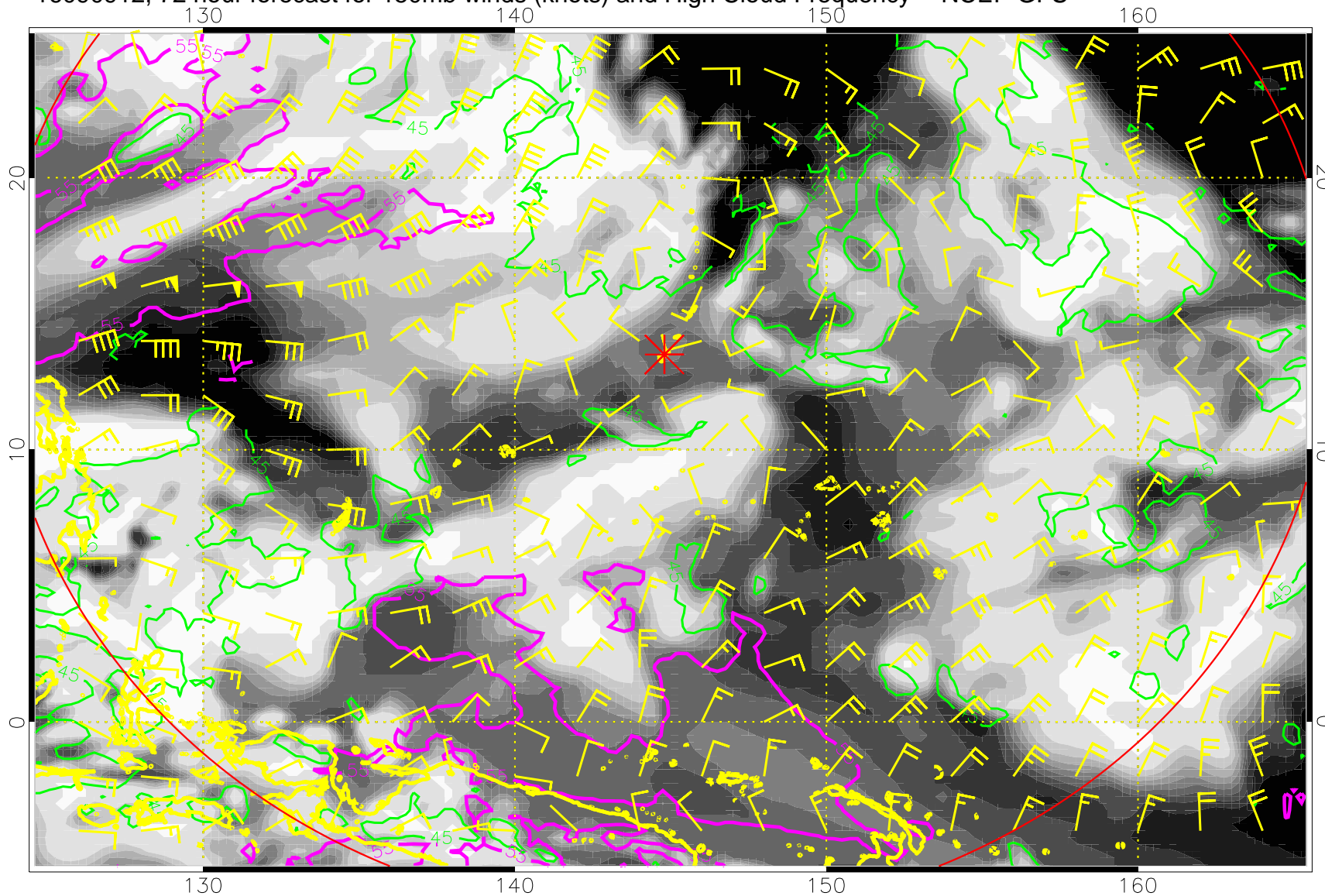
16090912, 72 hour forecast for 150mb winds (knots) and High Cloud Frequency -- NCEP GFS
