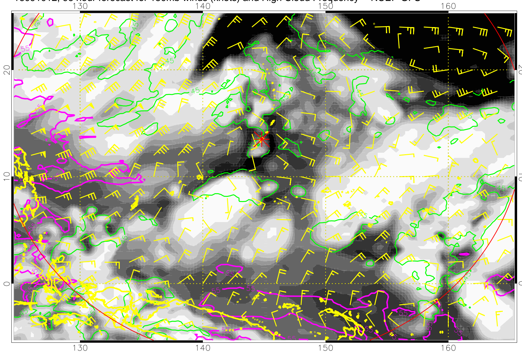
16091012, 96 hour forecast for 150mb winds (knots) and High Cloud Frequency -- NCEP GFS
