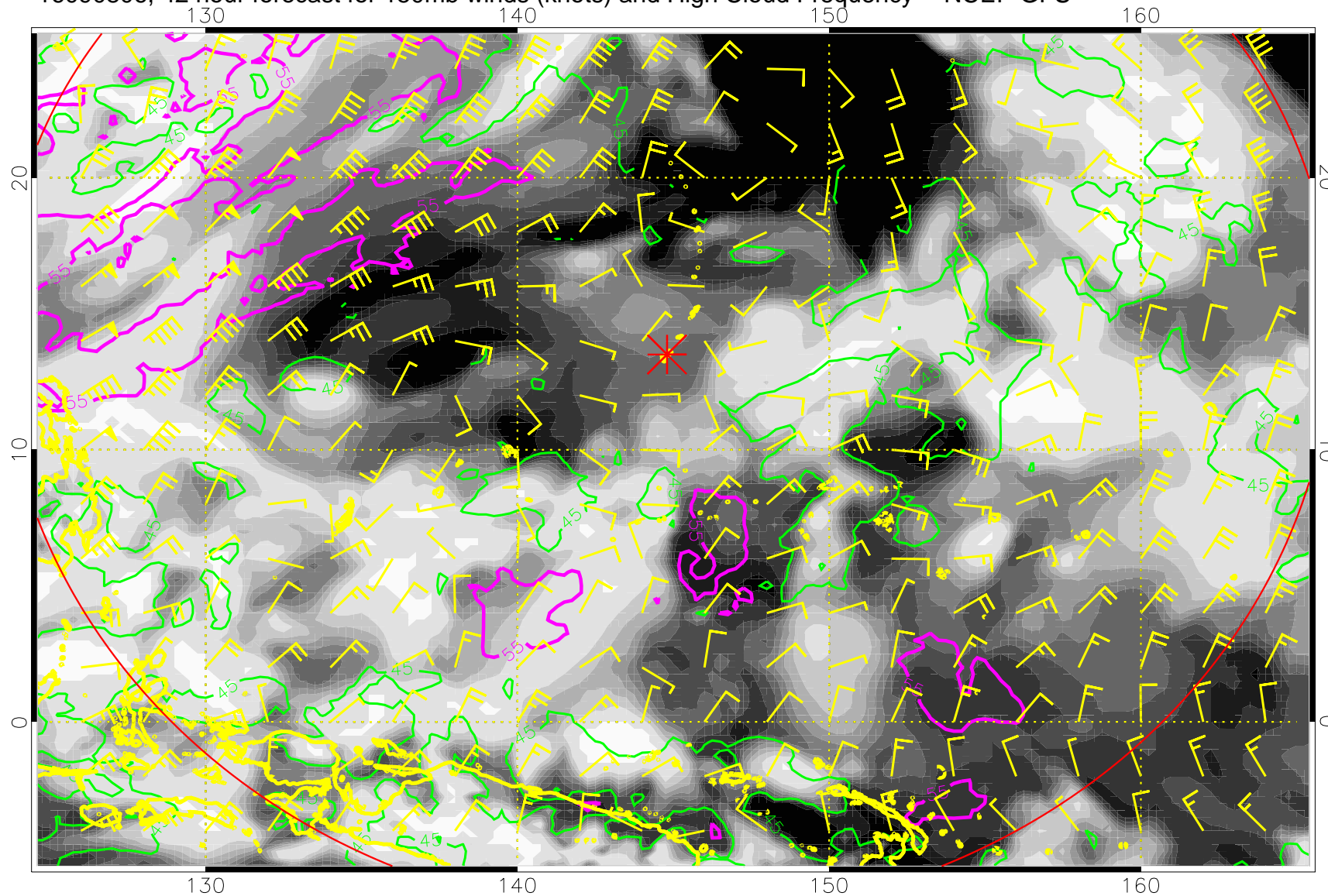
16090806, 42 hour forecast for 150mb winds (knots) and High Cloud Frequency -- NCEP GFS
