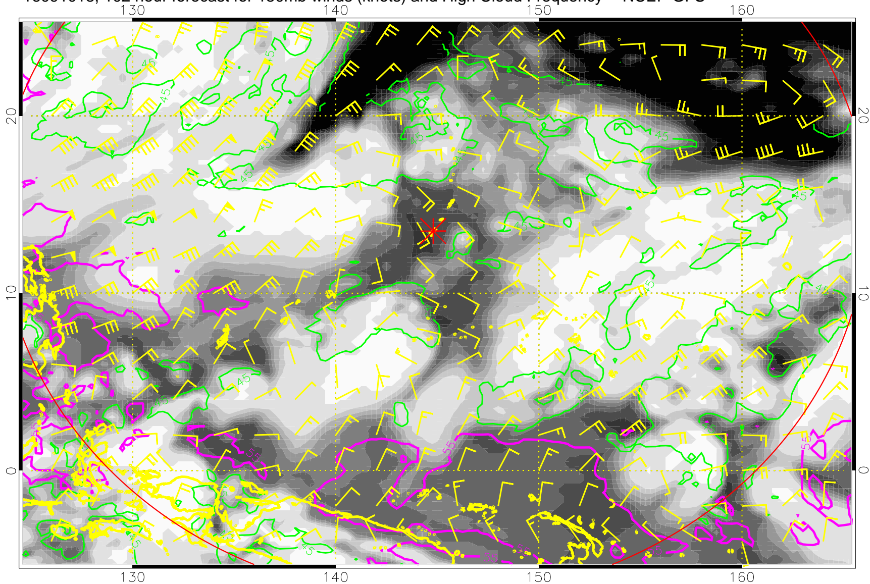
16091018, 102 hour forecast for 150mb winds (knots) and High Cloud Frequency -- NCEP GFS
