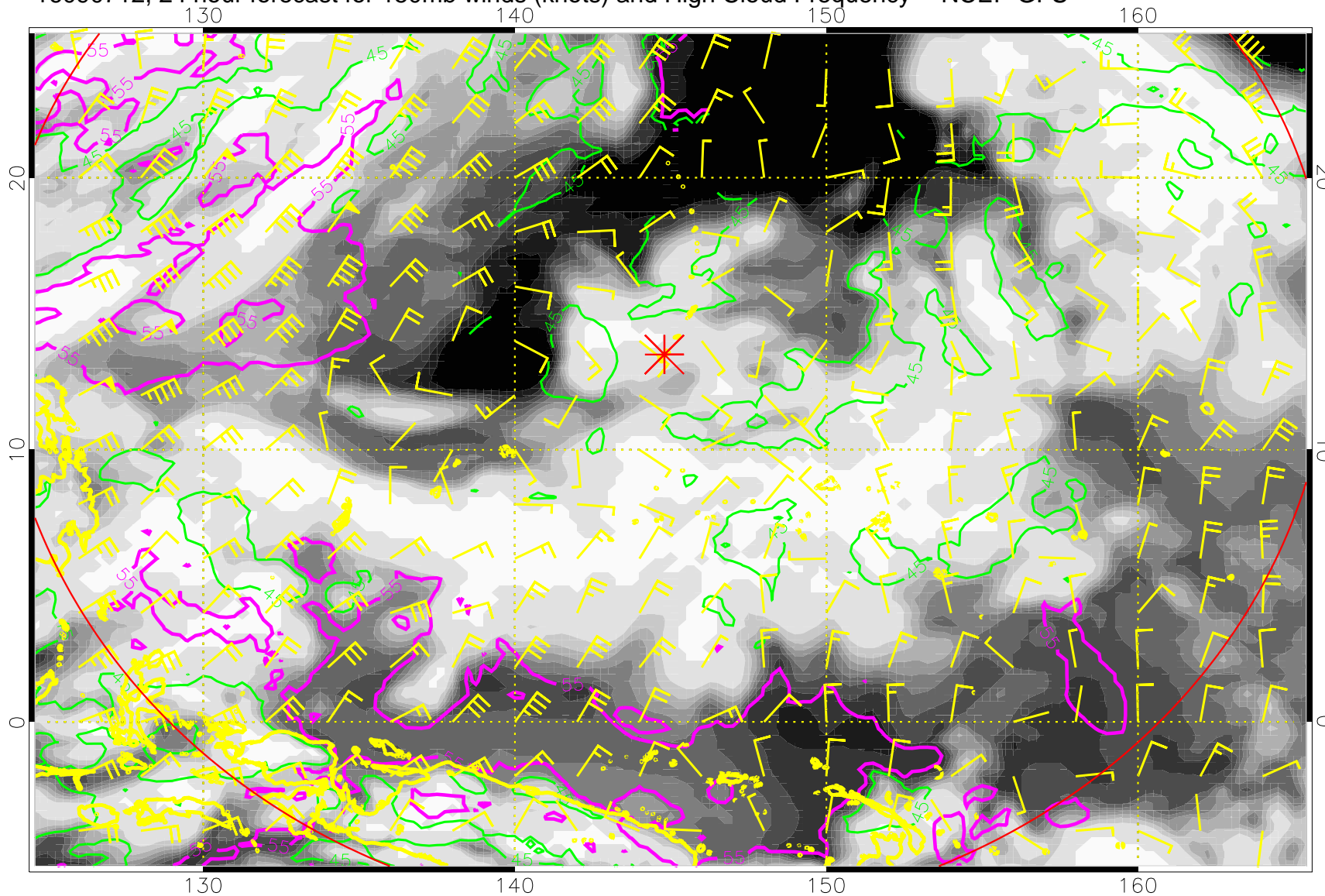
16090712, 24 hour forecast for 150mb winds (knots) and High Cloud Frequency -- NCEP GFS
