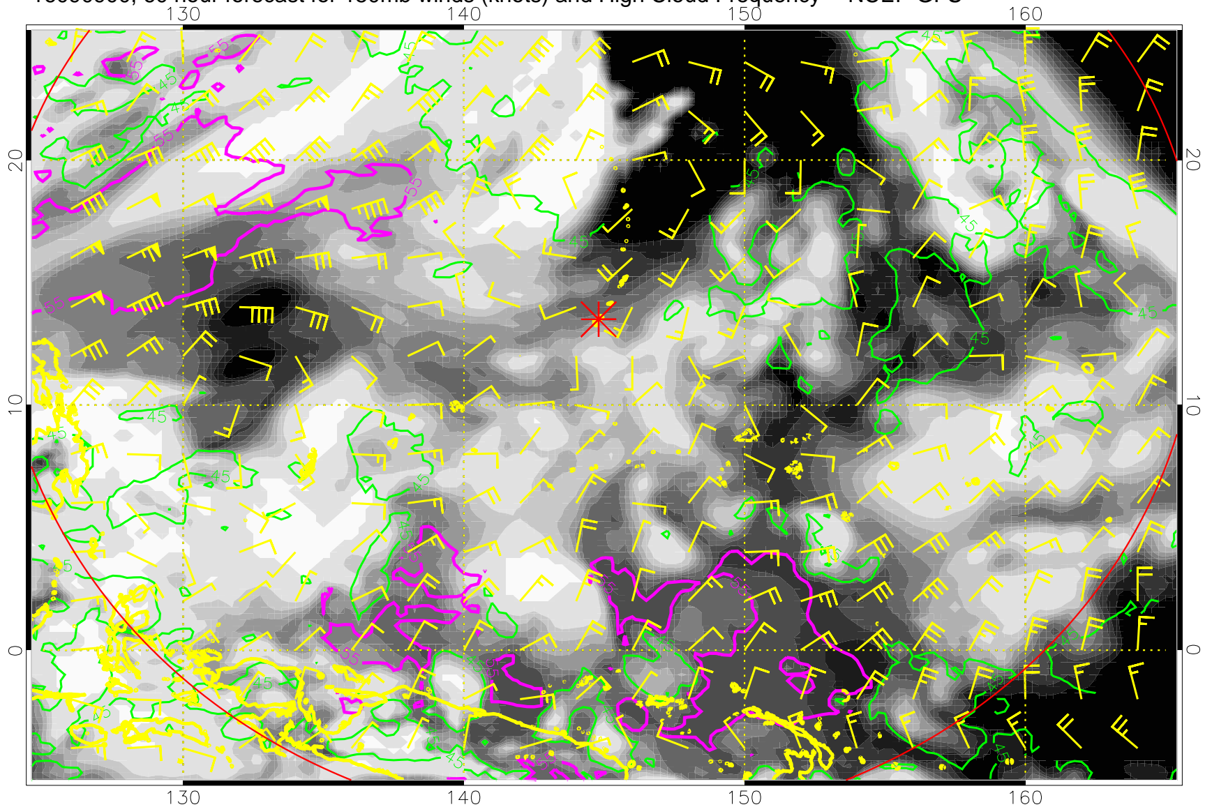
16090900, 60 hour forecast for 150mb winds (knots) and High Cloud Frequency -- NCEP GFS
