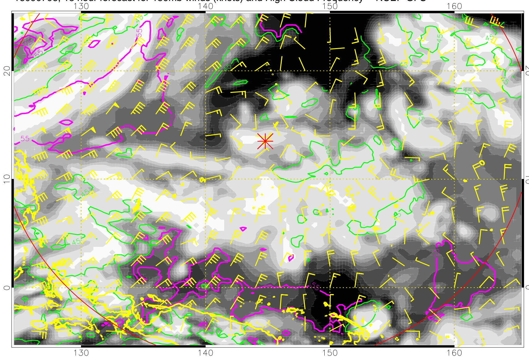
16090706, 18 hour forecast for 150mb winds (knots) and High Cloud Frequency -- NCEP GFS
