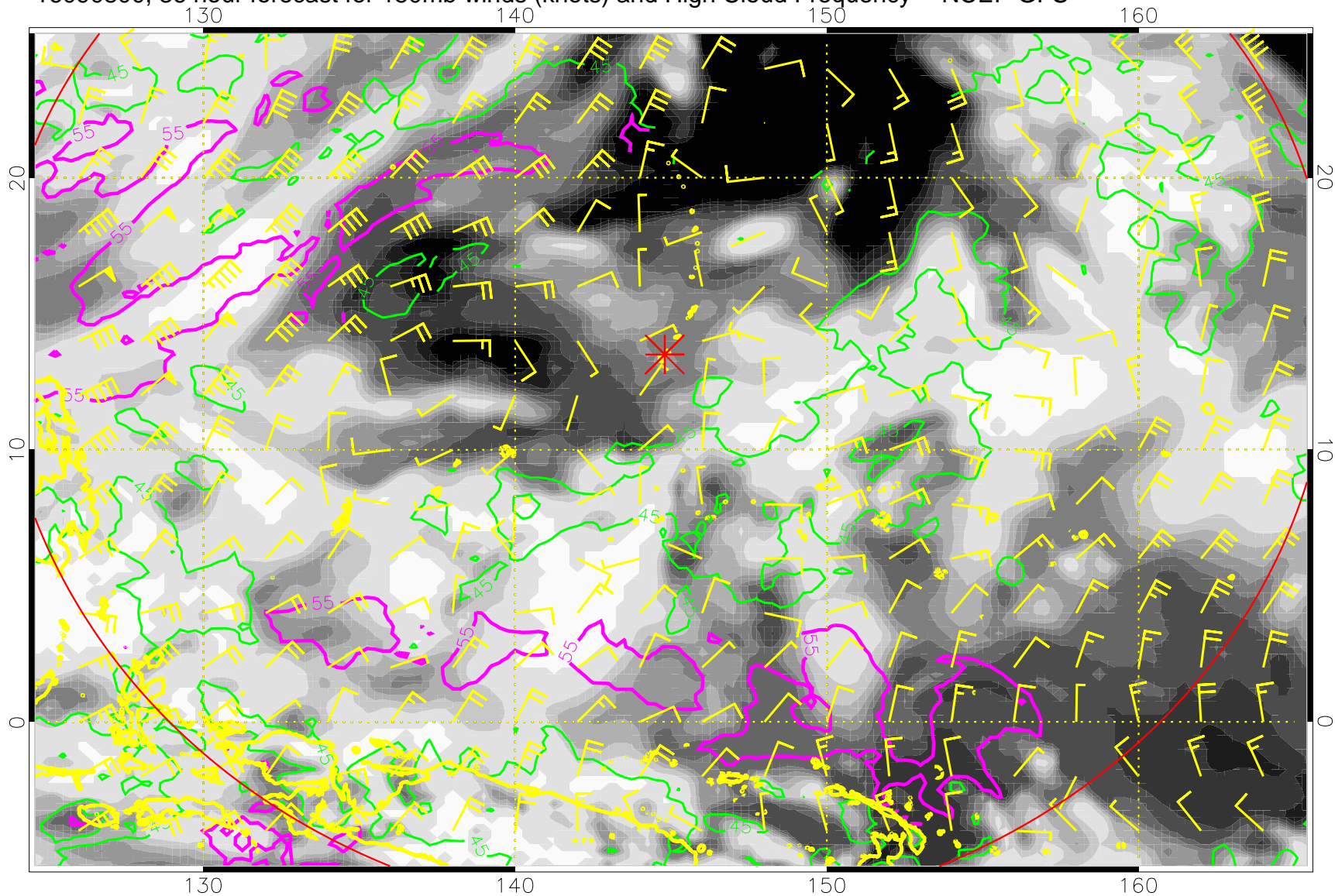
16090800, 36 hour forecast for 150mb winds (knots) and High Cloud Frequency -- NCEP GFS
