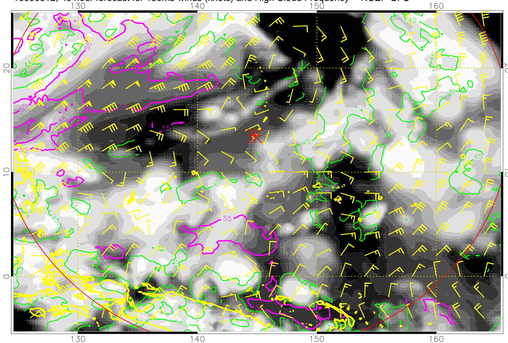
16090812, 48 hour forecast for 150mb winds (knots) and High Cloud Frequency -- NCEP GFS
