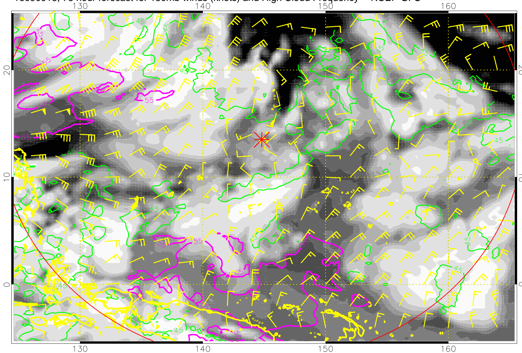
16090918, 78 hour forecast for 150mb winds (knots) and High Cloud Frequency -- NCEP GFS
