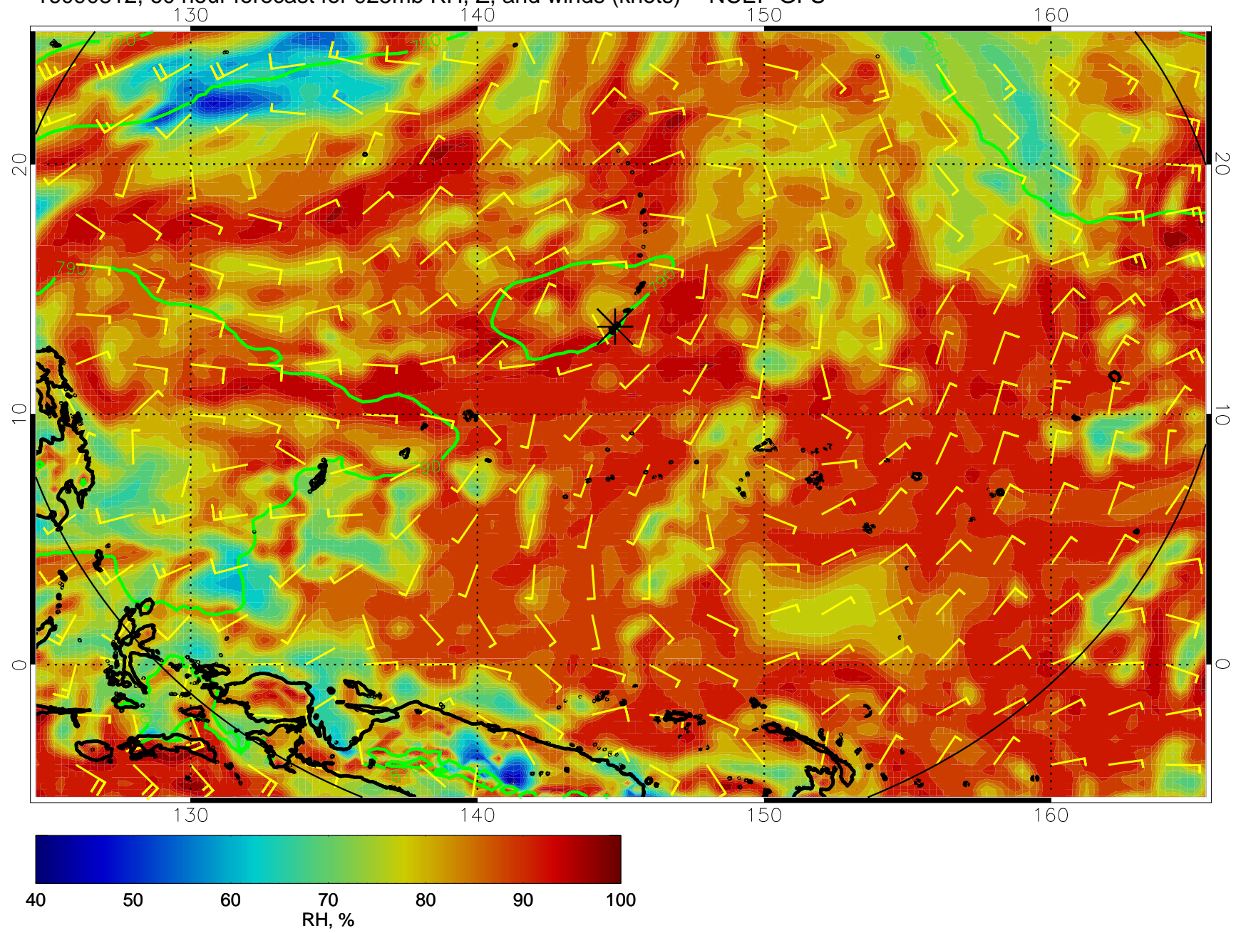
16090812, 60 hour forecast for 925mb RH, Z, and winds (knots) -- NCEP GFS
