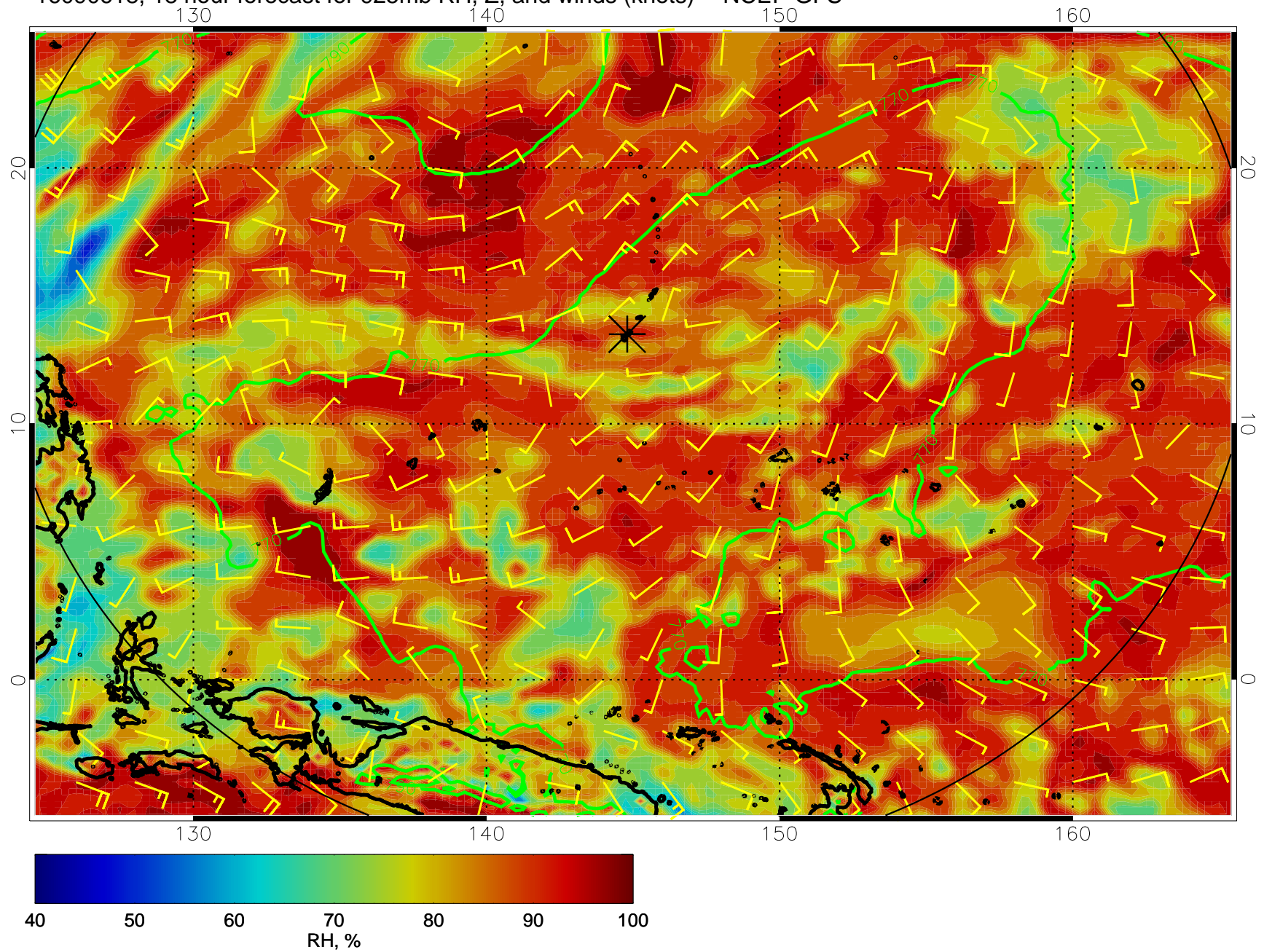
16090618, 18 hour forecast for 925mb RH, Z, and winds (knots) -- NCEP GFS
