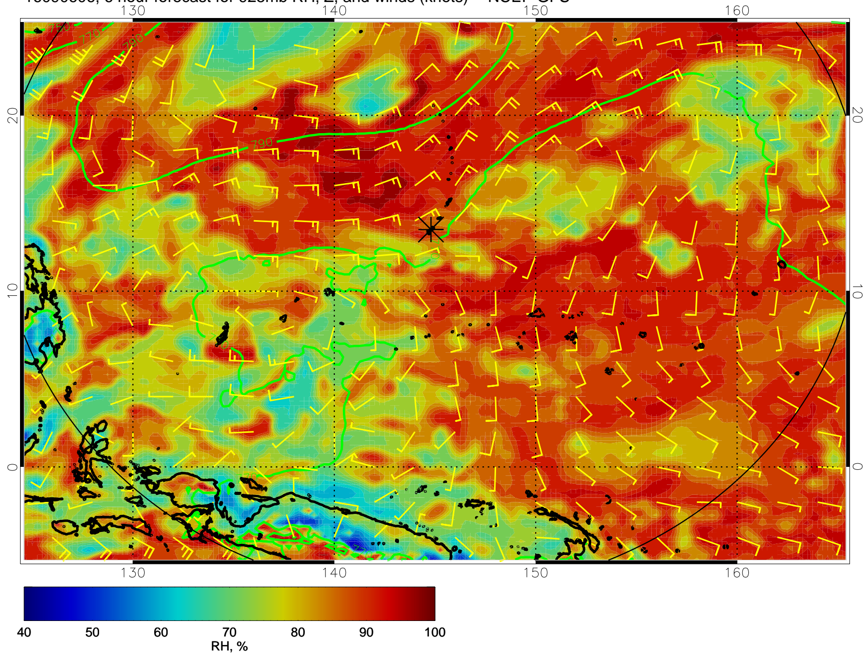
16090606, 6 hour forecast for 925mb RH, Z, and winds (knots) -- NCEP GFS
