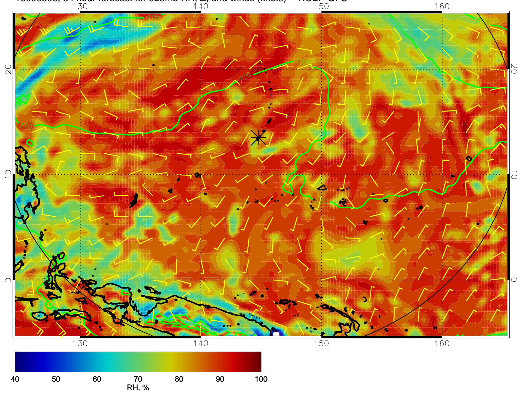
16090806, 54 hour forecast for 925mb RH, Z, and winds (knots) -- NCEP GFS
