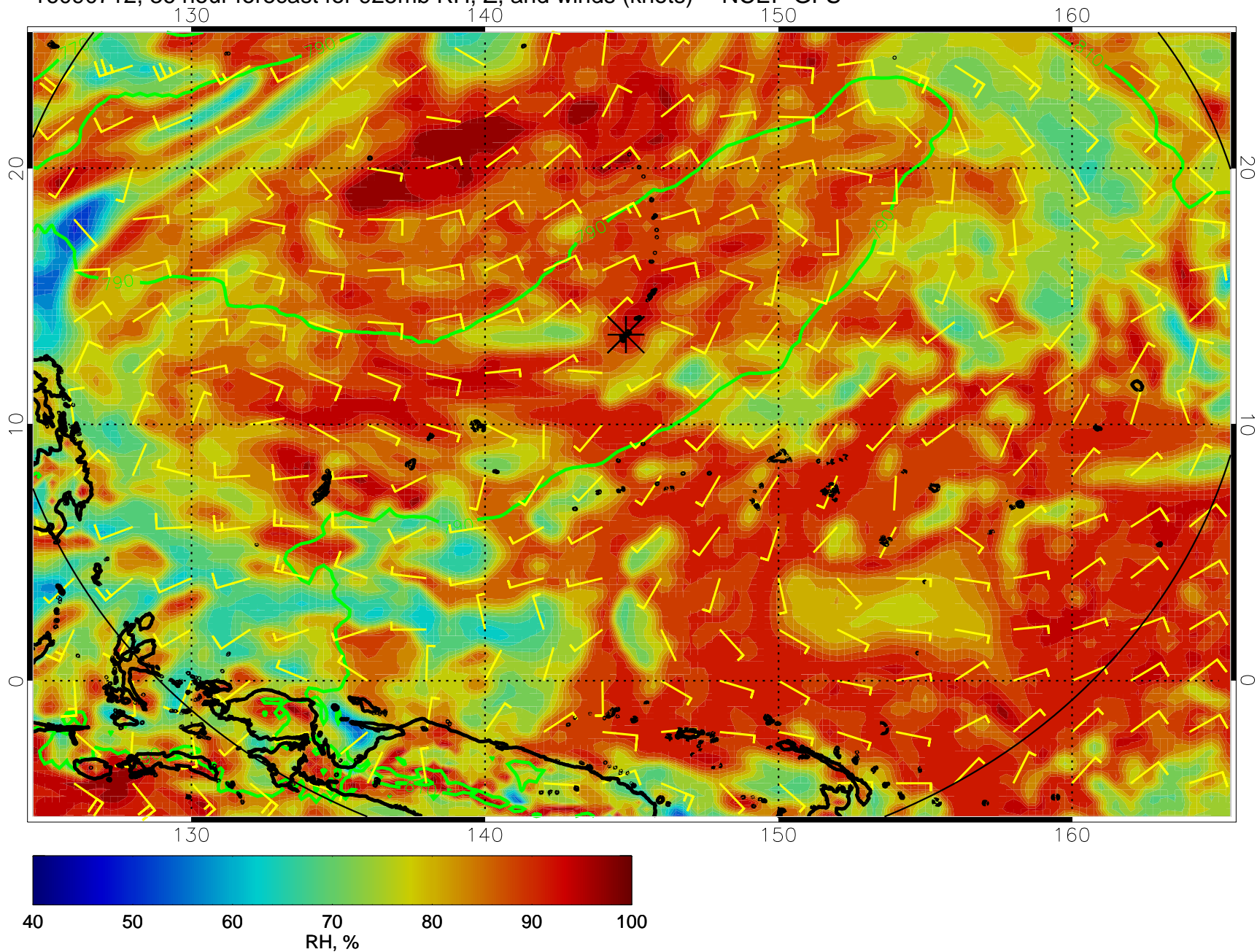
16090712, 36 hour forecast for 925mb RH, Z, and winds (knots) -- NCEP GFS
