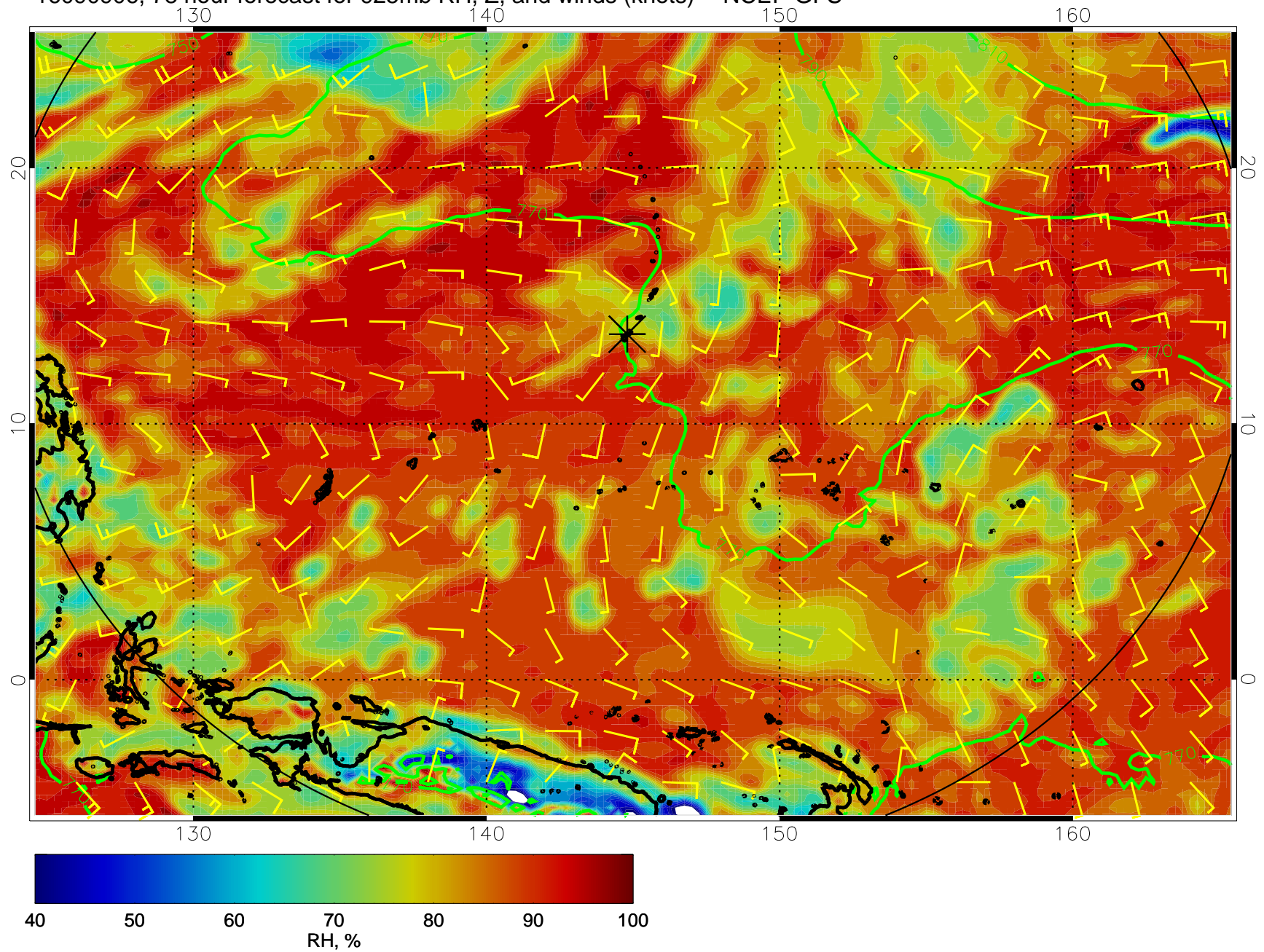
16090906, 78 hour forecast for 925mb RH, Z, and winds (knots) -- NCEP GFS
