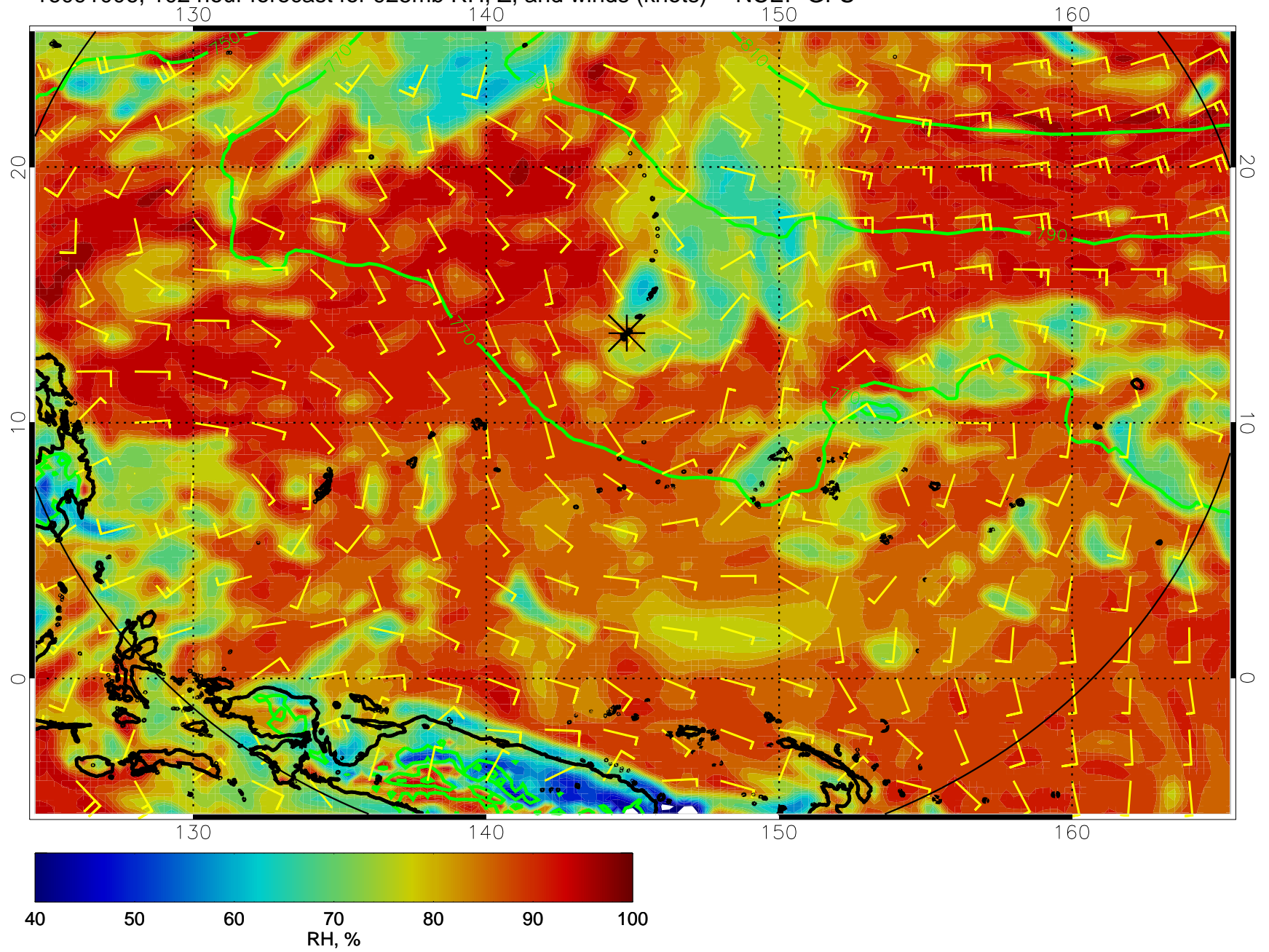
16091006, 102 hour forecast for 925mb RH, Z, and winds (knots) -- NCEP GFS
