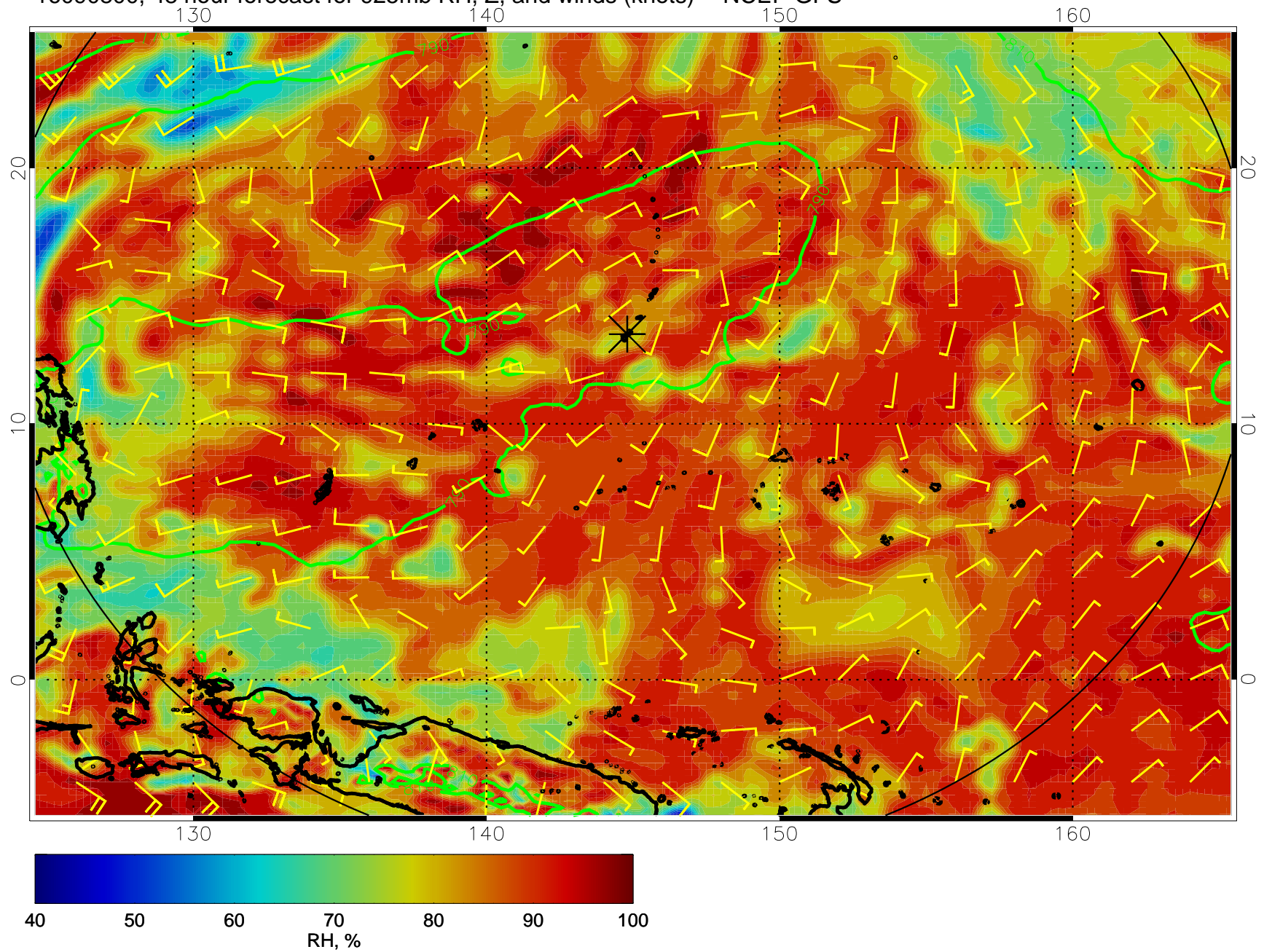
16090800, 48 hour forecast for 925mb RH, Z, and winds (knots) -- NCEP GFS
