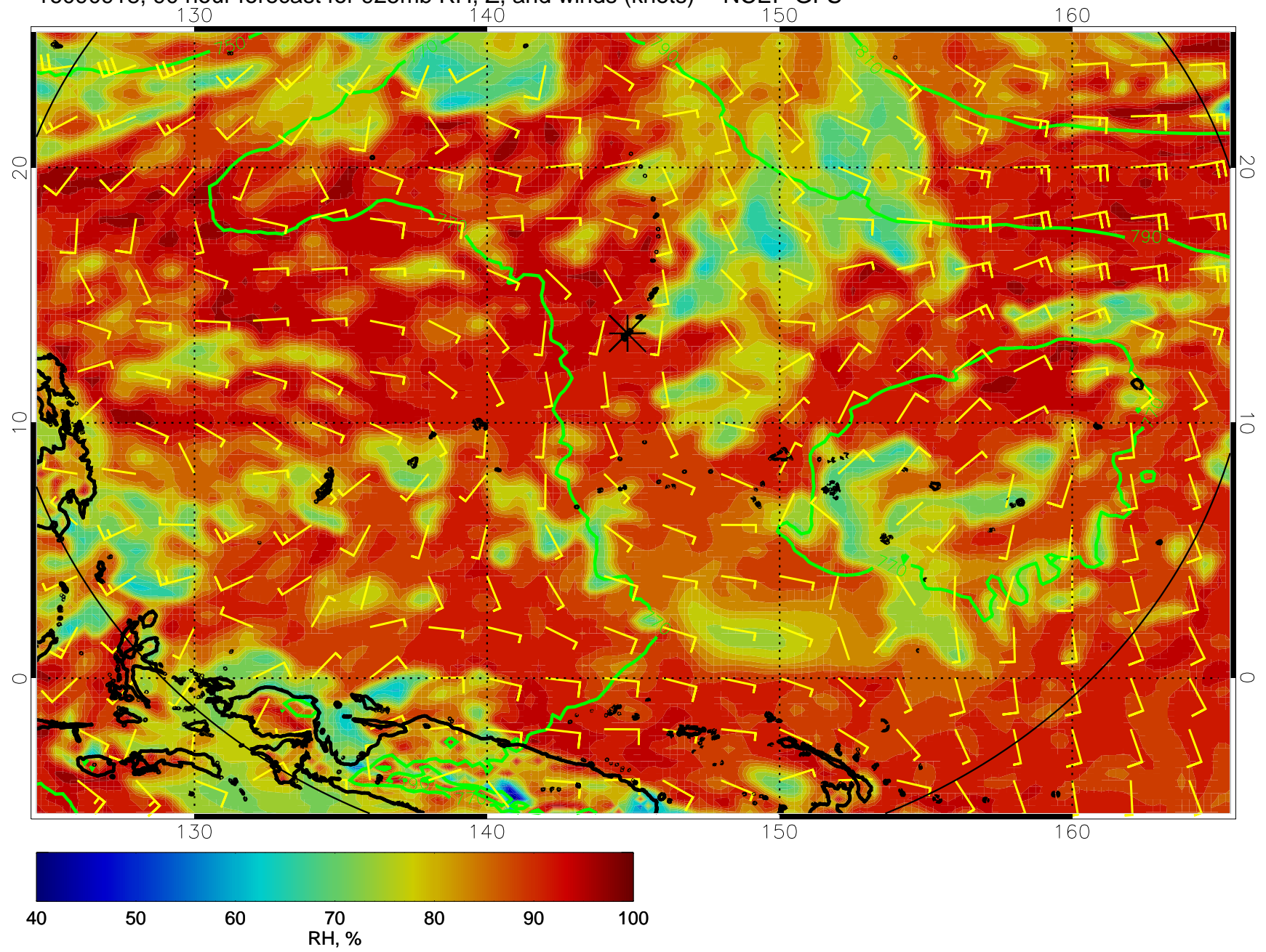
16090918, 90 hour forecast for 925mb RH, Z, and winds (knots) -- NCEP GFS
