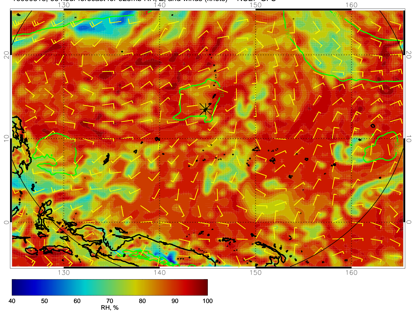
16090818, 66 hour forecast for 925mb RH, Z, and winds (knots) -- NCEP GFS
