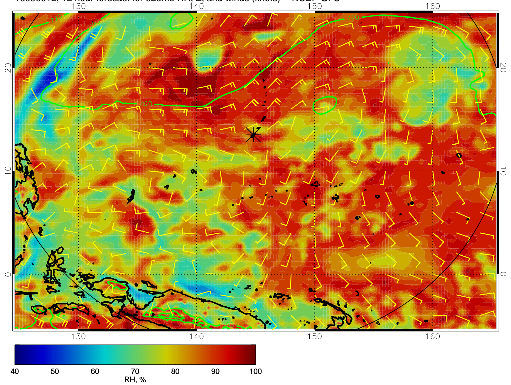
16090612, 12 hour forecast for 925mb RH, Z, and winds (knots) -- NCEP GFS
