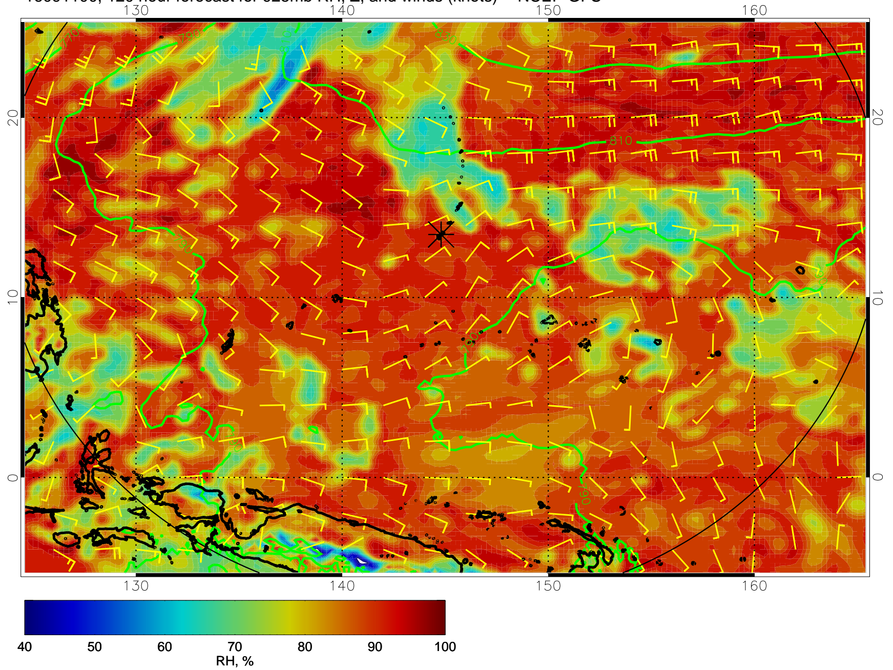
16091100, 120 hour forecast for 925mb RH, Z, and winds (knots) -- NCEP GFS
