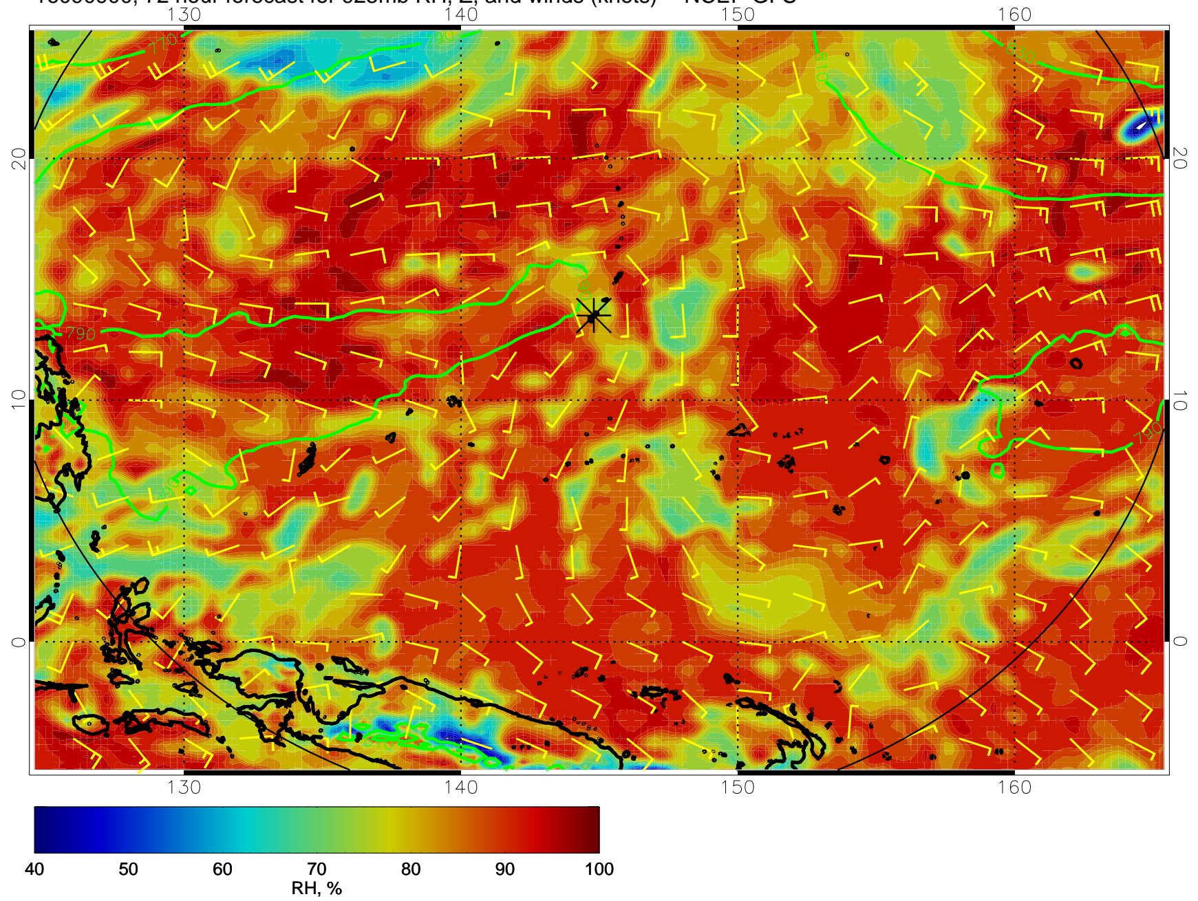
16090900, 72 hour forecast for 925mb RH, Z, and winds (knots) -- NCEP GFS
