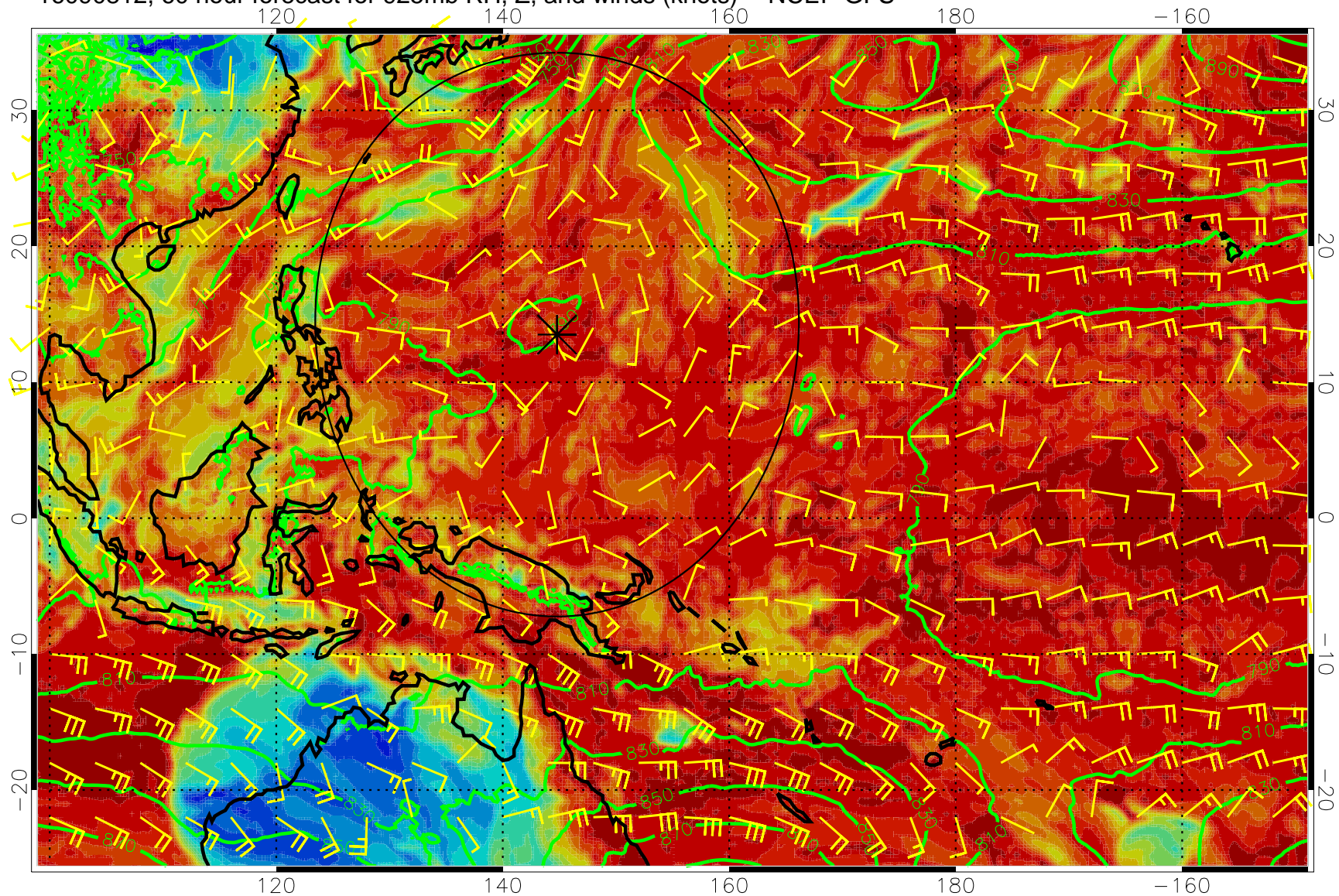
16090812, 60 hour forecast for 925mb RH, Z, and winds (knots) -- NCEP GFS
