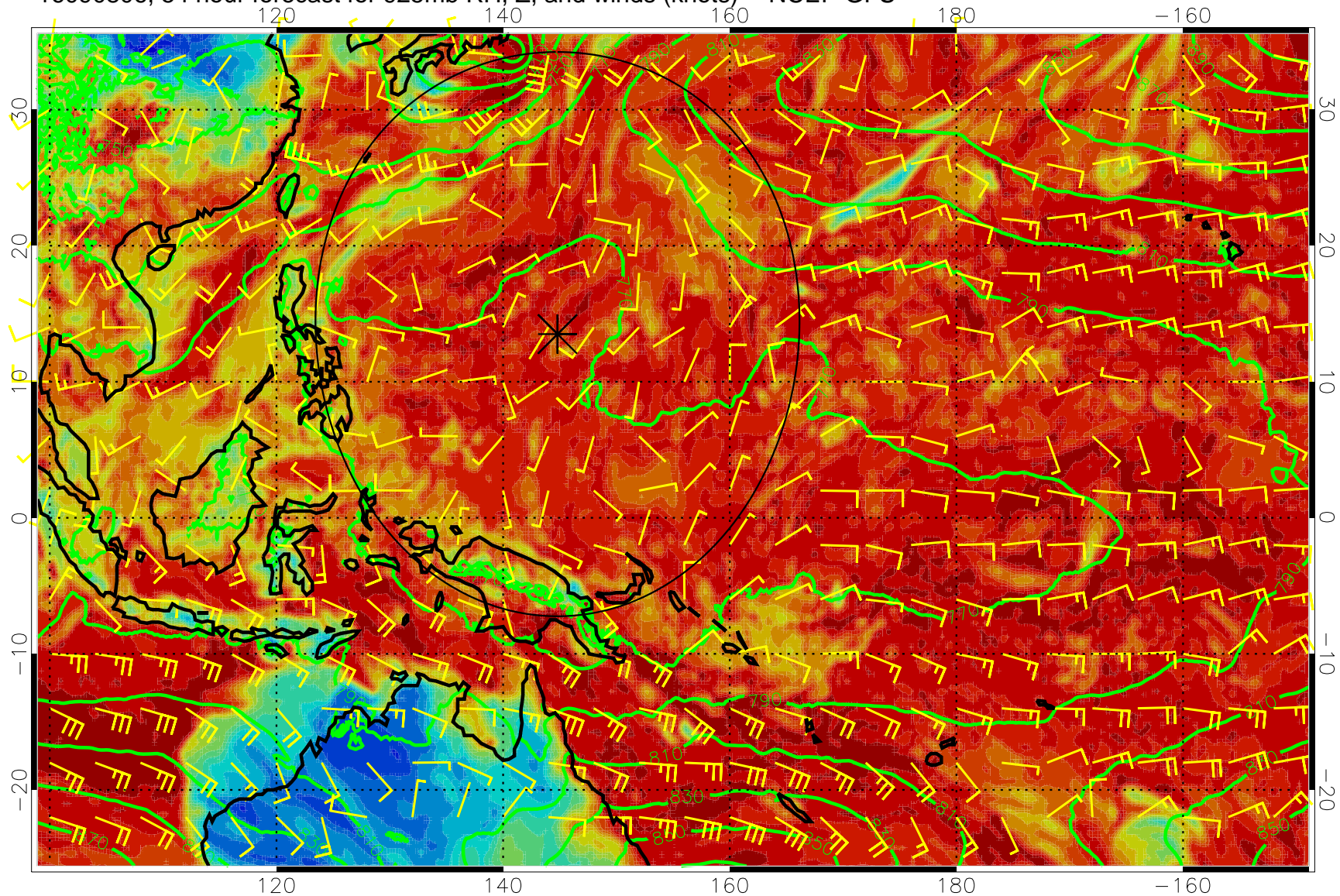
16090806, 54 hour forecast for 925mb RH, Z, and winds (knots) -- NCEP GFS
