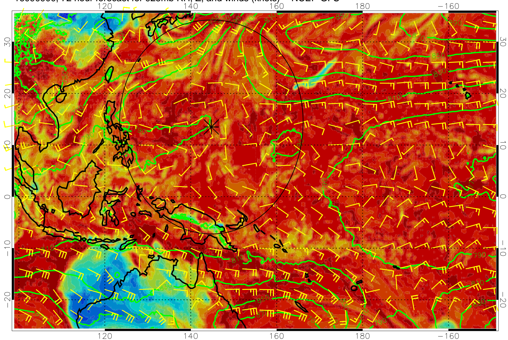
16090900, 72 hour forecast for 925mb RH, Z, and winds (knots) -- NCEP GFS
