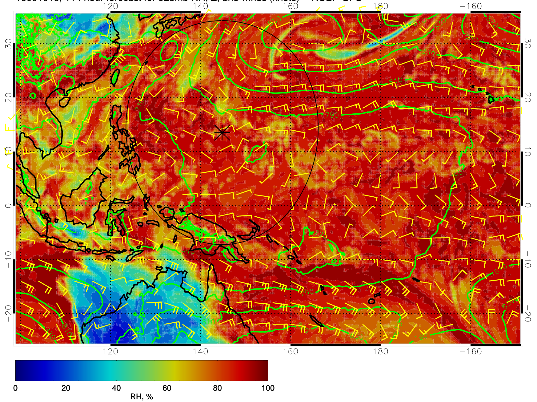
16091018, 114 hour forecast for 925mb RH, Z, and winds (knots) -- NCEP GFS
