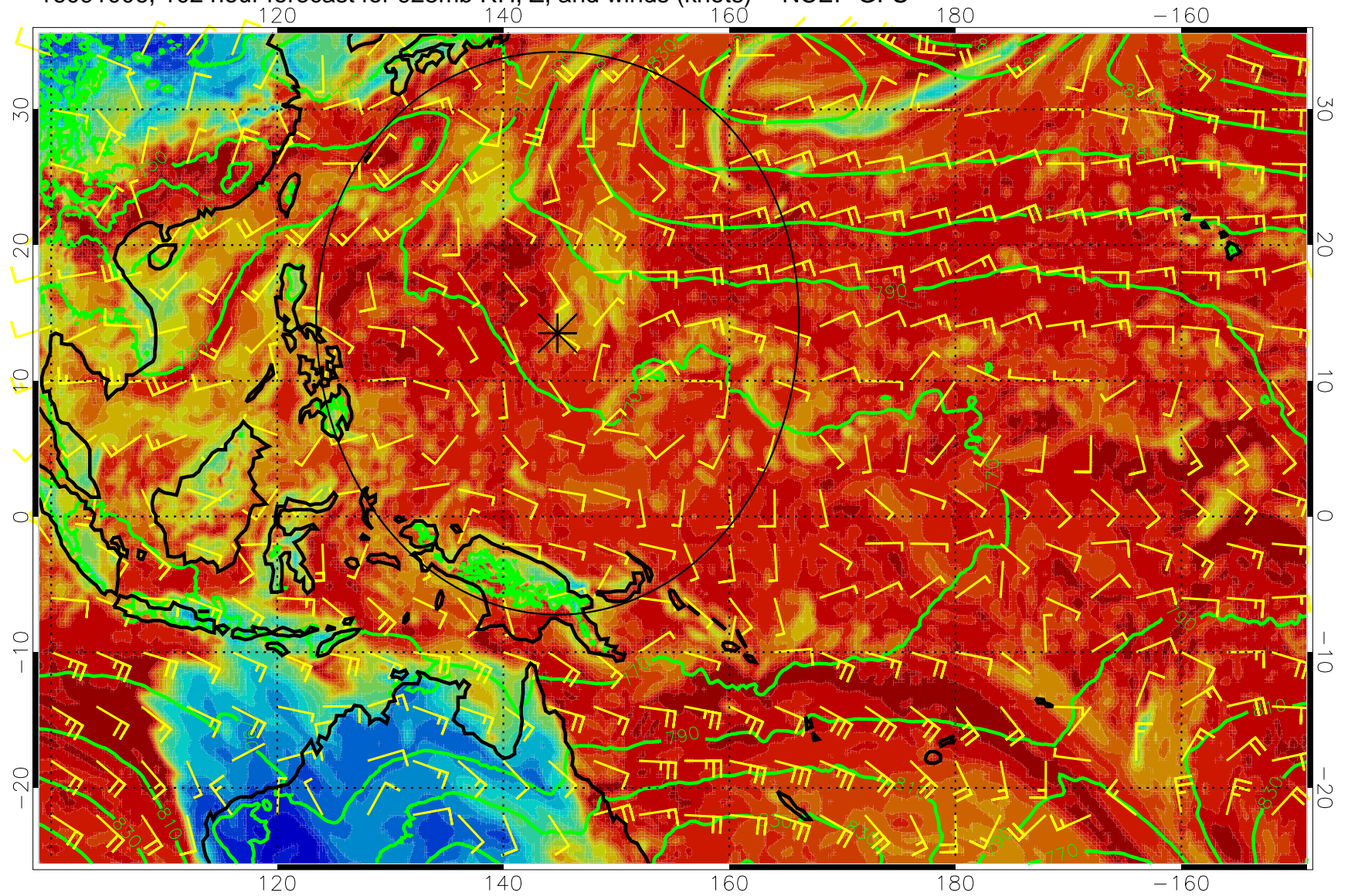
16091006, 102 hour forecast for 925mb RH, Z, and winds (knots) -- NCEP GFS
