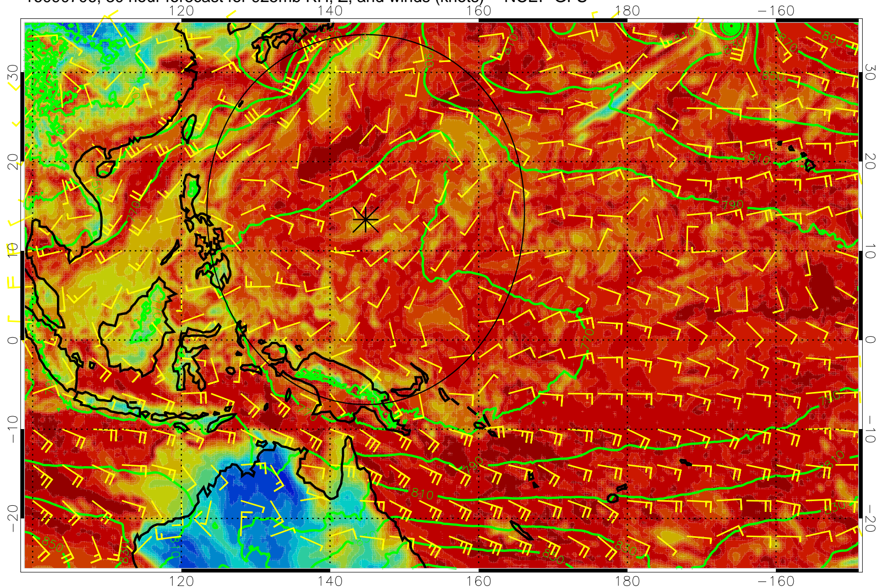
16090706, 30 hour forecast for 925mb RH, Z, and winds (knots) -- NCEP GFS
