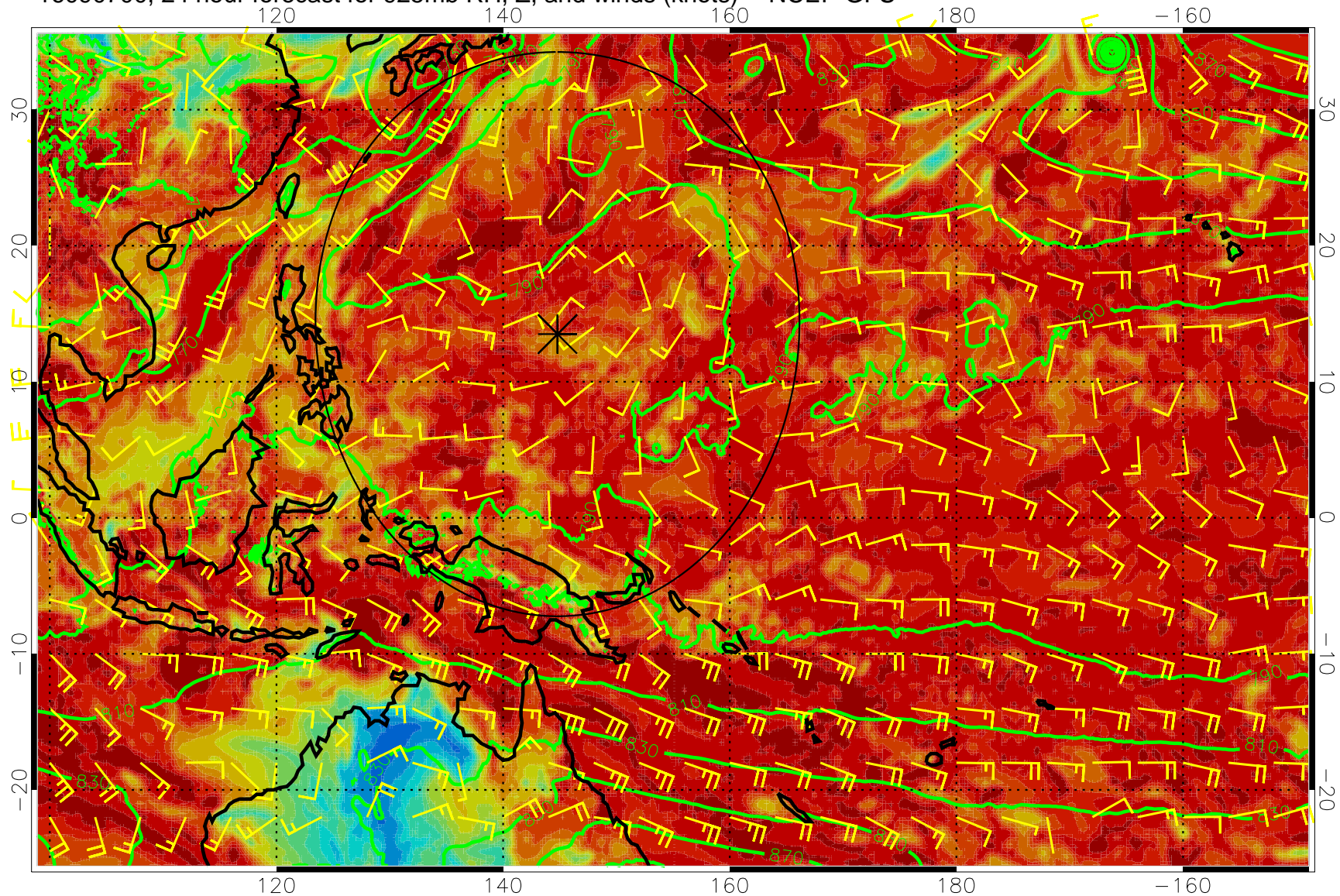
16090700, 24 hour forecast for 925mb RH, Z, and winds (knots) -- NCEP GFS
