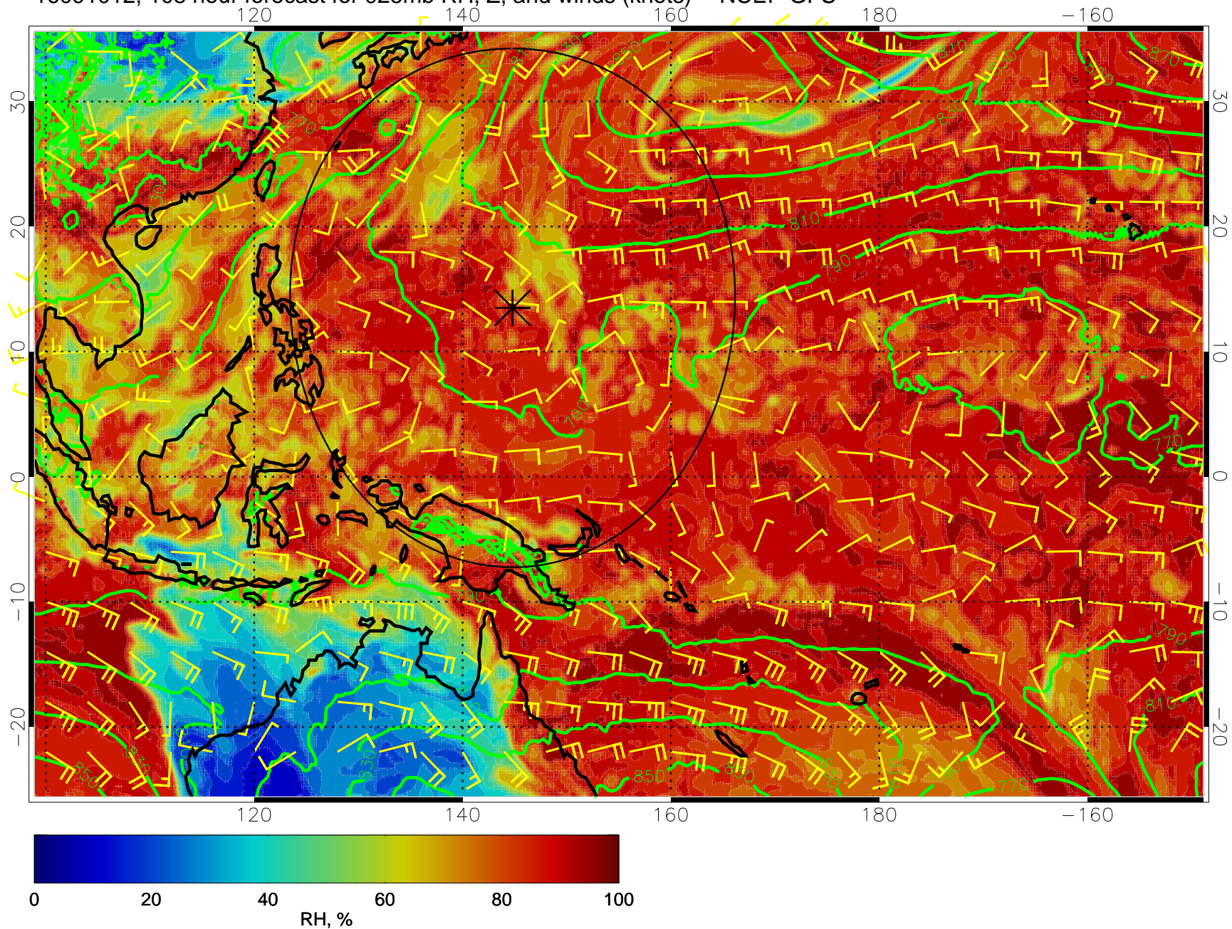
16091012, 108 hour forecast for 925mb RH, Z, and winds (knots) -- NCEP GFS
