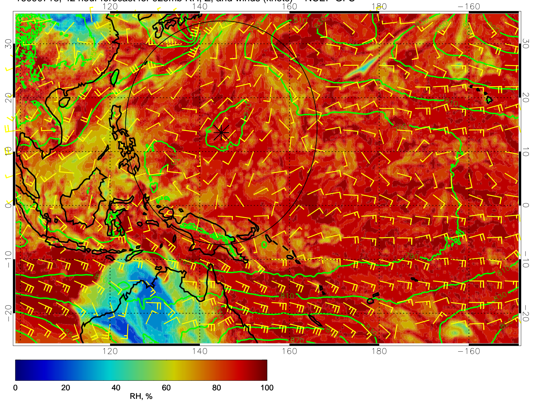
16090718, 42 hour forecast for 925mb RH, Z, and winds (knots) -- NCEP GFS
