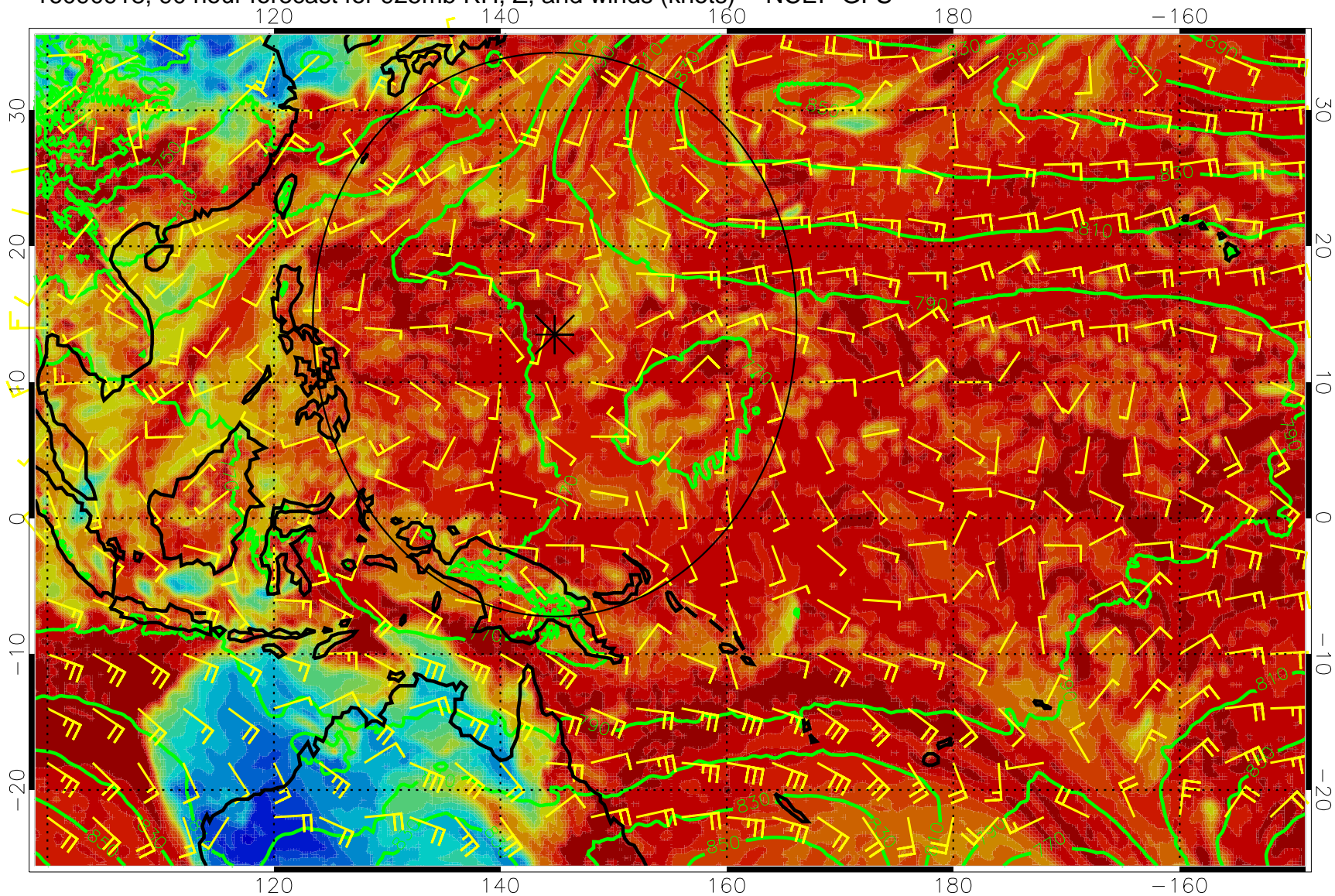
16090918, 90 hour forecast for 925mb RH, Z, and winds (knots) -- NCEP GFS
