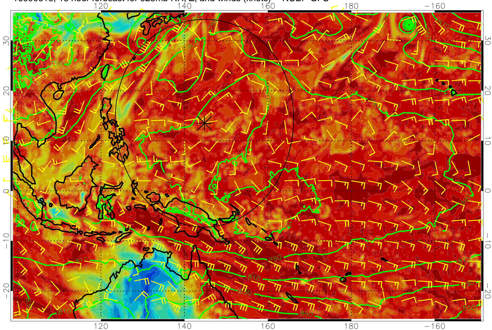
16090618, 18 hour forecast for 925mb RH, Z, and winds (knots) -- NCEP GFS
