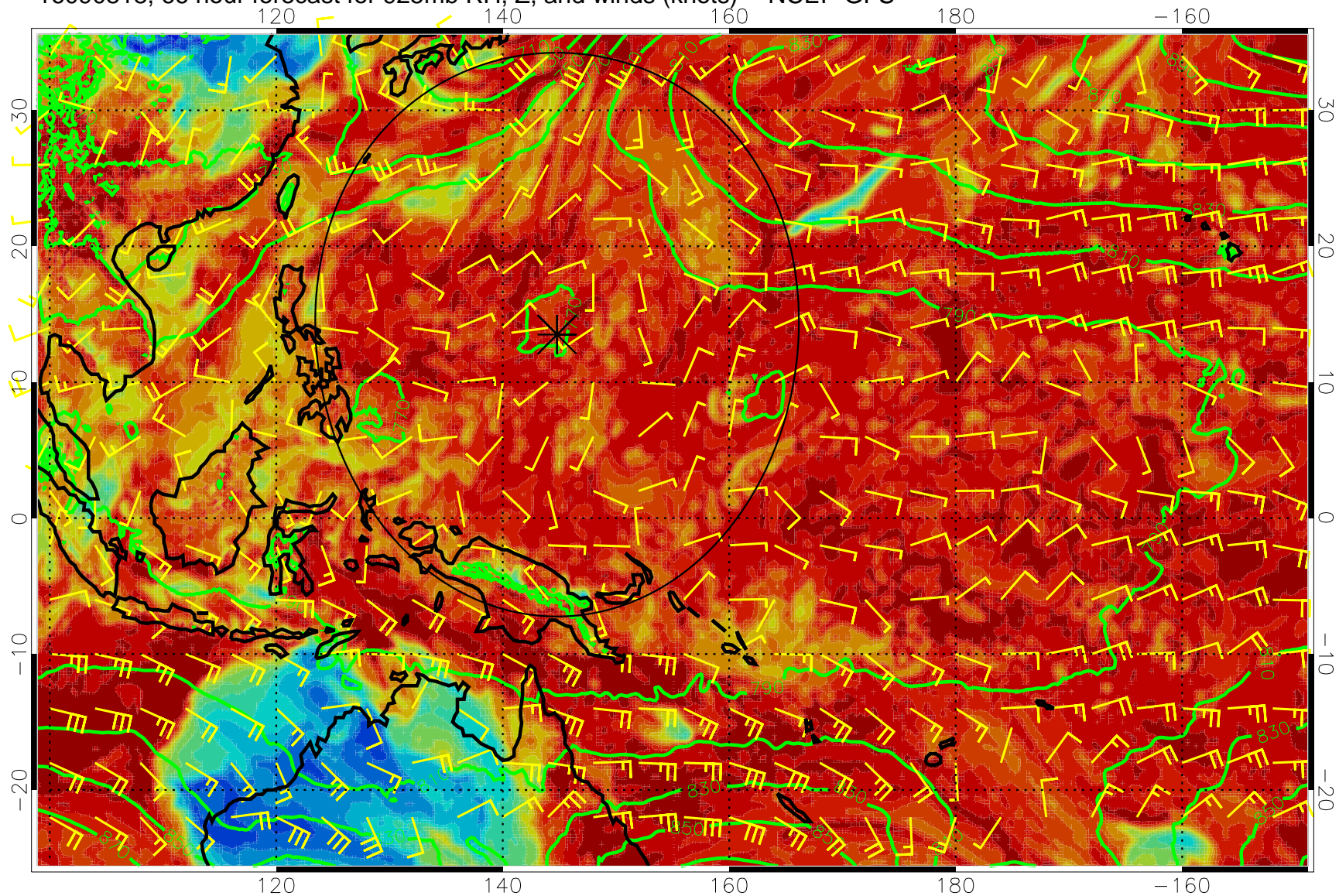
16090818, 66 hour forecast for 925mb RH, Z, and winds (knots) -- NCEP GFS
