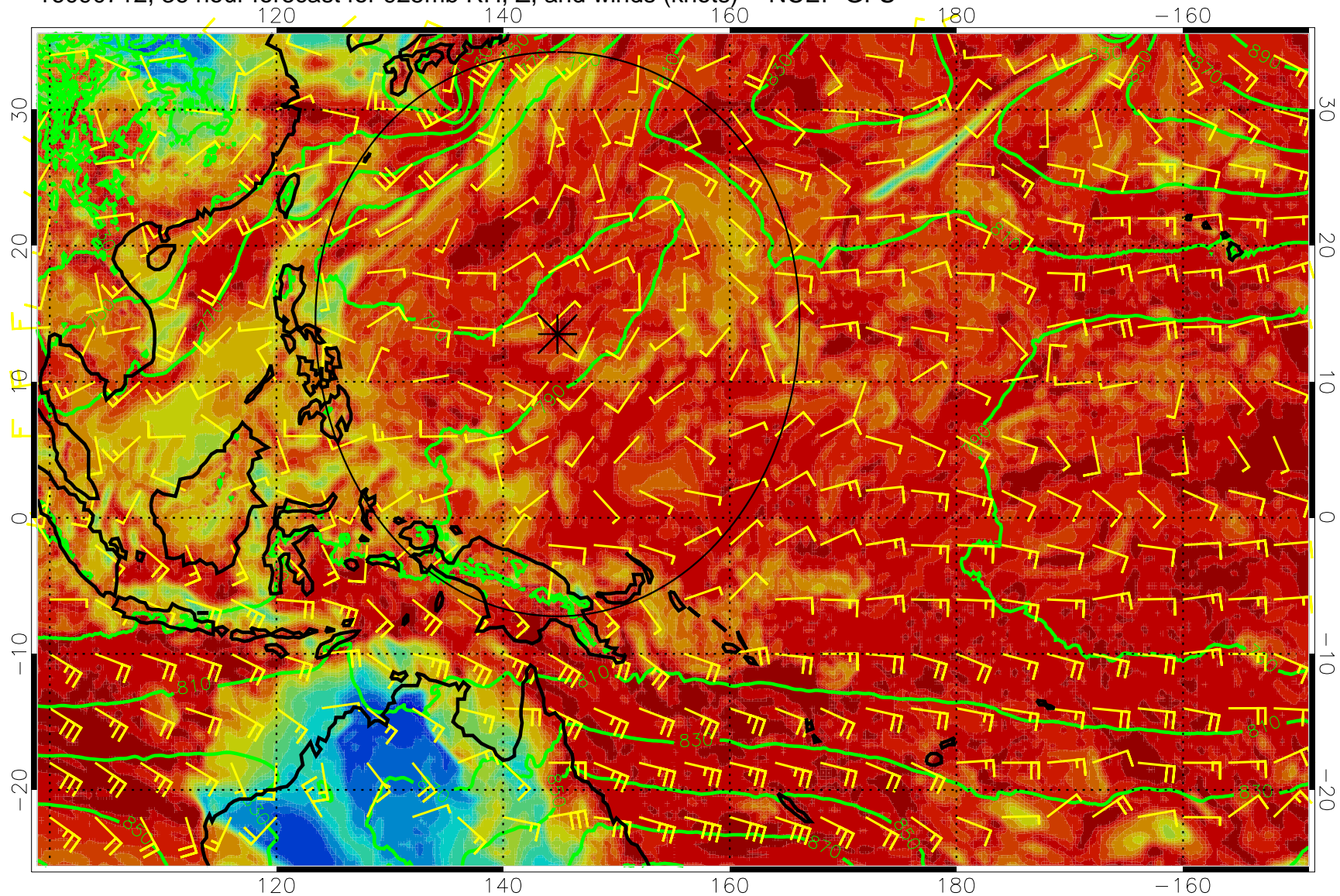
16090712, 36 hour forecast for 925mb RH, Z, and winds (knots) -- NCEP GFS
