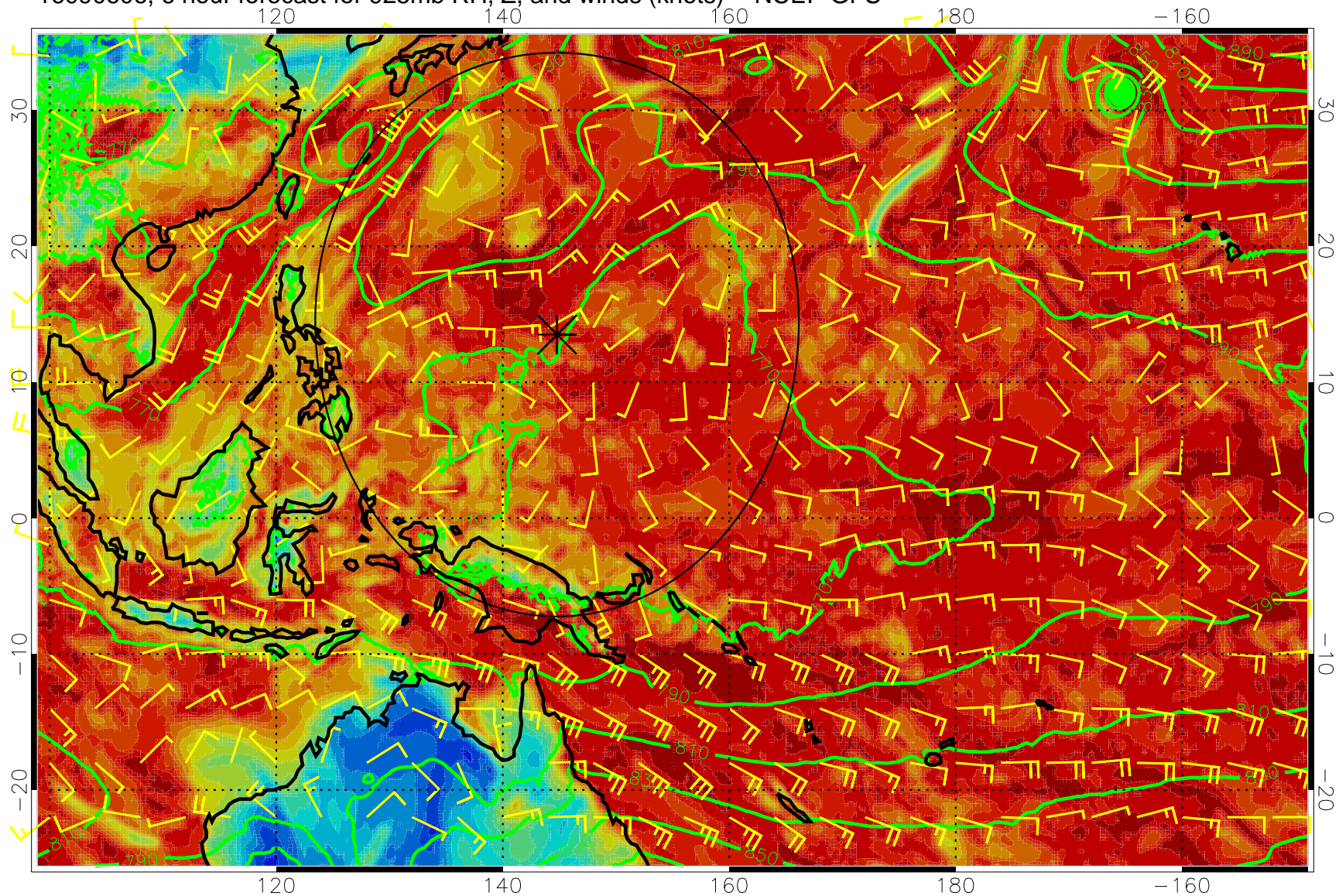
16090606, 6 hour forecast for 925mb RH, Z, and winds (knots) -- NCEP GFS
