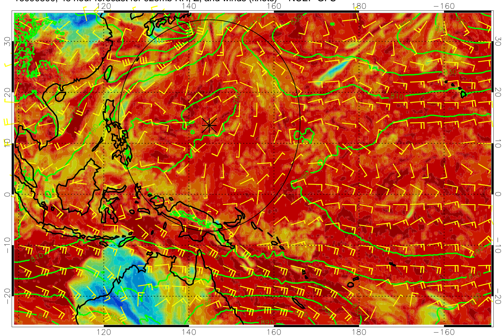
16090800, 48 hour forecast for 925mb RH, Z, and winds (knots) -- NCEP GFS
