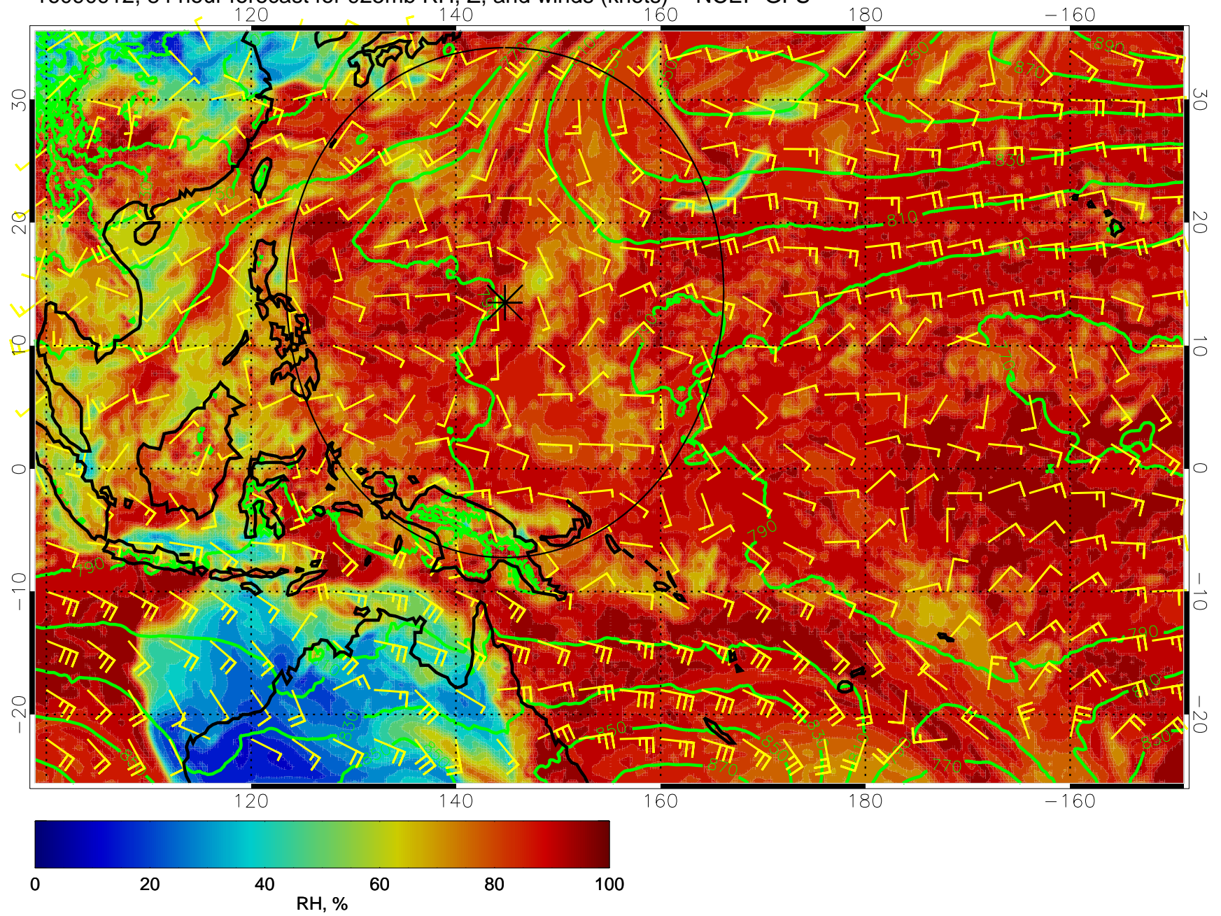
16090912, 84 hour forecast for 925mb RH, Z, and winds (knots) -- NCEP GFS
