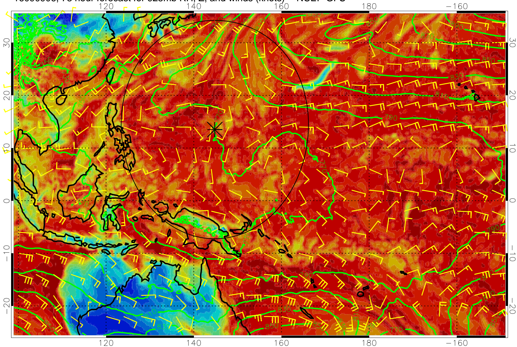
16090906, 78 hour forecast for 925mb RH, Z, and winds (knots) -- NCEP GFS
