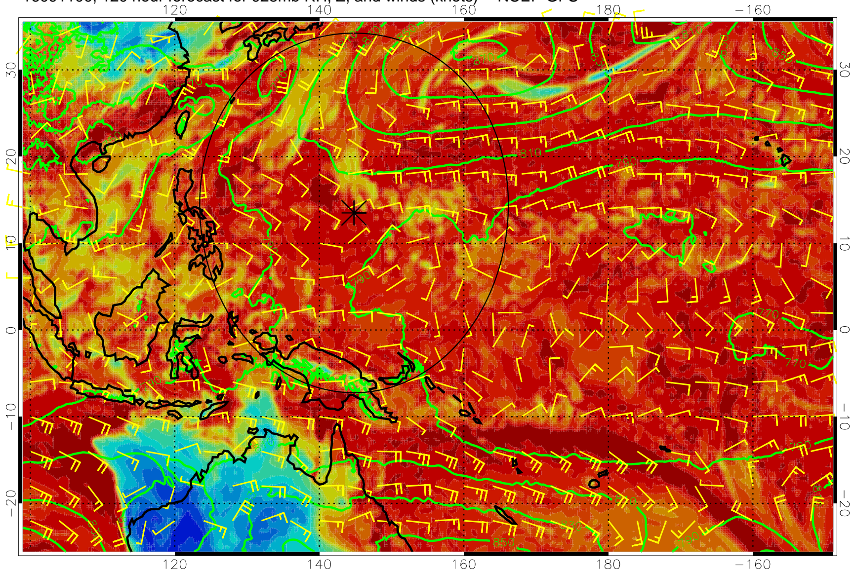
16091100, 120 hour forecast for 925mb RH, Z, and winds (knots) -- NCEP GFS
