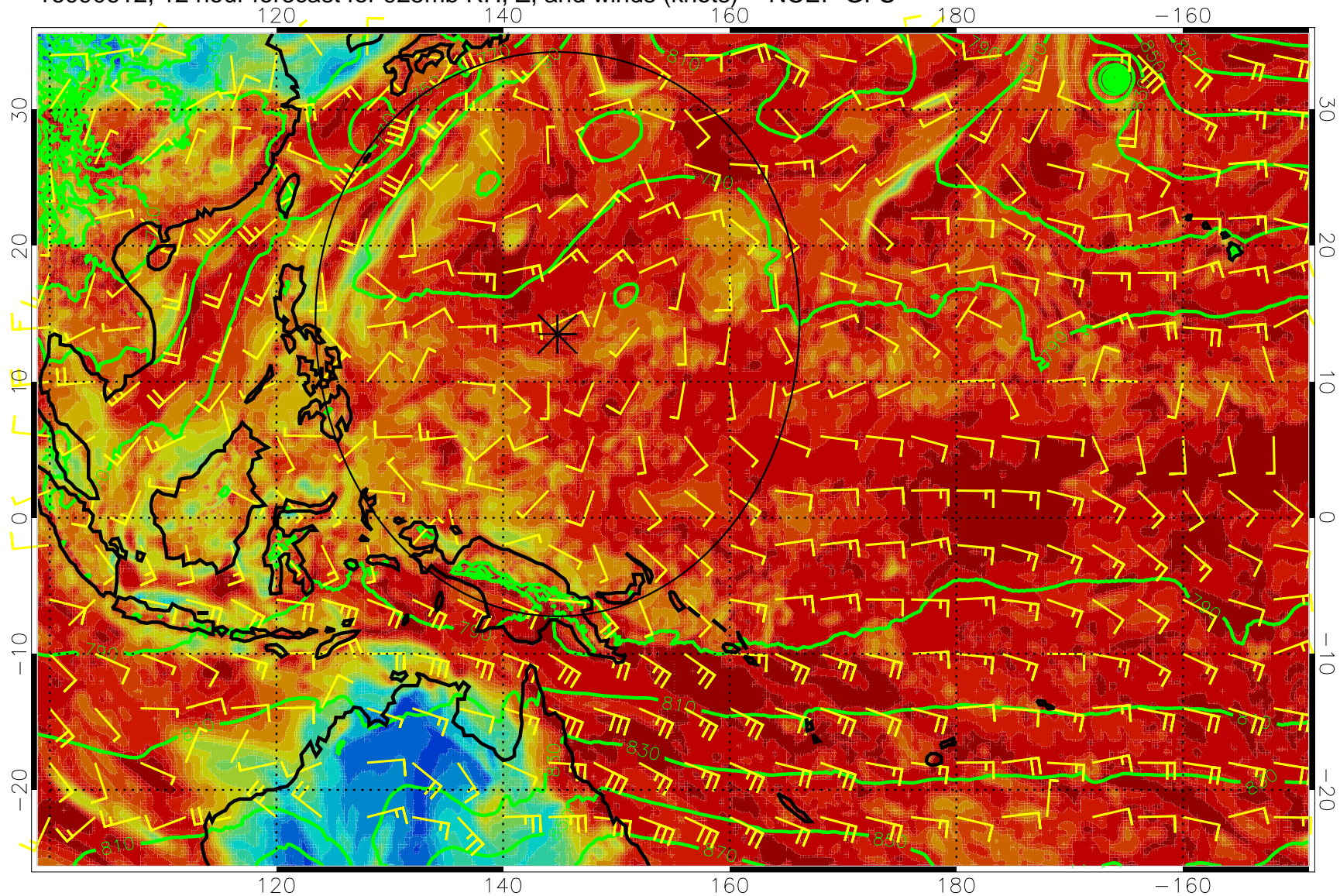
16090612, 12 hour forecast for 925mb RH, Z, and winds (knots) -- NCEP GFS
