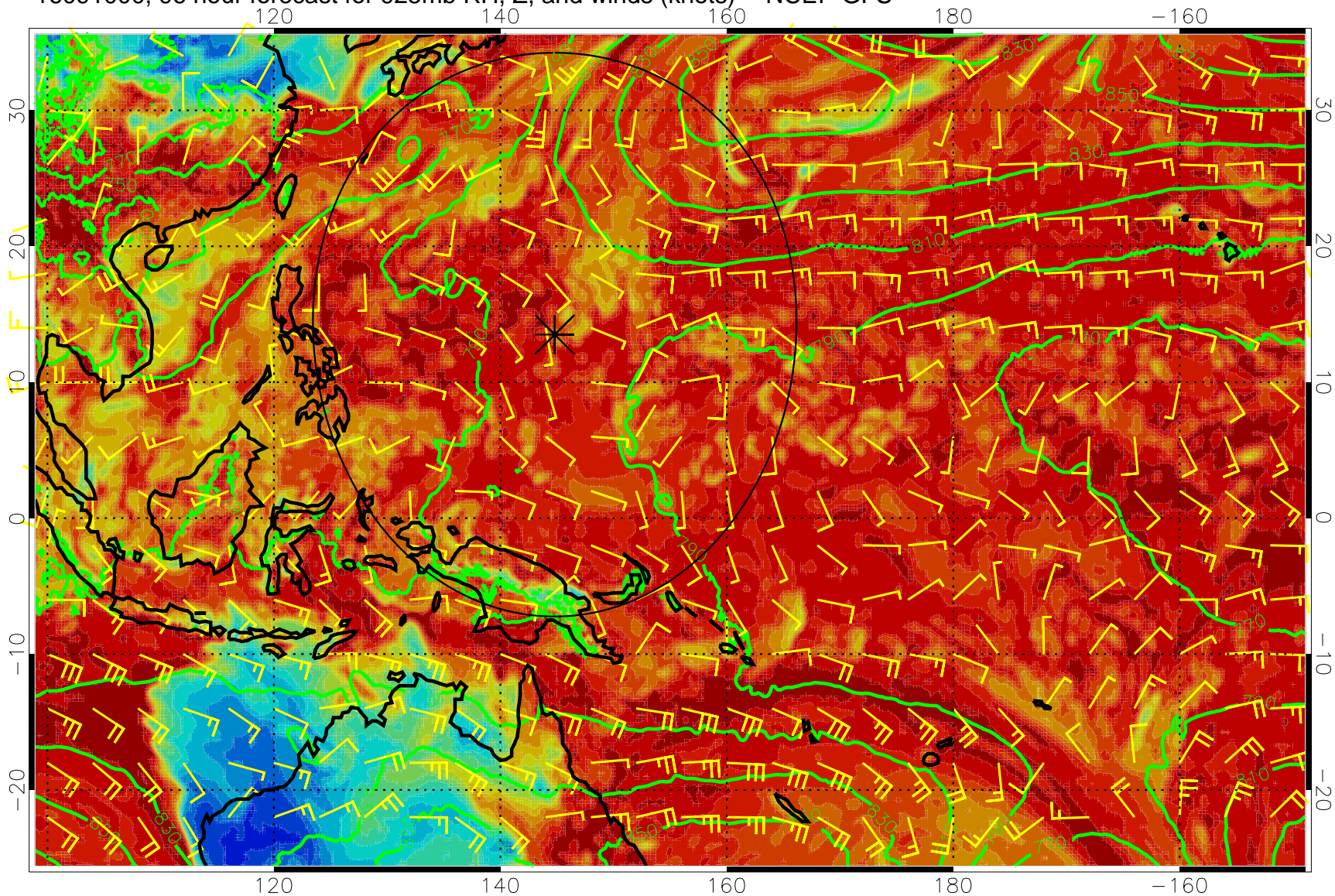
16091000, 96 hour forecast for 925mb RH, Z, and winds (knots) -- NCEP GFS
