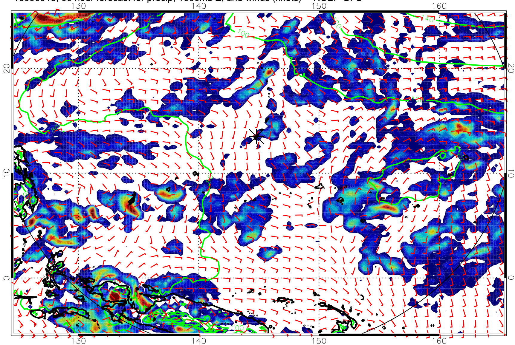
16090918, 90 hour forecast for precip, 1000mb Z, and winds (knots) -- NCEP GFS
