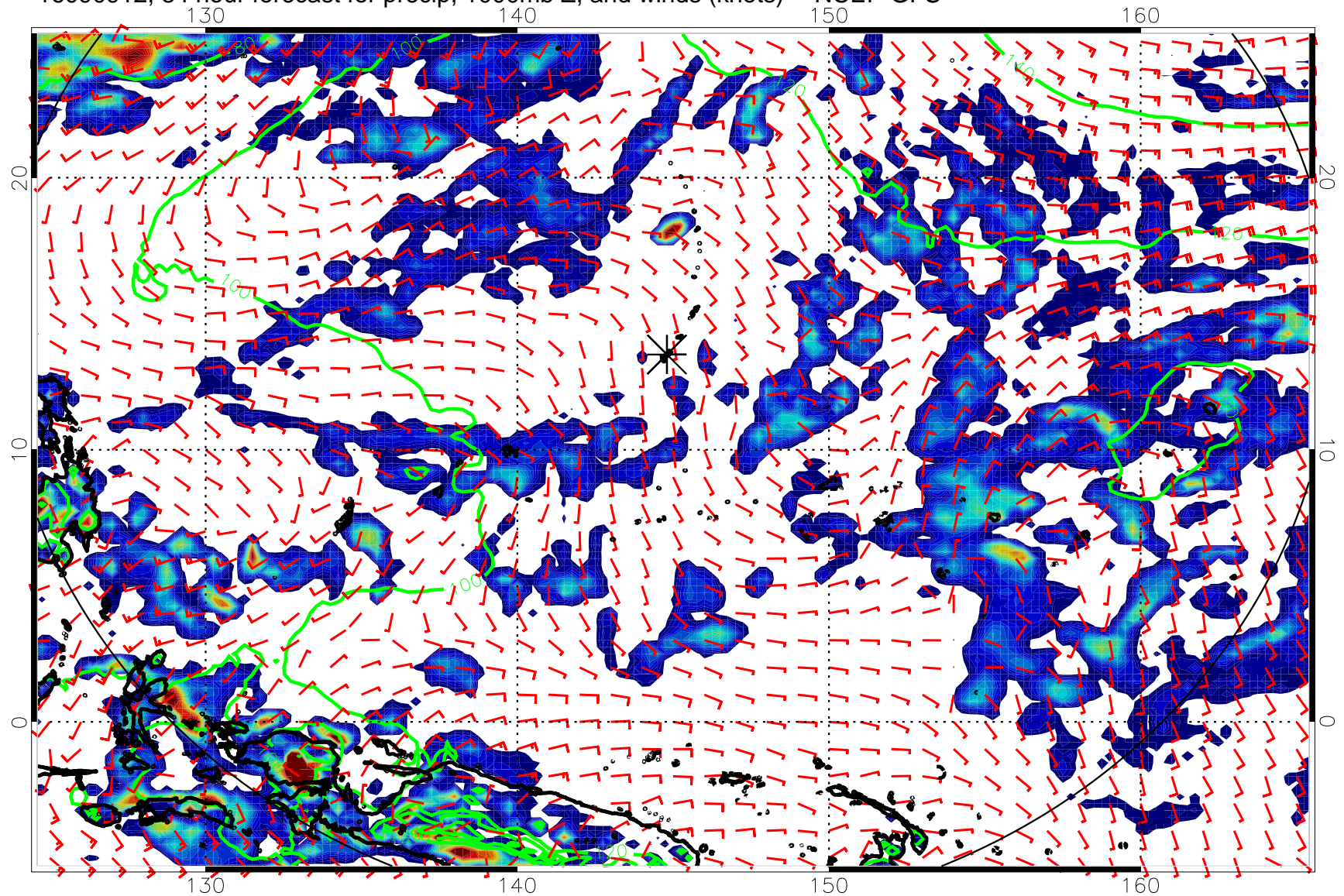
16090912, 84 hour forecast for precip, 1000mb Z, and winds (knots) -- NCEP GFS
