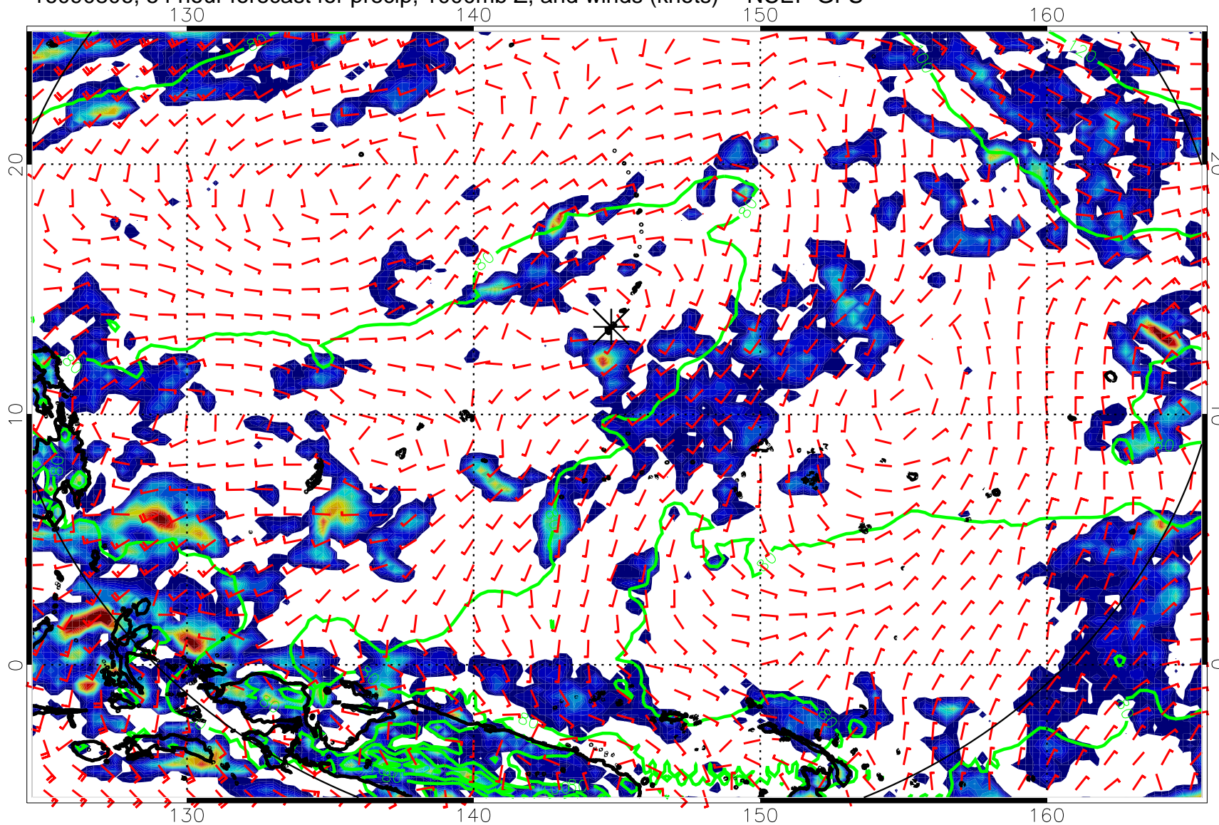
16090806, 54 hour forecast for precip, 1000mb Z, and winds (knots) -- NCEP GFS
