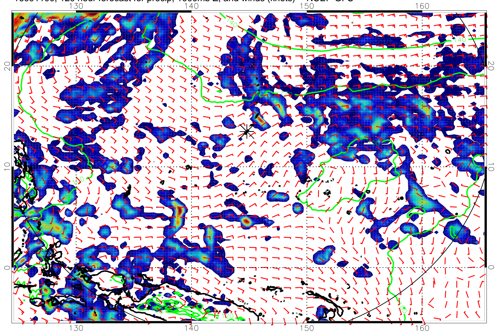
16091100, 120 hour forecast for precip, 1000mb Z, and winds (knots) -- NCEP GFS
