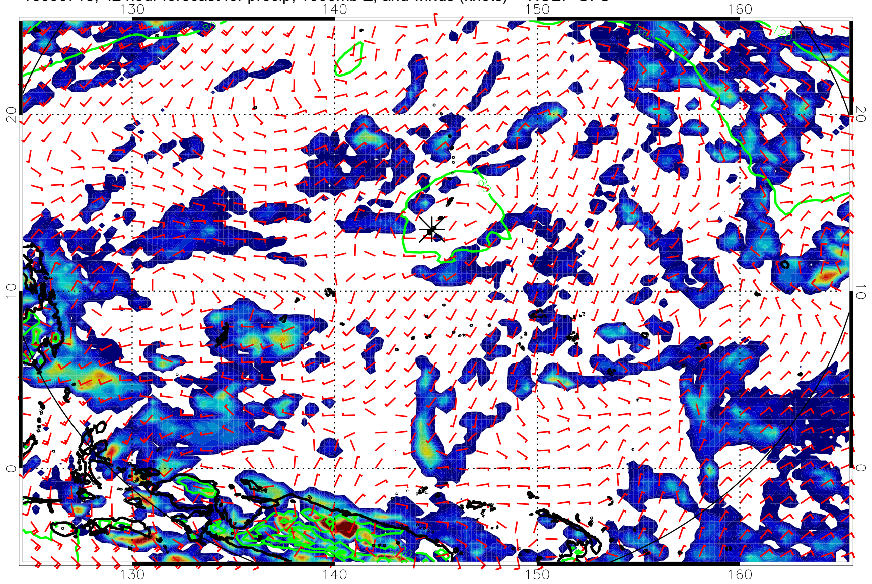
16090718, 42 hour forecast for precip, 1000mb Z, and winds (knots) -- NCEP GFS
