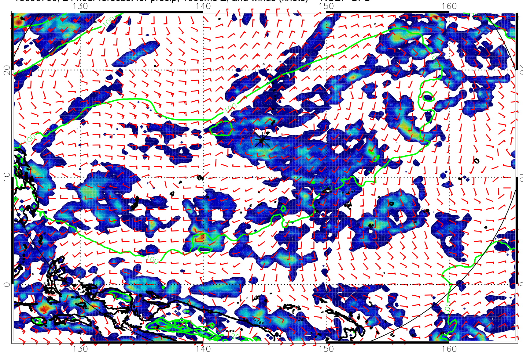
16090700, 24 hour forecast for precip, 1000mb Z, and winds (knots) -- NCEP GFS
