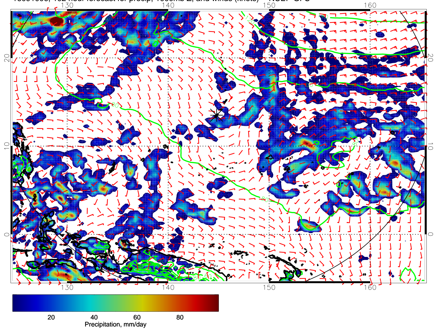
16091006, 102 hour forecast for precip, 1000mb Z, and winds (knots) -- NCEP GFS
