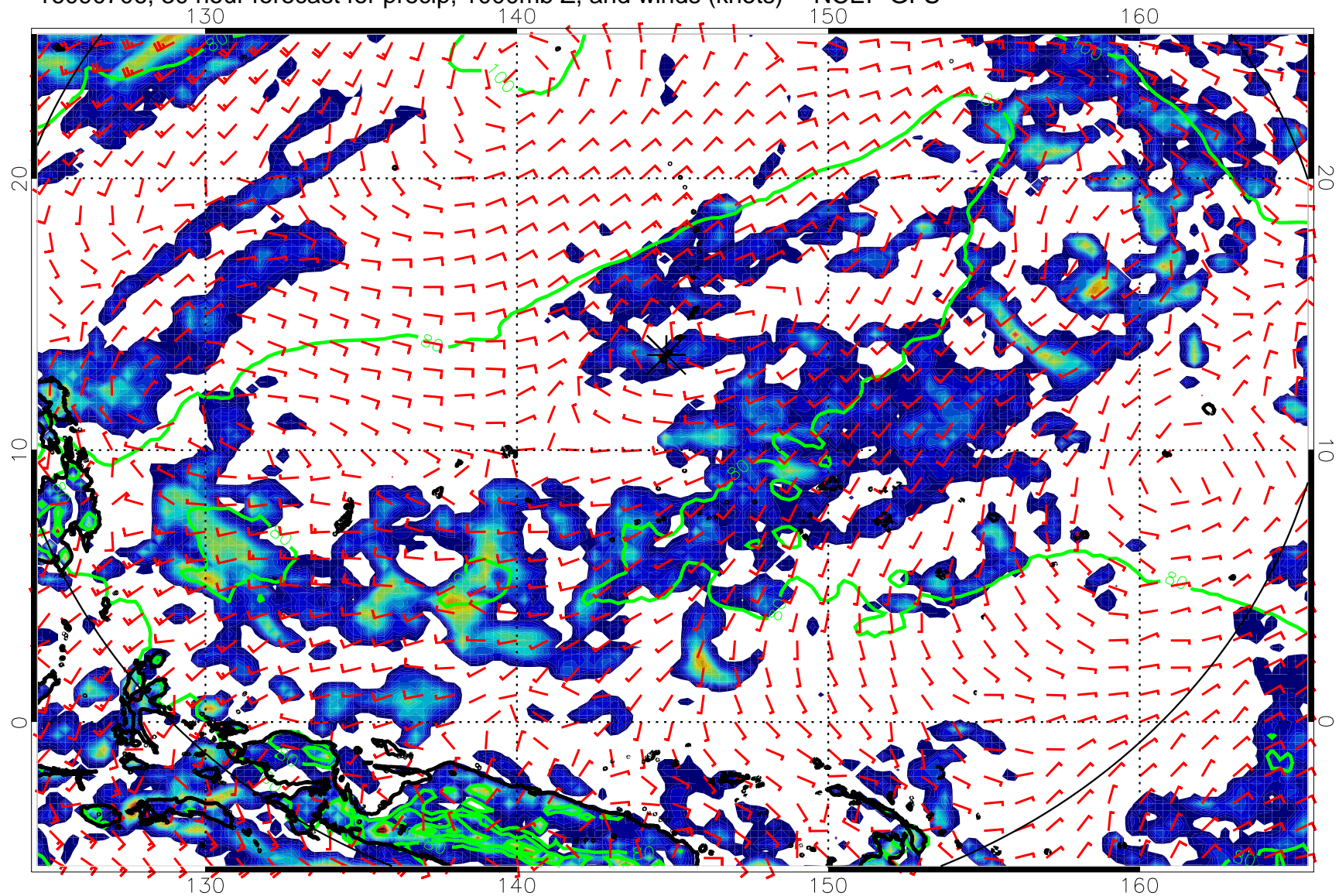
16090706, 30 hour forecast for precip, 1000mb Z, and winds (knots) -- NCEP GFS
