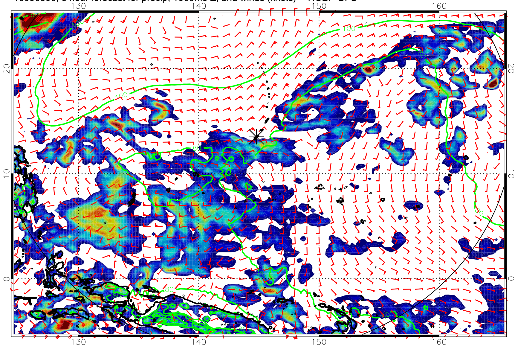
16090606, 6 hour forecast for precip, 1000mb Z, and winds (knots) -- NCEP GFS
