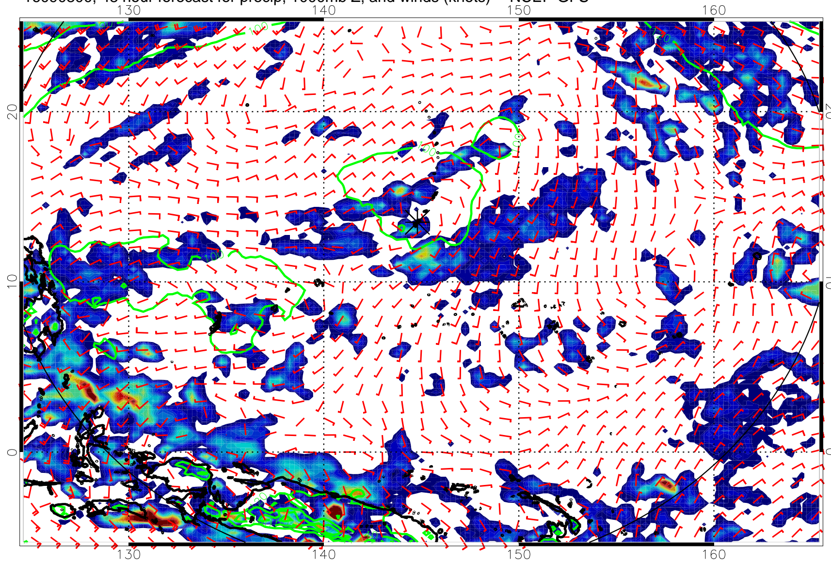
16090800, 48 hour forecast for precip, 1000mb Z, and winds (knots) -- NCEP GFS
