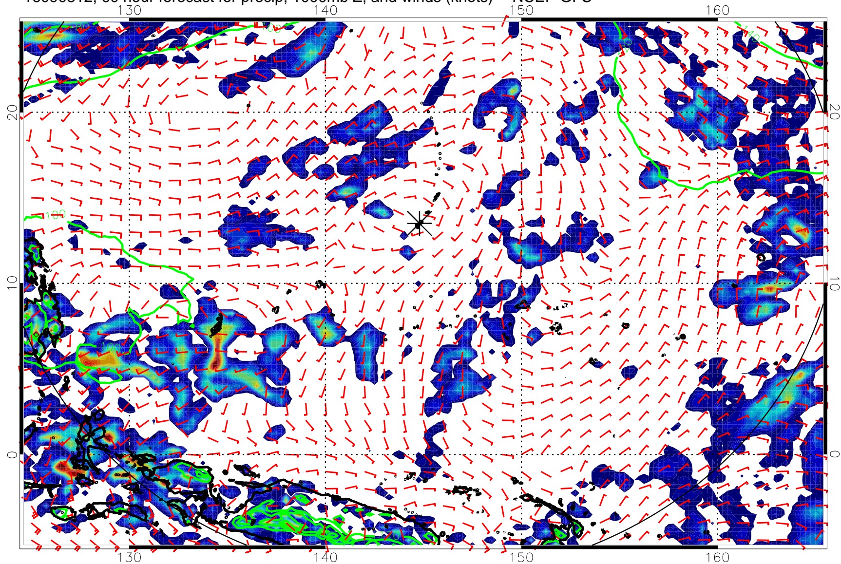
16090812, 60 hour forecast for precip, 1000mb Z, and winds (knots) -- NCEP GFS
