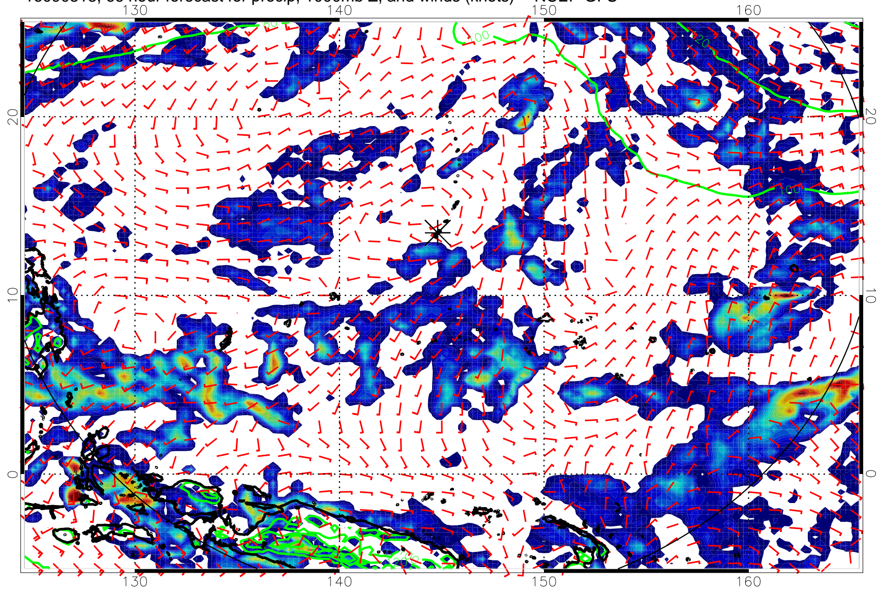
16090818, 66 hour forecast for precip, 1000mb Z, and winds (knots) -- NCEP GFS
