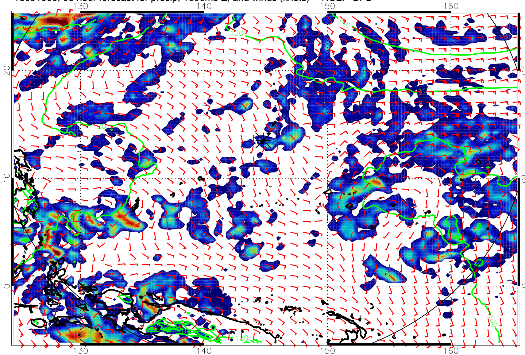
16091000, 96 hour forecast for precip, 1000mb Z, and winds (knots) -- NCEP GFS
