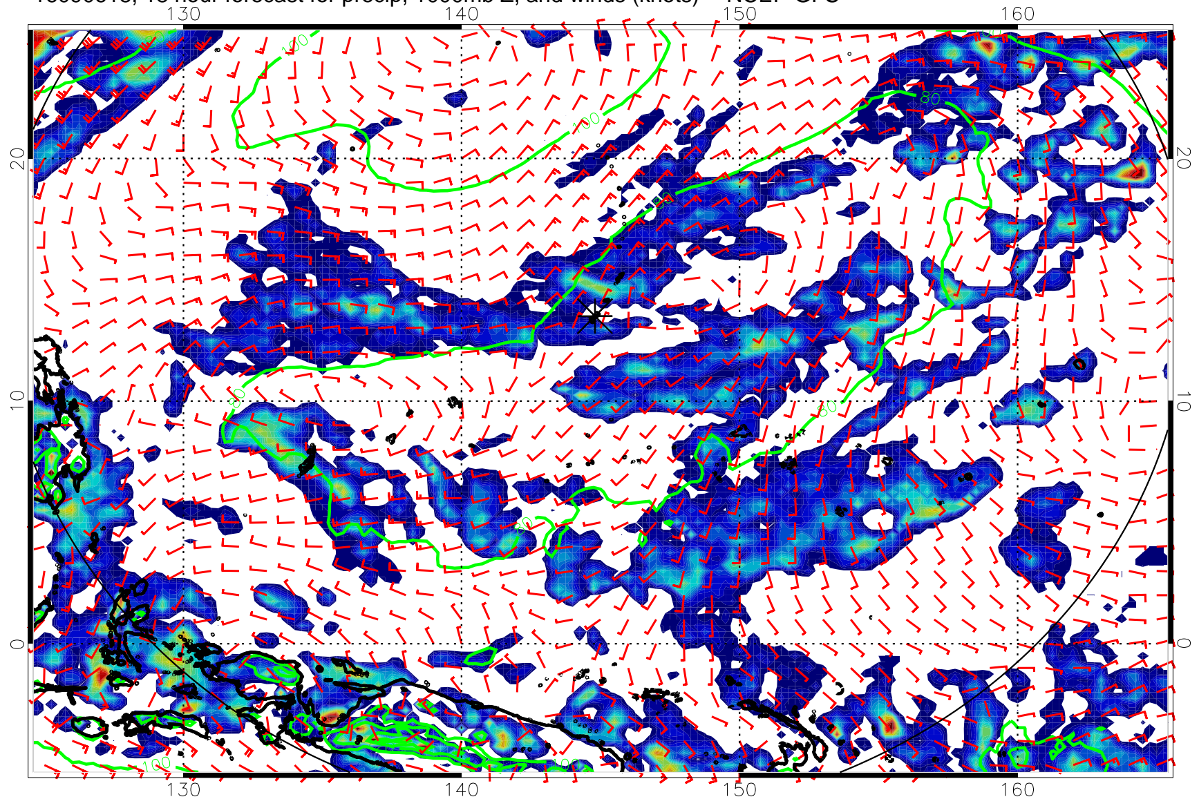
16090618, 18 hour forecast for precip, 1000mb Z, and winds (knots) -- NCEP GFS
