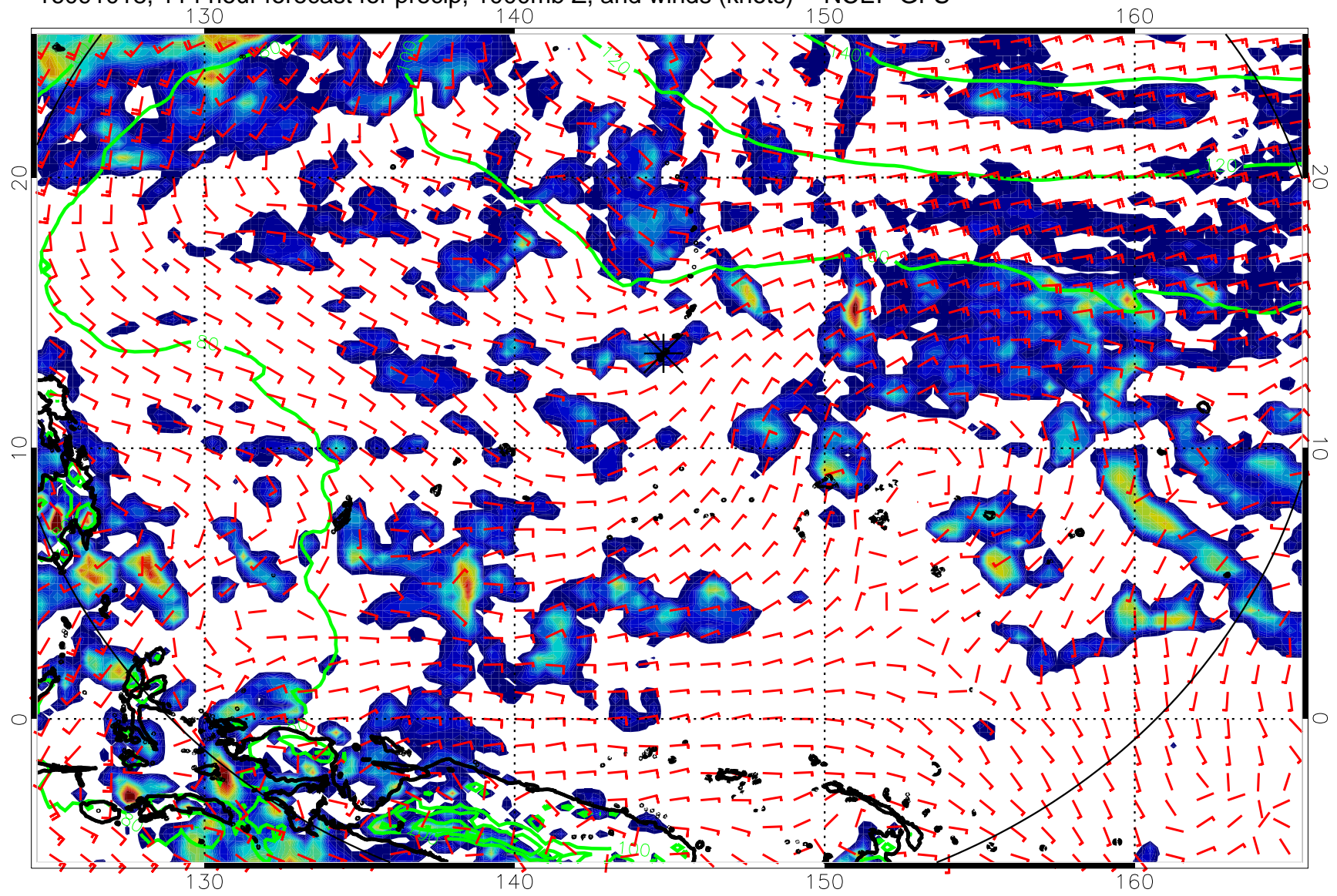
16091018, 114 hour forecast for precip, 1000mb Z, and winds (knots) -- NCEP GFS
