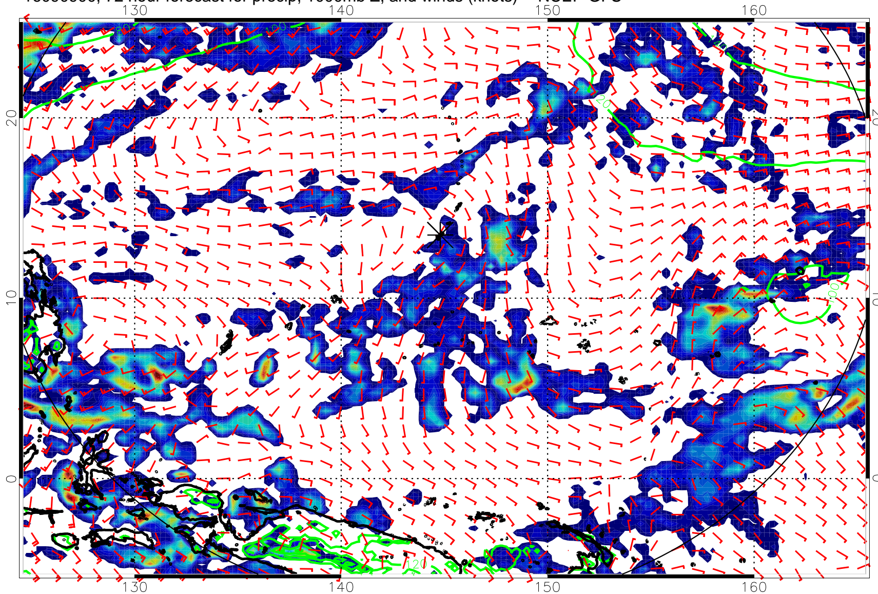
16090900, 72 hour forecast for precip, 1000mb Z, and winds (knots) -- NCEP GFS
