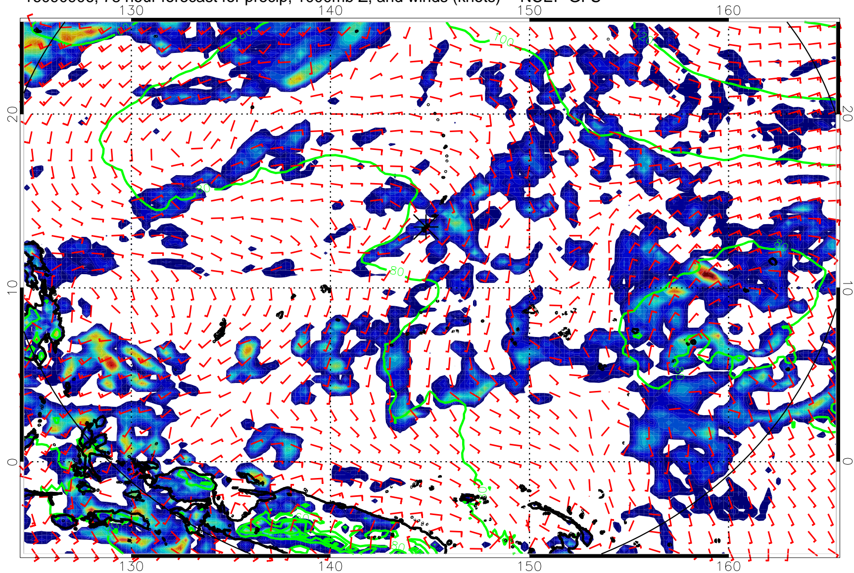
16090906, 78 hour forecast for precip, 1000mb Z, and winds (knots) -- NCEP GFS
