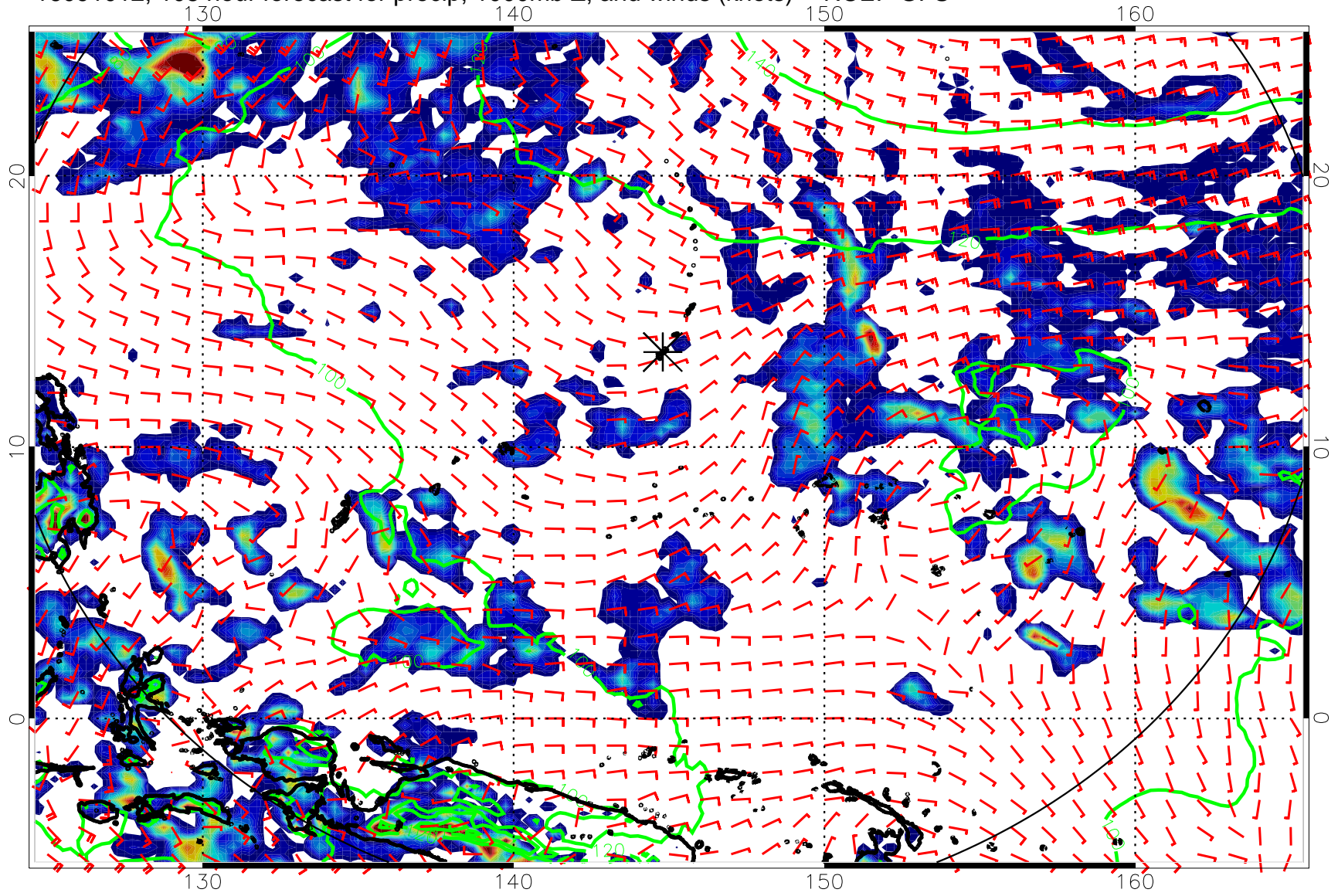
16091012, 108 hour forecast for precip, 1000mb Z, and winds (knots) -- NCEP GFS
