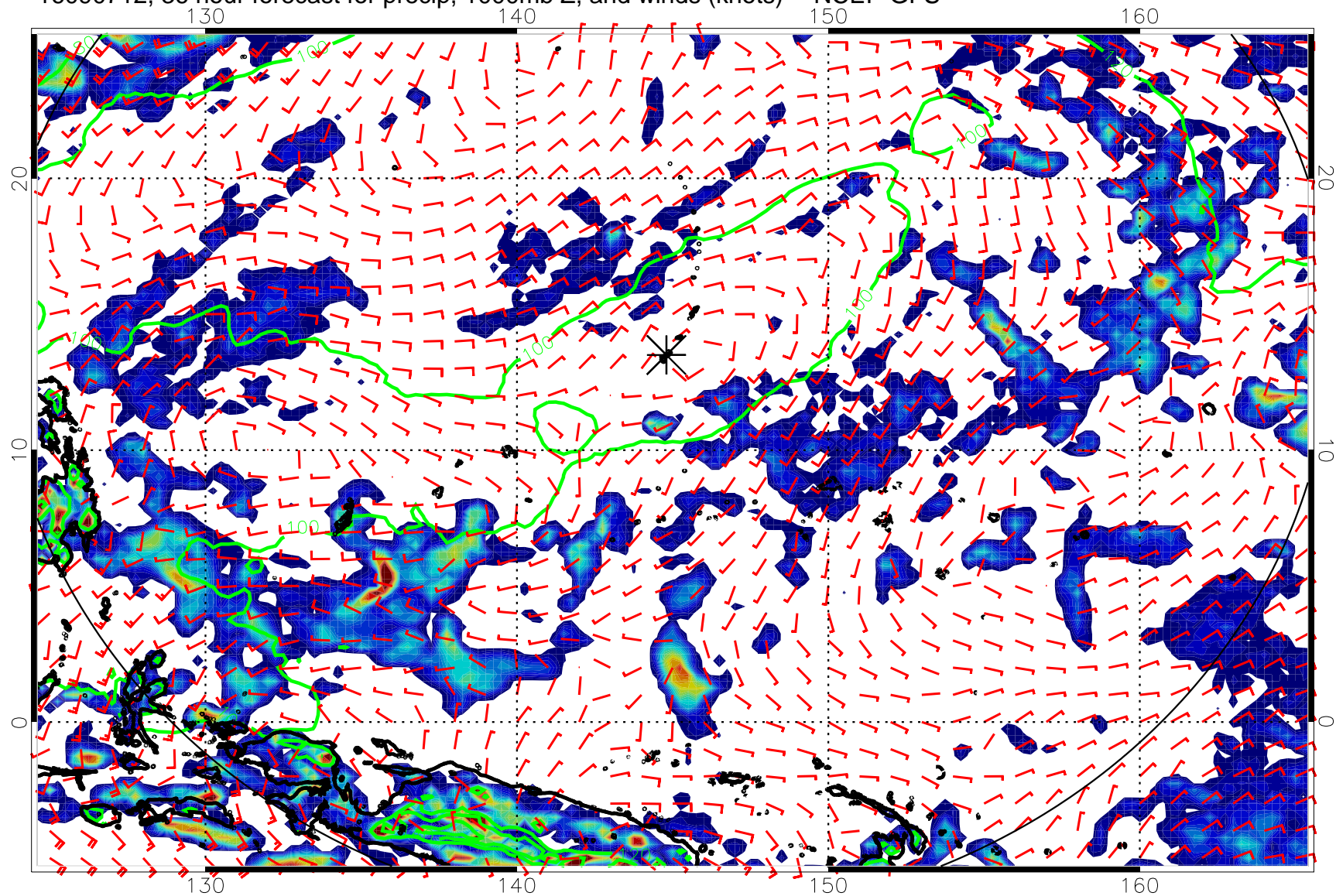
16090712, 36 hour forecast for precip, 1000mb Z, and winds (knots) -- NCEP GFS
