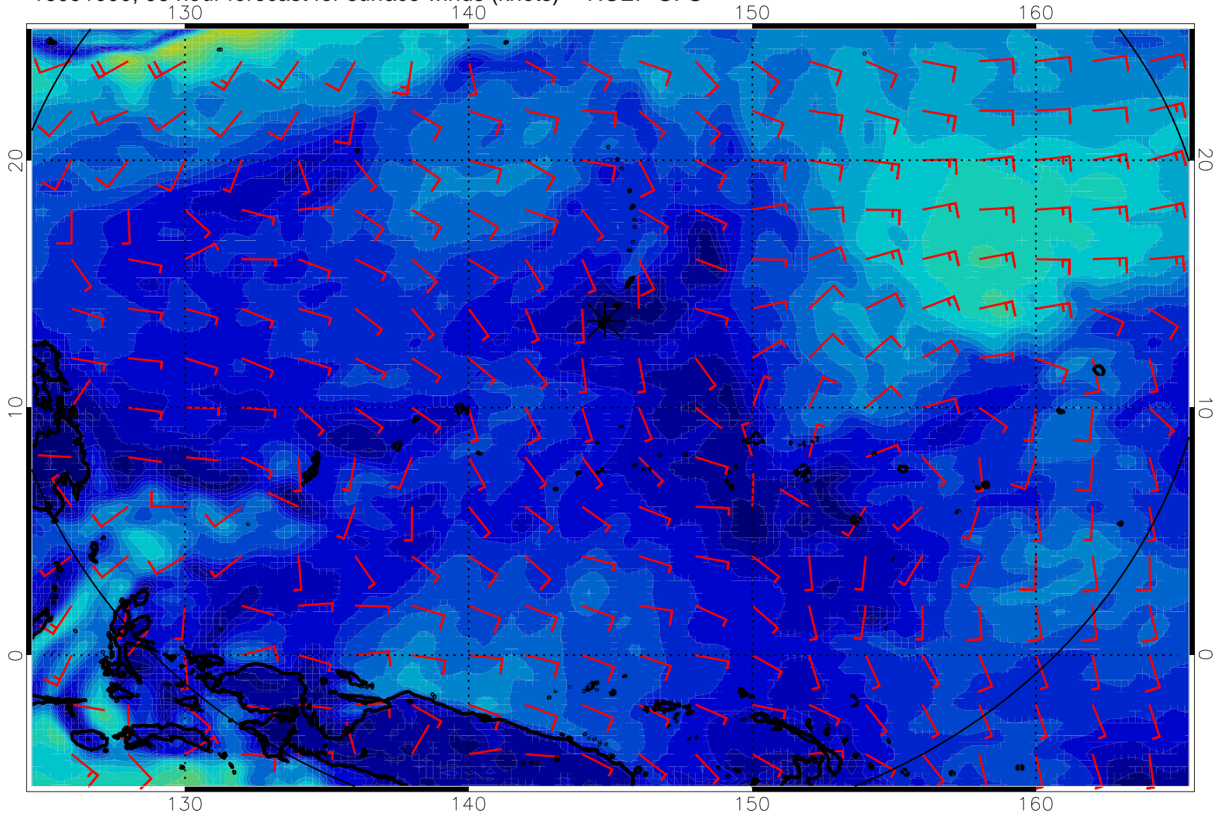
16091000, 96 hour forecast for surface winds (knots) -- NCEP GFS
