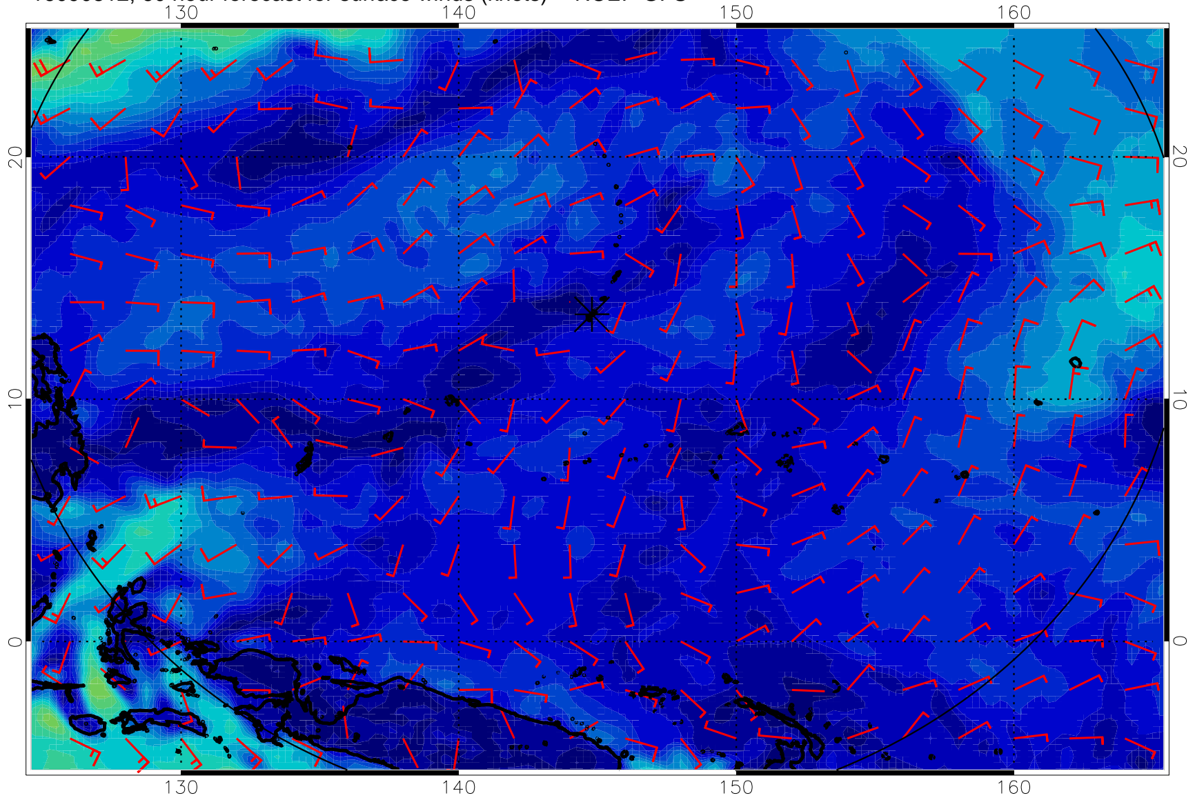
16090812, 60 hour forecast for surface winds (knots) -- NCEP GFS
