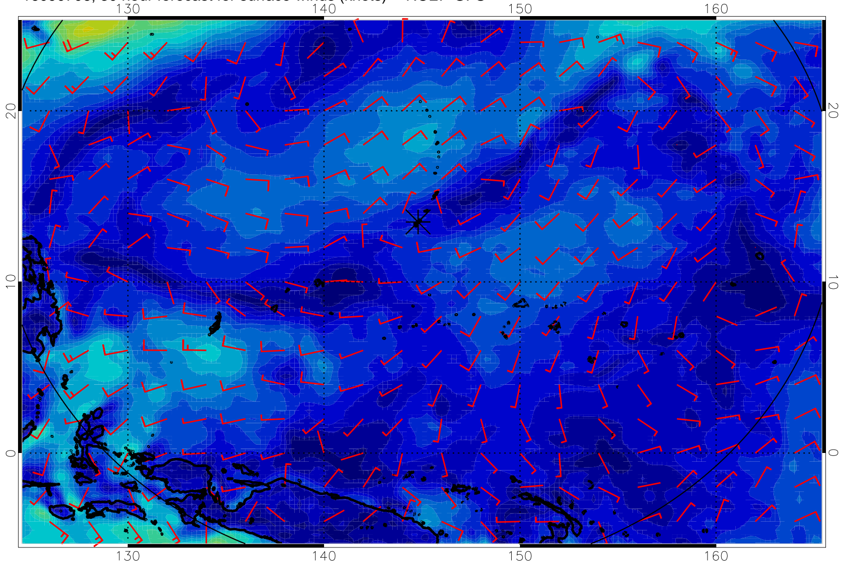
16090706, 30 hour forecast for surface winds (knots) -- NCEP GFS
