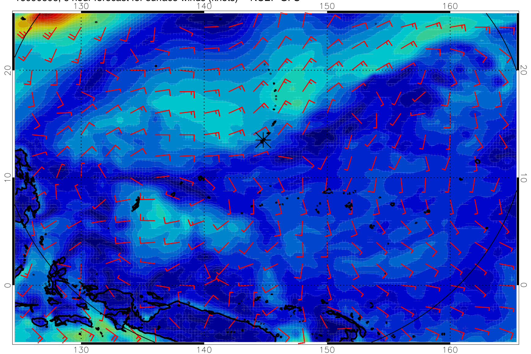
16090606, 6 hour forecast for surface winds (knots) -- NCEP GFS
