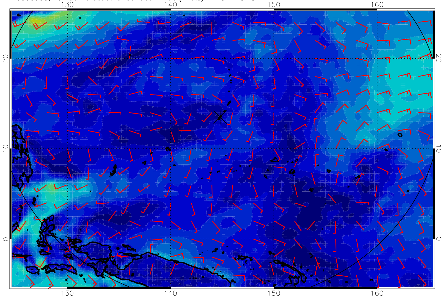
16090906, 78 hour forecast for surface winds (knots) -- NCEP GFS
