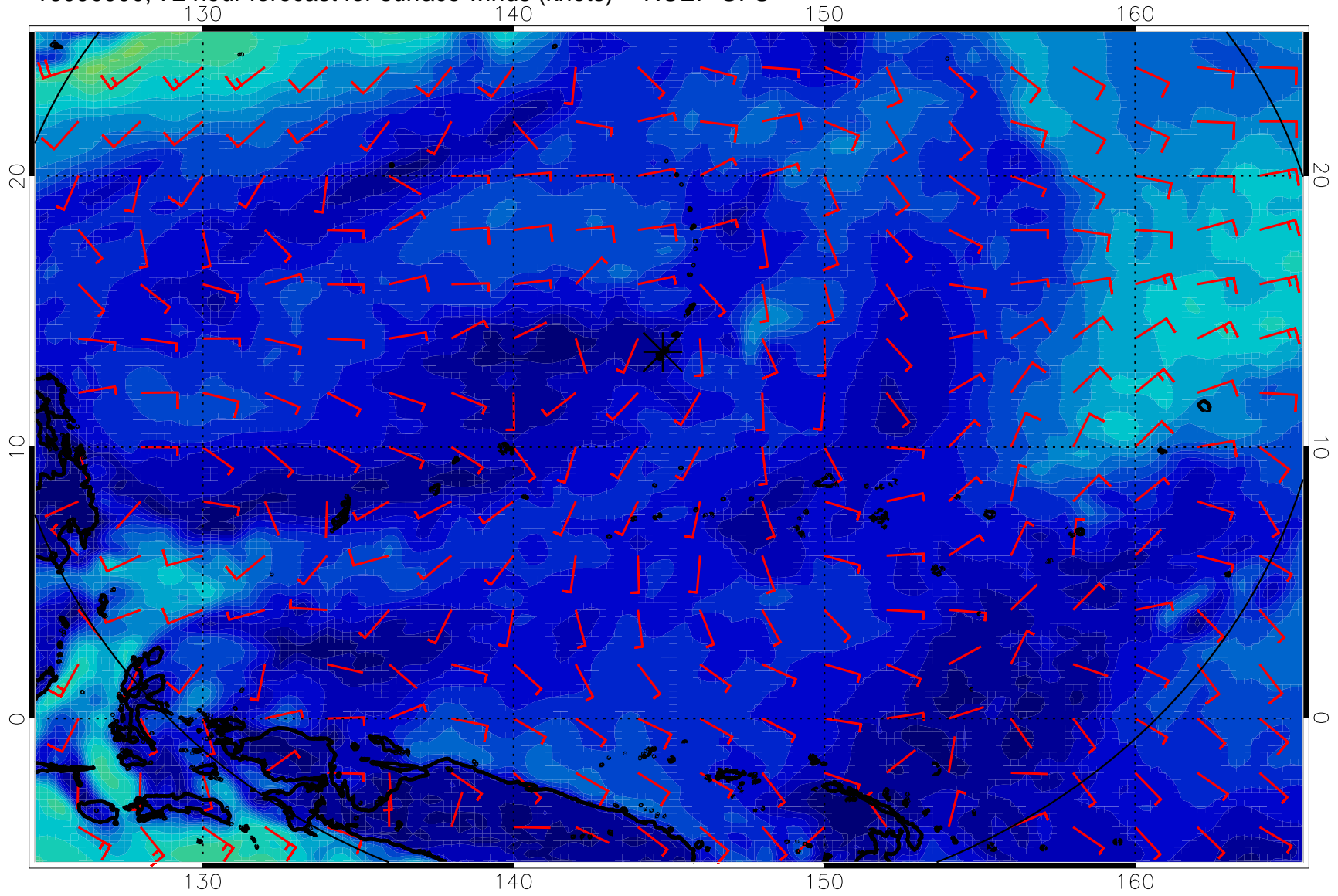
16090900, 72 hour forecast for surface winds (knots) -- NCEP GFS
