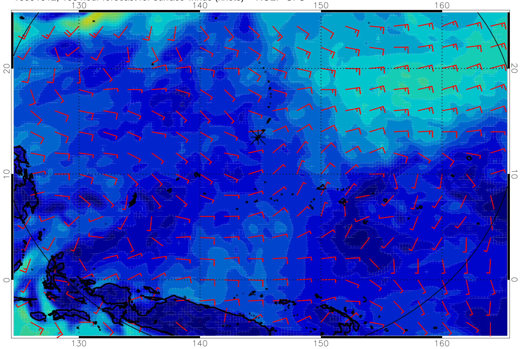
16091012, 108 hour forecast for surface winds (knots) -- NCEP GFS
