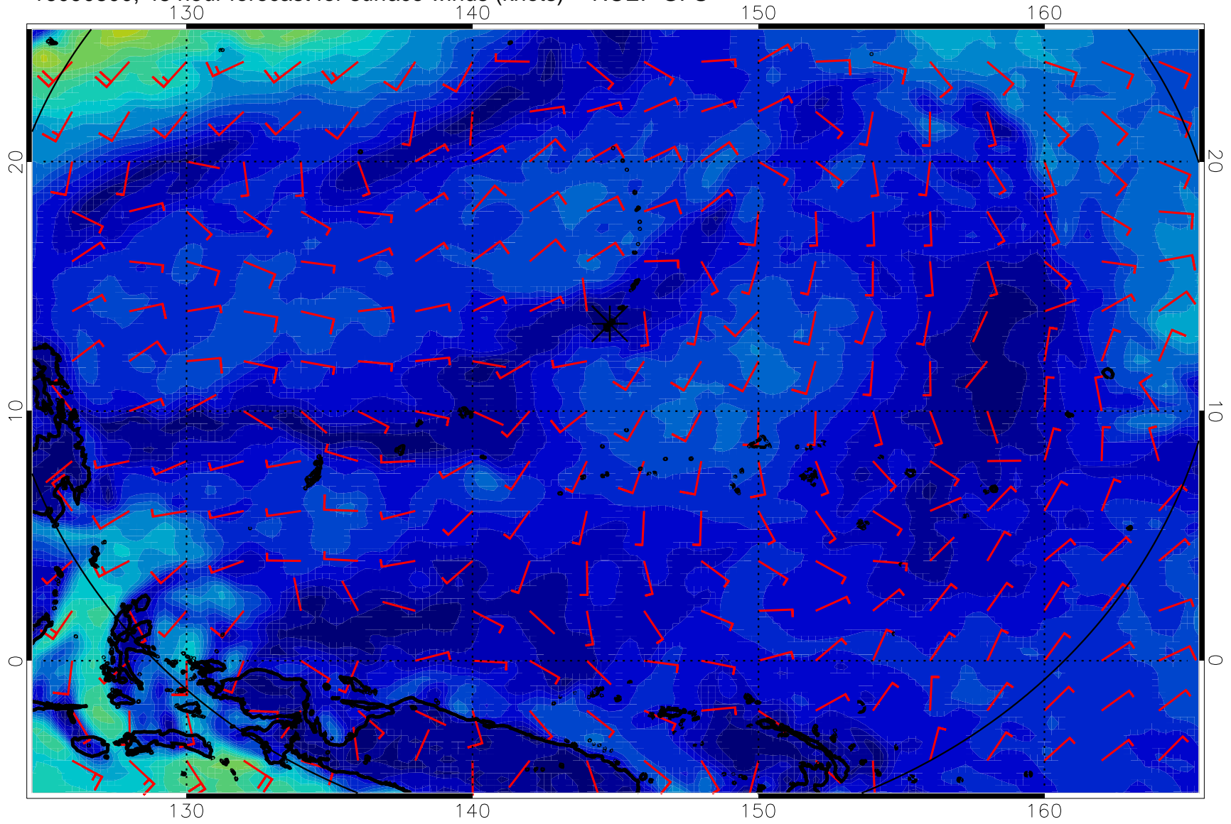
16090800, 48 hour forecast for surface winds (knots) -- NCEP GFS
