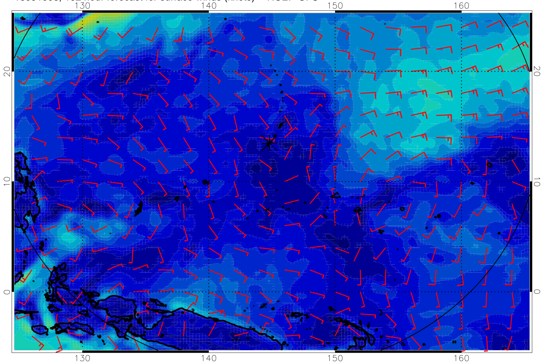
16091006, 102 hour forecast for surface winds (knots) -- NCEP GFS
