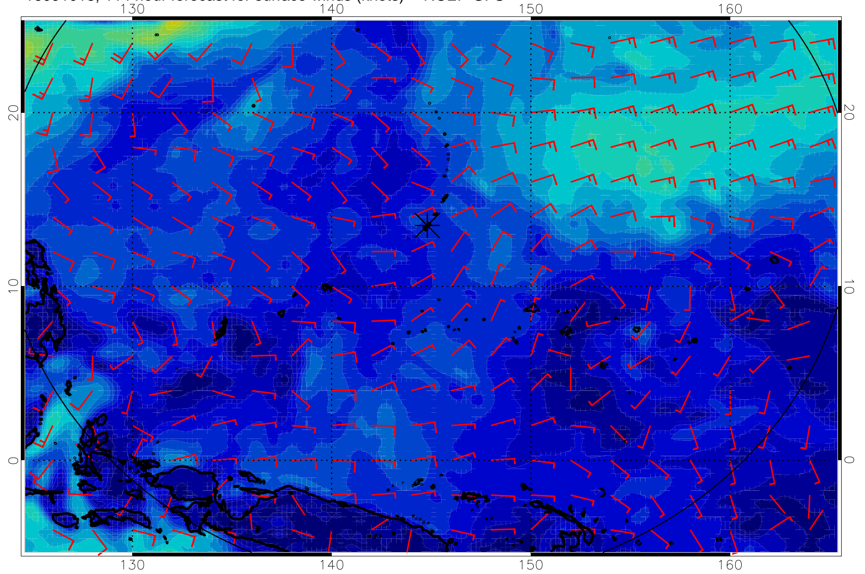
16091018, 114 hour forecast for surface winds (knots) -- NCEP GFS
