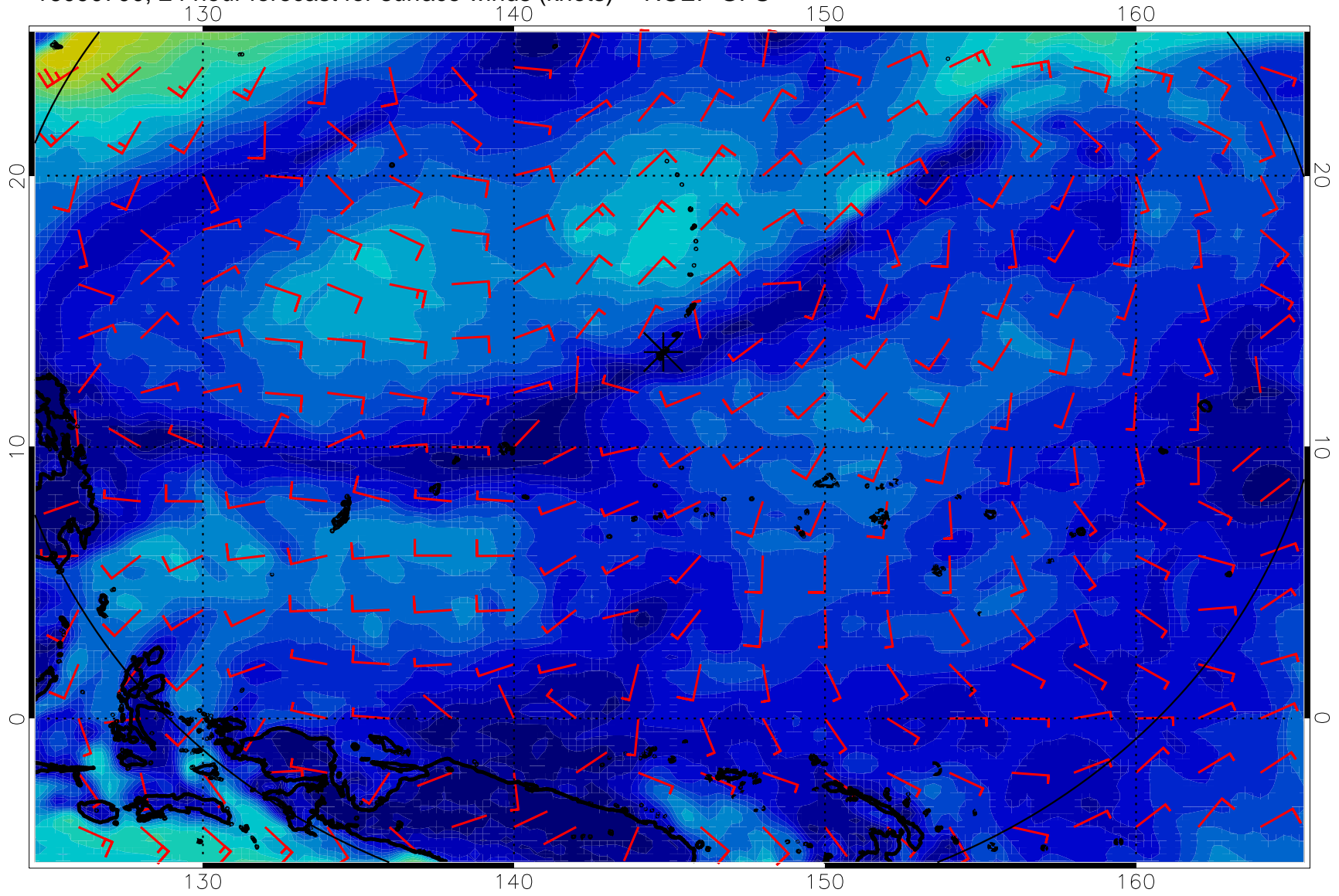
16090700, 24 hour forecast for surface winds (knots) -- NCEP GFS
