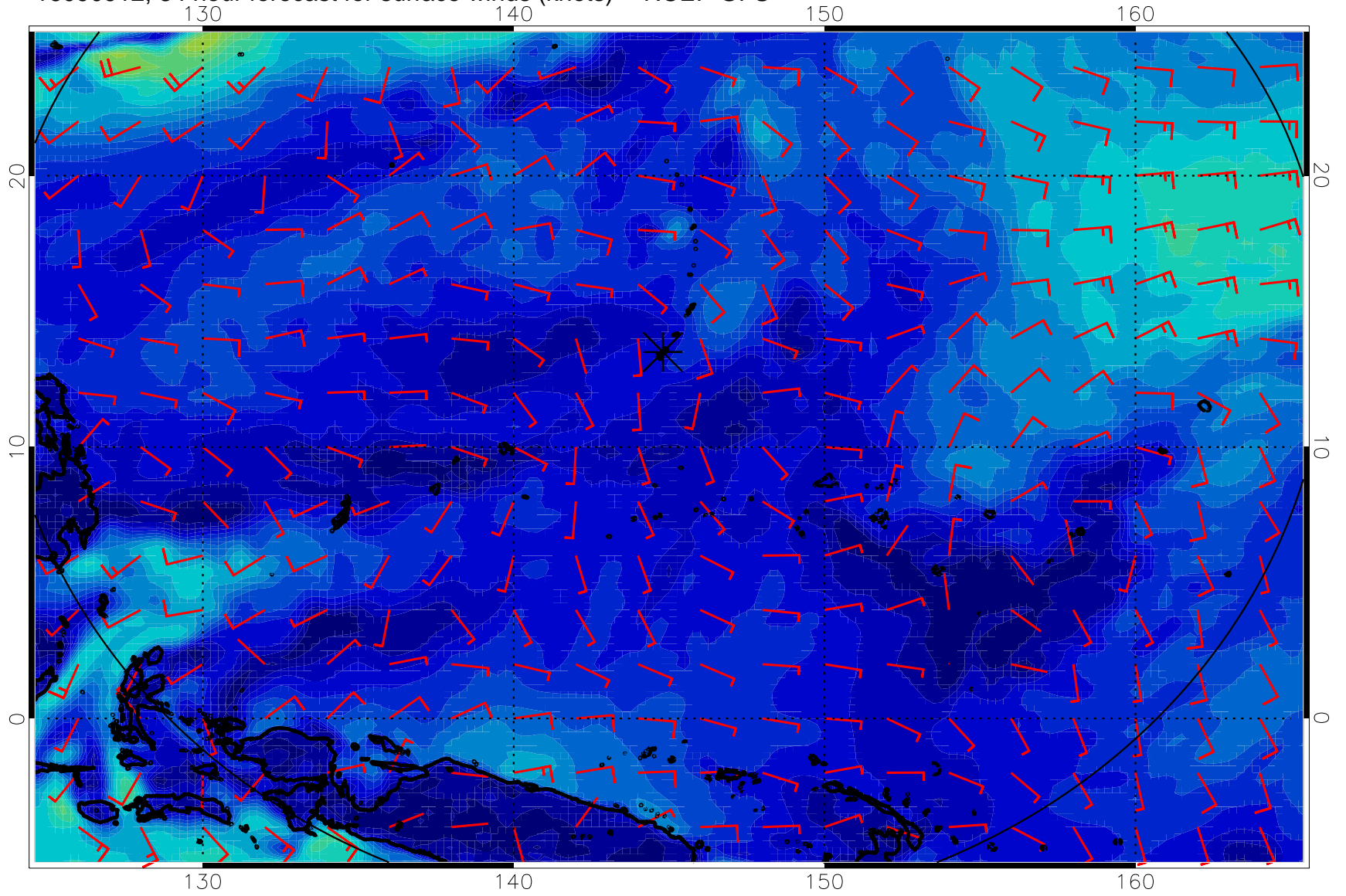
16090912, 84 hour forecast for surface winds (knots) -- NCEP GFS
