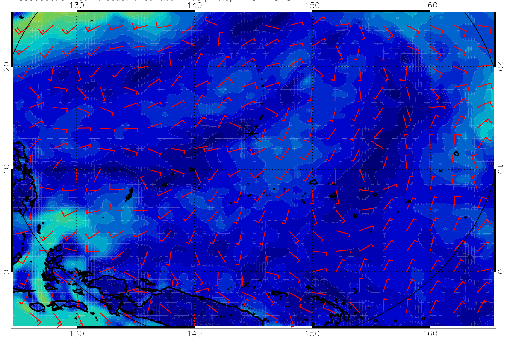
16090806, 54 hour forecast for surface winds (knots) -- NCEP GFS
