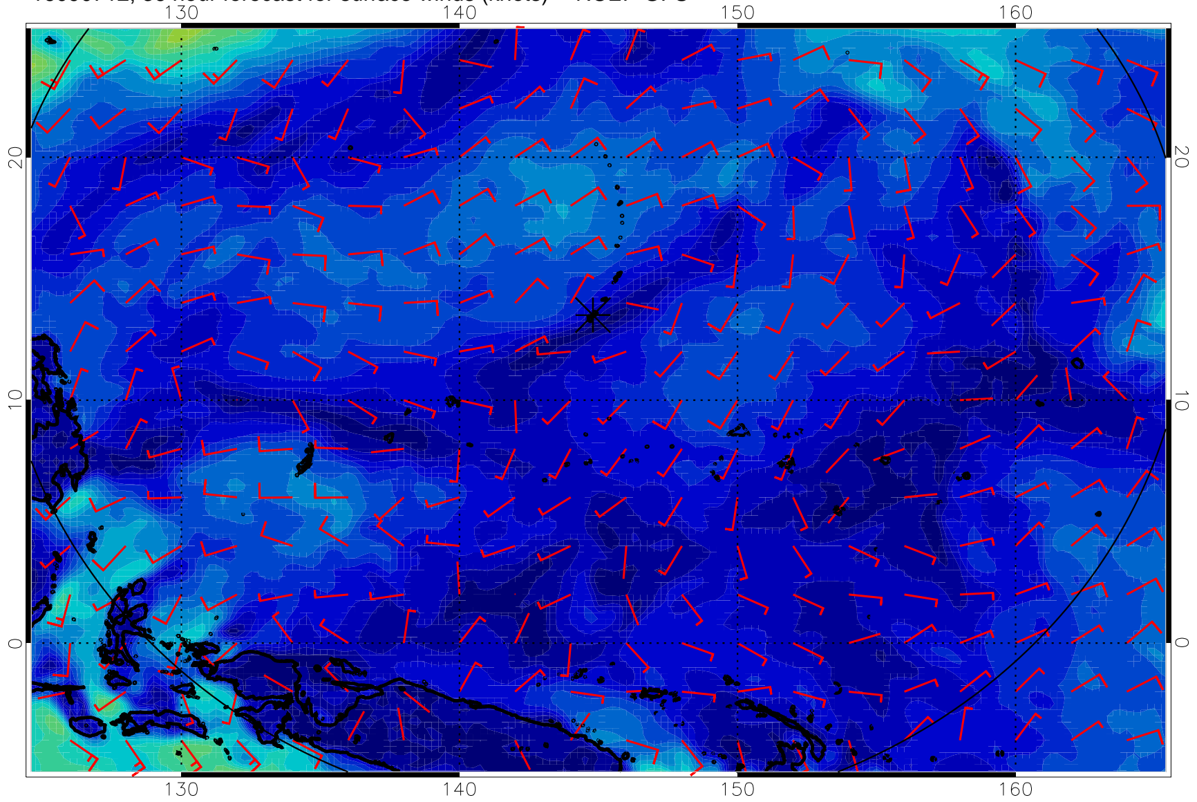
16090712, 36 hour forecast for surface winds (knots) -- NCEP GFS
