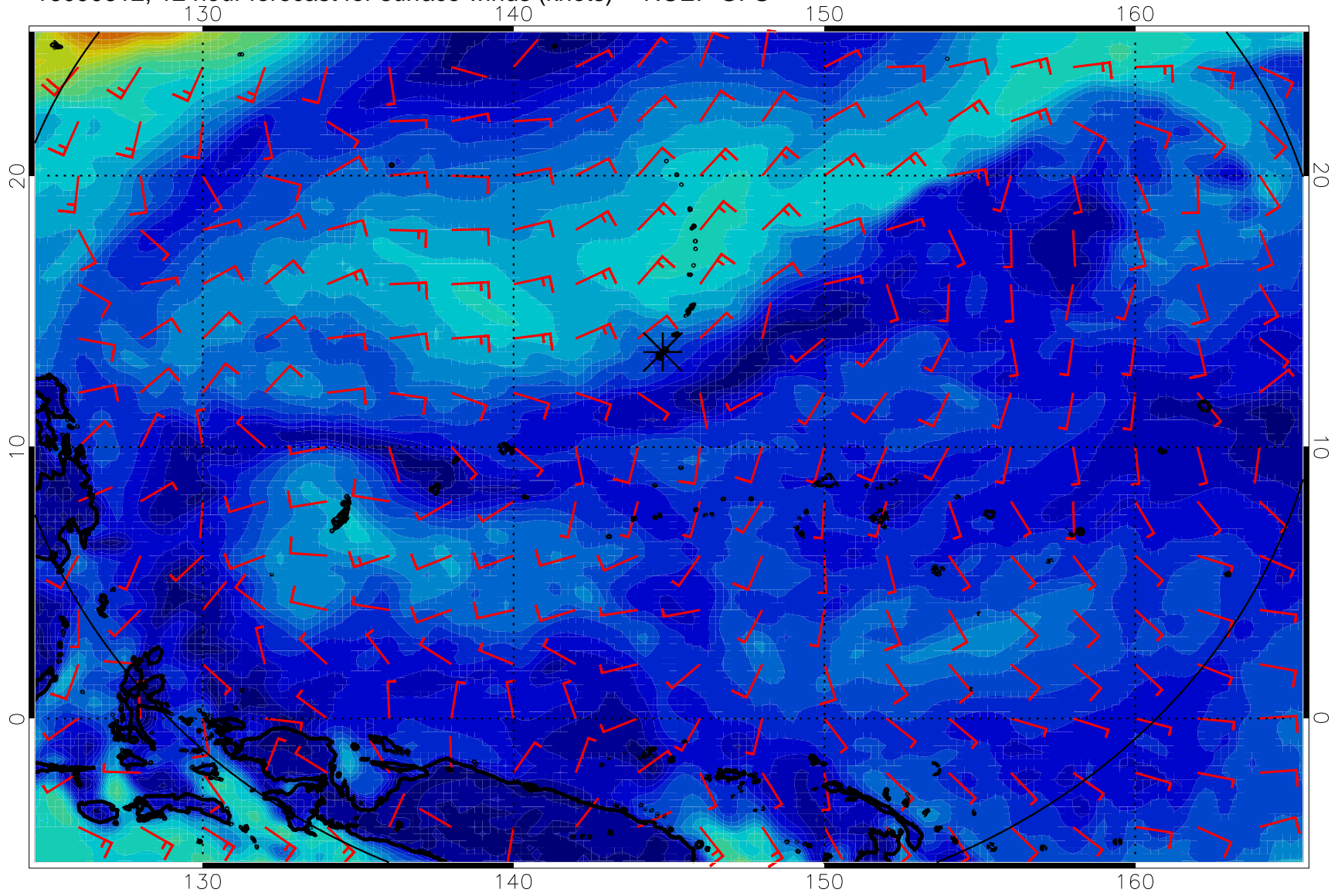
16090612, 12 hour forecast for surface winds (knots) -- NCEP GFS
