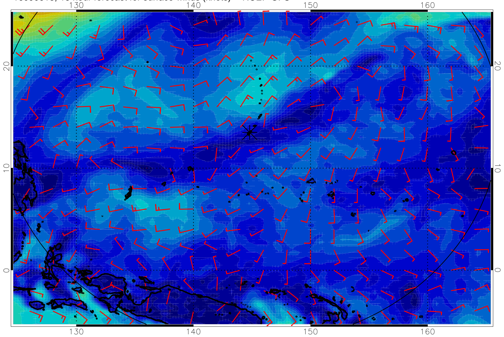
16090618, 18 hour forecast for surface winds (knots) -- NCEP GFS
