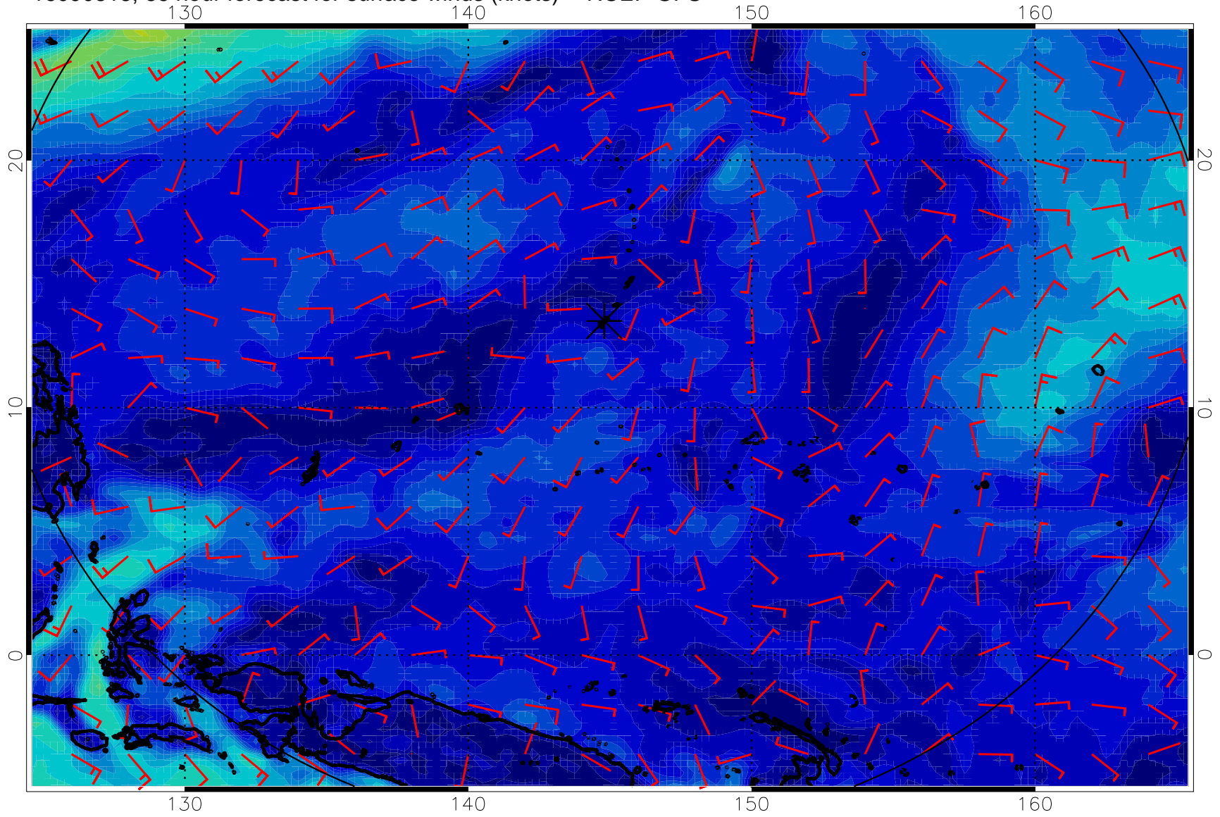
16090818, 66 hour forecast for surface winds (knots) -- NCEP GFS
