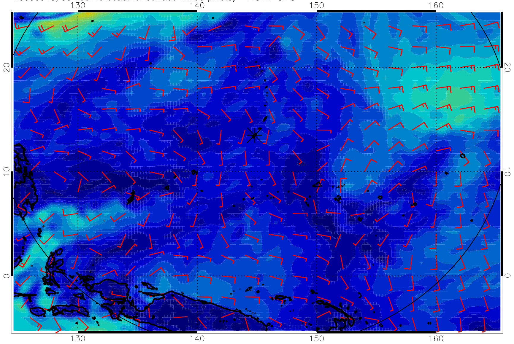
16090918, 90 hour forecast for surface winds (knots) -- NCEP GFS
