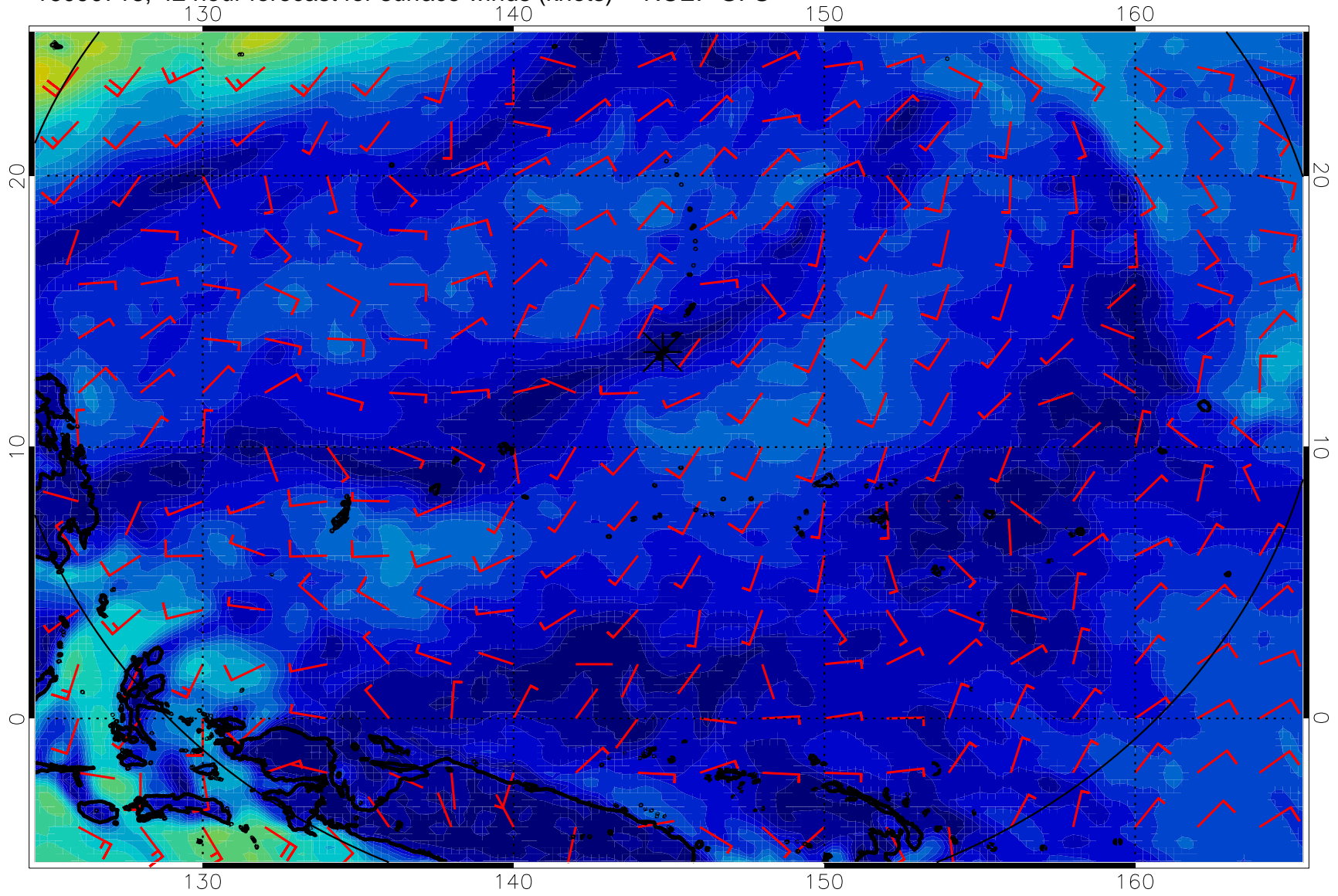
16090718, 42 hour forecast for surface winds (knots) -- NCEP GFS
