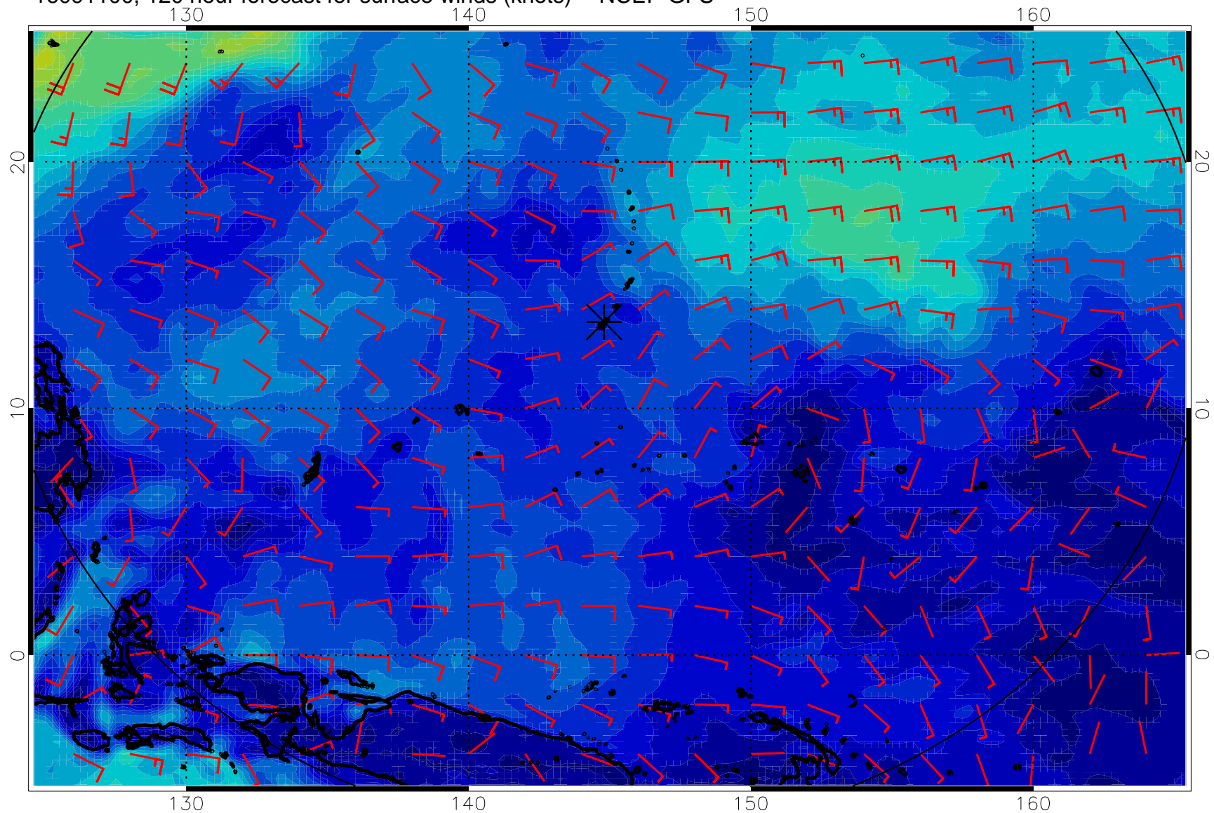
16091100, 120 hour forecast for surface winds (knots) -- NCEP GFS
