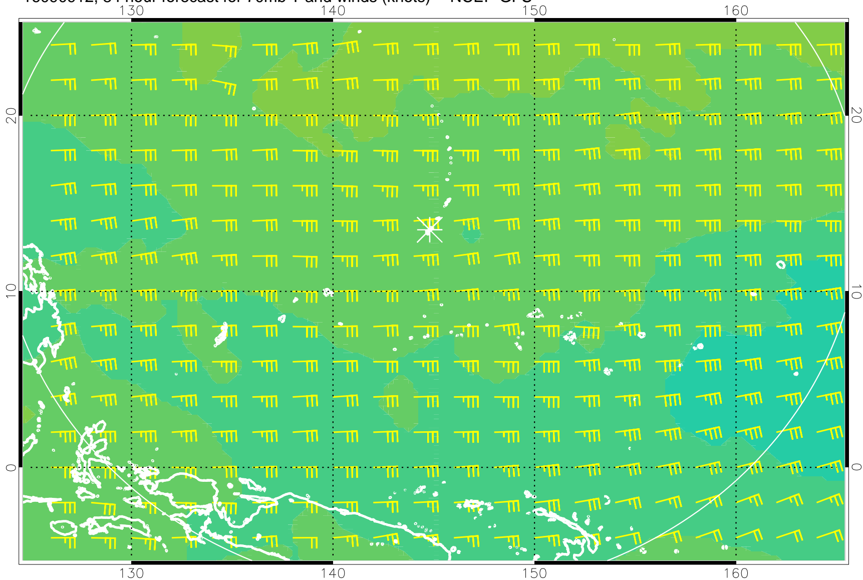
16090912, 84 hour forecast for 70mb T and winds (knots) -- NCEP GFS
