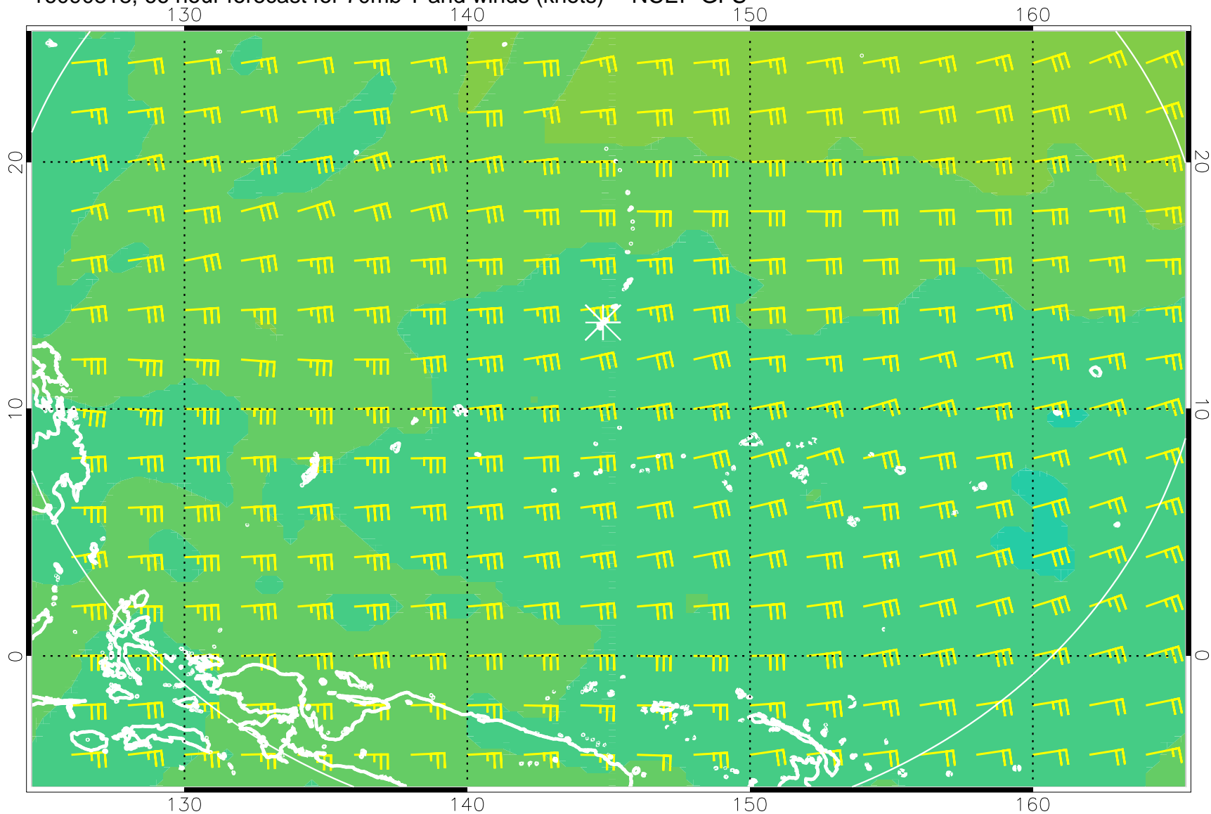
16090818, 66 hour forecast for 70mb T and winds (knots) -- NCEP GFS
