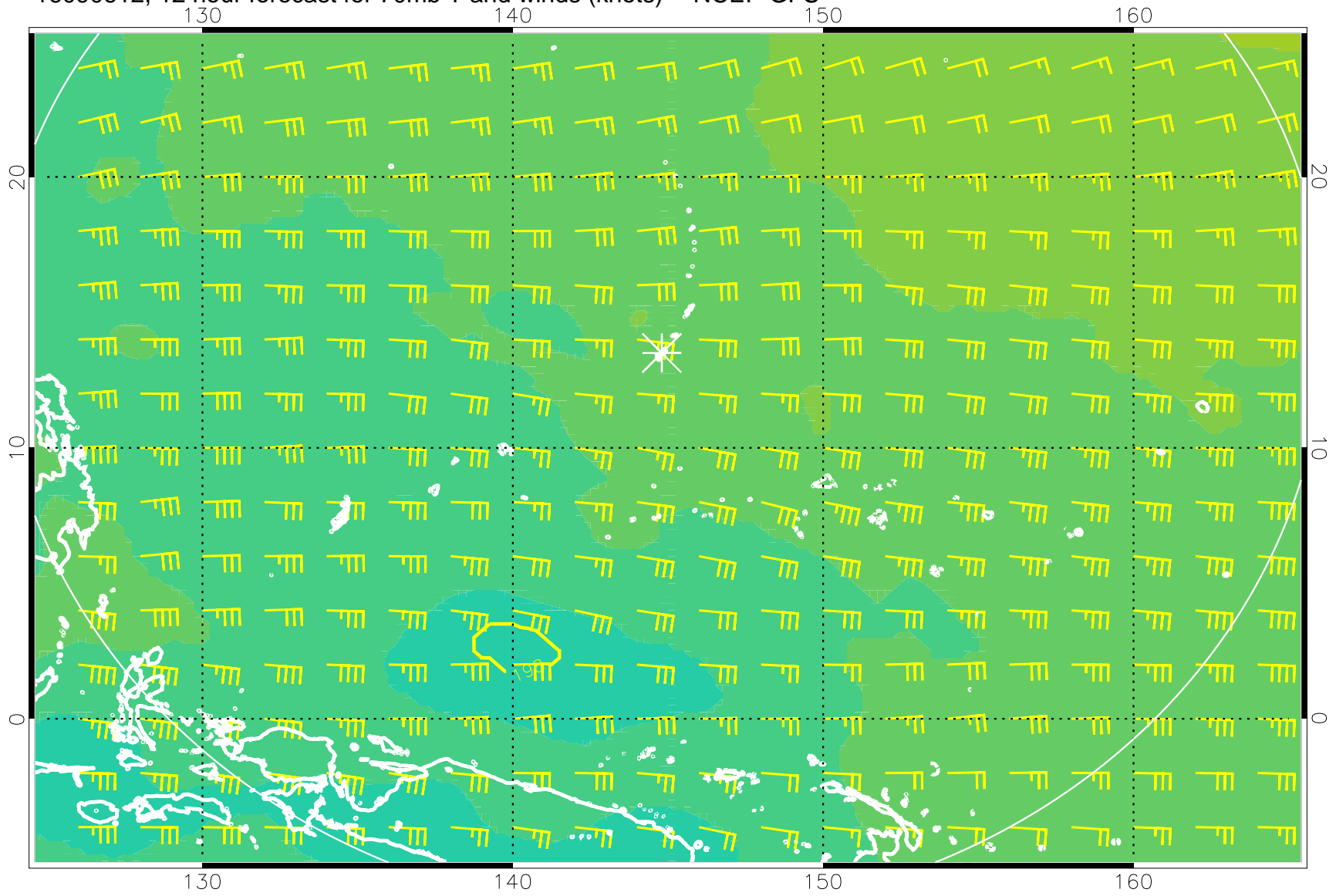
16090612, 12 hour forecast for 70mb T and winds (knots) -- NCEP GFS
