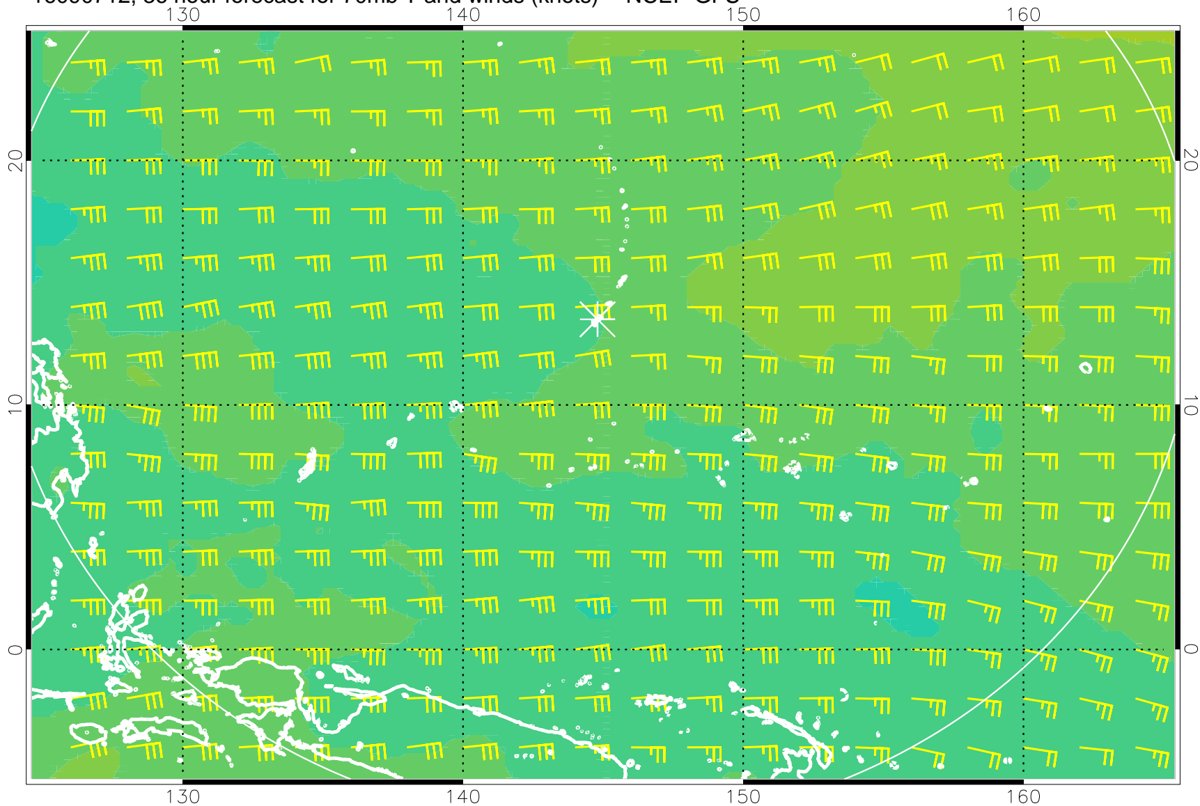
16090712, 36 hour forecast for 70mb T and winds (knots) -- NCEP GFS
