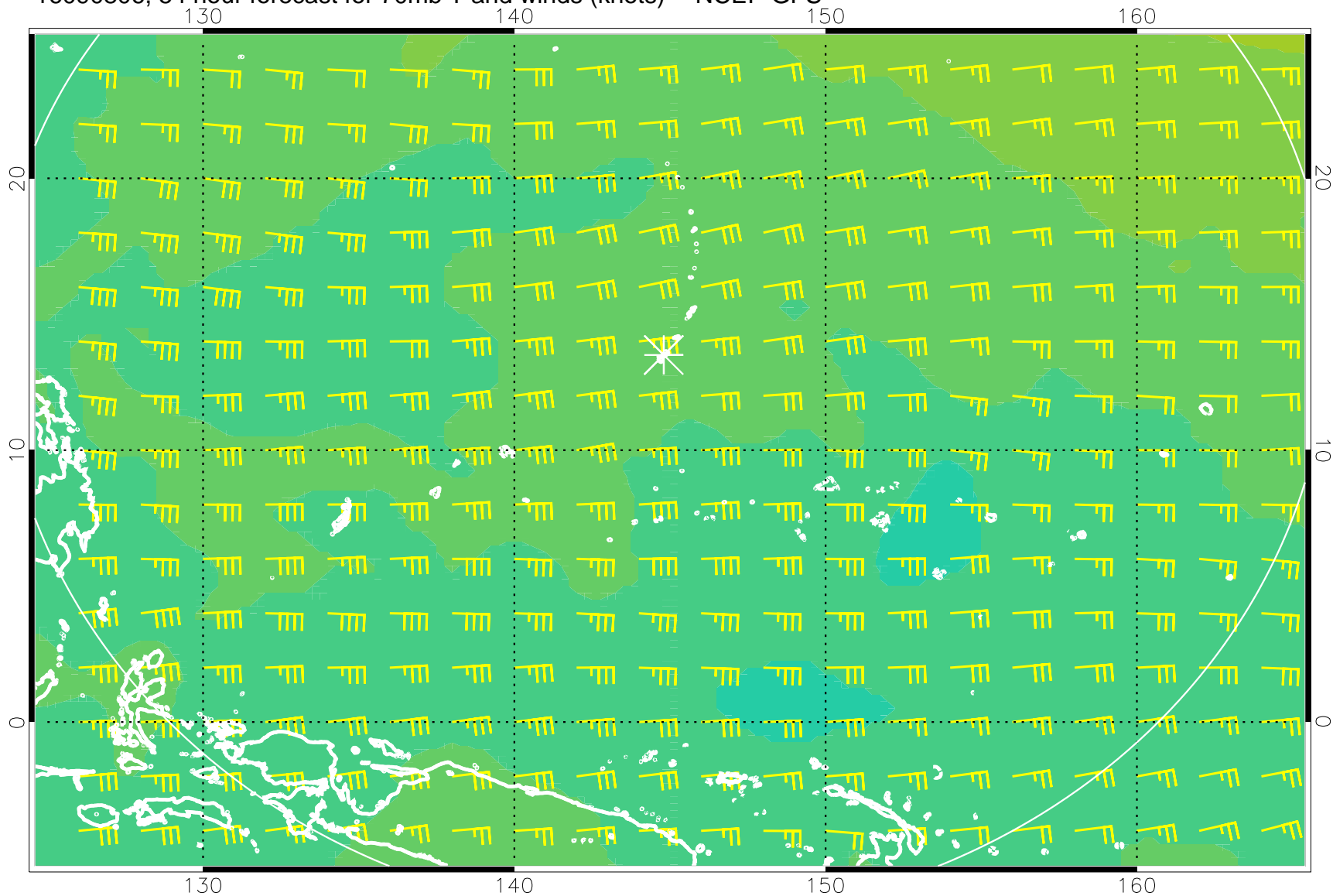
16090806, 54 hour forecast for 70mb T and winds (knots) -- NCEP GFS
