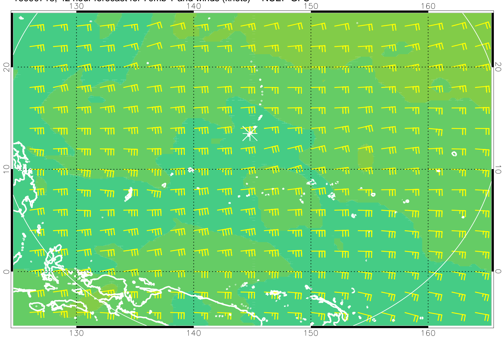
16090718, 42 hour forecast for 70mb T and winds (knots) -- NCEP GFS
