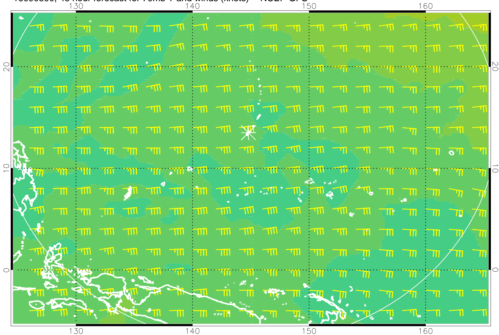
16090800, 48 hour forecast for 70mb T and winds (knots) -- NCEP GFS
