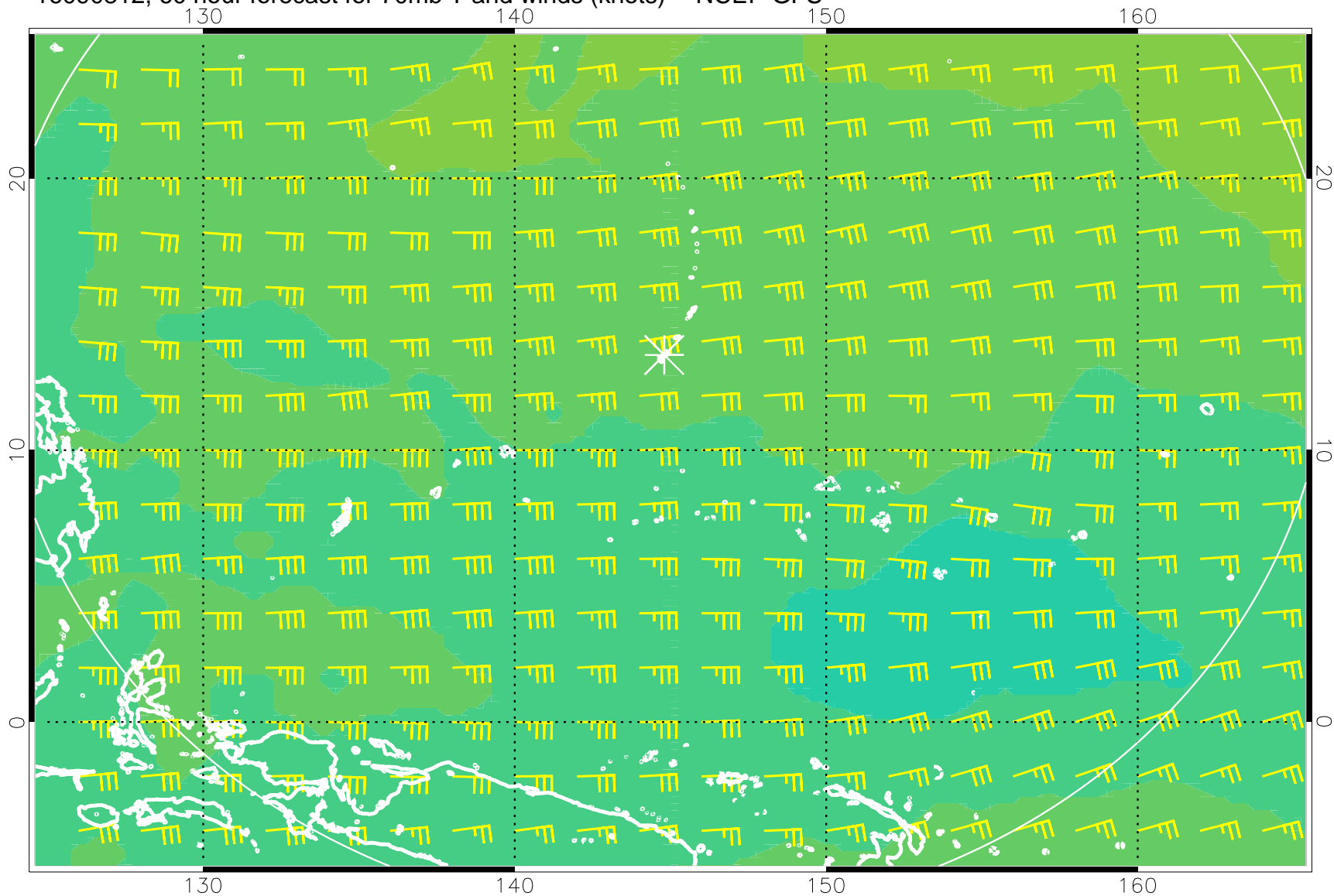
16090812, 60 hour forecast for 70mb T and winds (knots) -- NCEP GFS
