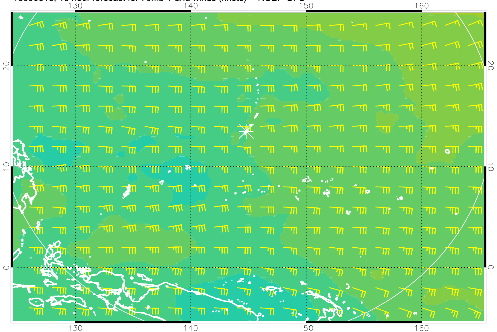
16090618, 18 hour forecast for 70mb T and winds (knots) -- NCEP GFS
