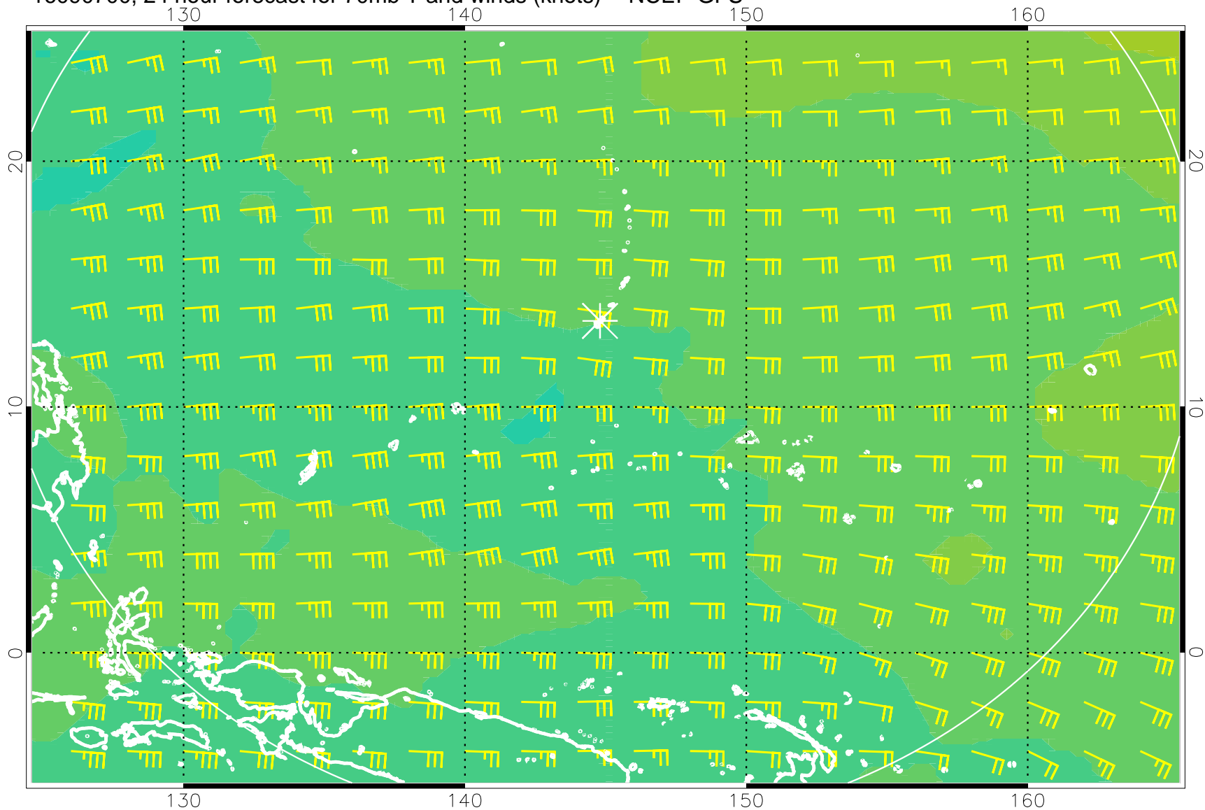
16090700, 24 hour forecast for 70mb T and winds (knots) -- NCEP GFS
