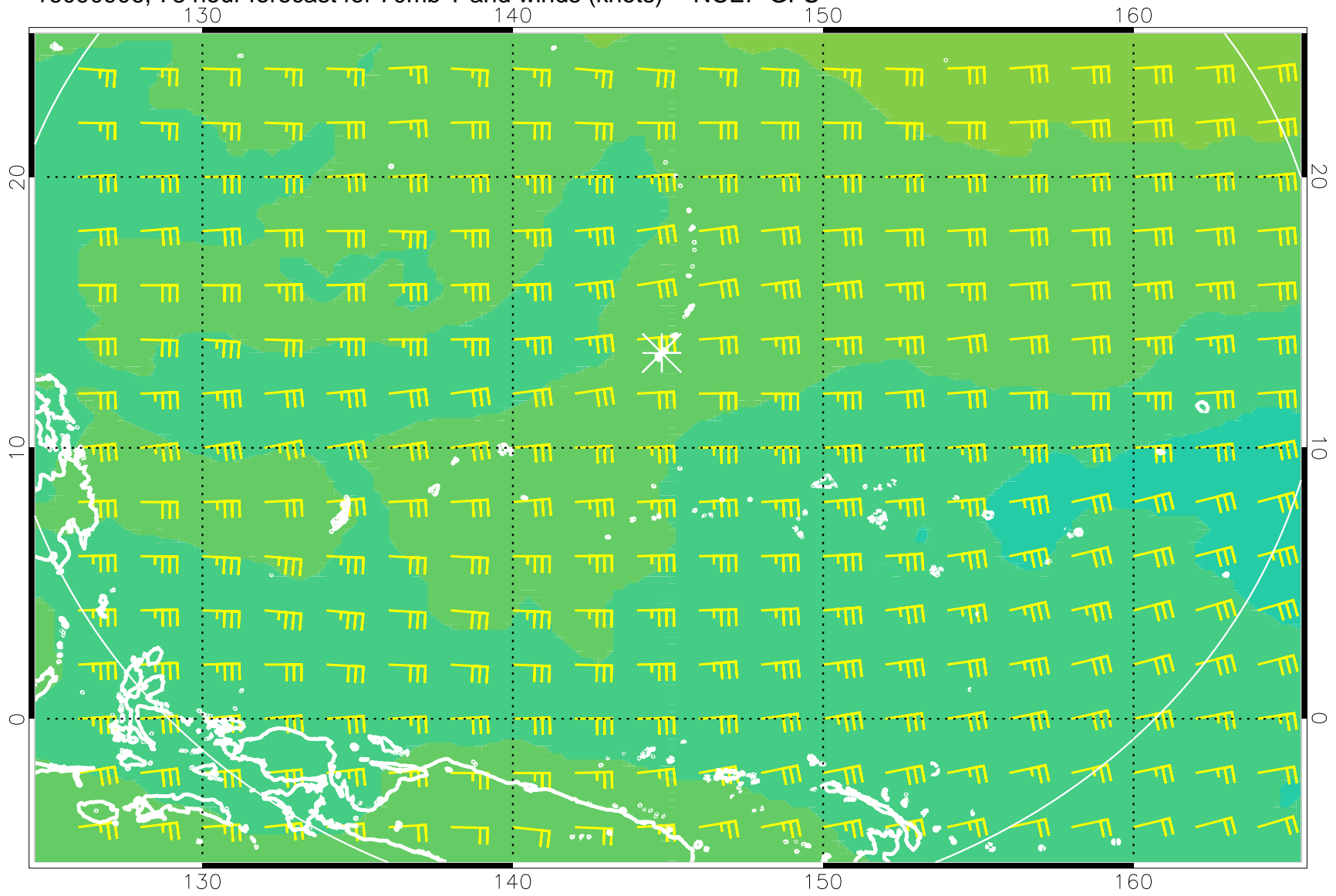
16090906, 78 hour forecast for 70mb T and winds (knots) -- NCEP GFS
