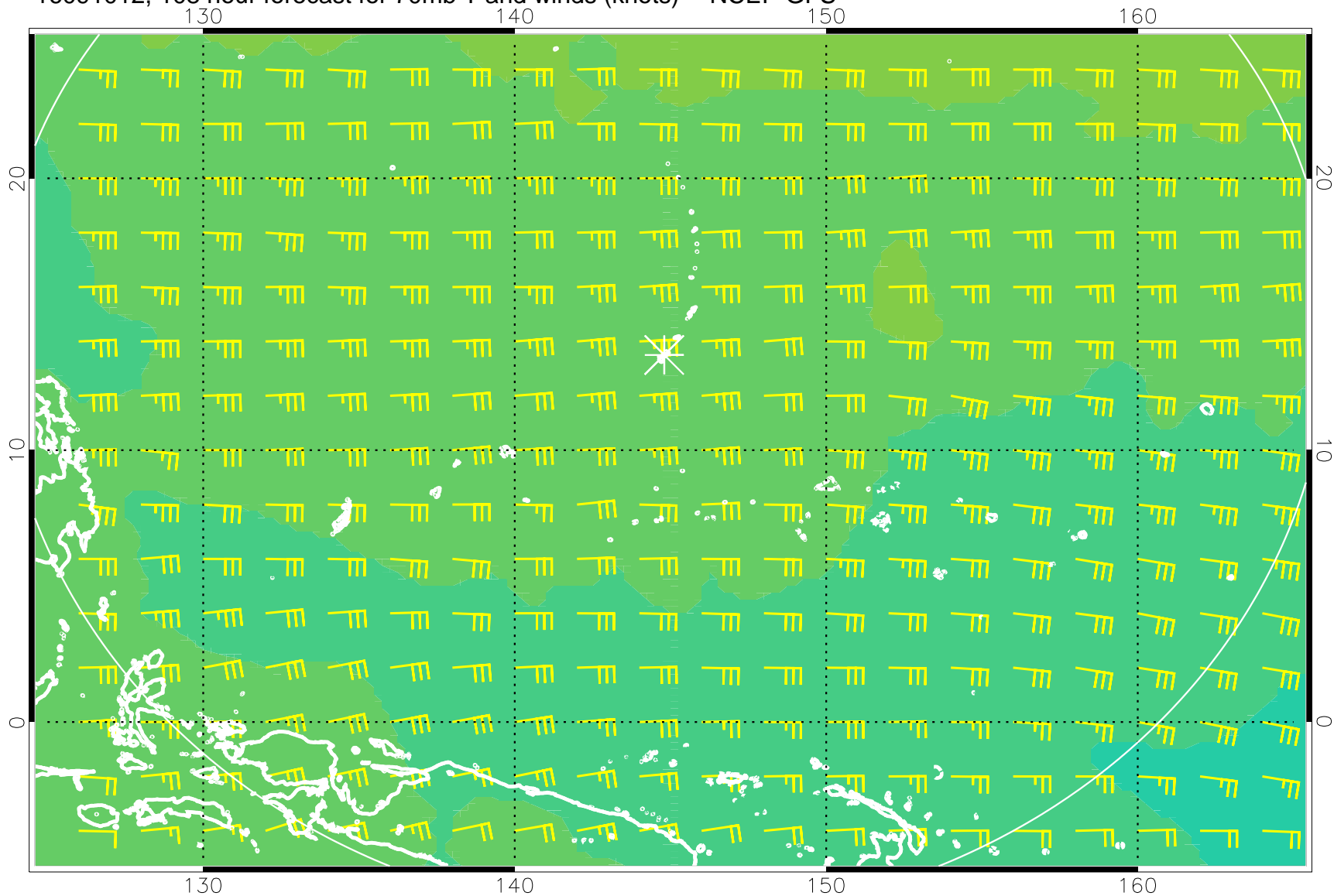
16091012, 108 hour forecast for 70mb T and winds (knots) -- NCEP GFS
