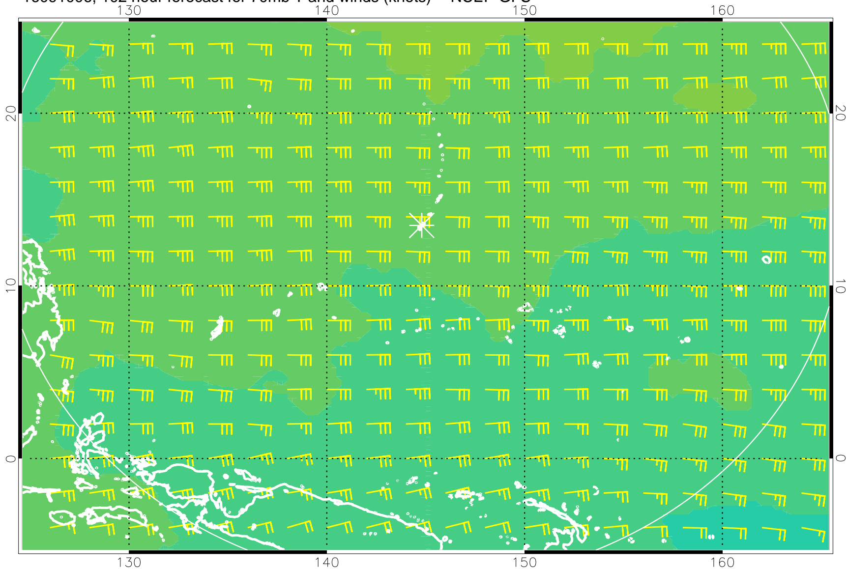
16091006, 102 hour forecast for 70mb T and winds (knots) -- NCEP GFS
