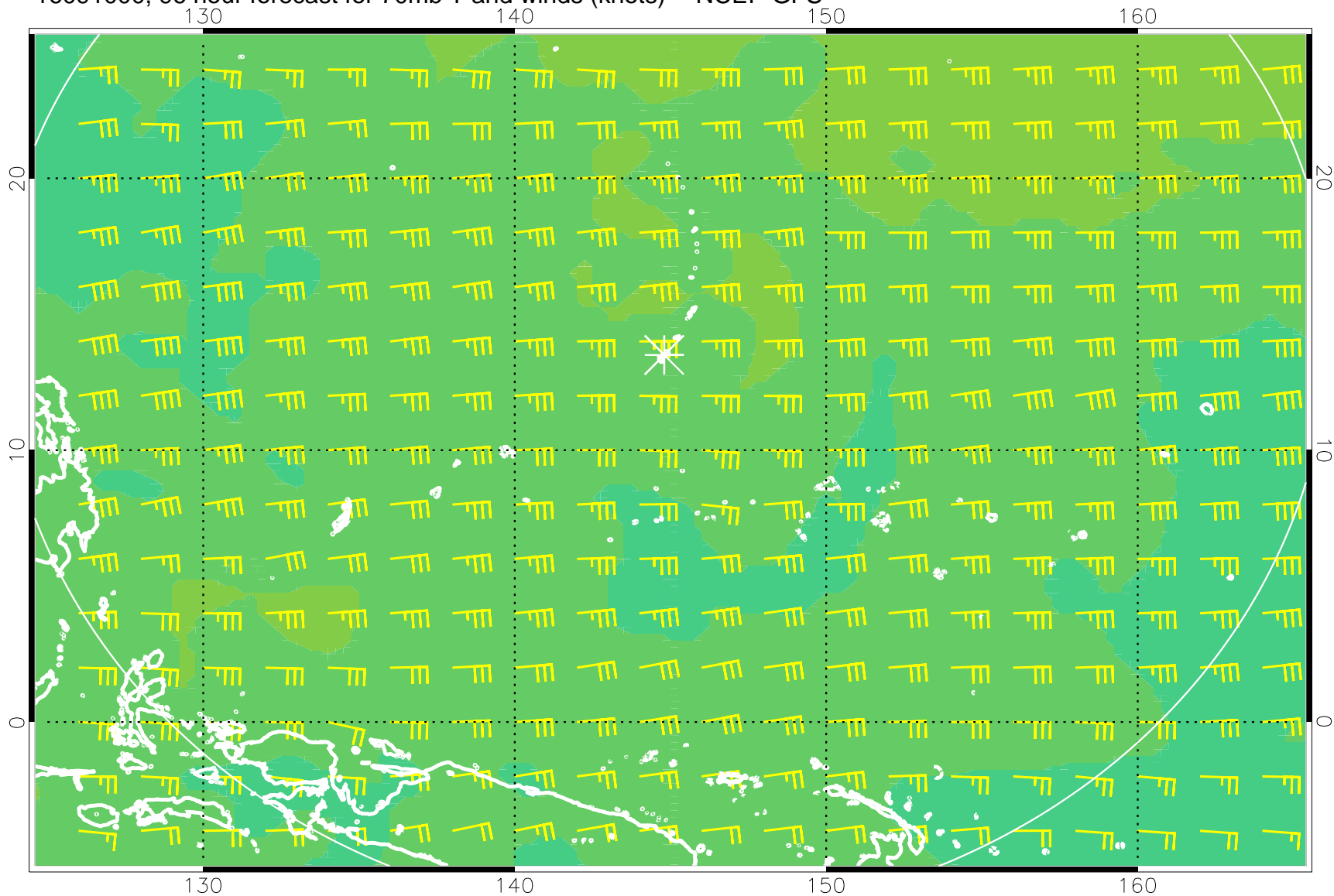
16091000, 96 hour forecast for 70mb T and winds (knots) -- NCEP GFS
