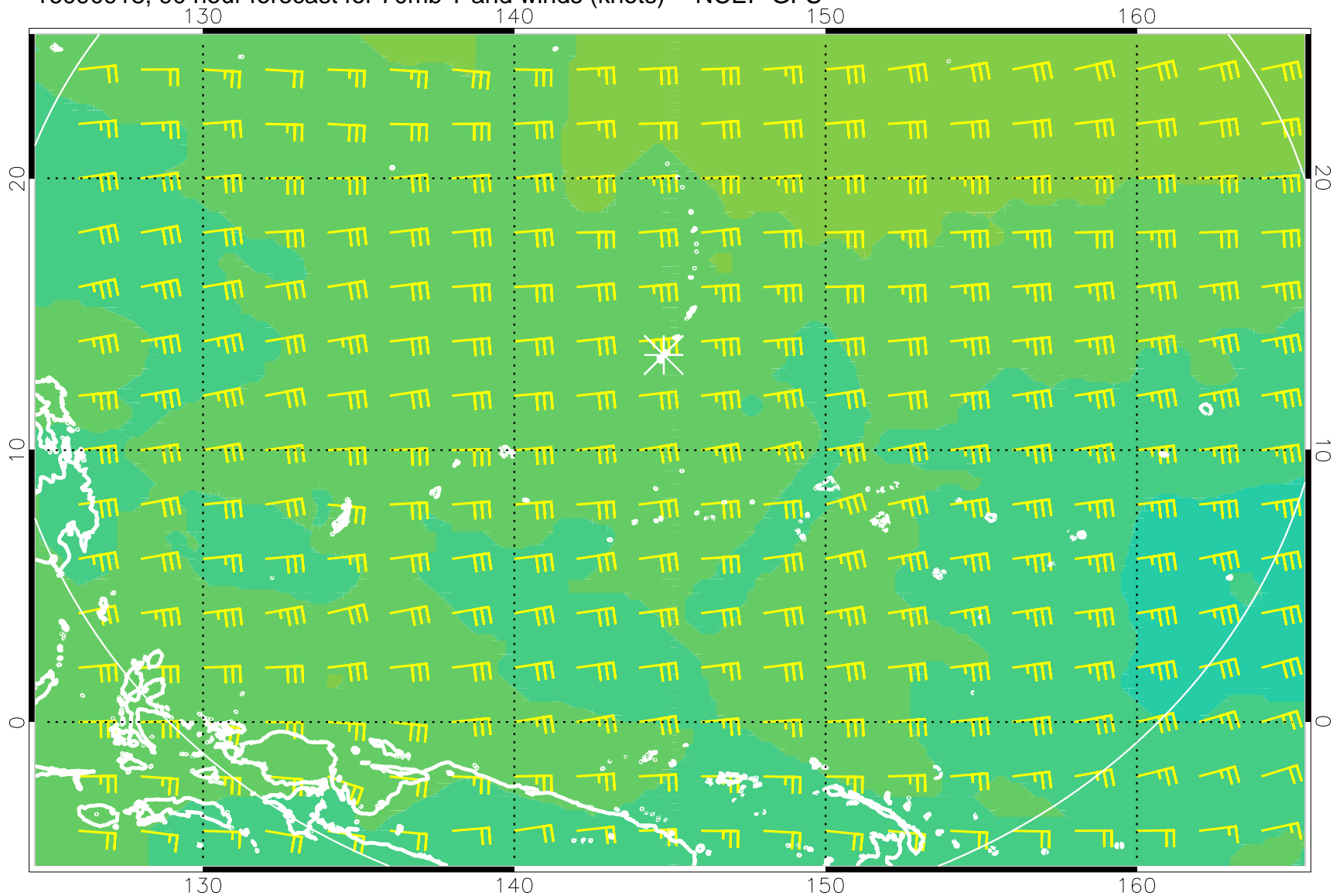
16090918, 90 hour forecast for 70mb T and winds (knots) -- NCEP GFS
