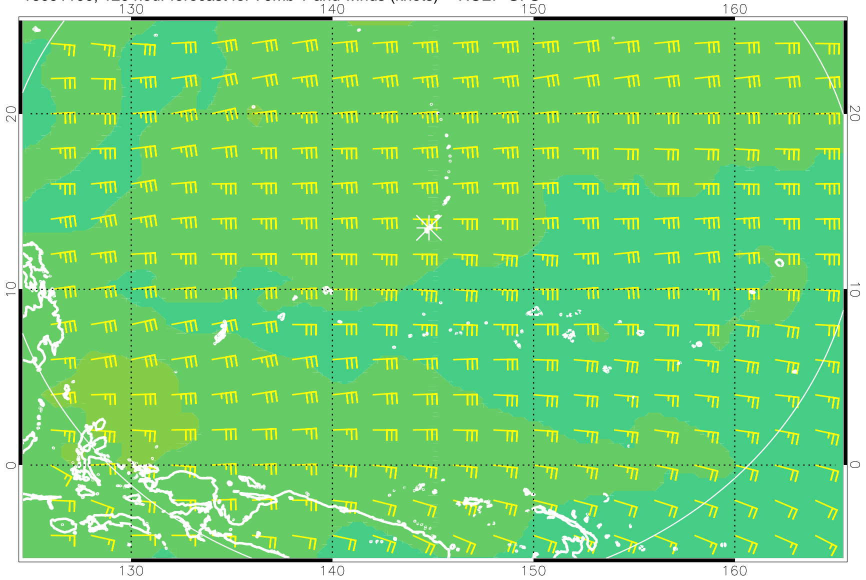
16091100, 120 hour forecast for 70mb T and winds (knots) -- NCEP GFS
