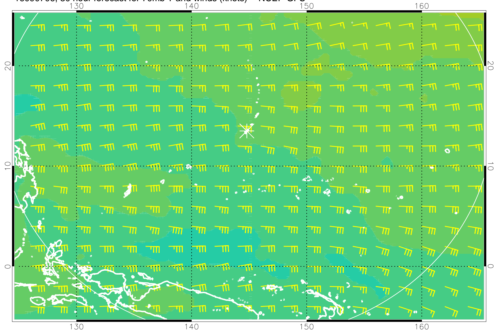
16090706, 30 hour forecast for 70mb T and winds (knots) -- NCEP GFS
