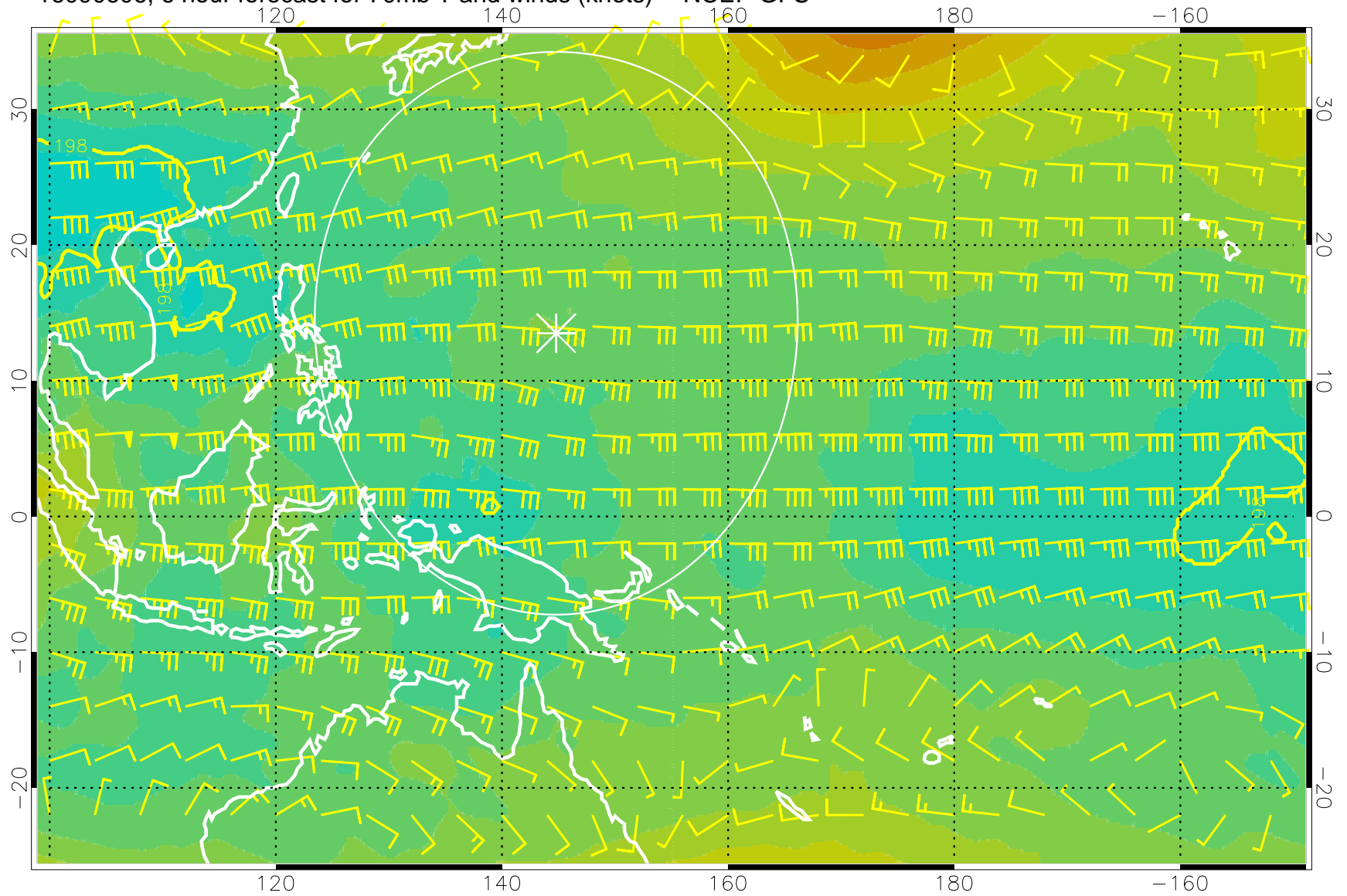
16090606, 6 hour forecast for 70mb T and winds (knots) -- NCEP GFS
