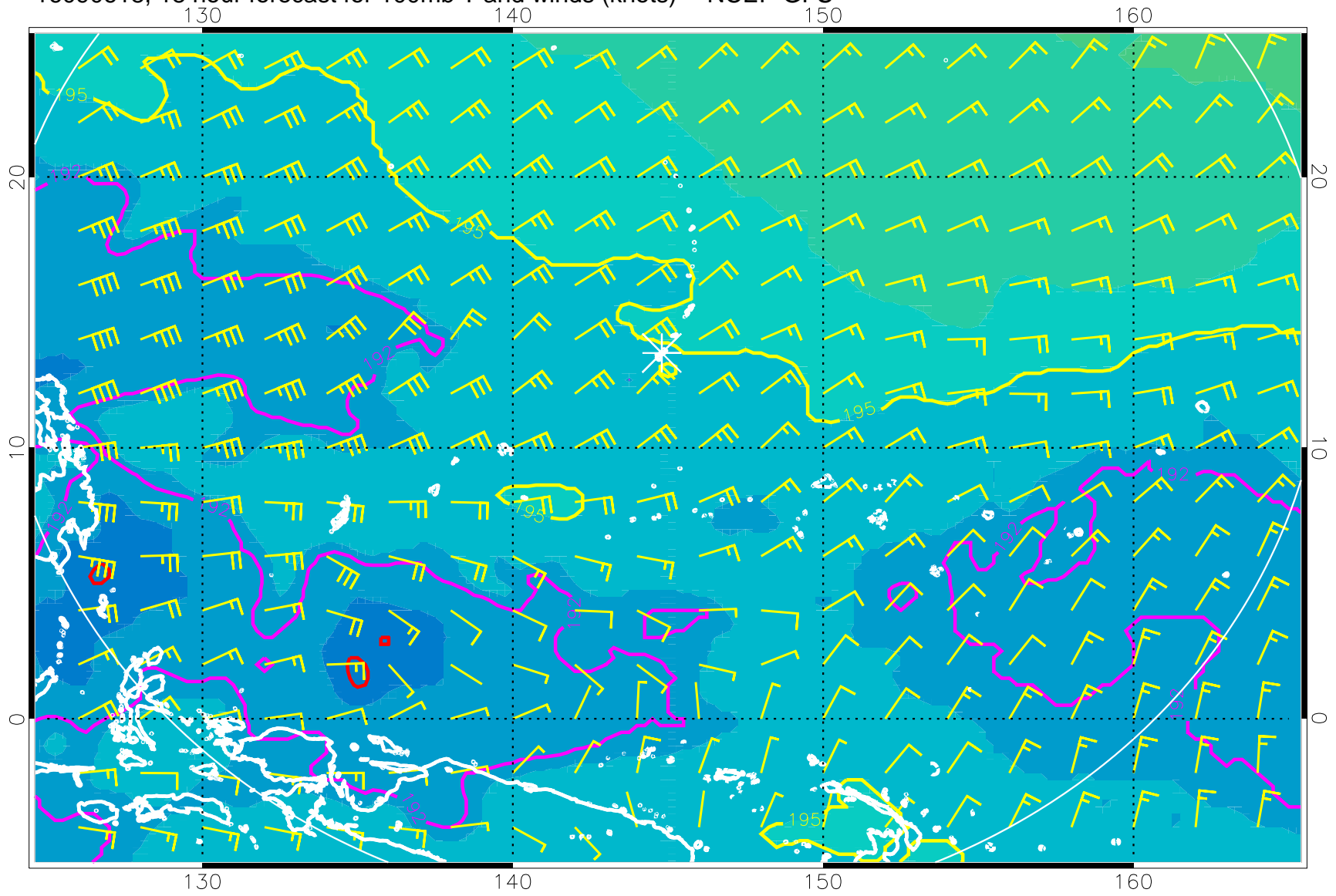
16090618, 18 hour forecast for 100mb T and winds (knots) -- NCEP GFS
