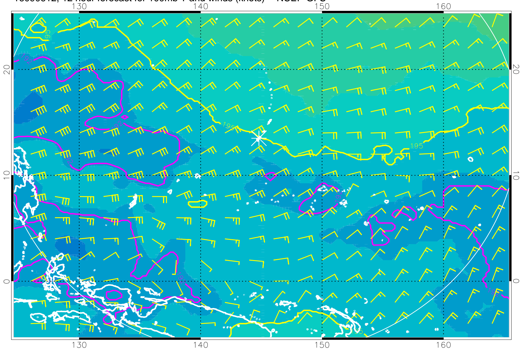
16090612, 12 hour forecast for 100mb T and winds (knots) -- NCEP GFS
