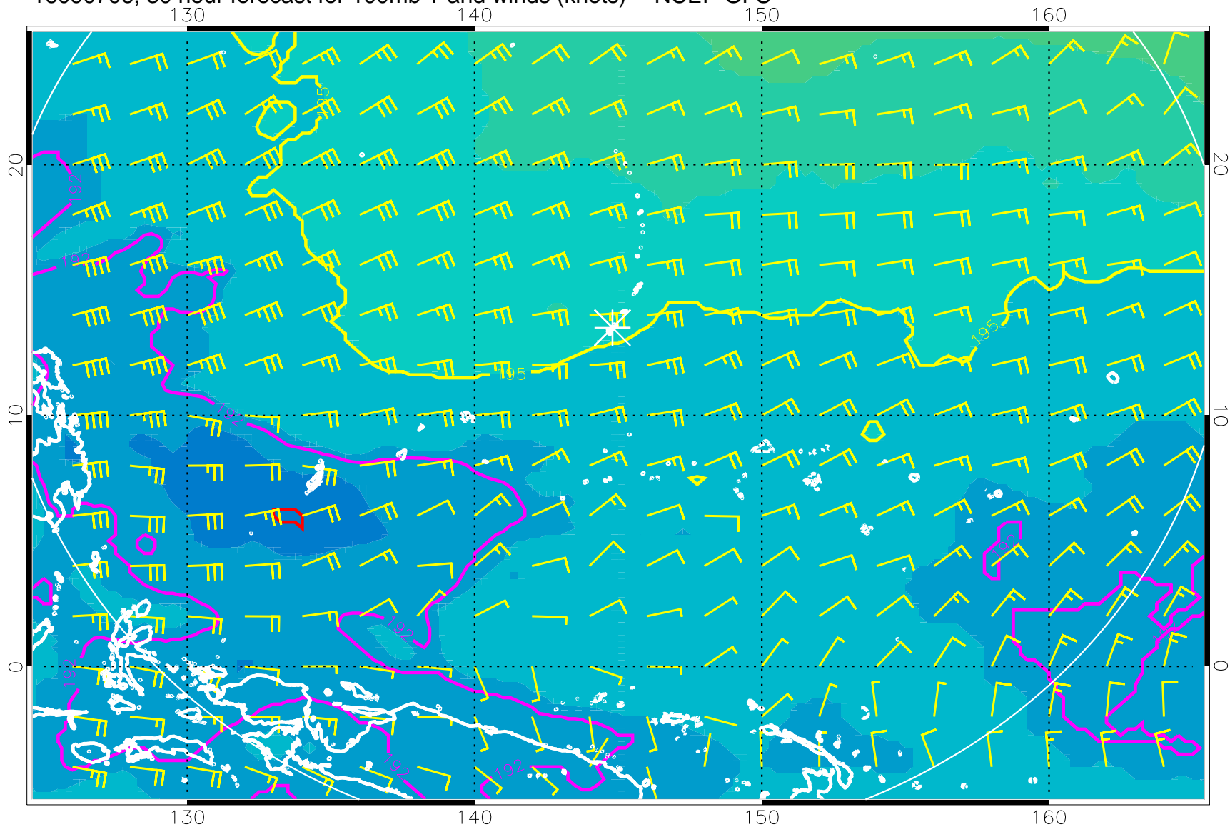
16090706, 30 hour forecast for 100mb T and winds (knots) -- NCEP GFS
