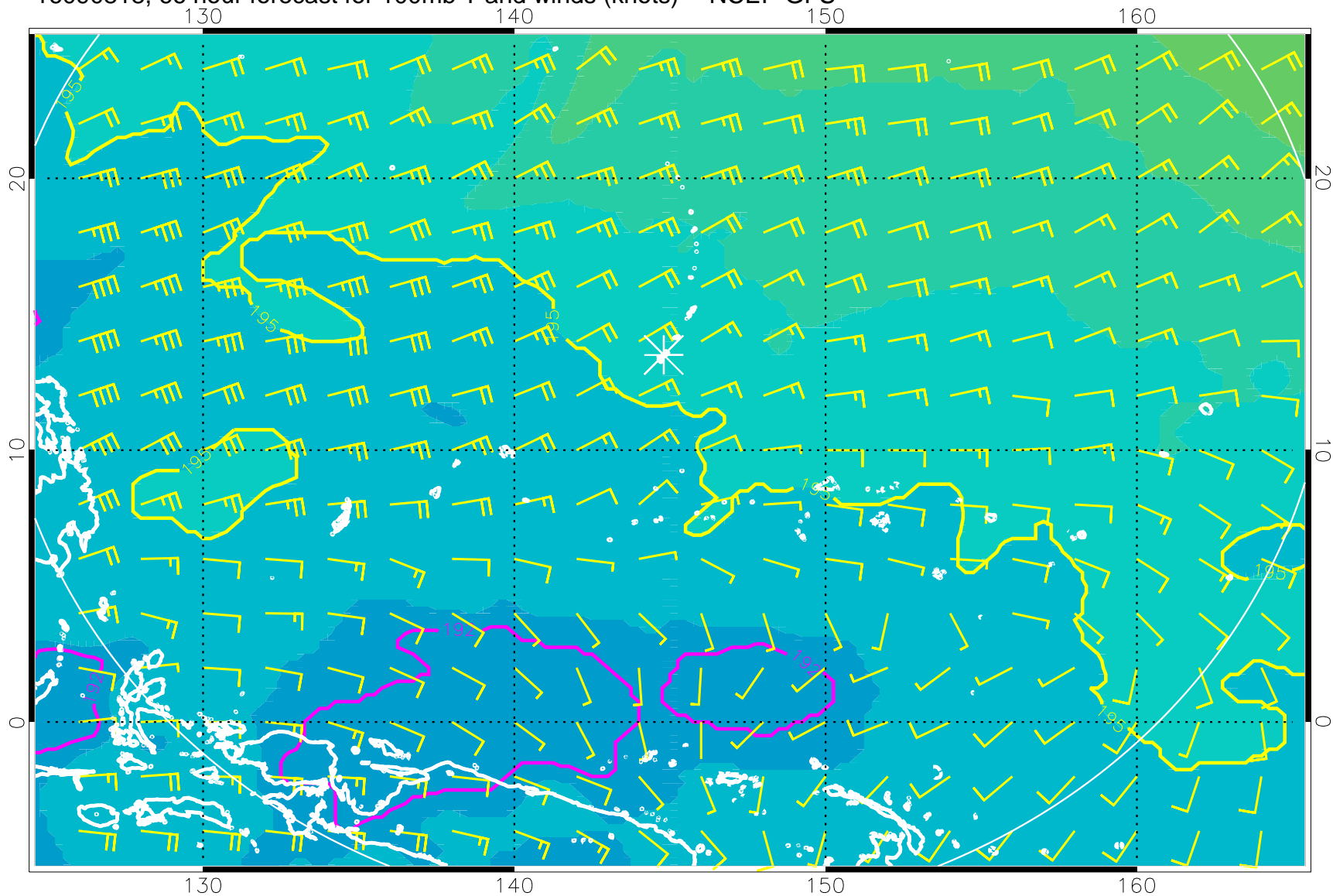
16090818, 66 hour forecast for 100mb T and winds (knots) -- NCEP GFS
