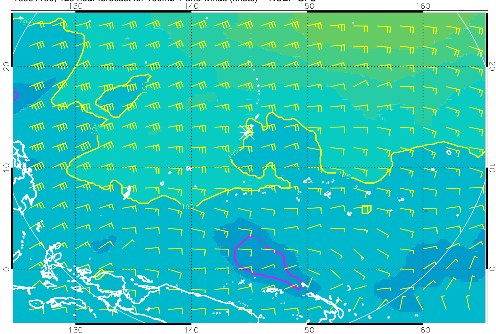
16091100, 120 hour forecast for 100mb T and winds (knots) -- NCEP GFS
