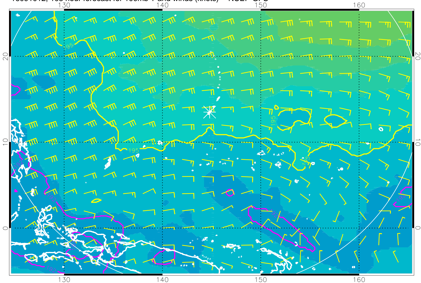
16091012, 108 hour forecast for 100mb T and winds (knots) -- NCEP GFS
