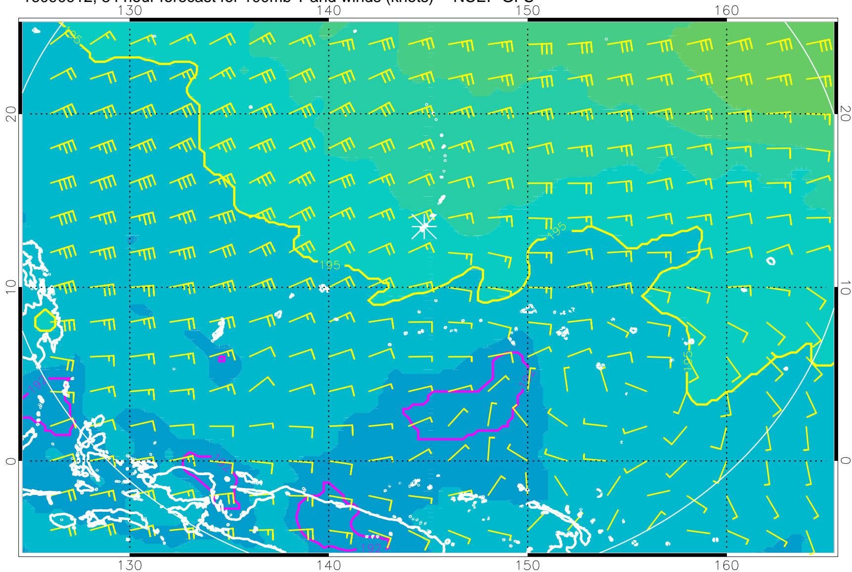
16090912, 84 hour forecast for 100mb T and winds (knots) -- NCEP GFS
