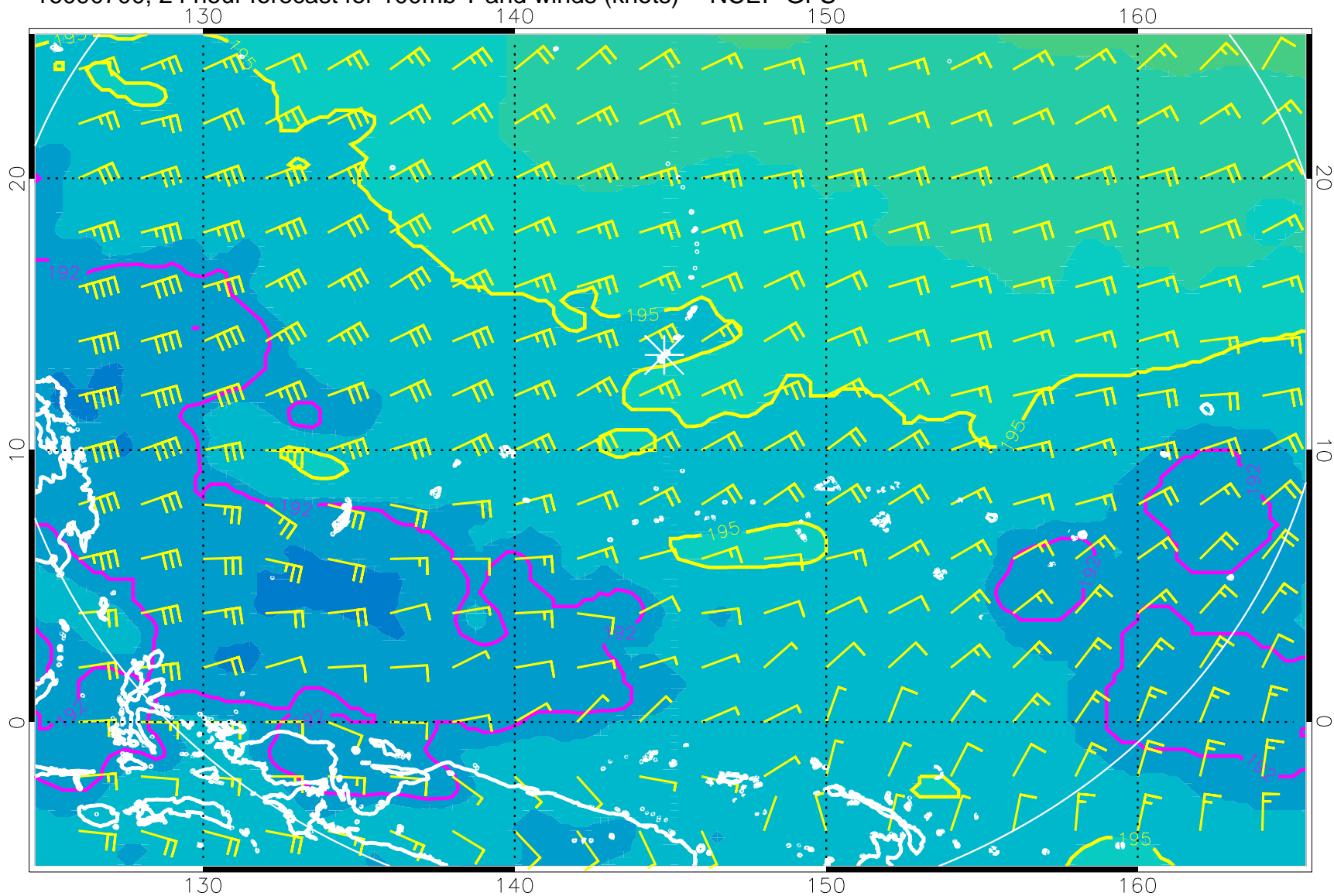
16090700, 24 hour forecast for 100mb T and winds (knots) -- NCEP GFS
