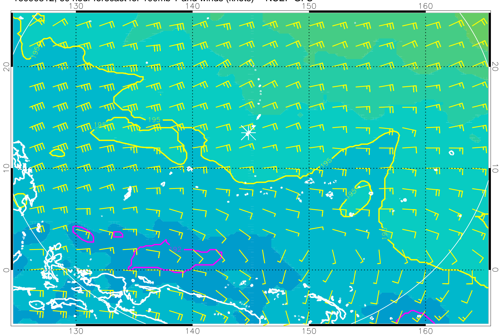
16090812, 60 hour forecast for 100mb T and winds (knots) -- NCEP GFS
