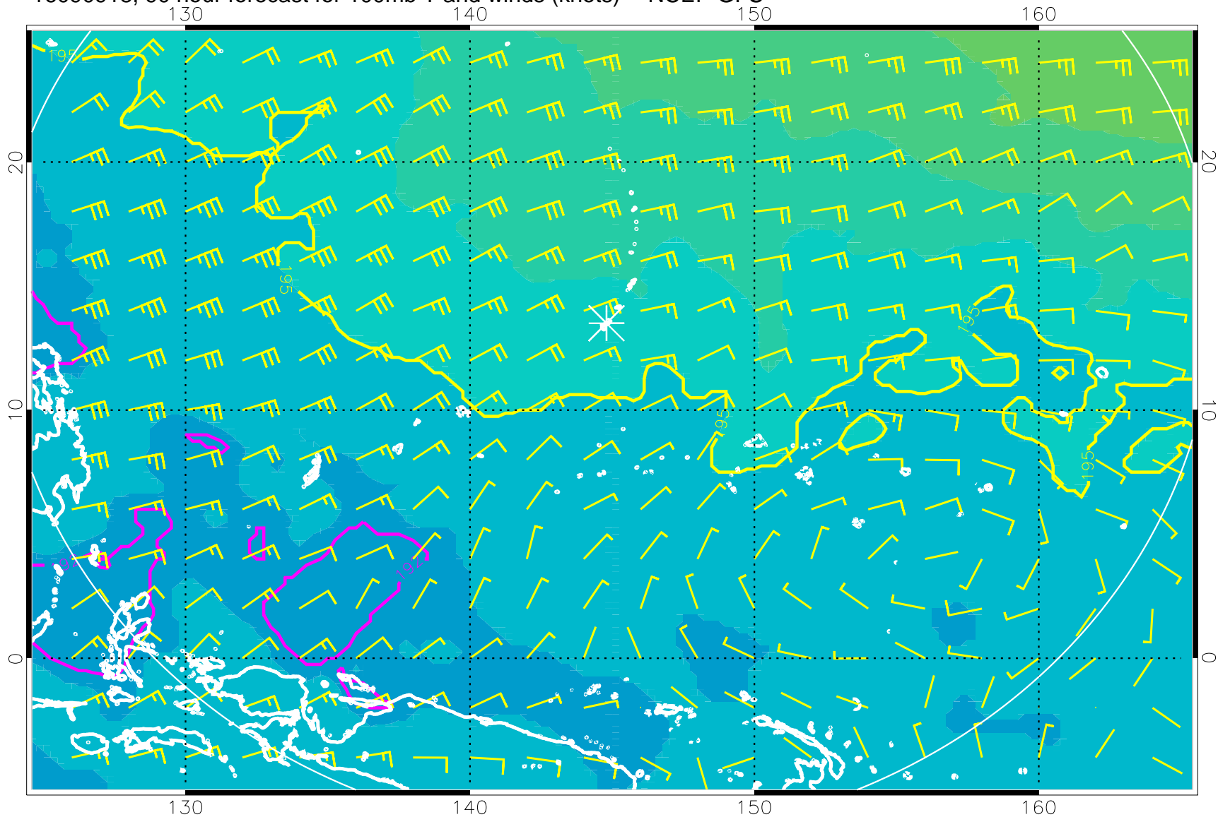
16090918, 90 hour forecast for 100mb T and winds (knots) -- NCEP GFS
