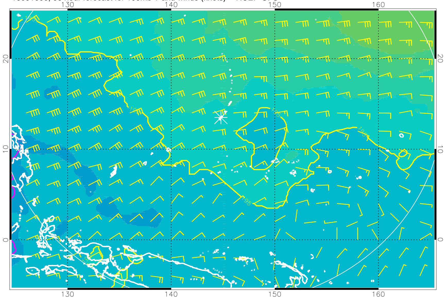
16091000, 96 hour forecast for 100mb T and winds (knots) -- NCEP GFS
