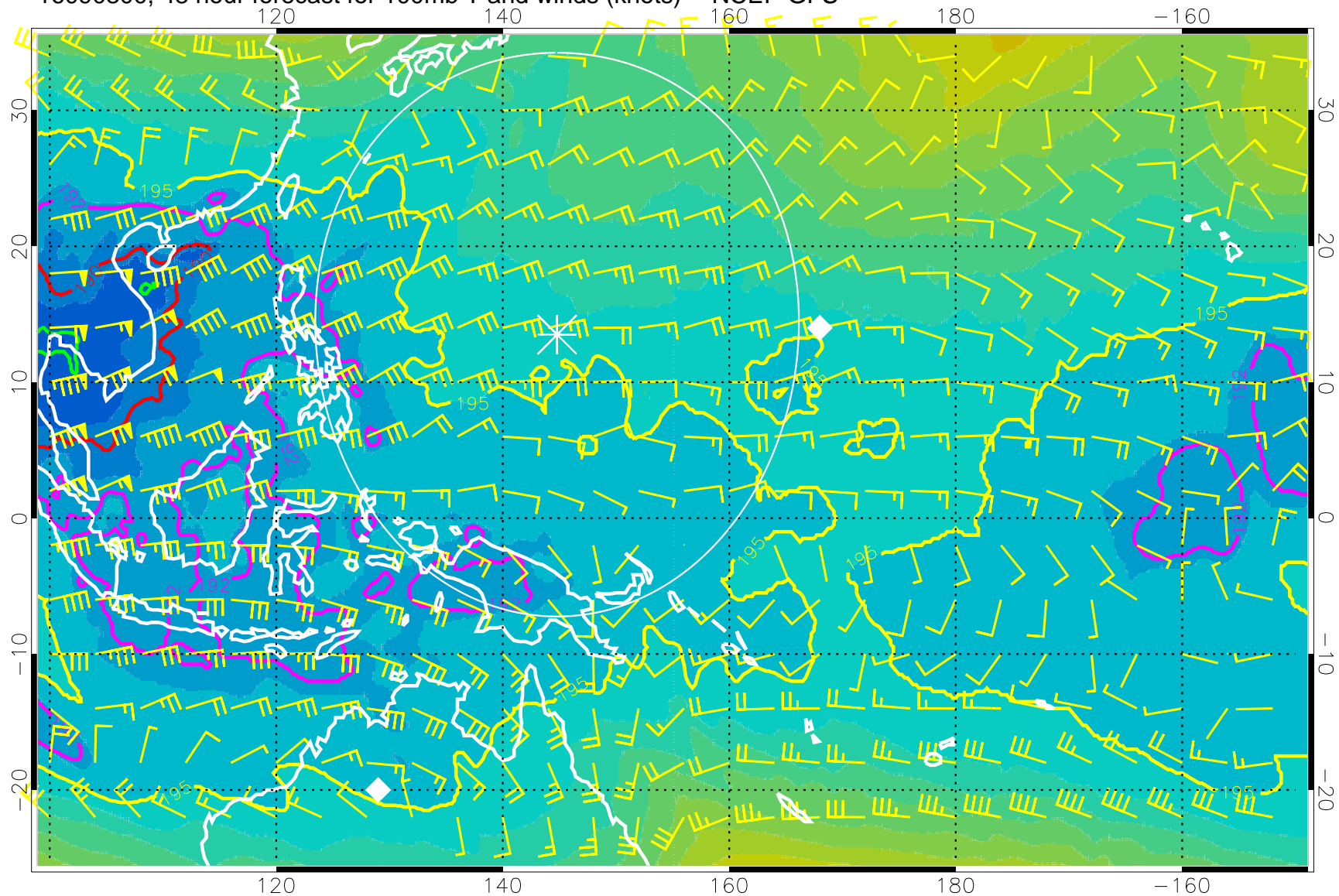
16090800, 48 hour forecast for 100mb T and winds (knots) -- NCEP GFS
