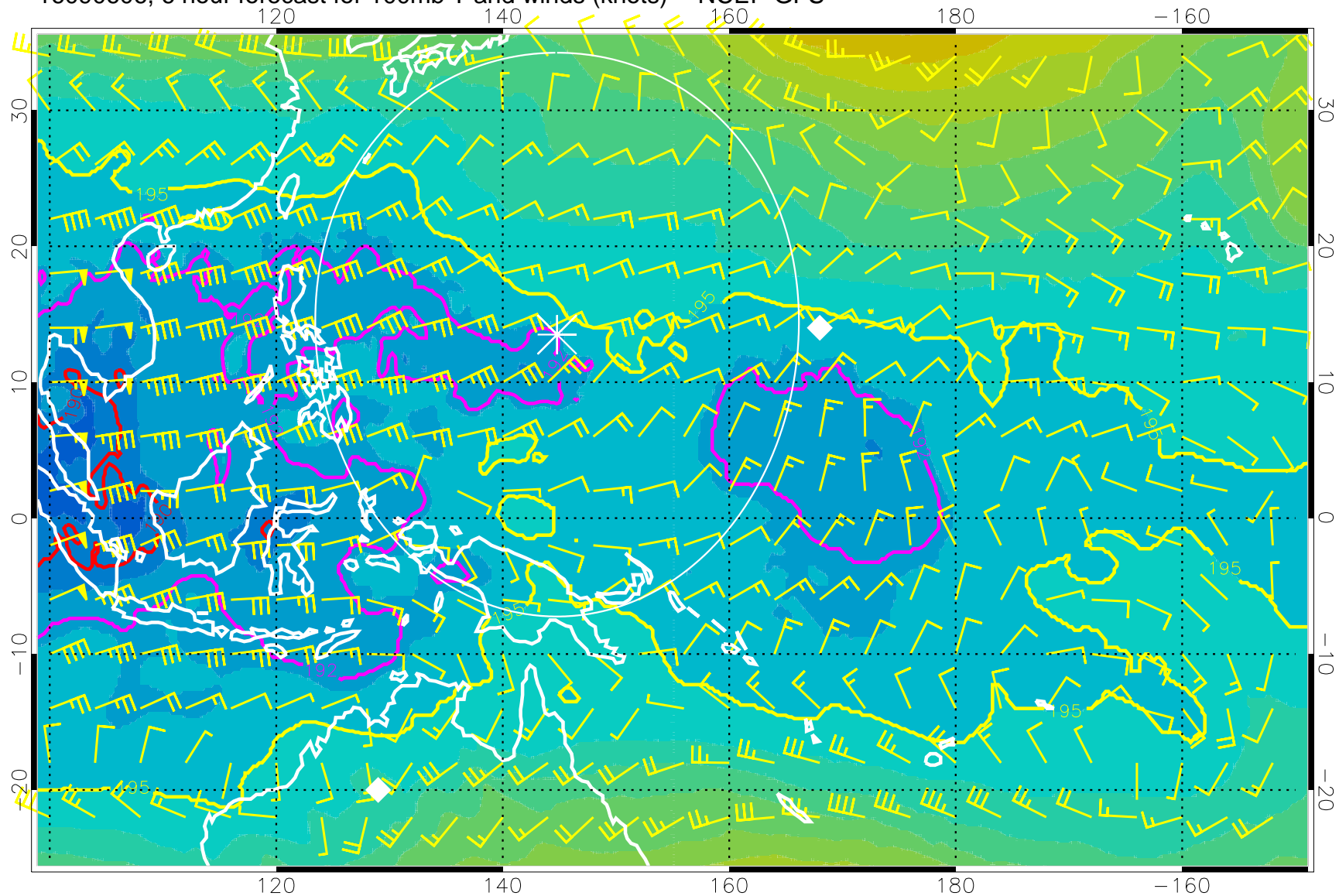
16090606, 6 hour forecast for 100mb T and winds (knots) -- NCEP GFS
