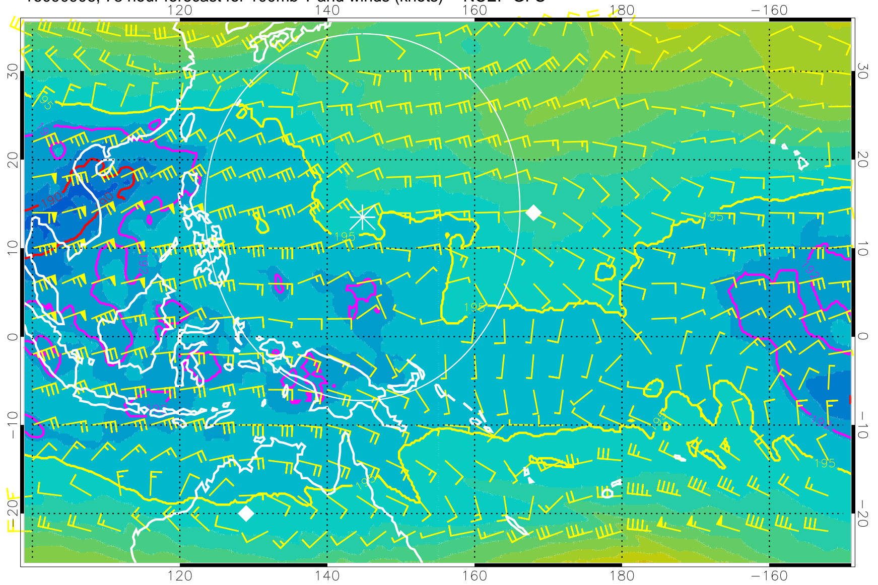
16090906, 78 hour forecast for 100mb T and winds (knots) -- NCEP GFS
