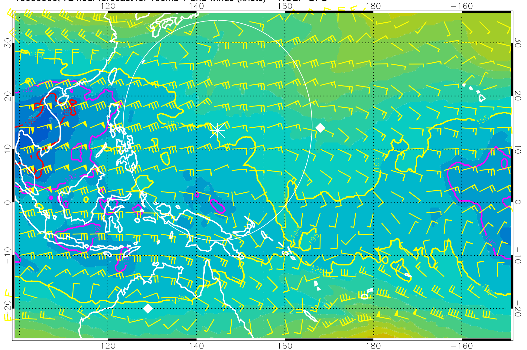
16090900, 72 hour forecast for 100mb T and winds (knots) -- NCEP GFS
