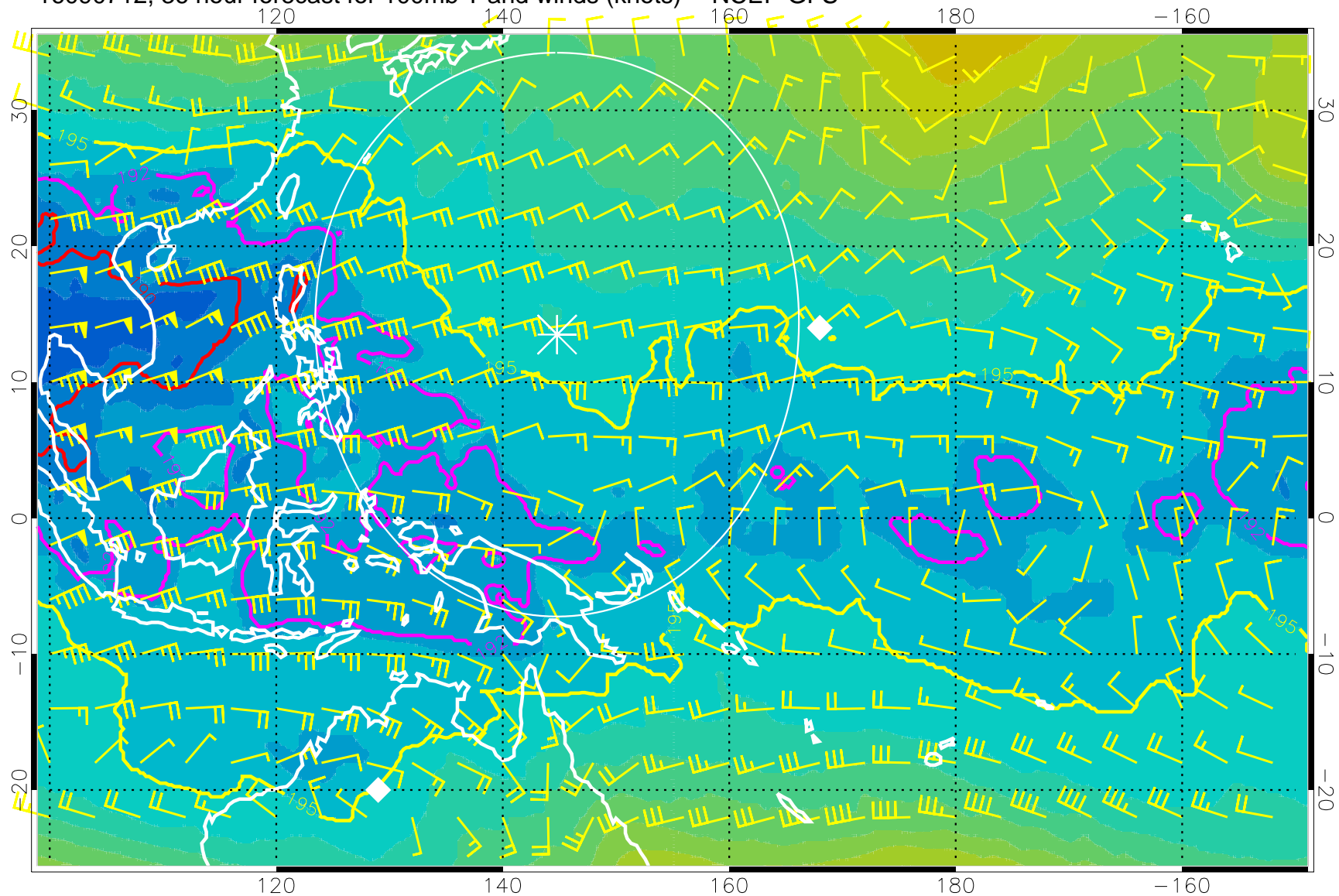
16090712, 36 hour forecast for 100mb T and winds (knots) -- NCEP GFS
