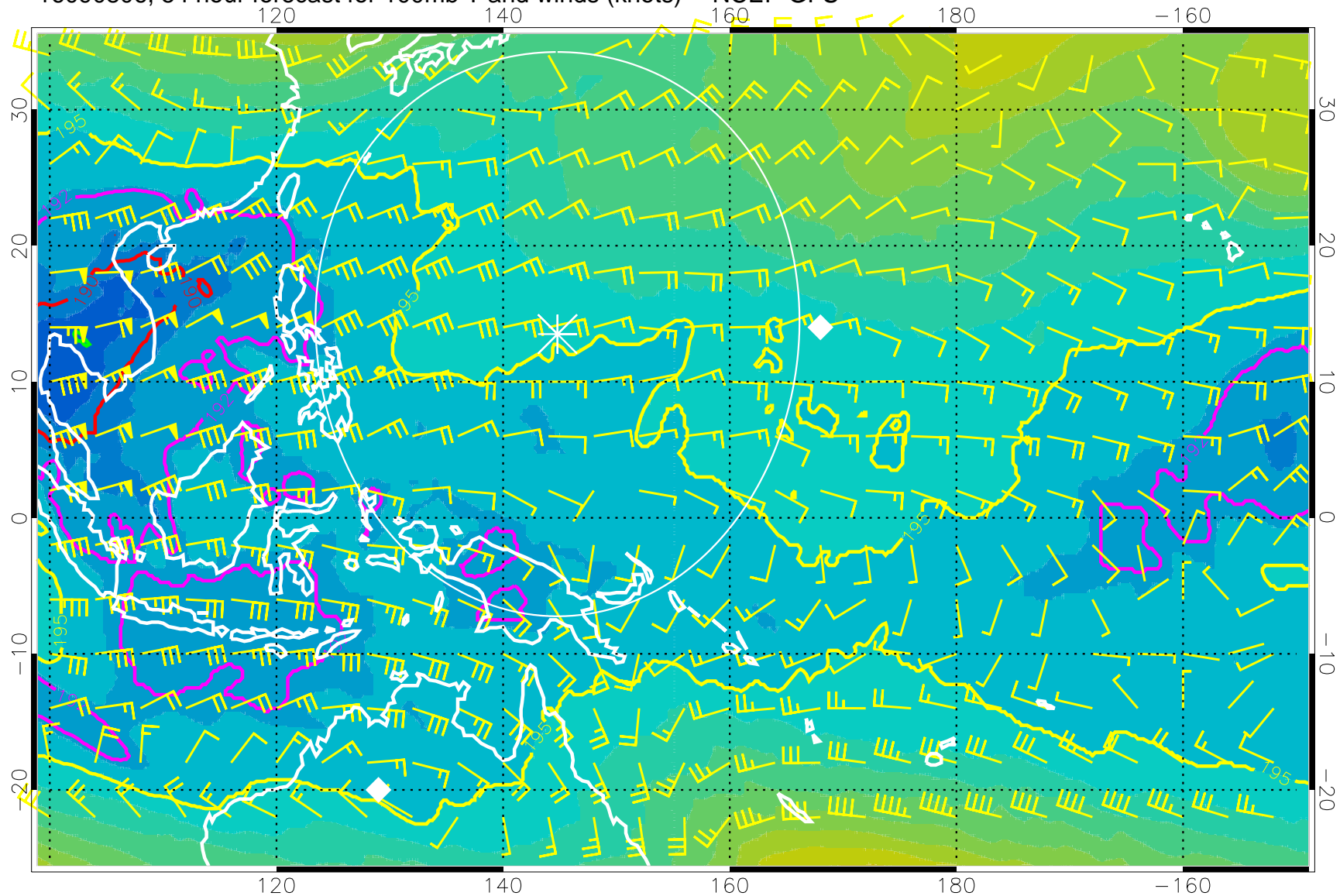
16090806, 54 hour forecast for 100mb T and winds (knots) -- NCEP GFS
