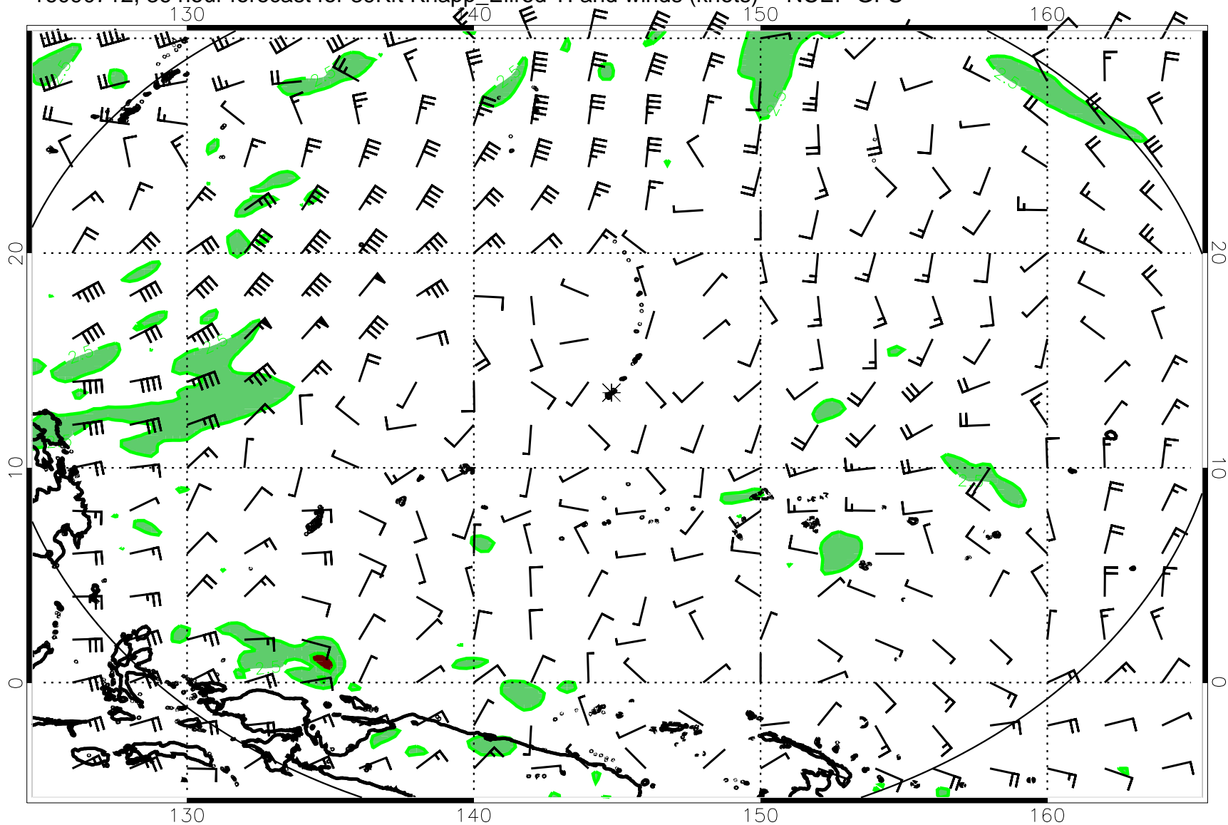
16090712, 36 hour forecast for 39Kft Knapp_Ellrod TI and winds (knots) -- NCEP GFS
