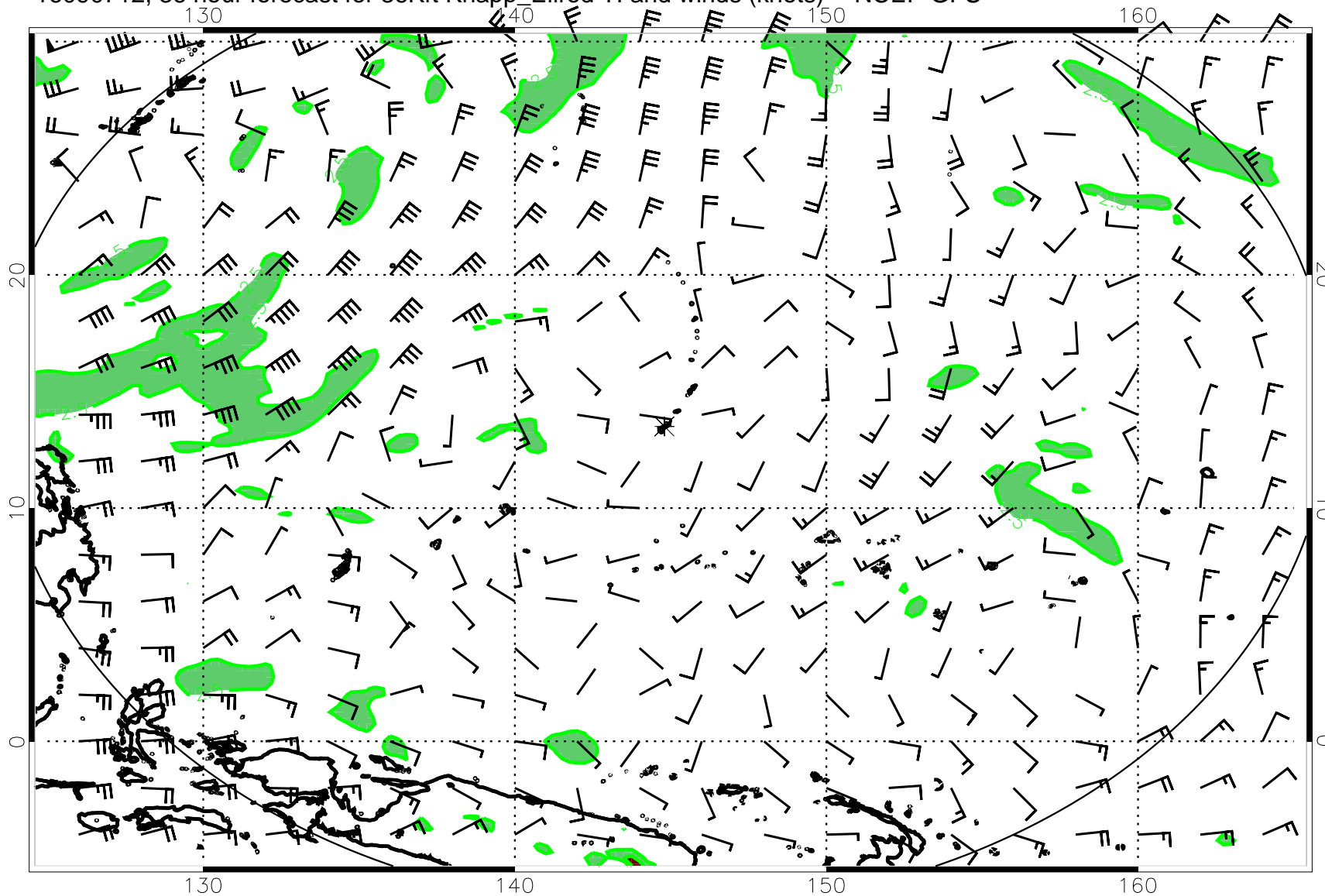
16090712, 36 hour forecast for 36Kft Knapp_Ellrod TI and winds (knots) -- NCEP GFS
