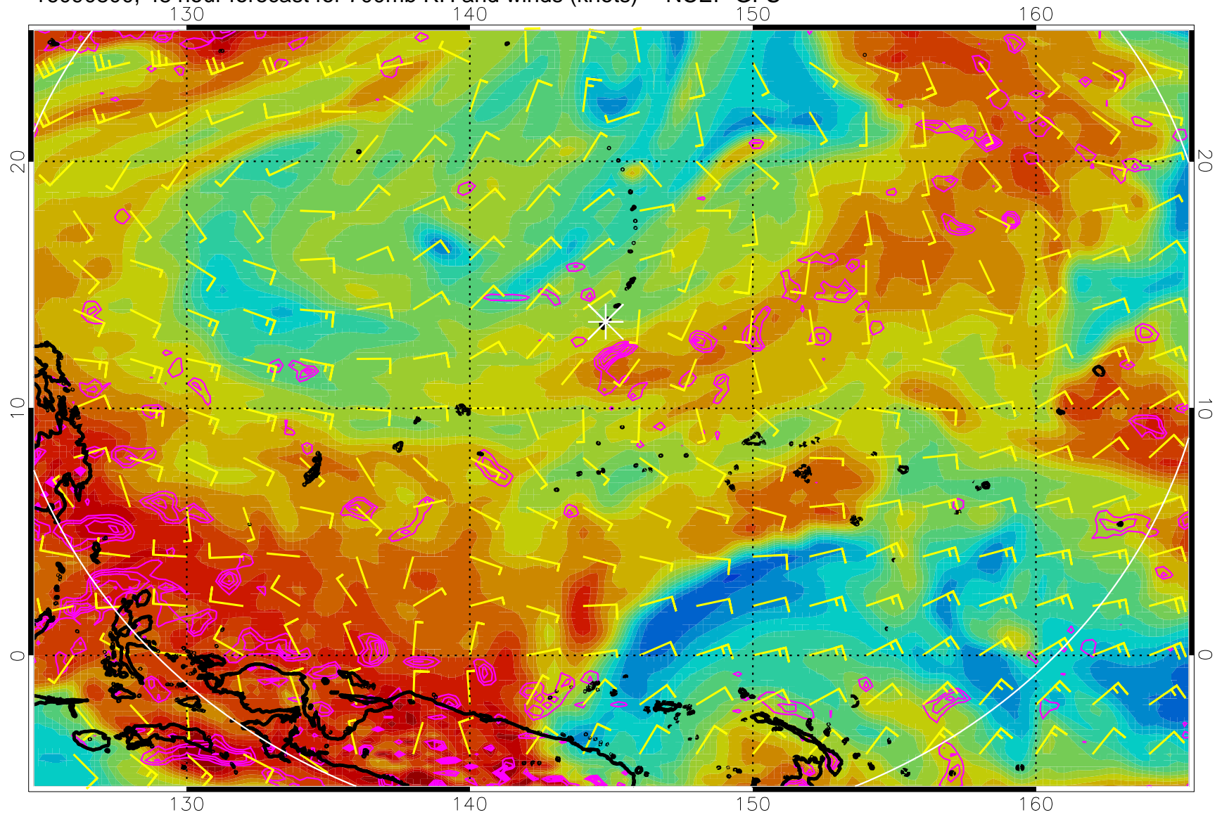
16090800, 48 hour forecast for 700mb RH and winds (knots) -- NCEP GFS
