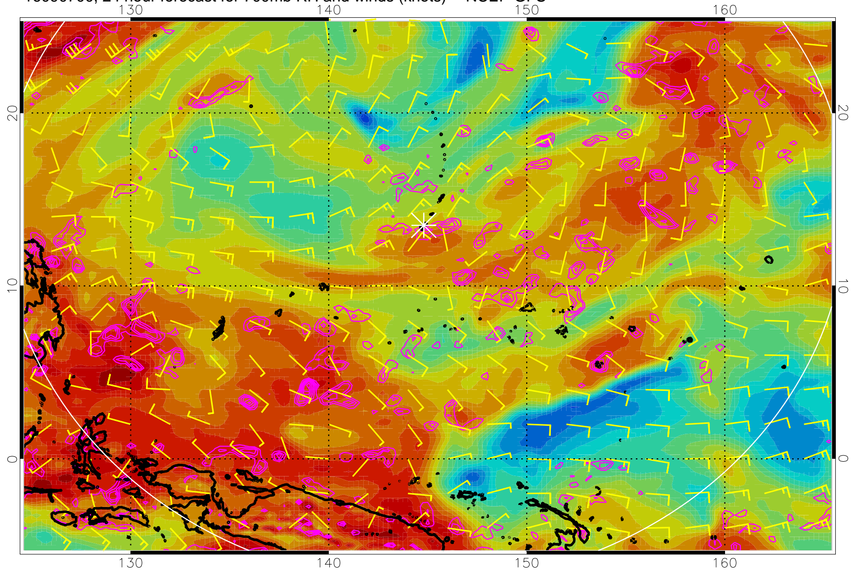
16090700, 24 hour forecast for 700mb RH and winds (knots) -- NCEP GFS
