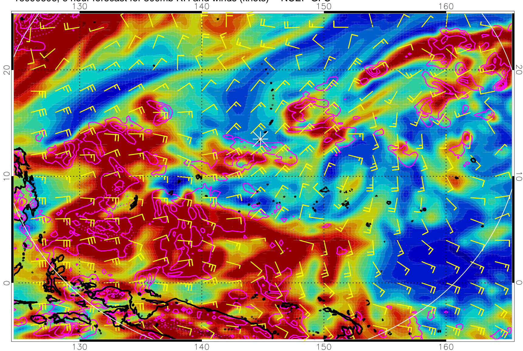
16090606, 6 hour forecast for 300mb RH and winds (knots) -- NCEP GFS
