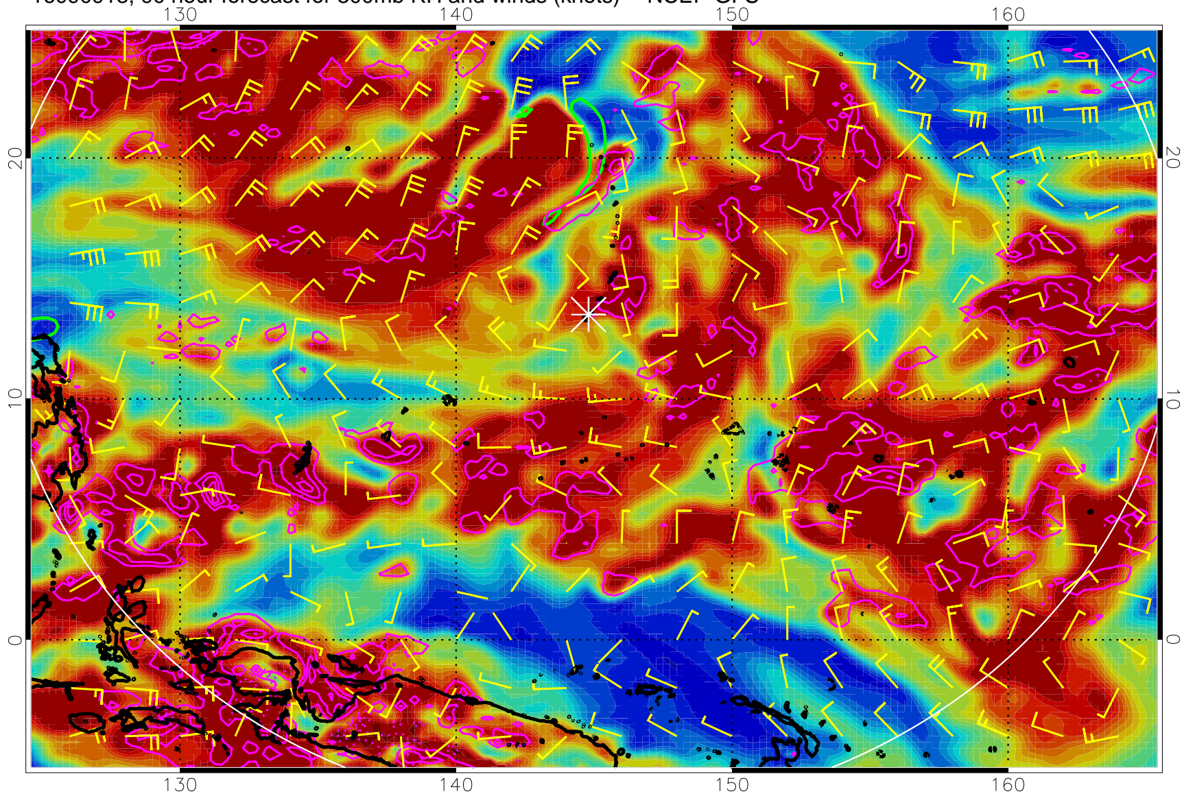
16090918, 90 hour forecast for 300mb RH and winds (knots) -- NCEP GFS
