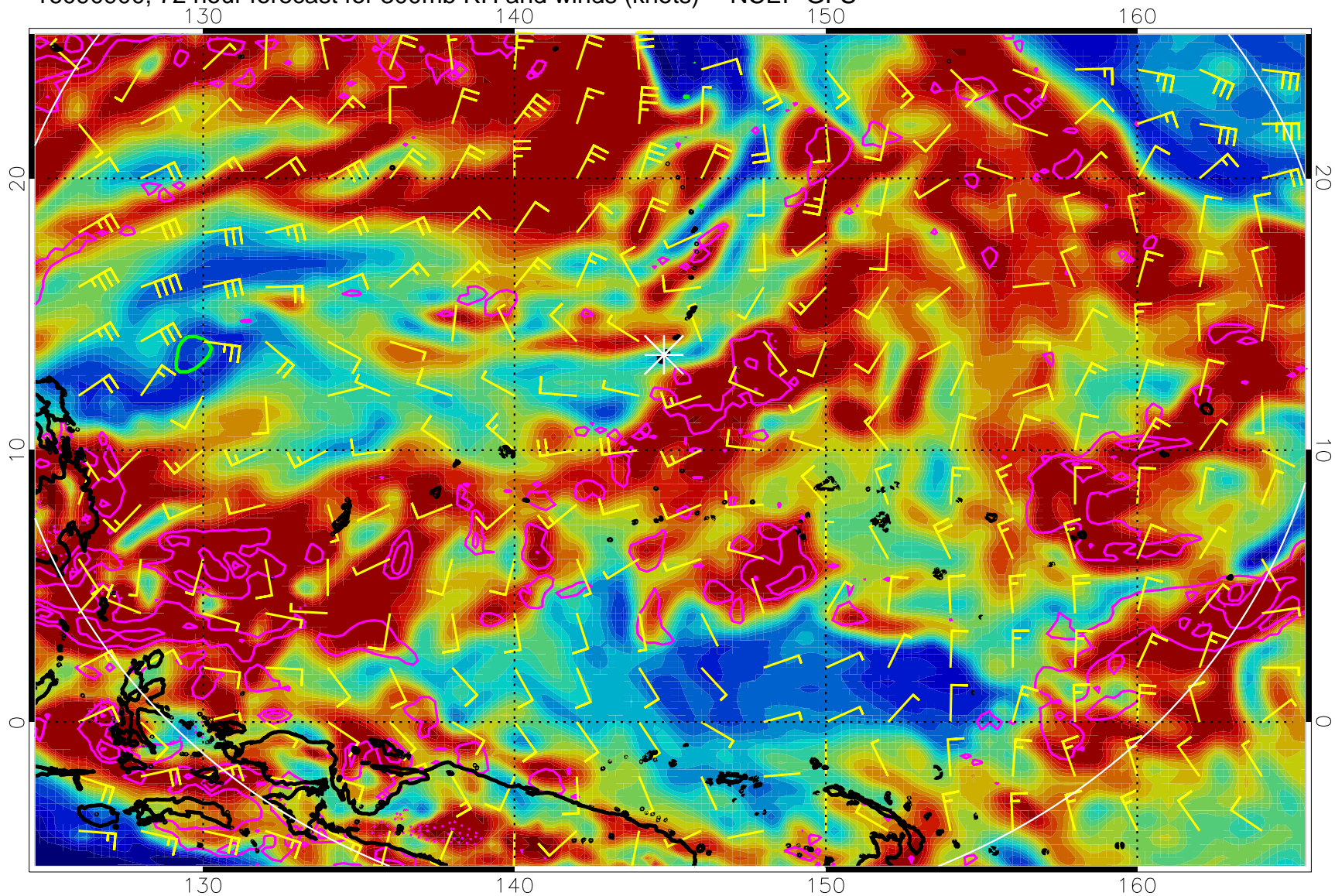
16090900, 72 hour forecast for 300mb RH and winds (knots) -- NCEP GFS
