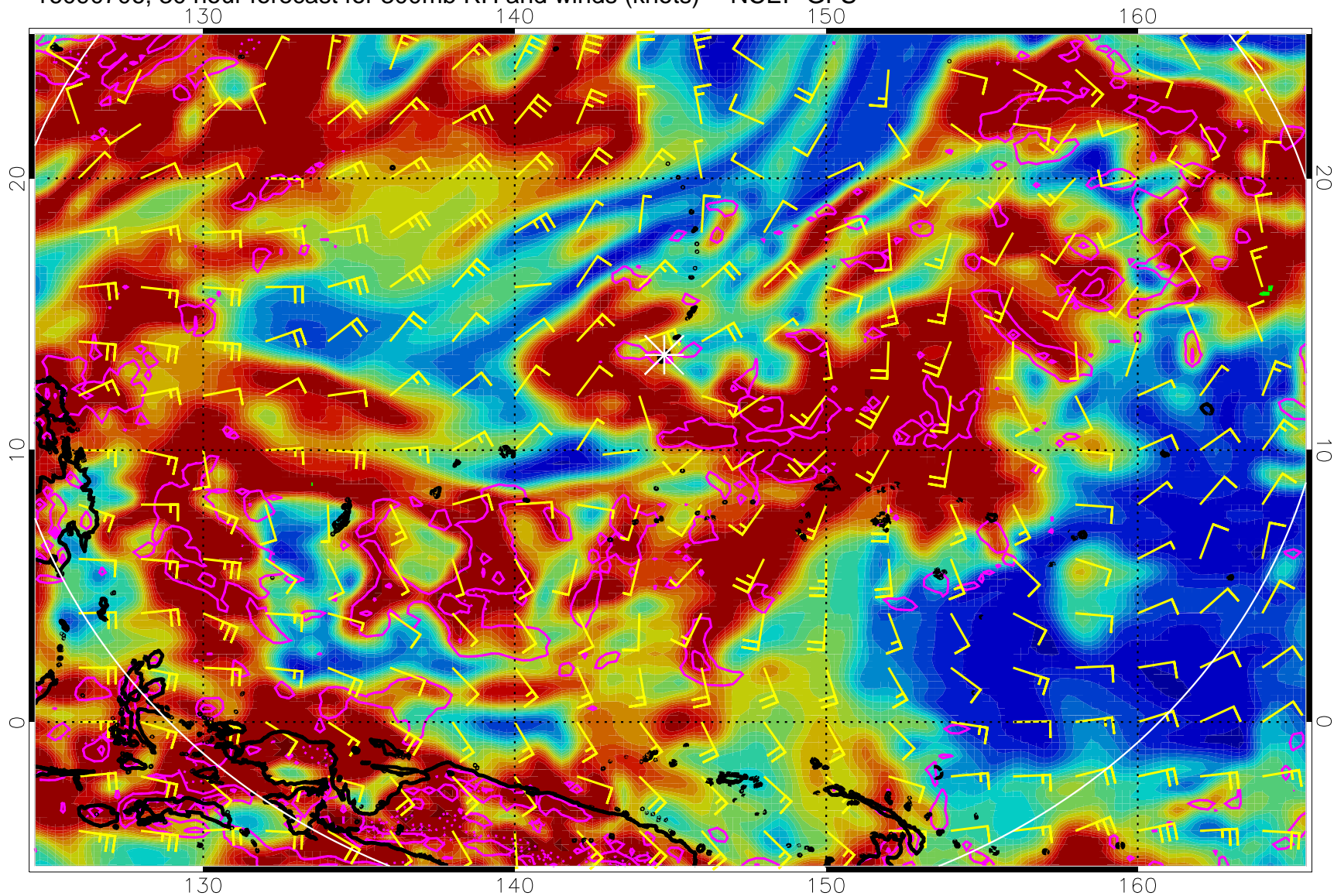
16090706, 30 hour forecast for 300mb RH and winds (knots) -- NCEP GFS
