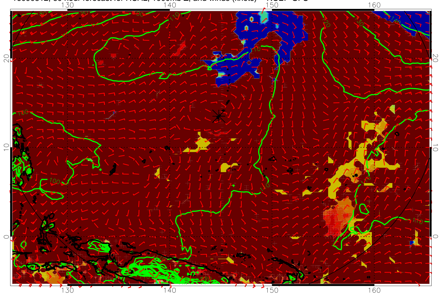
16090812, 60 hour forecast for HCAL, 1000mb Z, and winds (knots) -- NCEP GFS
