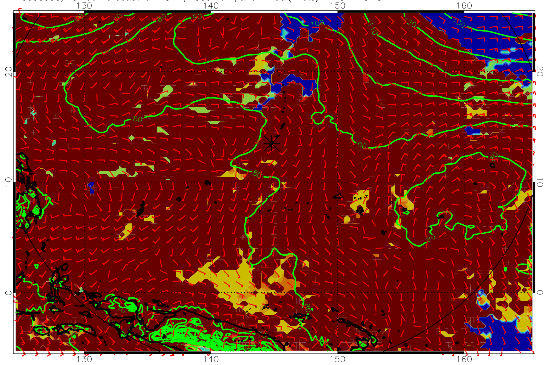
16090906, 78 hour forecast for HCAL, 1000mb Z, and winds (knots) -- NCEP GFS
