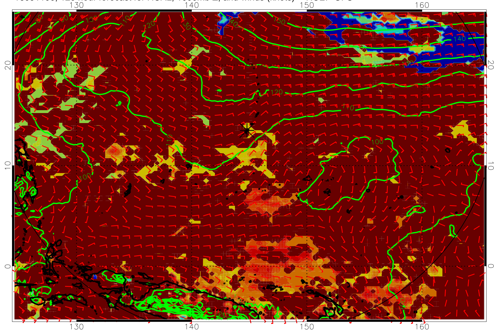
16091100, 120 hour forecast for HCAL, 1000mb Z, and winds (knots) -- NCEP GFS
