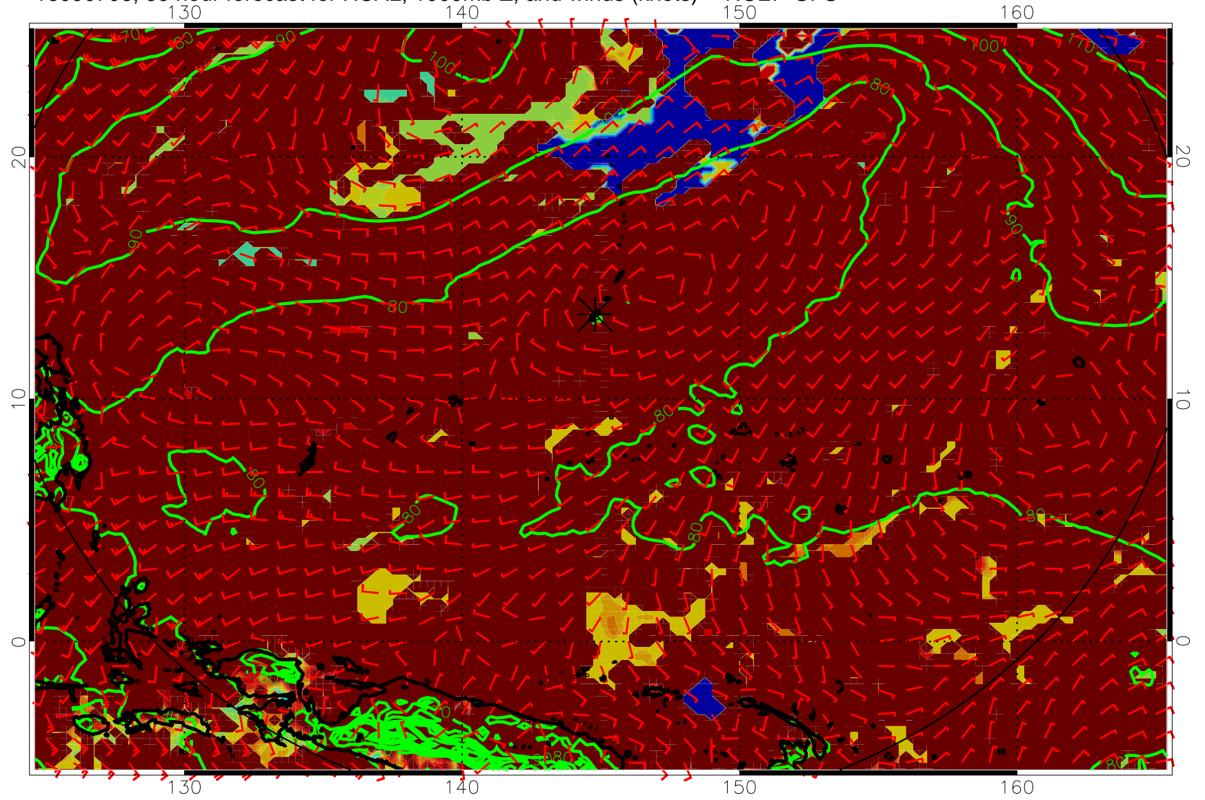
16090706, 30 hour forecast for HCAL, 1000mb Z, and winds (knots) -- NCEP GFS
