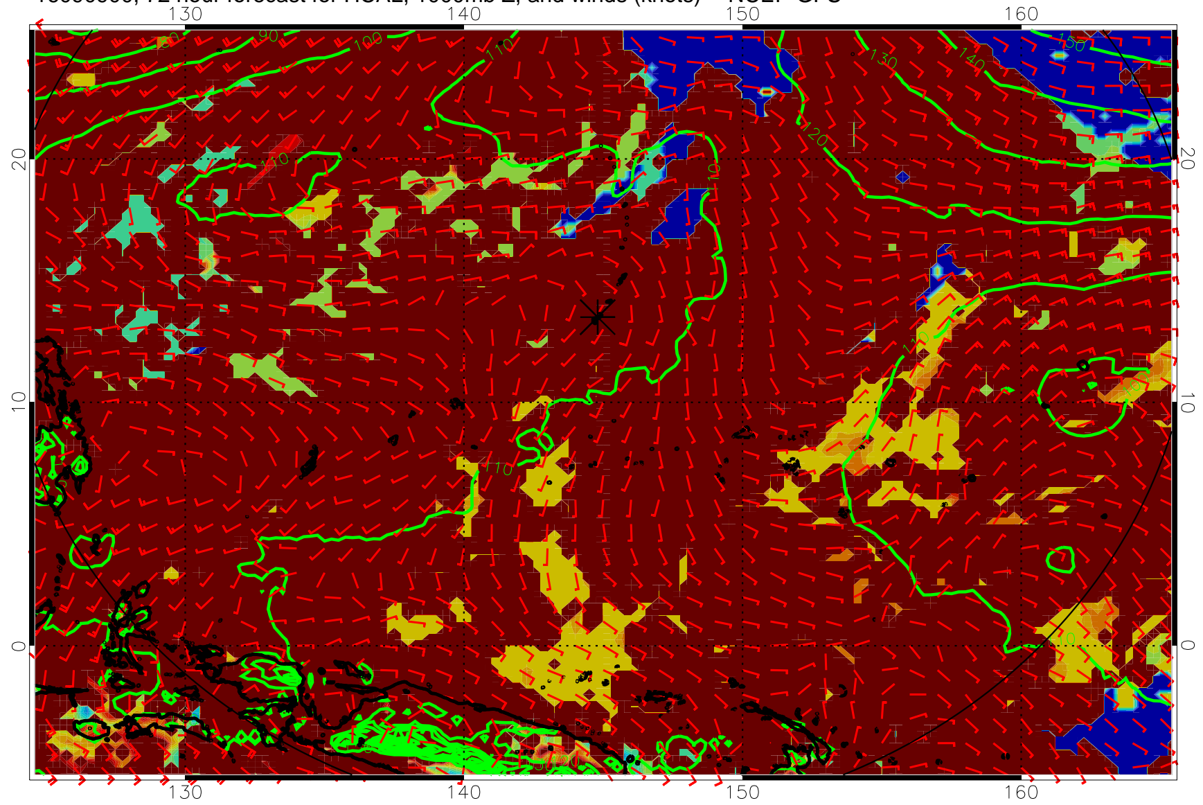
16090900, 72 hour forecast for HCAL, 1000mb Z, and winds (knots) -- NCEP GFS
