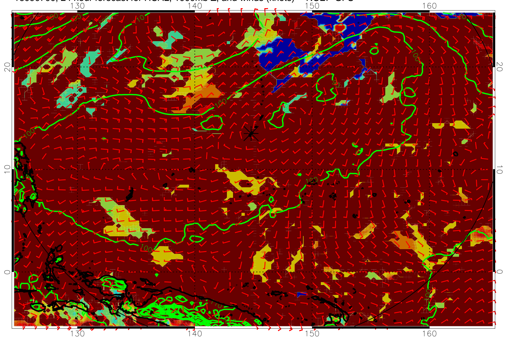
16090700, 24 hour forecast for HCAL, 1000mb Z, and winds (knots) -- NCEP GFS
