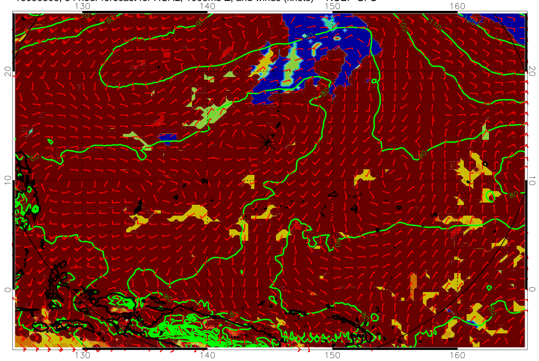
16090806, 54 hour forecast for HCAL, 1000mb Z, and winds (knots) -- NCEP GFS
