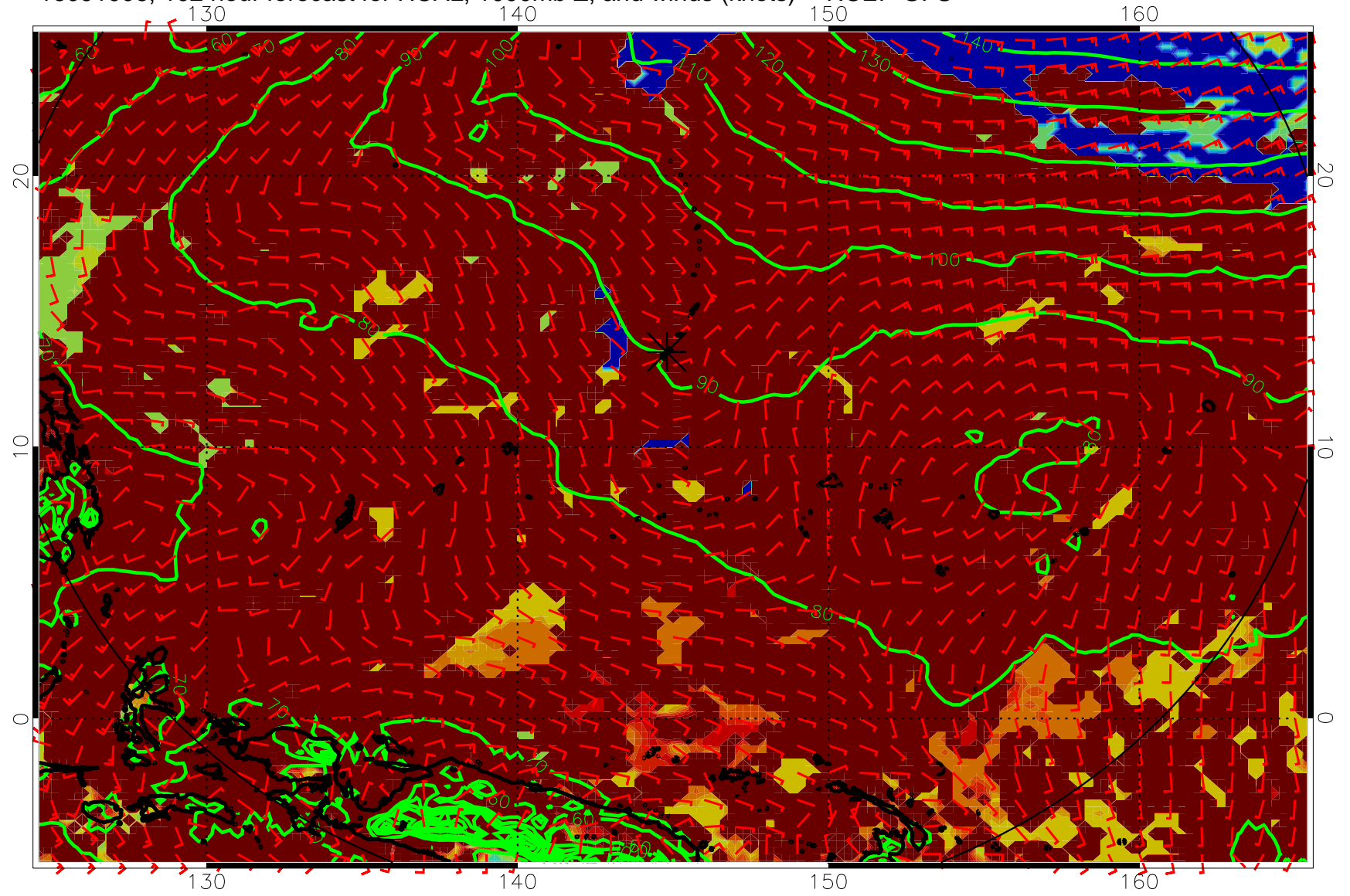
16091006, 102 hour forecast for HCAL, 1000mb Z, and winds (knots) -- NCEP GFS
