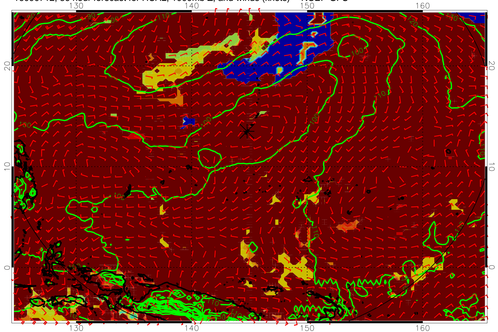
16090712, 36 hour forecast for HCAL, 1000mb Z, and winds (knots) -- NCEP GFS
