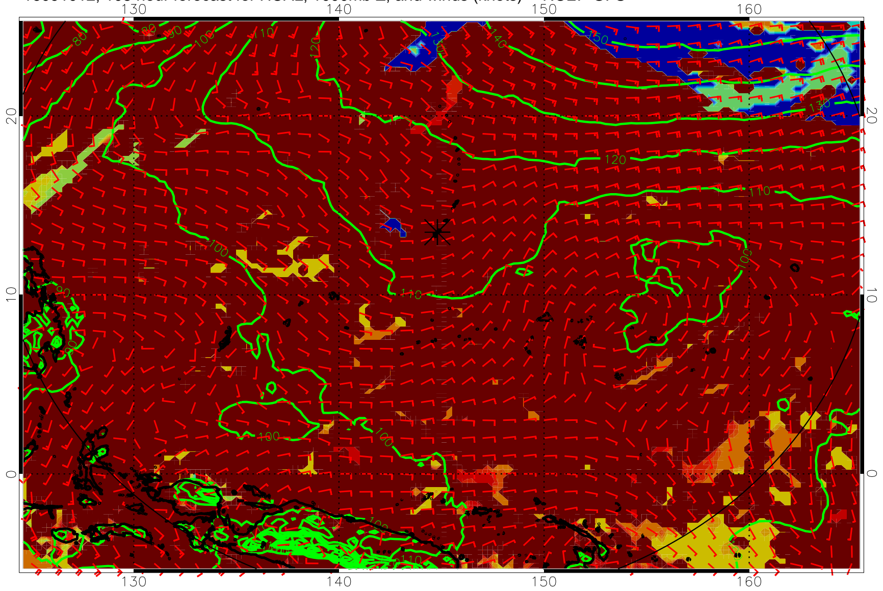
16091012, 108 hour forecast for HCAL, 1000mb Z, and winds (knots) -- NCEP GFS
