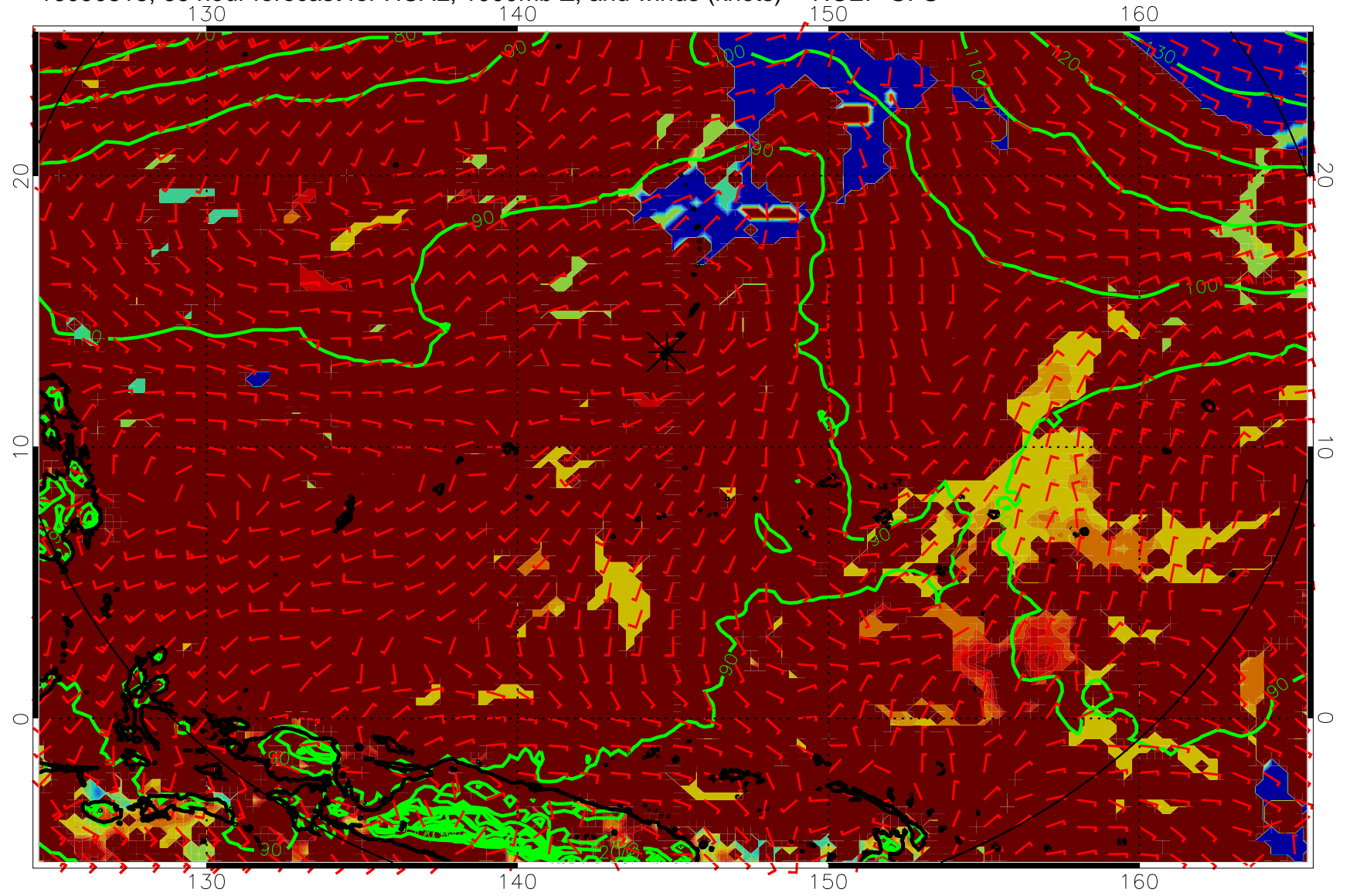
16090818, 66 hour forecast for HCAL, 1000mb Z, and winds (knots) -- NCEP GFS
