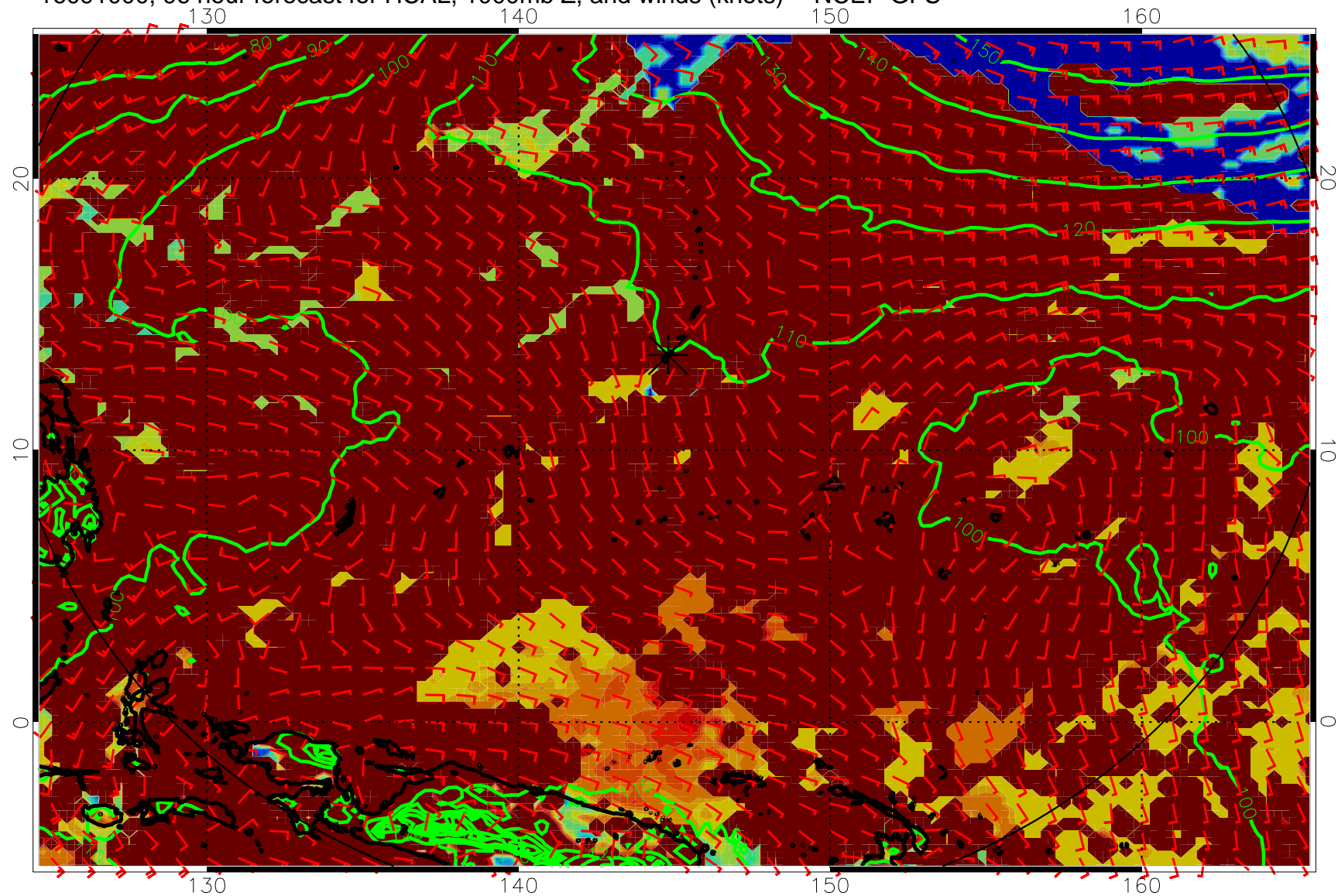
16091000, 96 hour forecast for HCAL, 1000mb Z, and winds (knots) -- NCEP GFS
