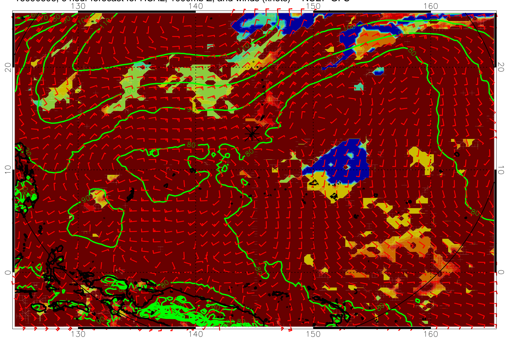
16090606, 6 hour forecast for HCAL, 1000mb Z, and winds (knots) -- NCEP GFS
