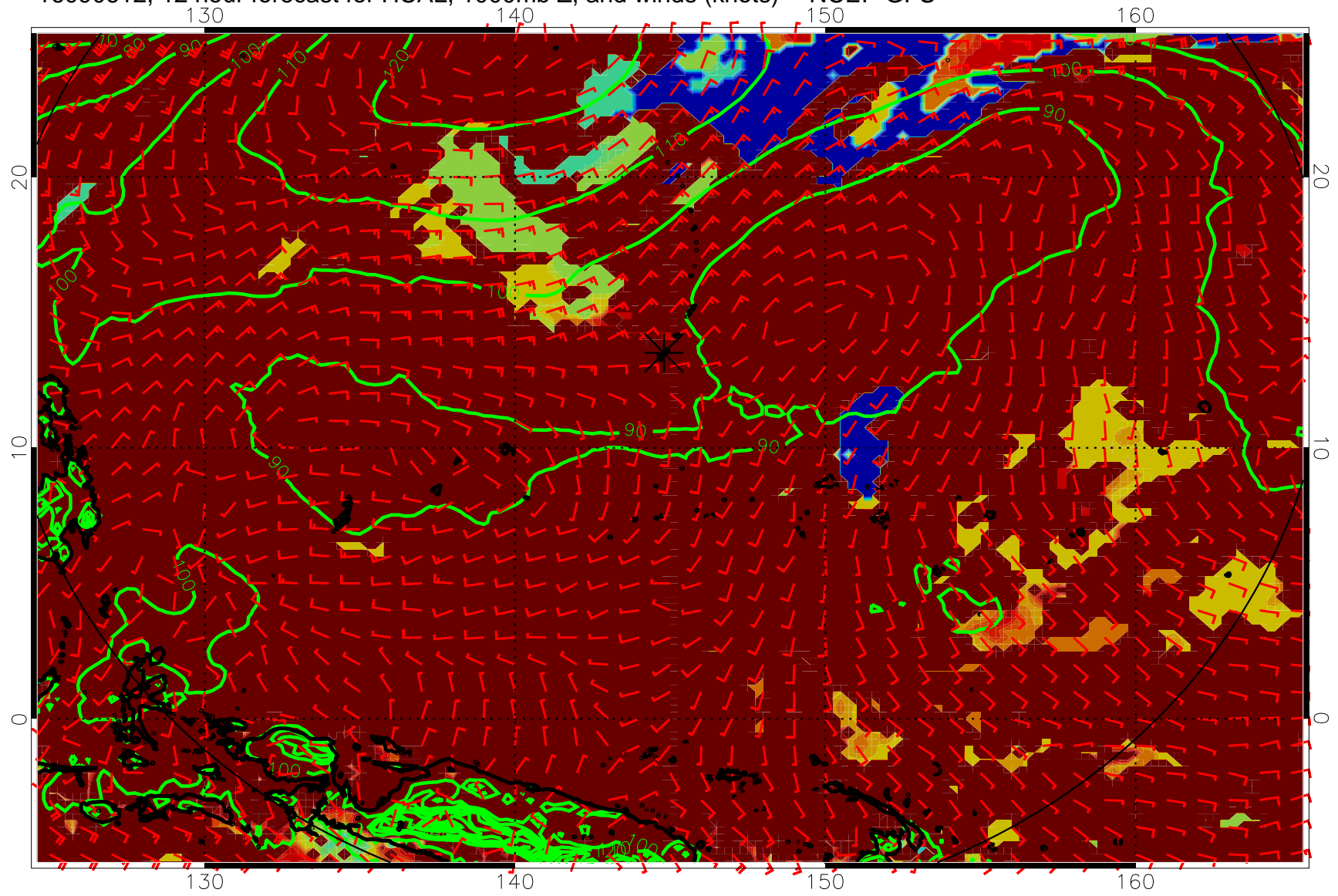
16090612, 12 hour forecast for HCAL, 1000mb Z, and winds (knots) -- NCEP GFS
