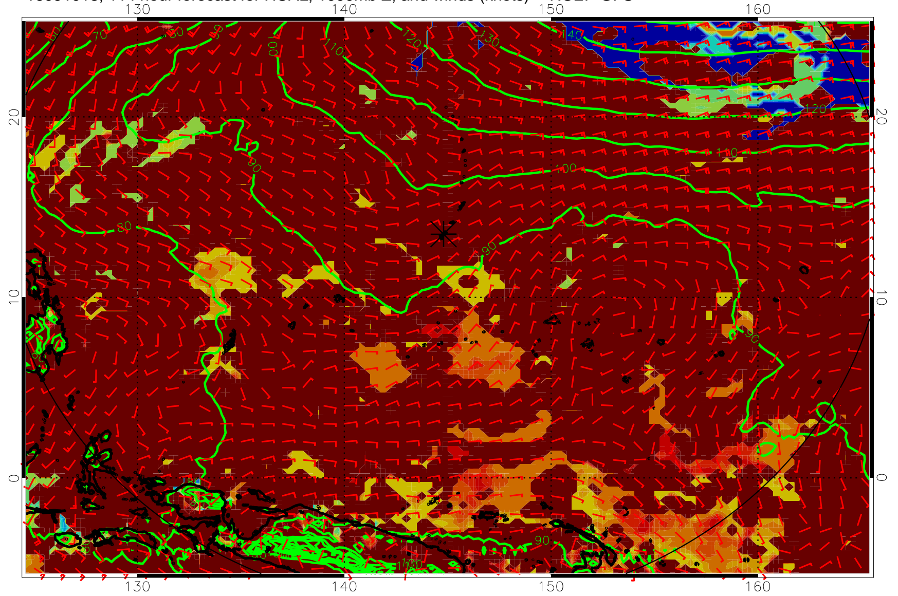
16091018, 114 hour forecast for HCAL, 1000mb Z, and winds (knots) -- NCEP GFS
