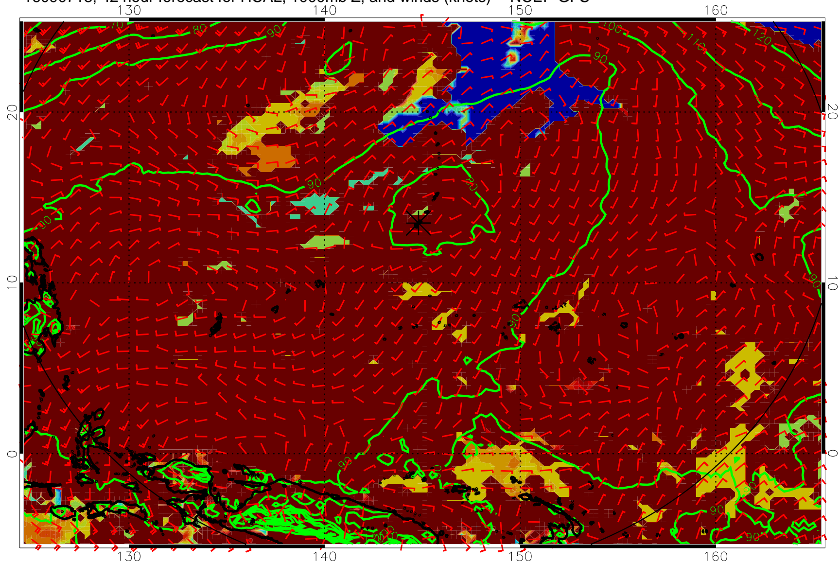
16090718, 42 hour forecast for HCAL, 1000mb Z, and winds (knots) -- NCEP GFS
