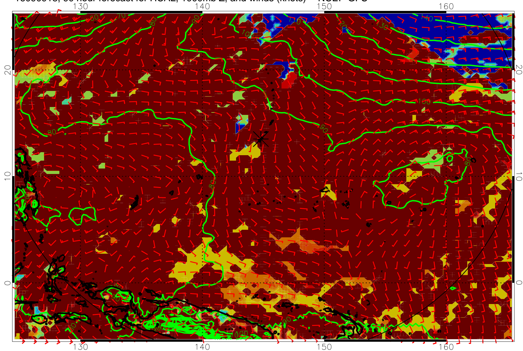
16090918, 90 hour forecast for HCAL, 1000mb Z, and winds (knots) -- NCEP GFS
