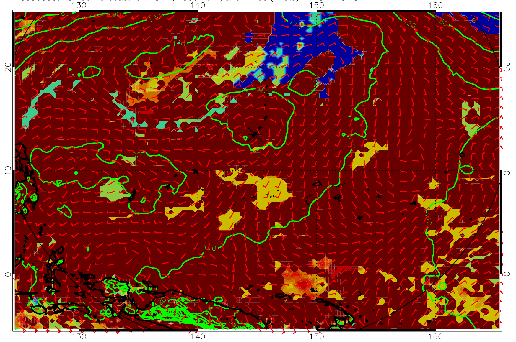
16090800, 48 hour forecast for HCAL, 1000mb Z, and winds (knots) -- NCEP GFS
