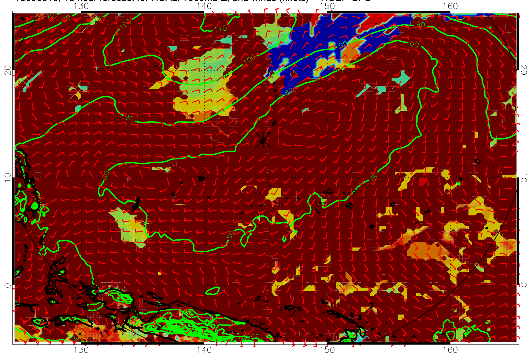
16090618, 18 hour forecast for HCAL, 1000mb Z, and winds (knots) -- NCEP GFS
