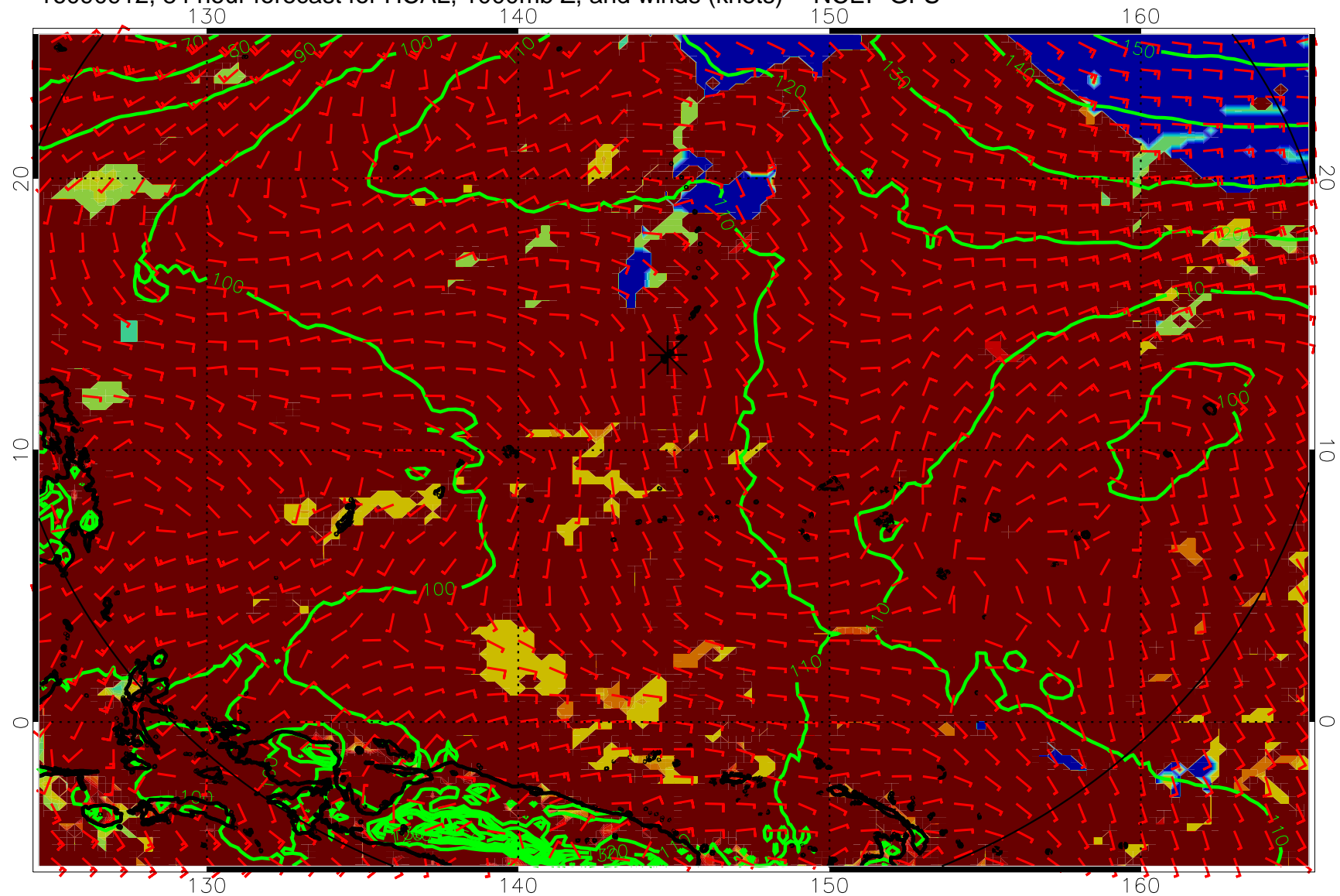
16090912, 84 hour forecast for HCAL, 1000mb Z, and winds (knots) -- NCEP GFS
