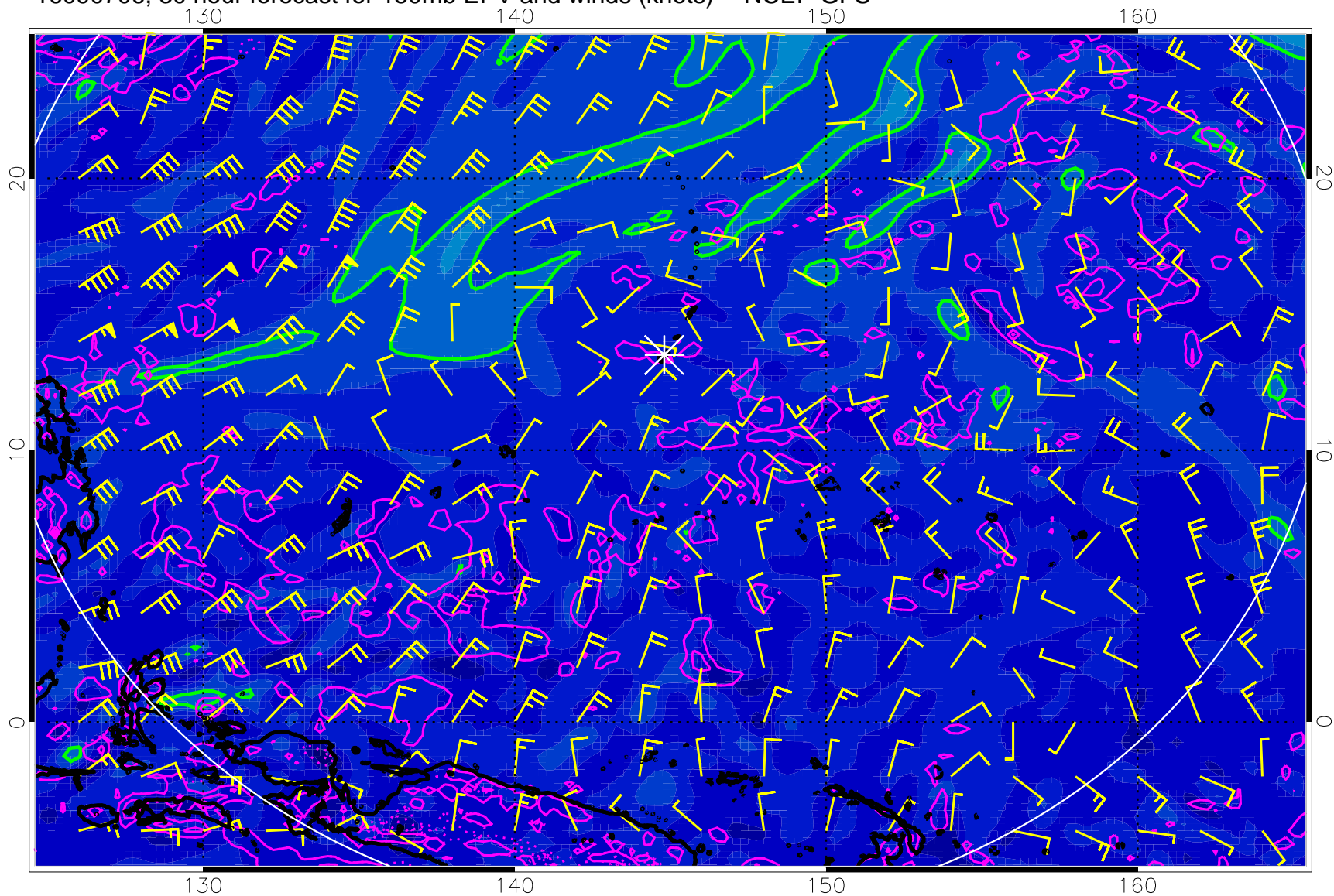
16090706, 30 hour forecast for 150mb EPV and winds (knots) -- NCEP GFS
