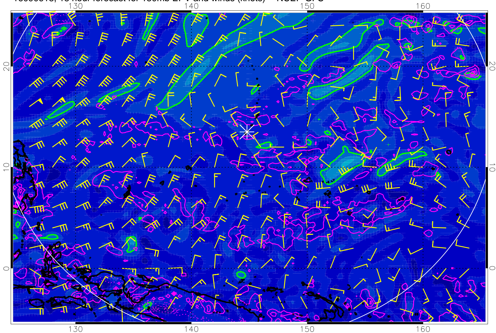
16090618, 18 hour forecast for 150mb EPV and winds (knots) -- NCEP GFS
