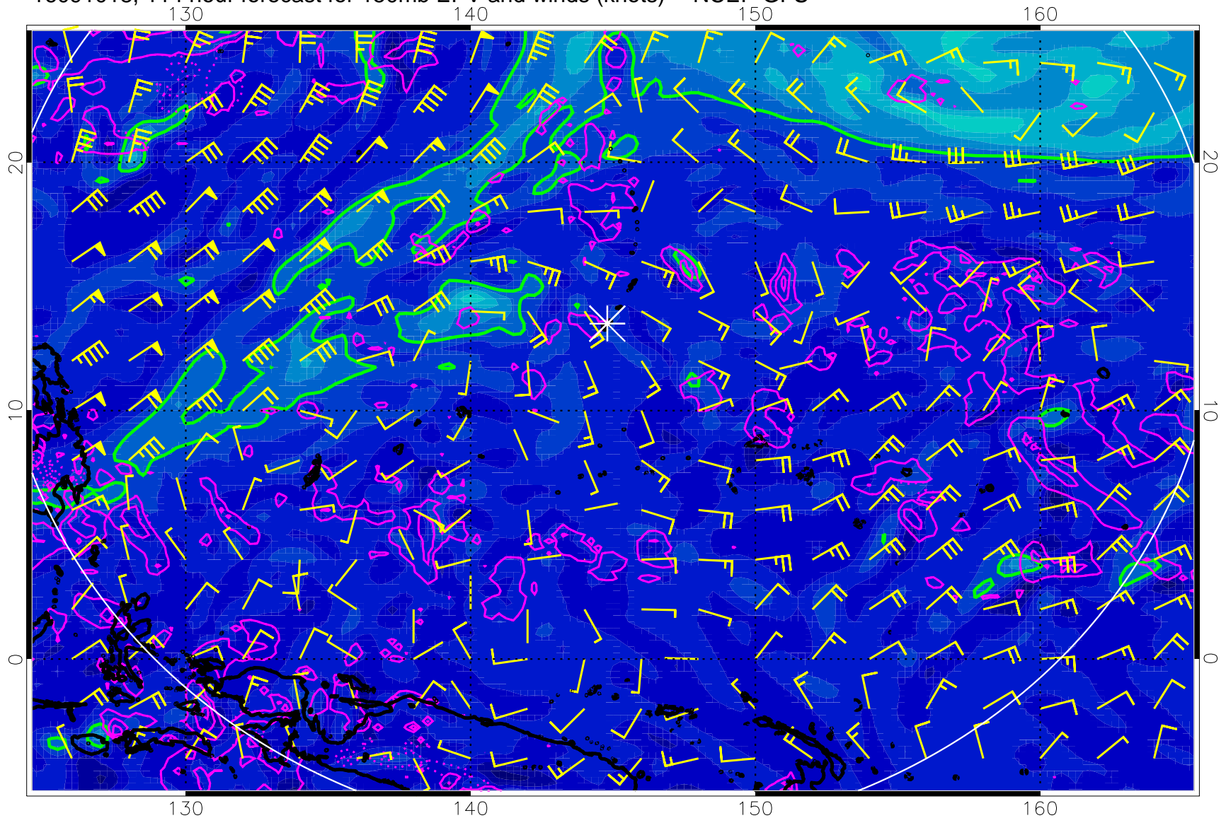
16091018, 114 hour forecast for 150mb EPV and winds (knots) -- NCEP GFS
