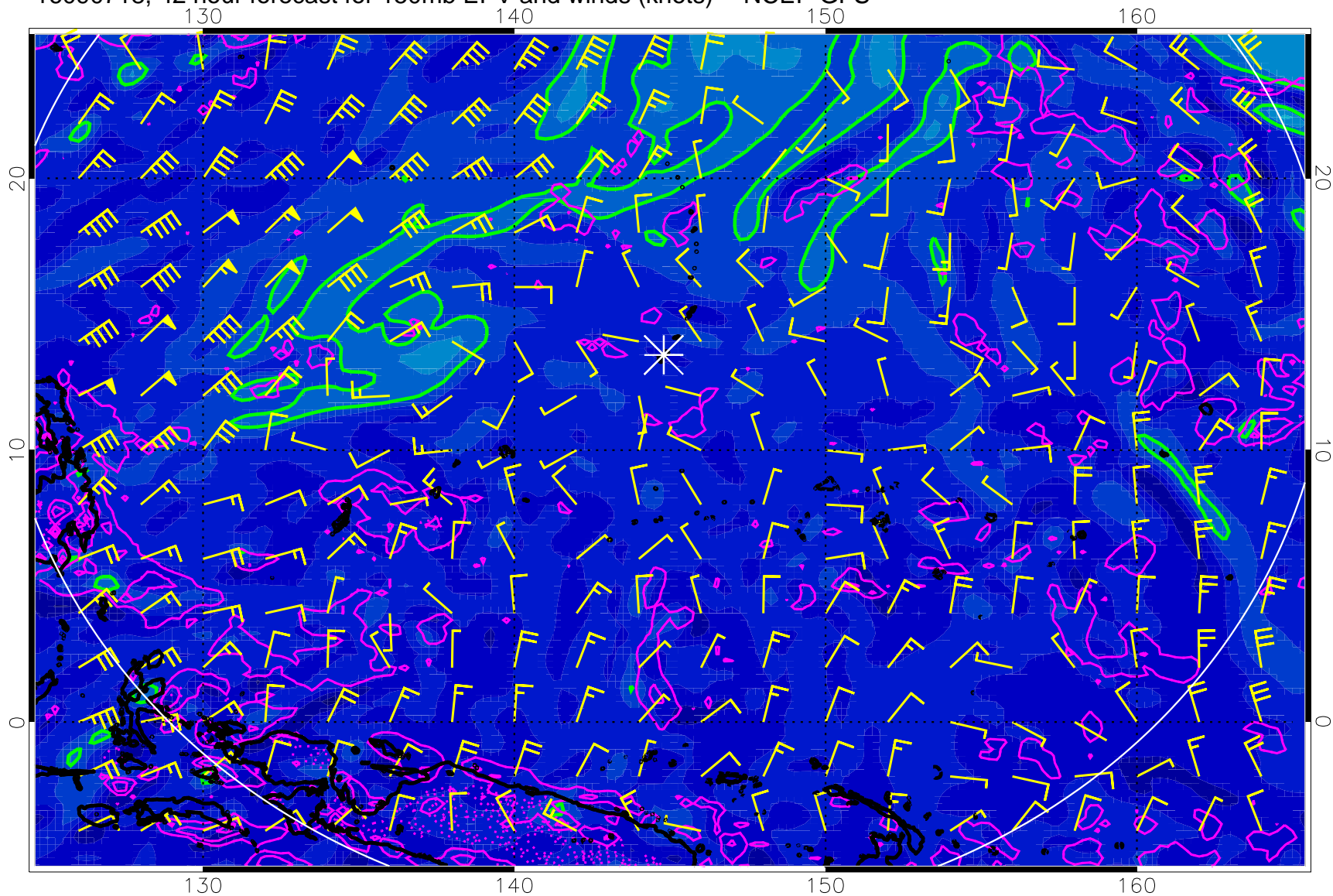
16090718, 42 hour forecast for 150mb EPV and winds (knots) -- NCEP GFS
