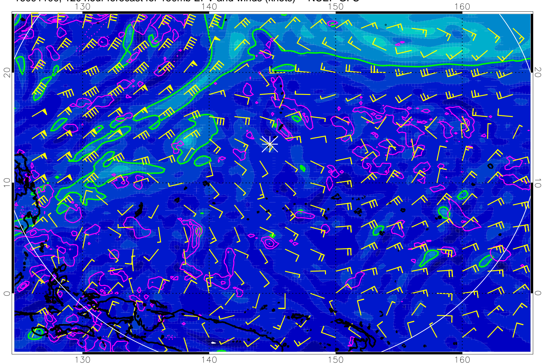
16091100, 120 hour forecast for 150mb EPV and winds (knots) -- NCEP GFS
