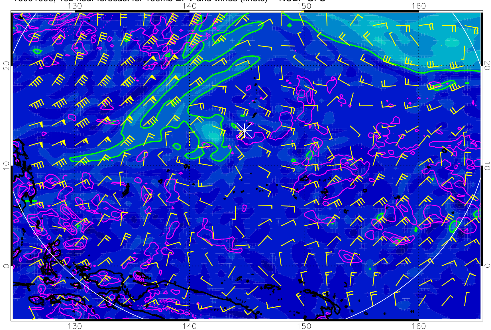
16091006, 102 hour forecast for 150mb EPV and winds (knots) -- NCEP GFS
