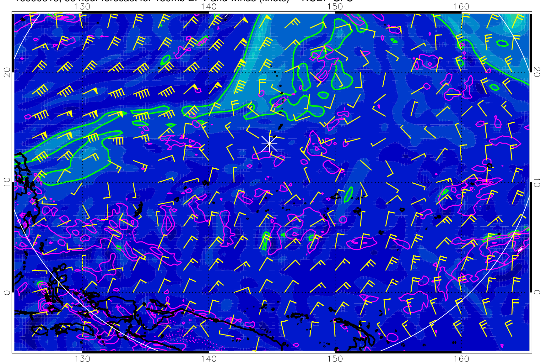
16090818, 66 hour forecast for 150mb EPV and winds (knots) -- NCEP GFS
