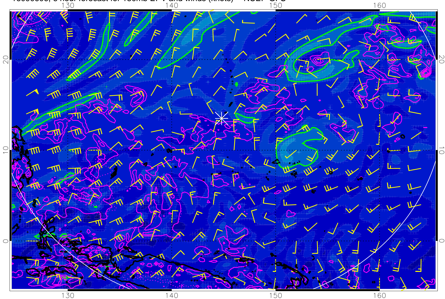
16090606, 6 hour forecast for 150mb EPV and winds (knots) -- NCEP GFS
