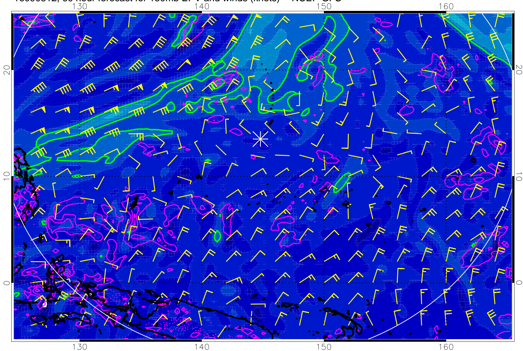
16090812, 60 hour forecast for 150mb EPV and winds (knots) -- NCEP GFS
