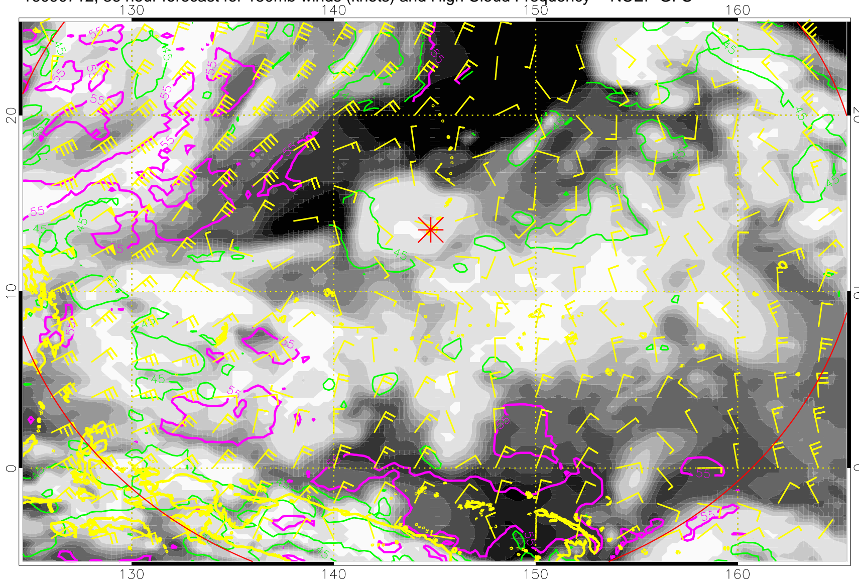
16090712, 36 hour forecast for 150mb winds (knots) and High Cloud Frequency -- NCEP GFS
