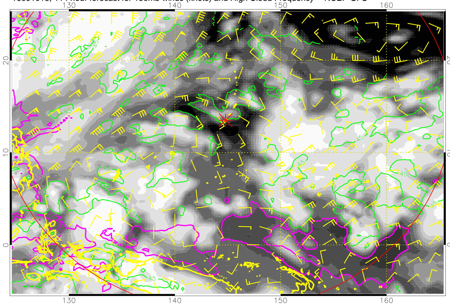
16091018, 114 hour forecast for 150mb winds (knots) and High Cloud Frequency -- NCEP GFS
