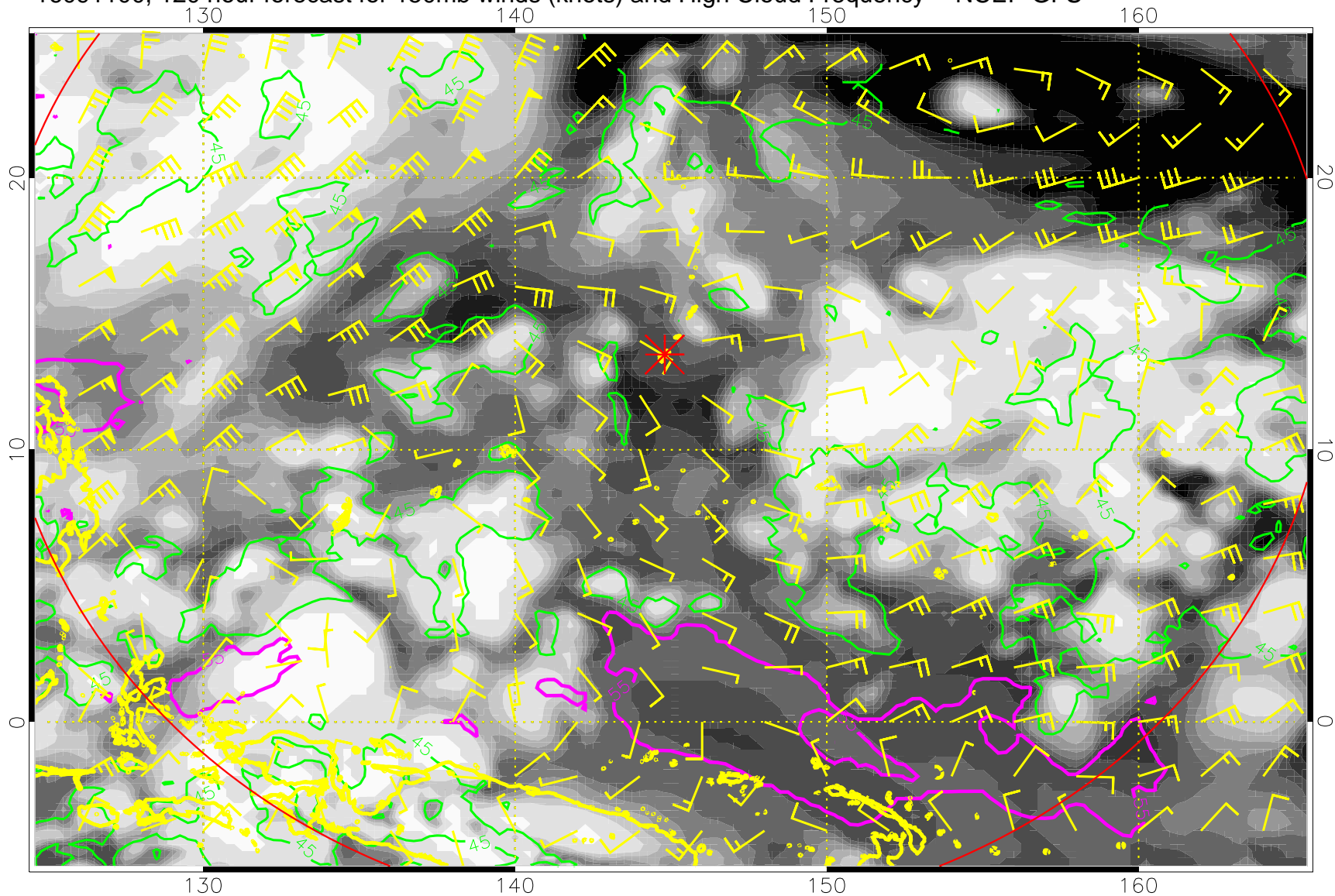
16091100, 120 hour forecast for 150mb winds (knots) and High Cloud Frequency -- NCEP GFS
