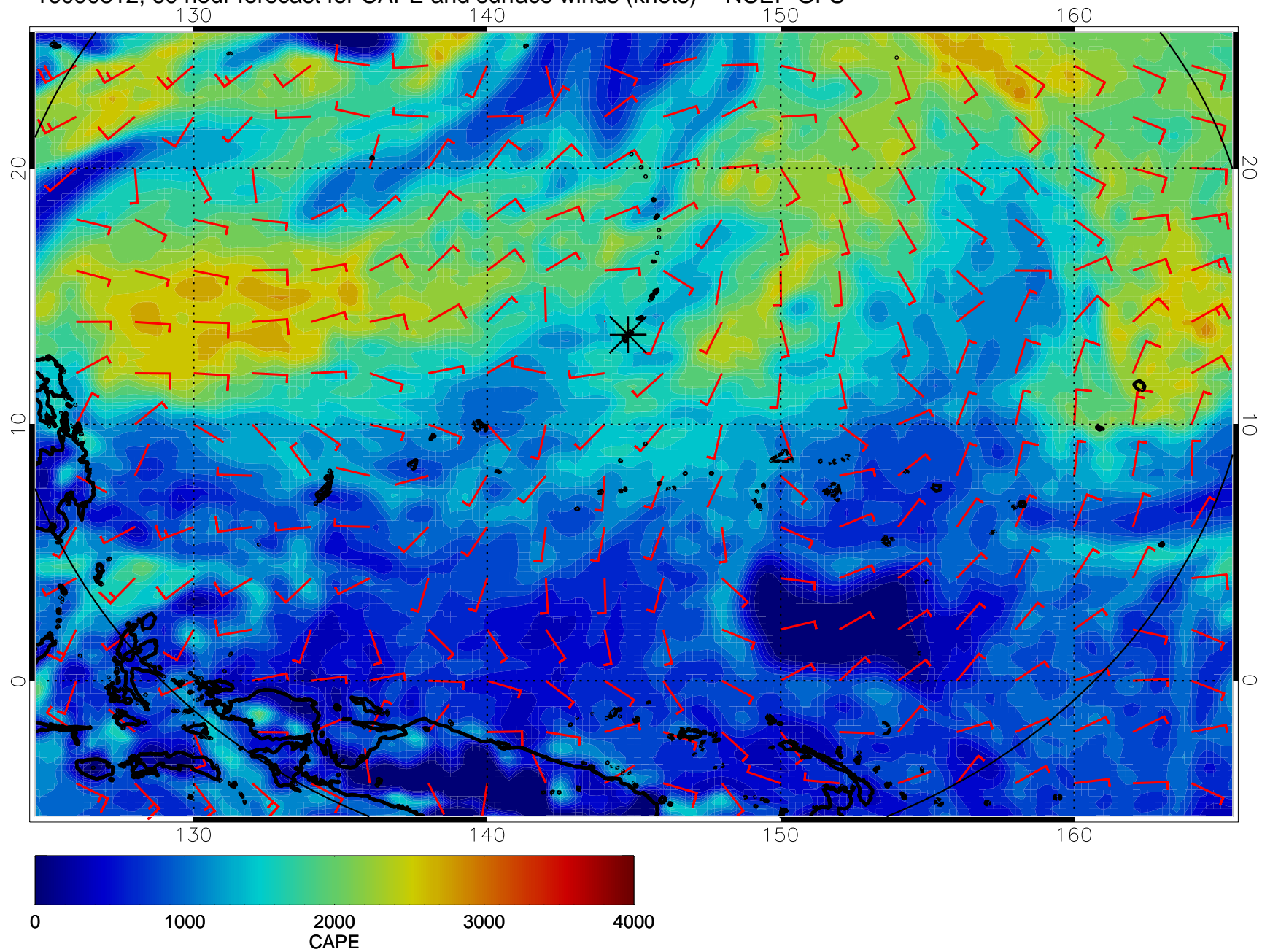
16090812, 60 hour forecast for CAPE and surface winds (knots) -- NCEP GFS
