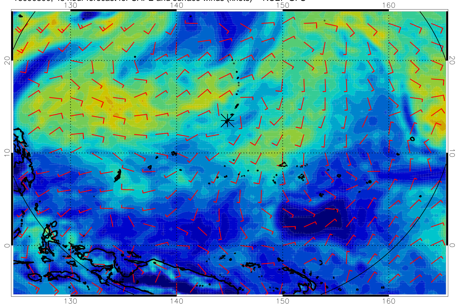
16090800, 48 hour forecast for CAPE and surface winds (knots) -- NCEP GFS
