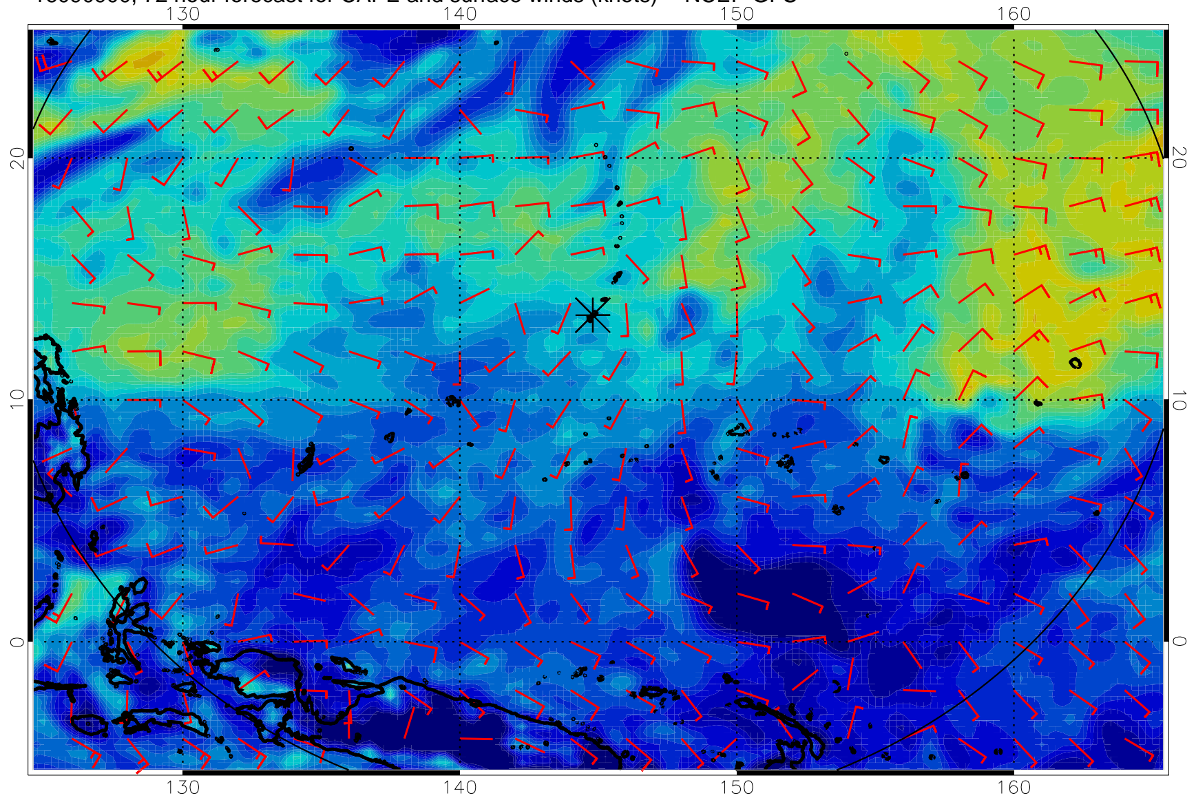
16090900, 72 hour forecast for CAPE and surface winds (knots) -- NCEP GFS
