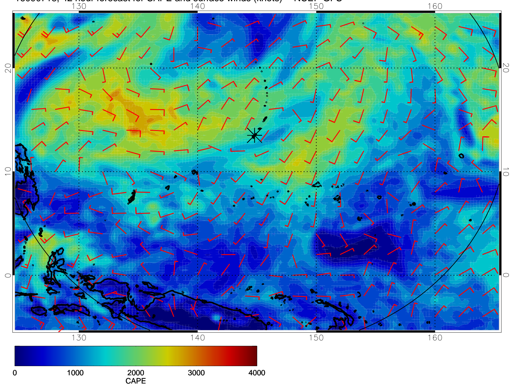
16090718, 42 hour forecast for CAPE and surface winds (knots) -- NCEP GFS
