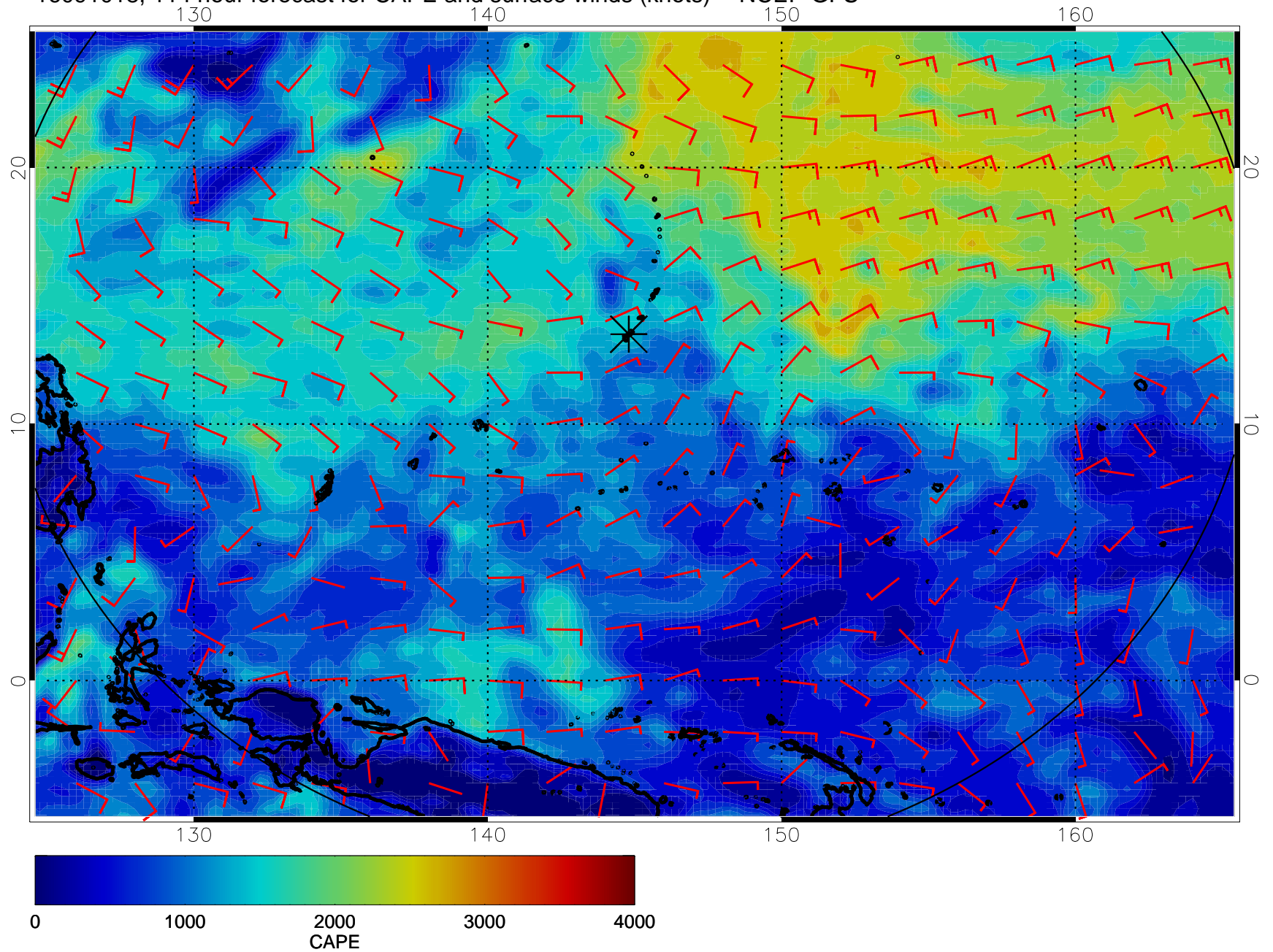
16091018, 114 hour forecast for CAPE and surface winds (knots) -- NCEP GFS
