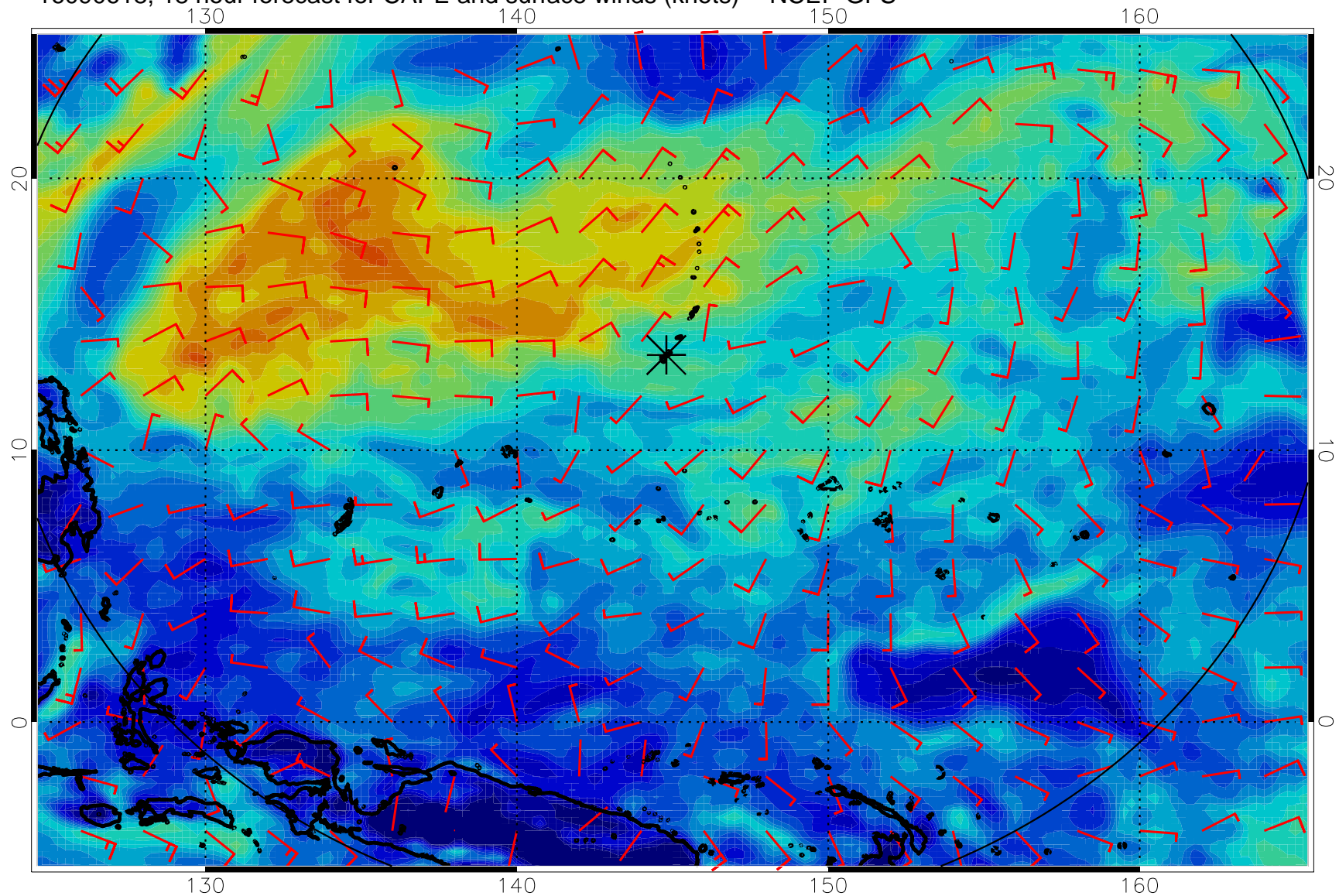
16090618, 18 hour forecast for CAPE and surface winds (knots) -- NCEP GFS
