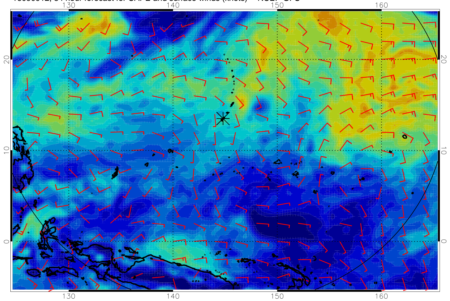
16090912, 84 hour forecast for CAPE and surface winds (knots) -- NCEP GFS
