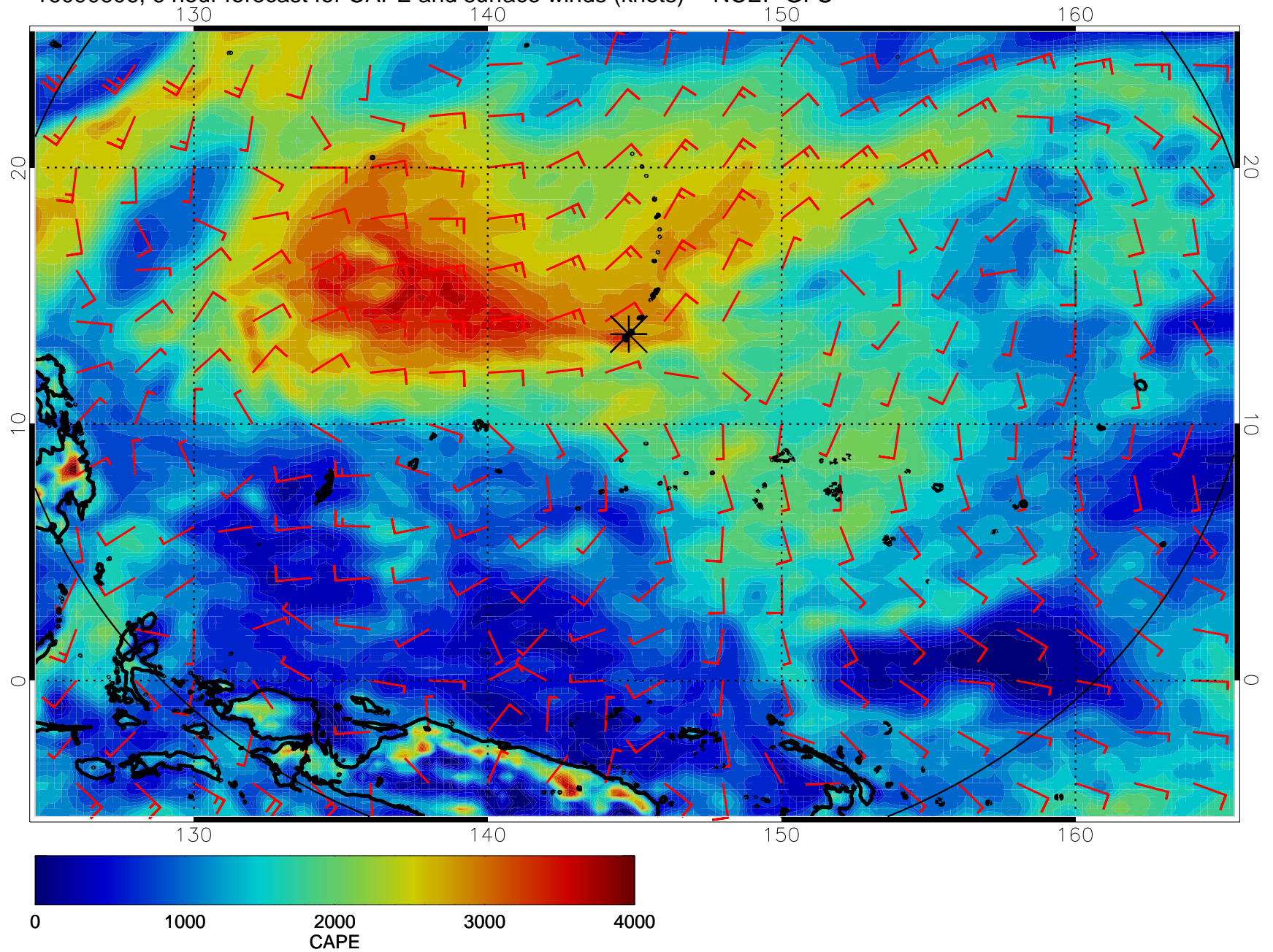
16090606, 6 hour forecast for CAPE and surface winds (knots) -- NCEP GFS
