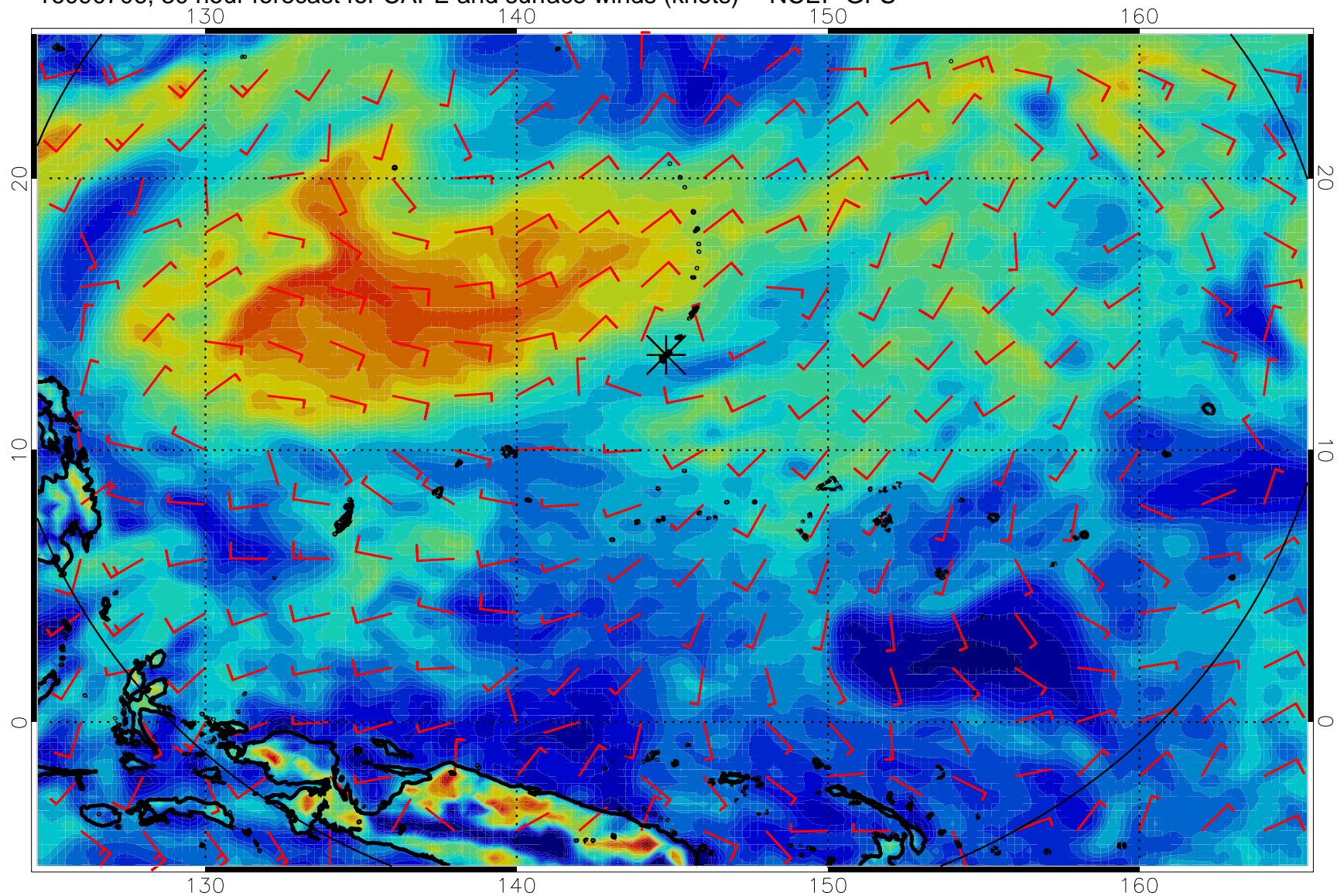
16090706, 30 hour forecast for CAPE and surface winds (knots) -- NCEP GFS
