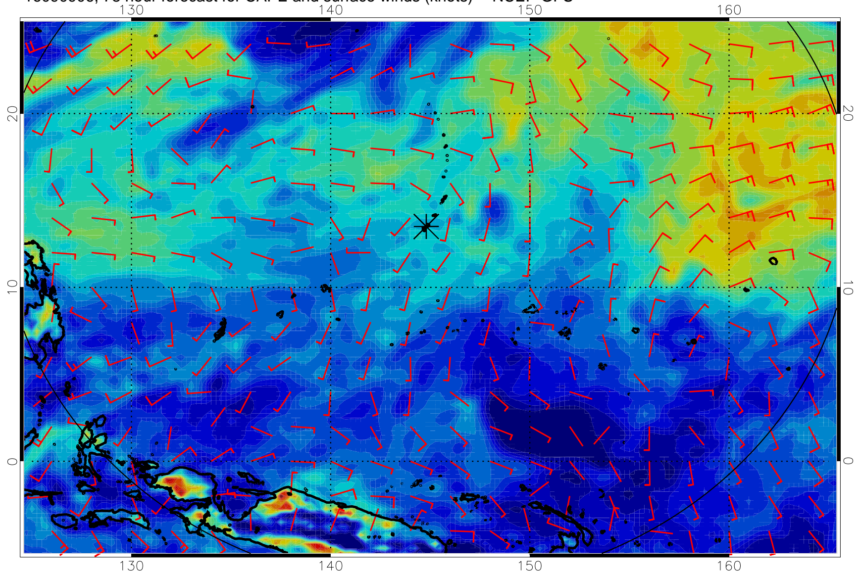
16090906, 78 hour forecast for CAPE and surface winds (knots) -- NCEP GFS
