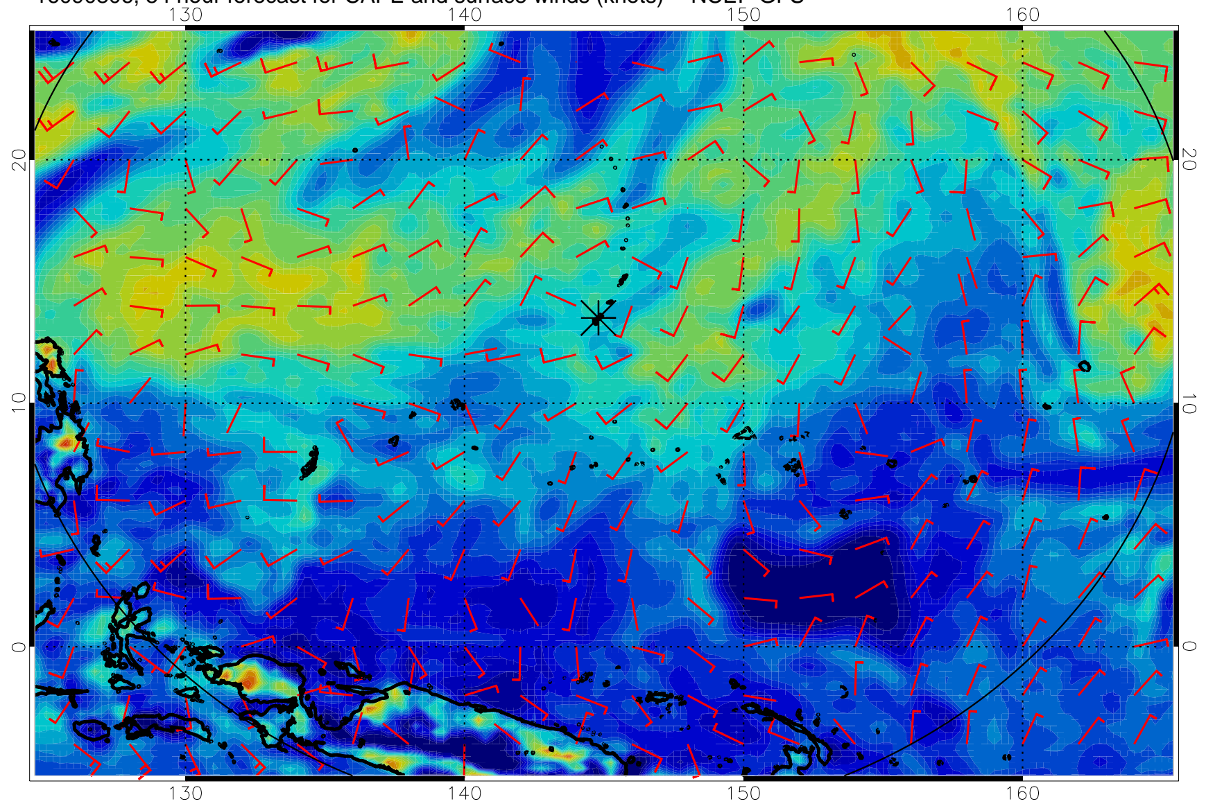
16090806, 54 hour forecast for CAPE and surface winds (knots) -- NCEP GFS
