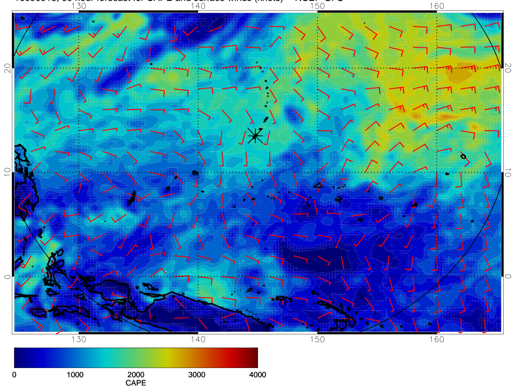
16090918, 90 hour forecast for CAPE and surface winds (knots) -- NCEP GFS
