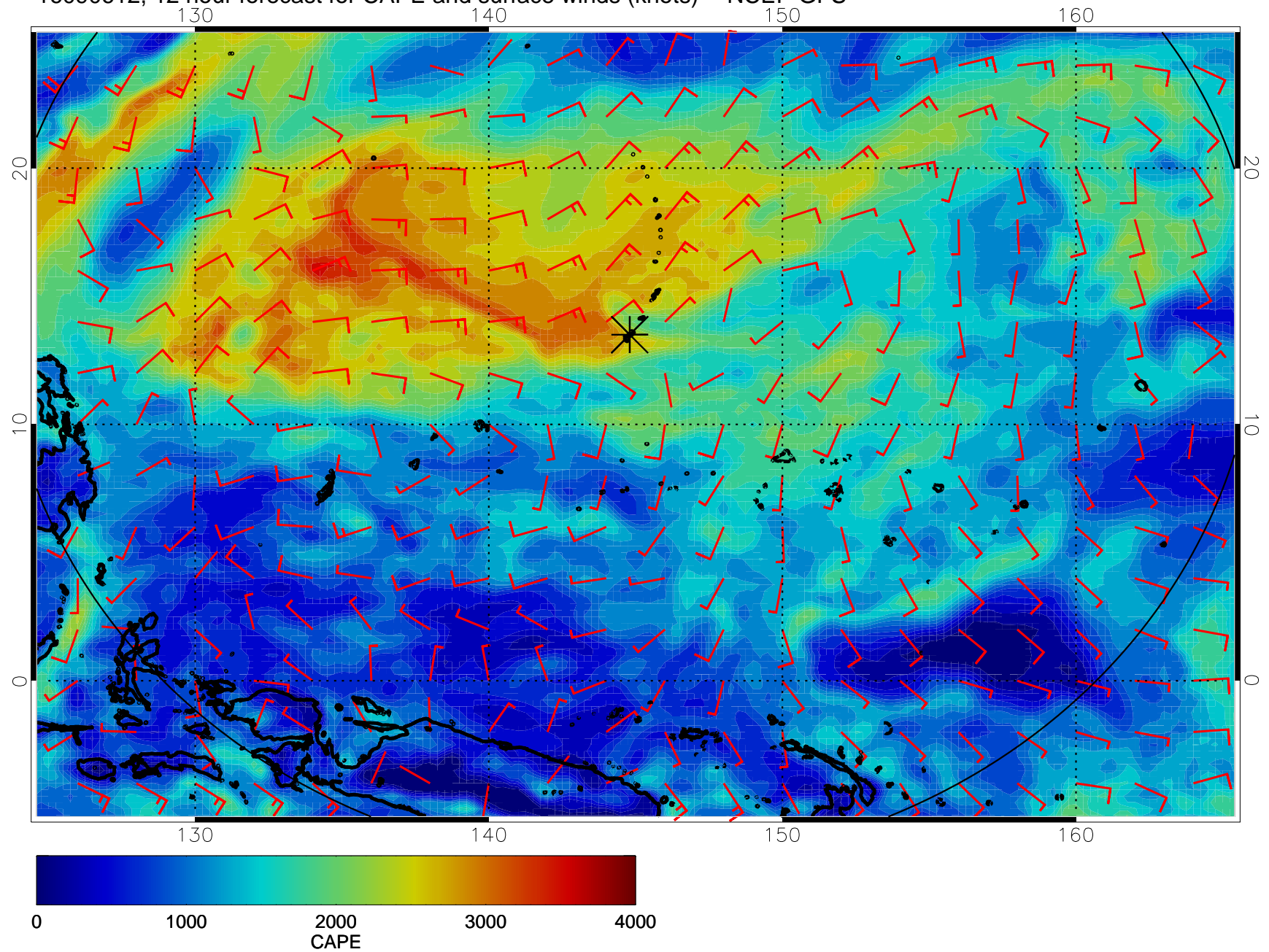
16090612, 12 hour forecast for CAPE and surface winds (knots) -- NCEP GFS
