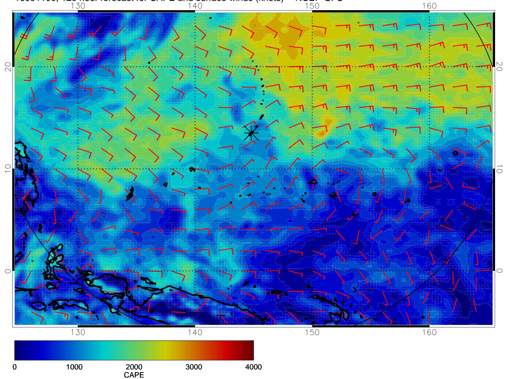
16091100, 120 hour forecast for CAPE and surface winds (knots) -- NCEP GFS
