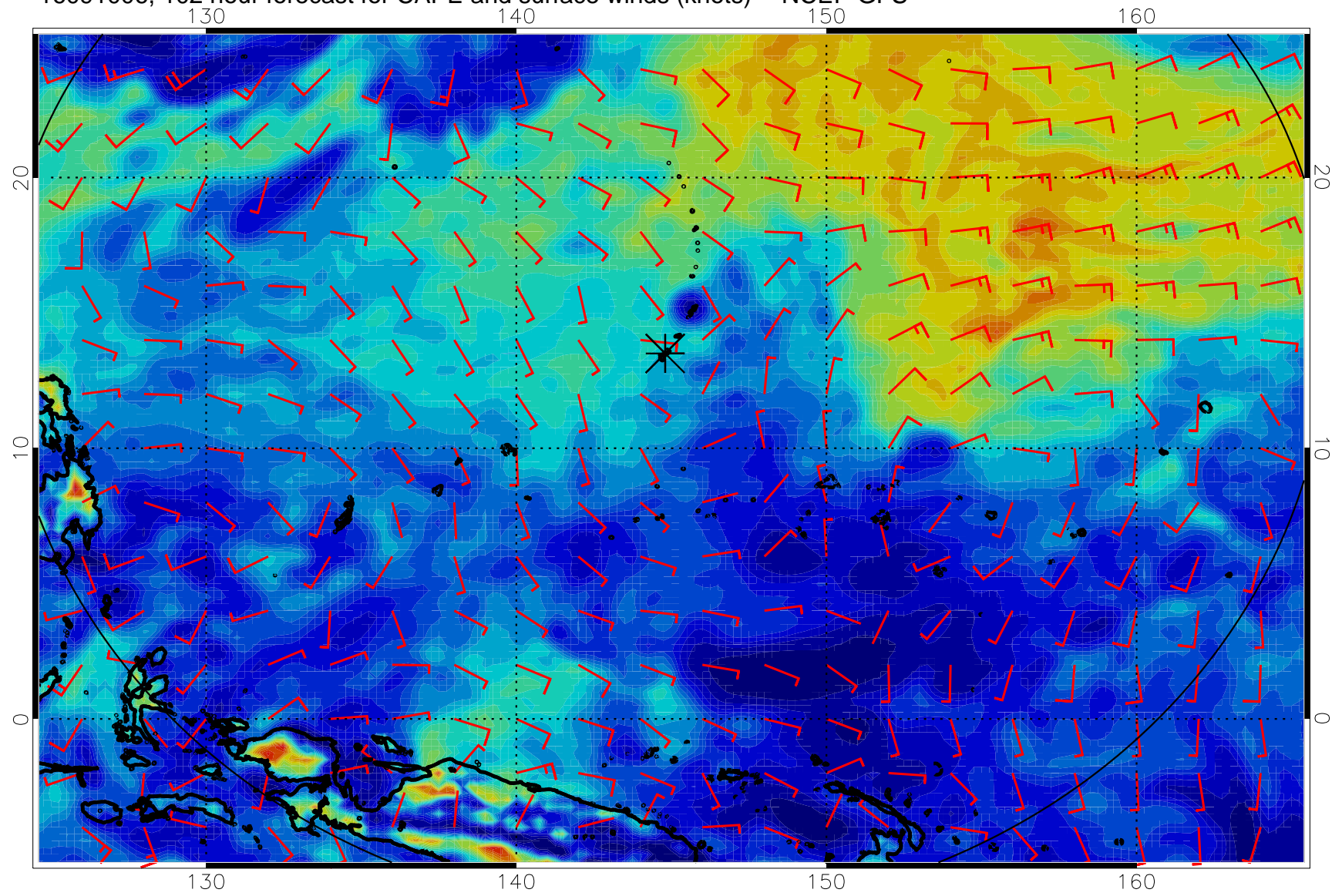
16091006, 102 hour forecast for CAPE and surface winds (knots) -- NCEP GFS
