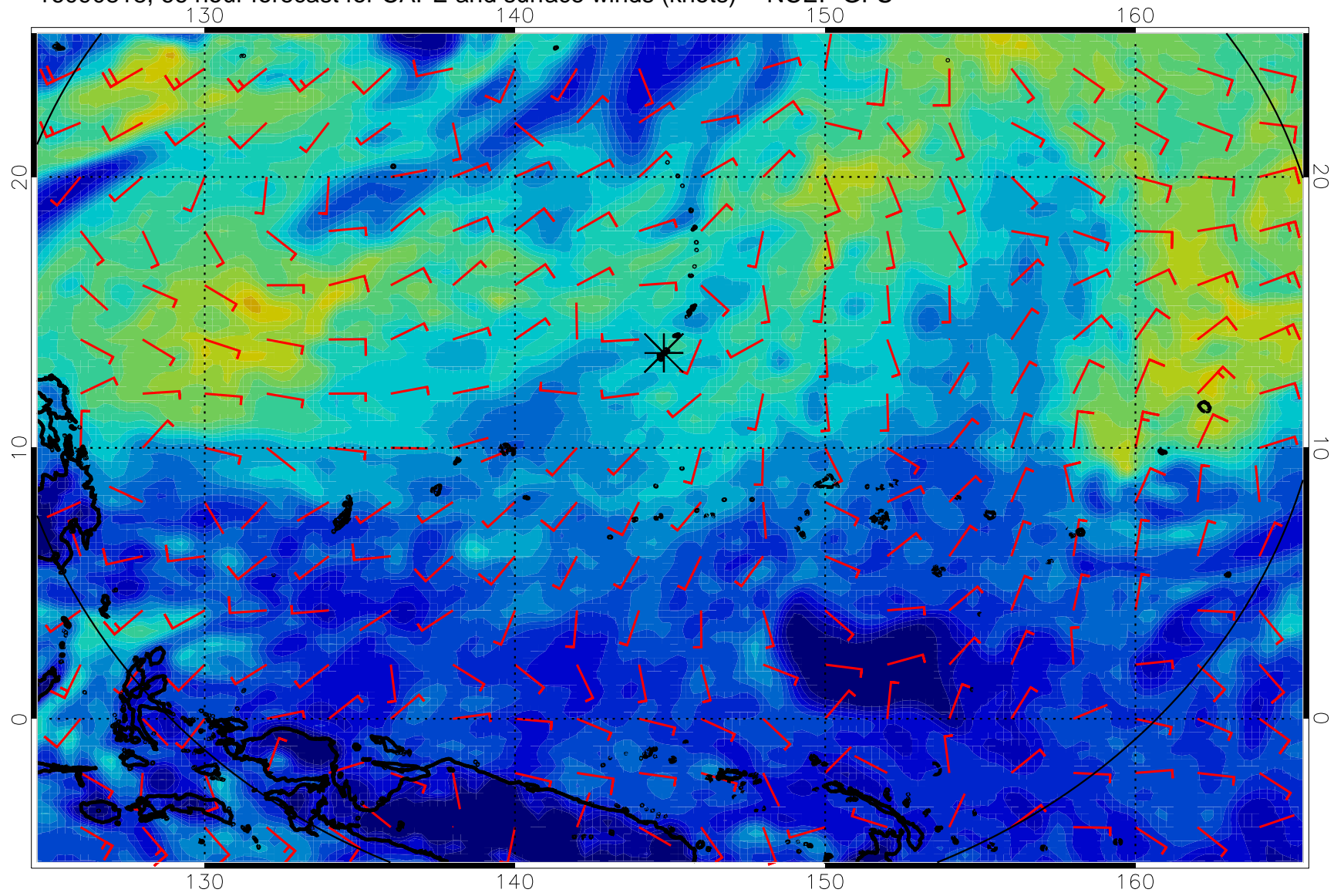
16090818, 66 hour forecast for CAPE and surface winds (knots) -- NCEP GFS
