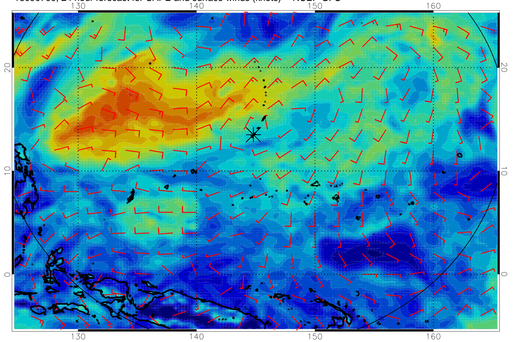
16090700, 24 hour forecast for CAPE and surface winds (knots) -- NCEP GFS
