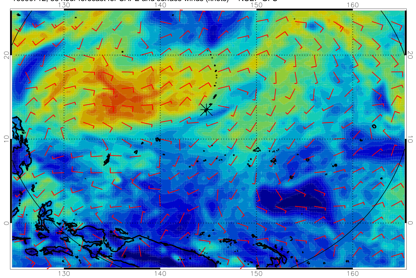
16090712, 36 hour forecast for CAPE and surface winds (knots) -- NCEP GFS
