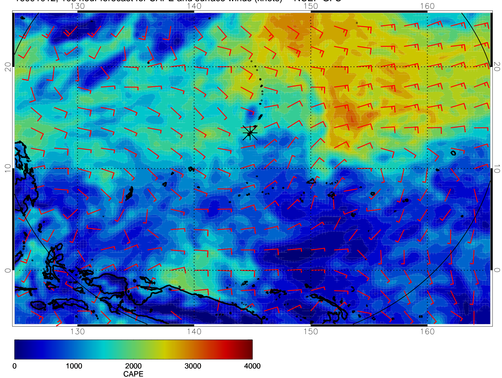
16091012, 108 hour forecast for CAPE and surface winds (knots) -- NCEP GFS
