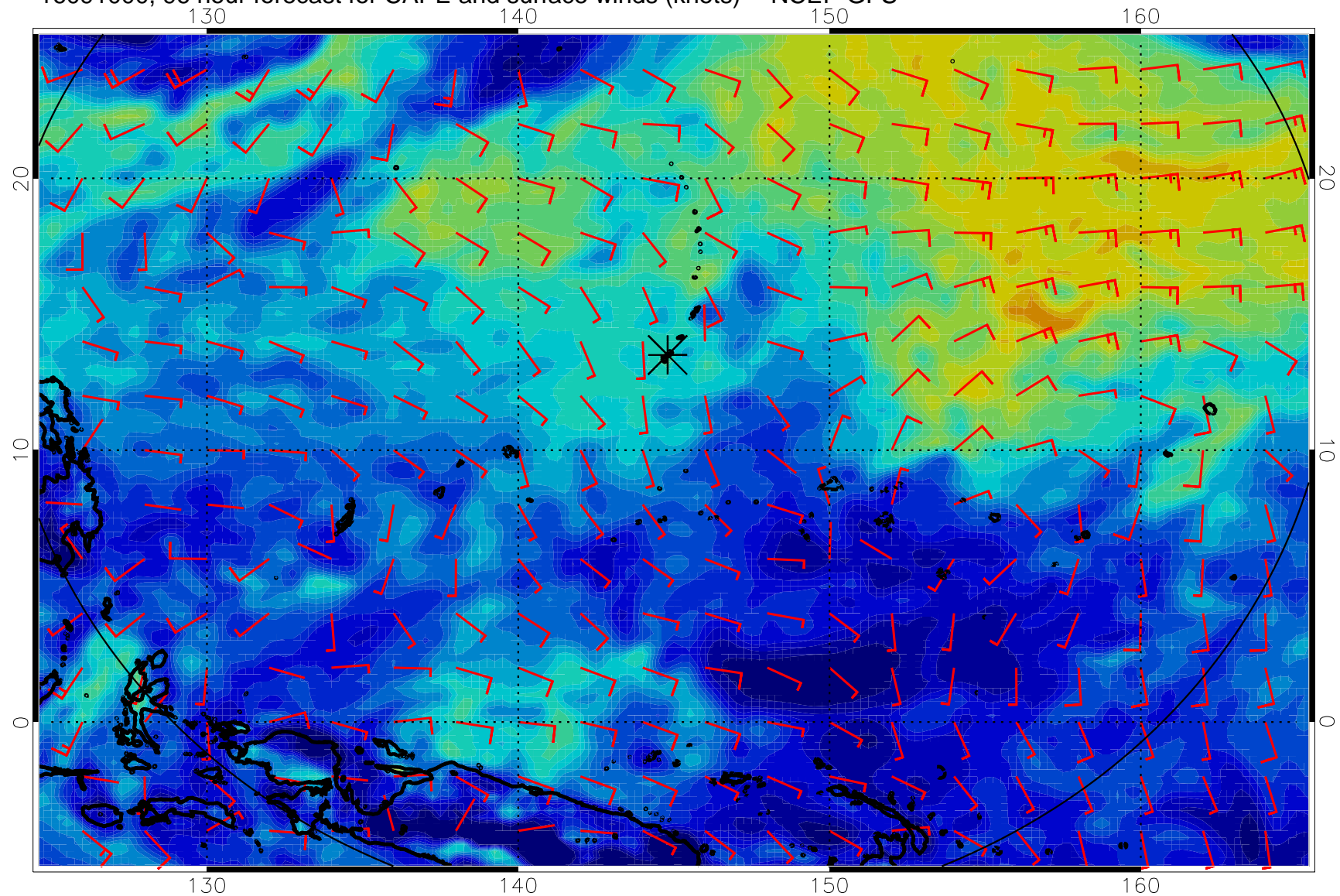
16091000, 96 hour forecast for CAPE and surface winds (knots) -- NCEP GFS
