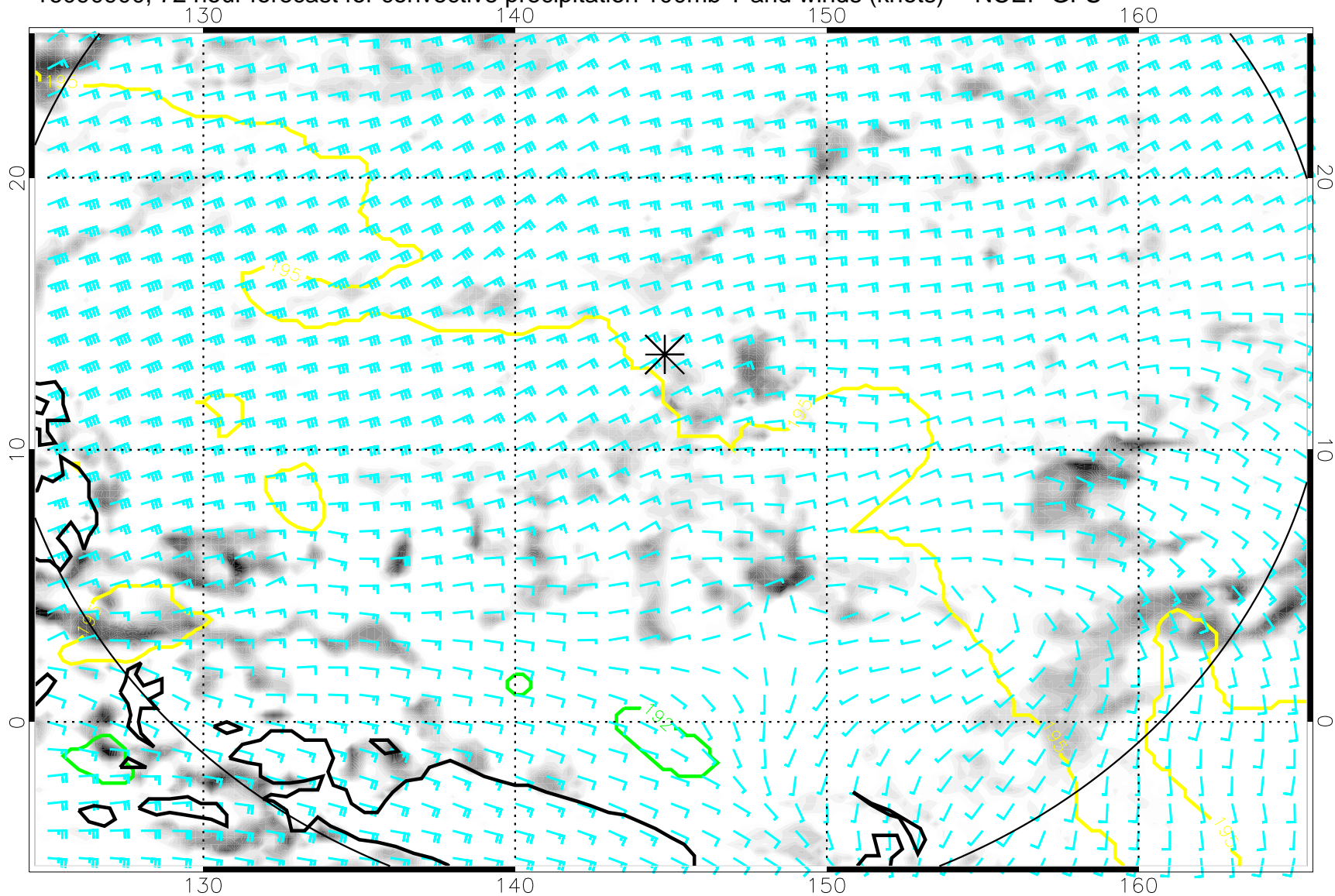
16090900, 72 hour forecast for convective precipitation 100mb T and winds (knots) -- NCEP GFS
