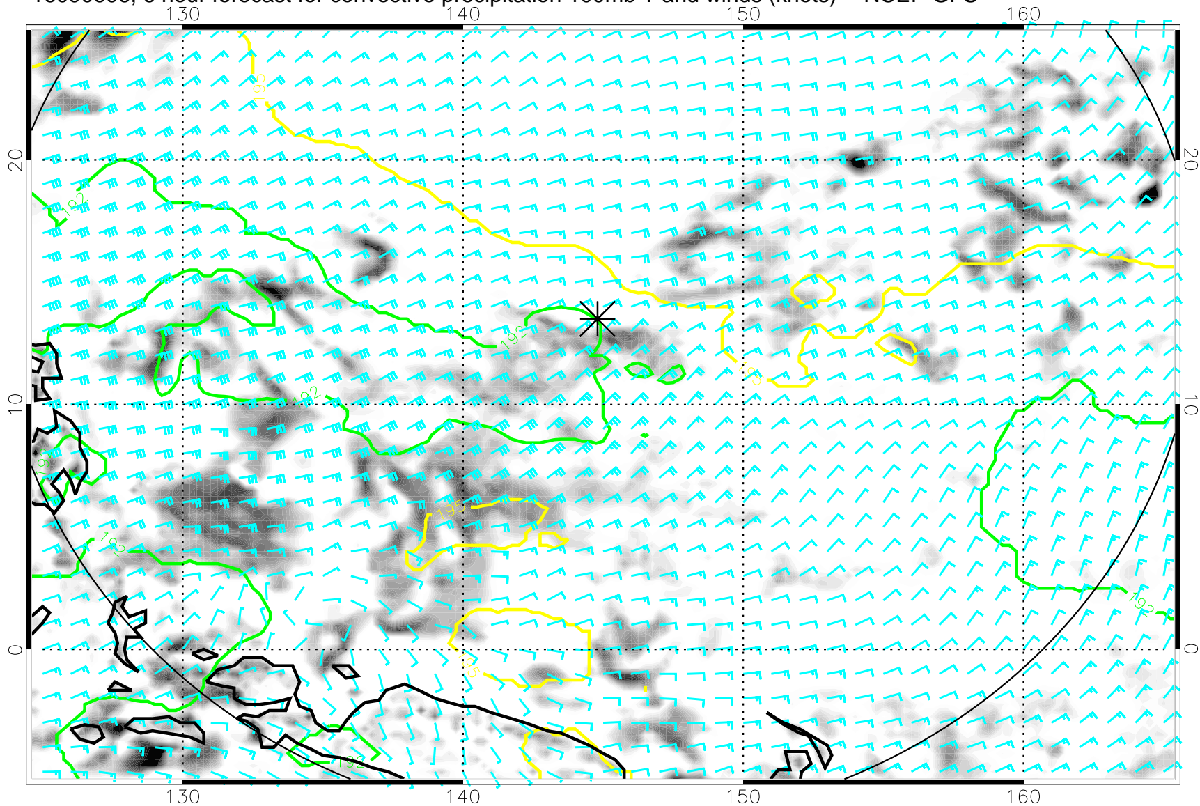
16090606, 6 hour forecast for convective precipitation 100mb T and winds (knots) -- NCEP GFS
