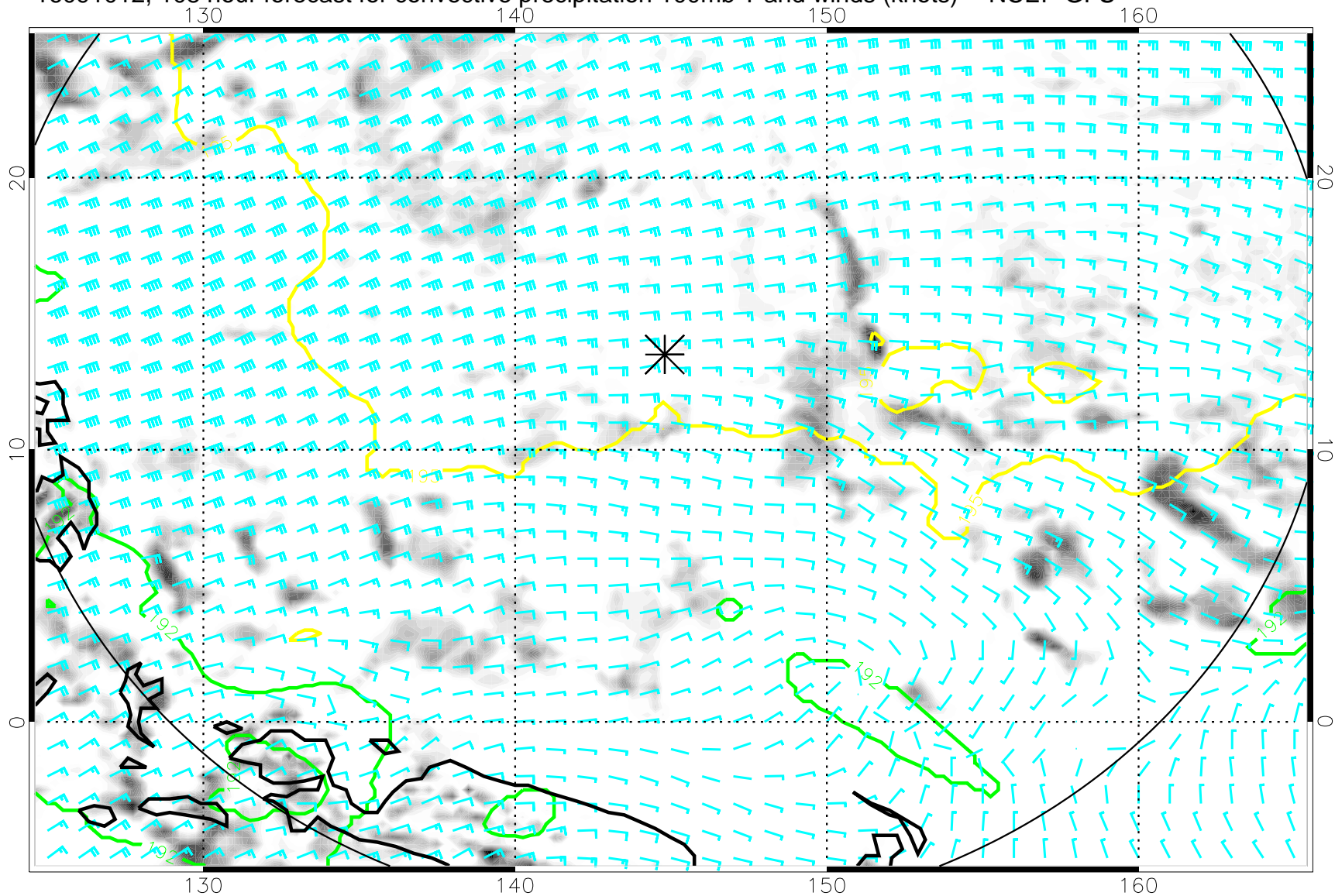
16091012, 108 hour forecast for convective precipitation 100mb T and winds (knots) -- NCEP GFS
