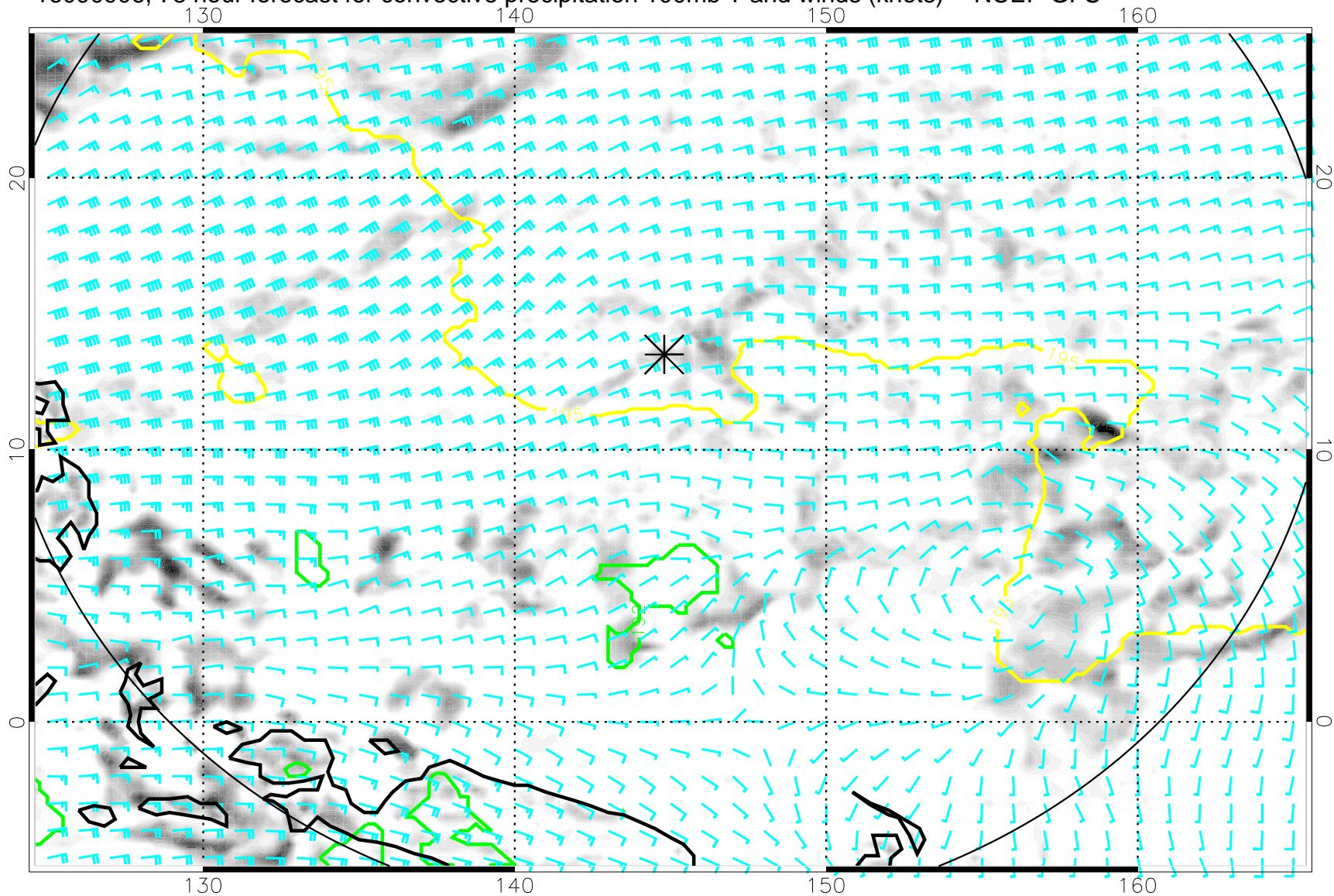
16090906, 78 hour forecast for convective precipitation 100mb T and winds (knots) -- NCEP GFS
