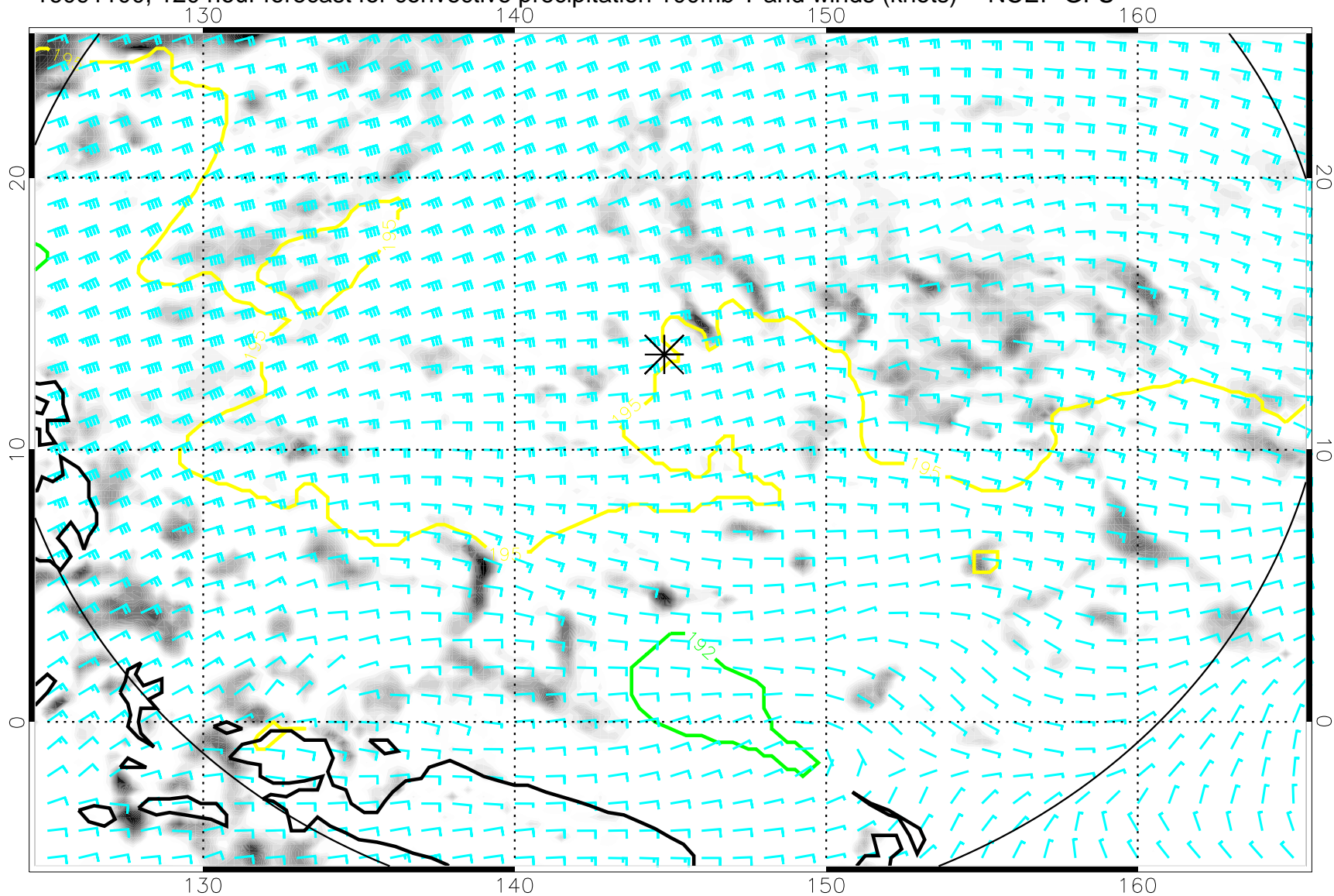
16091100, 120 hour forecast for convective precipitation 100mb T and winds (knots) -- NCEP GFS
