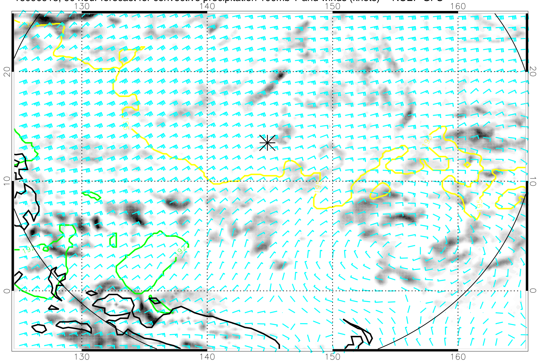
16090918, 90 hour forecast for convective precipitation 100mb T and winds (knots) -- NCEP GFS
