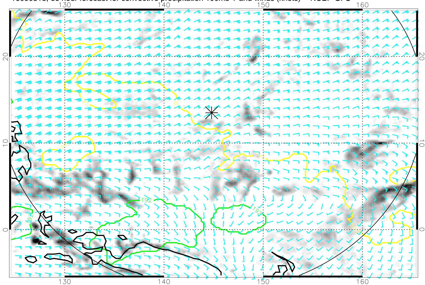
16090818, 66 hour forecast for convective precipitation 100mb T and winds (knots) -- NCEP GFS
