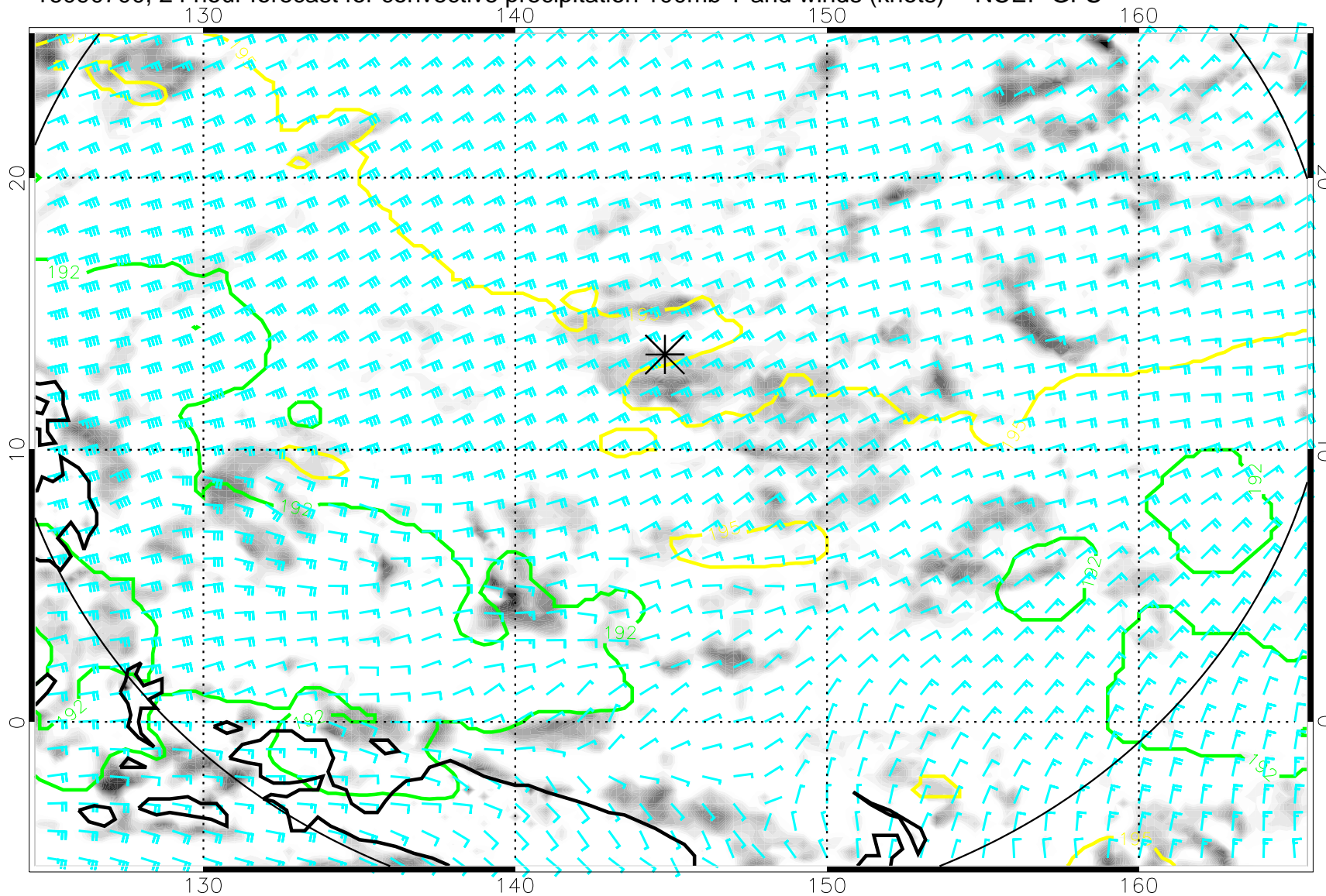
16090700, 24 hour forecast for convective precipitation 100mb T and winds (knots) -- NCEP GFS
