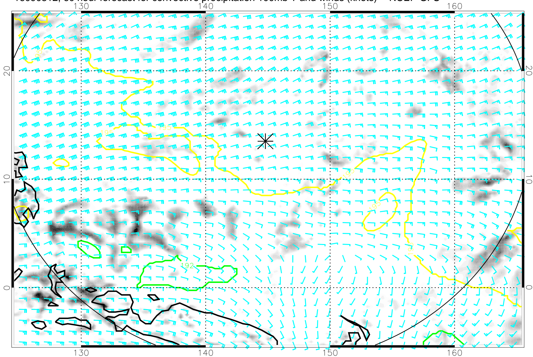
16090812, 60 hour forecast for convective precipitation 100mb T and winds (knots) -- NCEP GFS
