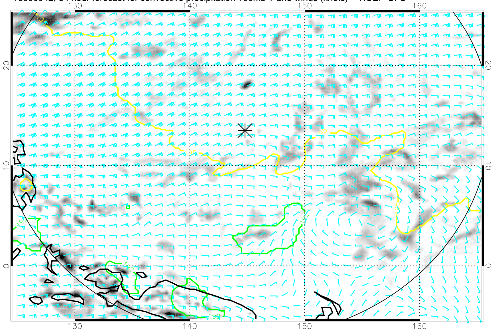
16090912, 84 hour forecast for convective precipitation 100mb T and winds (knots) -- NCEP GFS
