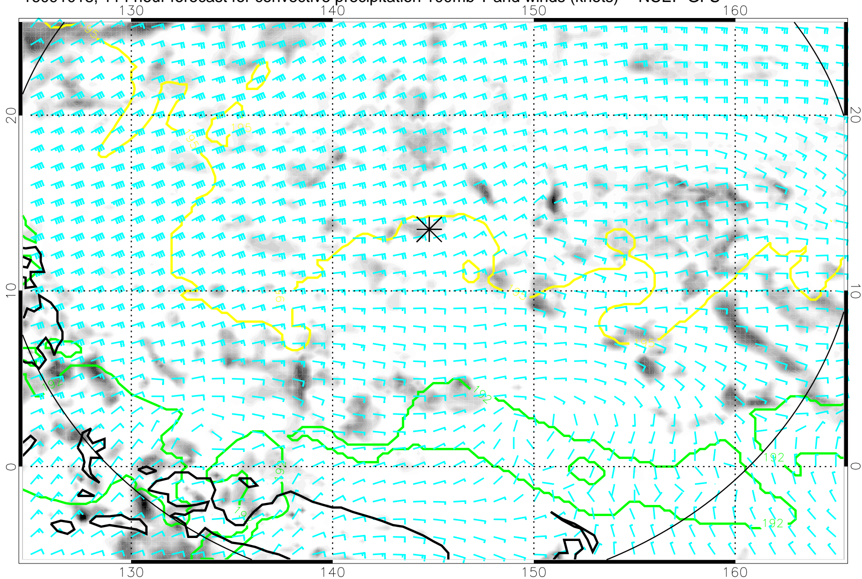
16091018, 114 hour forecast for convective precipitation 100mb T and winds (knots) -- NCEP GFS
