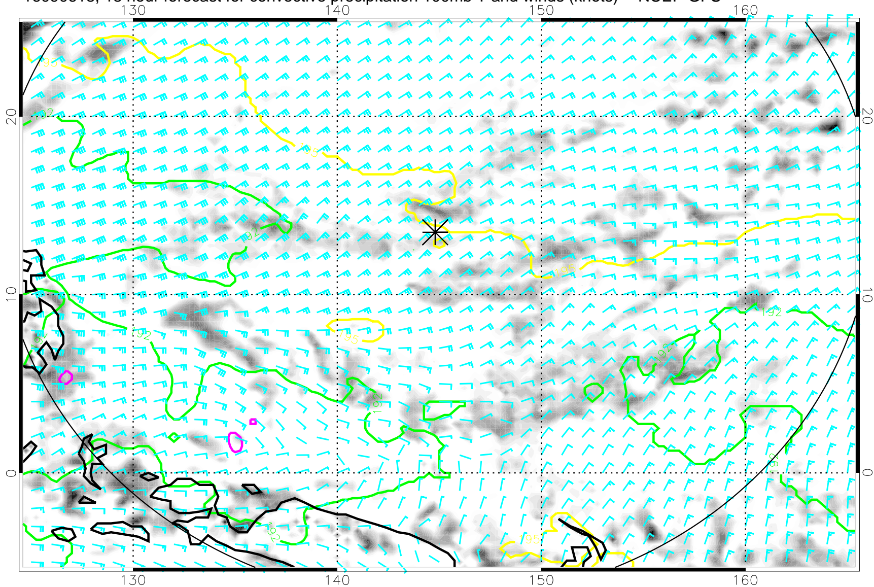
16090618, 18 hour forecast for convective precipitation 100mb T and winds (knots) -- NCEP GFS
