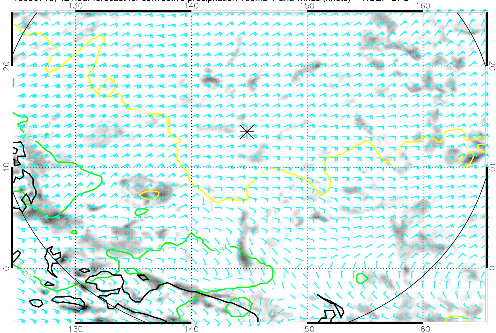
16090718, 42 hour forecast for convective precipitation 100mb T and winds (knots) -- NCEP GFS
