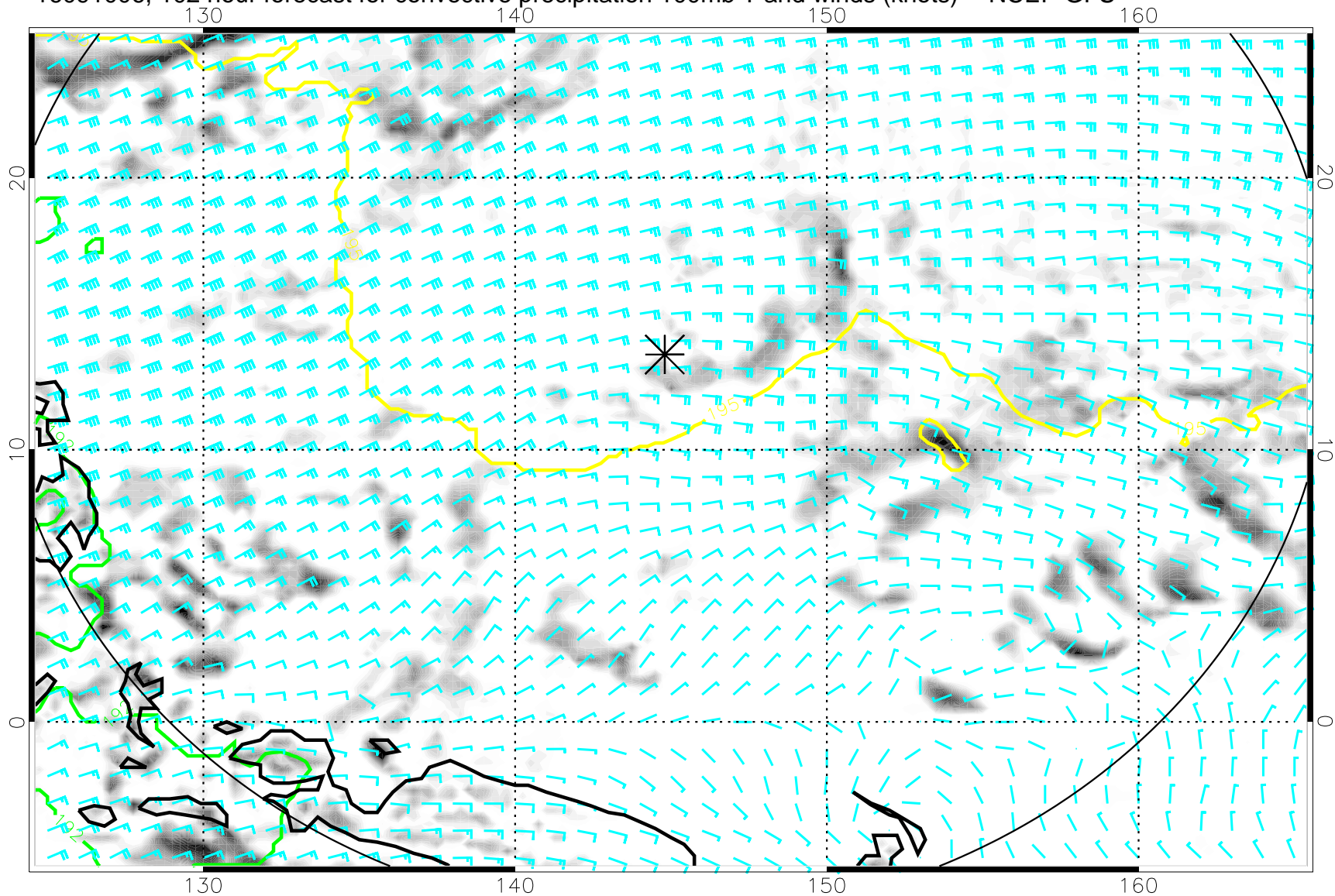
16091006, 102 hour forecast for convective precipitation 100mb T and winds (knots) -- NCEP GFS
