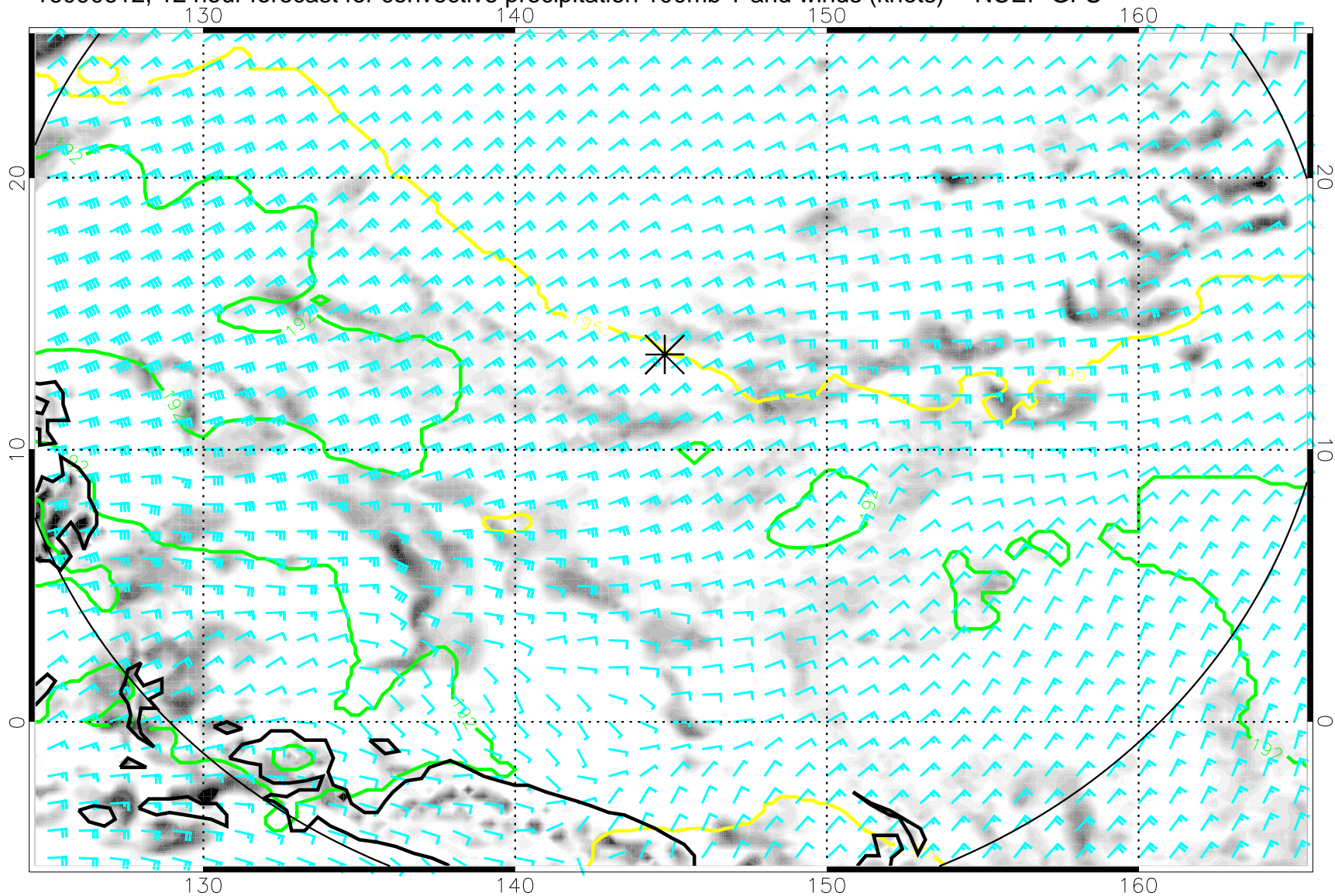
16090612, 12 hour forecast for convective precipitation 100mb T and winds (knots) -- NCEP GFS
