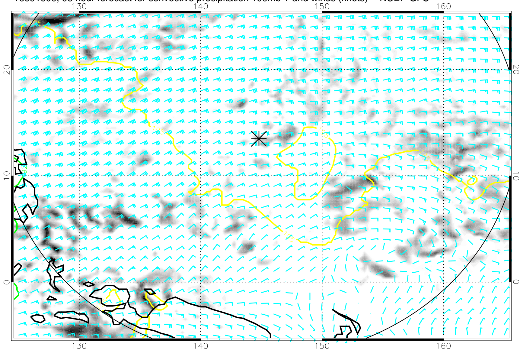
16091000, 96 hour forecast for convective precipitation 100mb T and winds (knots) -- NCEP GFS
