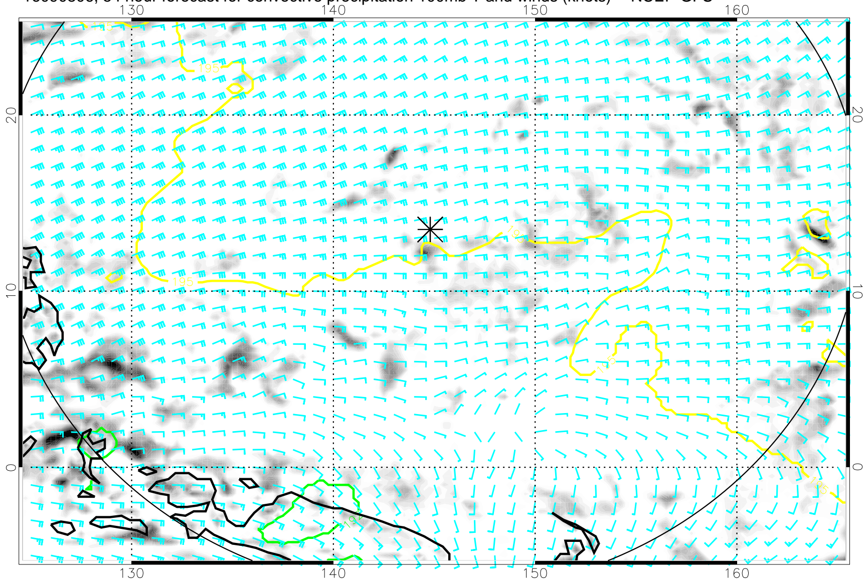
16090806, 54 hour forecast for convective precipitation 100mb T and winds (knots) -- NCEP GFS
