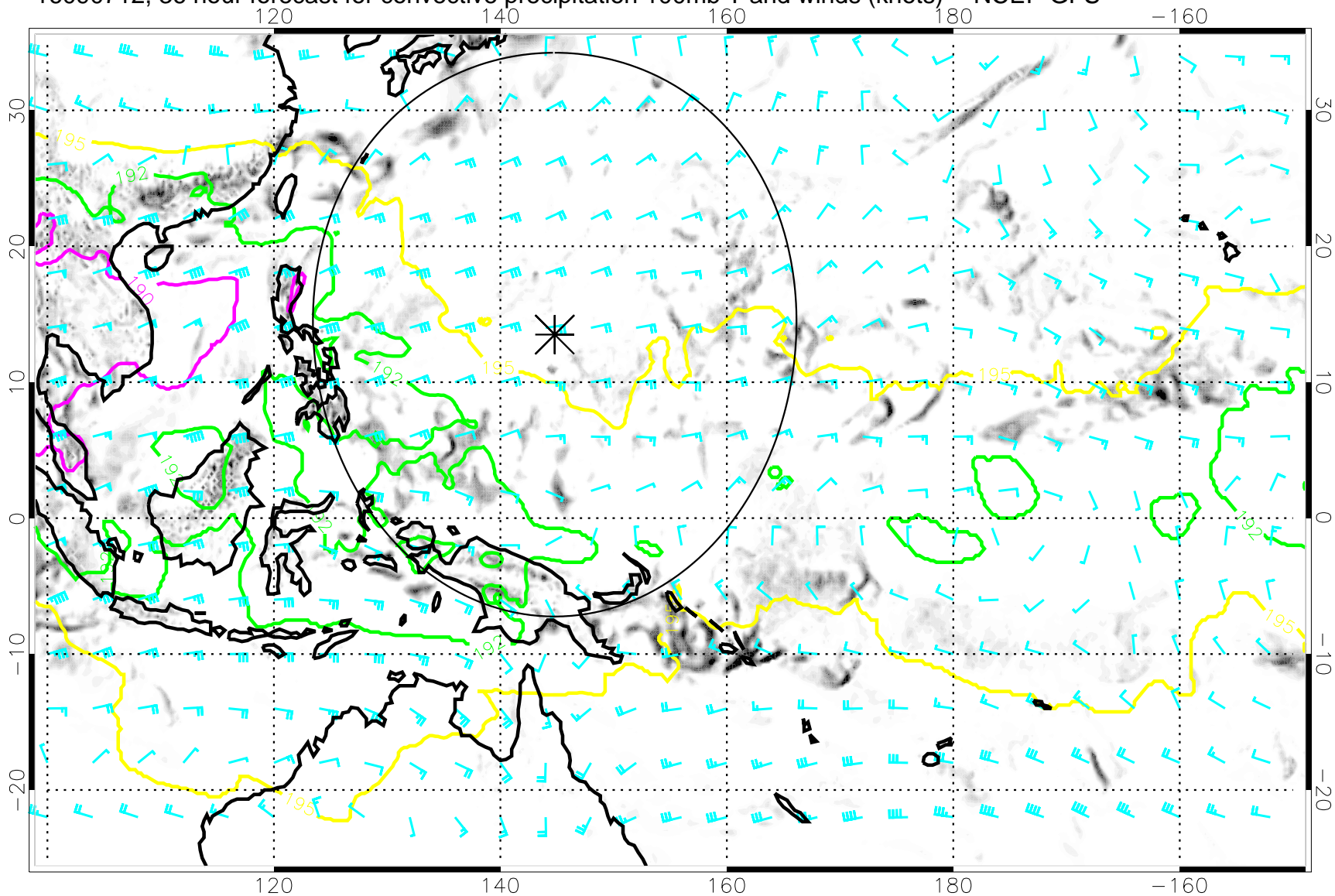
16090712, 36 hour forecast for convective precipitation 100mb T and winds (knots) -- NCEP GFS
