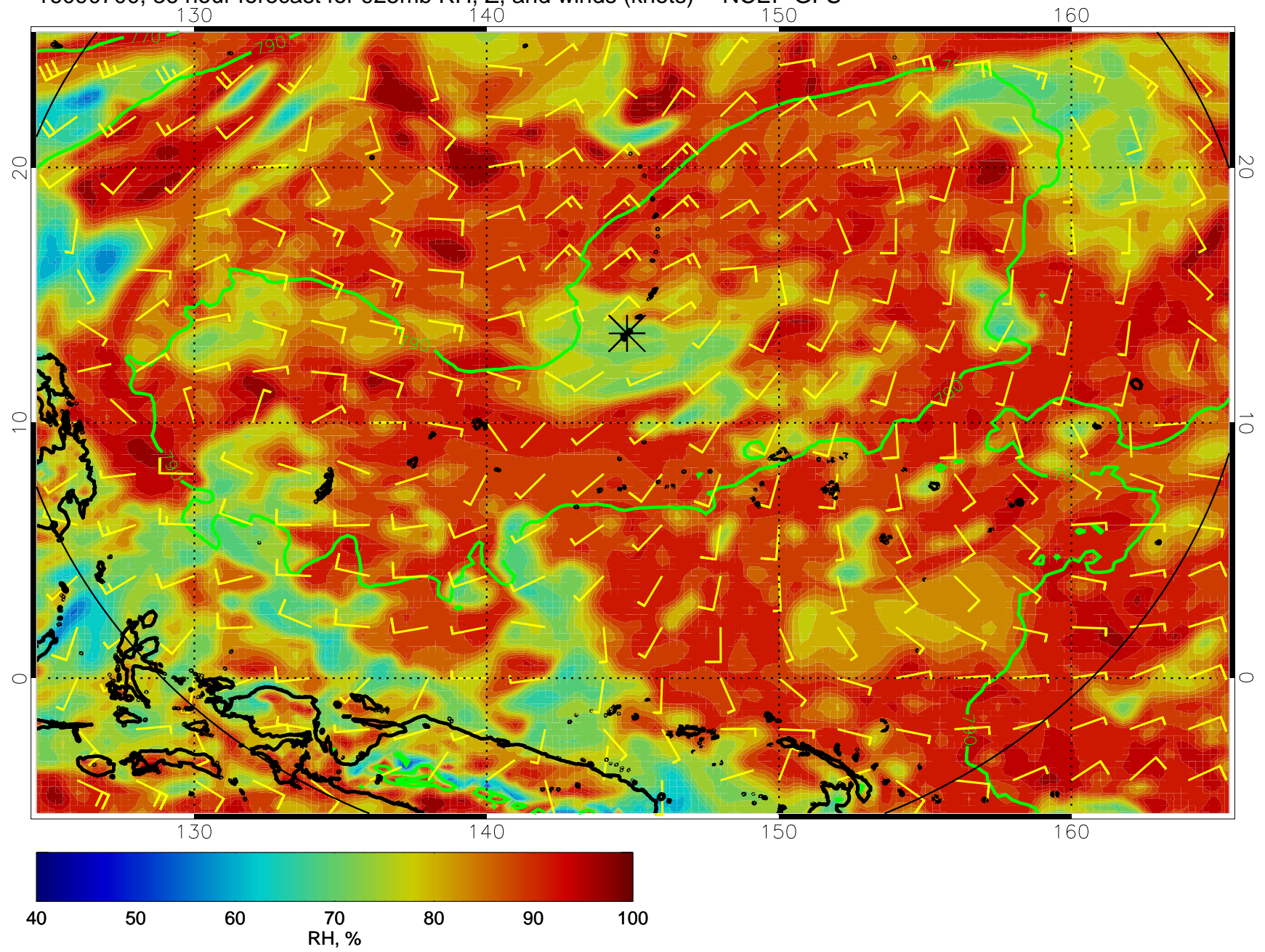
16090700, 36 hour forecast for 925mb RH, Z, and winds (knots) -- NCEP GFS
