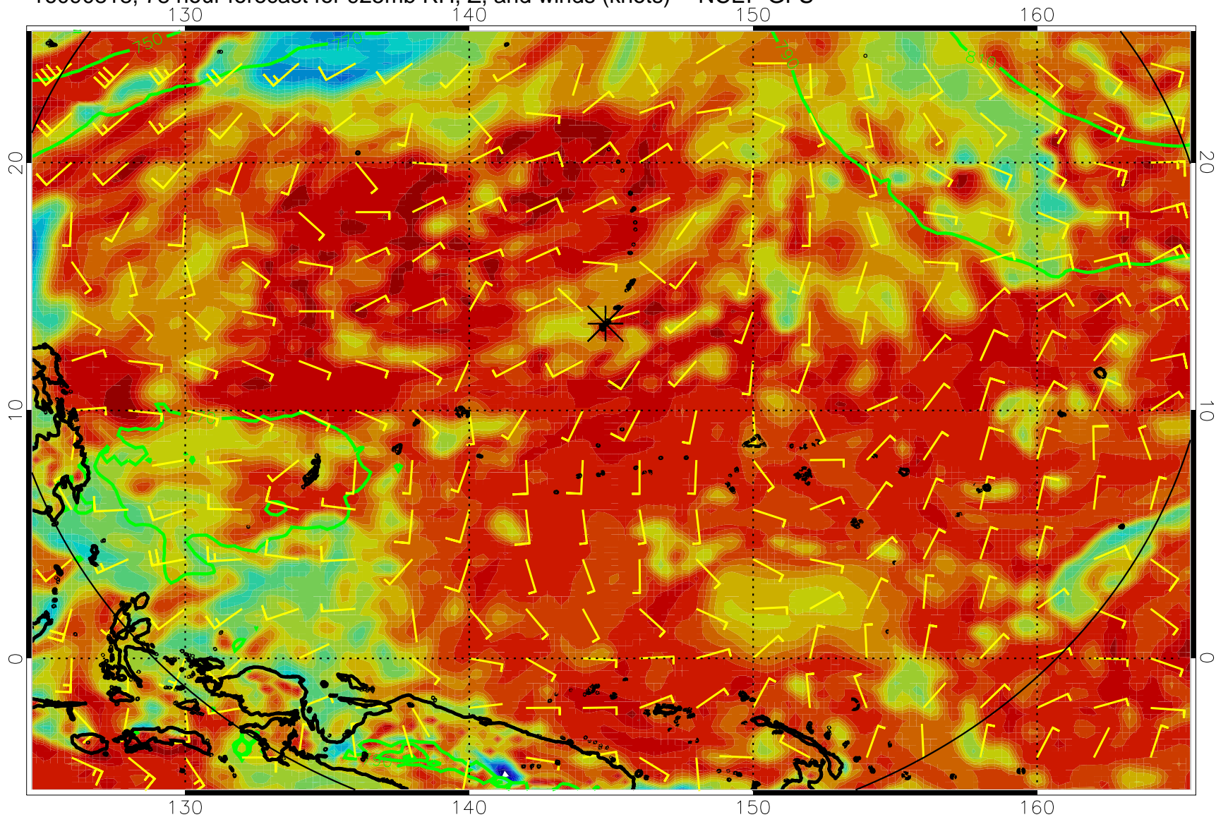
16090818, 78 hour forecast for 925mb RH, Z, and winds (knots) -- NCEP GFS
