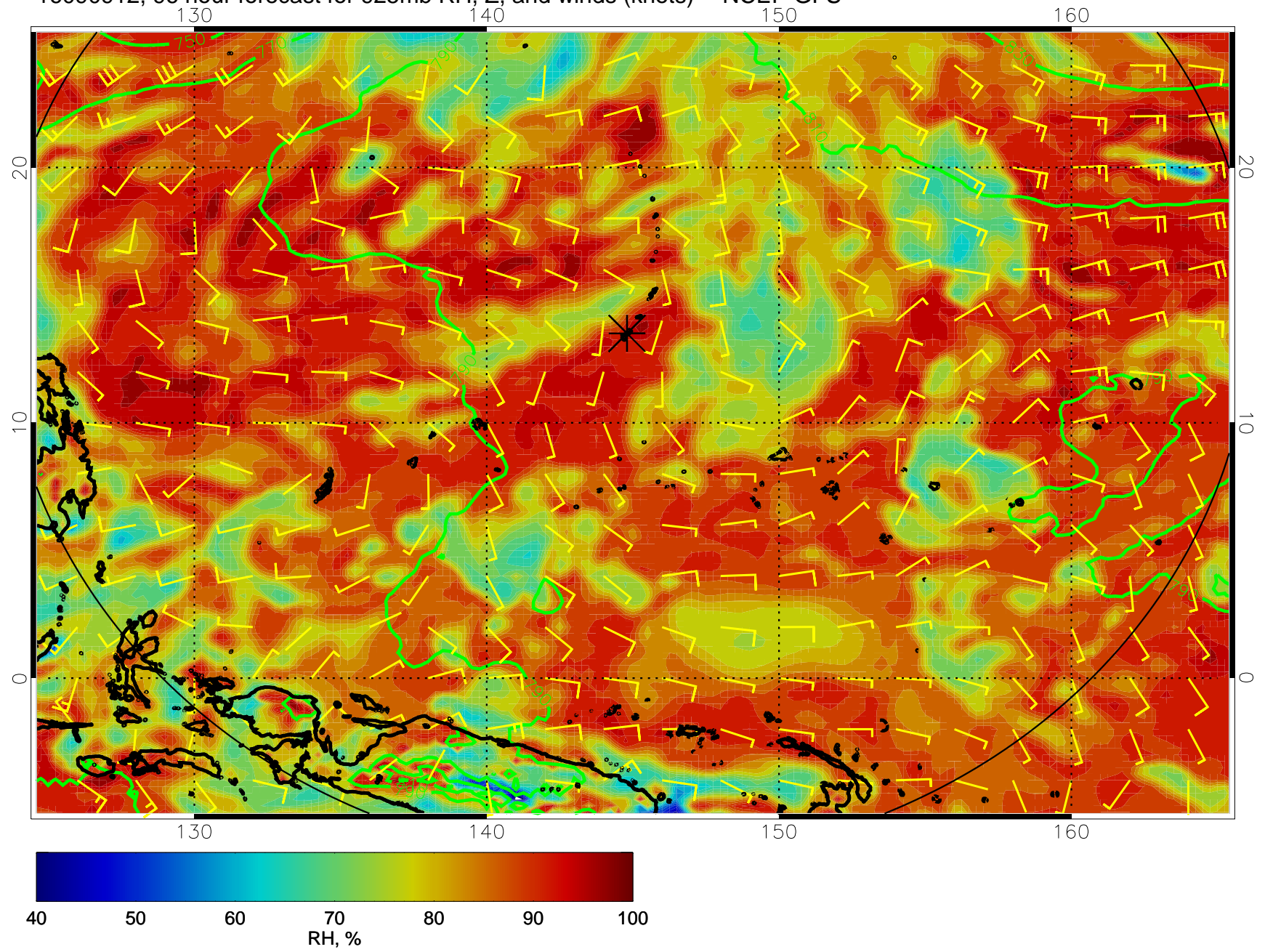
16090912, 96 hour forecast for 925mb RH, Z, and winds (knots) -- NCEP GFS
