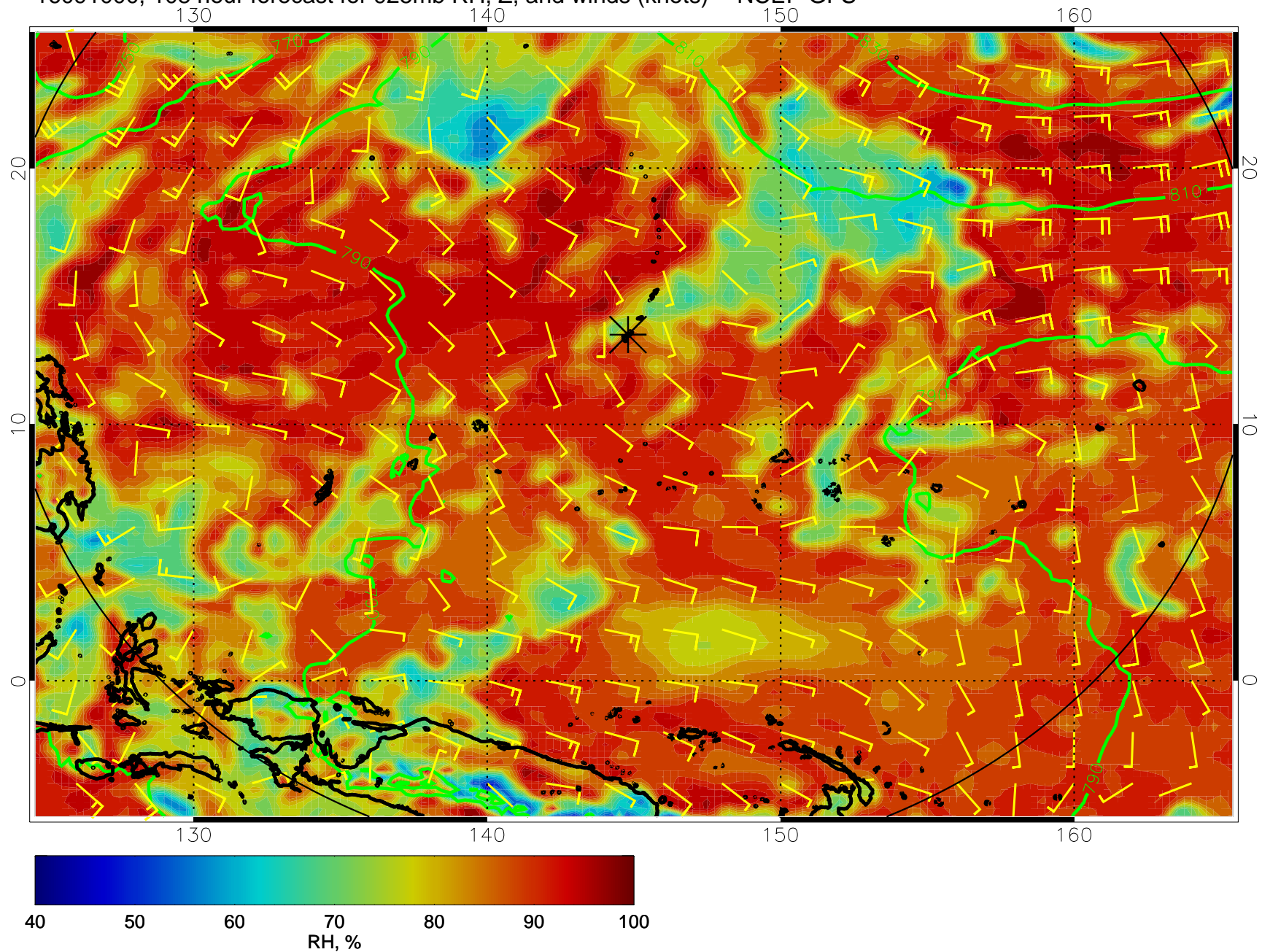
16091000, 108 hour forecast for 925mb RH, Z, and winds (knots) -- NCEP GFS
