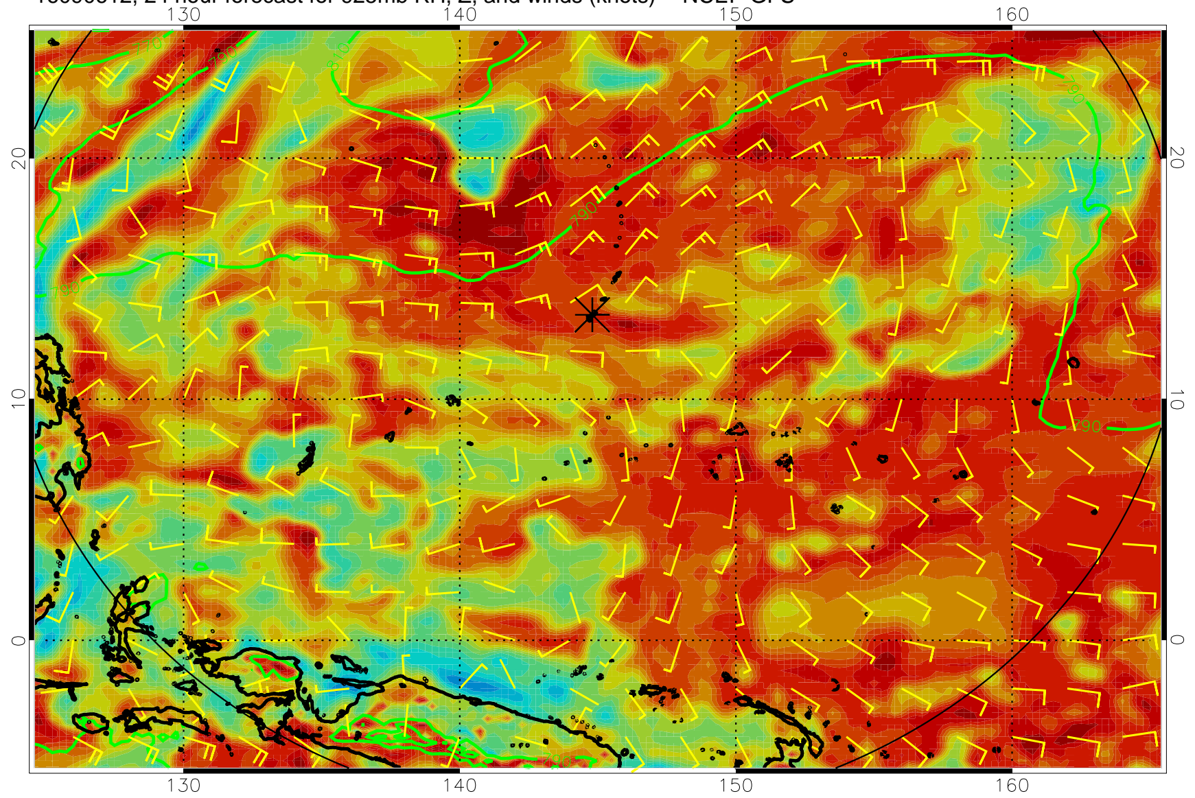
16090612, 24 hour forecast for 925mb RH, Z, and winds (knots) -- NCEP GFS
