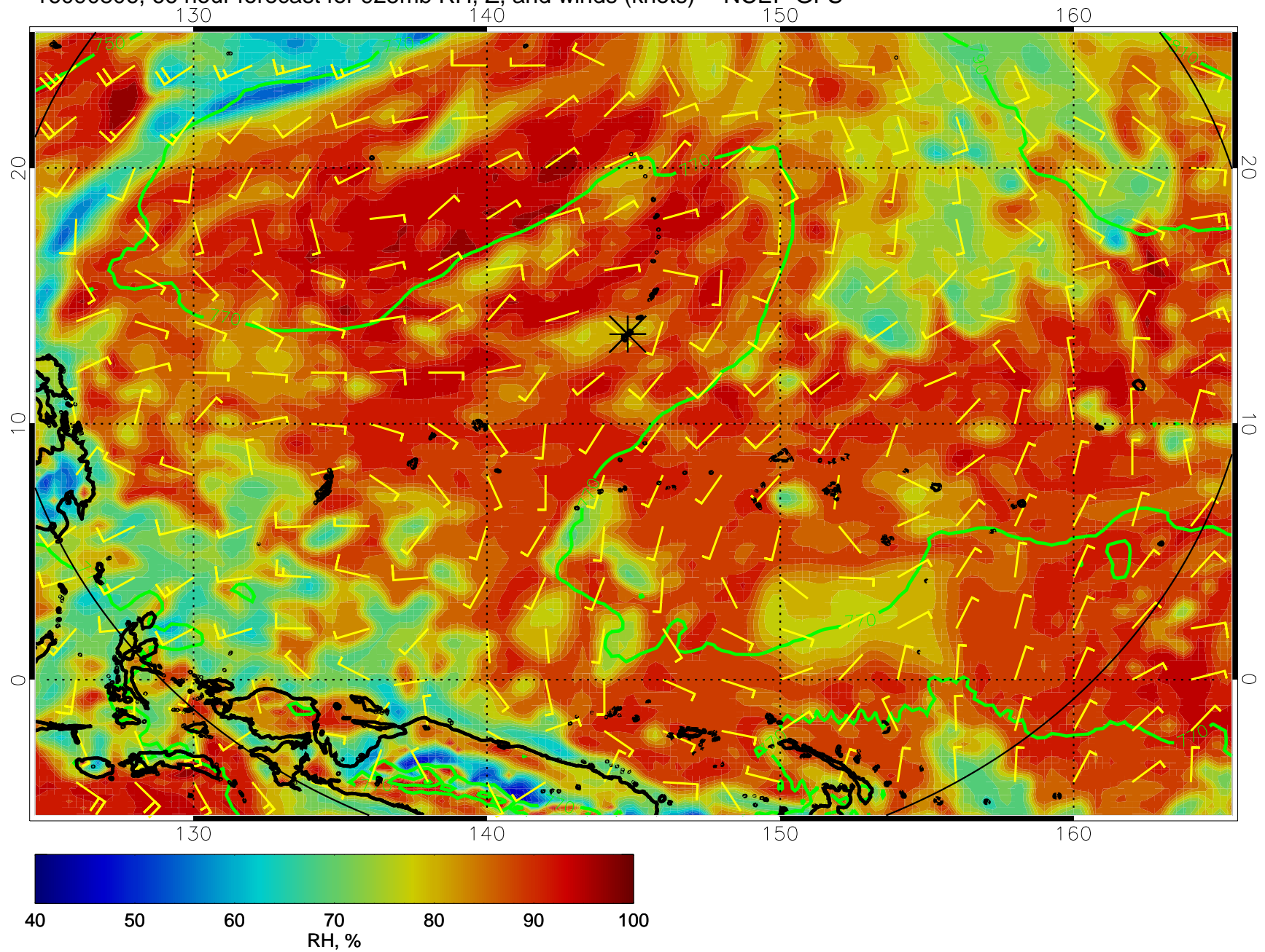
16090806, 66 hour forecast for 925mb RH, Z, and winds (knots) -- NCEP GFS
