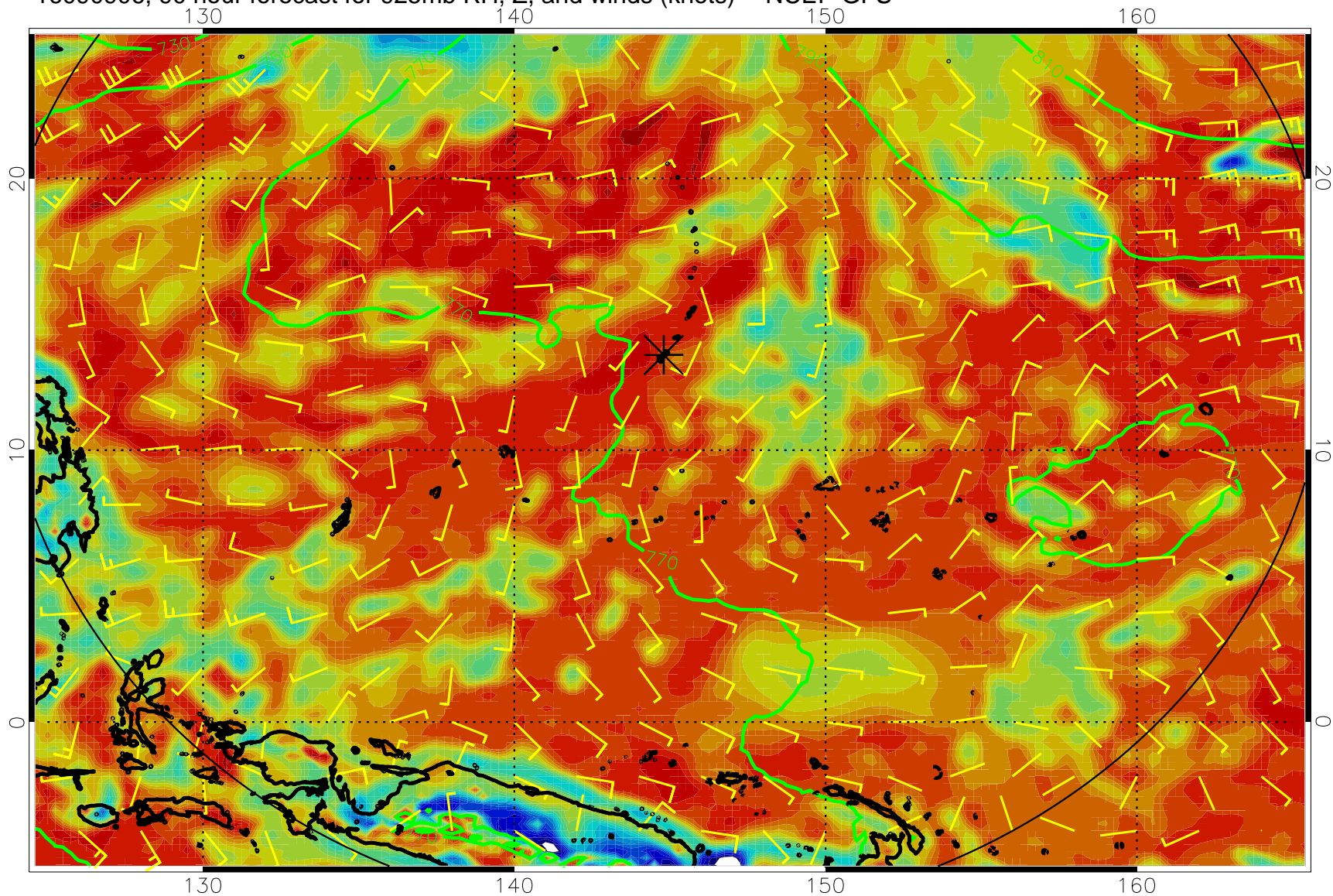
16090906, 90 hour forecast for 925mb RH, Z, and winds (knots) -- NCEP GFS
