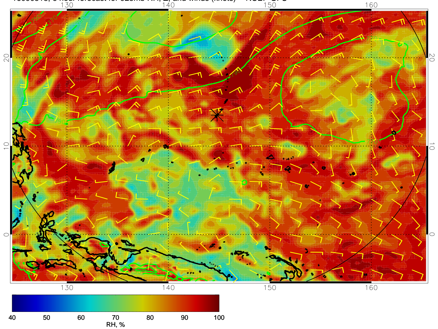
16090518, 6 hour forecast for 925mb RH, Z, and winds (knots) -- NCEP GFS
