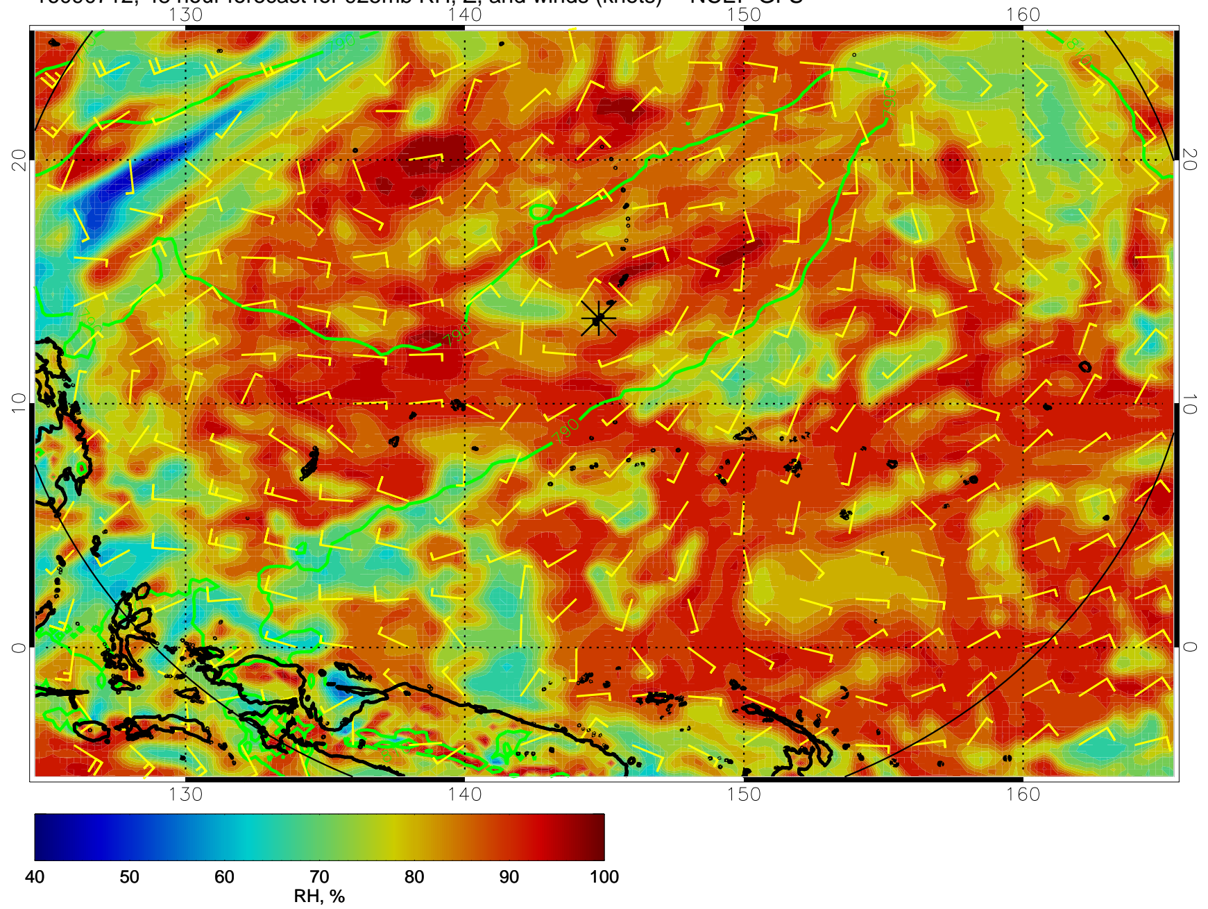
16090712, 48 hour forecast for 925mb RH, Z, and winds (knots) -- NCEP GFS
