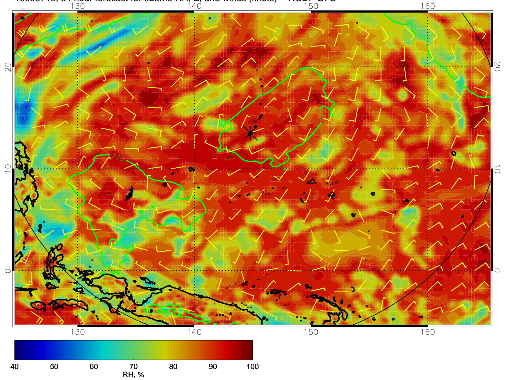
16090718, 54 hour forecast for 925mb RH, Z, and winds (knots) -- NCEP GFS
