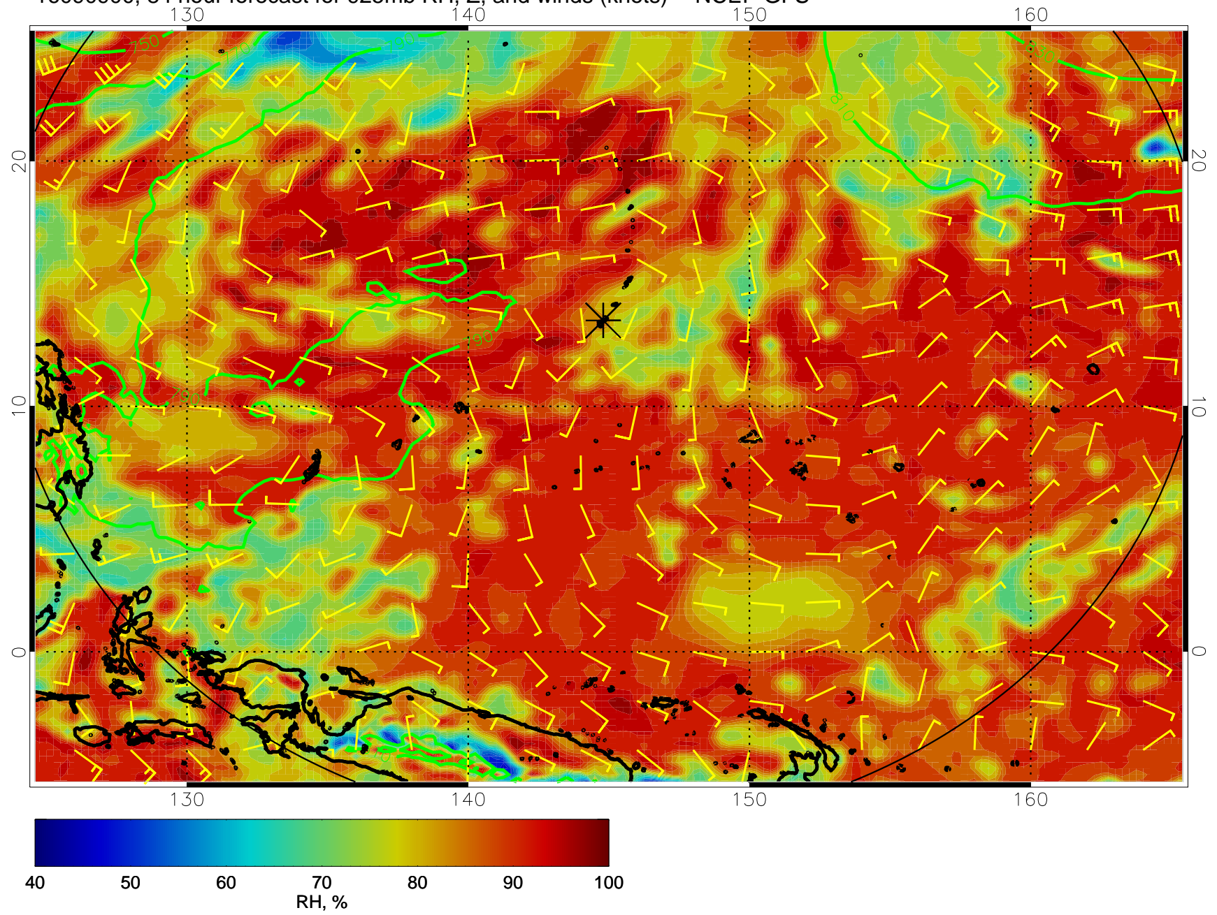
16090900, 84 hour forecast for 925mb RH, Z, and winds (knots) -- NCEP GFS
