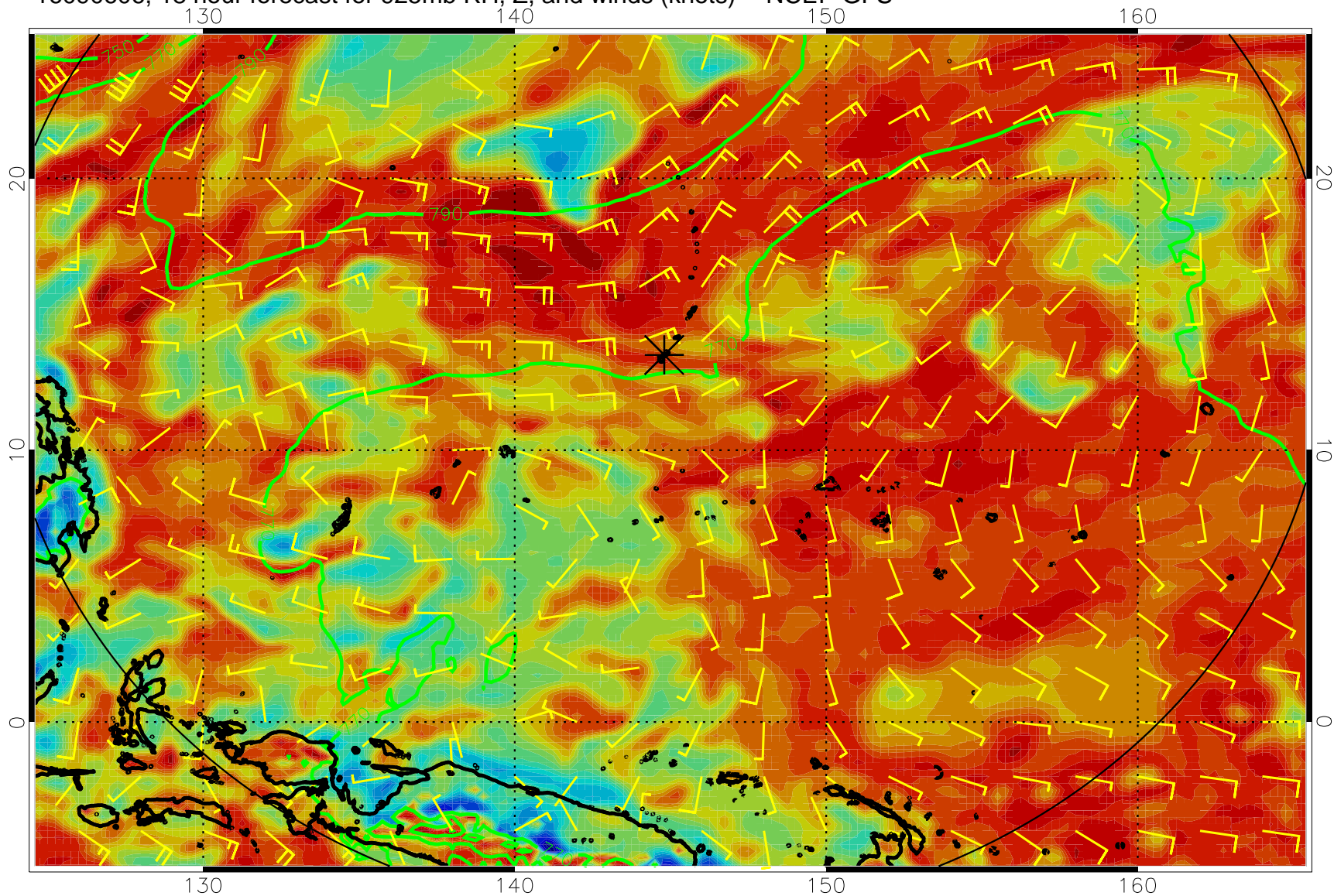
16090606, 18 hour forecast for 925mb RH, Z, and winds (knots) -- NCEP GFS
