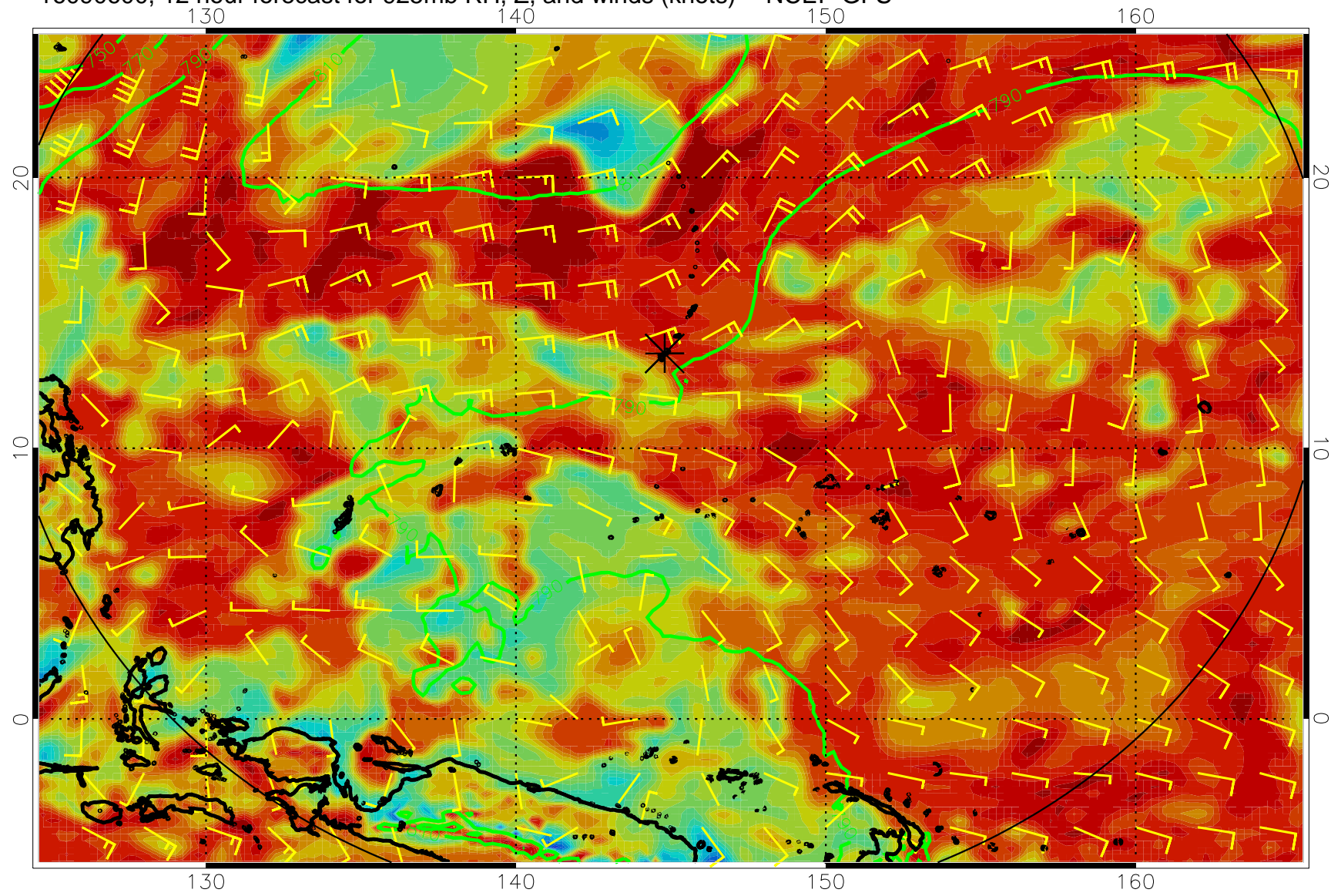
16090600, 12 hour forecast for 925mb RH, Z, and winds (knots) -- NCEP GFS
