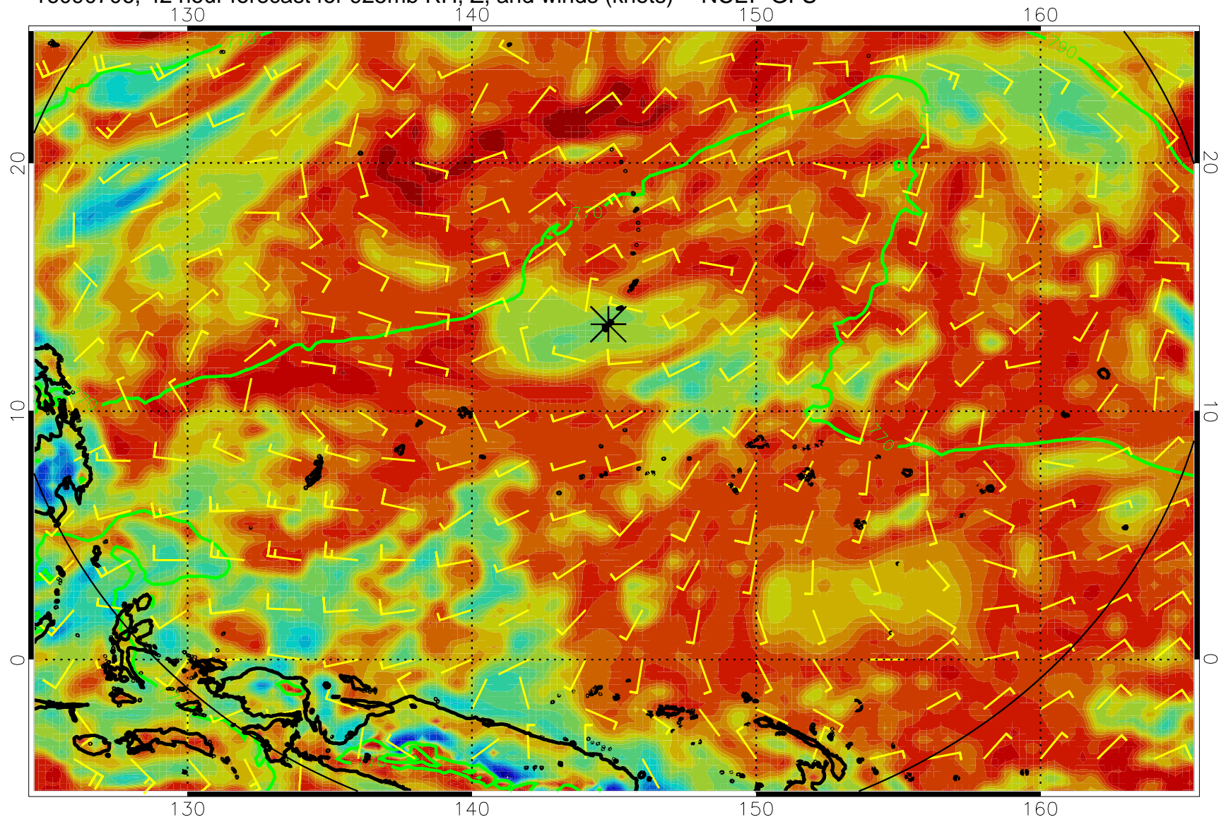
16090706, 42 hour forecast for 925mb RH, Z, and winds (knots) -- NCEP GFS
