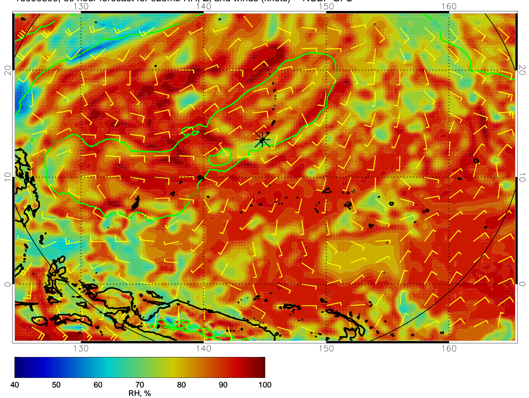
16090800, 60 hour forecast for 925mb RH, Z, and winds (knots) -- NCEP GFS
