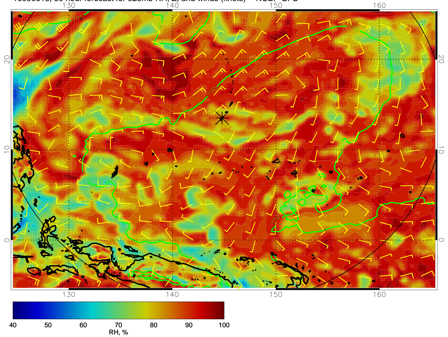
16090618, 30 hour forecast for 925mb RH, Z, and winds (knots) -- NCEP GFS
