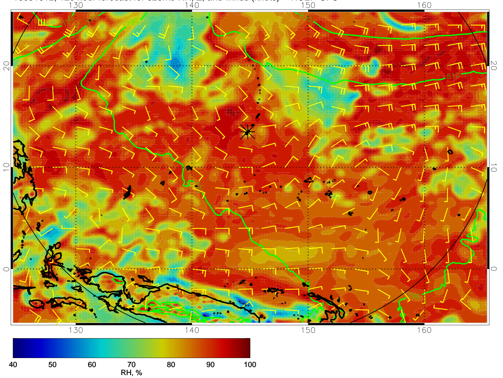
16091012, 120 hour forecast for 925mb RH, Z, and winds (knots) -- NCEP GFS
