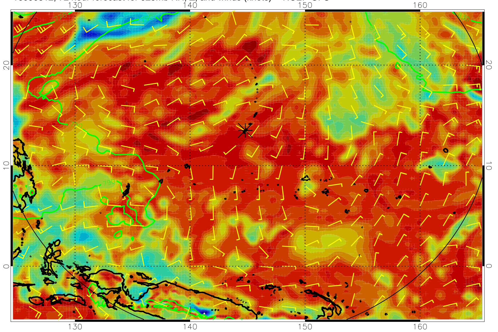
16090812, 72 hour forecast for 925mb RH, Z, and winds (knots) -- NCEP GFS
