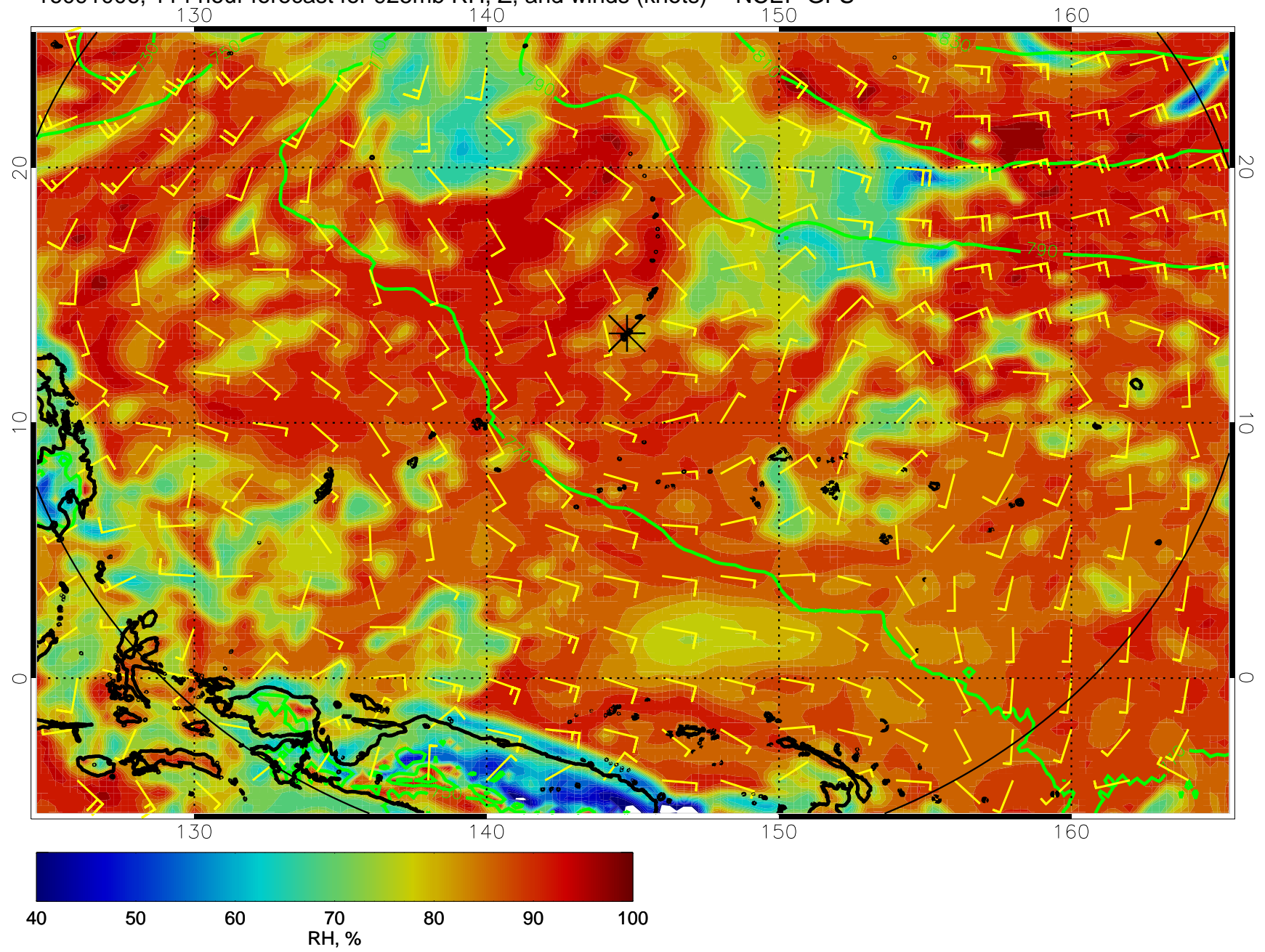
16091006, 114 hour forecast for 925mb RH, Z, and winds (knots) -- NCEP GFS
