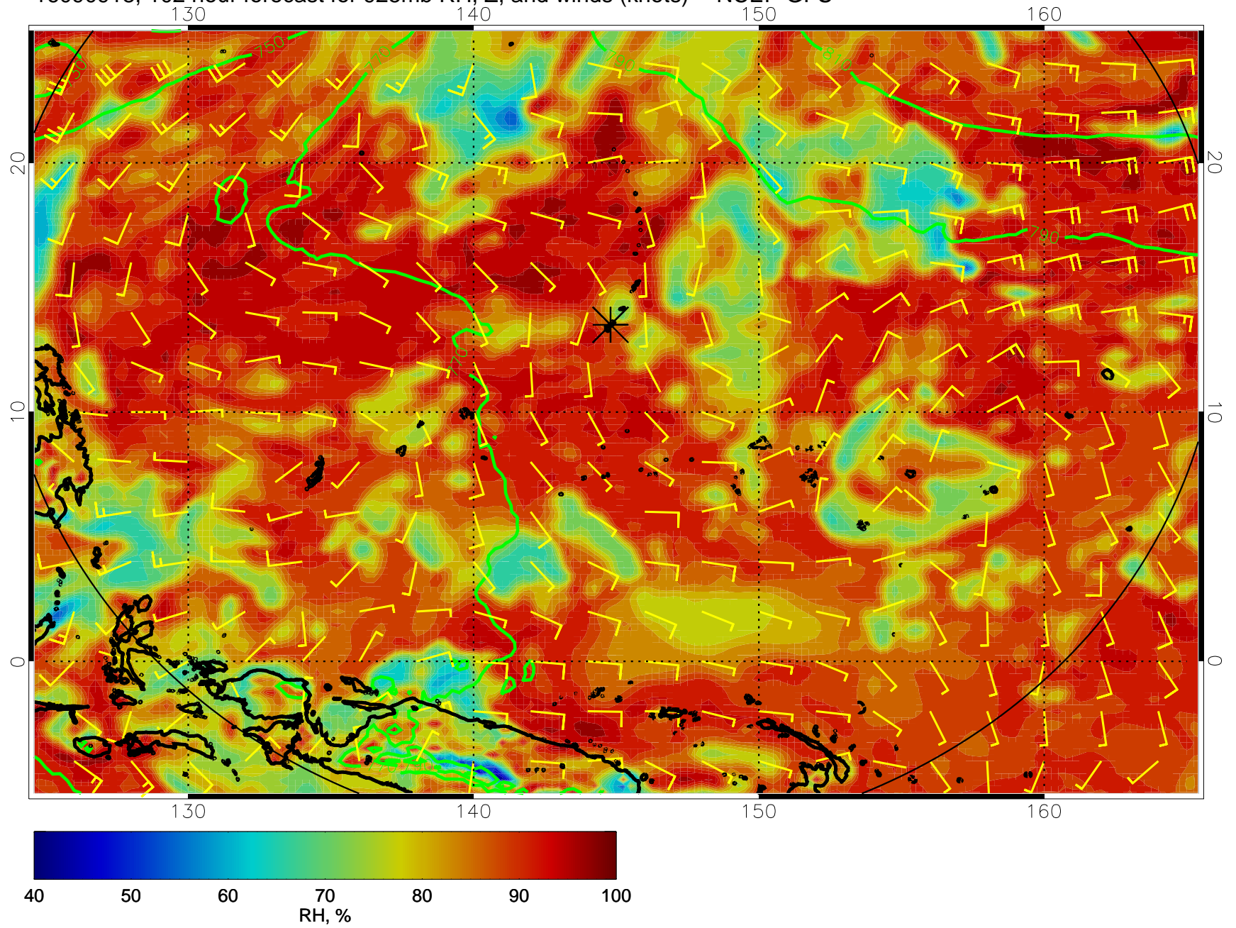
16090918, 102 hour forecast for 925mb RH, Z, and winds (knots) -- NCEP GFS
