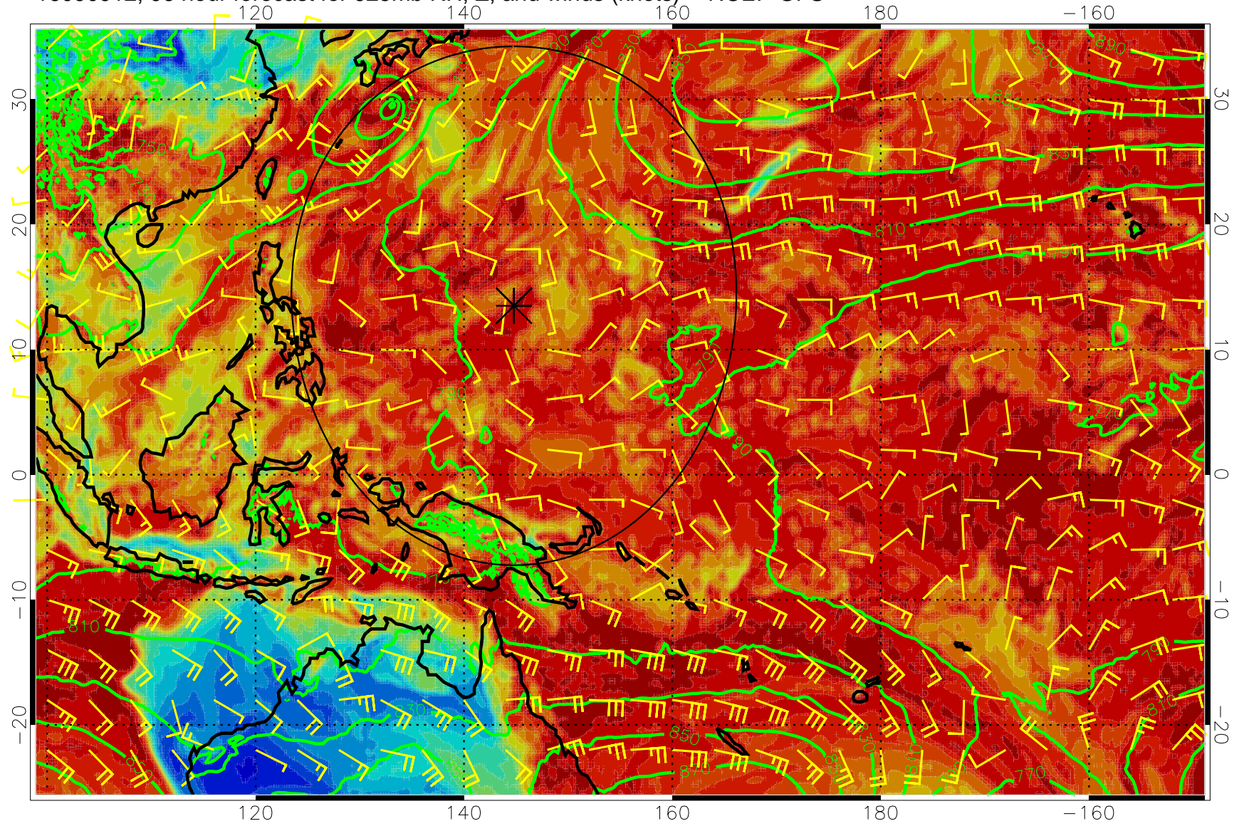
16090912, 96 hour forecast for 925mb RH, Z, and winds (knots) -- NCEP GFS
