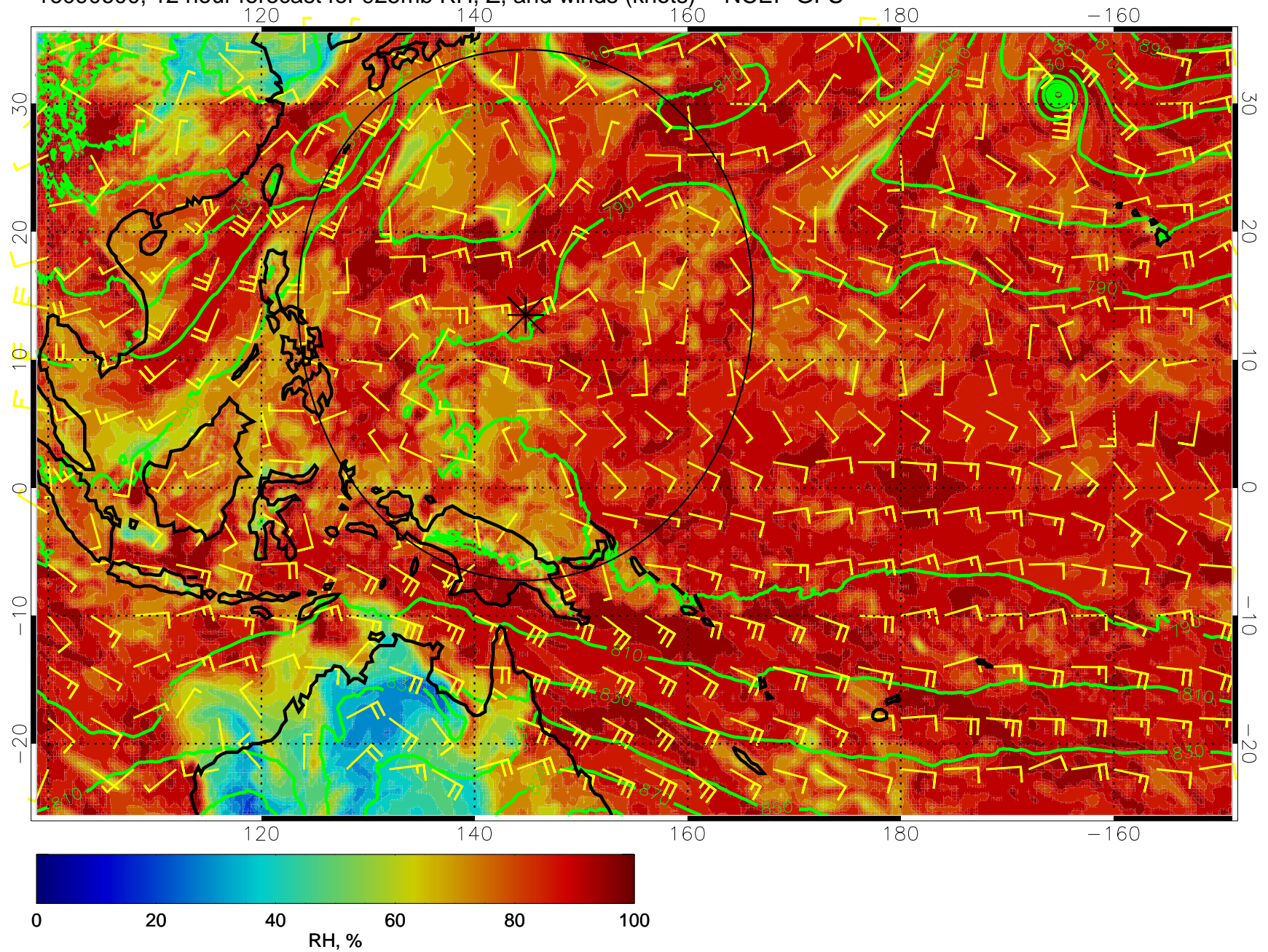
16090600, 12 hour forecast for 925mb RH, Z, and winds (knots) -- NCEP GFS
