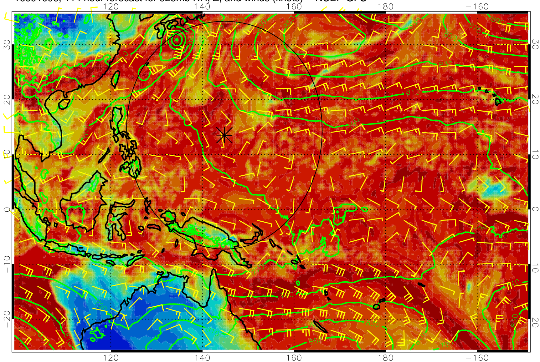
16091006, 114 hour forecast for 925mb RH, Z, and winds (knots) -- NCEP GFS
