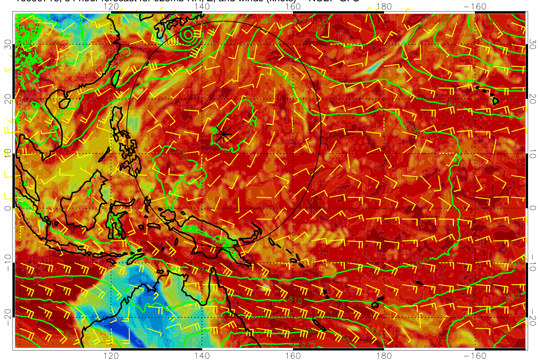
16090718, 54 hour forecast for 925mb RH, Z, and winds (knots) -- NCEP GFS
