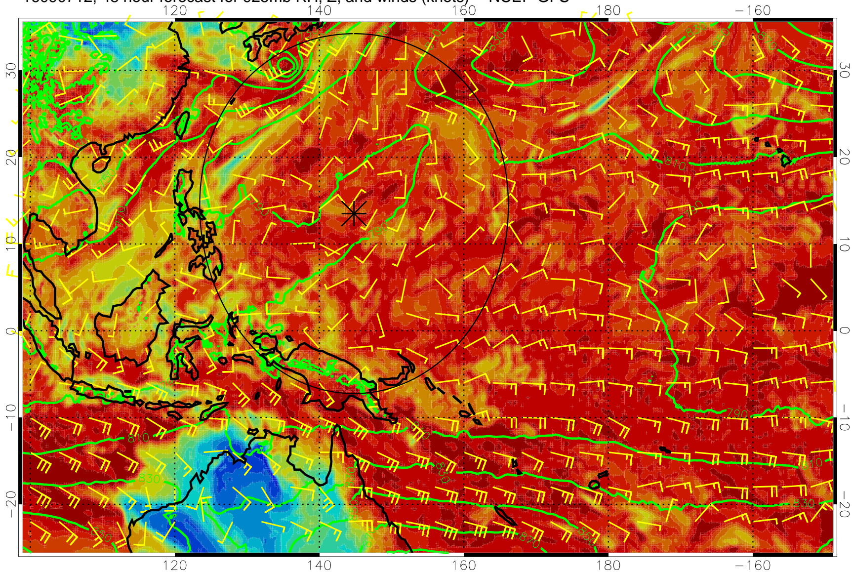
16090712, 48 hour forecast for 925mb RH, Z, and winds (knots) -- NCEP GFS
