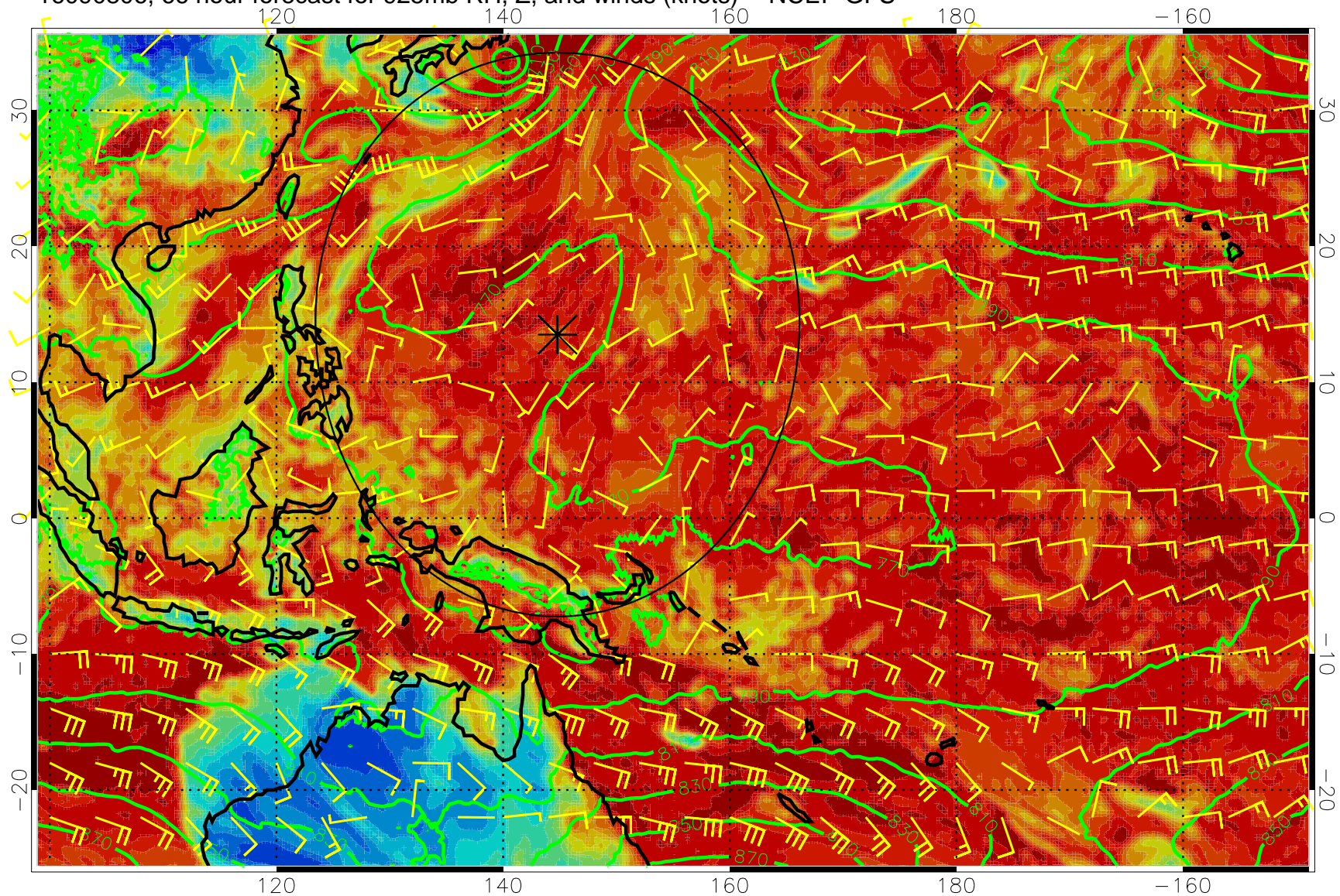
16090806, 66 hour forecast for 925mb RH, Z, and winds (knots) -- NCEP GFS
