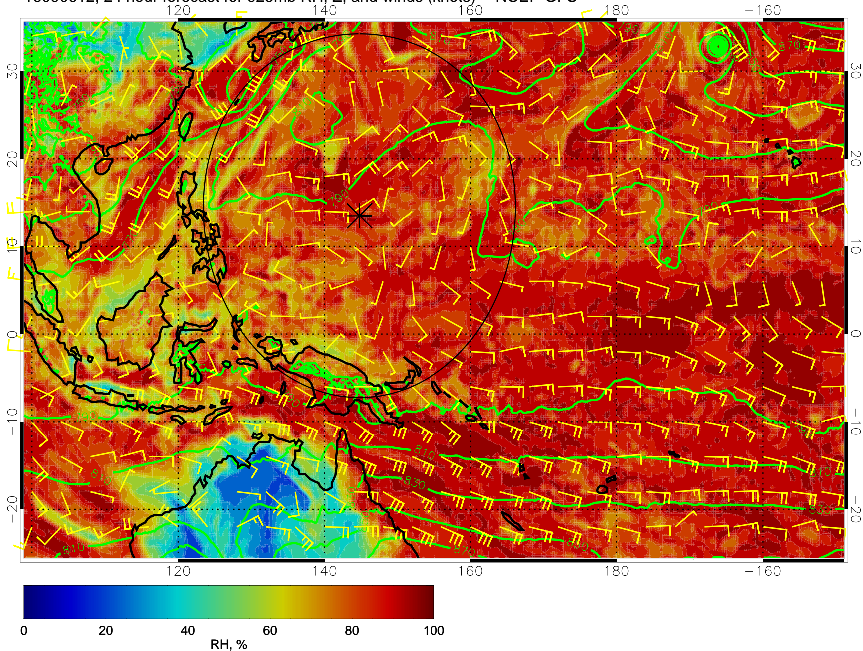
16090612, 24 hour forecast for 925mb RH, Z, and winds (knots) -- NCEP GFS
