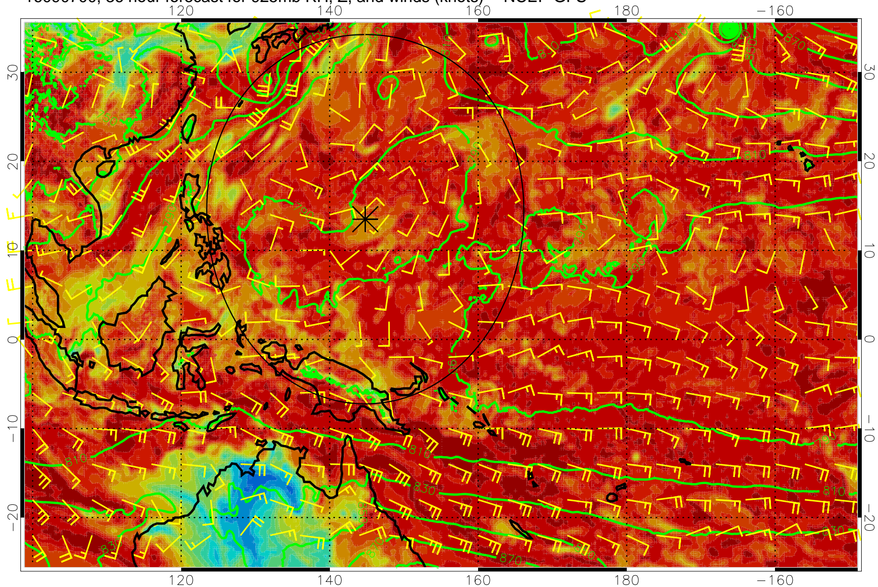
16090700, 36 hour forecast for 925mb RH, Z, and winds (knots) -- NCEP GFS
