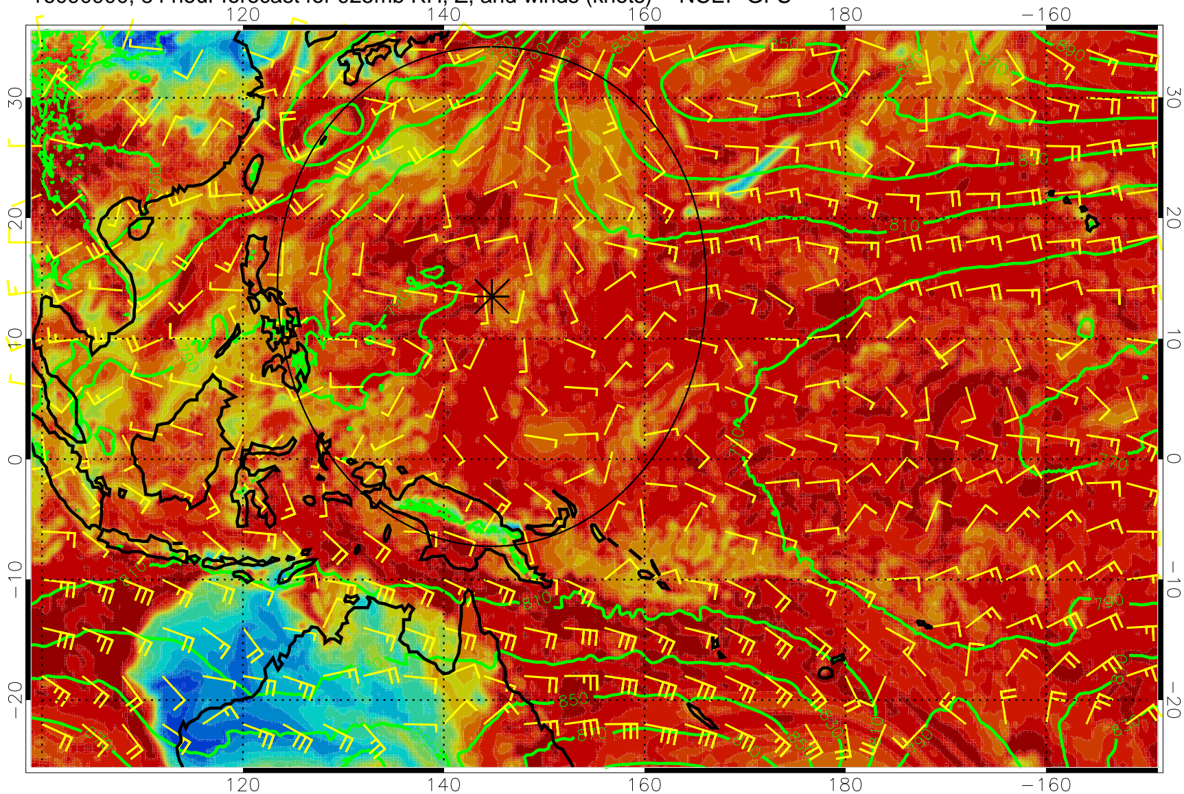
16090900, 84 hour forecast for 925mb RH, Z, and winds (knots) -- NCEP GFS
