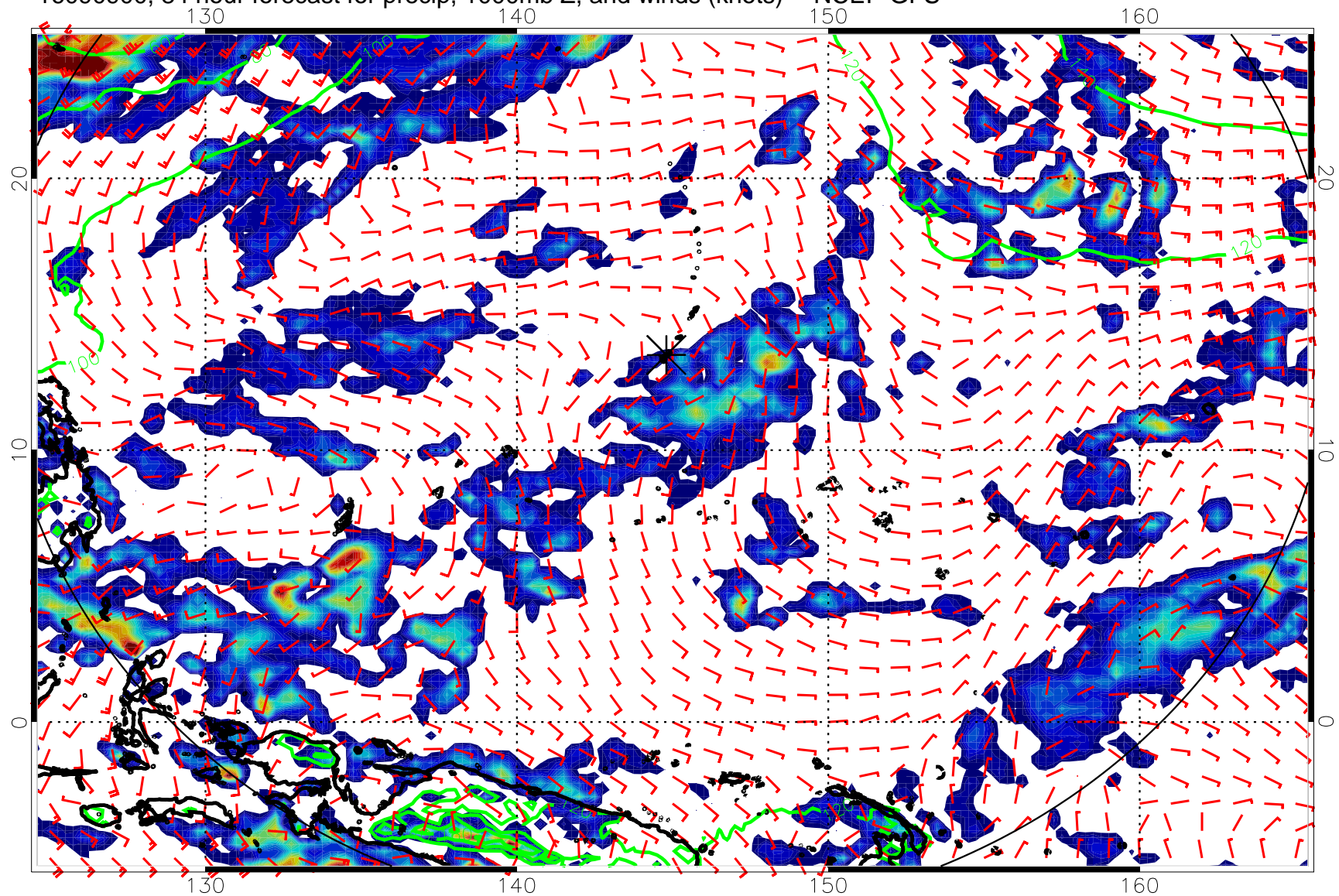
16090900, 84 hour forecast for precip, 1000mb Z, and winds (knots) -- NCEP GFS
