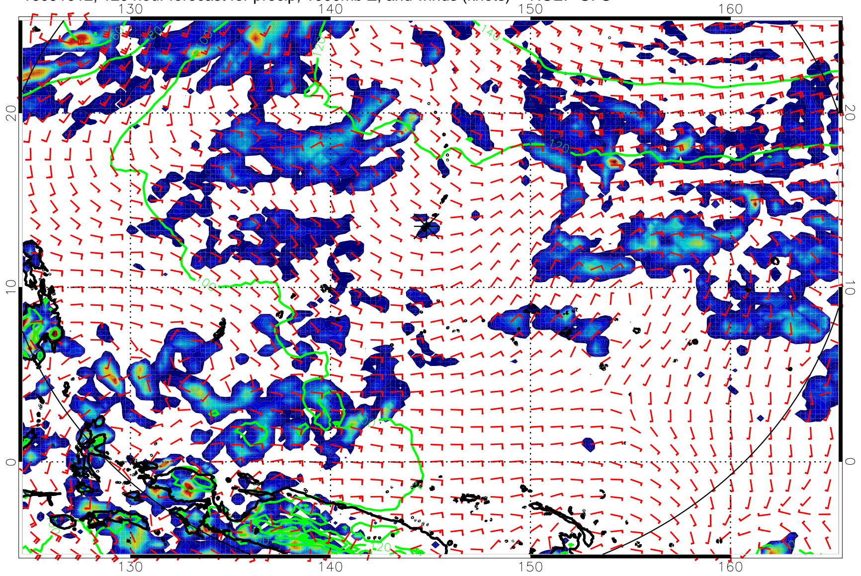
16091012, 120 hour forecast for precip, 1000mb Z, and winds (knots) -- NCEP GFS
