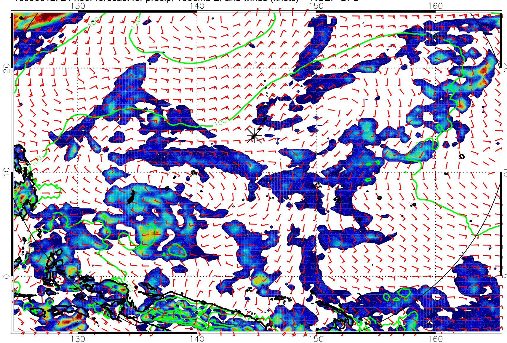
16090612, 24 hour forecast for precip, 1000mb Z, and winds (knots) -- NCEP GFS
