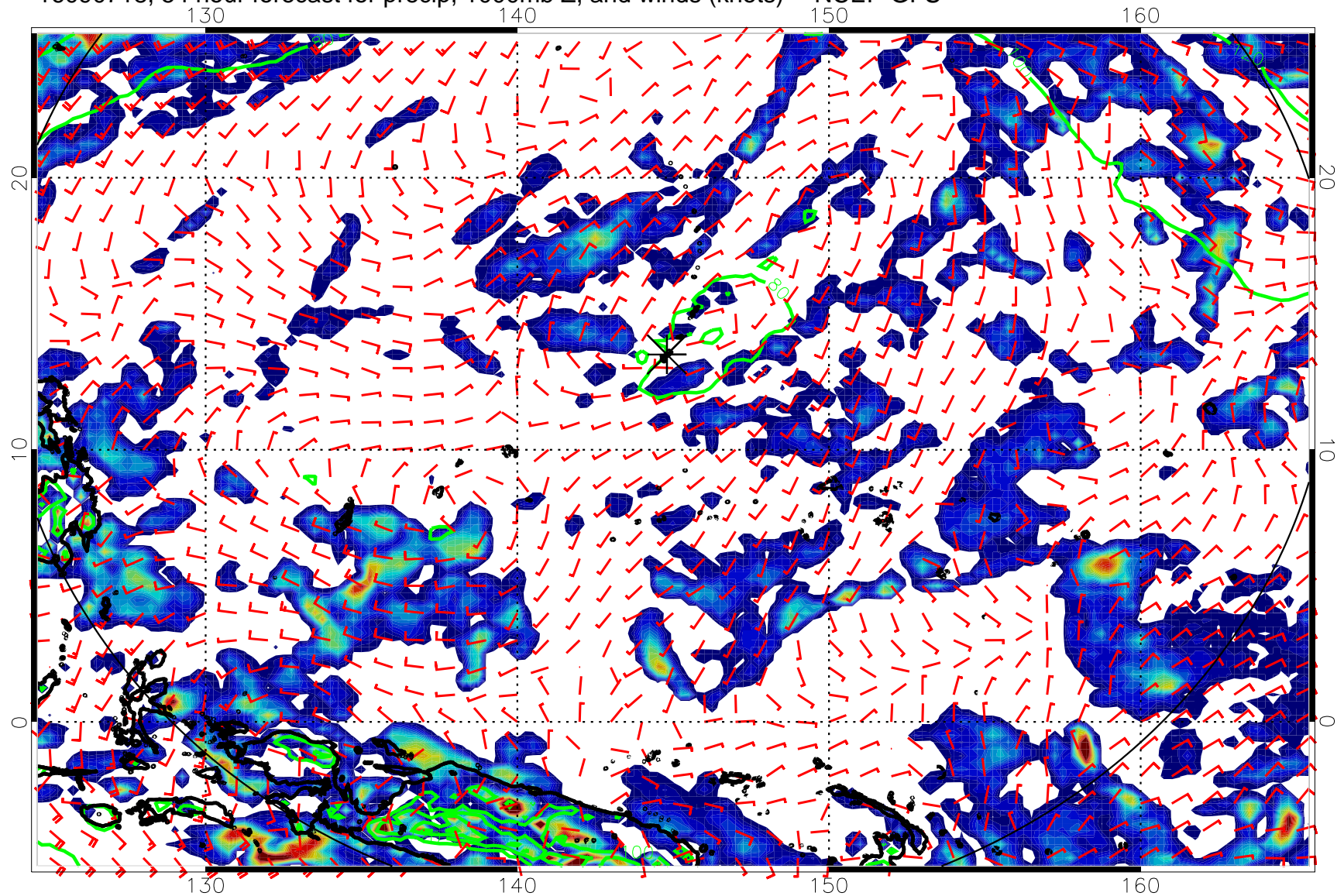
16090718, 54 hour forecast for precip, 1000mb Z, and winds (knots) -- NCEP GFS
