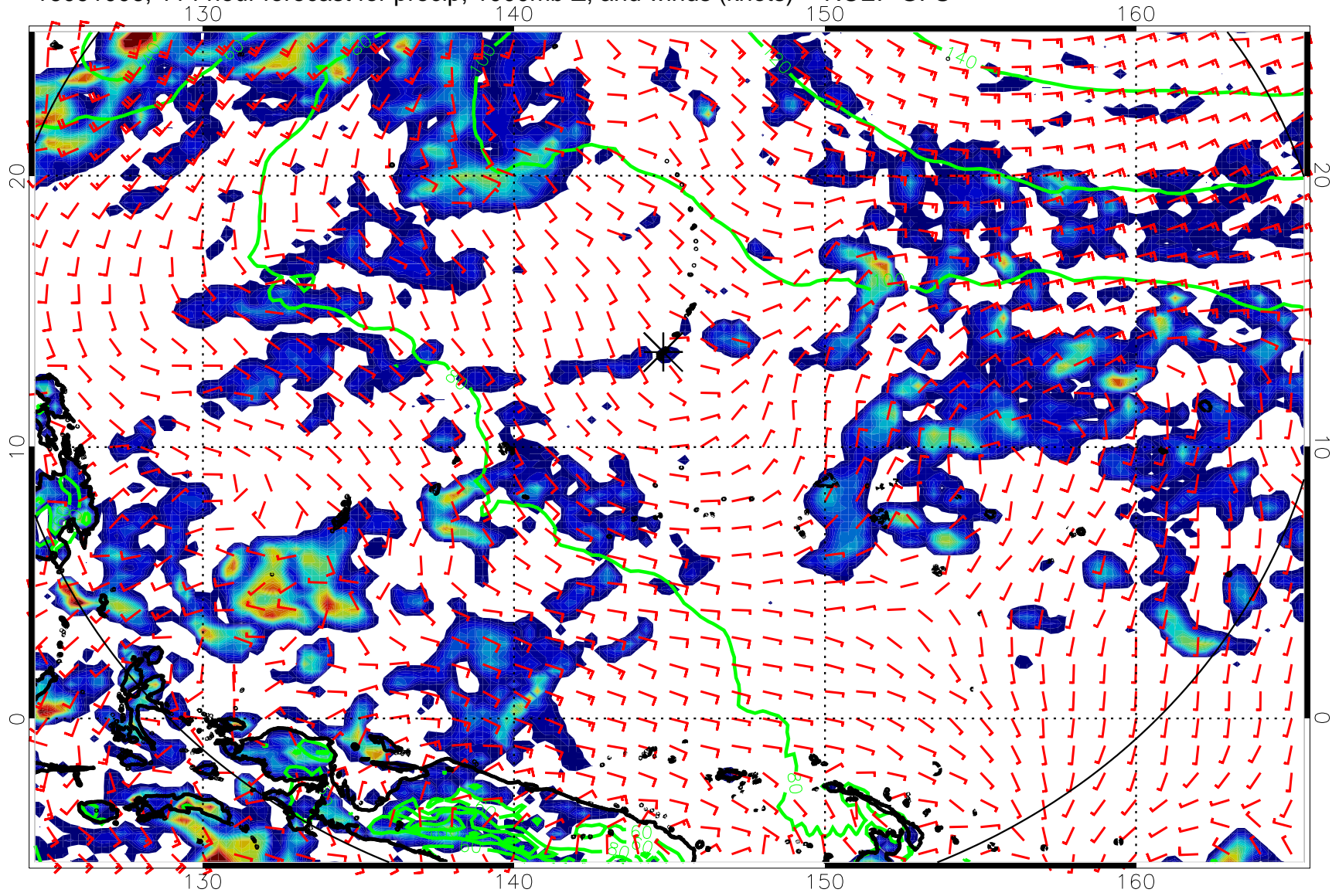
16091006, 114 hour forecast for precip, 1000mb Z, and winds (knots) -- NCEP GFS
