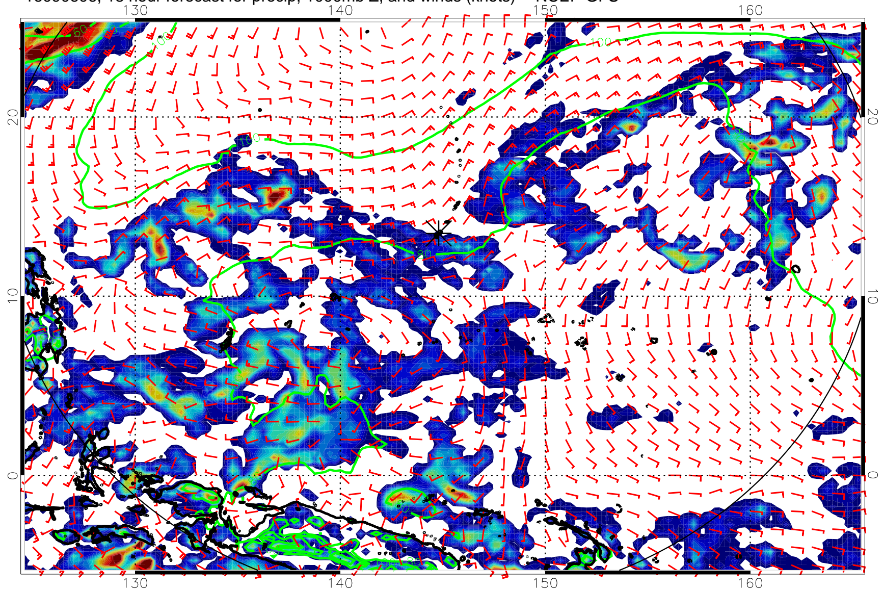
16090606, 18 hour forecast for precip, 1000mb Z, and winds (knots) -- NCEP GFS
