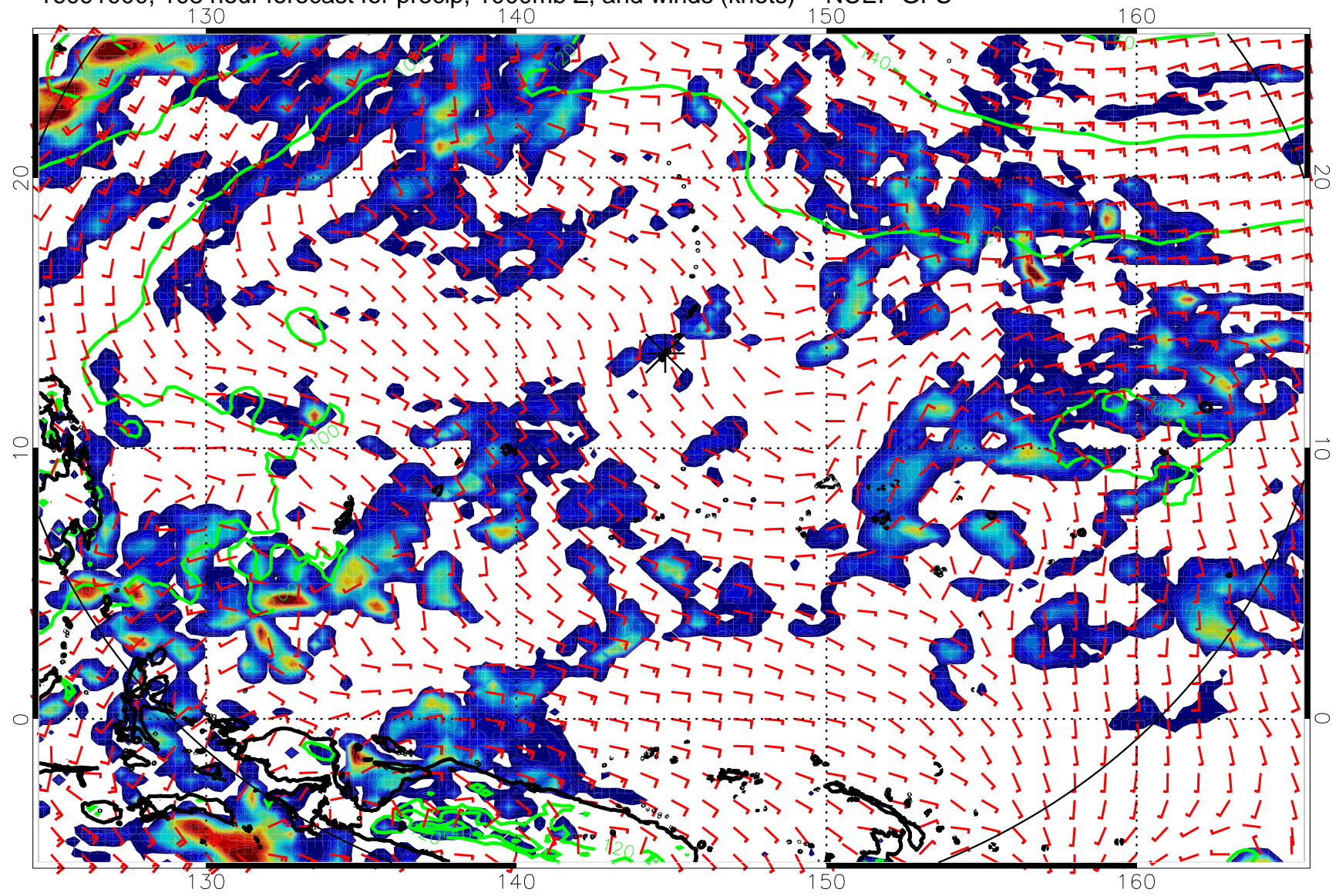
16091000, 108 hour forecast for precip, 1000mb Z, and winds (knots) -- NCEP GFS
