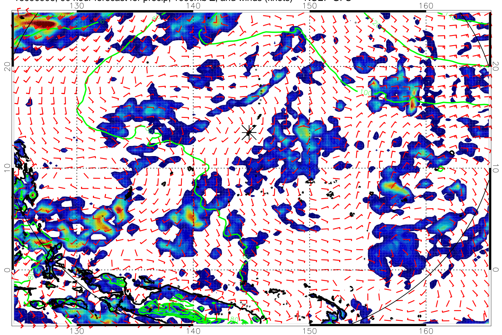
16090906, 90 hour forecast for precip, 1000mb Z, and winds (knots) -- NCEP GFS
