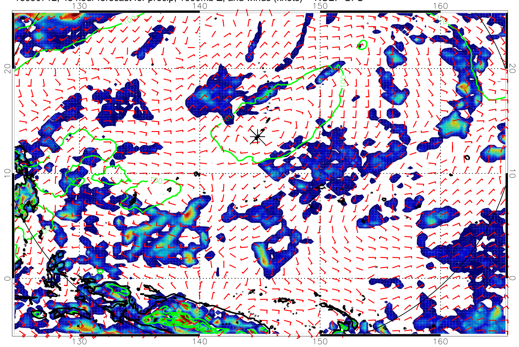
16090712, 48 hour forecast for precip, 1000mb Z, and winds (knots) -- NCEP GFS
