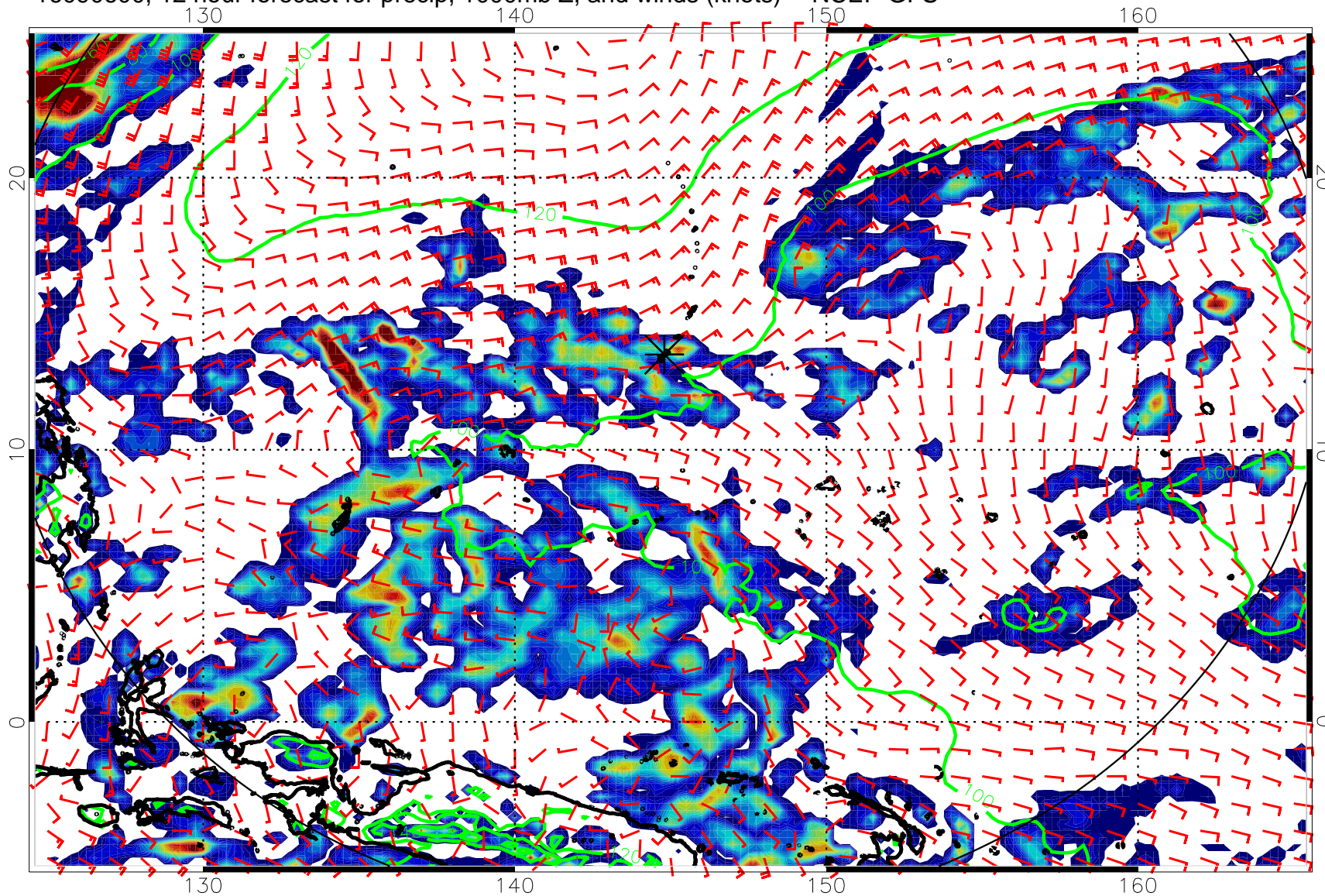
16090600, 12 hour forecast for precip, 1000mb Z, and winds (knots) -- NCEP GFS
