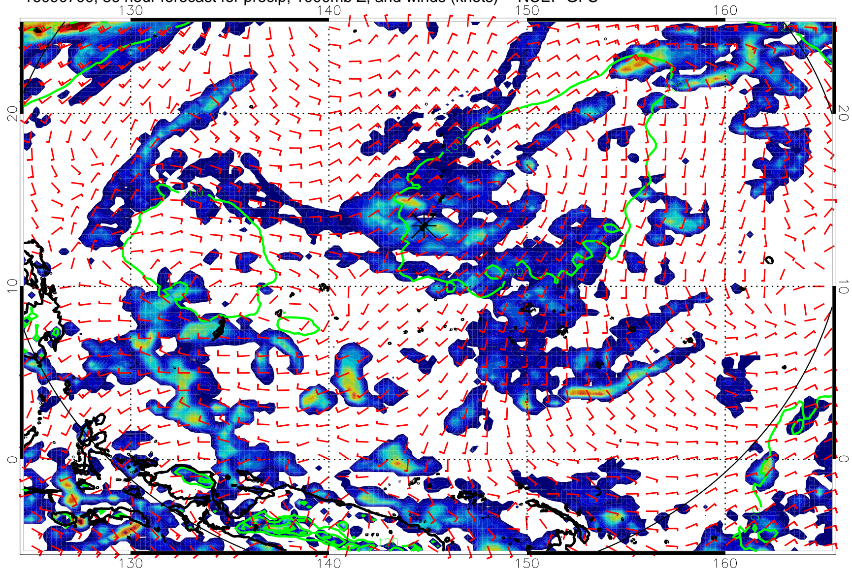
16090700, 36 hour forecast for precip, 1000mb Z, and winds (knots) -- NCEP GFS
