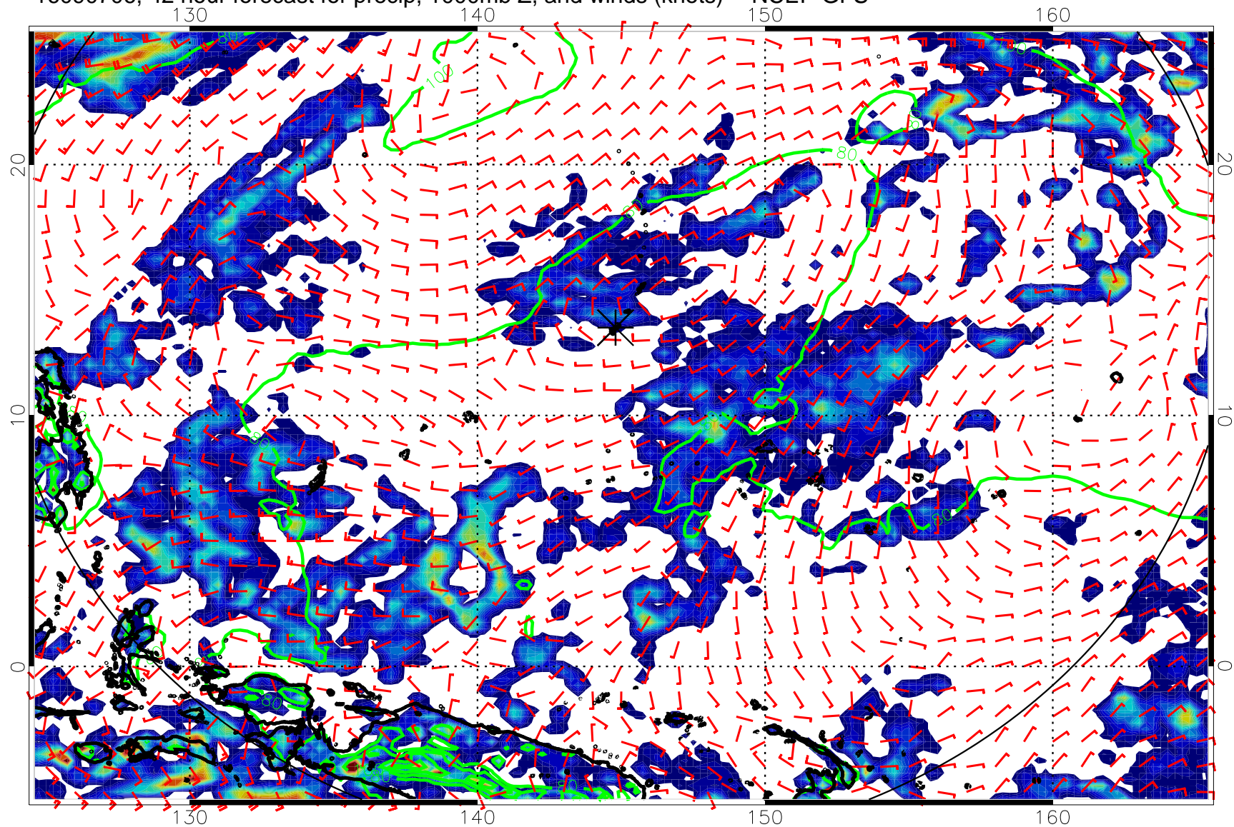
16090706, 42 hour forecast for precip, 1000mb Z, and winds (knots) -- NCEP GFS
