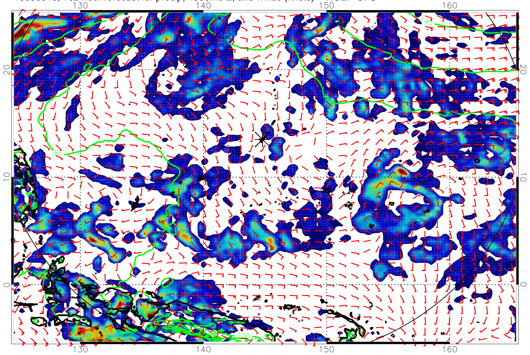
16090918, 102 hour forecast for precip, 1000mb Z, and winds (knots) -- NCEP GFS
