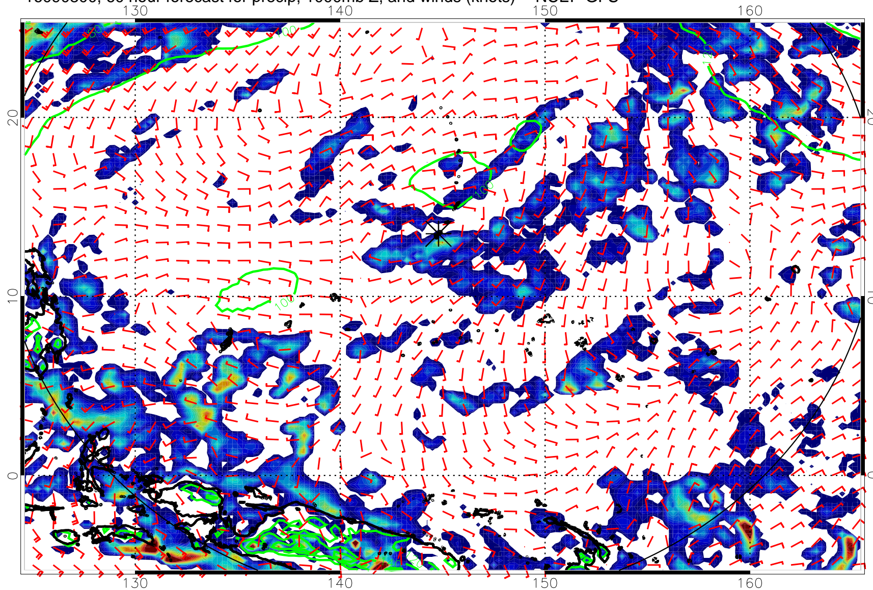
16090800, 60 hour forecast for precip, 1000mb Z, and winds (knots) -- NCEP GFS
