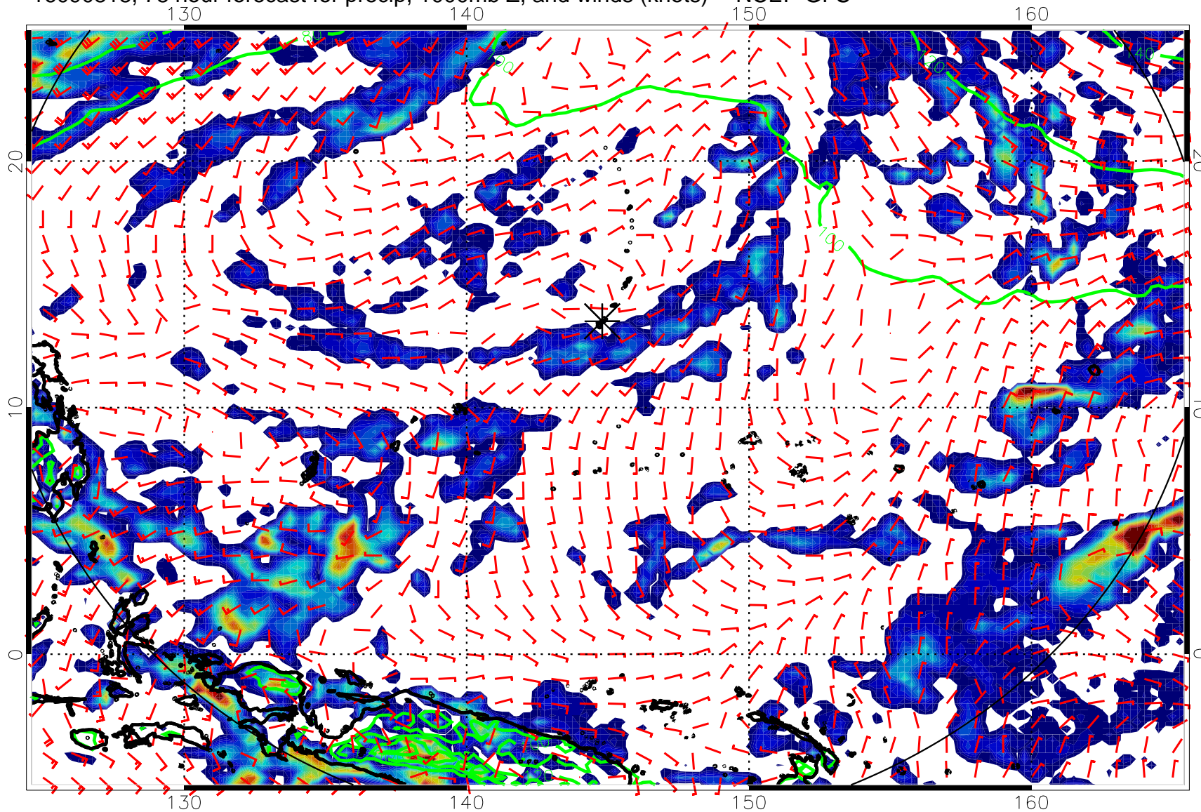
16090818, 78 hour forecast for precip, 1000mb Z, and winds (knots) -- NCEP GFS
