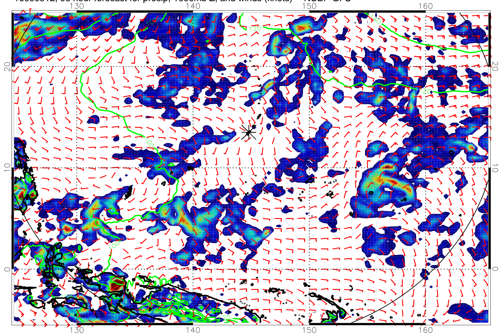
16090912, 96 hour forecast for precip, 1000mb Z, and winds (knots) -- NCEP GFS
