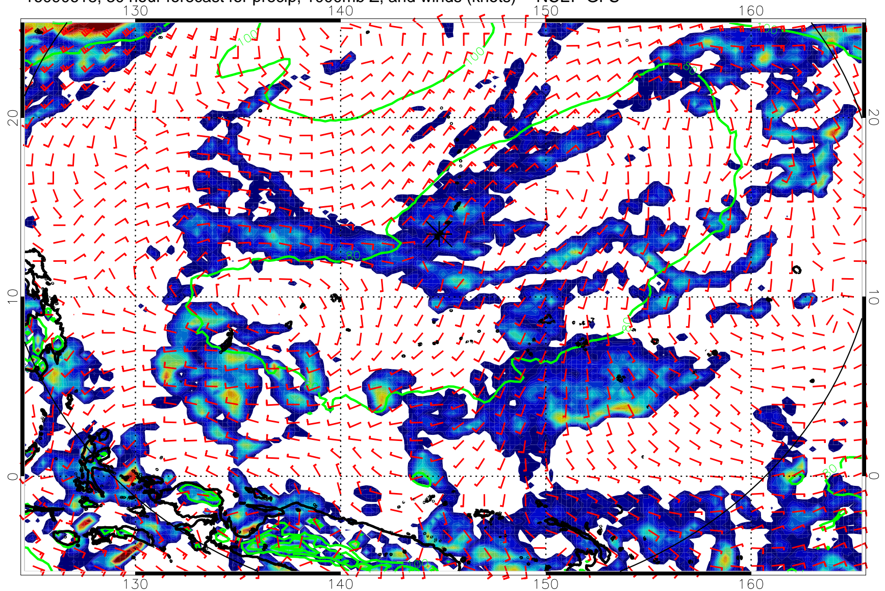
16090618, 30 hour forecast for precip, 1000mb Z, and winds (knots) -- NCEP GFS
