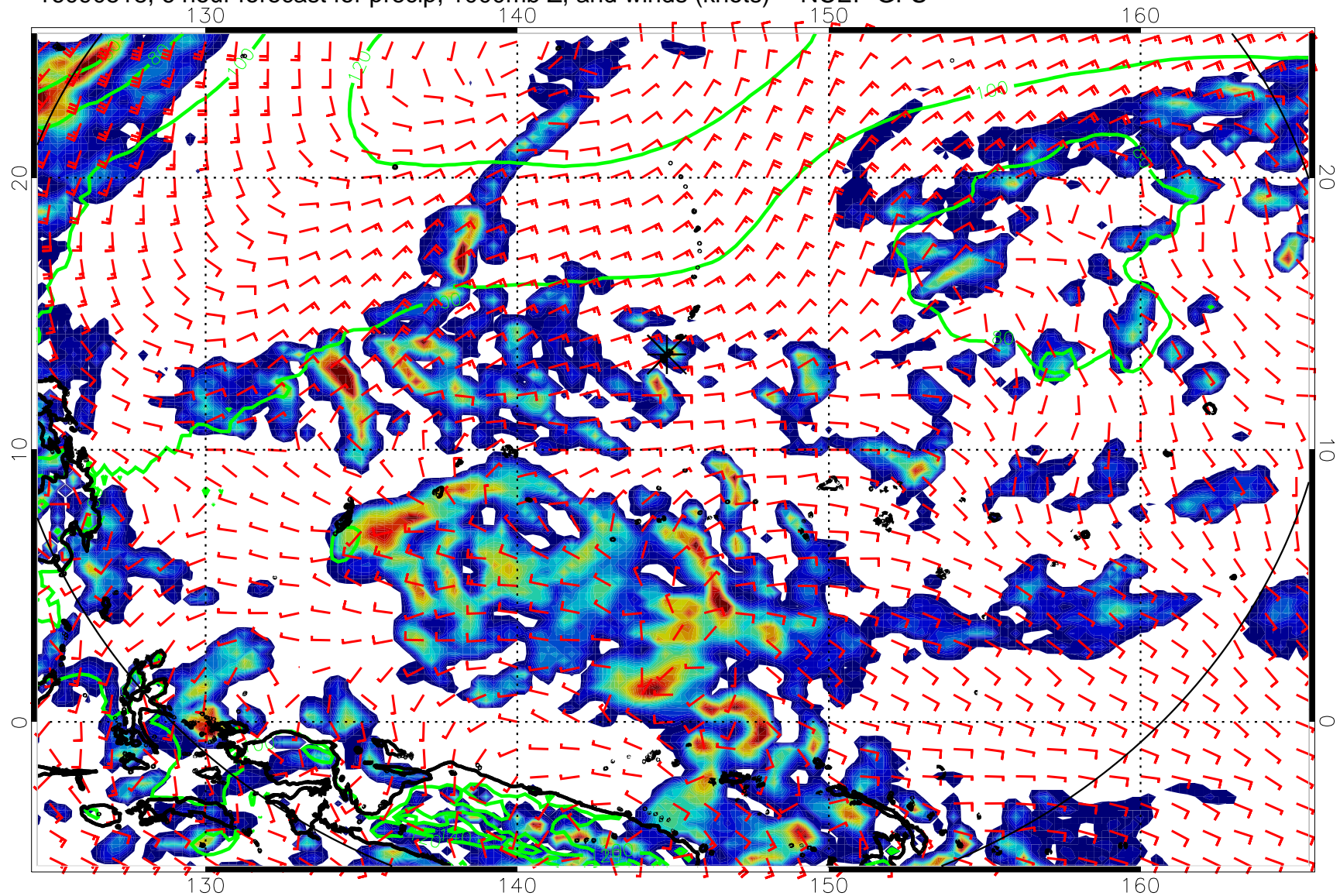
16090518, 6 hour forecast for precip, 1000mb Z, and winds (knots) -- NCEP GFS
