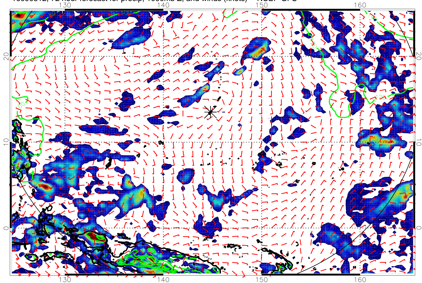
16090812, 72 hour forecast for precip, 1000mb Z, and winds (knots) -- NCEP GFS
