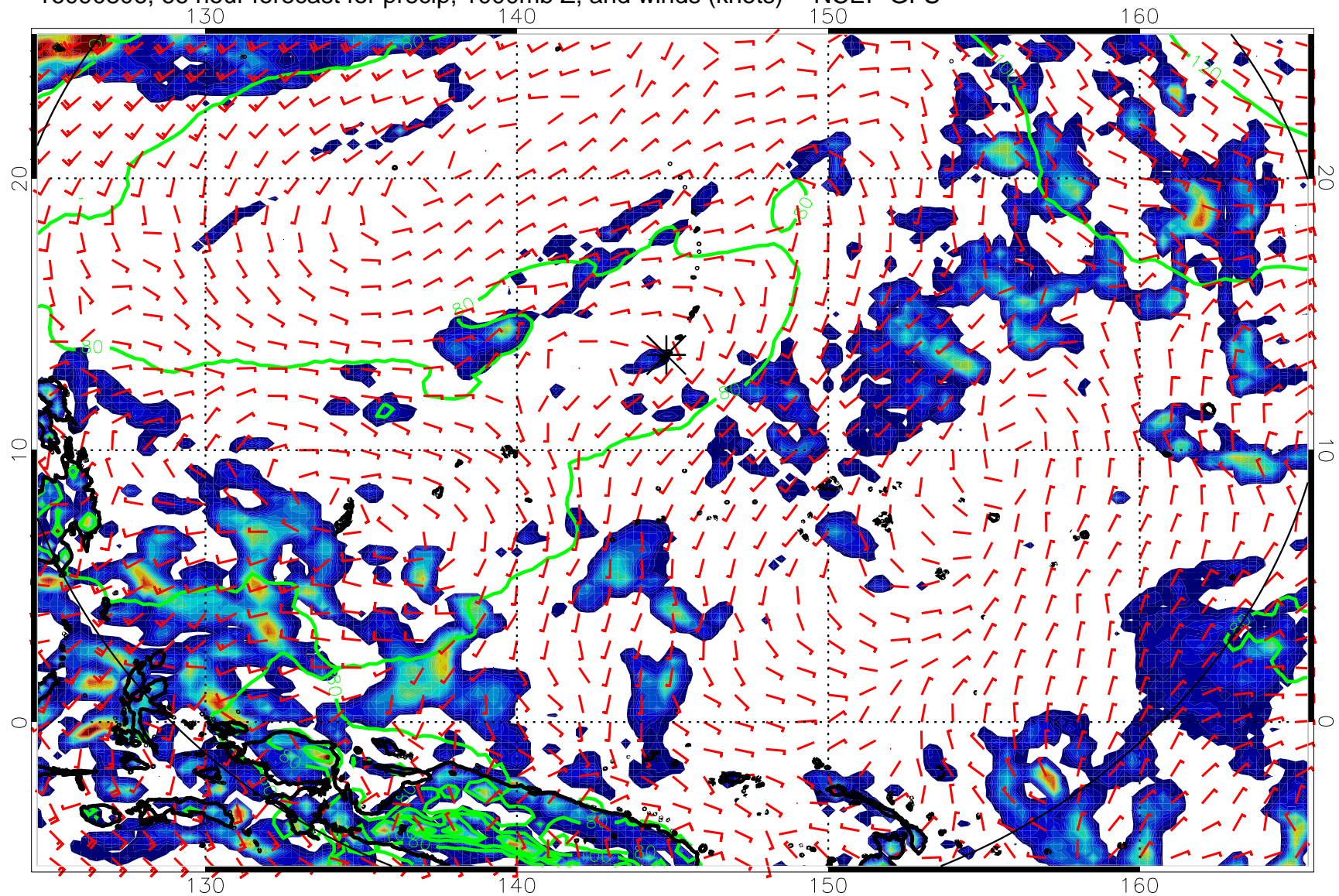
16090806, 66 hour forecast for precip, 1000mb Z, and winds (knots) -- NCEP GFS
