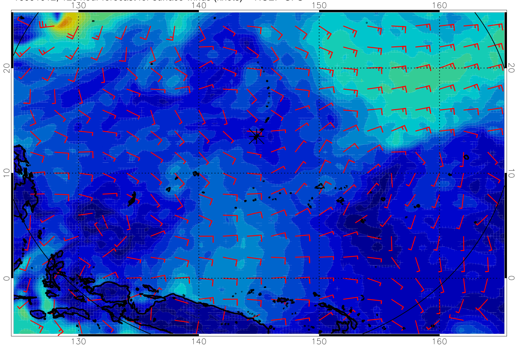
16091012, 120 hour forecast for surface winds (knots) -- NCEP GFS
