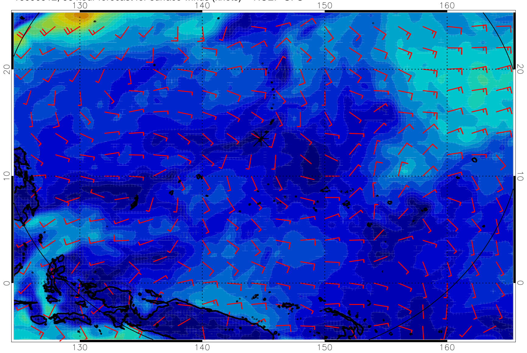
16090912, 96 hour forecast for surface winds (knots) -- NCEP GFS
