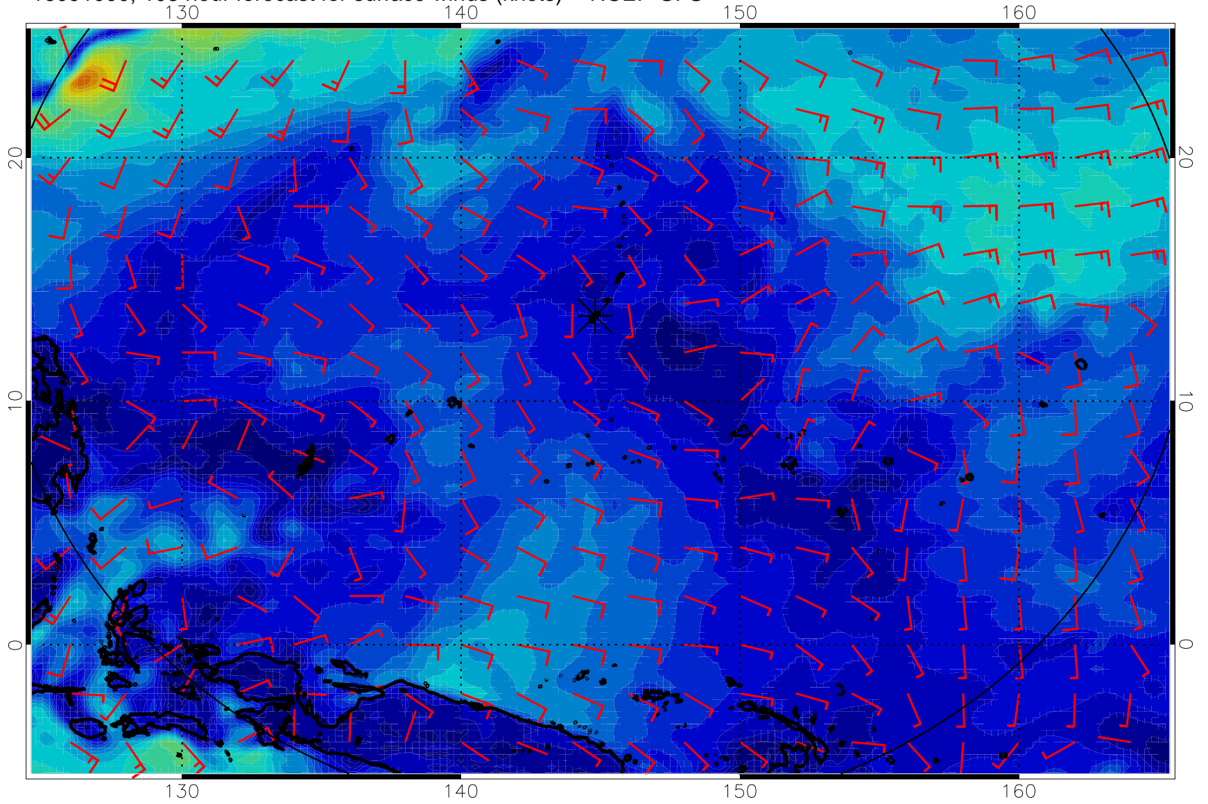
16091000, 108 hour forecast for surface winds (knots) -- NCEP GFS
