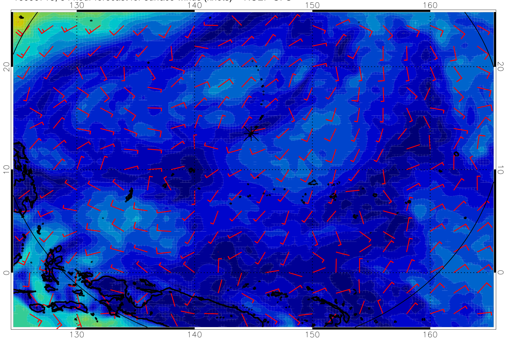
16090718, 54 hour forecast for surface winds (knots) -- NCEP GFS
