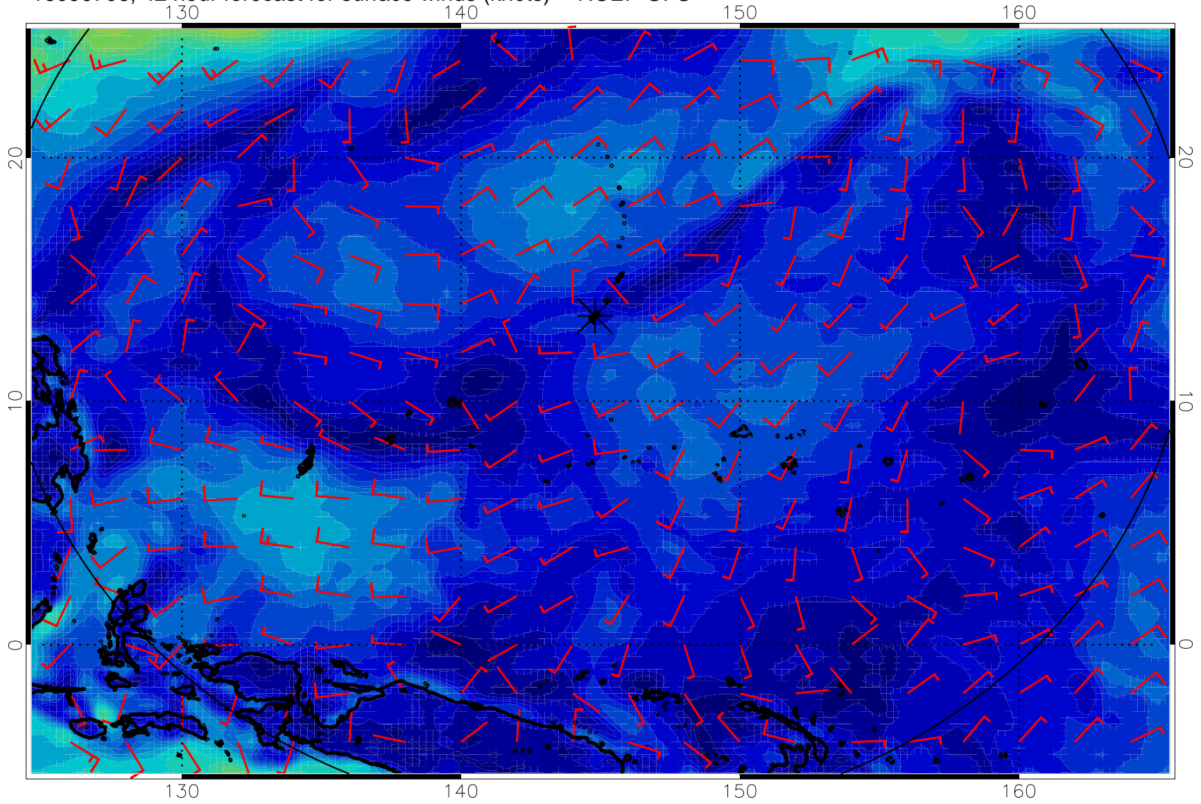
16090706, 42 hour forecast for surface winds (knots) -- NCEP GFS
