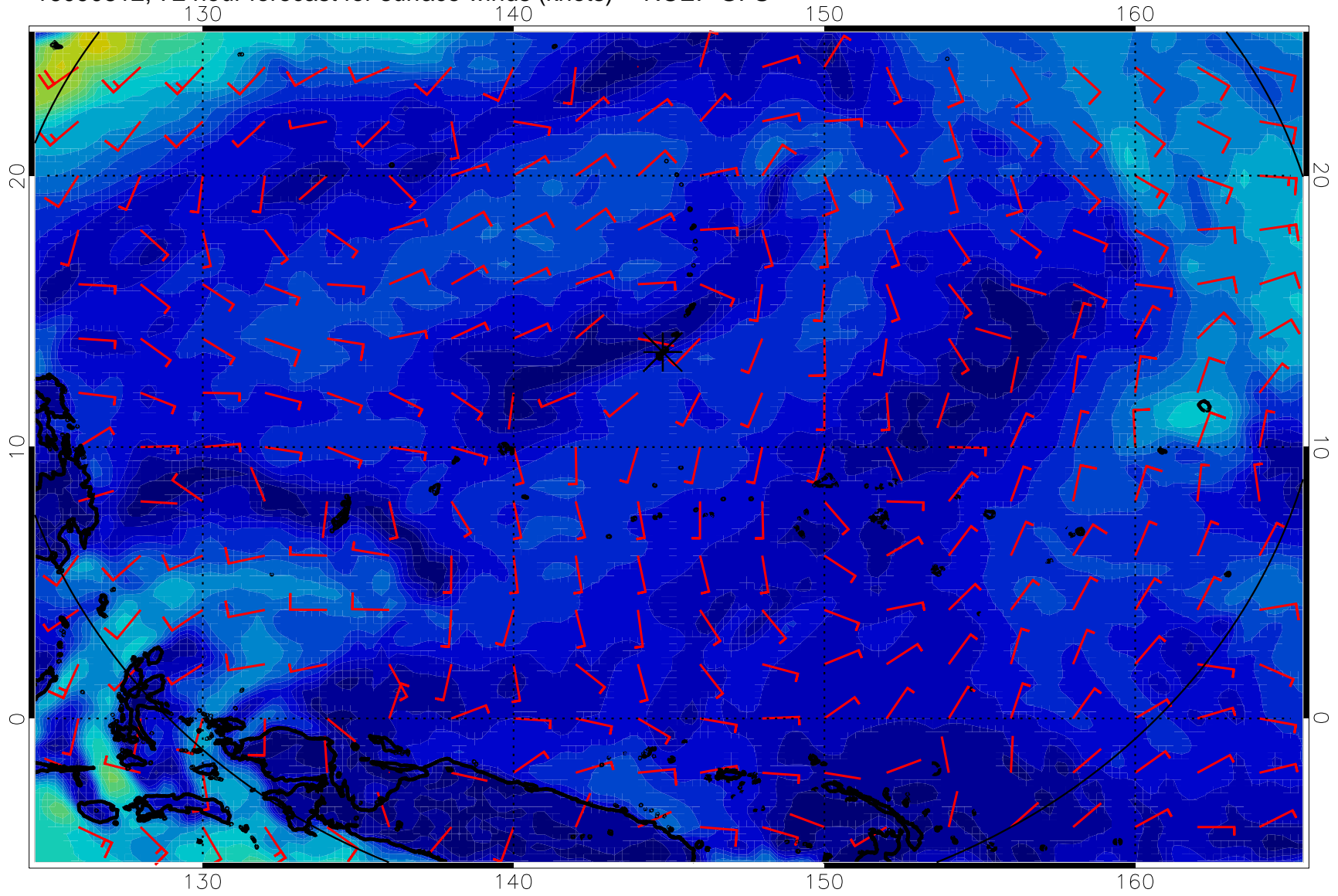
16090812, 72 hour forecast for surface winds (knots) -- NCEP GFS
