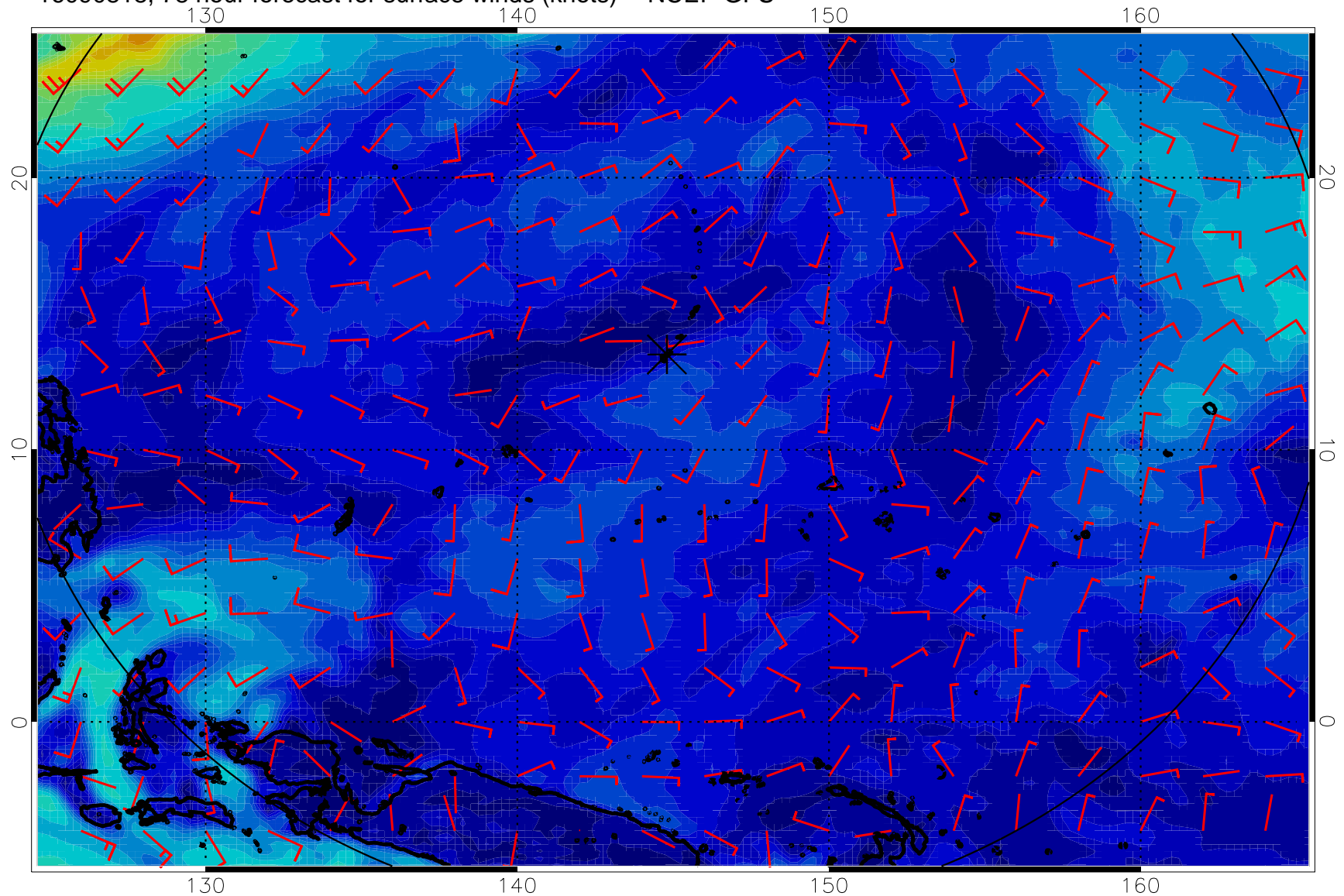
16090818, 78 hour forecast for surface winds (knots) -- NCEP GFS
