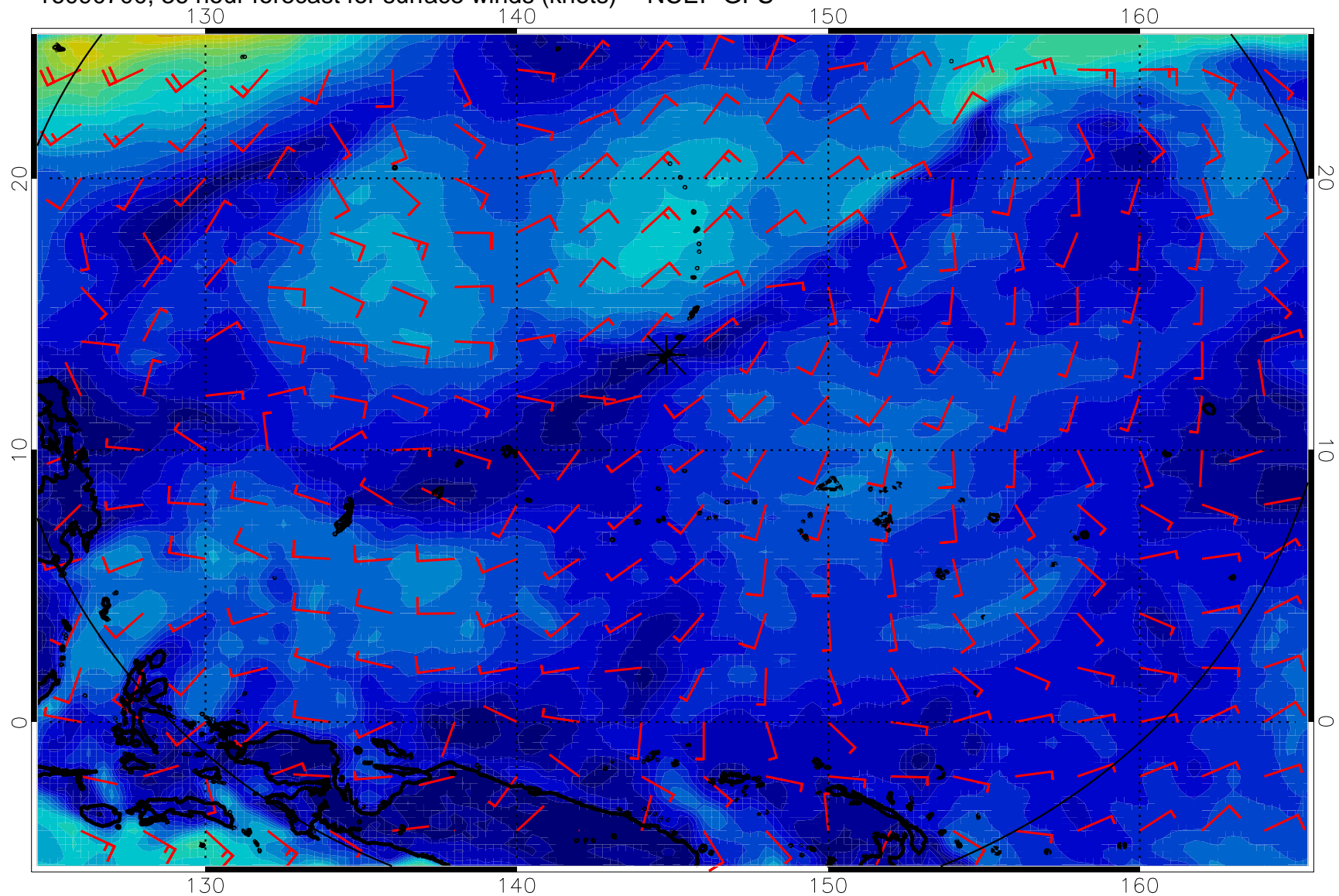
16090700, 36 hour forecast for surface winds (knots) -- NCEP GFS
