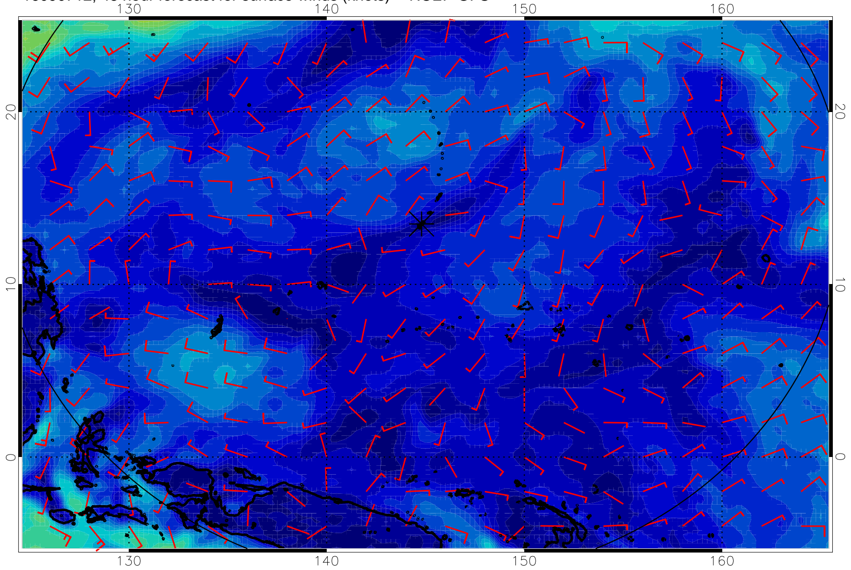
16090712, 48 hour forecast for surface winds (knots) -- NCEP GFS
