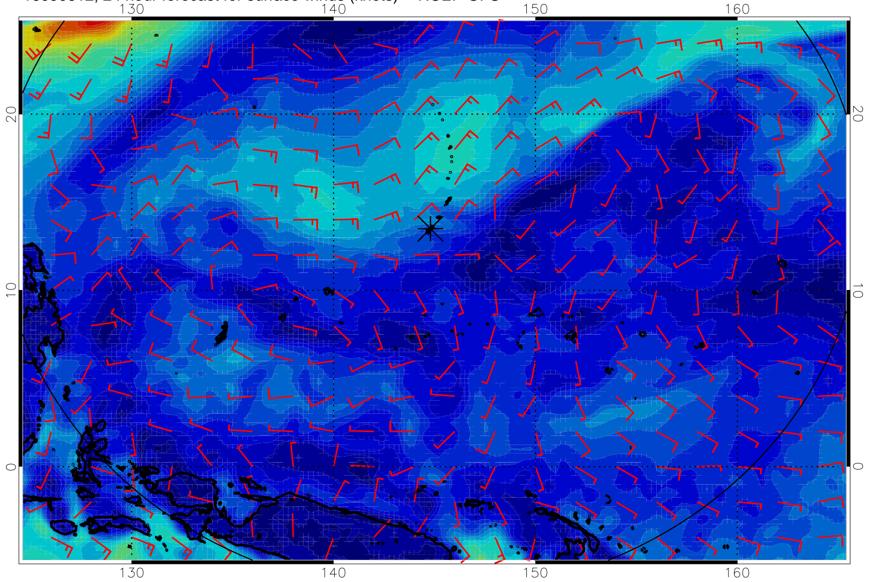
16090612, 24 hour forecast for surface winds (knots) -- NCEP GFS
