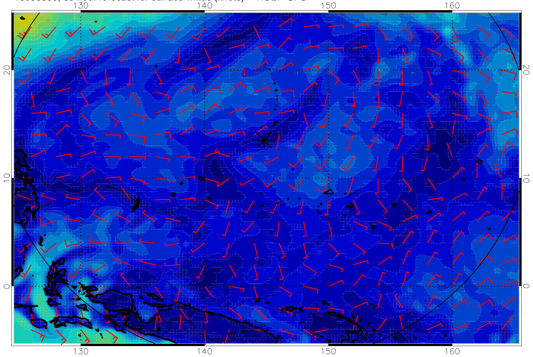
16090800, 60 hour forecast for surface winds (knots) -- NCEP GFS
