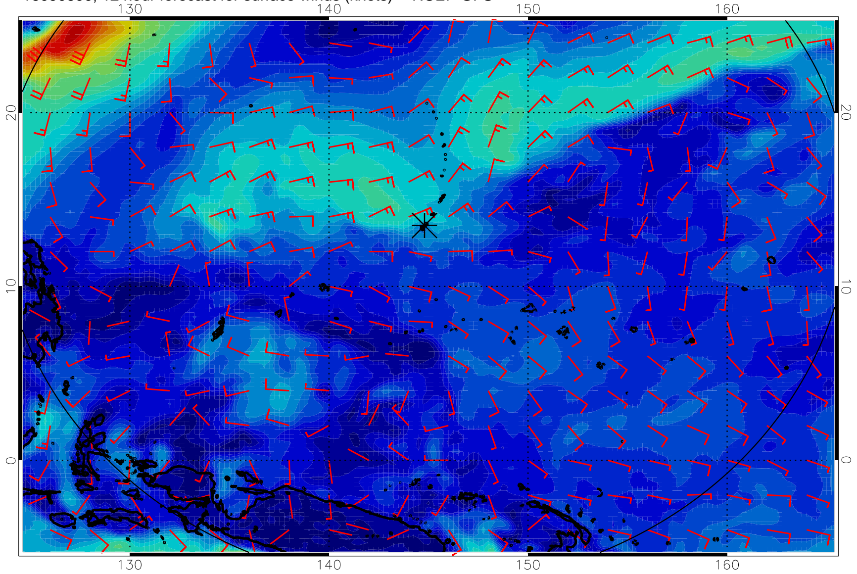
16090600, 12 hour forecast for surface winds (knots) -- NCEP GFS
