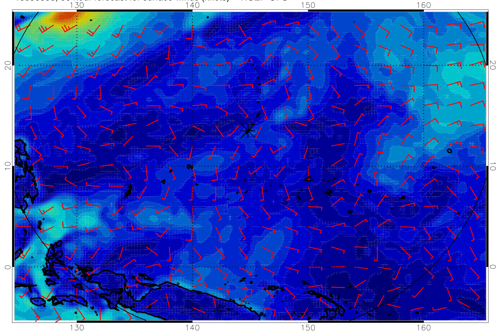
16090906, 90 hour forecast for surface winds (knots) -- NCEP GFS
