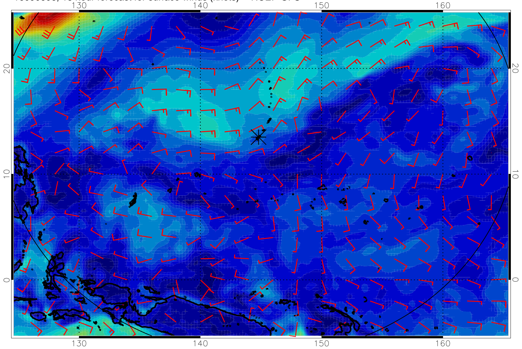
16090606, 18 hour forecast for surface winds (knots) -- NCEP GFS
