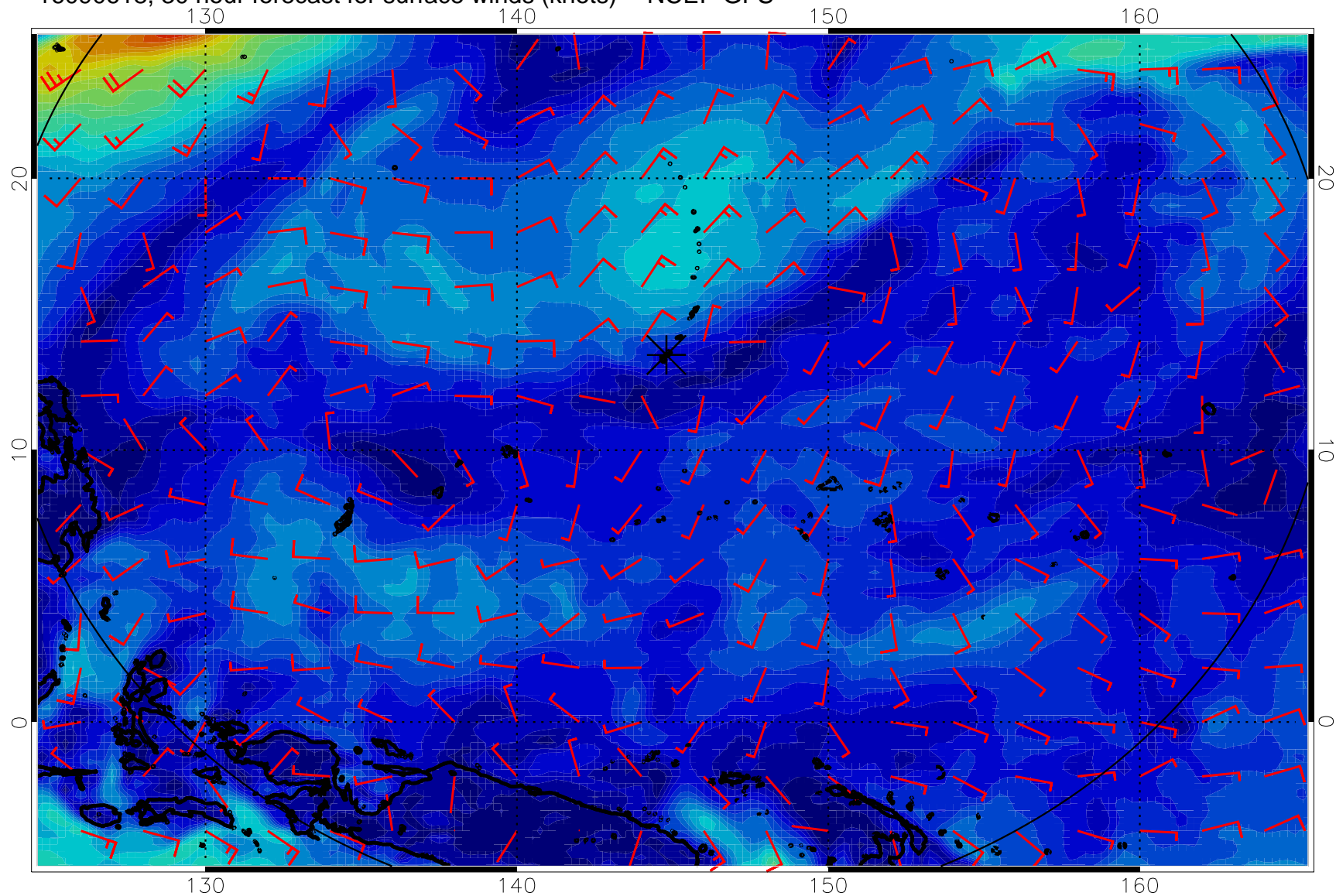
16090618, 30 hour forecast for surface winds (knots) -- NCEP GFS
