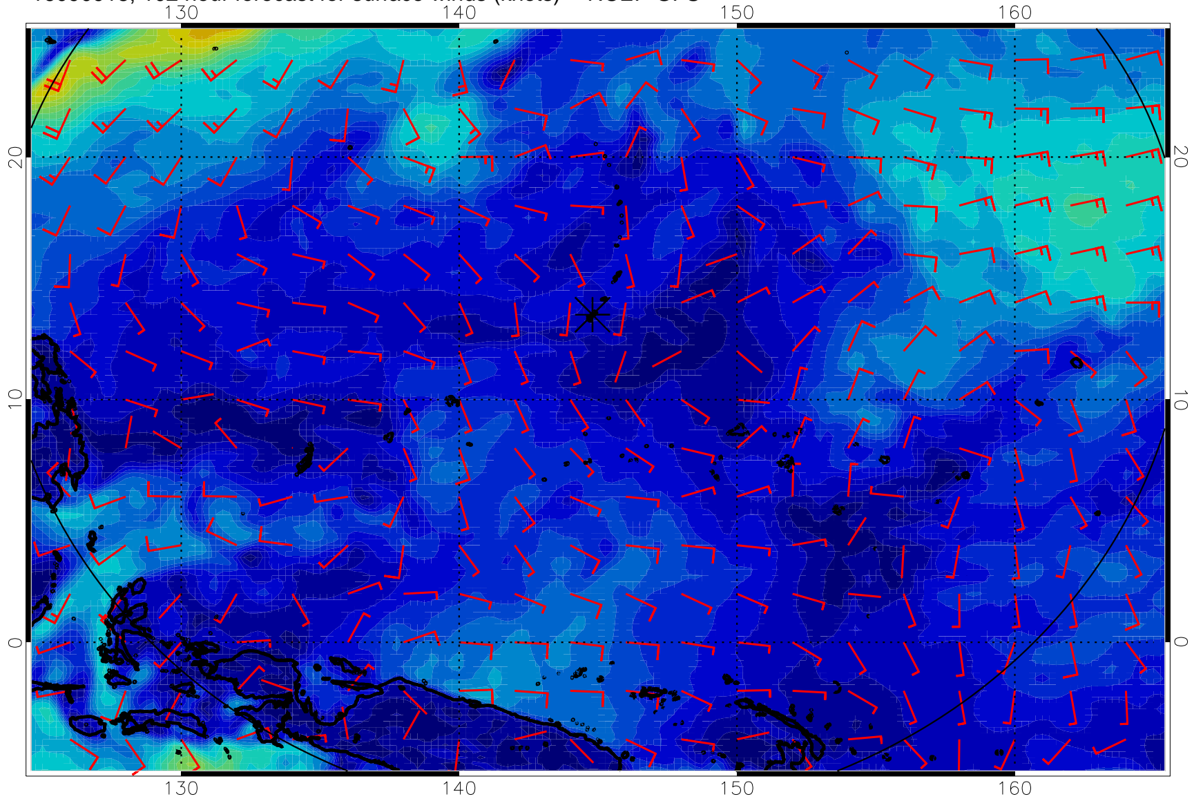
16090918, 102 hour forecast for surface winds (knots) -- NCEP GFS
