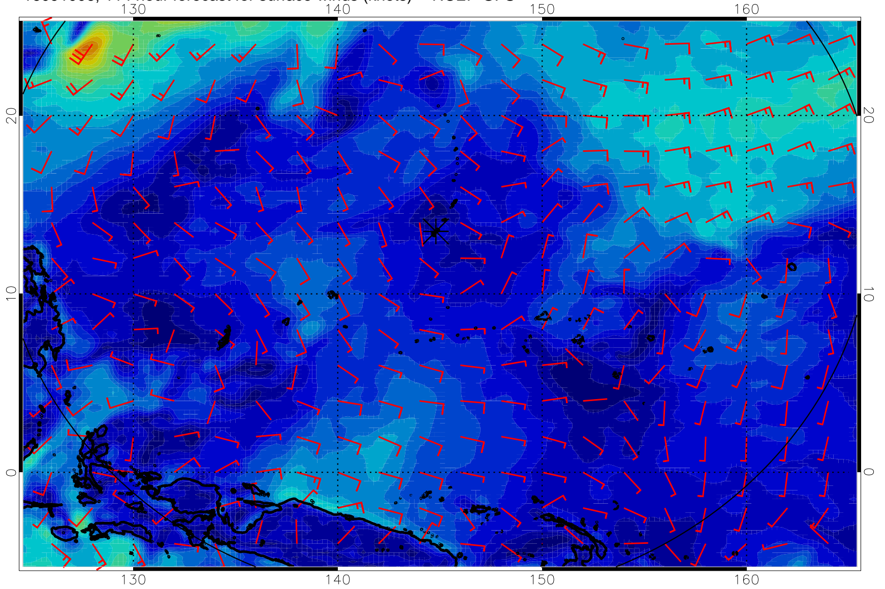
16091006, 114 hour forecast for surface winds (knots) -- NCEP GFS
