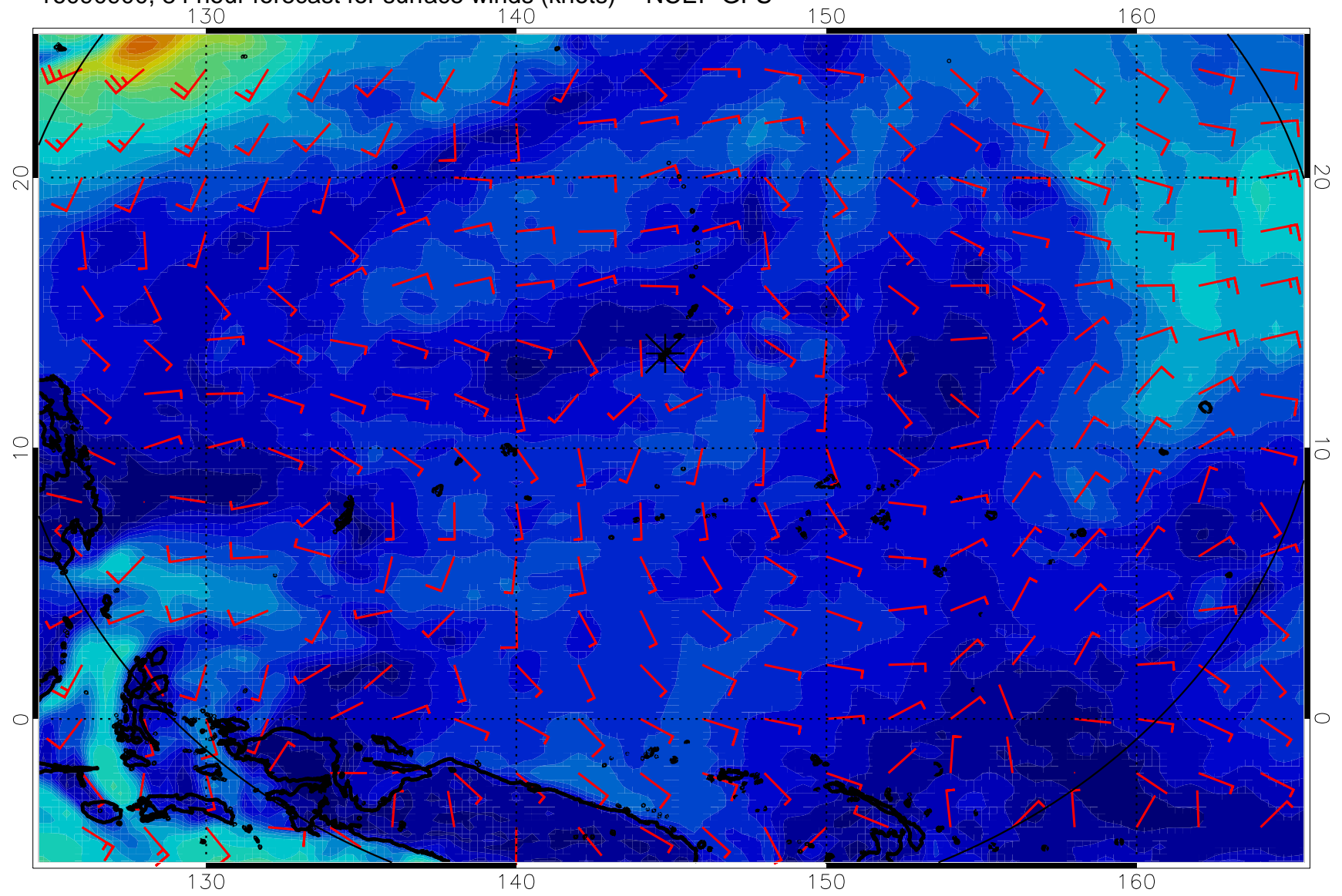
16090900, 84 hour forecast for surface winds (knots) -- NCEP GFS
