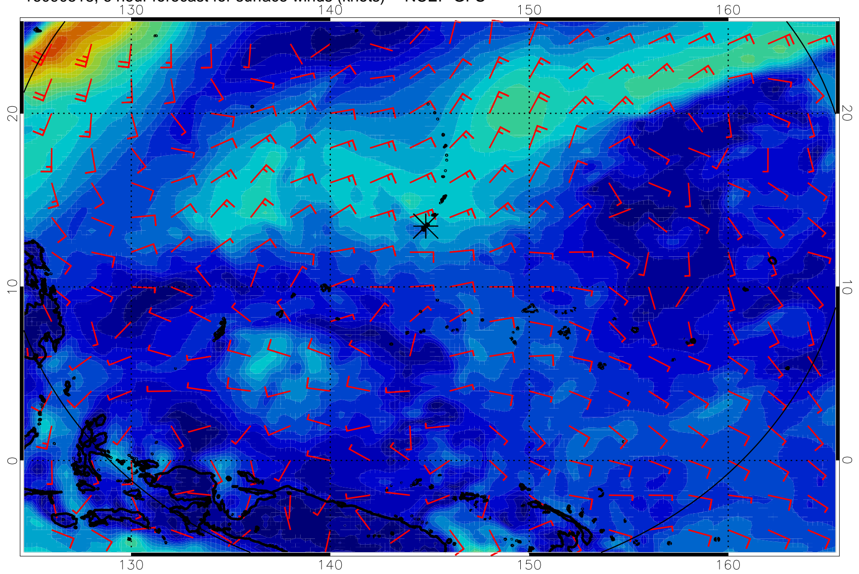
16090518, 6 hour forecast for surface winds (knots) -- NCEP GFS
