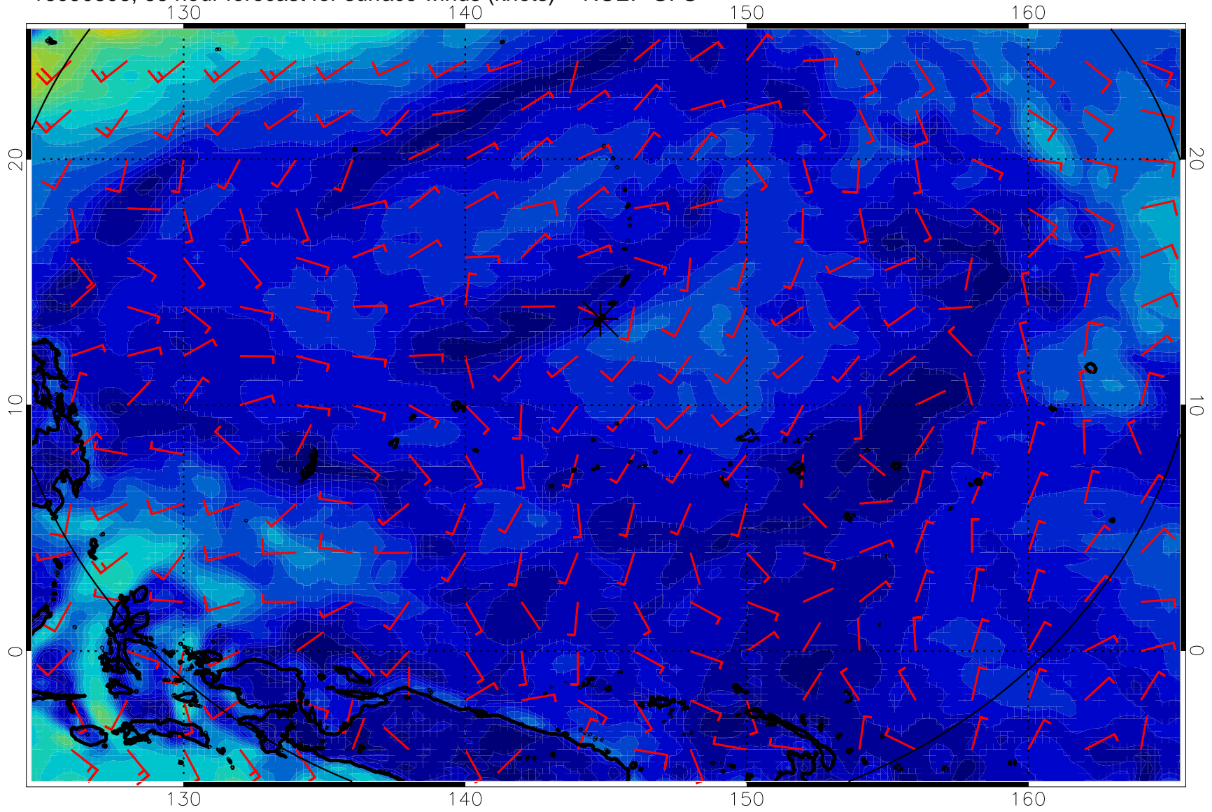
16090806, 66 hour forecast for surface winds (knots) -- NCEP GFS
