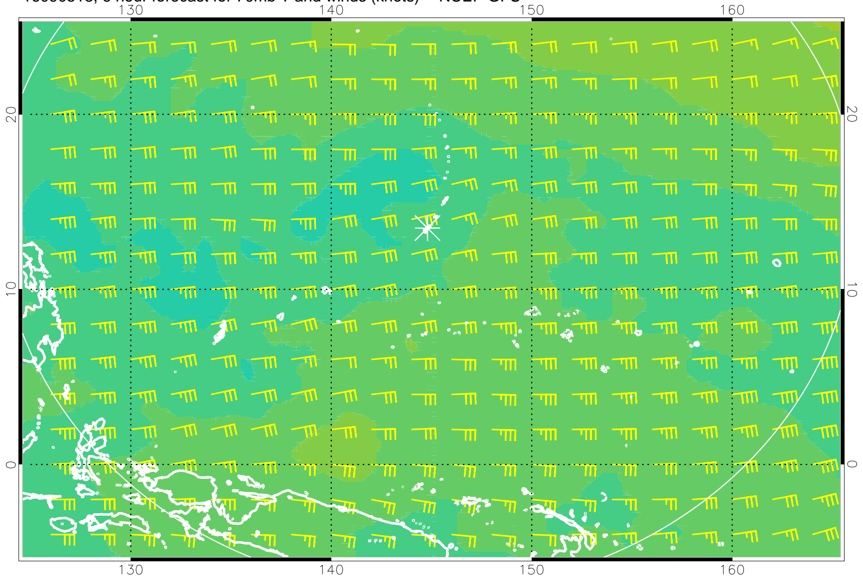
16090518, 6 hour forecast for 70mb T and winds (knots) -- NCEP GFS
