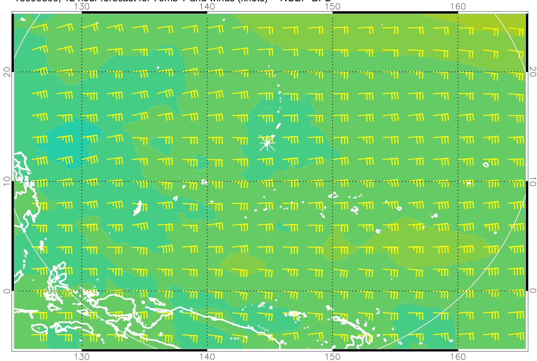
16090600, 12 hour forecast for 70mb T and winds (knots) -- NCEP GFS
