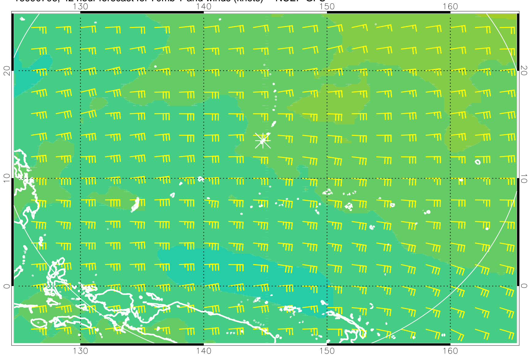
16090706, 42 hour forecast for 70mb T and winds (knots) -- NCEP GFS
