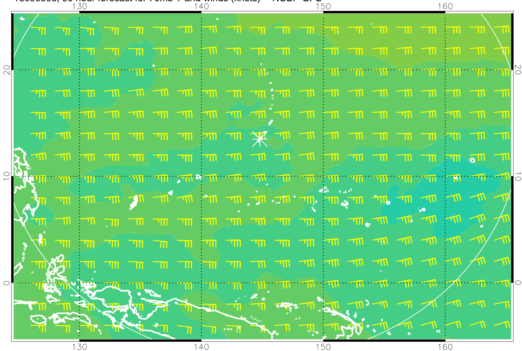
16090906, 90 hour forecast for 70mb T and winds (knots) -- NCEP GFS
