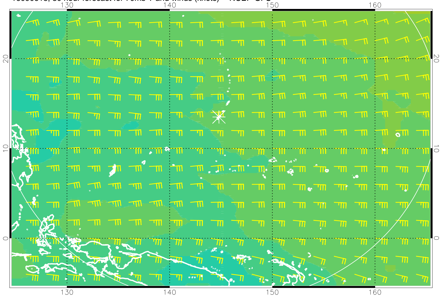
16090618, 30 hour forecast for 70mb T and winds (knots) -- NCEP GFS
