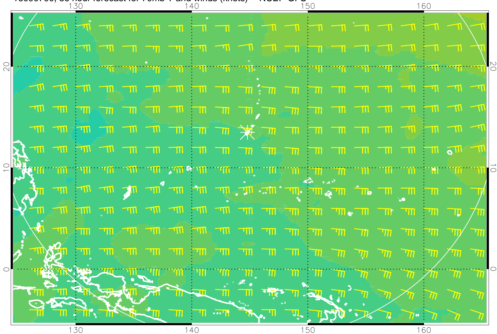
16090700, 36 hour forecast for 70mb T and winds (knots) -- NCEP GFS
