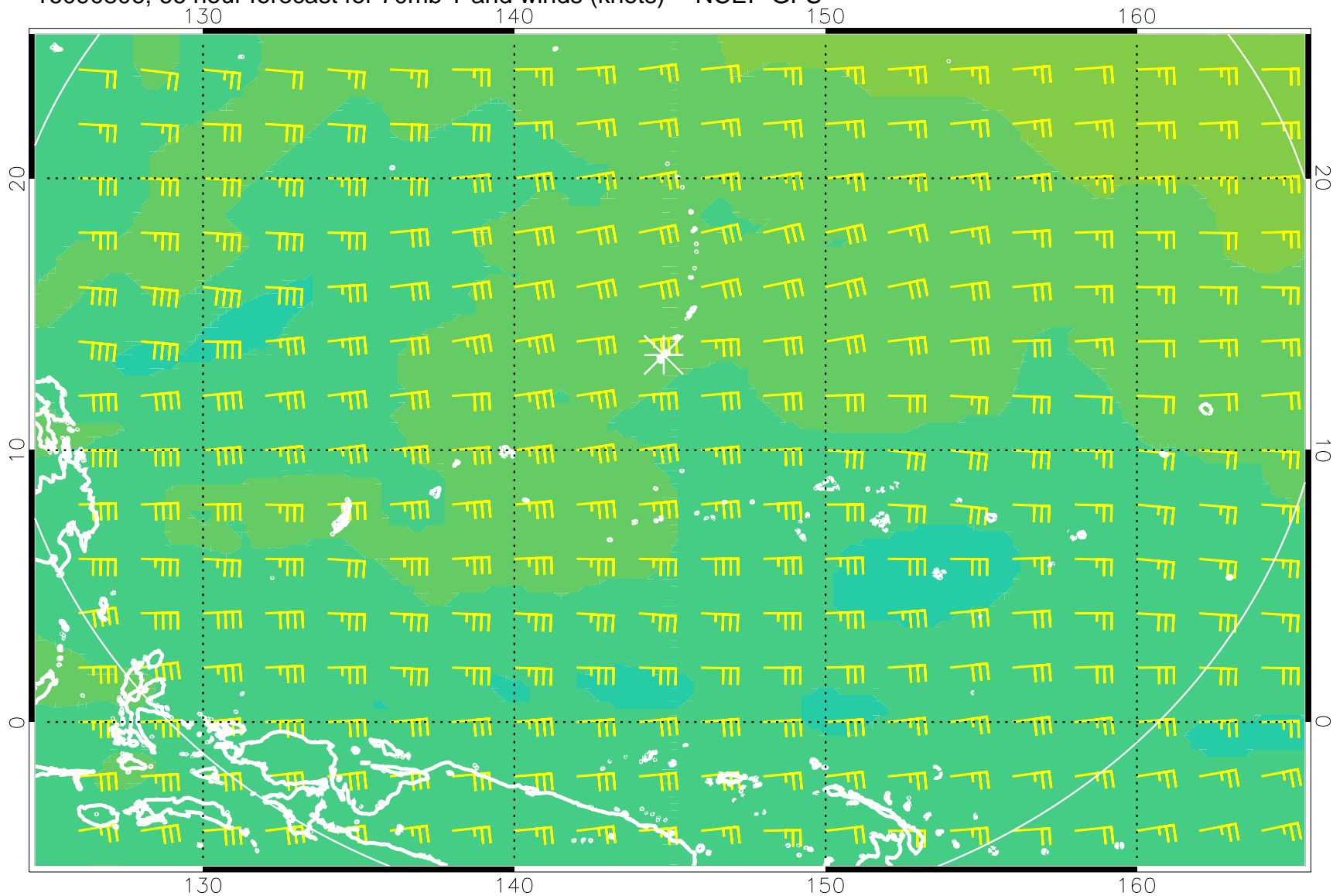
16090806, 66 hour forecast for 70mb T and winds (knots) -- NCEP GFS
