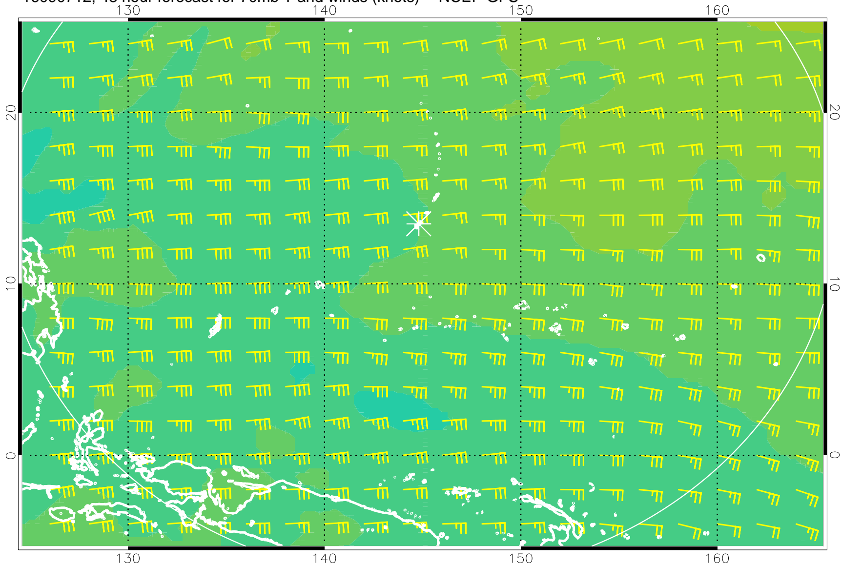
16090712, 48 hour forecast for 70mb T and winds (knots) -- NCEP GFS
