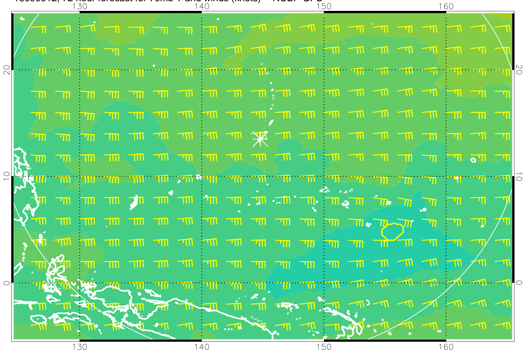
16090812, 72 hour forecast for 70mb T and winds (knots) -- NCEP GFS
