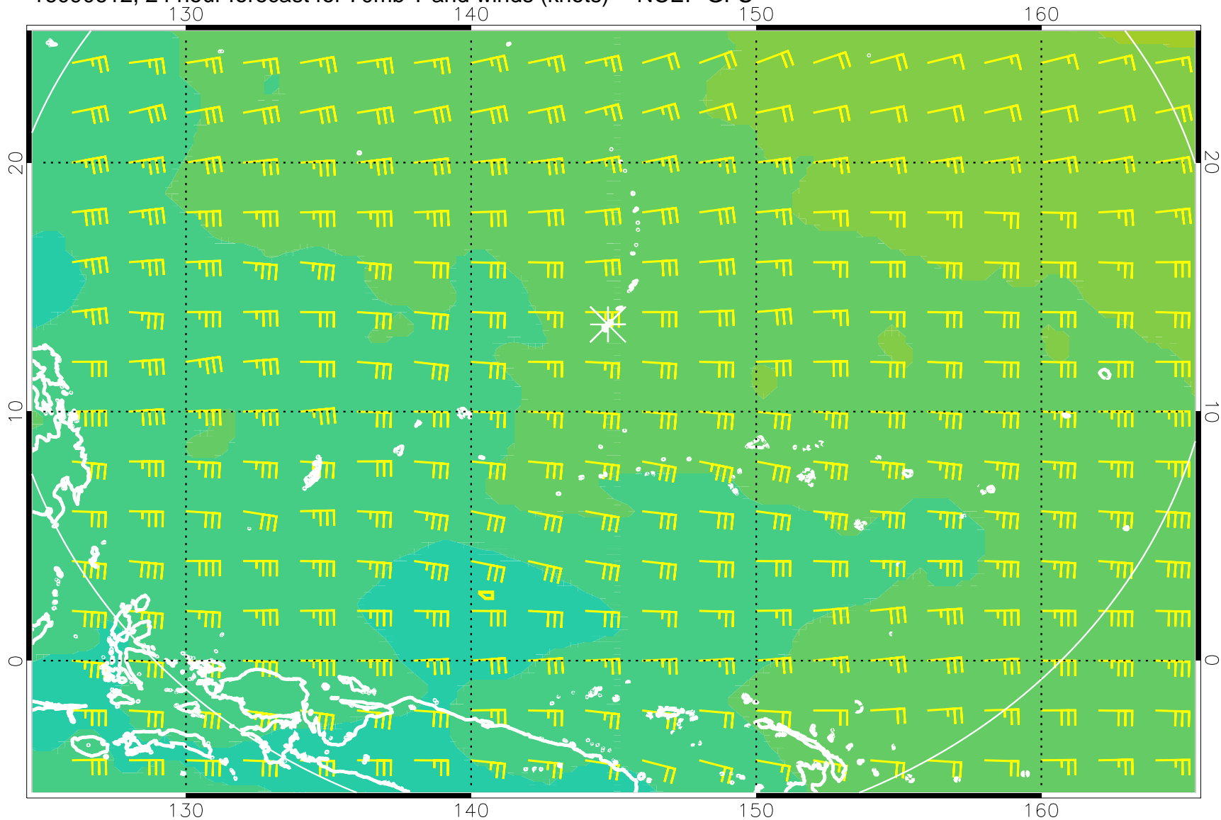
16090612, 24 hour forecast for 70mb T and winds (knots) -- NCEP GFS
