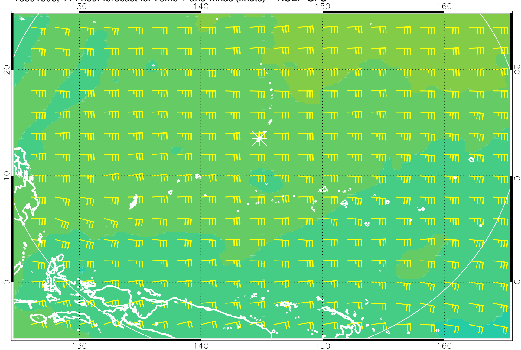
16091006, 114 hour forecast for 70mb T and winds (knots) -- NCEP GFS
