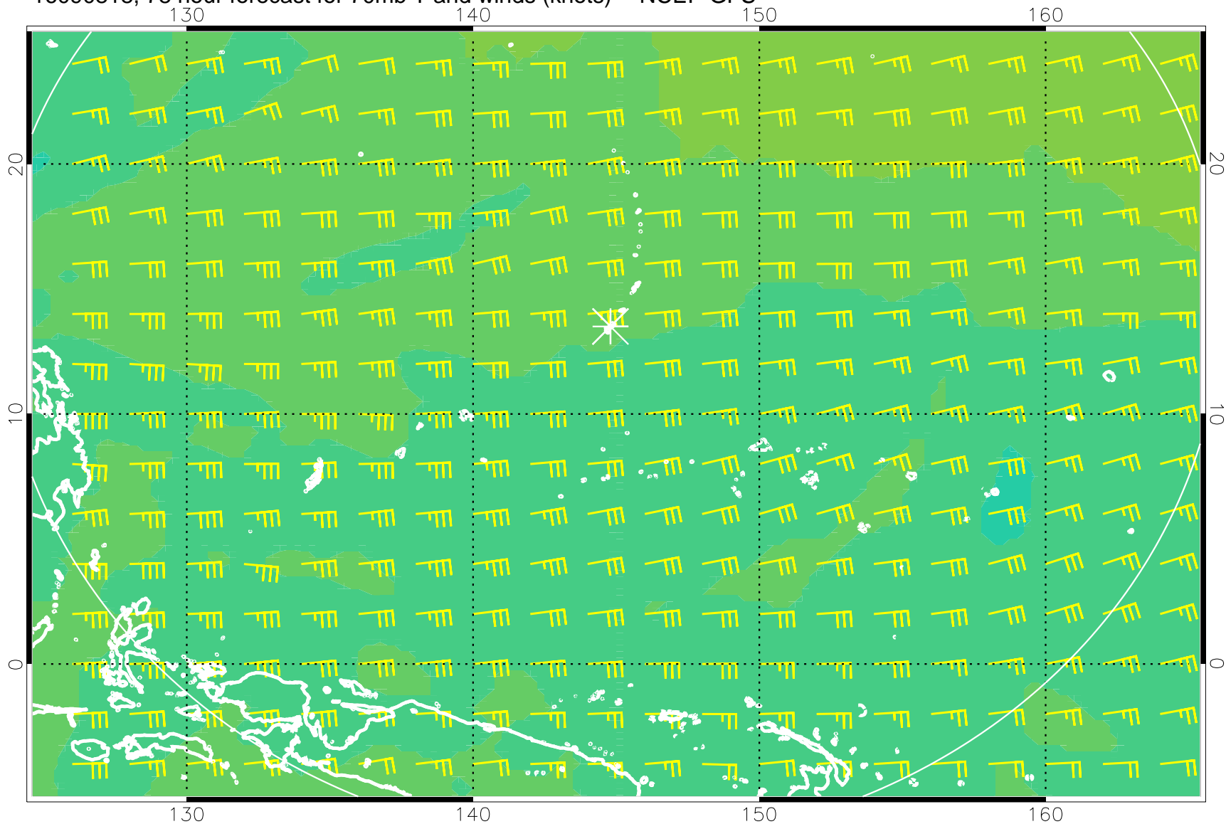
16090818, 78 hour forecast for 70mb T and winds (knots) -- NCEP GFS
