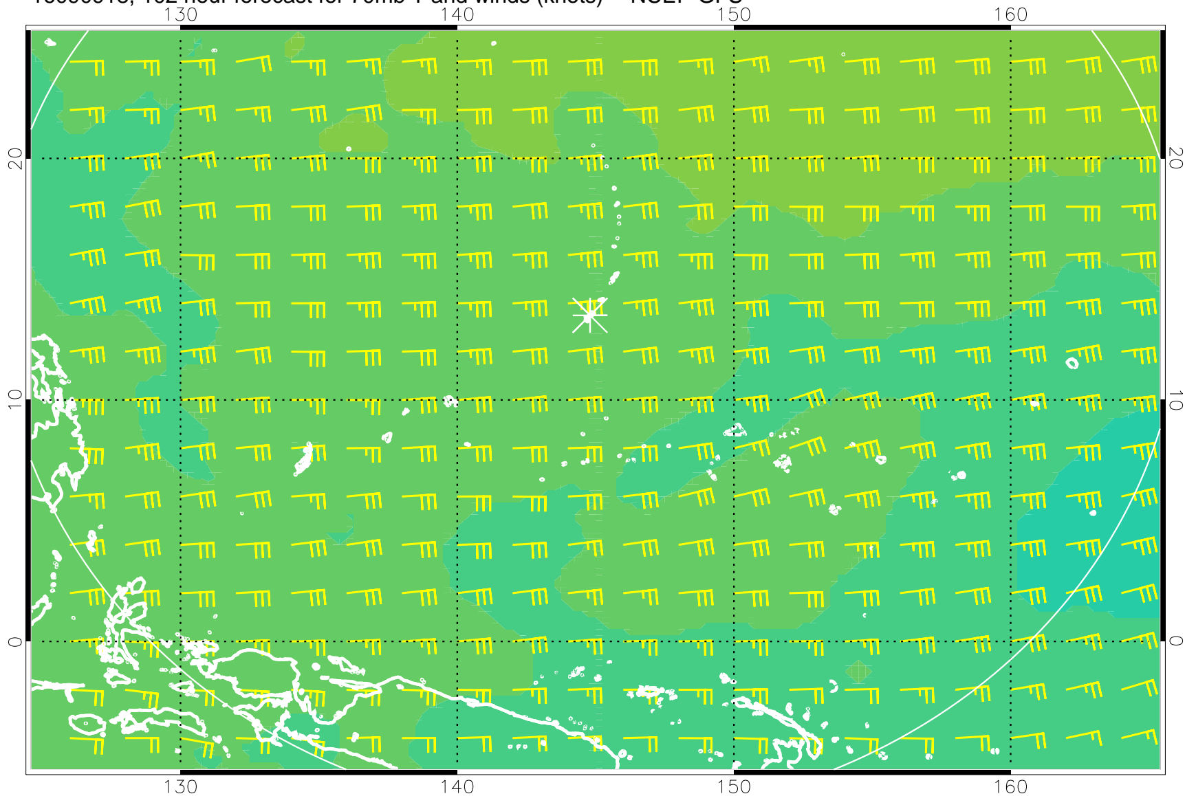
16090918, 102 hour forecast for 70mb T and winds (knots) -- NCEP GFS
