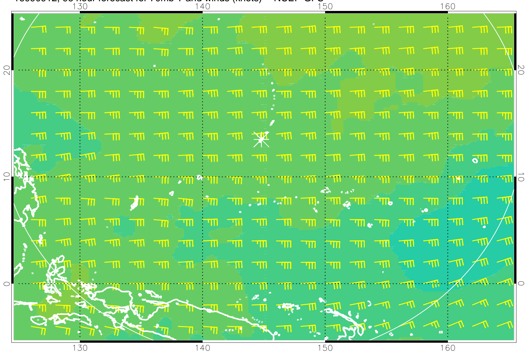
16090912, 96 hour forecast for 70mb T and winds (knots) -- NCEP GFS
