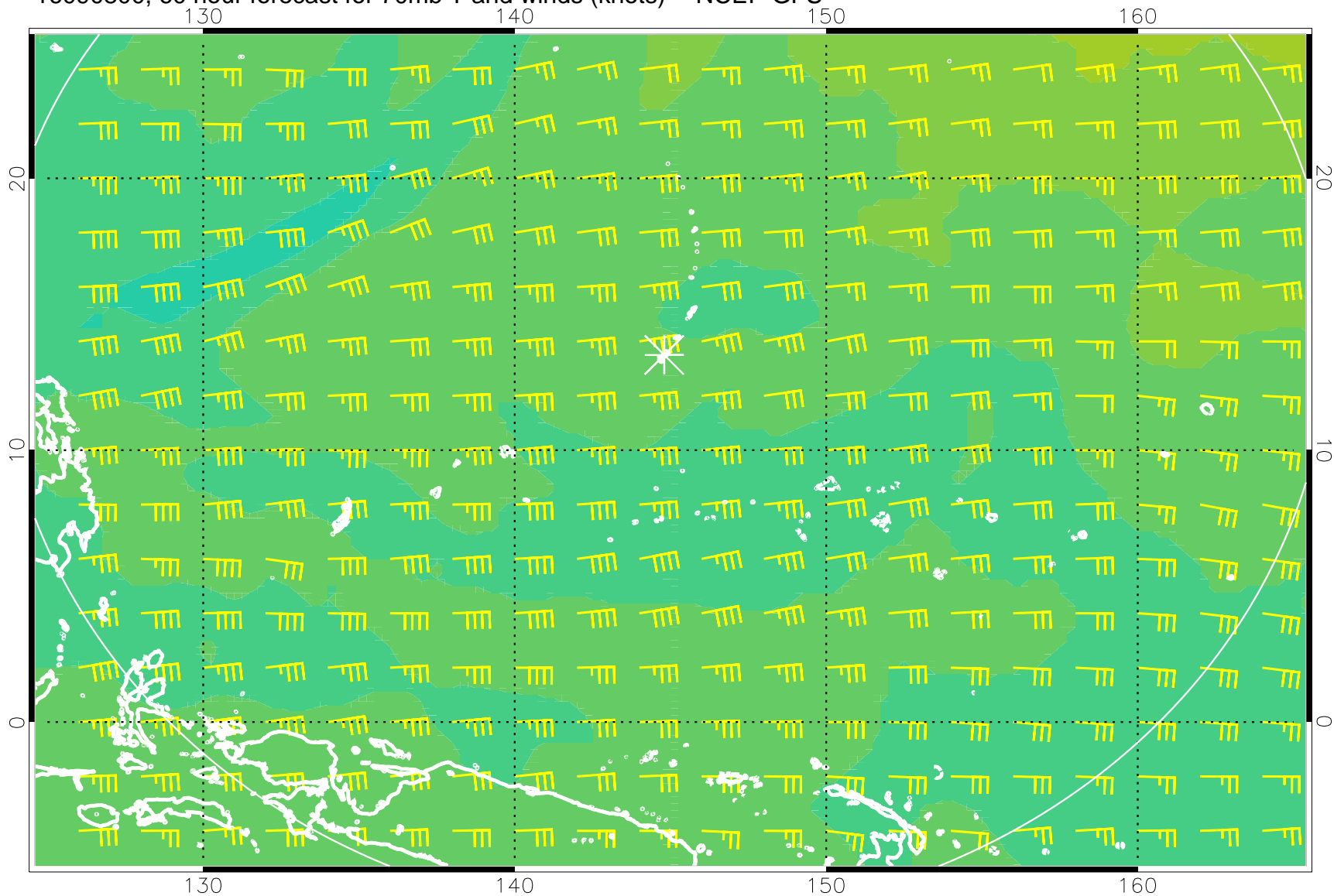
16090800, 60 hour forecast for 70mb T and winds (knots) -- NCEP GFS
