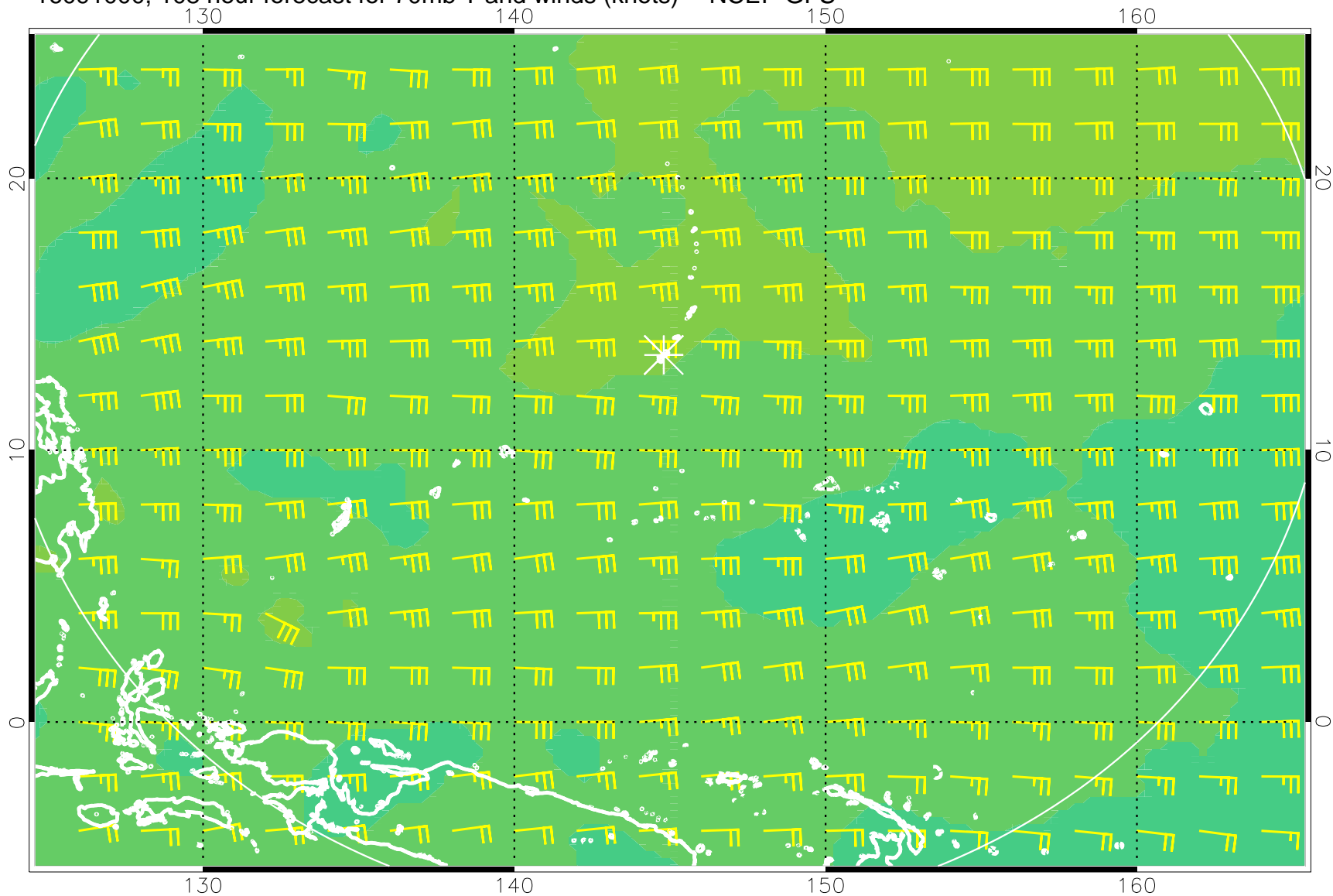
16091000, 108 hour forecast for 70mb T and winds (knots) -- NCEP GFS
