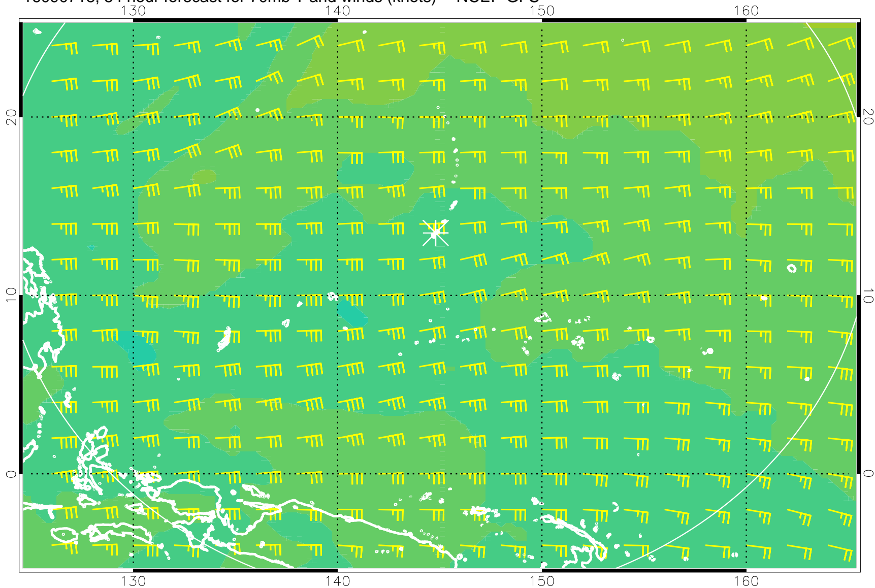
16090718, 54 hour forecast for 70mb T and winds (knots) -- NCEP GFS
