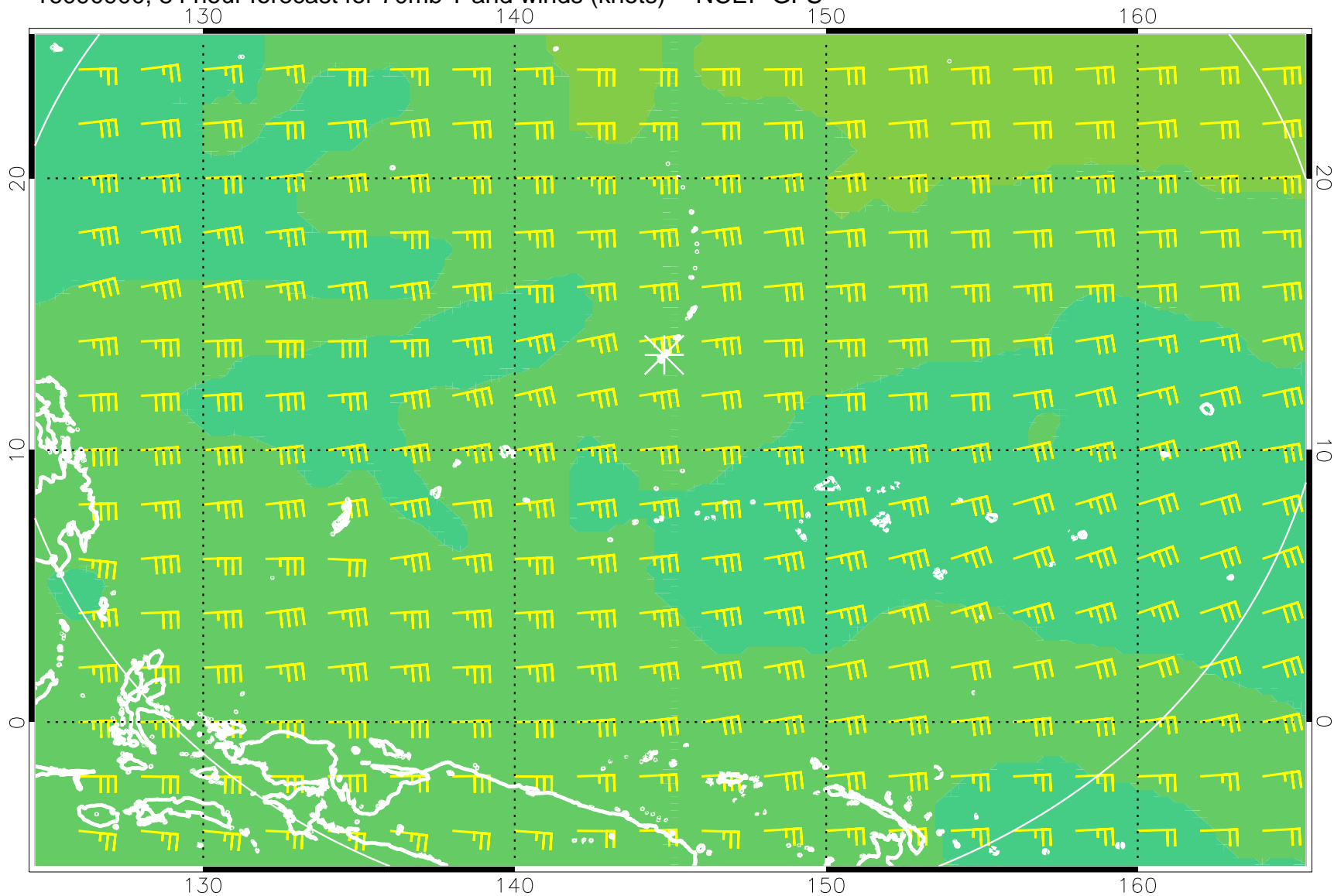
16090900, 84 hour forecast for 70mb T and winds (knots) -- NCEP GFS
