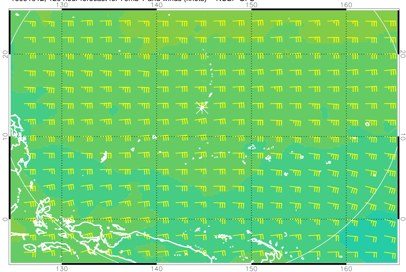
16091012, 120 hour forecast for 70mb T and winds (knots) -- NCEP GFS
