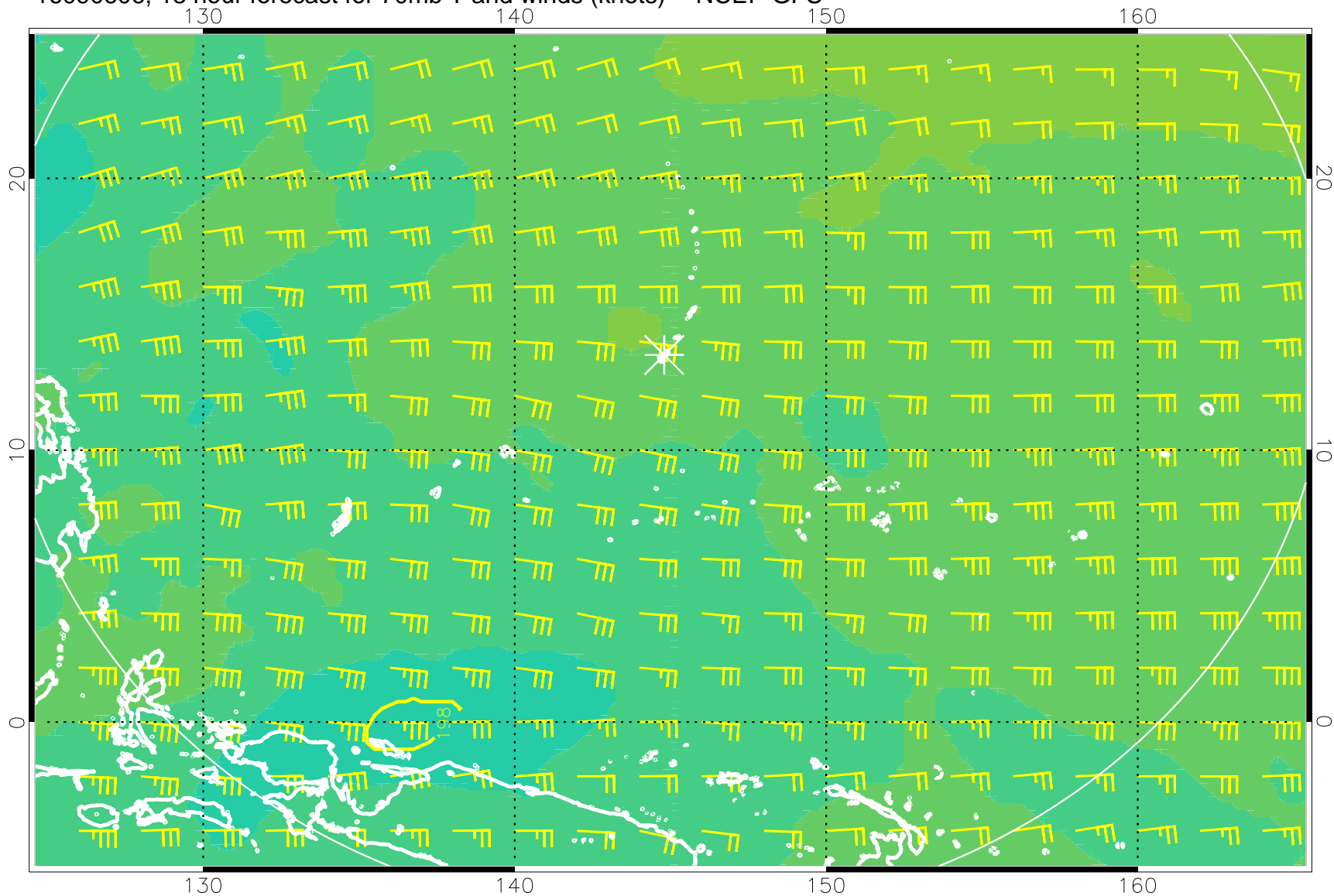
16090606, 18 hour forecast for 70mb T and winds (knots) -- NCEP GFS
