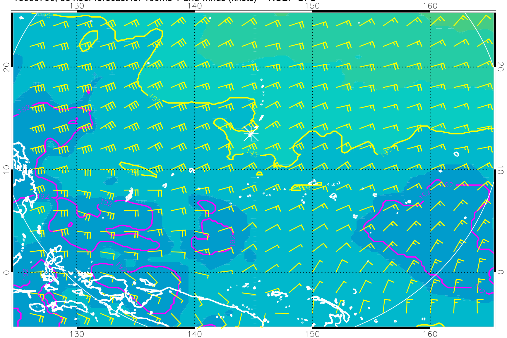
16090700, 36 hour forecast for 100mb T and winds (knots) -- NCEP GFS
