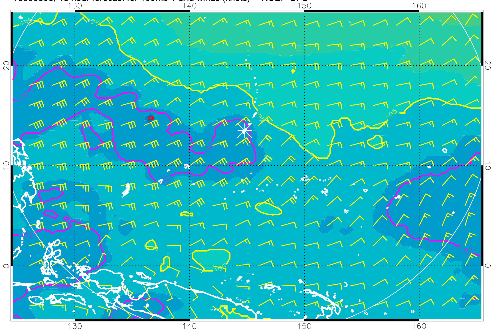
16090606, 18 hour forecast for 100mb T and winds (knots) -- NCEP GFS
