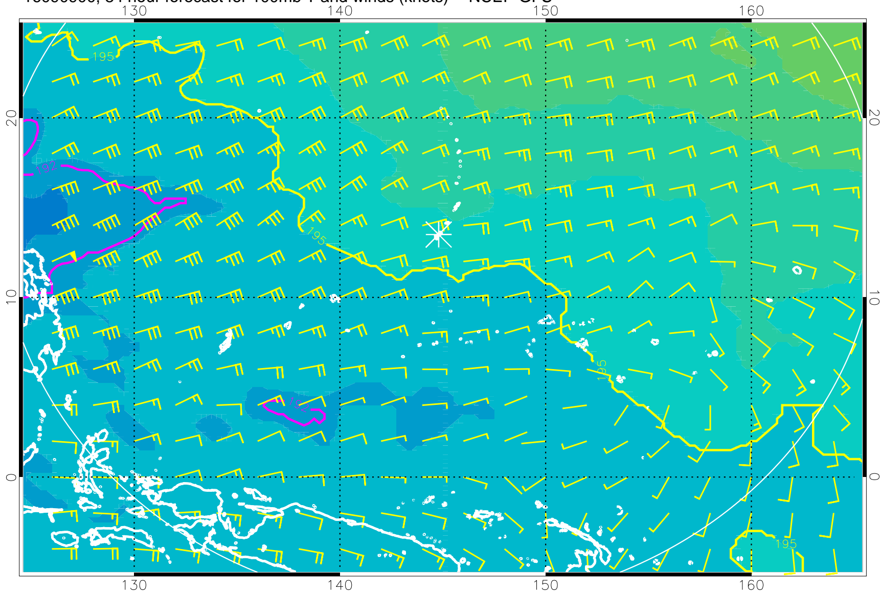
16090900, 84 hour forecast for 100mb T and winds (knots) -- NCEP GFS
