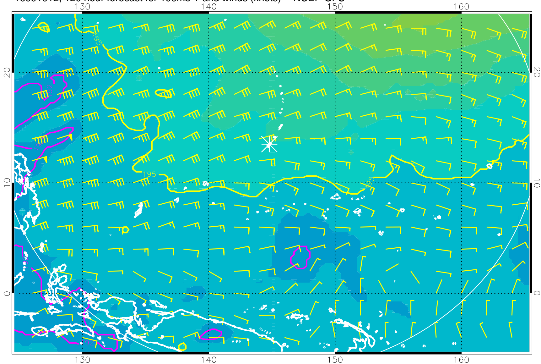
16091012, 120 hour forecast for 100mb T and winds (knots) -- NCEP GFS
