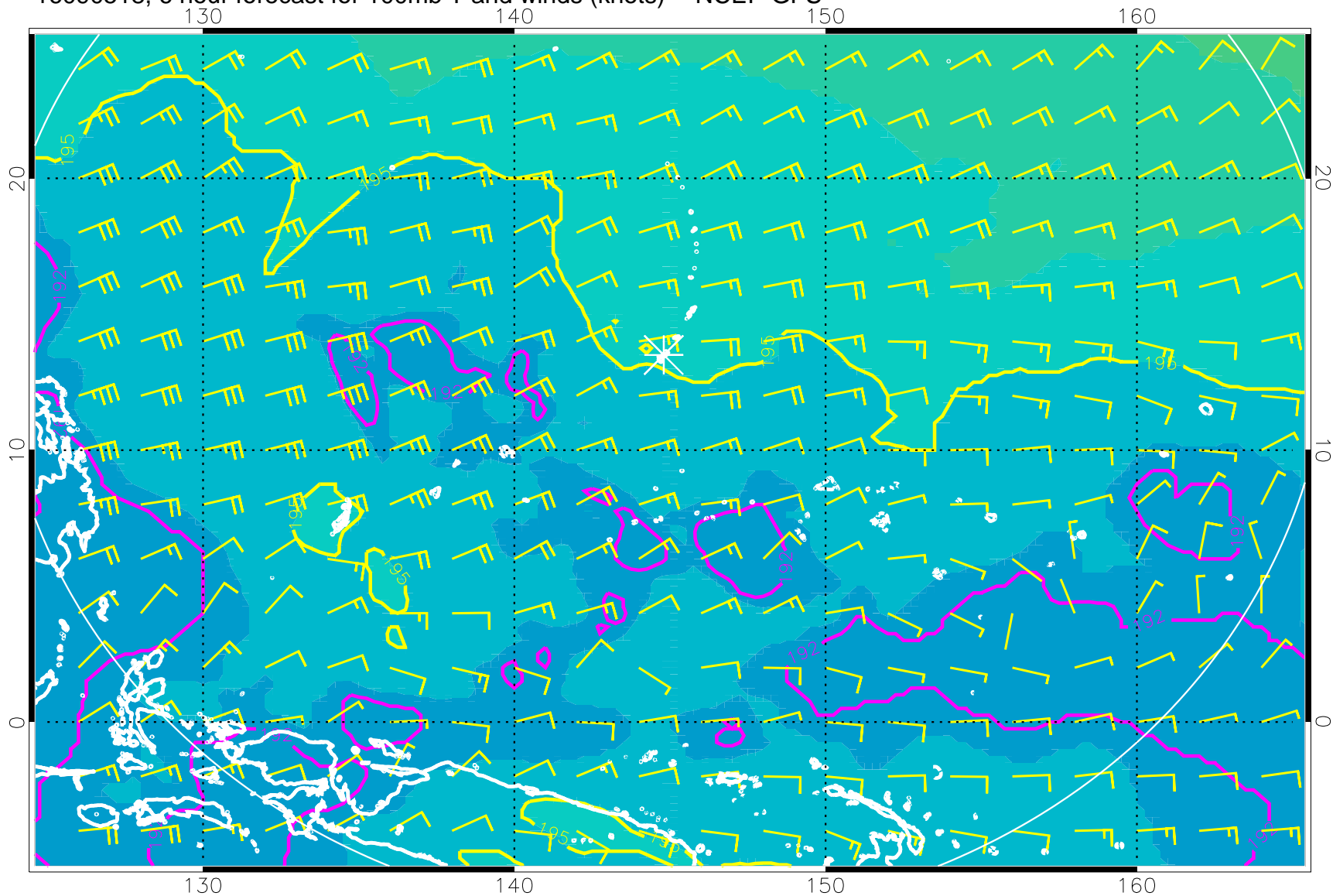
16090518, 6 hour forecast for 100mb T and winds (knots) -- NCEP GFS
