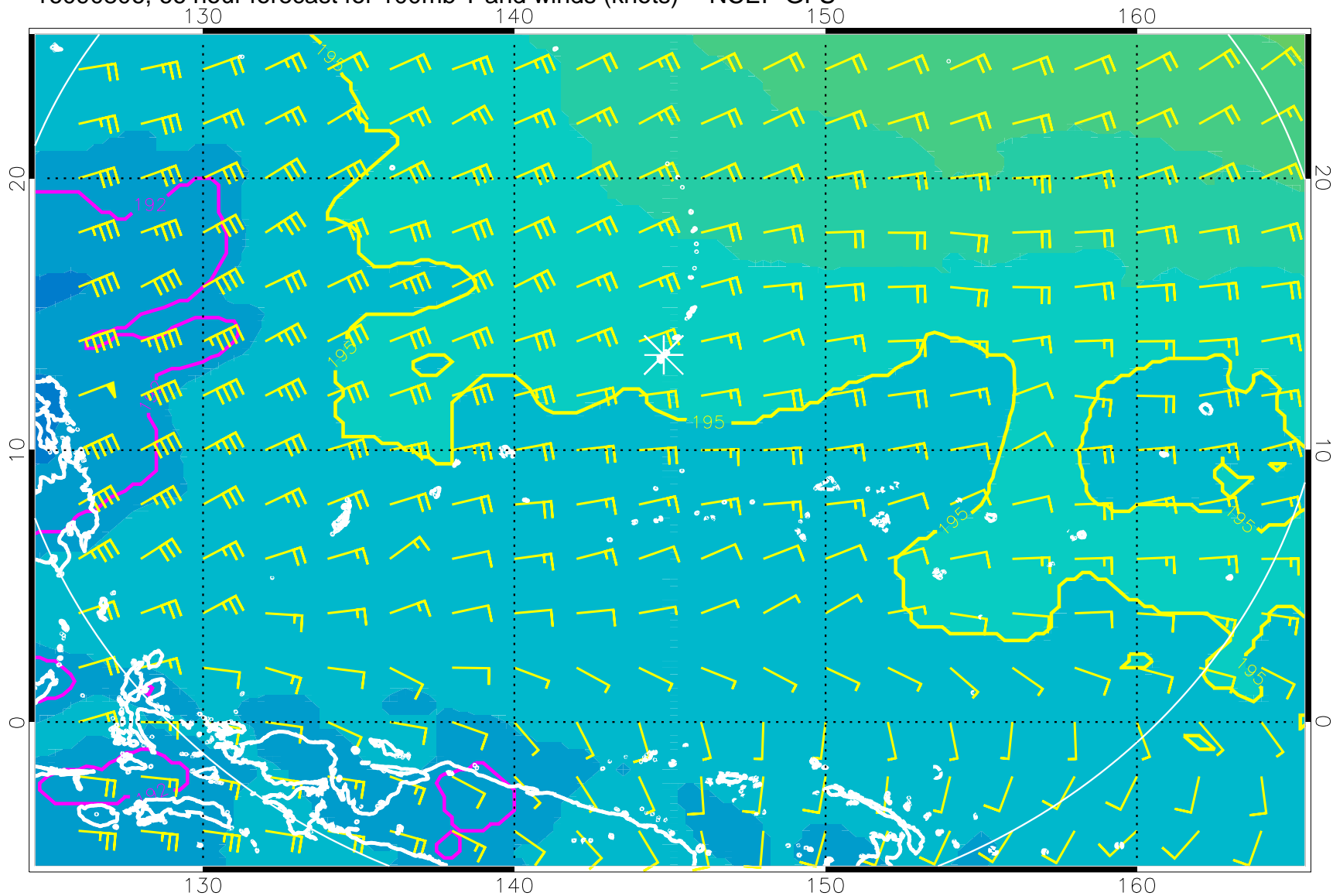
16090806, 66 hour forecast for 100mb T and winds (knots) -- NCEP GFS
