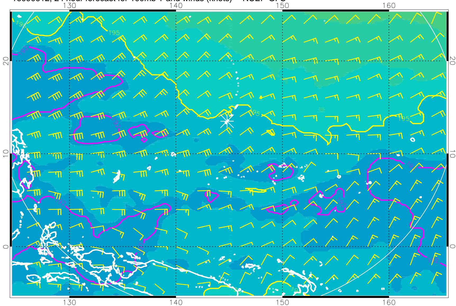
16090612, 24 hour forecast for 100mb T and winds (knots) -- NCEP GFS
