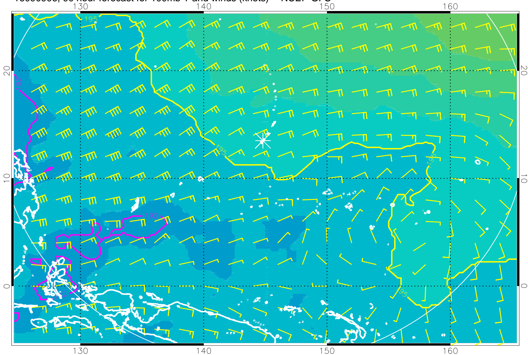
16090906, 90 hour forecast for 100mb T and winds (knots) -- NCEP GFS
