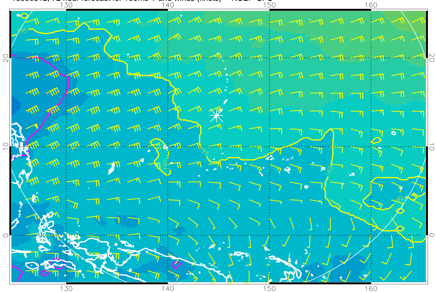
16090812, 72 hour forecast for 100mb T and winds (knots) -- NCEP GFS
