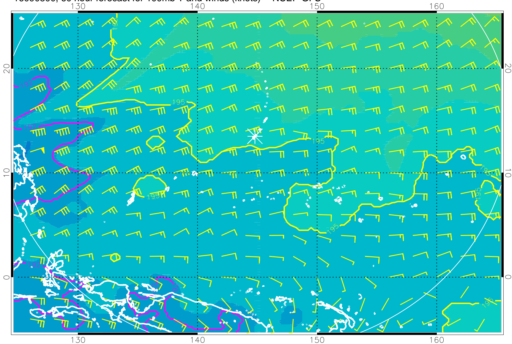
16090800, 60 hour forecast for 100mb T and winds (knots) -- NCEP GFS
