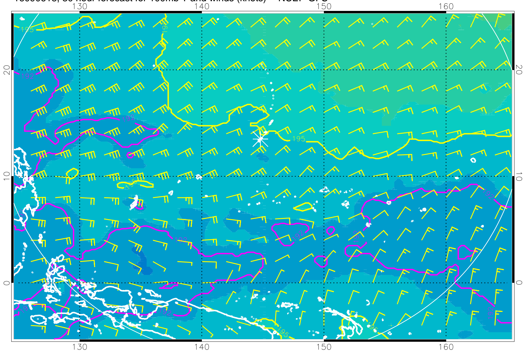
16090618, 30 hour forecast for 100mb T and winds (knots) -- NCEP GFS
