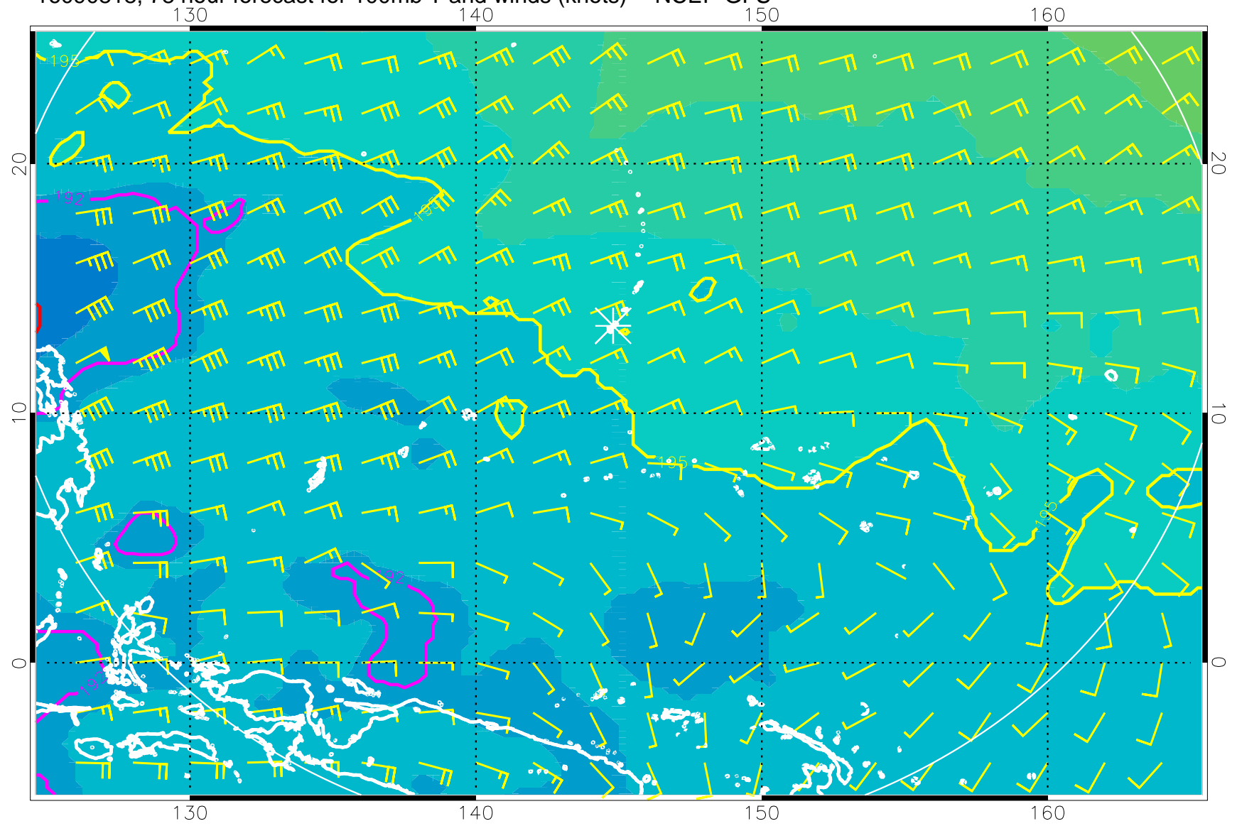
16090818, 78 hour forecast for 100mb T and winds (knots) -- NCEP GFS
