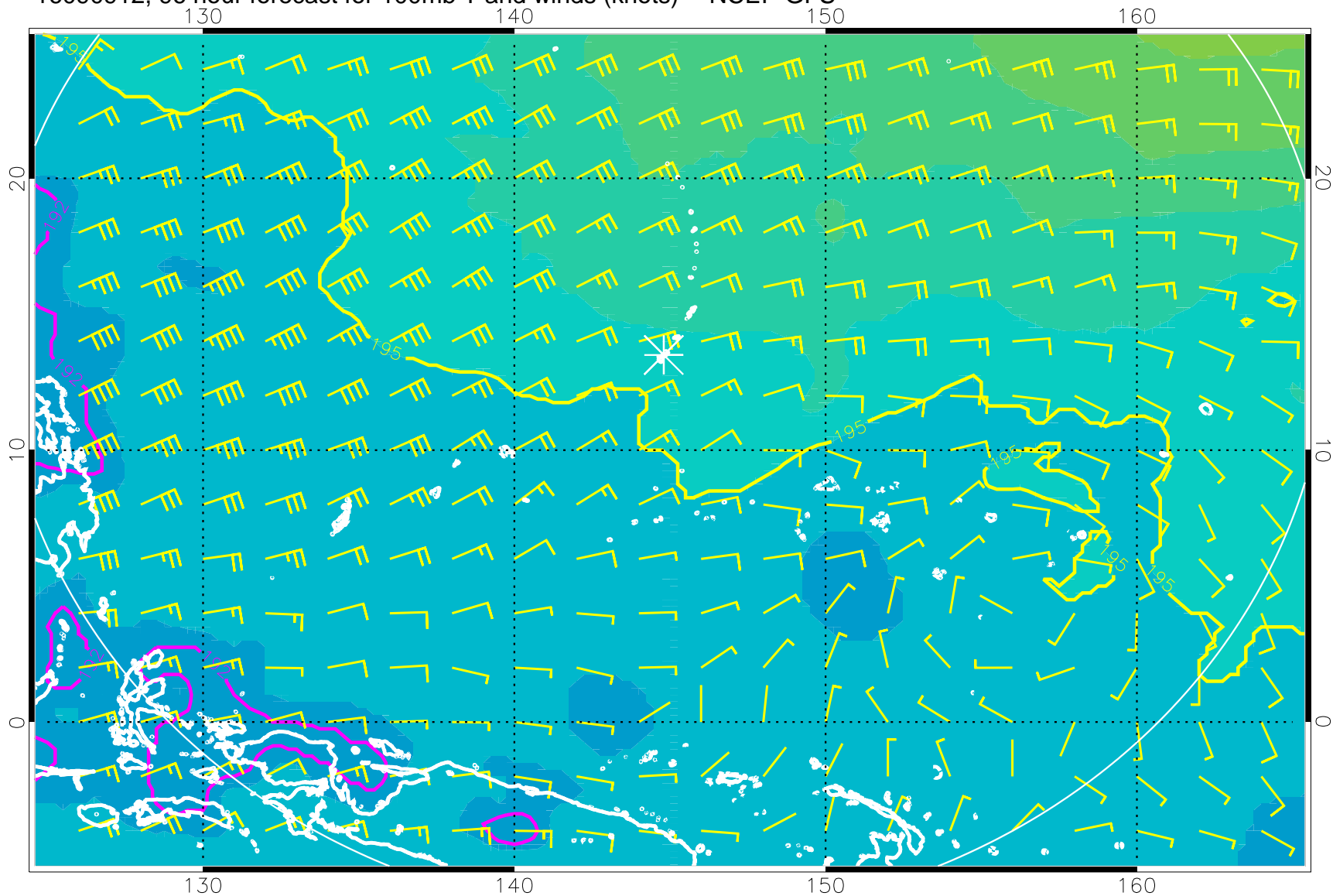
16090912, 96 hour forecast for 100mb T and winds (knots) -- NCEP GFS
