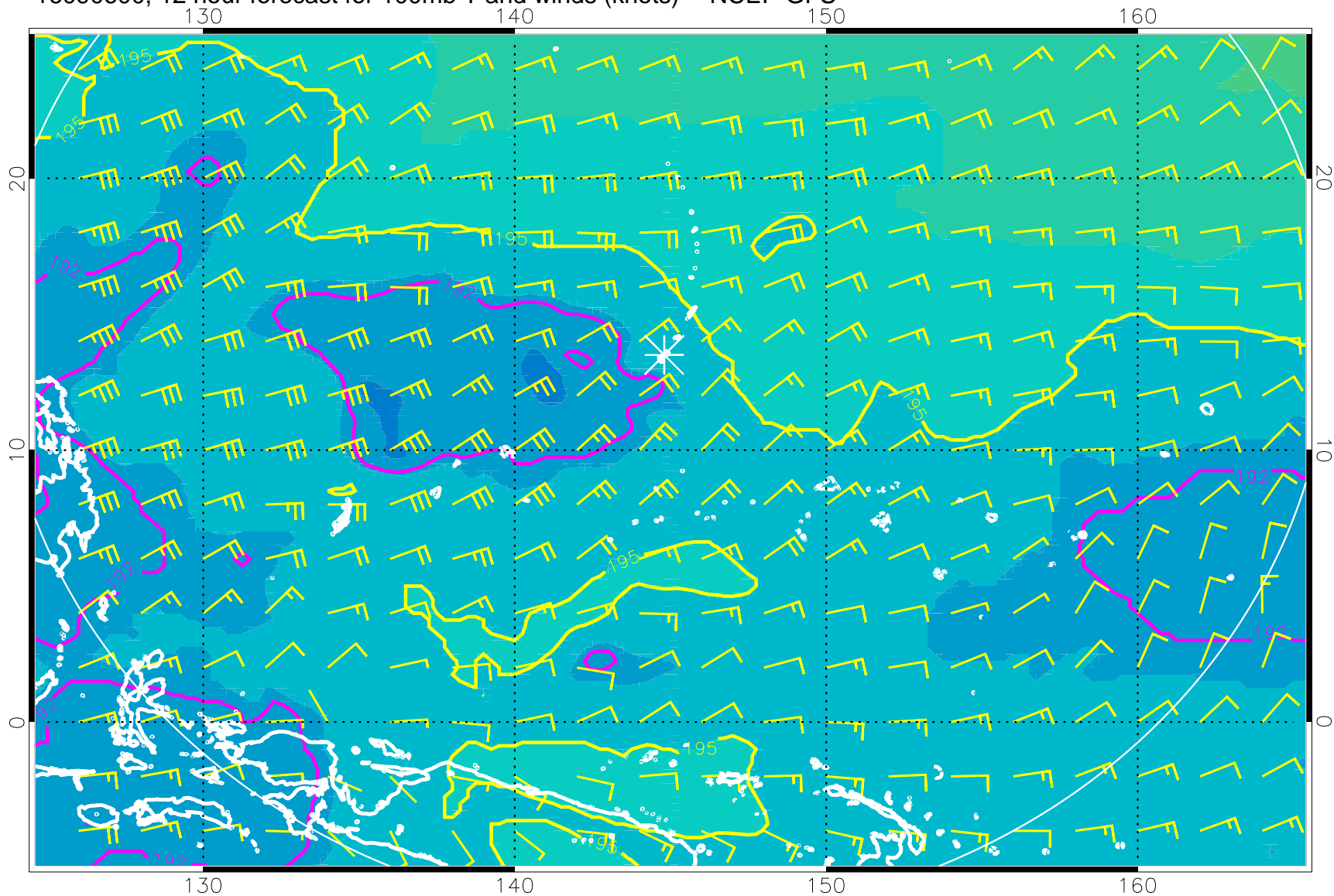
16090600, 12 hour forecast for 100mb T and winds (knots) -- NCEP GFS
