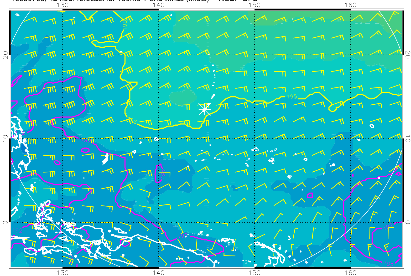
16090706, 42 hour forecast for 100mb T and winds (knots) -- NCEP GFS
