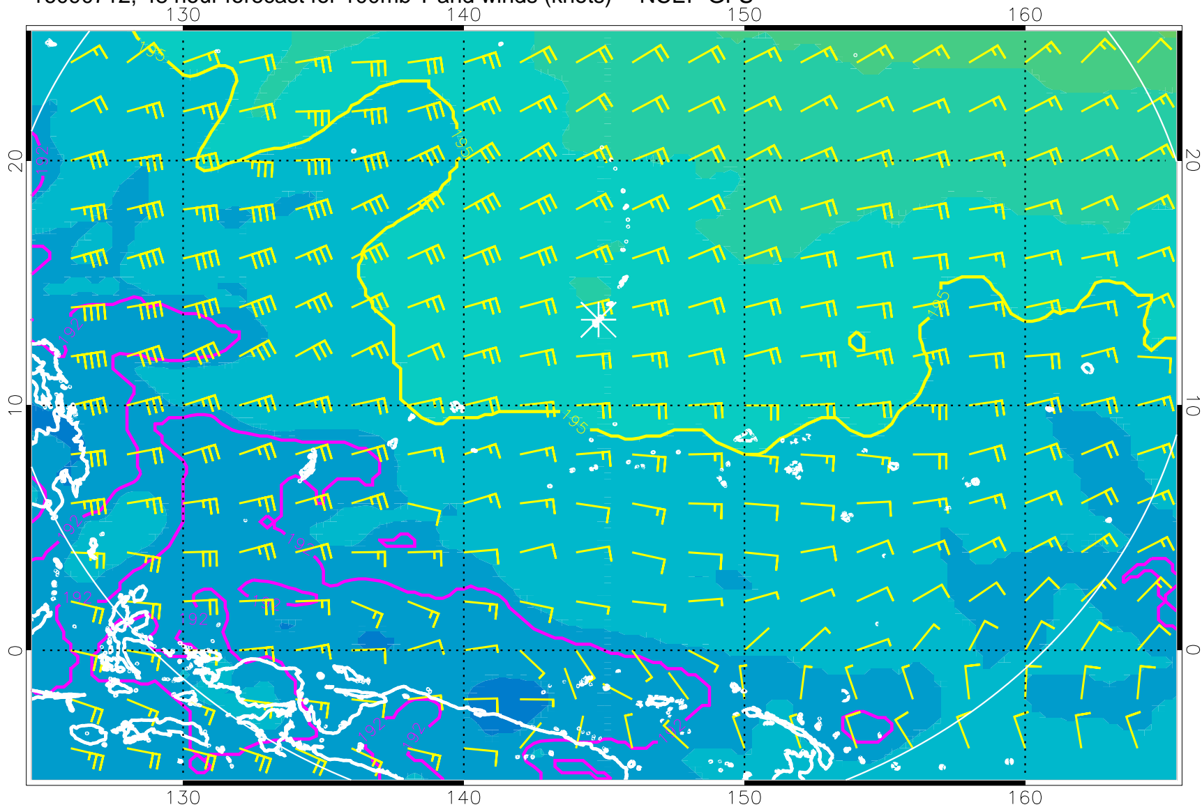
16090712, 48 hour forecast for 100mb T and winds (knots) -- NCEP GFS
