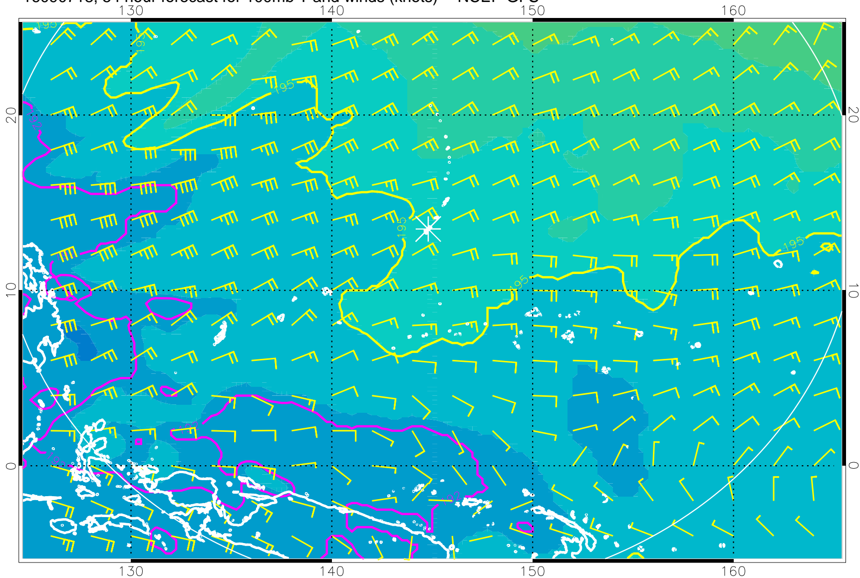
16090718, 54 hour forecast for 100mb T and winds (knots) -- NCEP GFS
