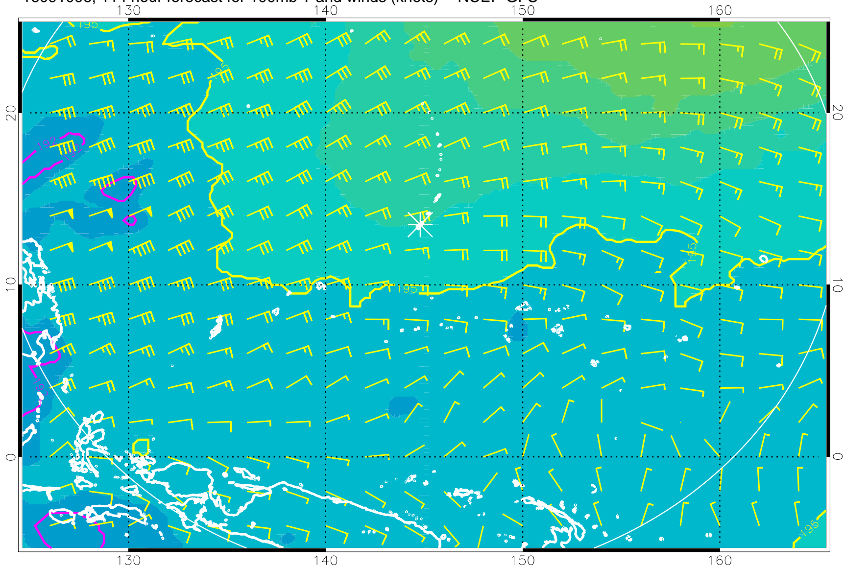
16091006, 114 hour forecast for 100mb T and winds (knots) -- NCEP GFS
