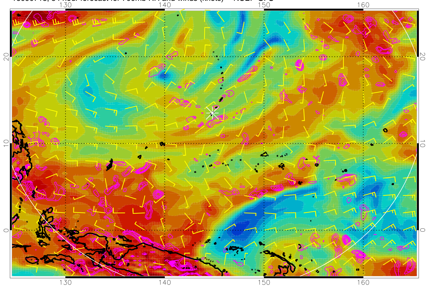
16090718, 54 hour forecast for 700mb RH and winds (knots) -- NCEP GFS
