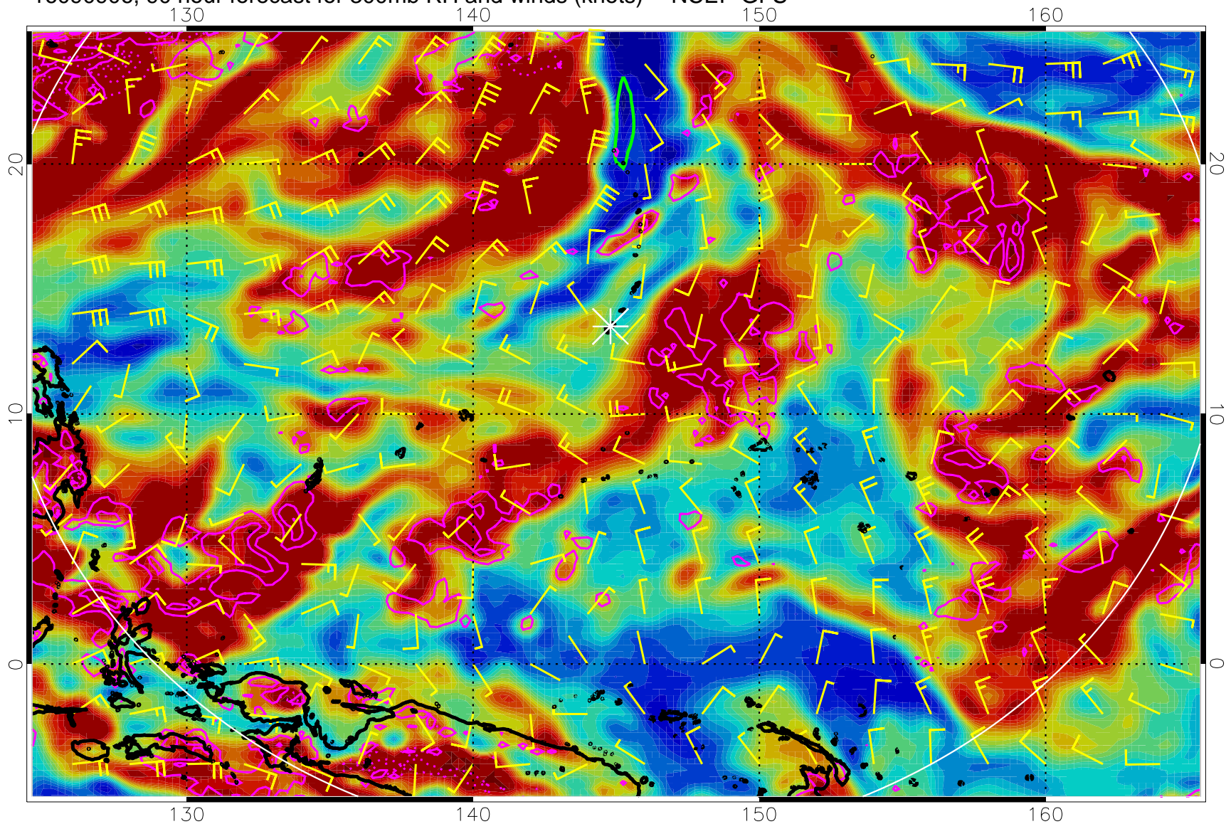
16090906, 90 hour forecast for 300mb RH and winds (knots) -- NCEP GFS
