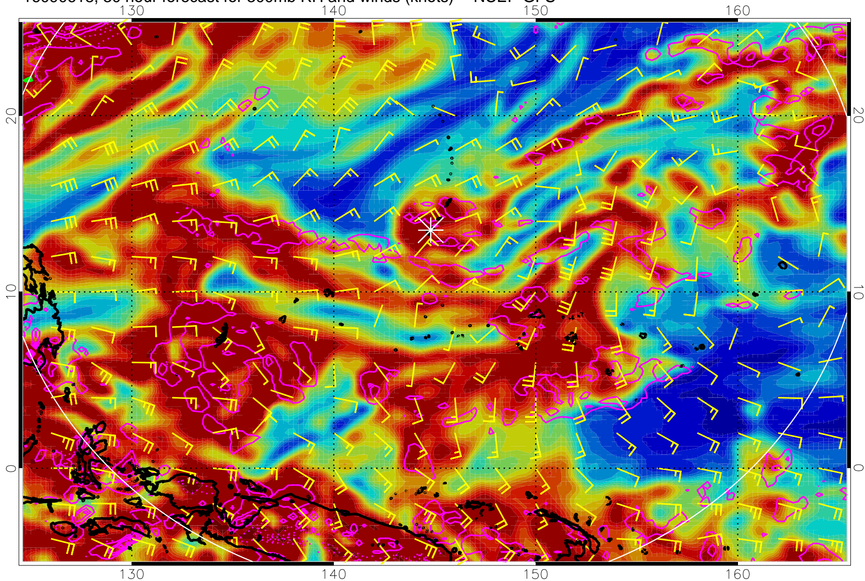
16090618, 30 hour forecast for 300mb RH and winds (knots) -- NCEP GFS
