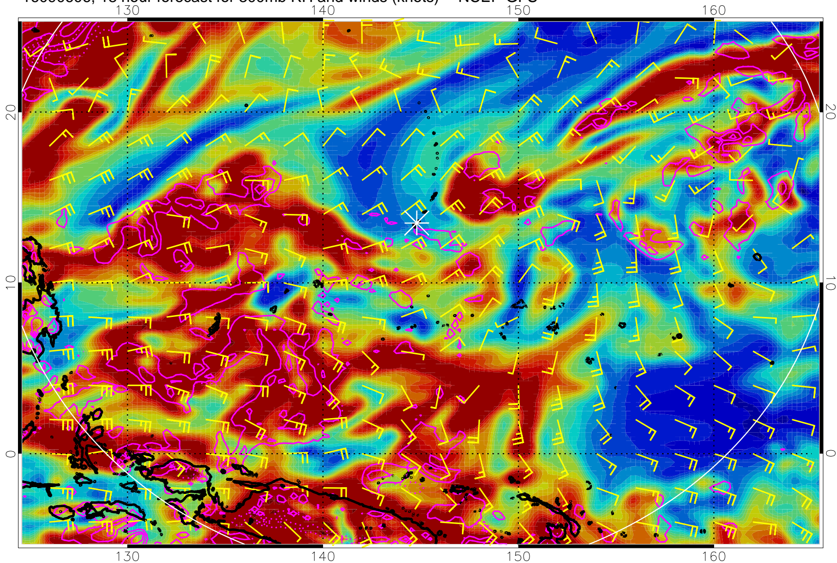
16090606, 18 hour forecast for 300mb RH and winds (knots) -- NCEP GFS
