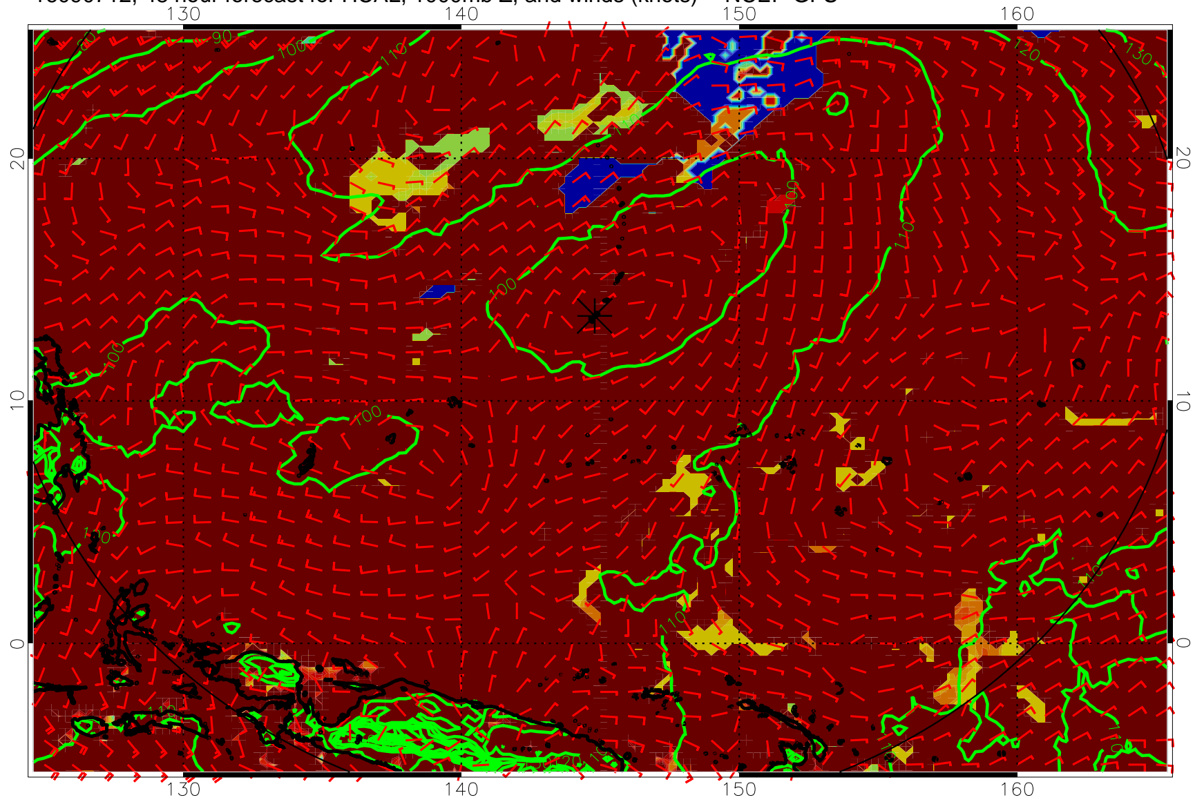
16090712, 48 hour forecast for HCAL, 1000mb Z, and winds (knots) -- NCEP GFS
