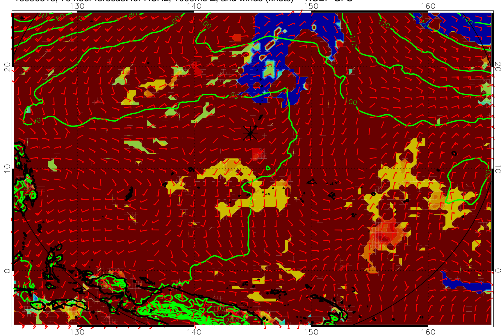
16090818, 78 hour forecast for HCAL, 1000mb Z, and winds (knots) -- NCEP GFS
