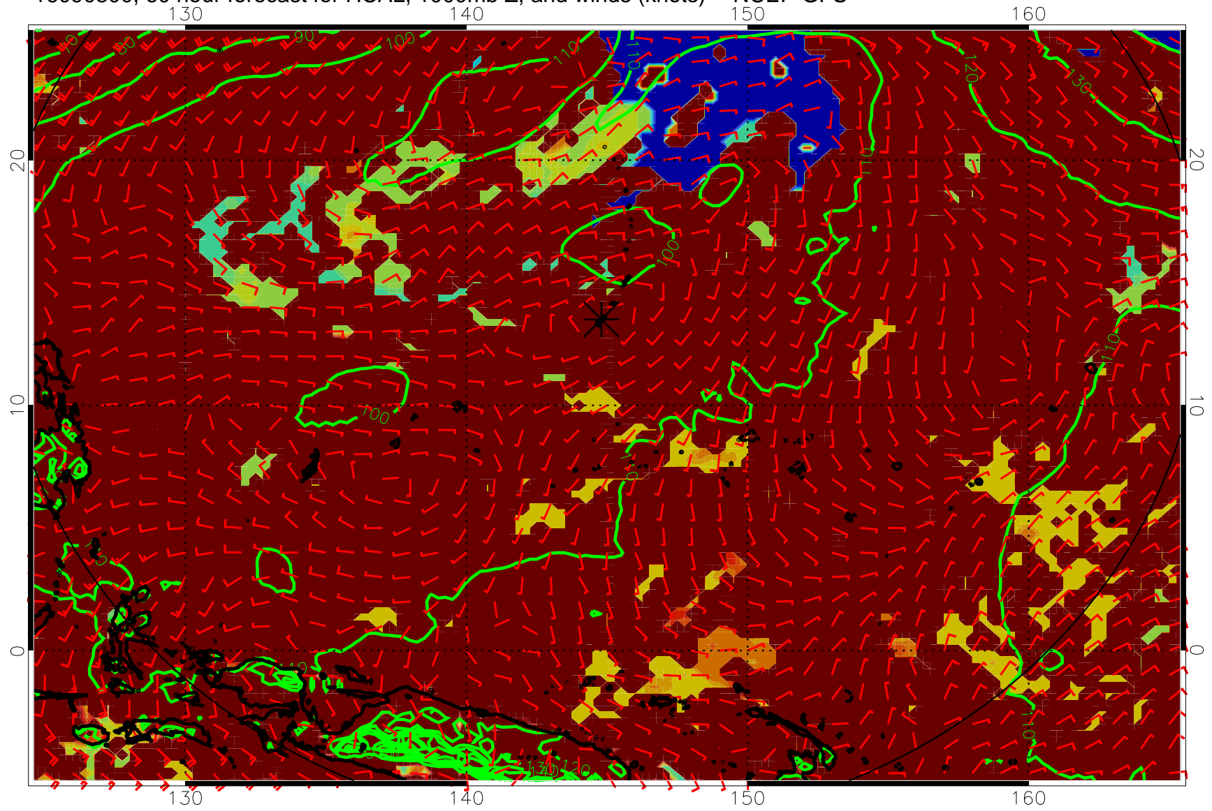
16090800, 60 hour forecast for HCAL, 1000mb Z, and winds (knots) -- NCEP GFS
