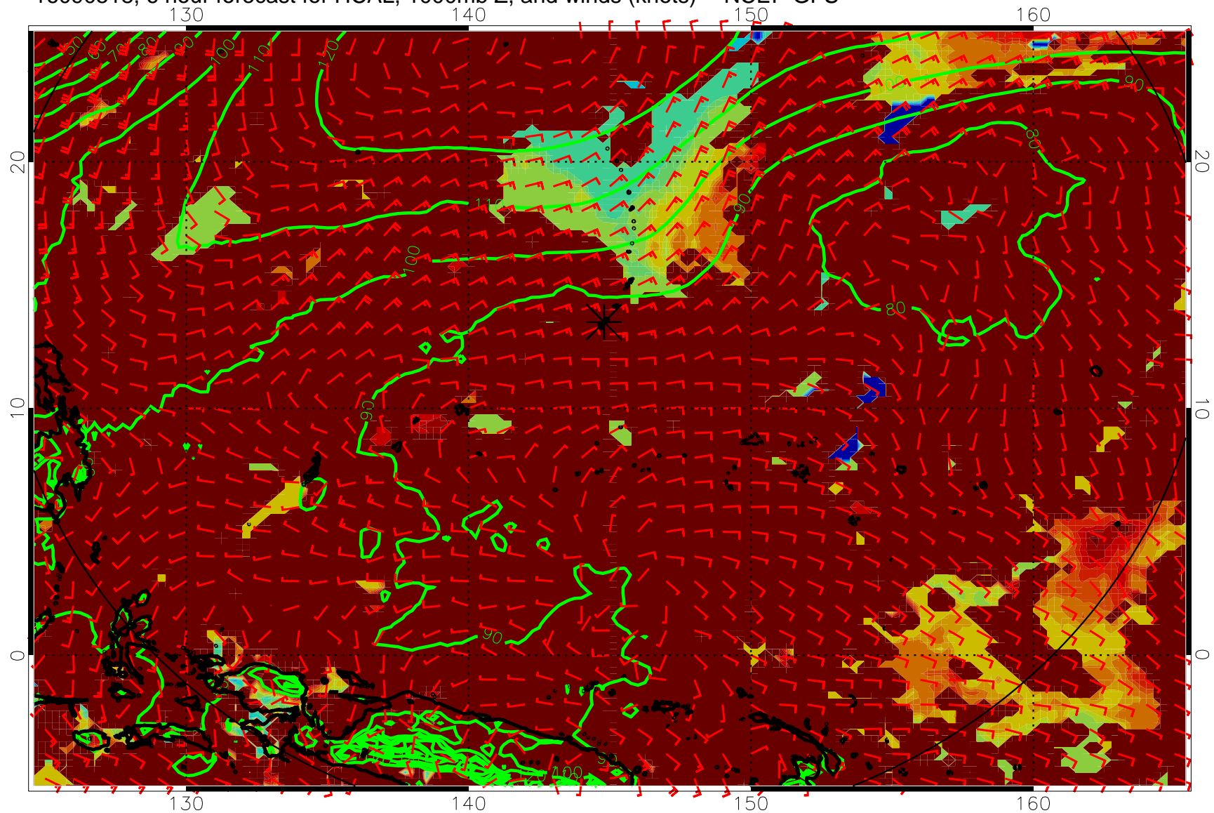
16090518, 6 hour forecast for HCAL, 1000mb Z, and winds (knots) -- NCEP GFS
