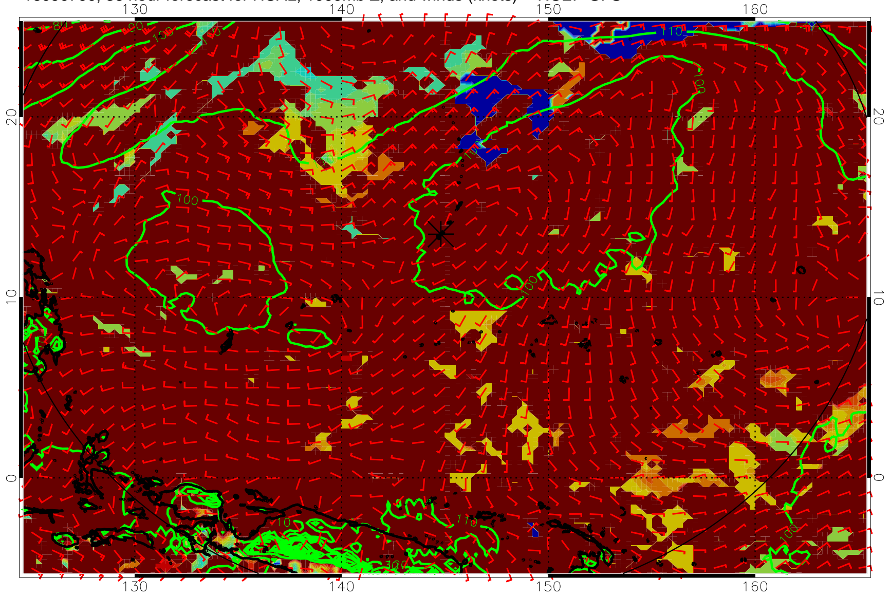
16090700, 36 hour forecast for HCAL, 1000mb Z, and winds (knots) -- NCEP GFS
