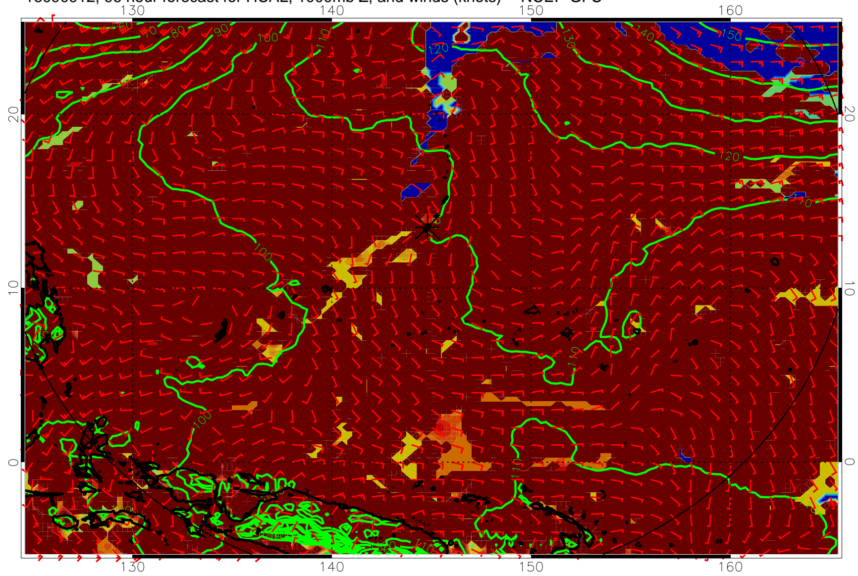
16090912, 96 hour forecast for HCAL, 1000mb Z, and winds (knots) -- NCEP GFS
