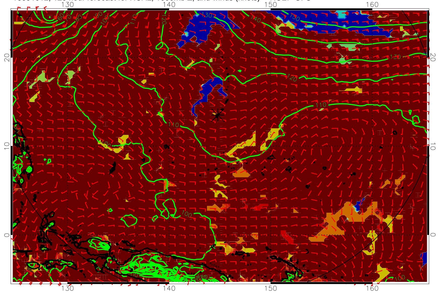
16091012, 120 hour forecast for HCAL, 1000mb Z, and winds (knots) -- NCEP GFS
