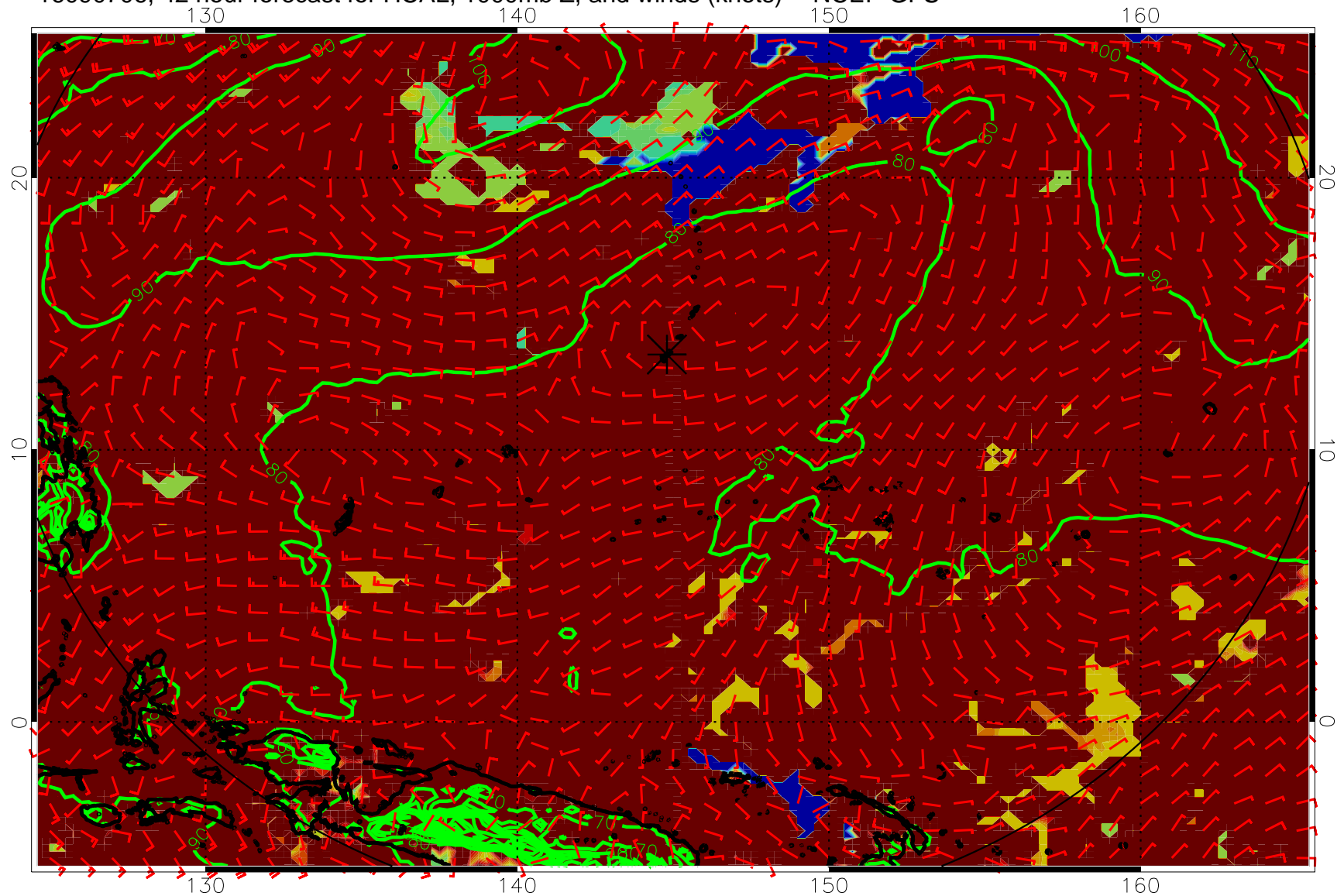
16090706, 42 hour forecast for HCAL, 1000mb Z, and winds (knots) -- NCEP GFS
