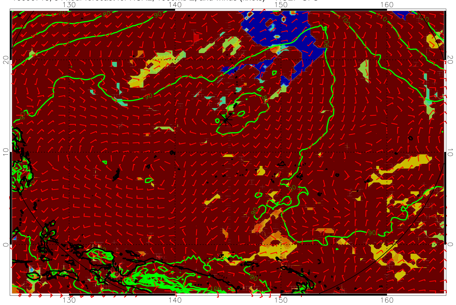
16090718, 54 hour forecast for HCAL, 1000mb Z, and winds (knots) -- NCEP GFS
