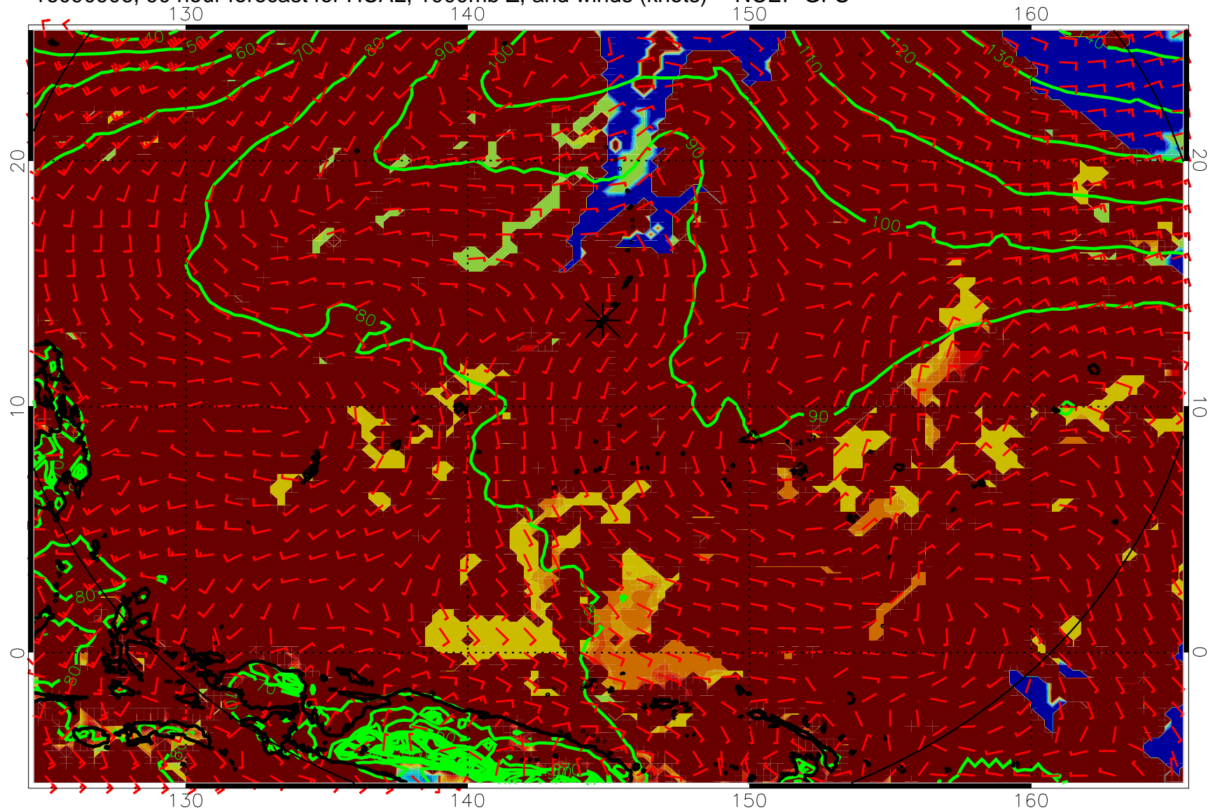
16090906, 90 hour forecast for HCAL, 1000mb Z, and winds (knots) -- NCEP GFS
