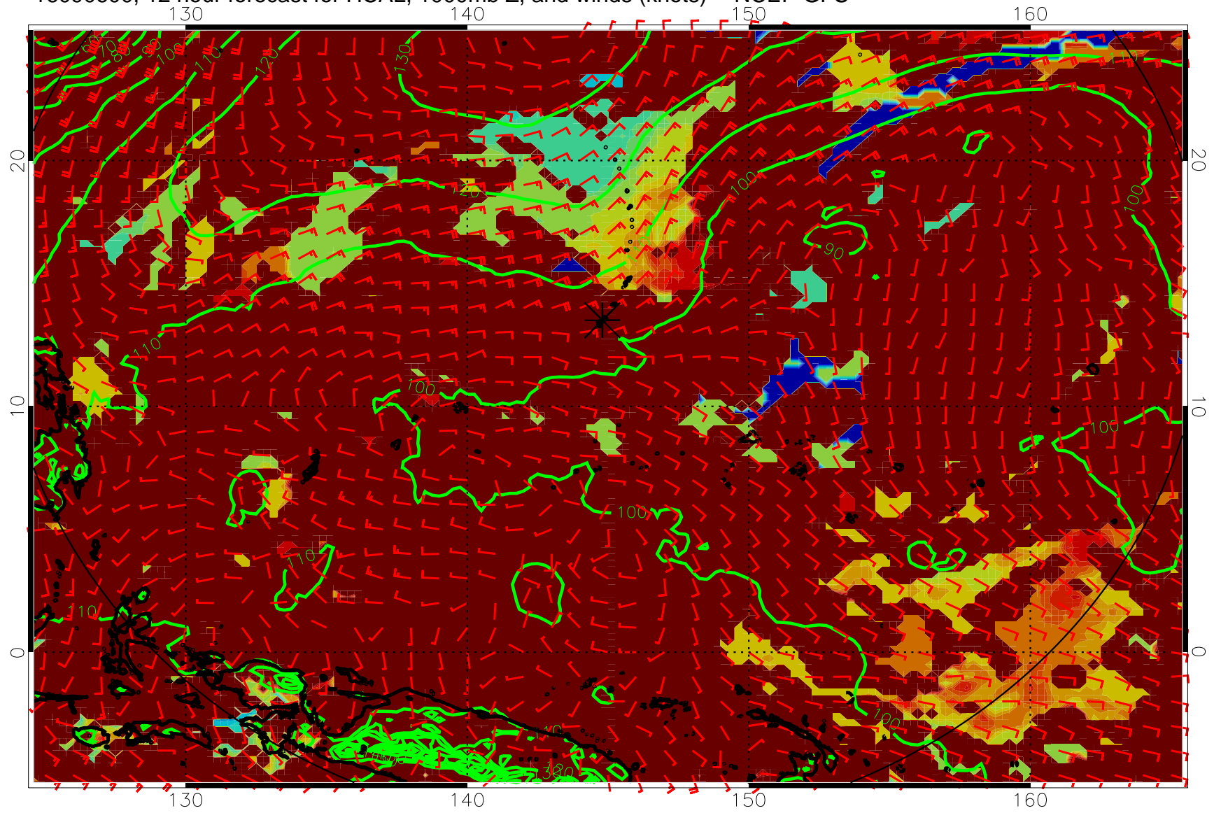
16090600, 12 hour forecast for HCAL, 1000mb Z, and winds (knots) -- NCEP GFS
