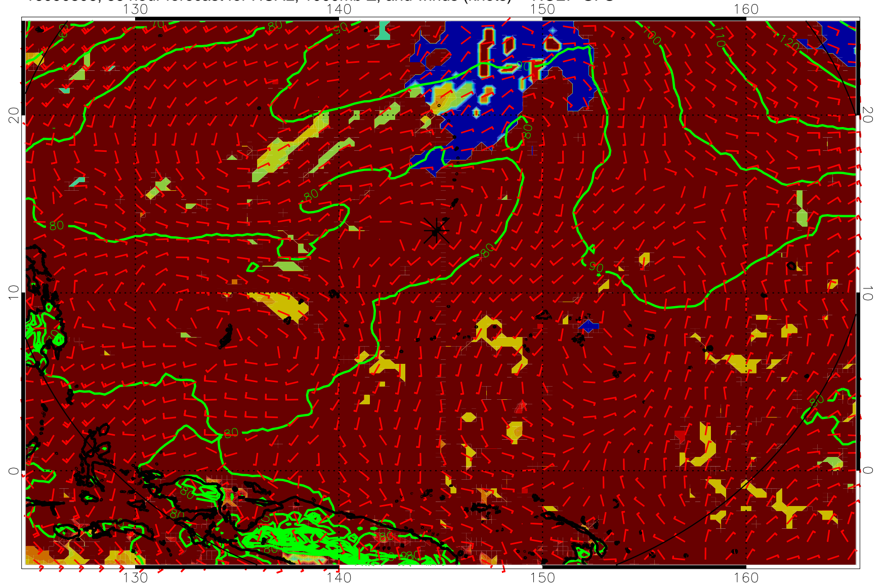
16090806, 66 hour forecast for HCAL, 1000mb Z, and winds (knots) -- NCEP GFS
