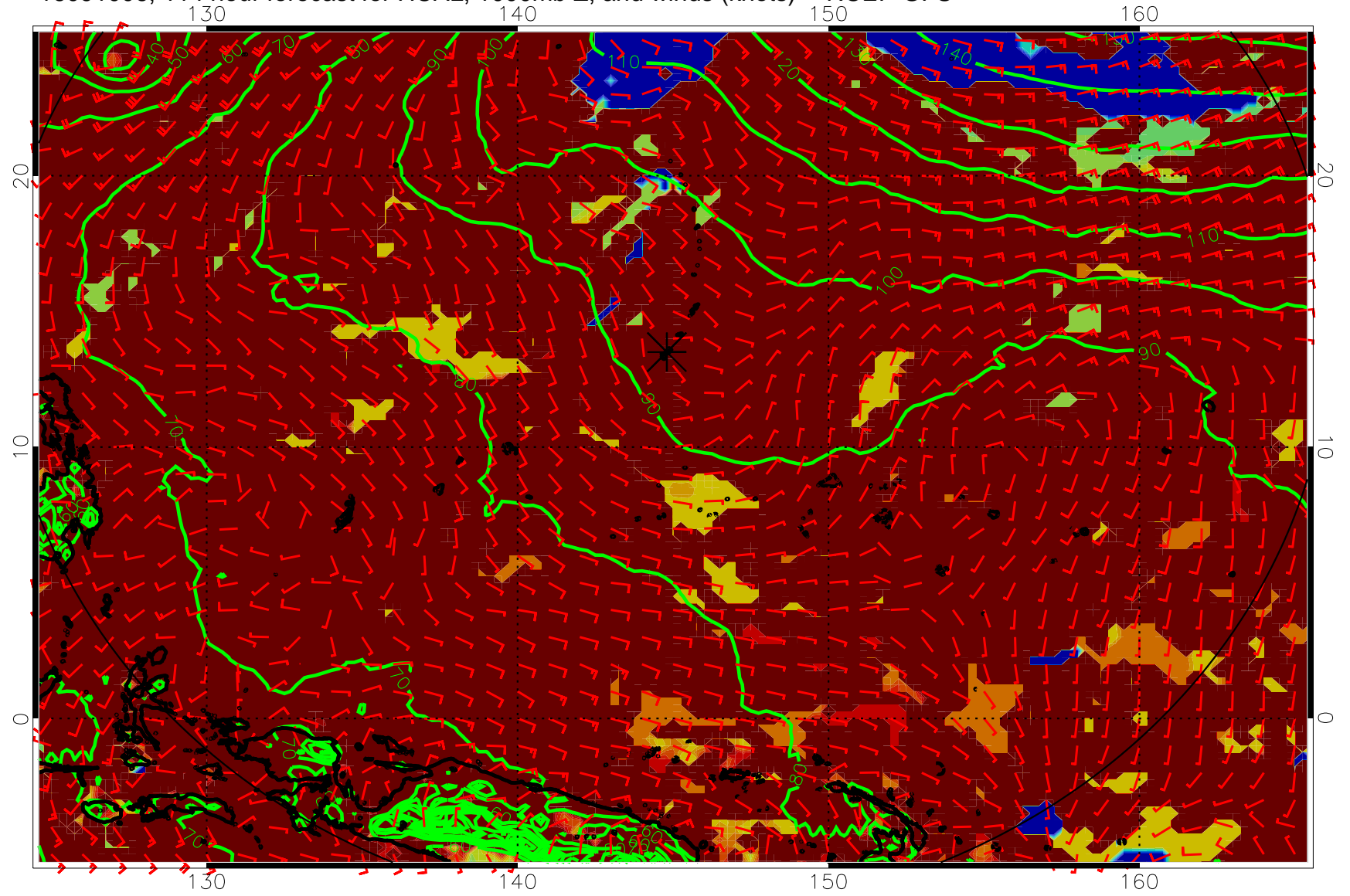
16091006, 114 hour forecast for HCAL, 1000mb Z, and winds (knots) -- NCEP GFS
