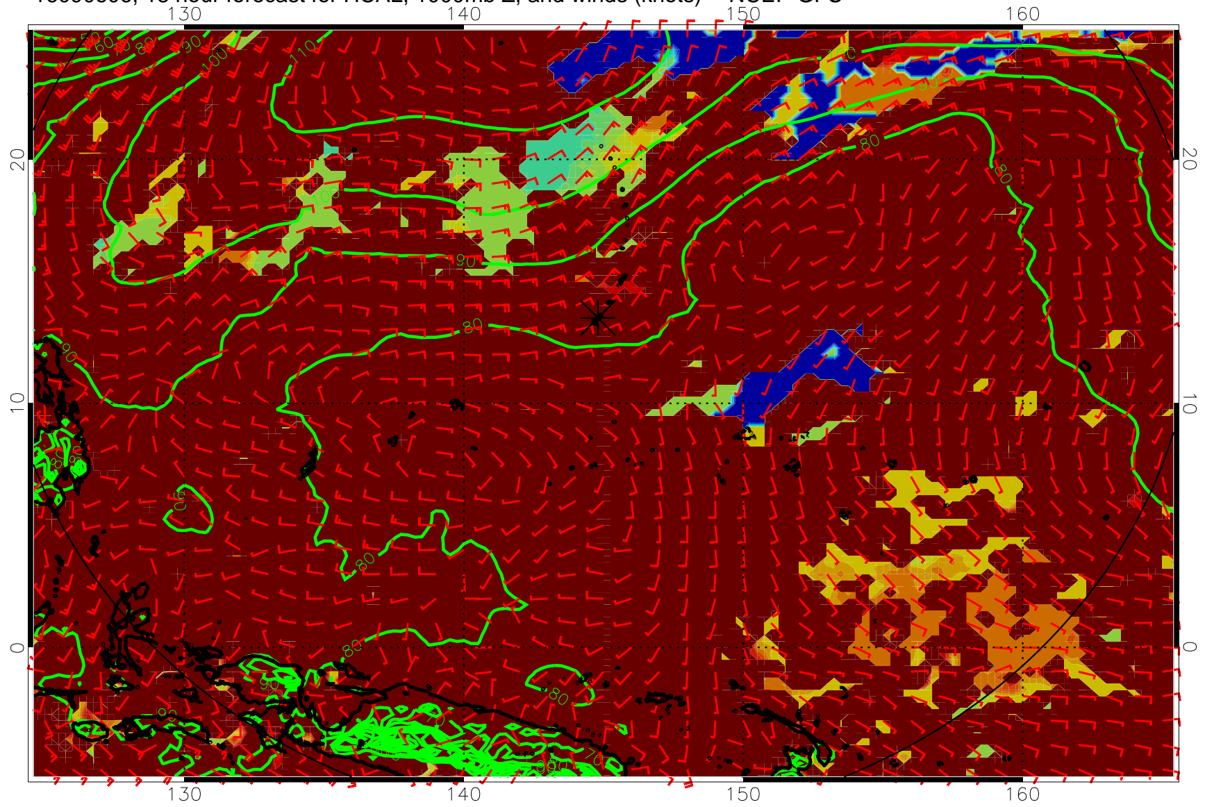
16090606, 18 hour forecast for HCAL, 1000mb Z, and winds (knots) -- NCEP GFS
