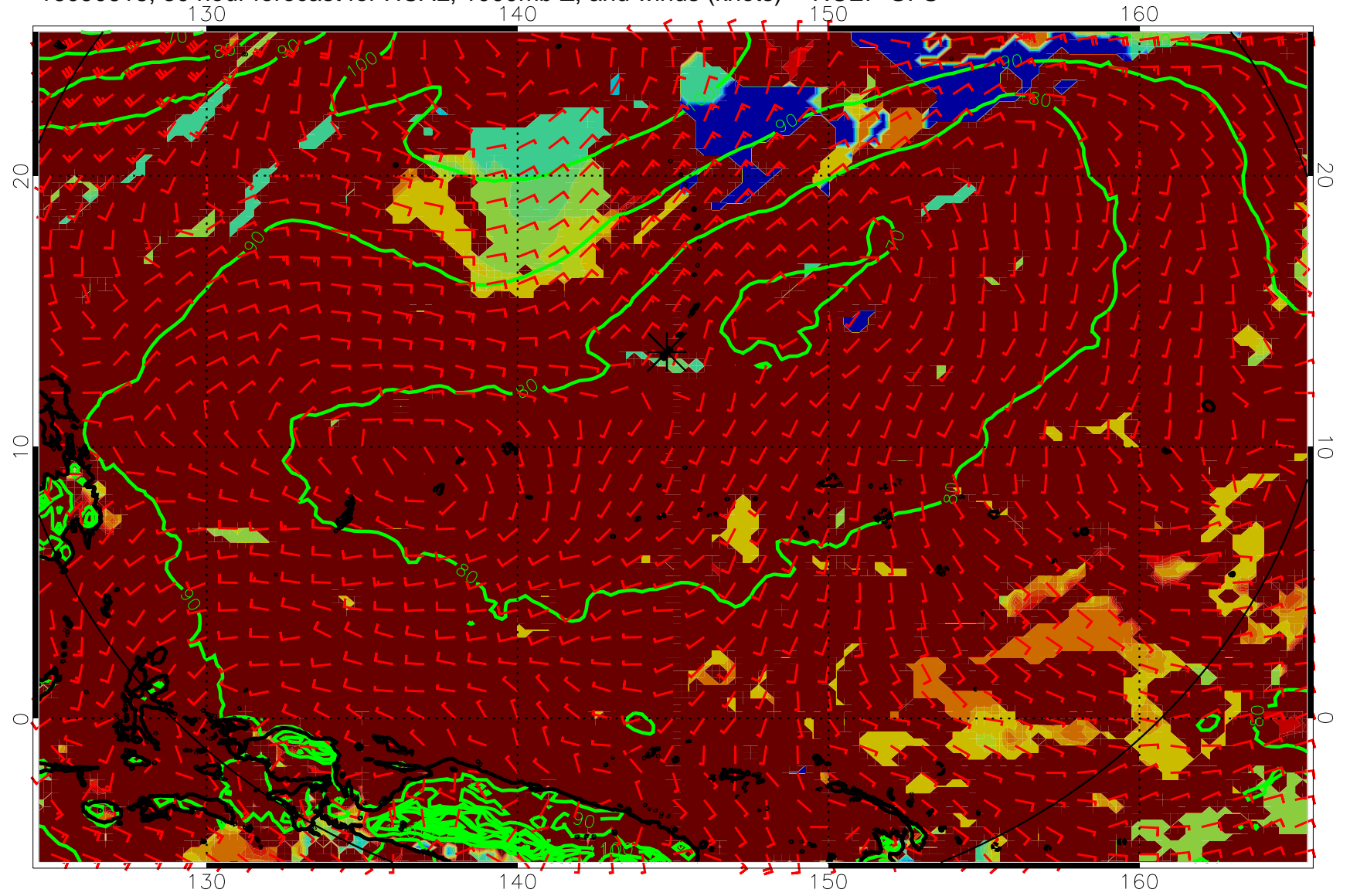
16090618, 30 hour forecast for HCAL, 1000mb Z, and winds (knots) -- NCEP GFS
