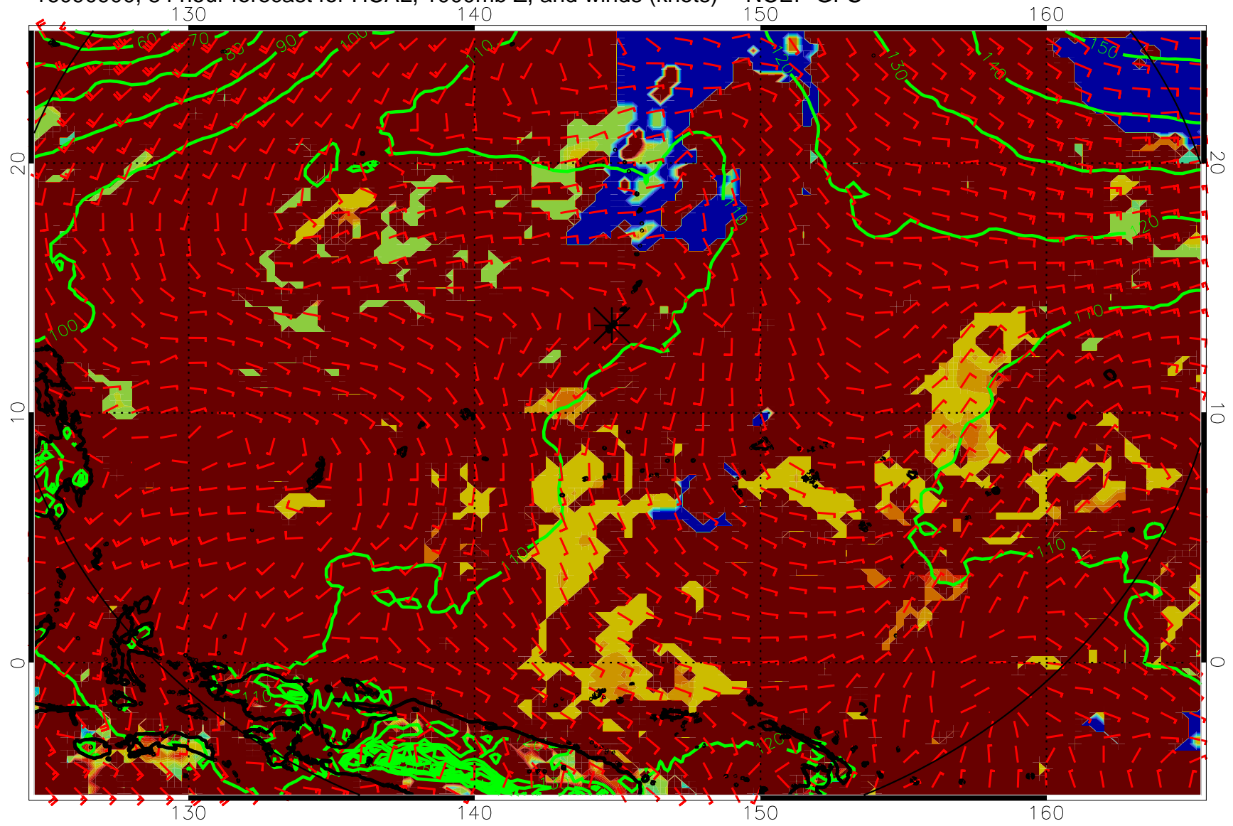
16090900, 84 hour forecast for HCAL, 1000mb Z, and winds (knots) -- NCEP GFS
