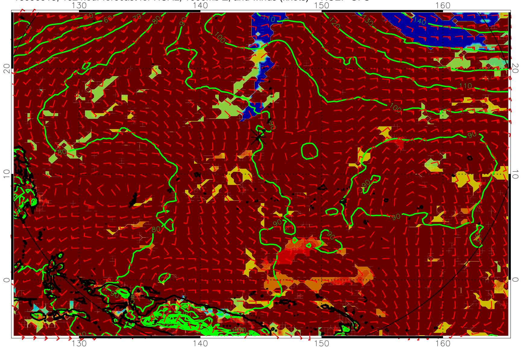
16090918, 102 hour forecast for HCAL, 1000mb Z, and winds (knots) -- NCEP GFS
