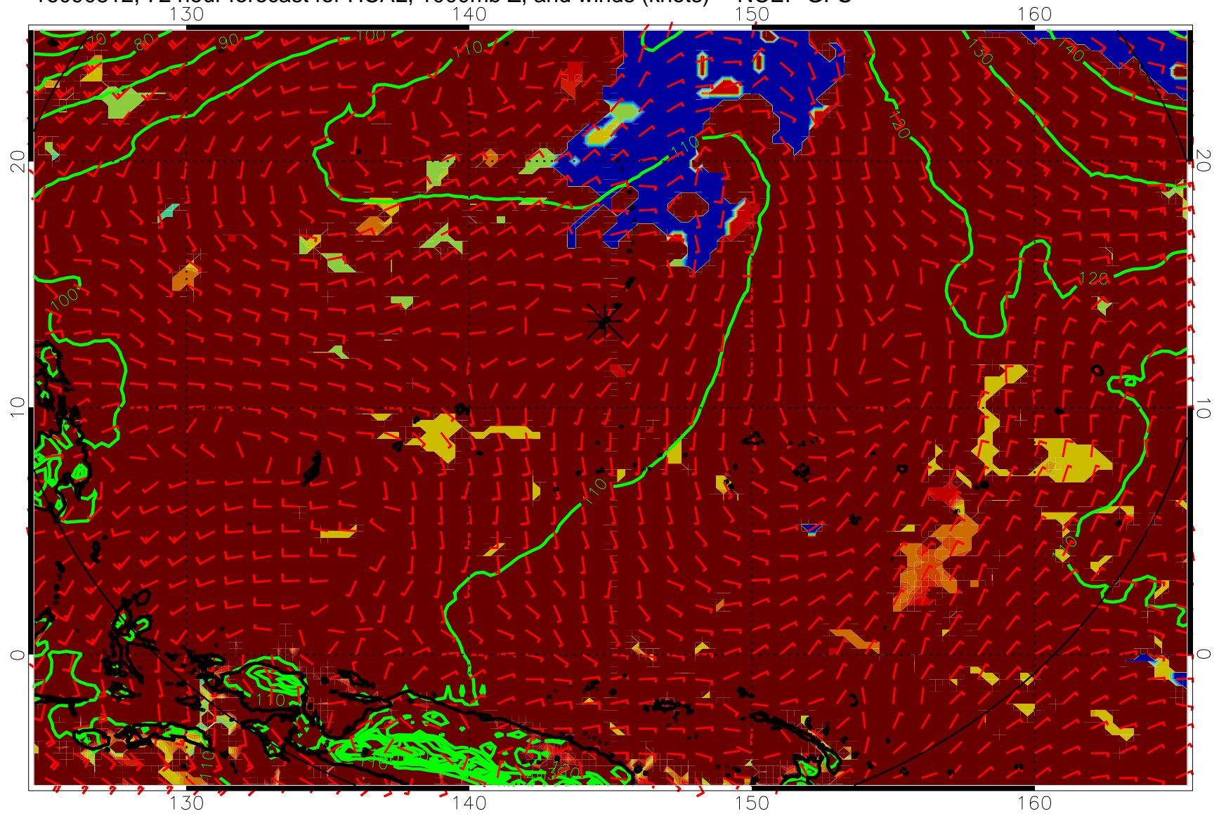
16090812, 72 hour forecast for HCAL, 1000mb Z, and winds (knots) -- NCEP GFS
