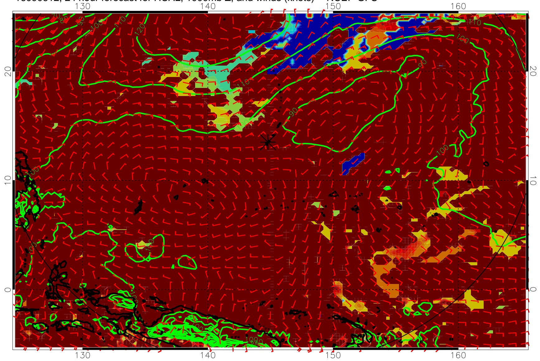
16090612, 24 hour forecast for HCAL, 1000mb Z, and winds (knots) -- NCEP GFS
