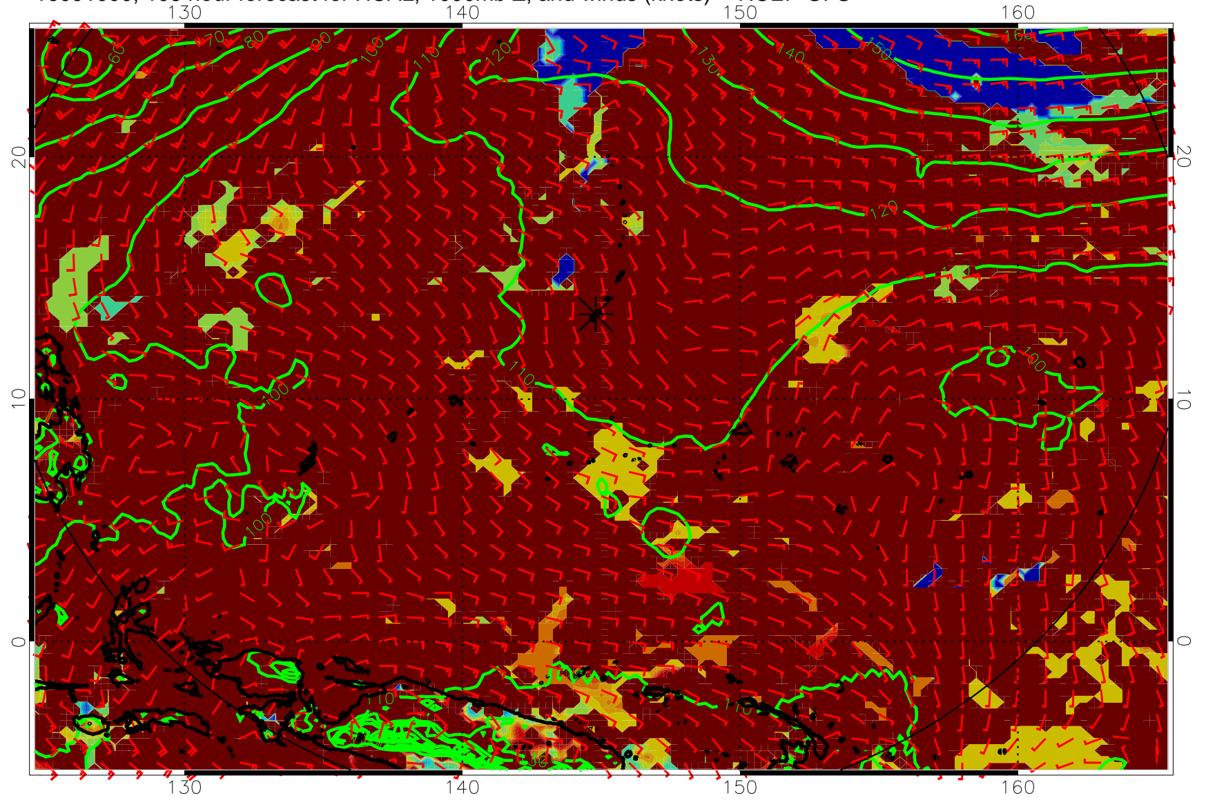
16091000, 108 hour forecast for HCAL, 1000mb Z, and winds (knots) -- NCEP GFS
