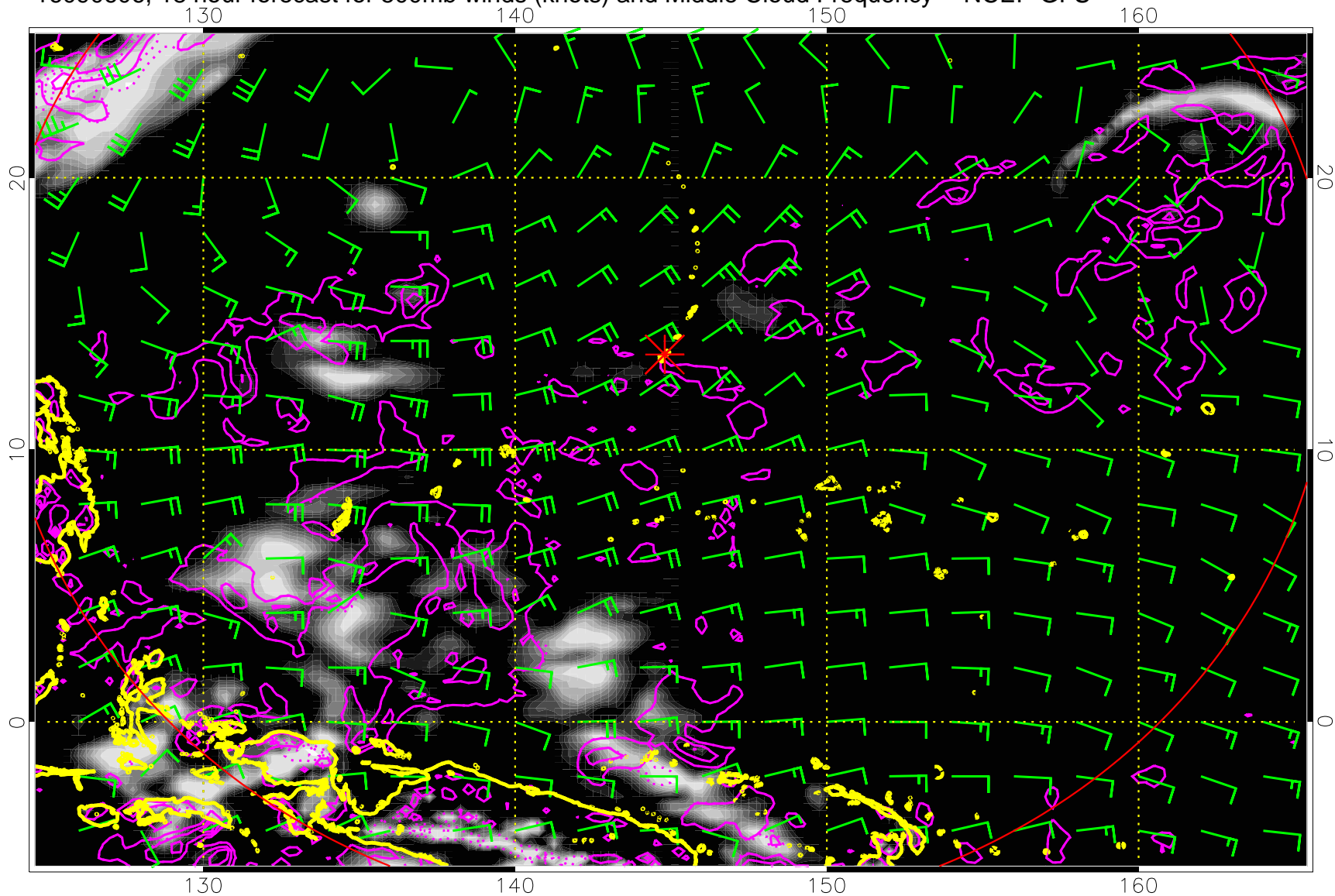
16090606, 18 hour forecast for 500mb winds (knots) and Middle Cloud Frequency -- NCEP GFS
