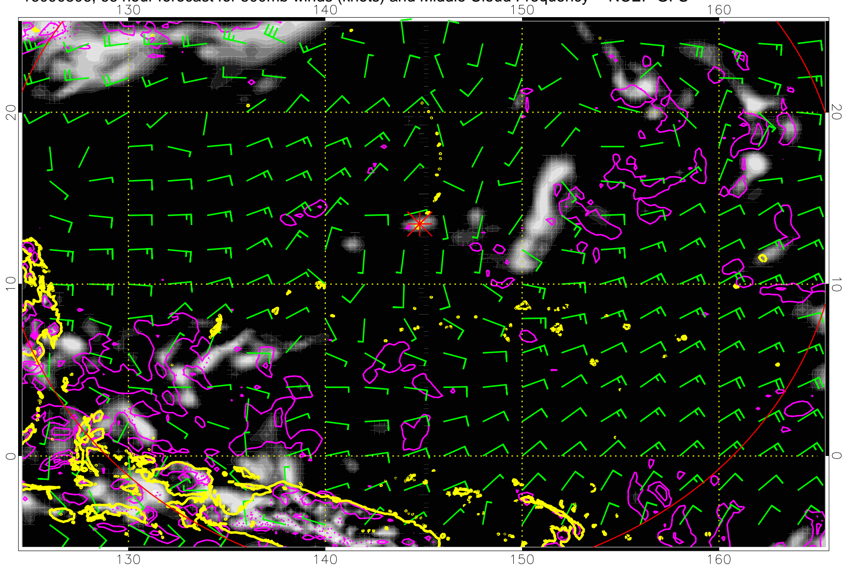
16090806, 66 hour forecast for 500mb winds (knots) and Middle Cloud Frequency -- NCEP GFS
