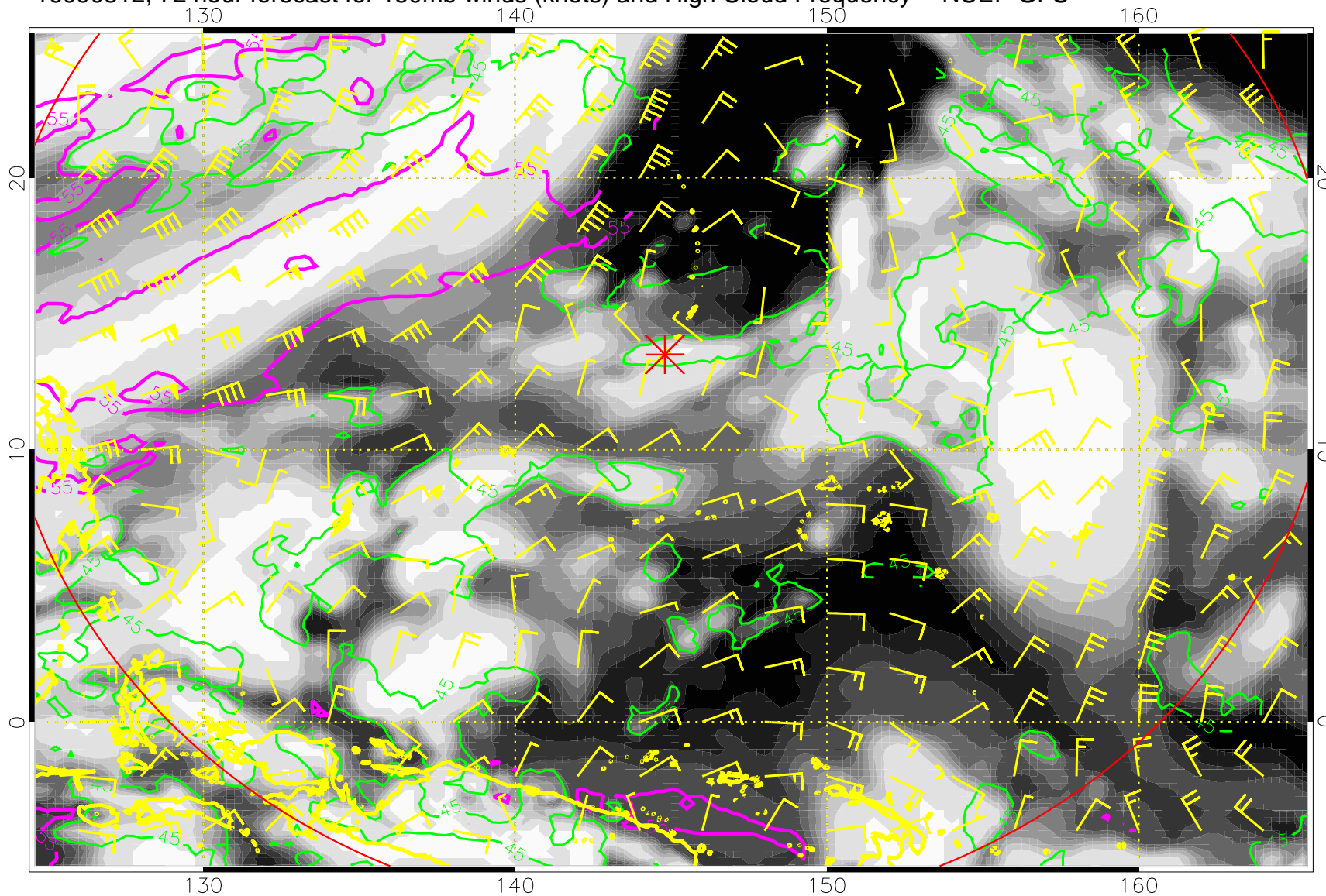
16090812, 72 hour forecast for 150mb winds (knots) and High Cloud Frequency -- NCEP GFS
