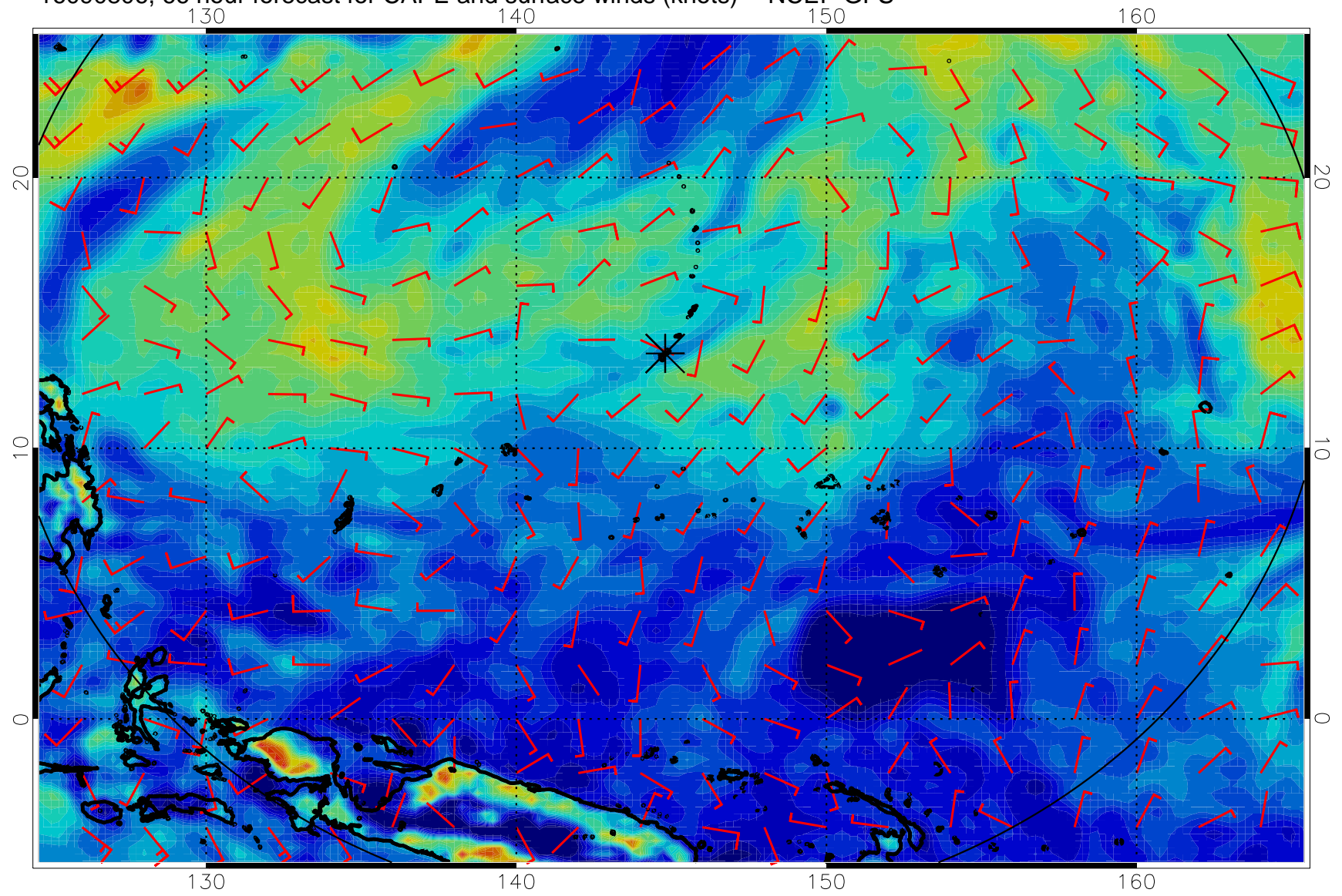
16090806, 66 hour forecast for CAPE and surface winds (knots) -- NCEP GFS
