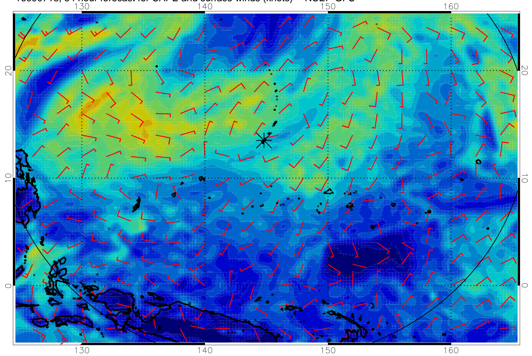
16090718, 54 hour forecast for CAPE and surface winds (knots) -- NCEP GFS
