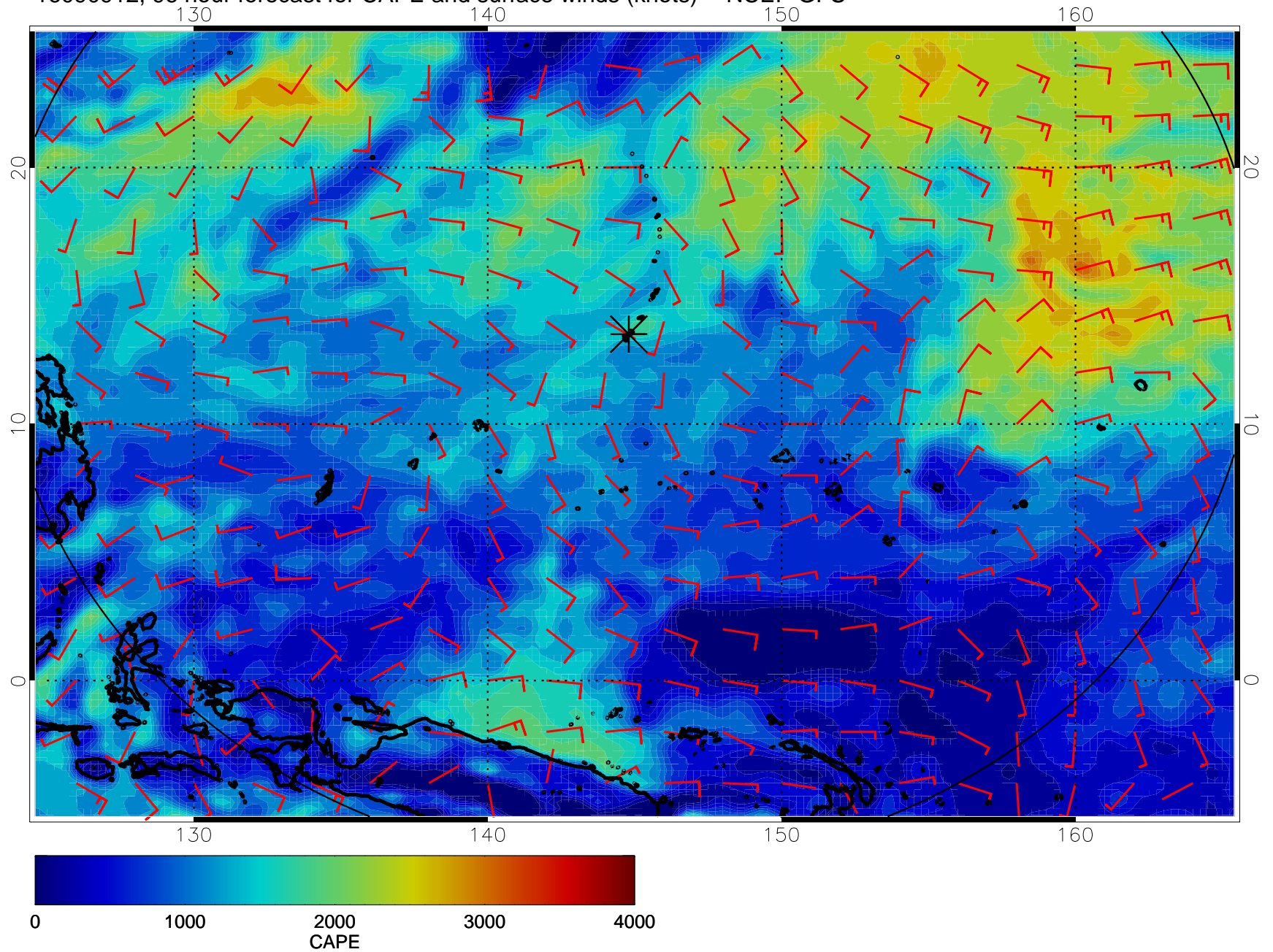
16090912, 96 hour forecast for CAPE and surface winds (knots) -- NCEP GFS
