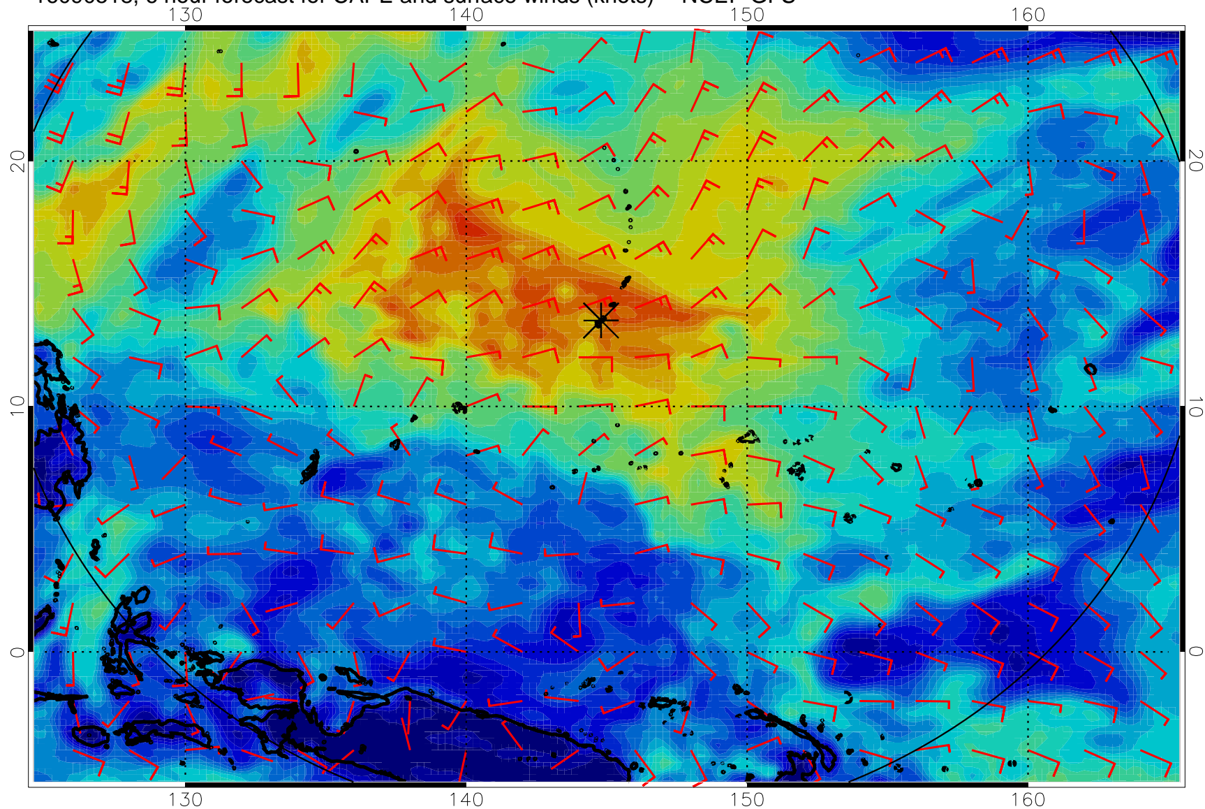
16090518, 6 hour forecast for CAPE and surface winds (knots) -- NCEP GFS
