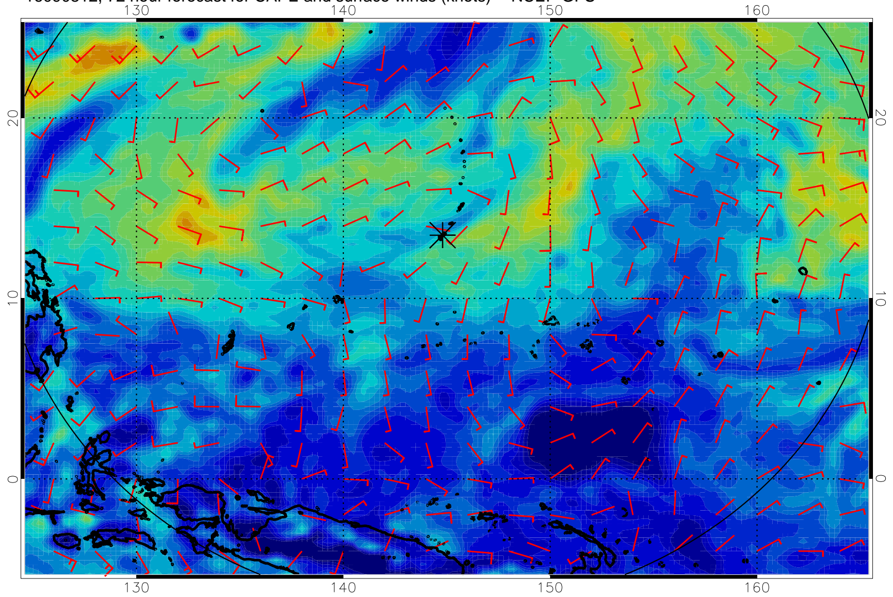
16090812, 72 hour forecast for CAPE and surface winds (knots) -- NCEP GFS
