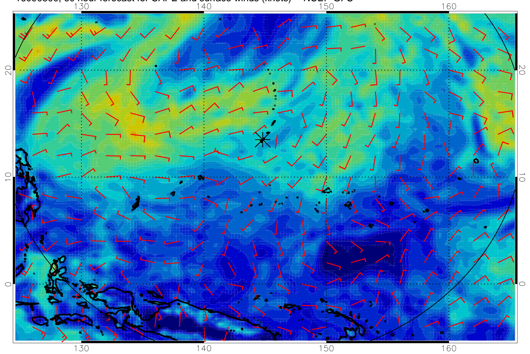
16090800, 60 hour forecast for CAPE and surface winds (knots) -- NCEP GFS
