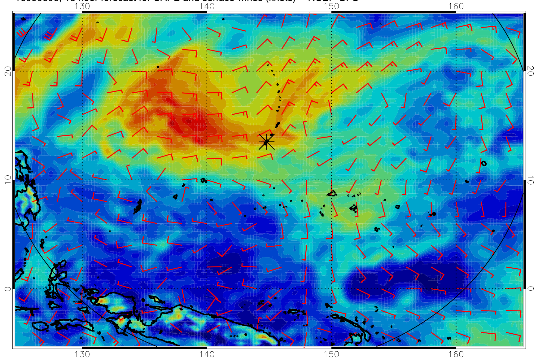
16090606, 18 hour forecast for CAPE and surface winds (knots) -- NCEP GFS
