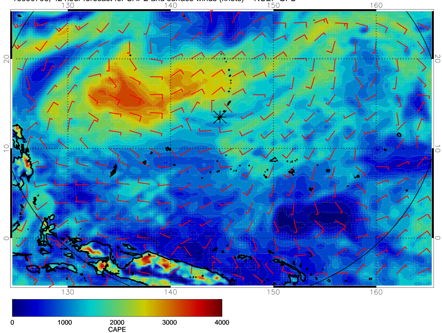
16090706, 42 hour forecast for CAPE and surface winds (knots) -- NCEP GFS
