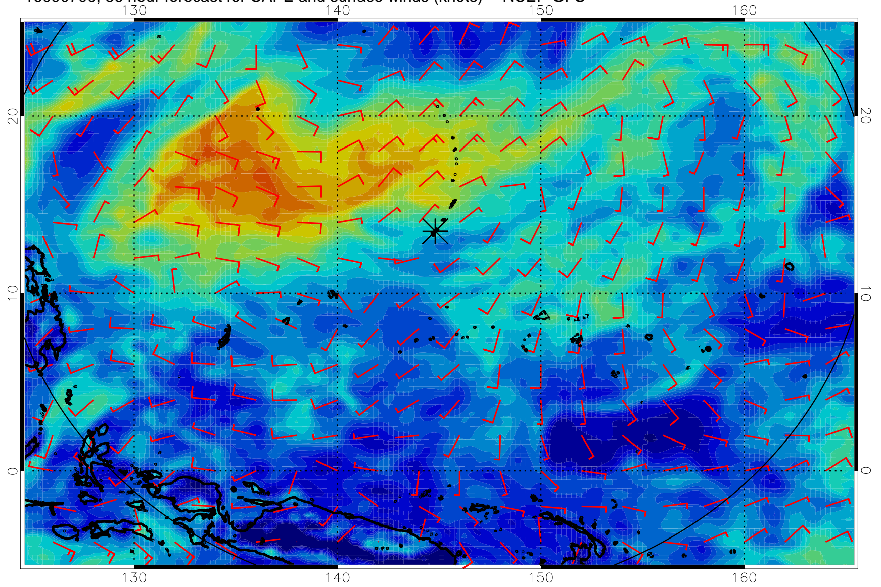
16090700, 36 hour forecast for CAPE and surface winds (knots) -- NCEP GFS
