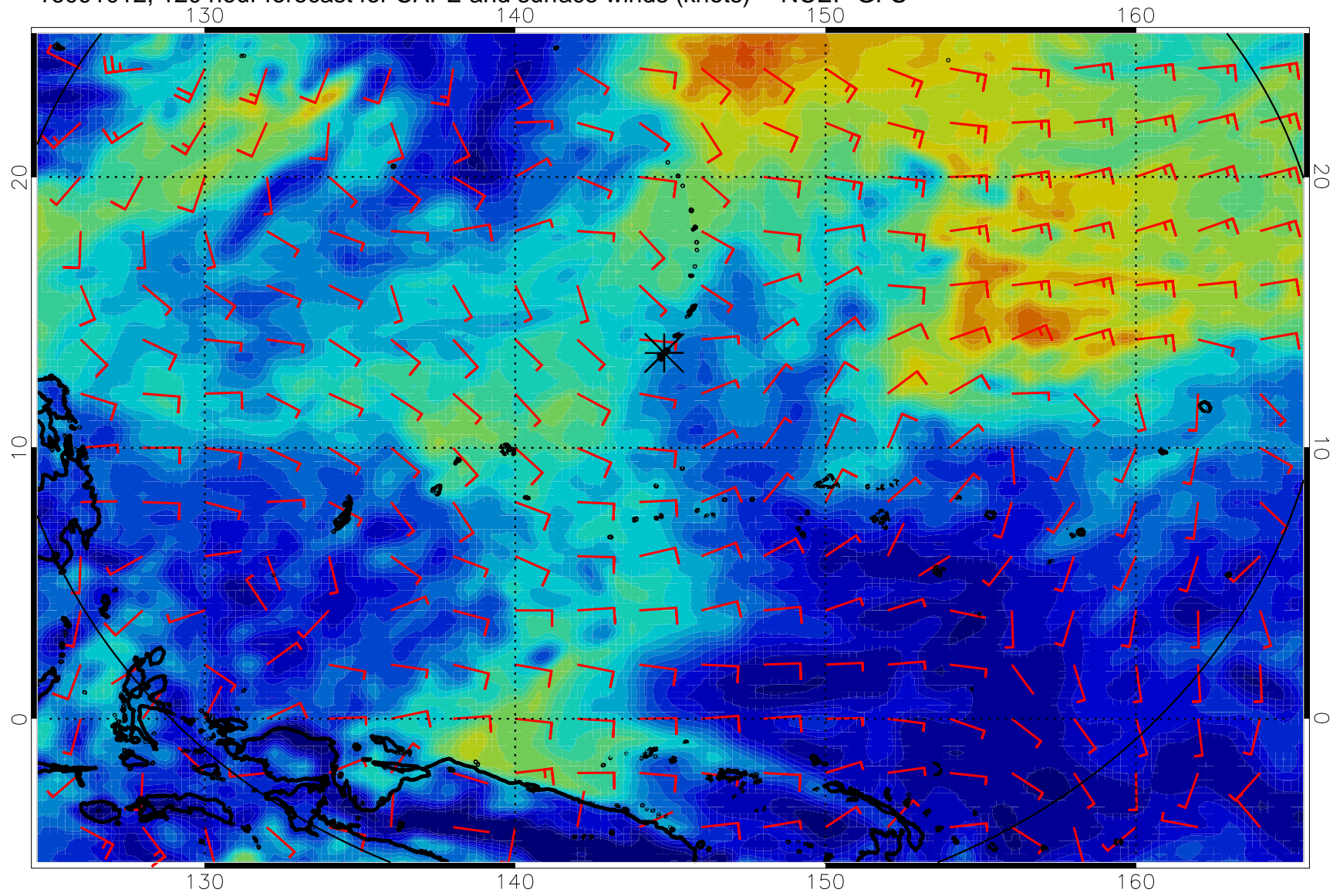
16091012, 120 hour forecast for CAPE and surface winds (knots) -- NCEP GFS
