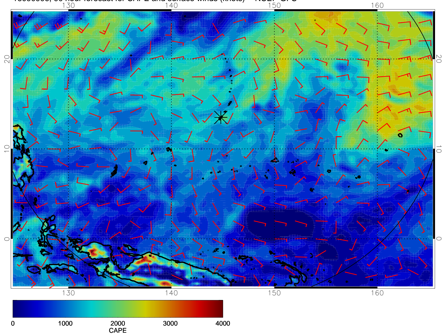
16090906, 90 hour forecast for CAPE and surface winds (knots) -- NCEP GFS
