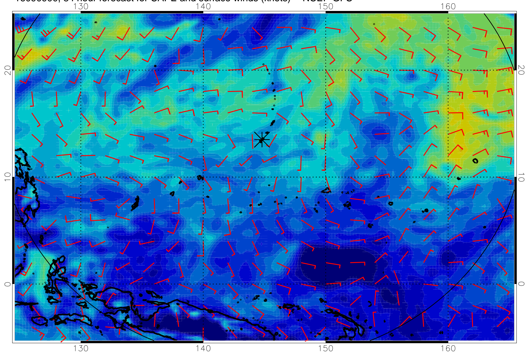
16090900, 84 hour forecast for CAPE and surface winds (knots) -- NCEP GFS
