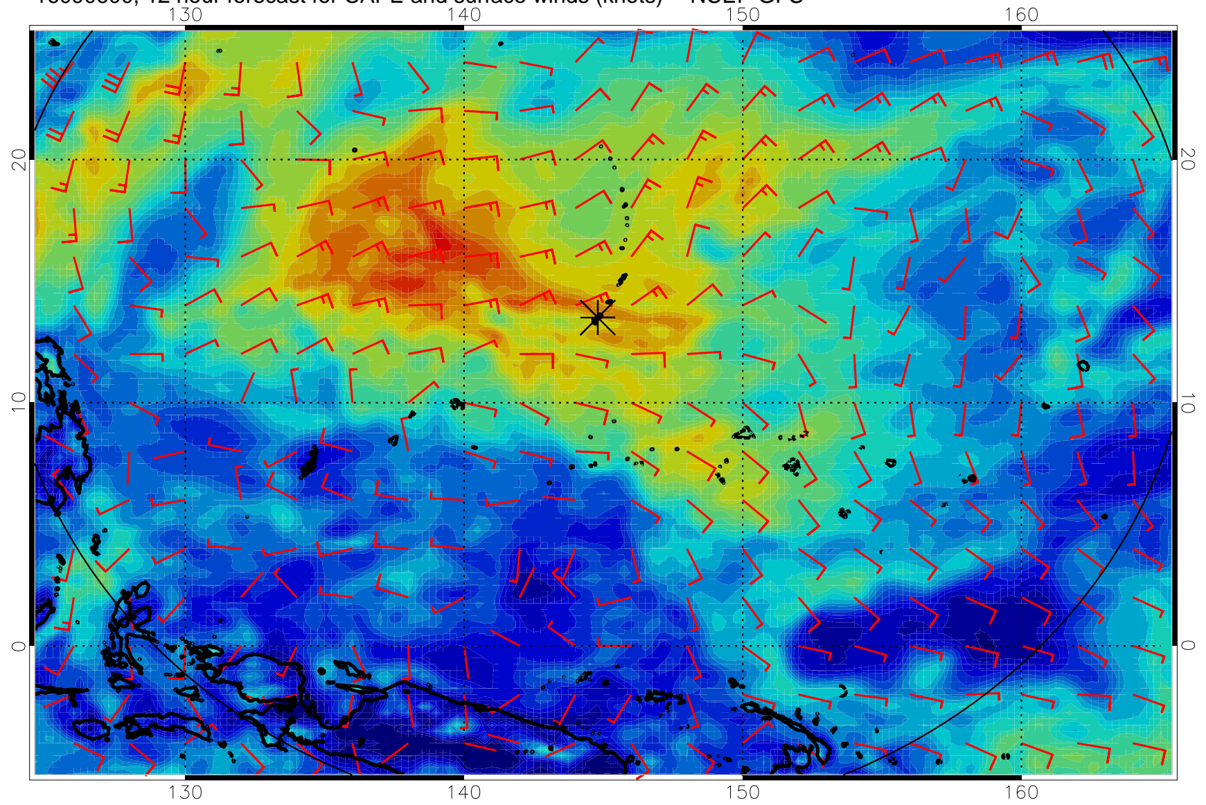
16090600, 12 hour forecast for CAPE and surface winds (knots) -- NCEP GFS
