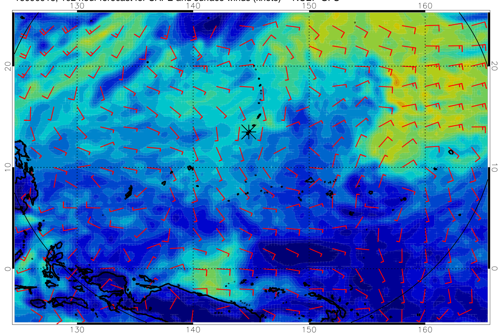
16090918, 102 hour forecast for CAPE and surface winds (knots) -- NCEP GFS
