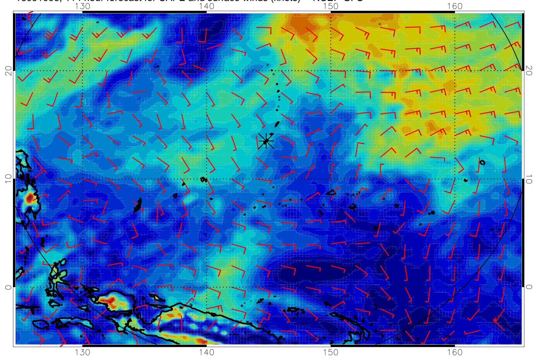
16091006, 114 hour forecast for CAPE and surface winds (knots) -- NCEP GFS
