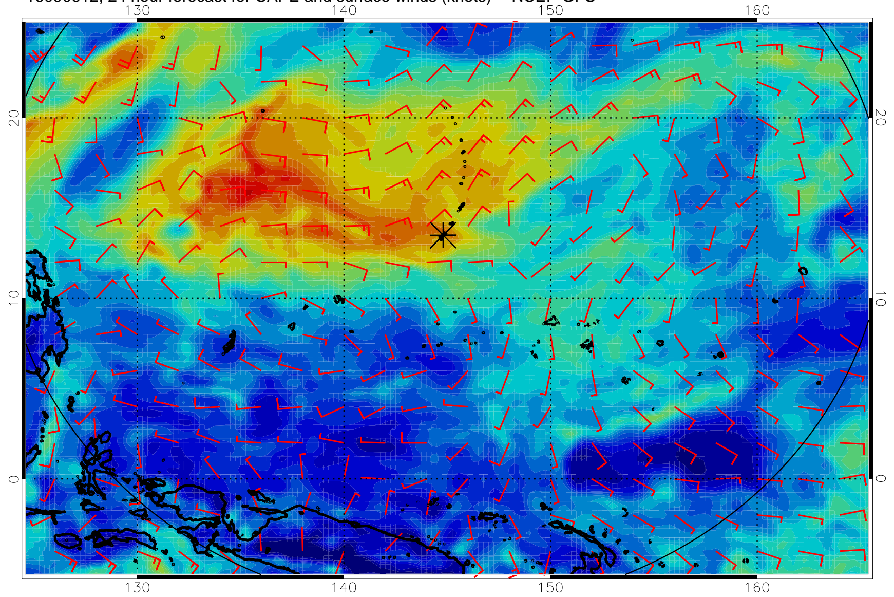
16090612, 24 hour forecast for CAPE and surface winds (knots) -- NCEP GFS
