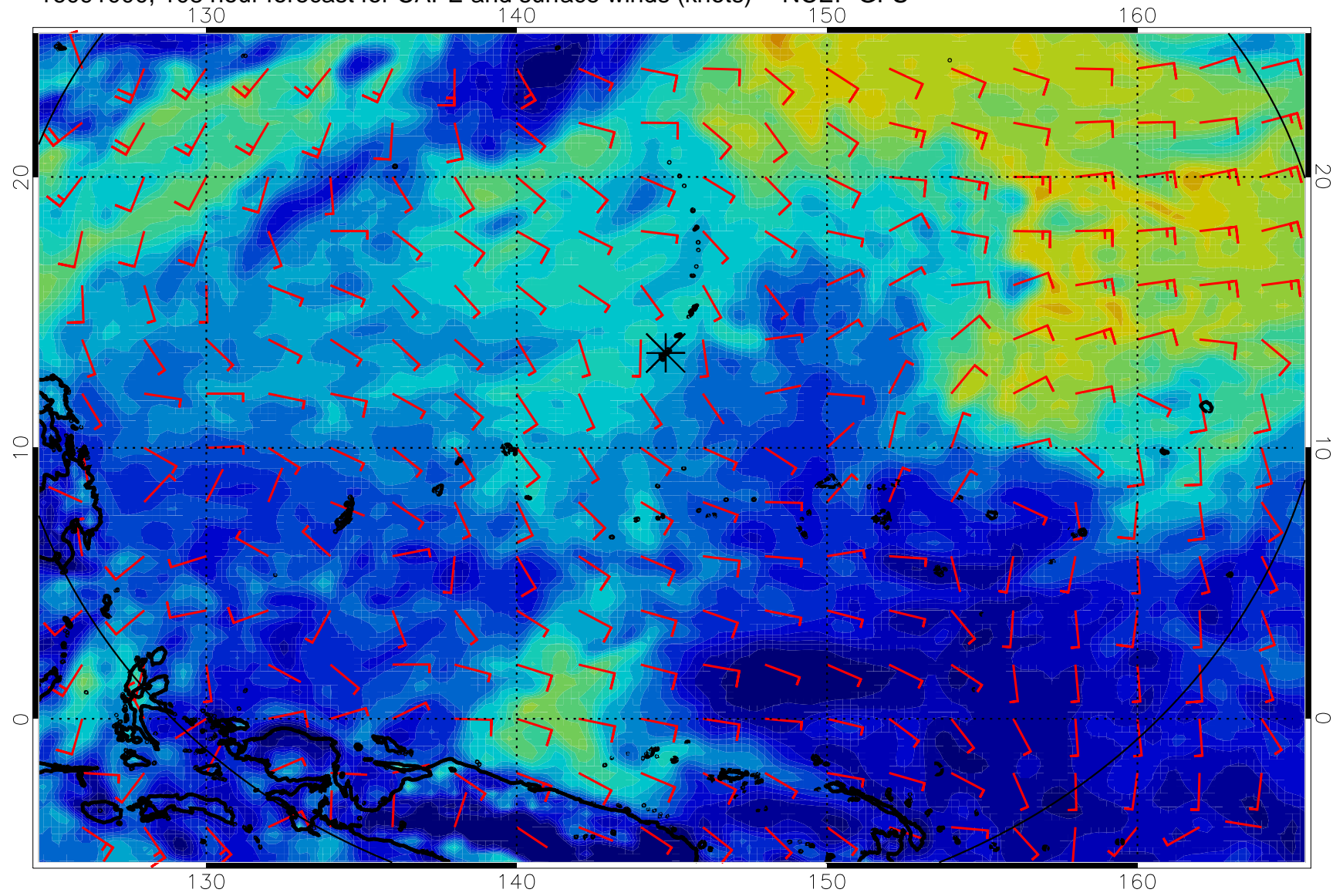
16091000, 108 hour forecast for CAPE and surface winds (knots) -- NCEP GFS
