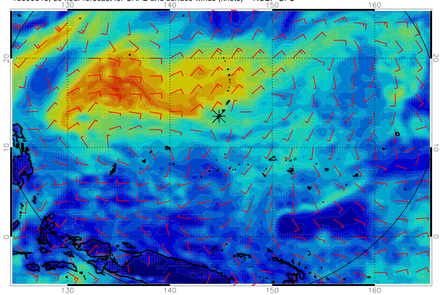
16090618, 30 hour forecast for CAPE and surface winds (knots) -- NCEP GFS
