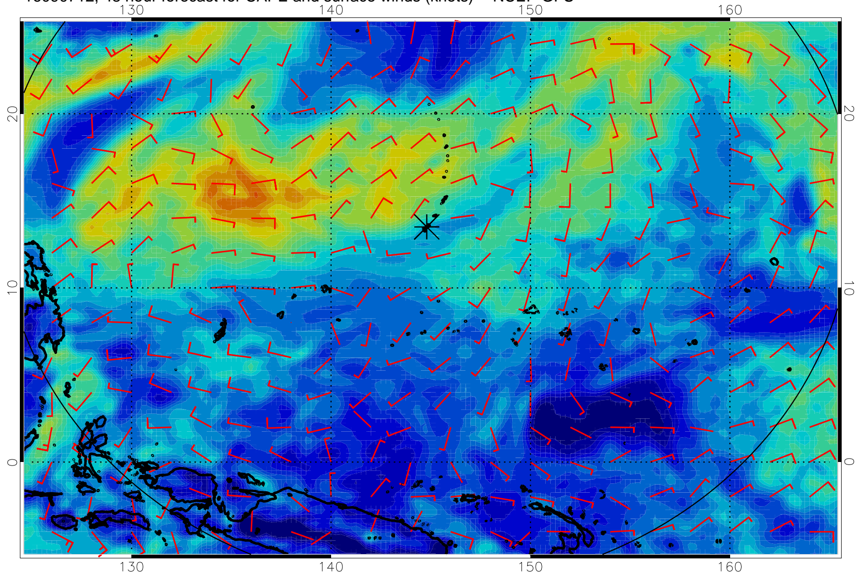
16090712, 48 hour forecast for CAPE and surface winds (knots) -- NCEP GFS
