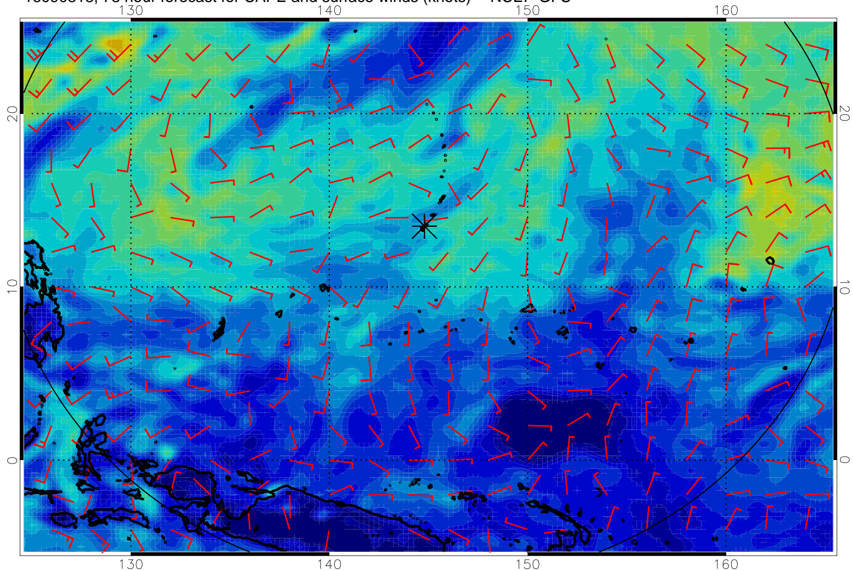
16090818, 78 hour forecast for CAPE and surface winds (knots) -- NCEP GFS
