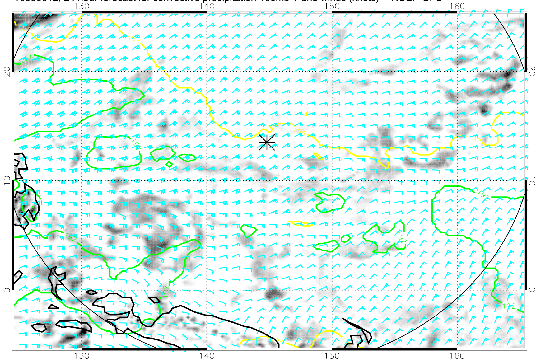
16090612, 24 hour forecast for convective precipitation 100mb T and winds (knots) -- NCEP GFS
