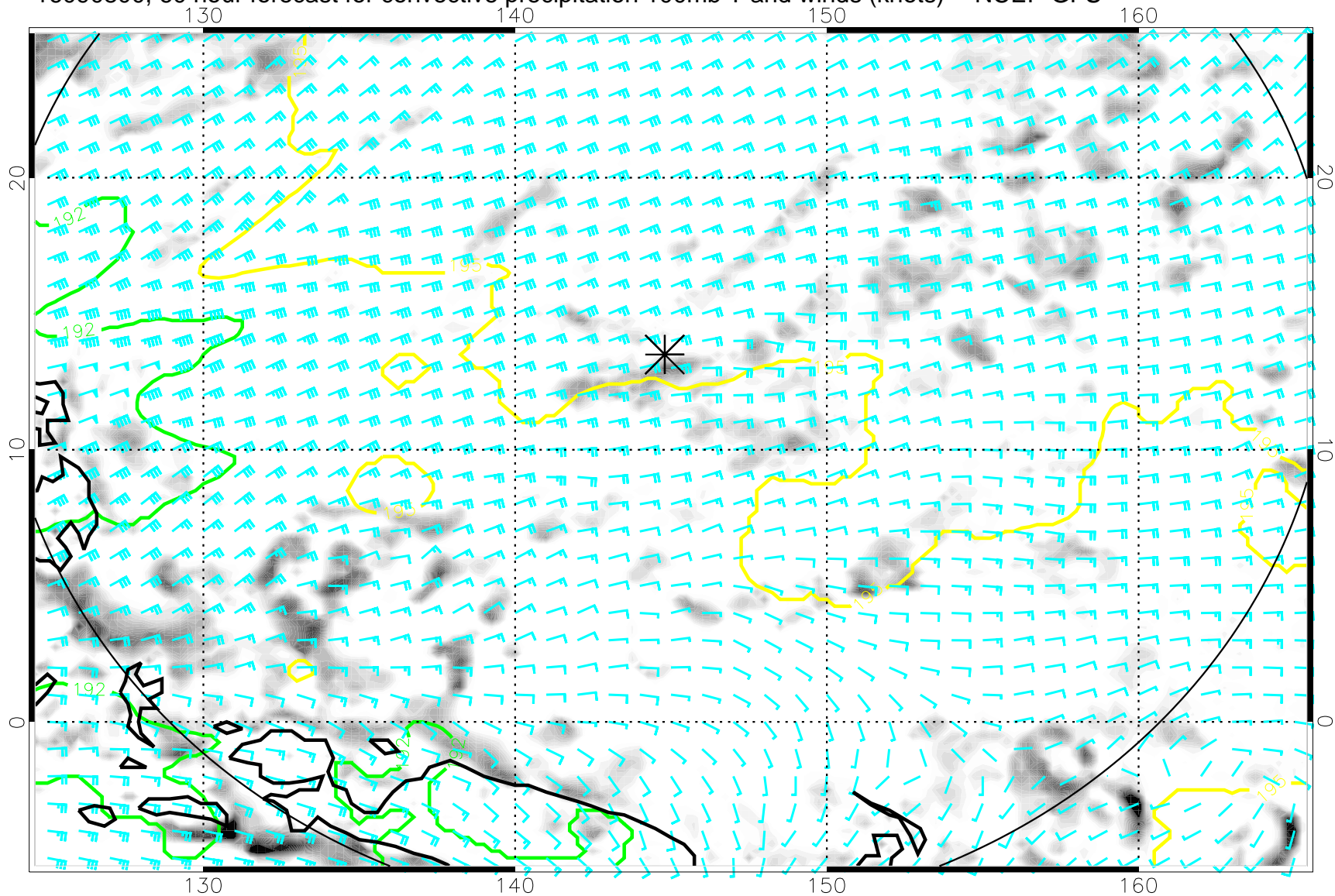
16090800, 60 hour forecast for convective precipitation 100mb T and winds (knots) -- NCEP GFS
