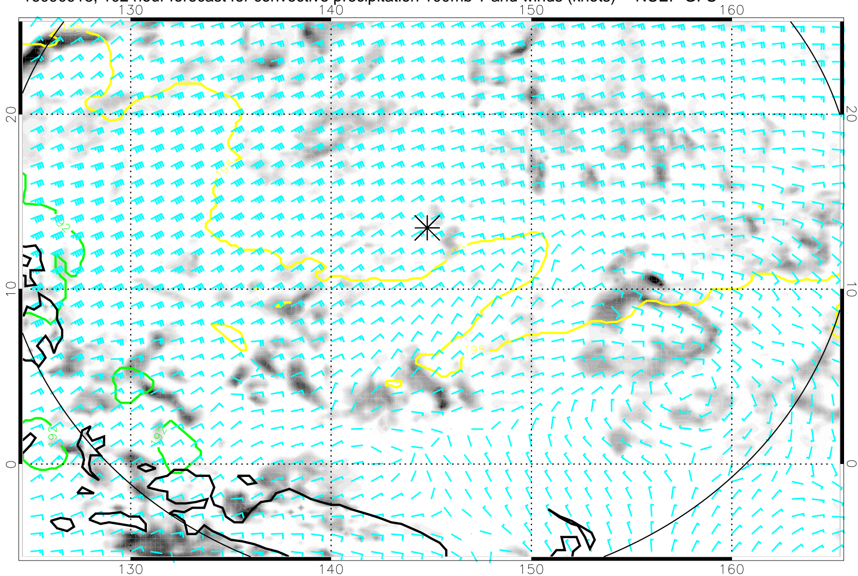
16090918, 102 hour forecast for convective precipitation 100mb T and winds (knots) -- NCEP GFS
