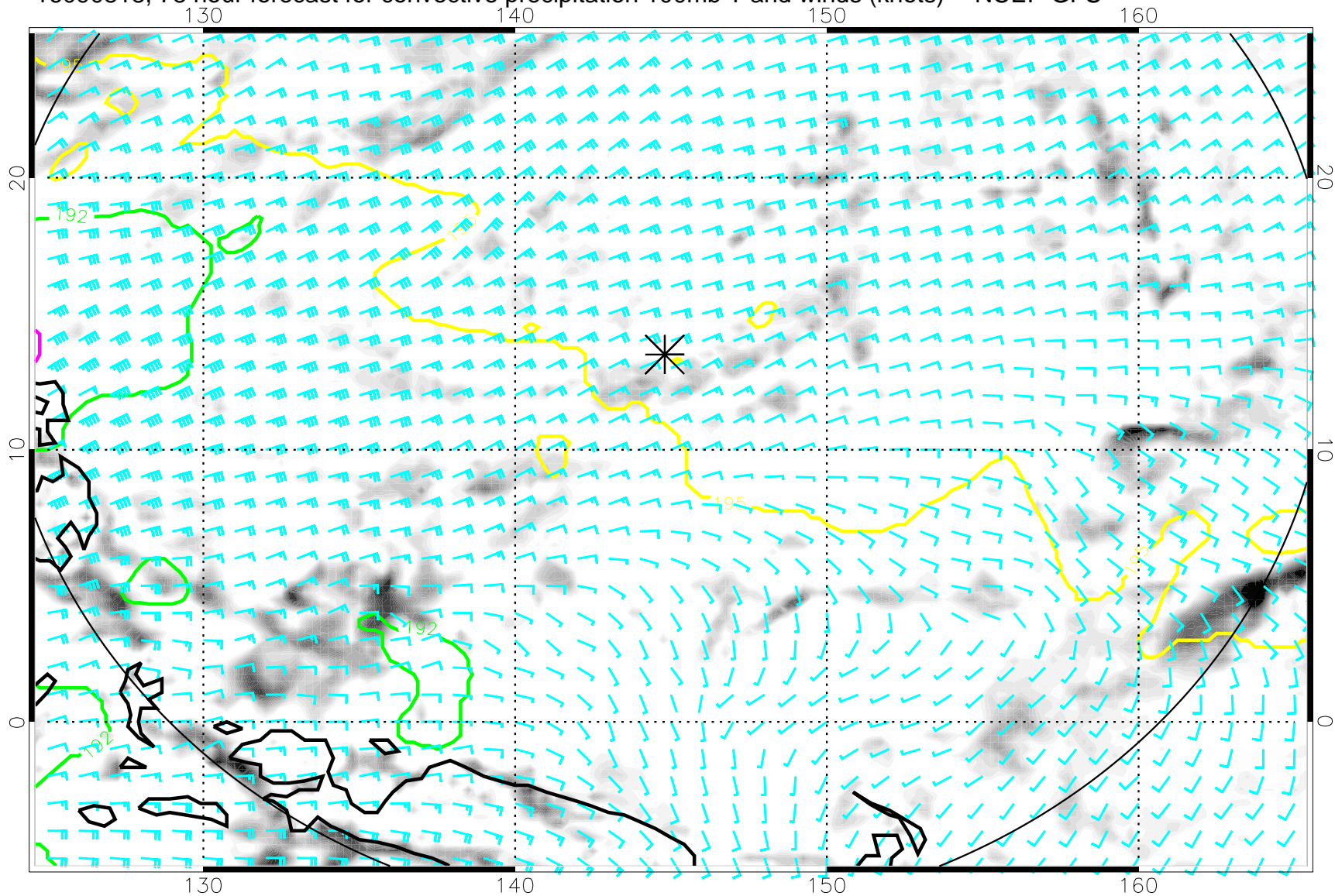
16090818, 78 hour forecast for convective precipitation 100mb T and winds (knots) -- NCEP GFS
