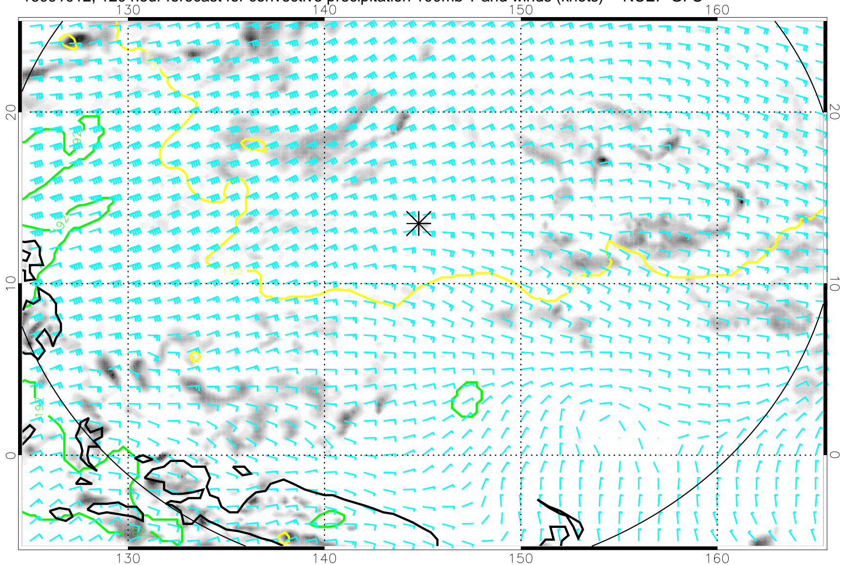
16091012, 120 hour forecast for convective precipitation 100mb T and winds (knots) -- NCEP GFS
