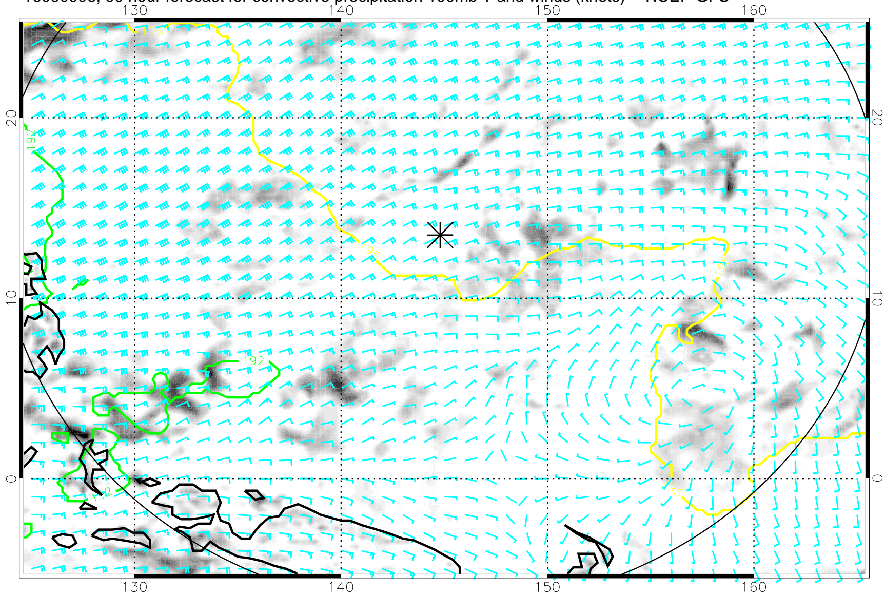
16090906, 90 hour forecast for convective precipitation 100mb T and winds (knots) -- NCEP GFS
