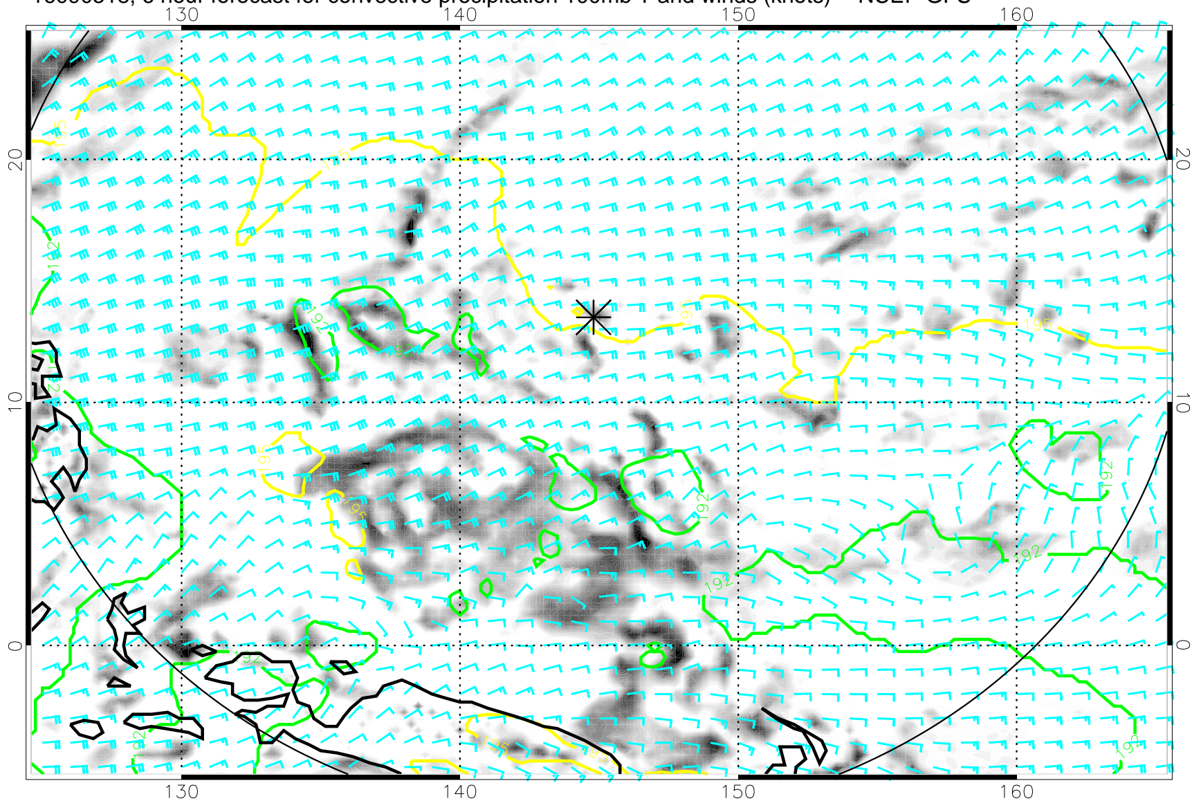
16090518, 6 hour forecast for convective precipitation 100mb T and winds (knots) -- NCEP GFS
