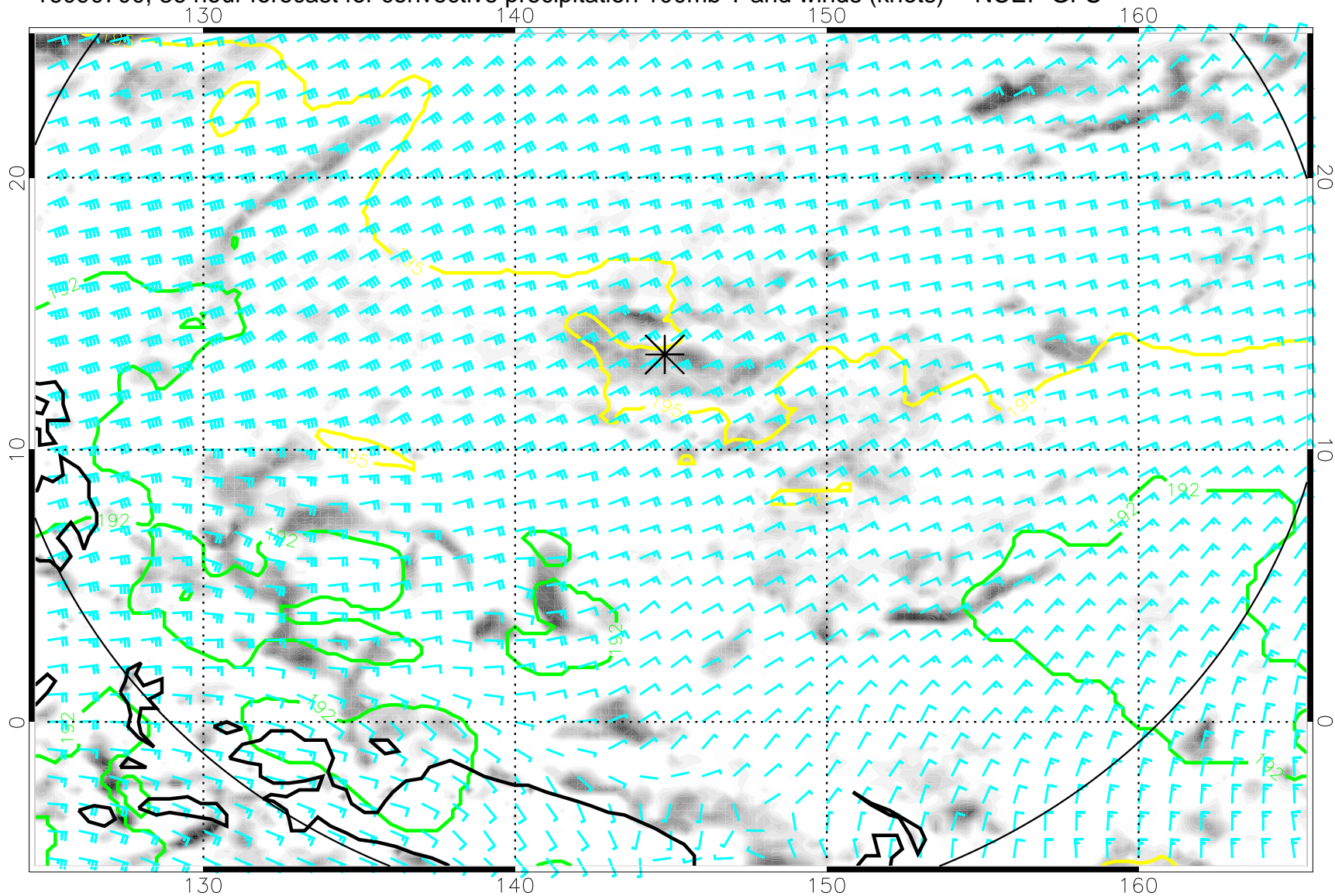
16090700, 36 hour forecast for convective precipitation 100mb T and winds (knots) -- NCEP GFS
