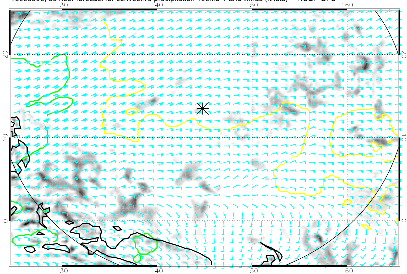
16090806, 66 hour forecast for convective precipitation 100mb T and winds (knots) -- NCEP GFS
