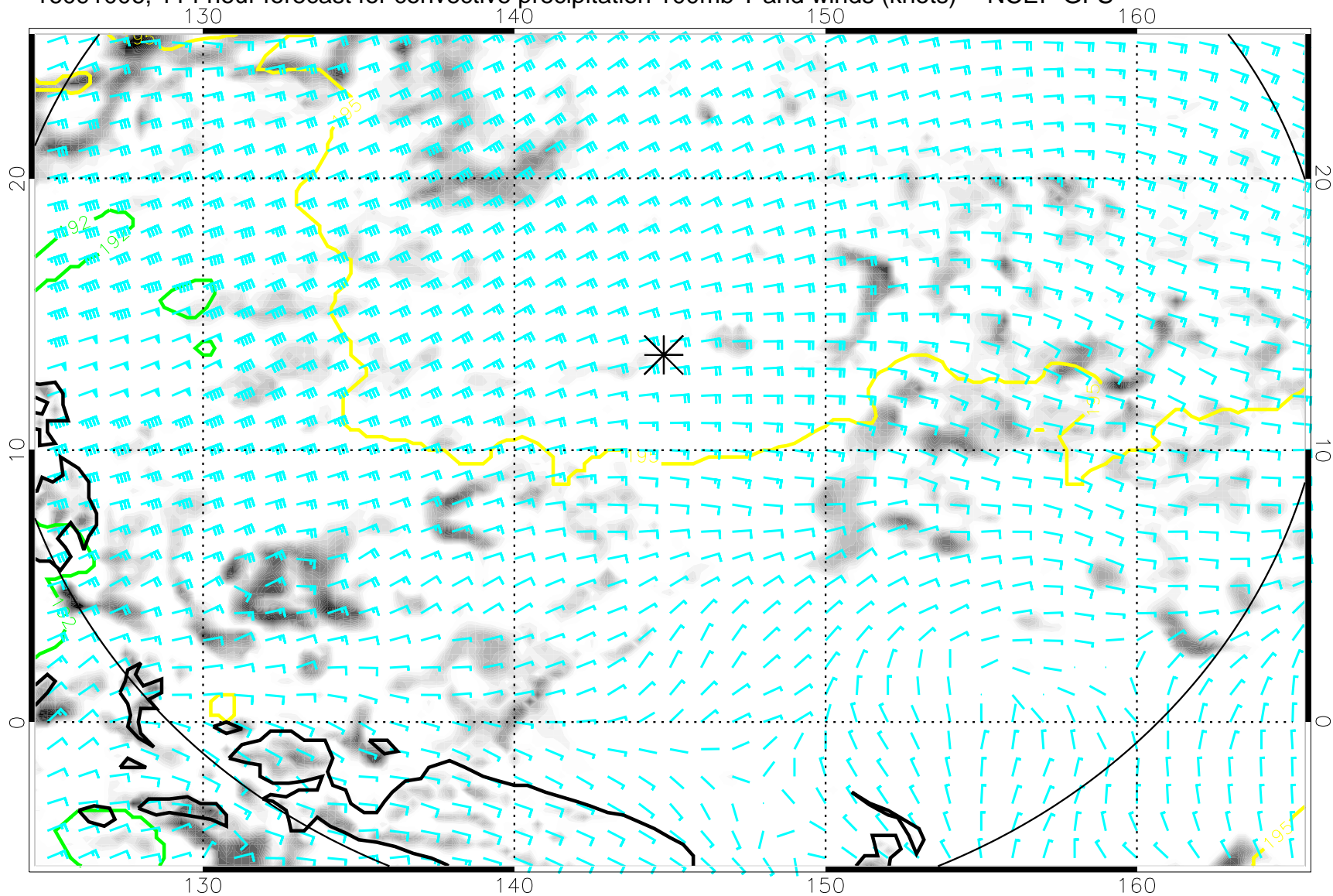
16091006, 114 hour forecast for convective precipitation 100mb T and winds (knots) -- NCEP GFS
