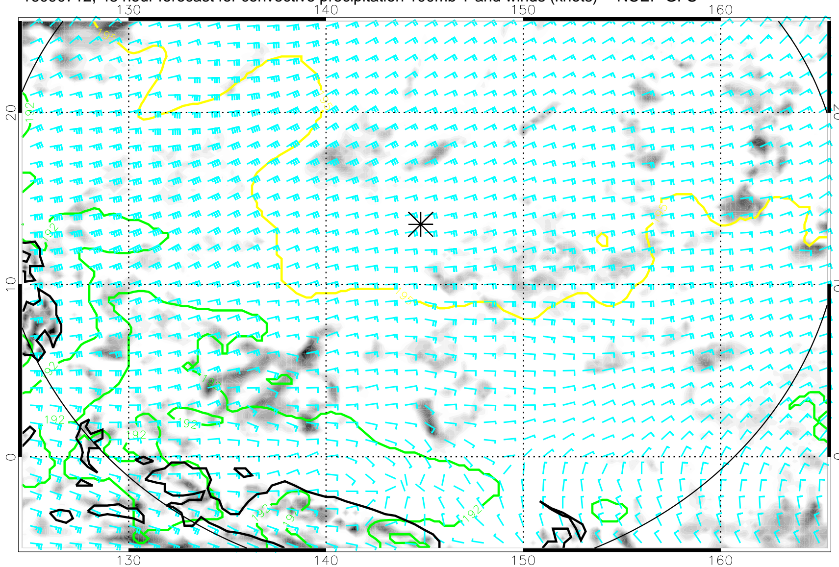
16090712, 48 hour forecast for convective precipitation 100mb T and winds (knots) -- NCEP GFS
