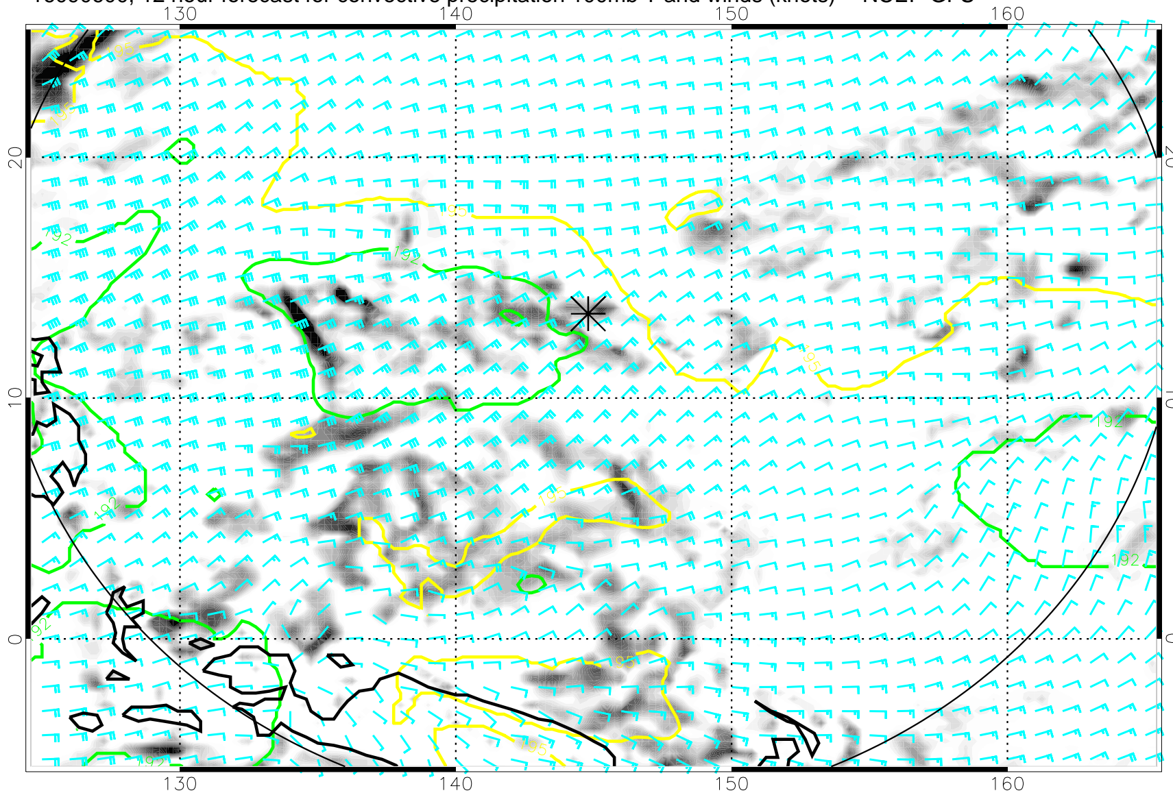
16090600, 12 hour forecast for convective precipitation 100mb T and winds (knots) -- NCEP GFS
