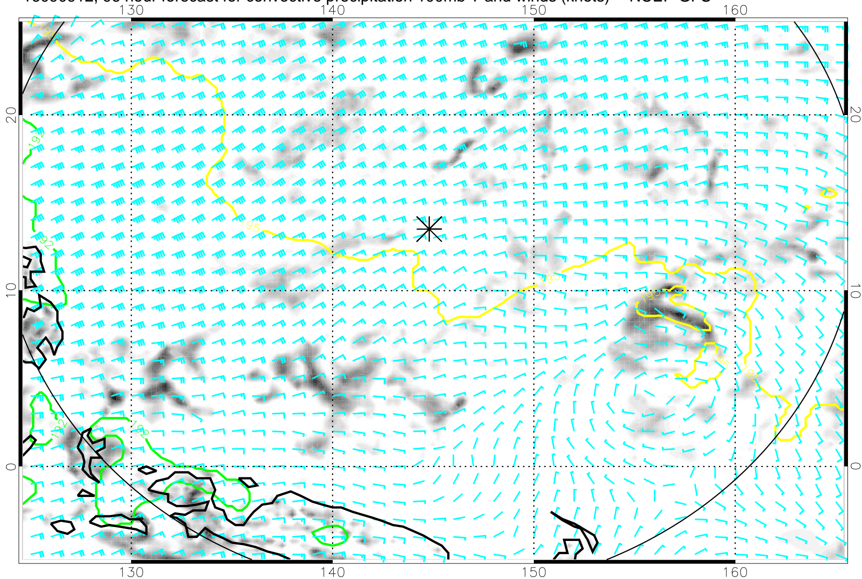
16090912, 96 hour forecast for convective precipitation 100mb T and winds (knots) -- NCEP GFS
