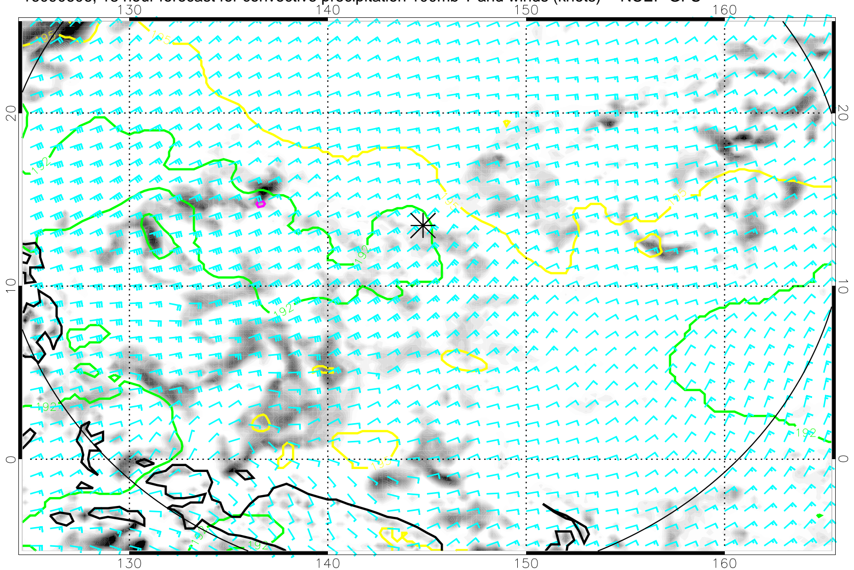
16090606, 18 hour forecast for convective precipitation 100mb T and winds (knots) -- NCEP GFS
