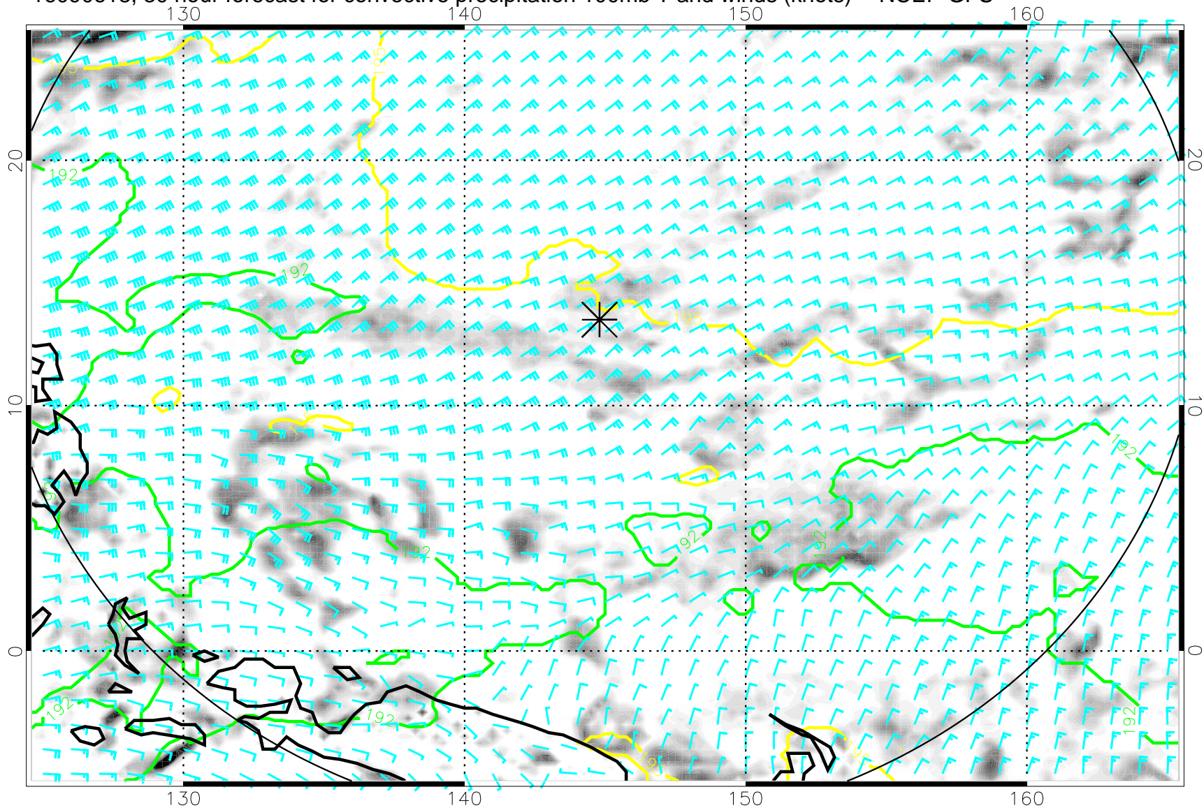
16090618, 30 hour forecast for convective precipitation 100mb T and winds (knots) -- NCEP GFS
