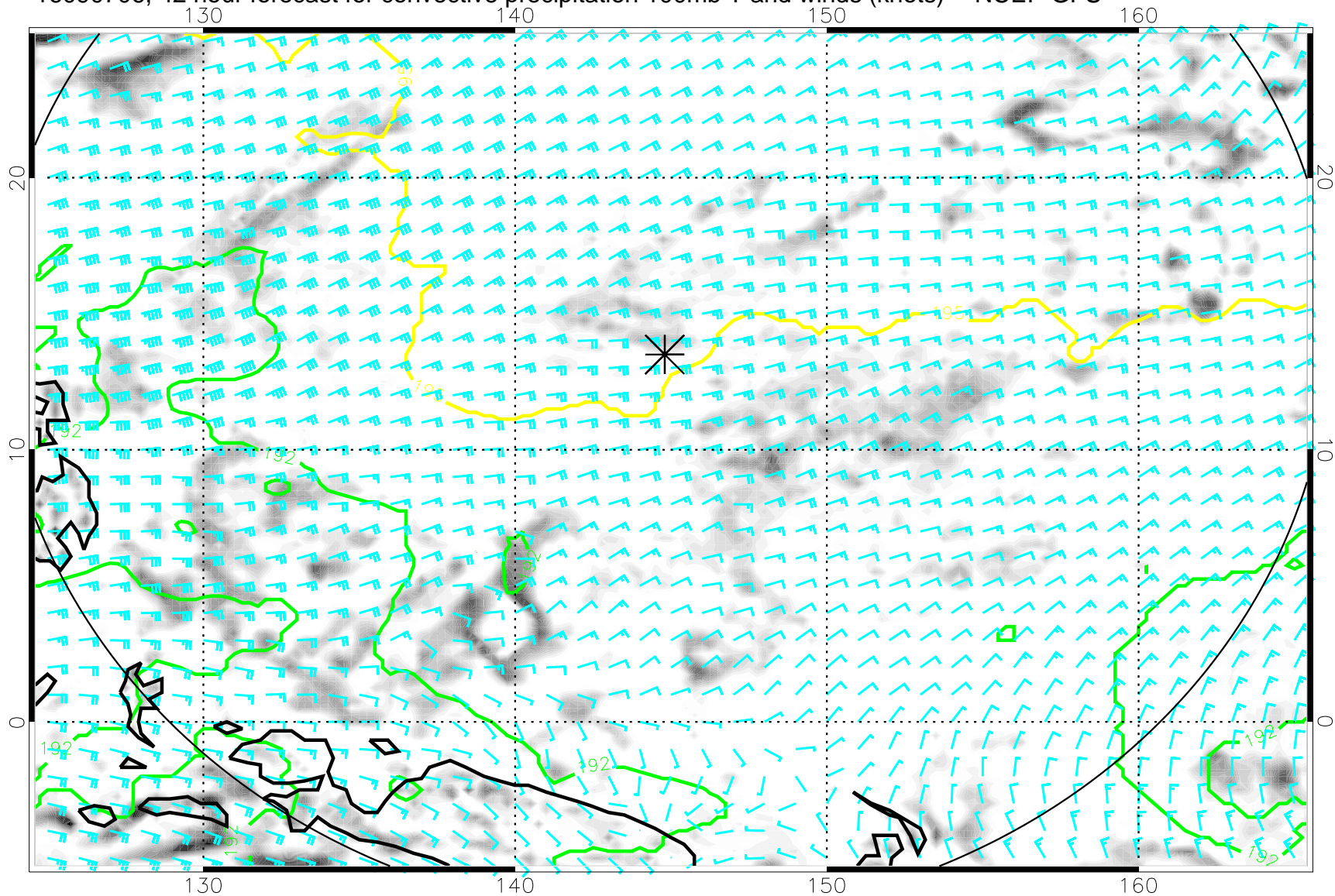
16090706, 42 hour forecast for convective precipitation 100mb T and winds (knots) -- NCEP GFS
