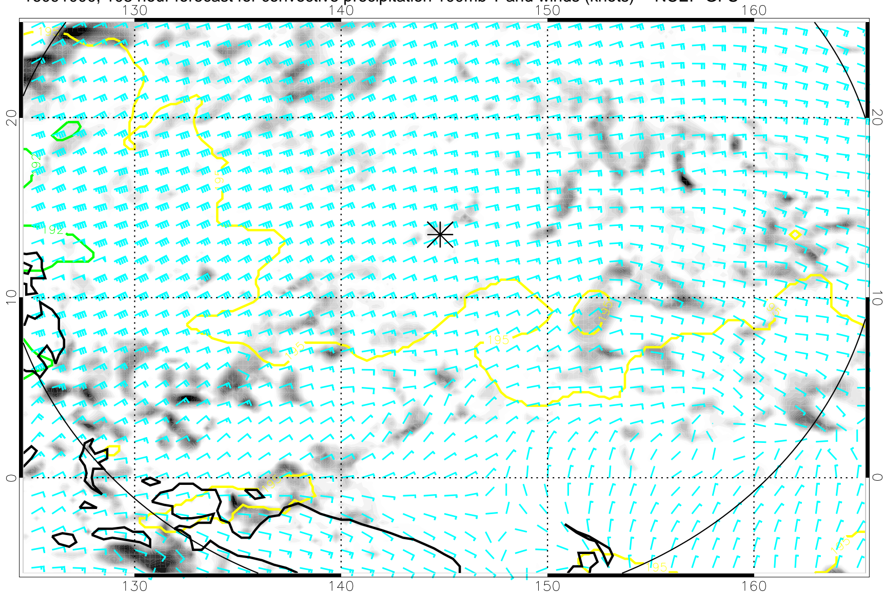
16091000, 108 hour forecast for convective precipitation 100mb T and winds (knots) -- NCEP GFS
