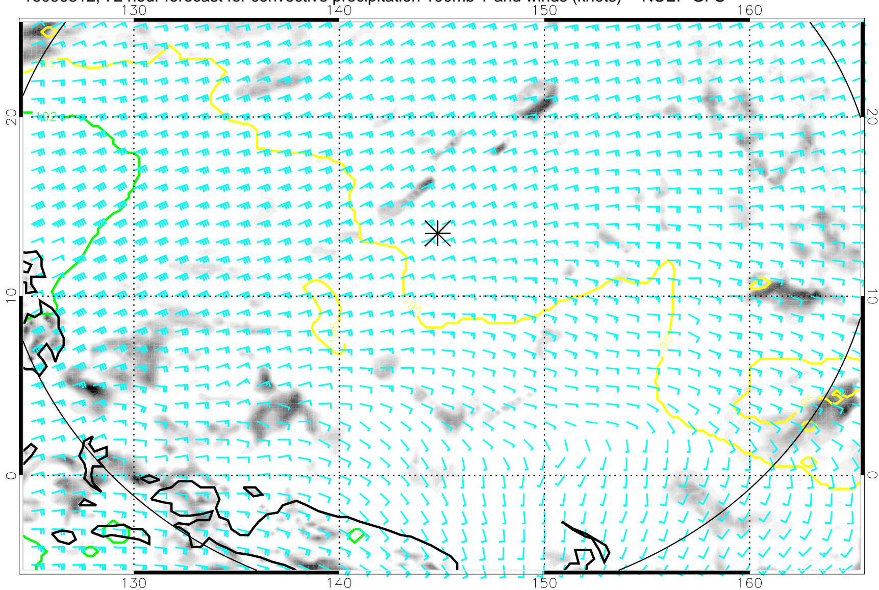
16090812, 72 hour forecast for convective precipitation 100mb T and winds (knots) -- NCEP GFS
