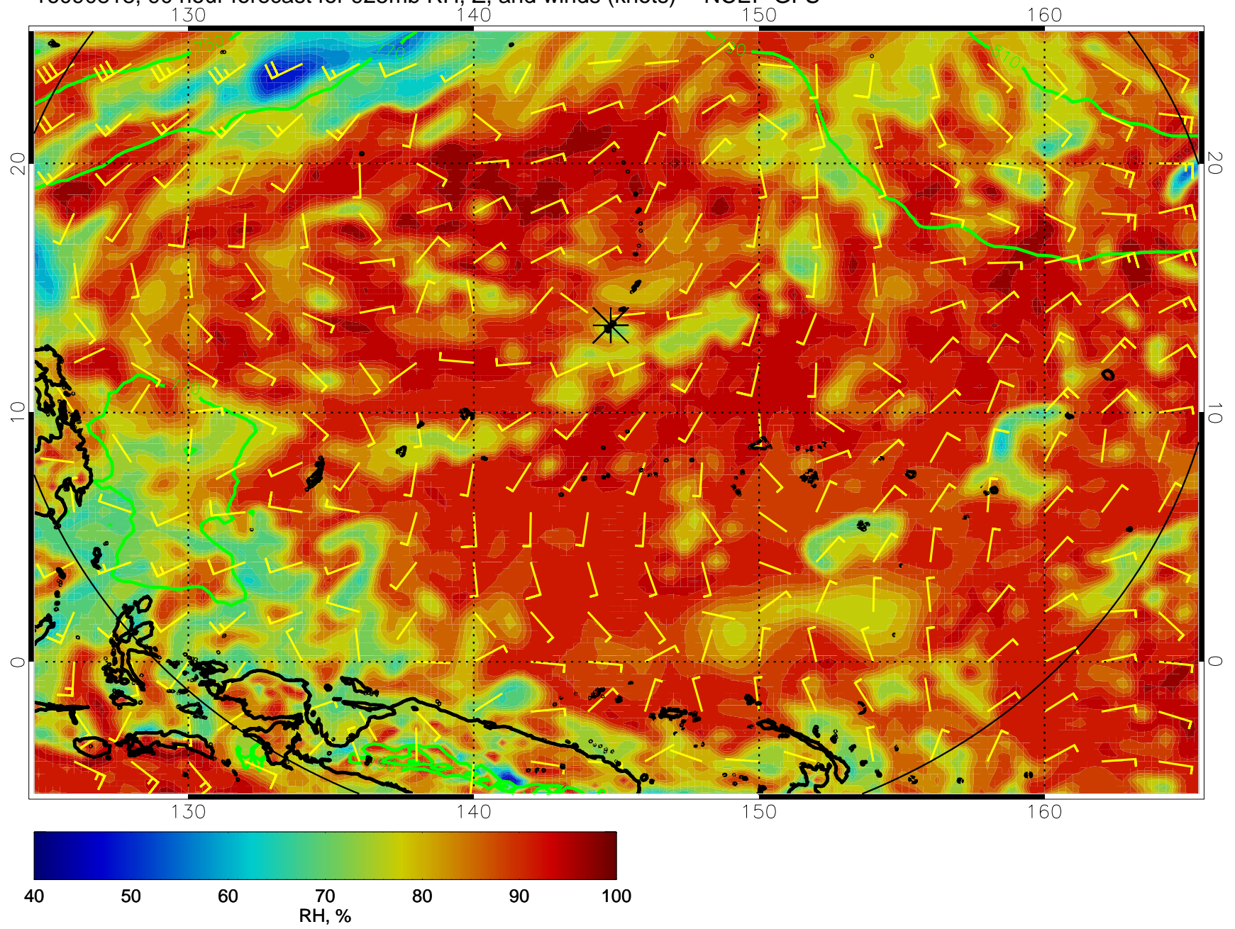
16090818, 90 hour forecast for 925mb RH, Z, and winds (knots) -- NCEP GFS
