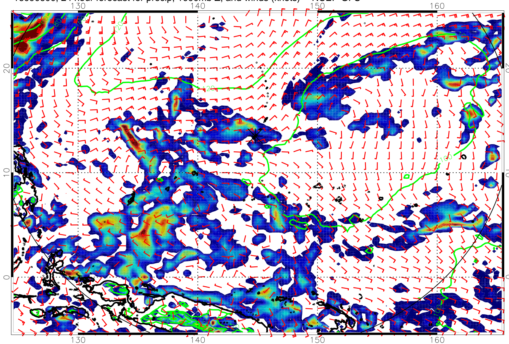
16090600, 24 hour forecast for precip, 1000mb Z, and winds (knots) -- NCEP GFS
