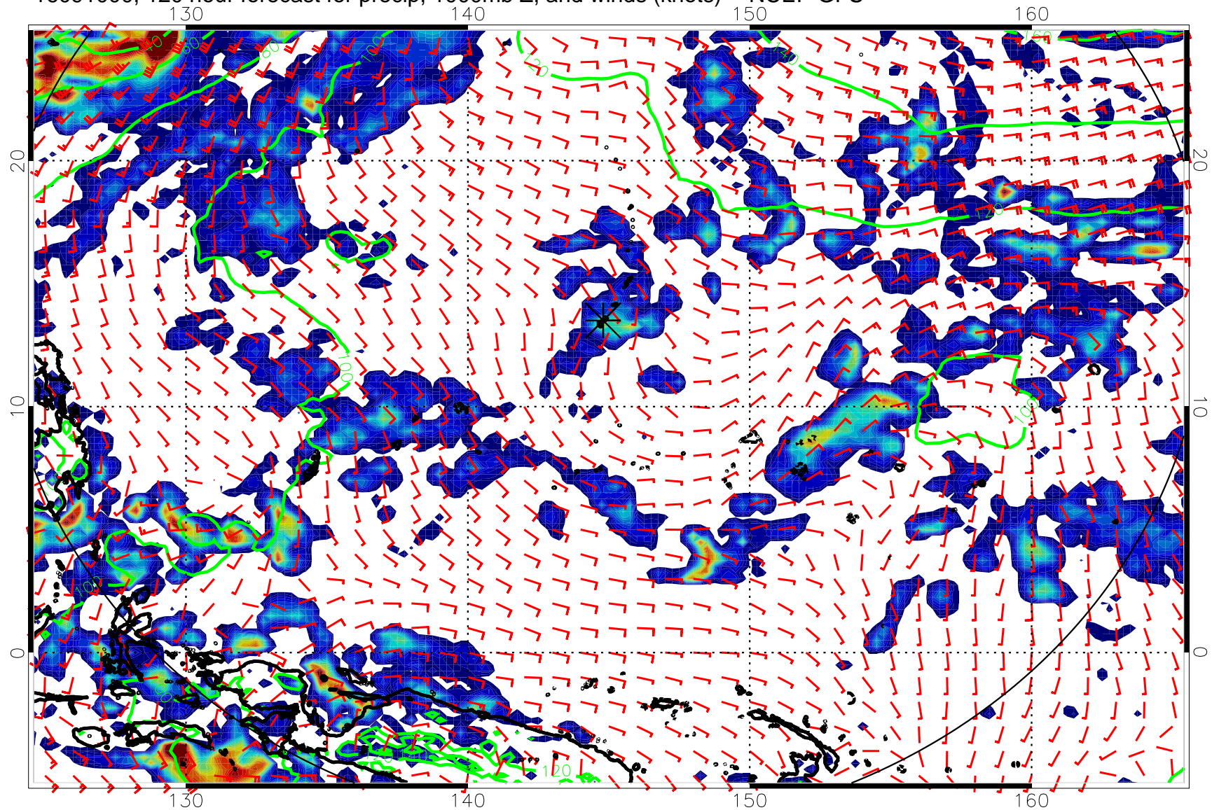
16091000, 120 hour forecast for precip, 1000mb Z, and winds (knots) -- NCEP GFS
