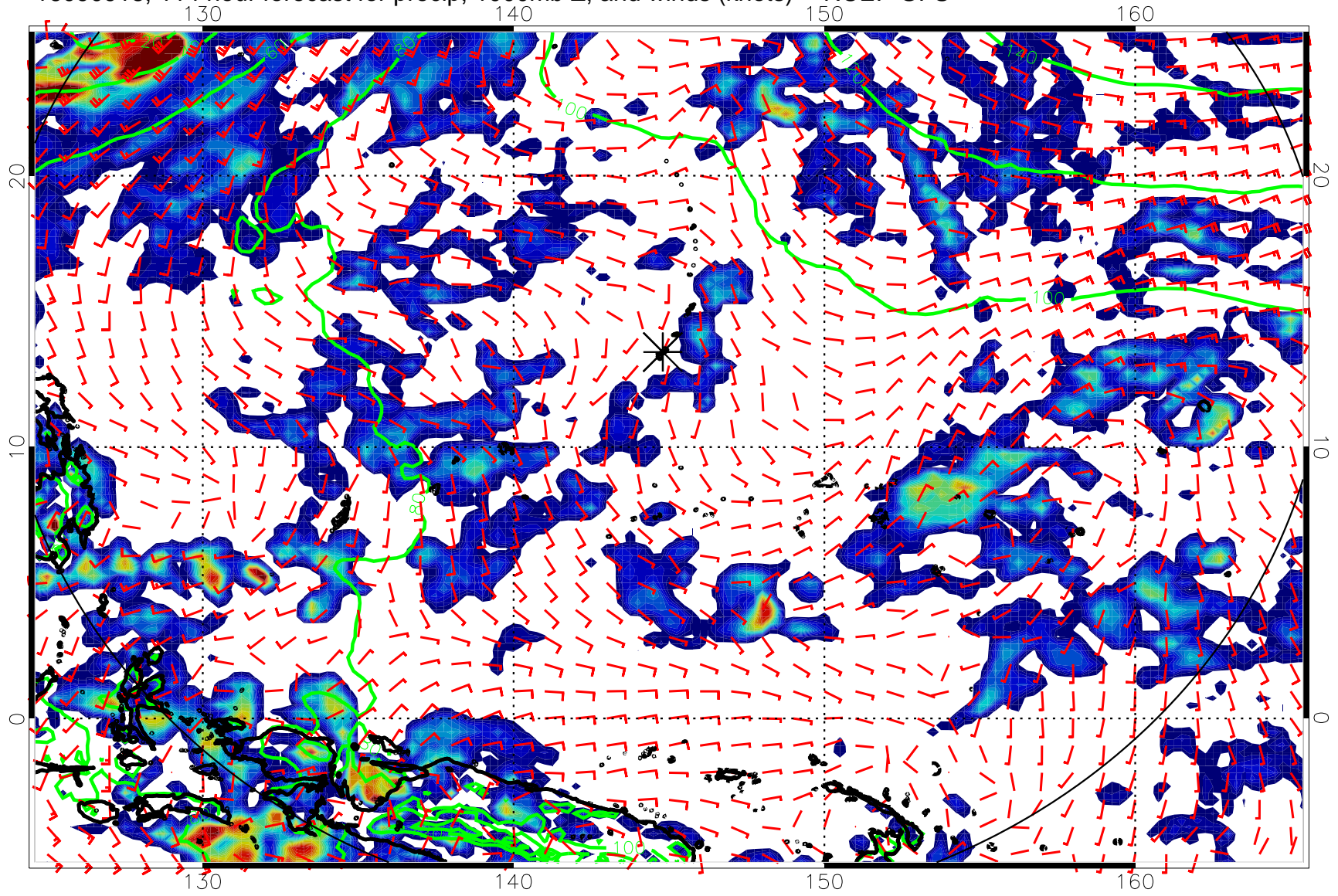
16090918, 114 hour forecast for precip, 1000mb Z, and winds (knots) -- NCEP GFS
