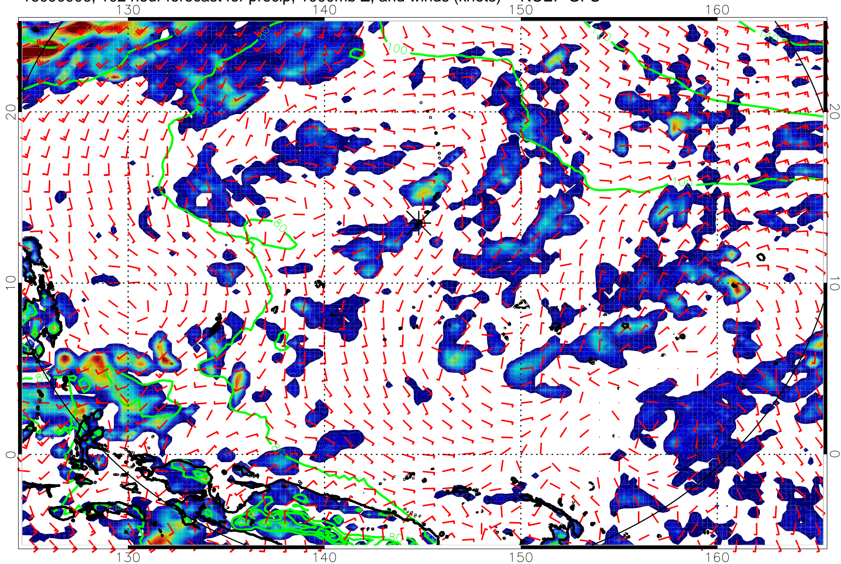
16090906, 102 hour forecast for precip, 1000mb Z, and winds (knots) -- NCEP GFS
