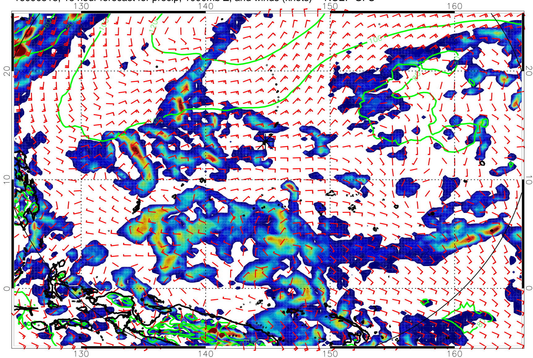
16090518, 18 hour forecast for precip, 1000mb Z, and winds (knots) -- NCEP GFS
