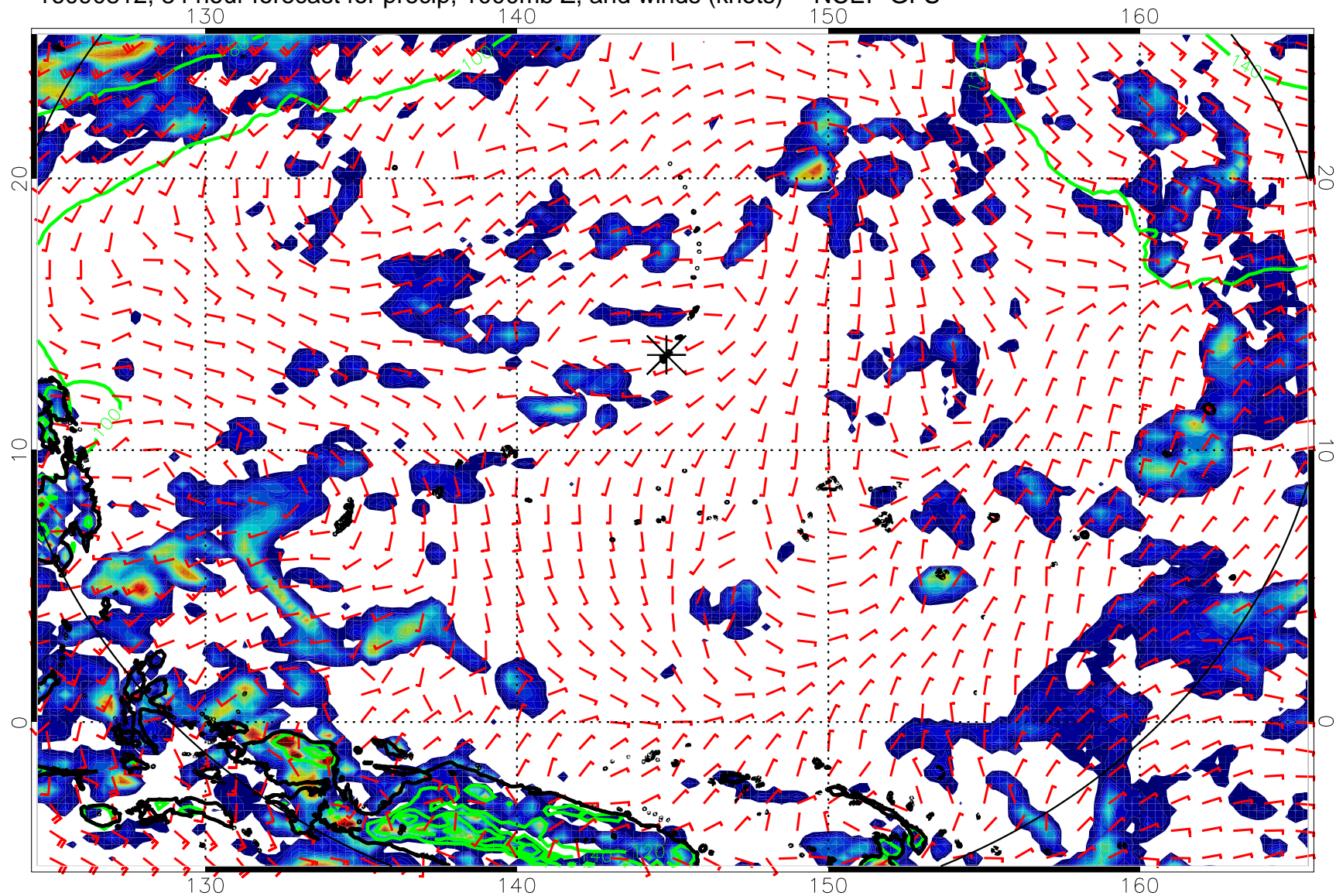
16090812, 84 hour forecast for precip, 1000mb Z, and winds (knots) -- NCEP GFS
