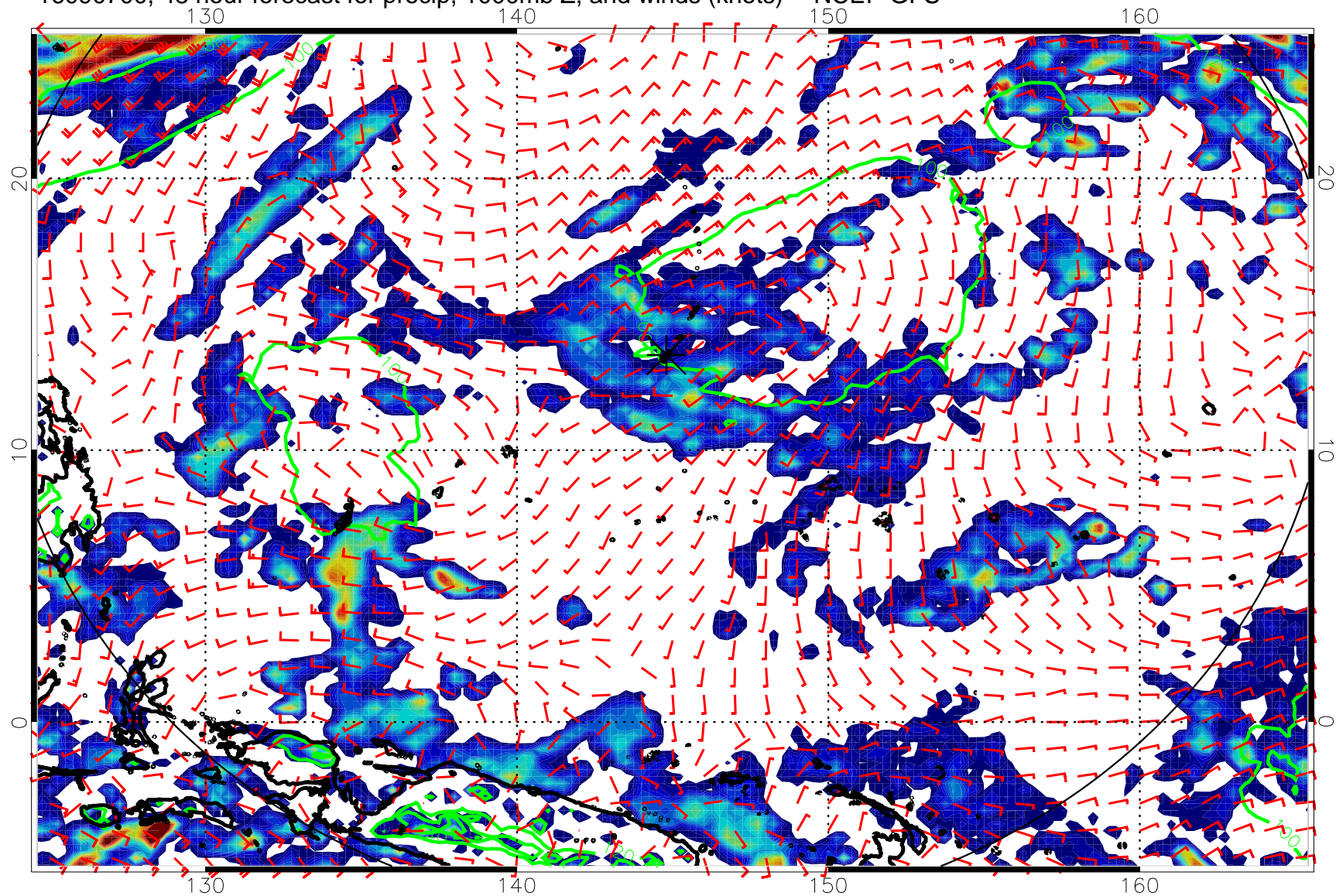
16090700, 48 hour forecast for precip, 1000mb Z, and winds (knots) -- NCEP GFS
