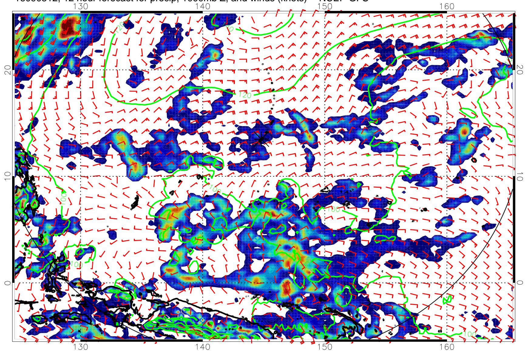
16090512, 12 hour forecast for precip, 1000mb Z, and winds (knots) -- NCEP GFS
