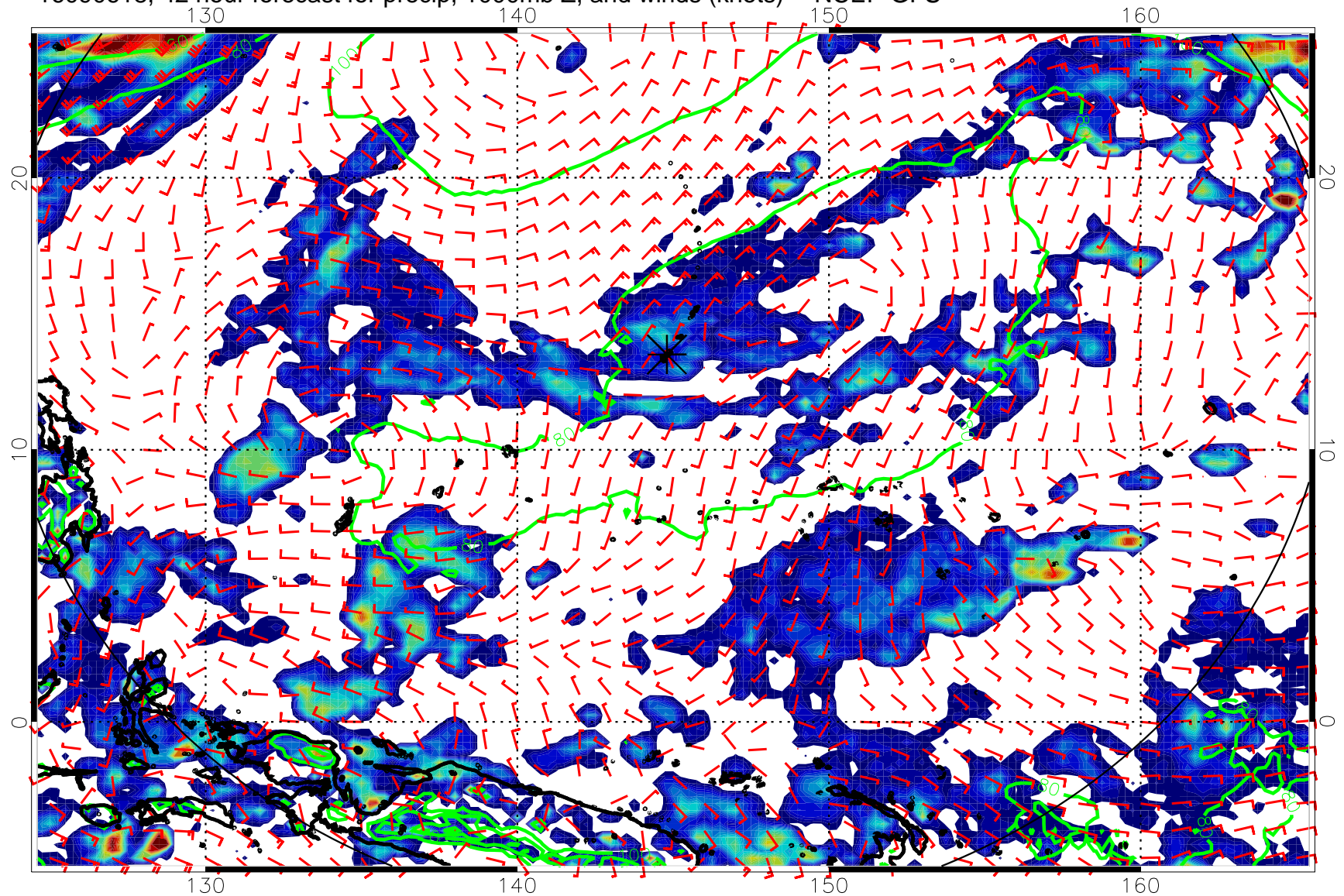
16090618, 42 hour forecast for precip, 1000mb Z, and winds (knots) -- NCEP GFS
