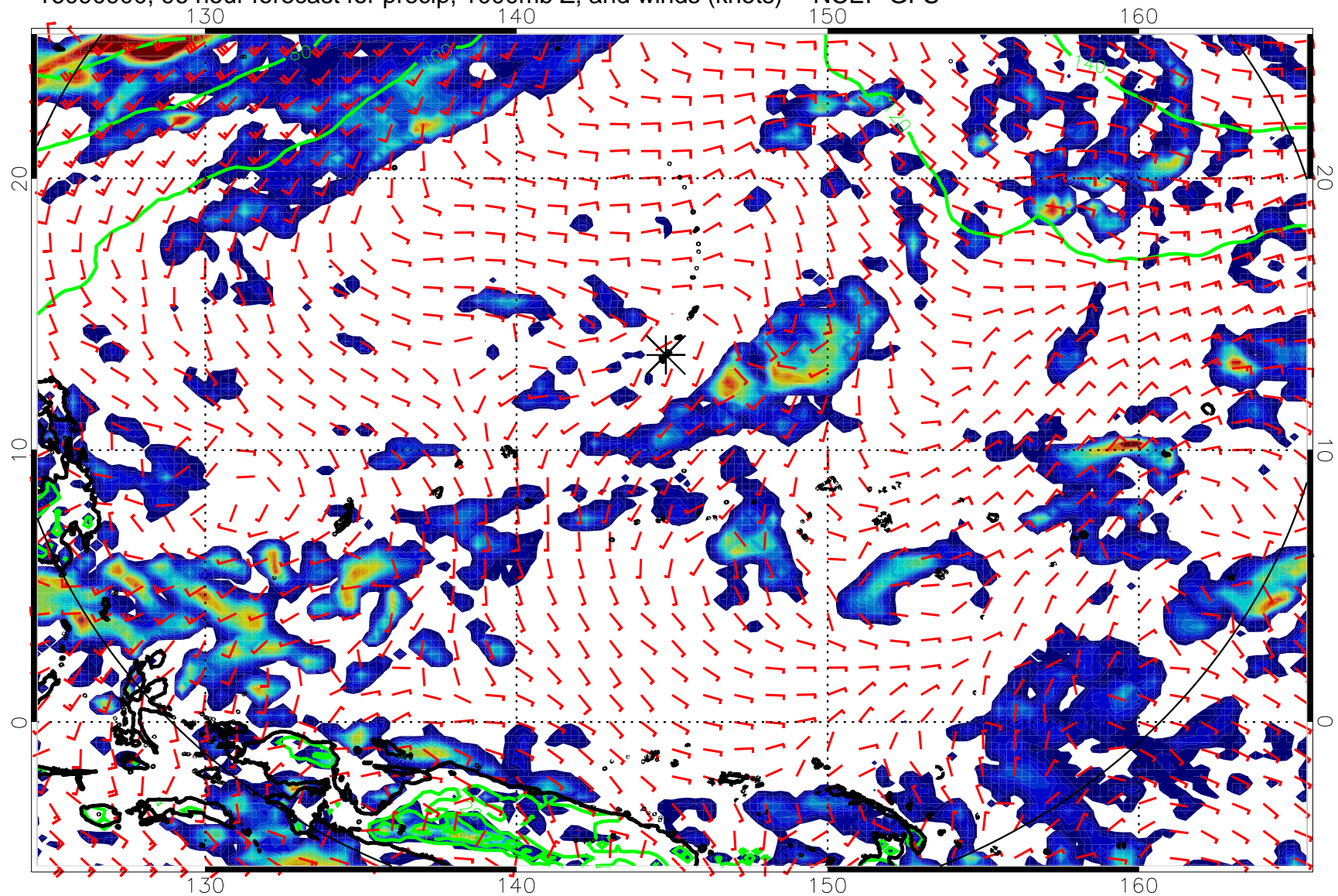
16090900, 96 hour forecast for precip, 1000mb Z, and winds (knots) -- NCEP GFS
