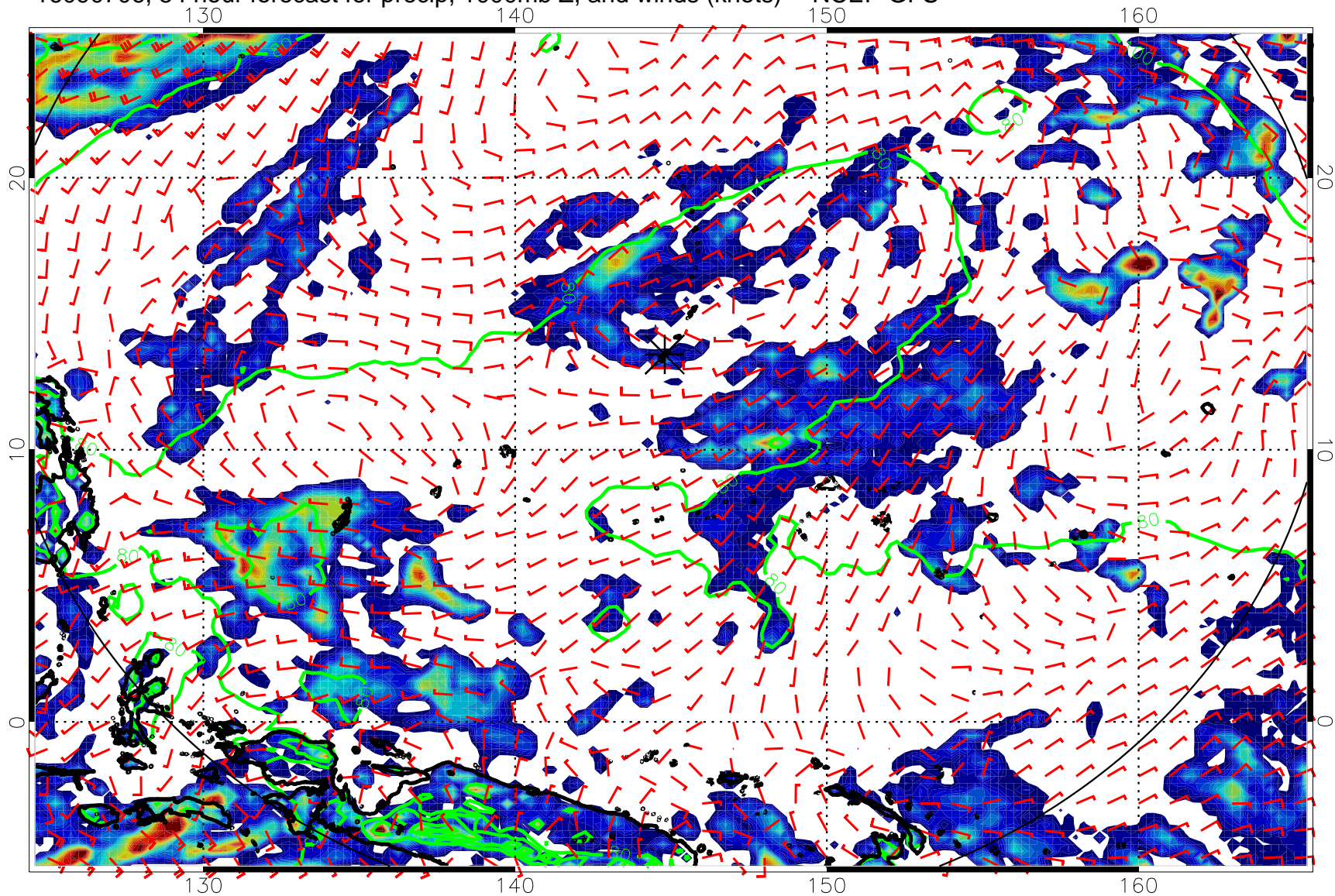
16090706, 54 hour forecast for precip, 1000mb Z, and winds (knots) -- NCEP GFS
