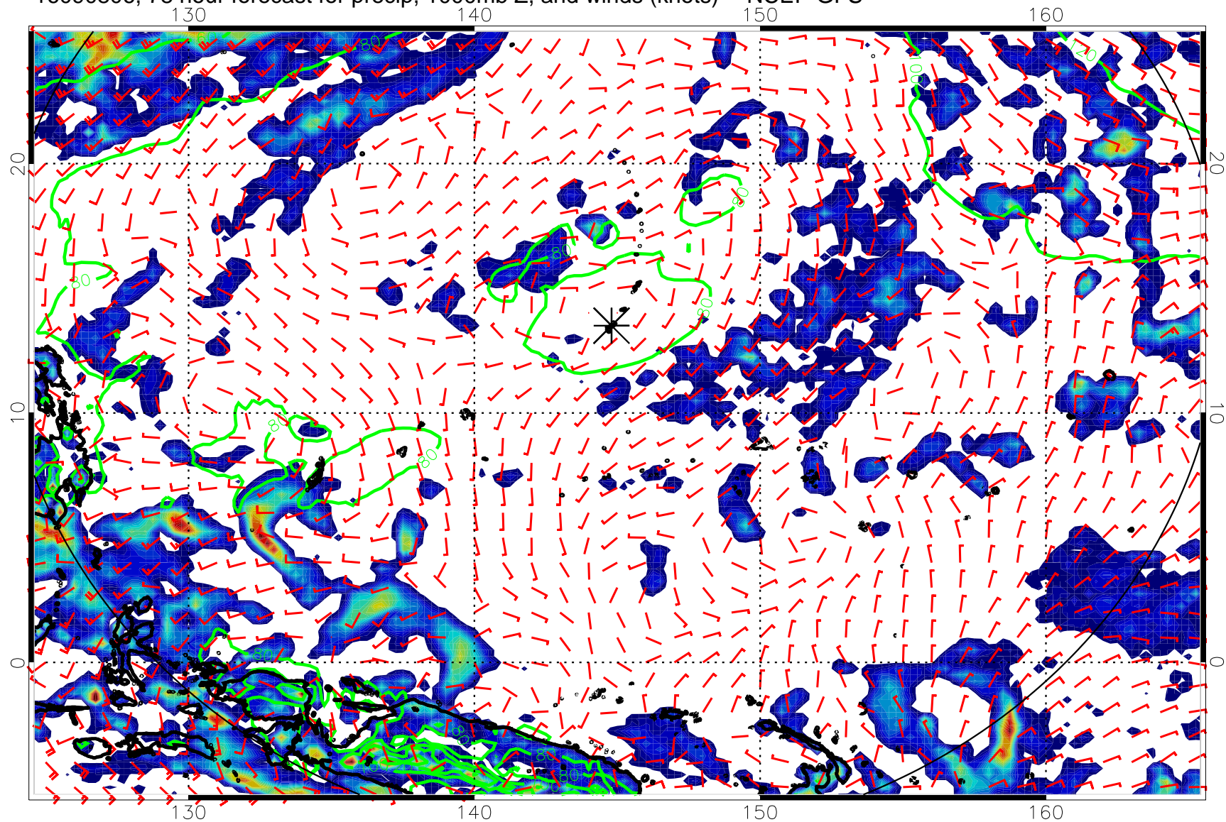
16090806, 78 hour forecast for precip, 1000mb Z, and winds (knots) -- NCEP GFS
