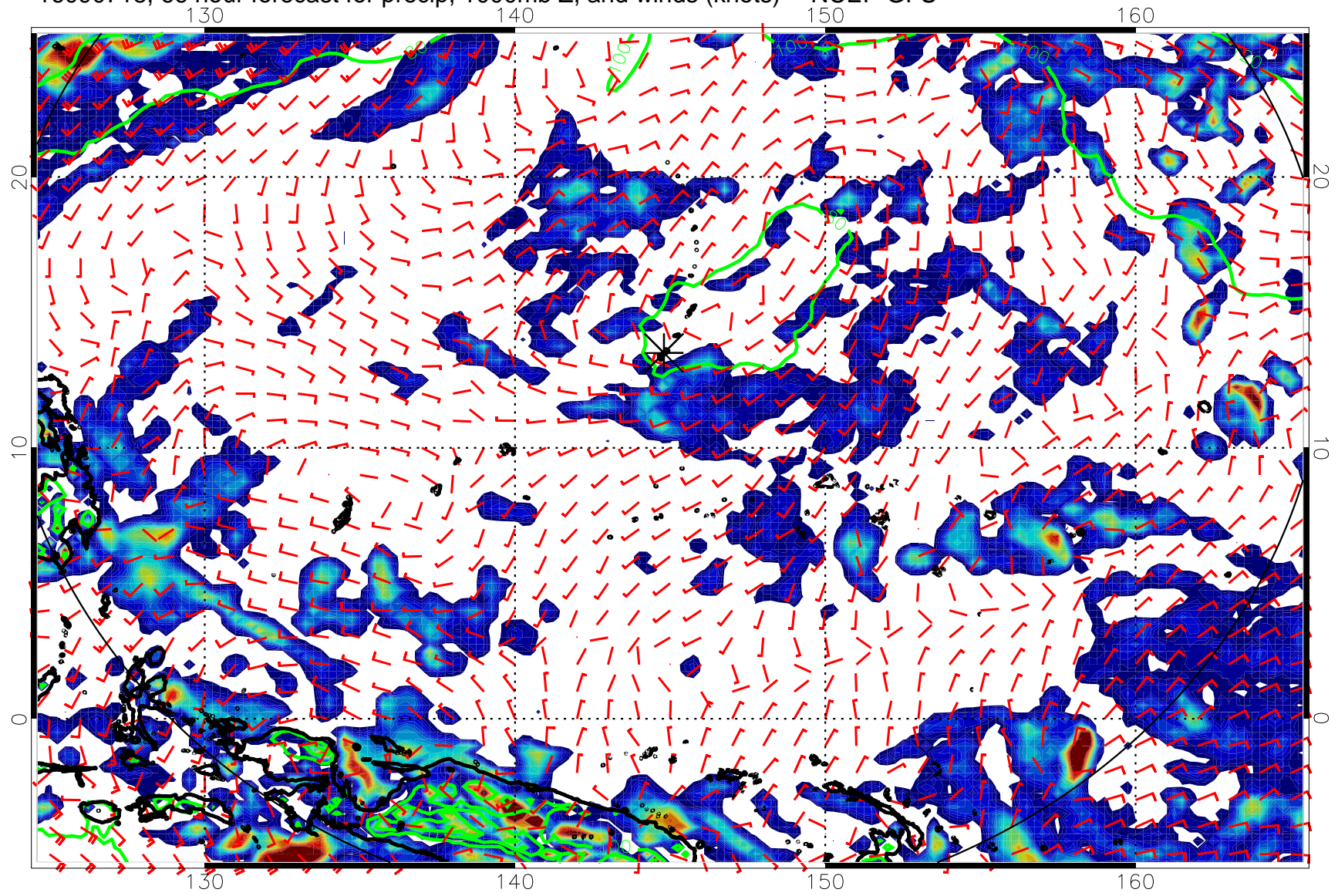
16090718, 66 hour forecast for precip, 1000mb Z, and winds (knots) -- NCEP GFS
