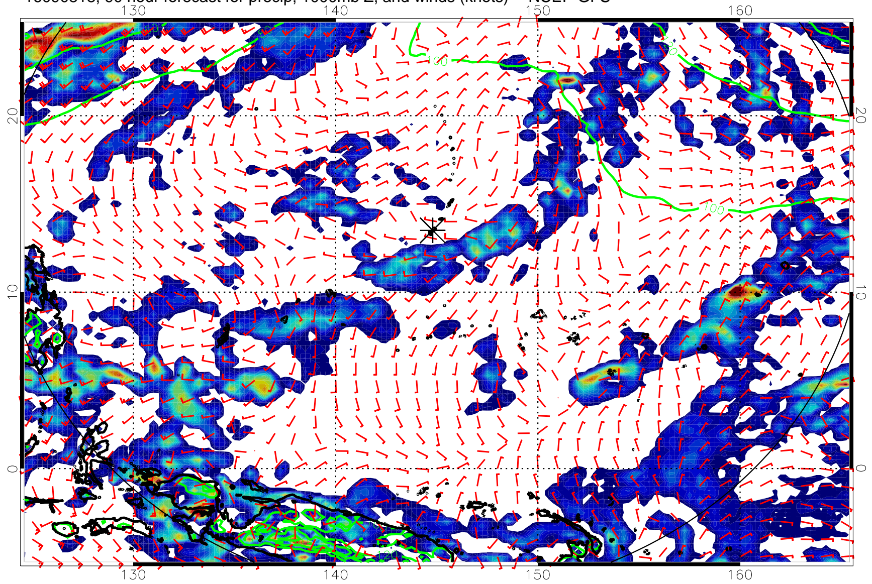
16090818, 90 hour forecast for precip, 1000mb Z, and winds (knots) -- NCEP GFS
