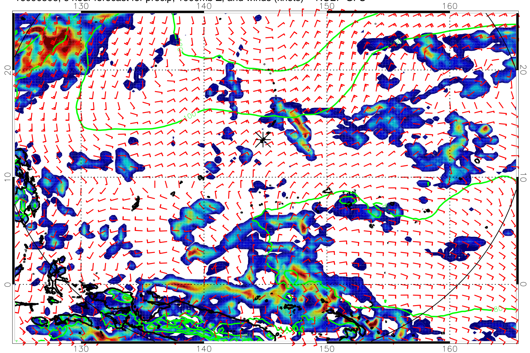
16090506, 6 hour forecast for precip, 1000mb Z, and winds (knots) -- NCEP GFS
