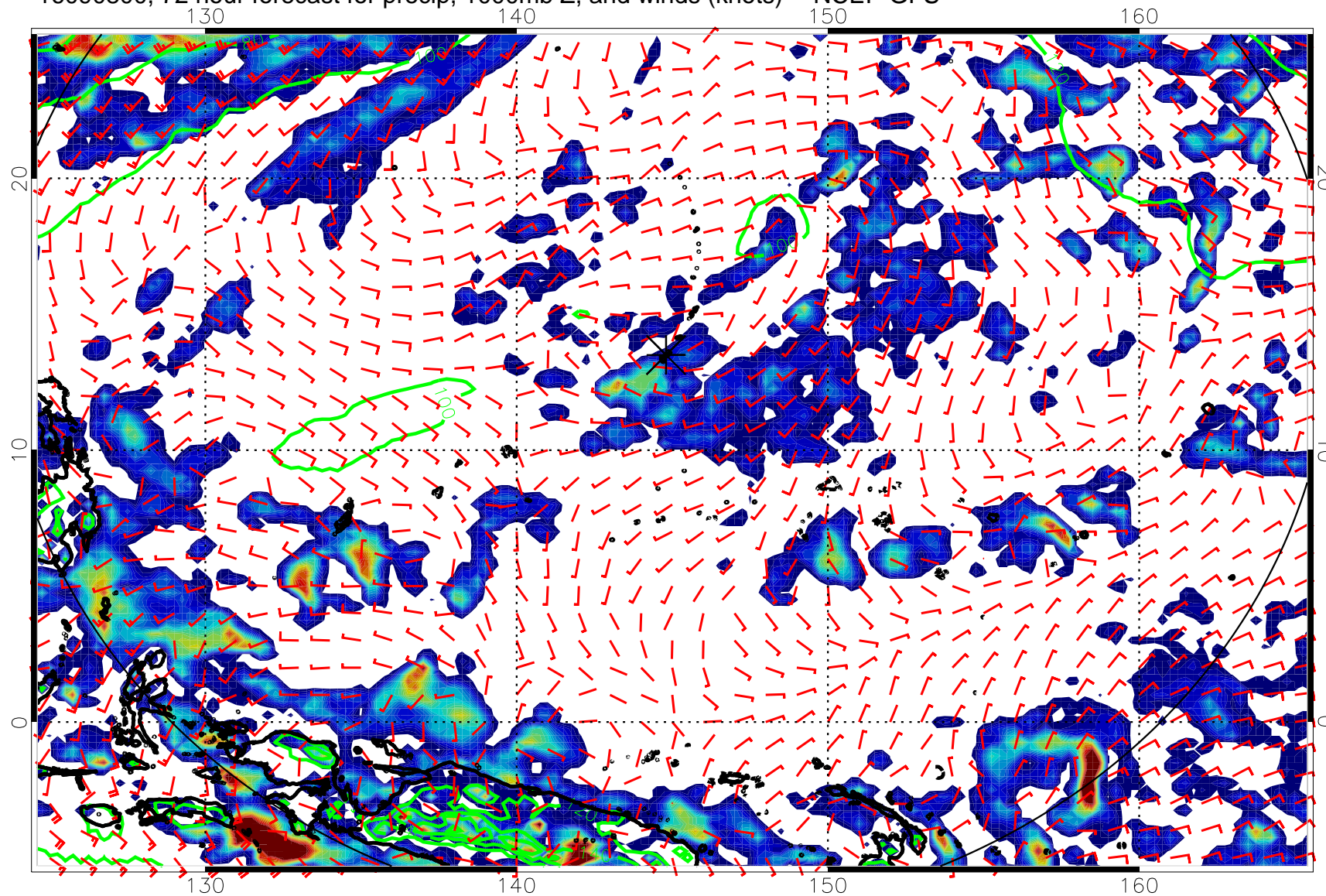
16090800, 72 hour forecast for precip, 1000mb Z, and winds (knots) -- NCEP GFS
