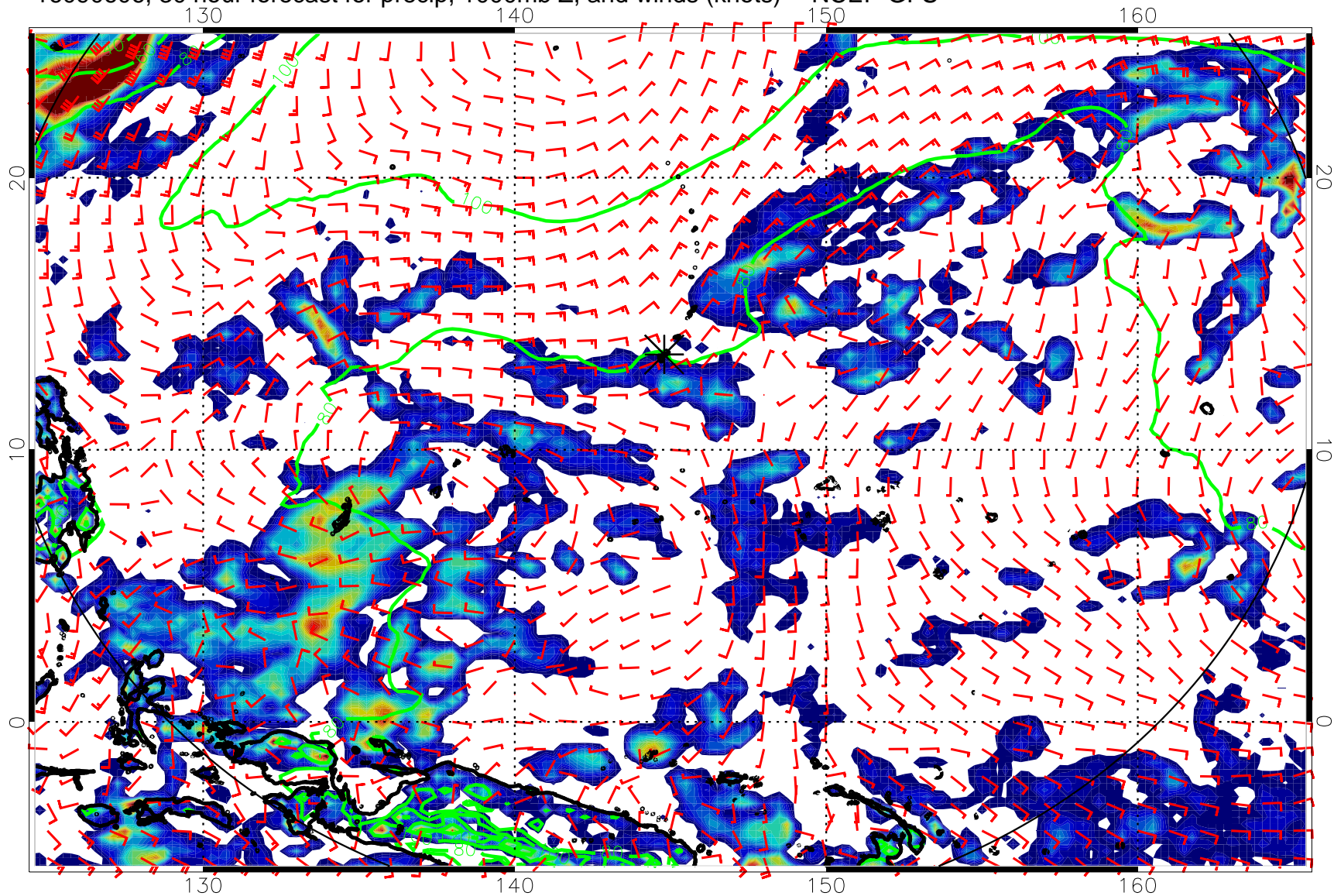
16090606, 30 hour forecast for precip, 1000mb Z, and winds (knots) -- NCEP GFS
