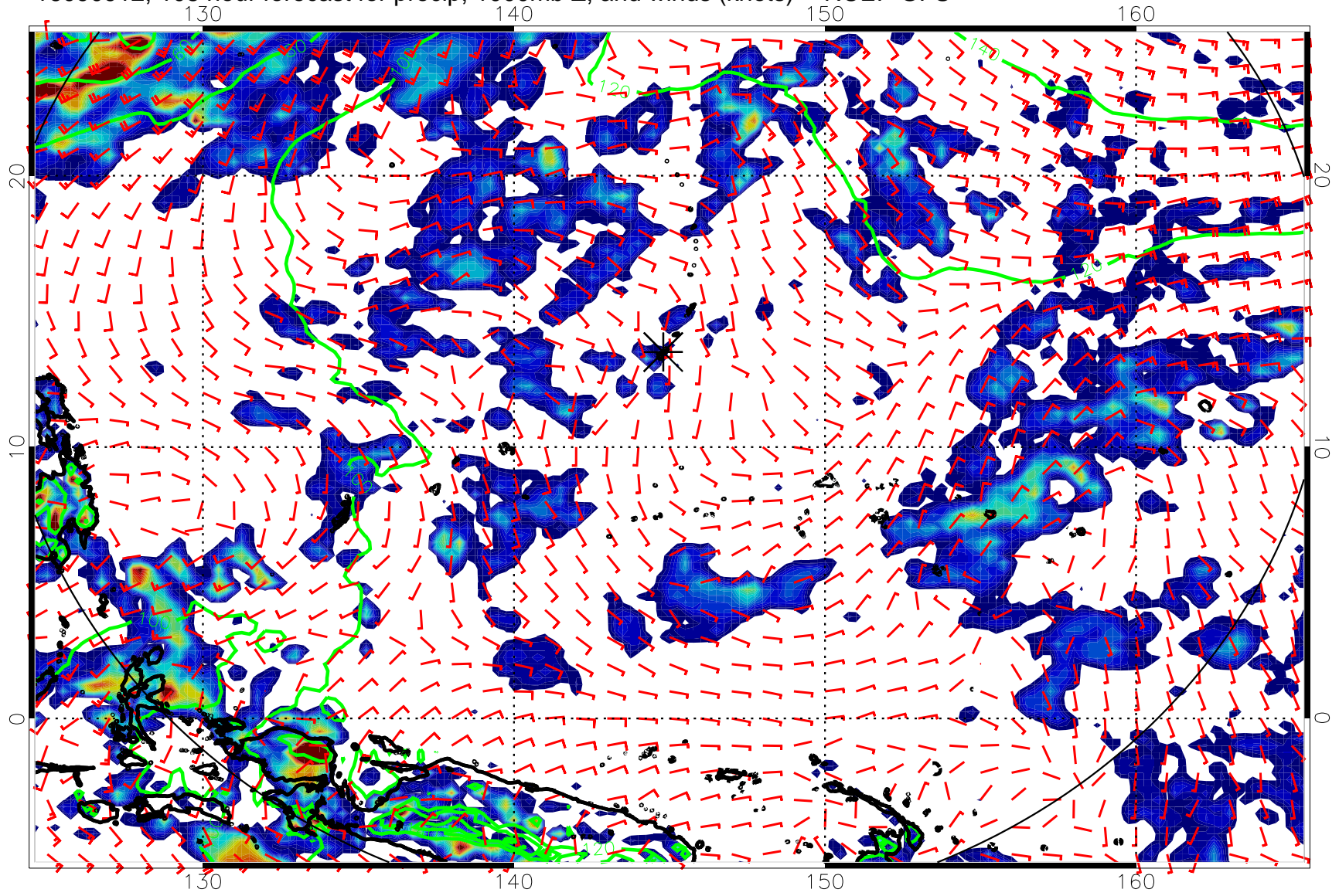
16090912, 108 hour forecast for precip, 1000mb Z, and winds (knots) -- NCEP GFS
