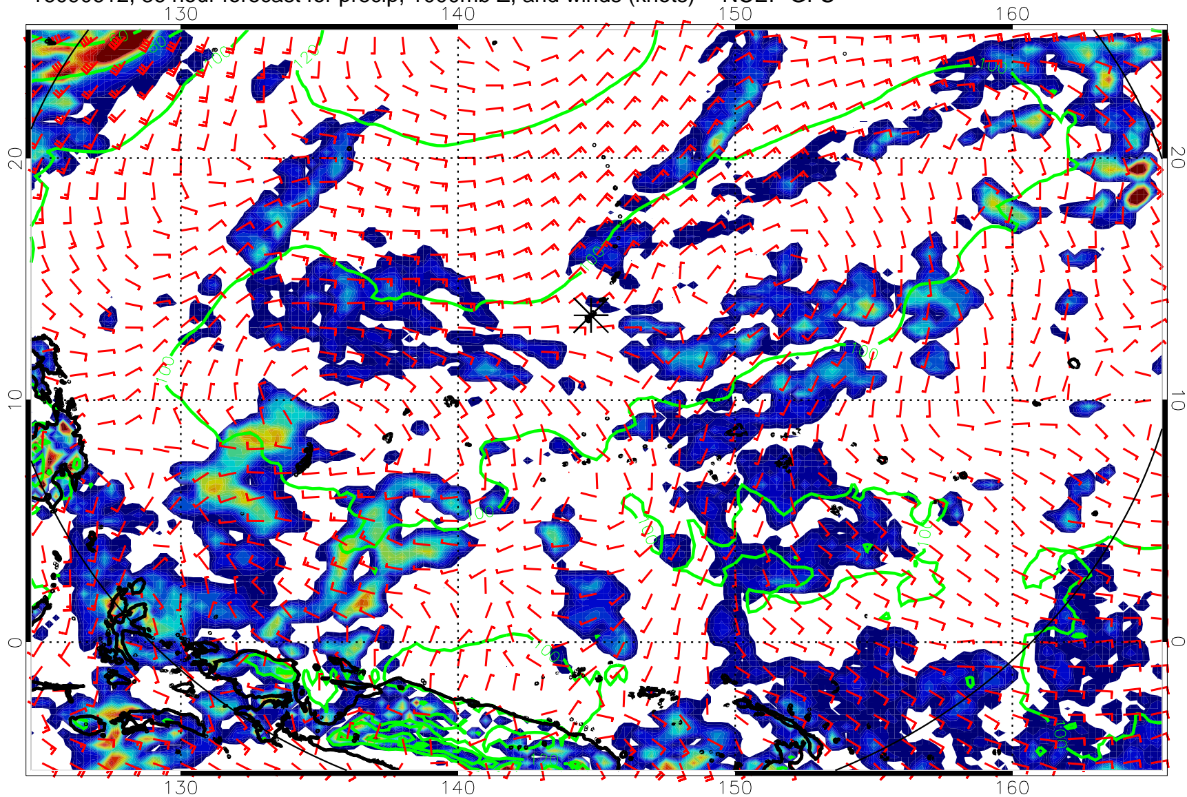
16090612, 36 hour forecast for precip, 1000mb Z, and winds (knots) -- NCEP GFS
