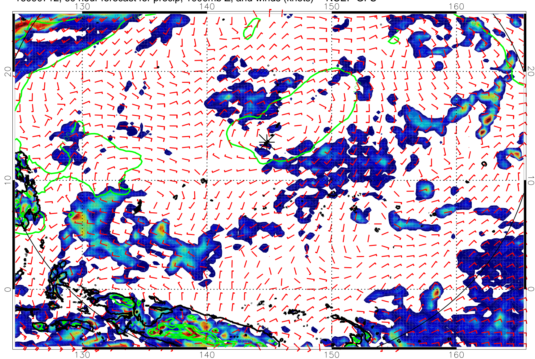
16090712, 60 hour forecast for precip, 1000mb Z, and winds (knots) -- NCEP GFS
