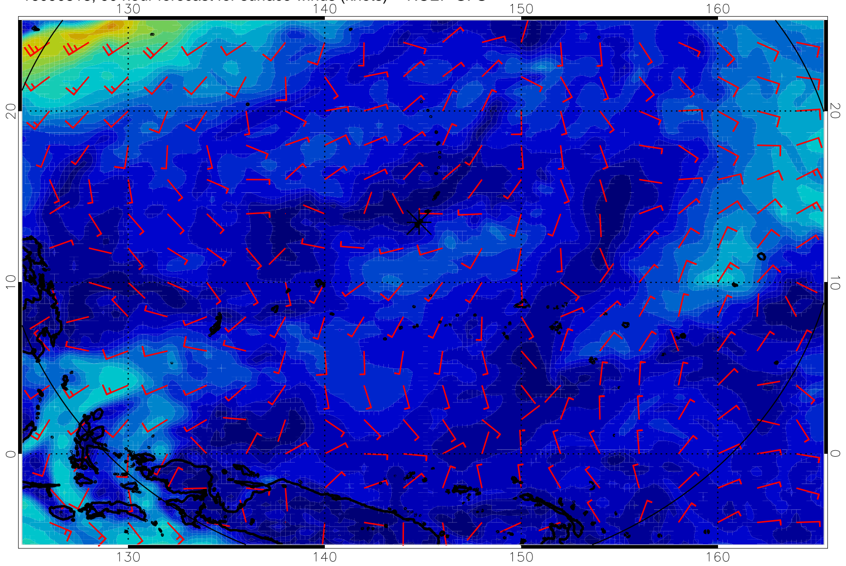
16090818, 90 hour forecast for surface winds (knots) -- NCEP GFS
