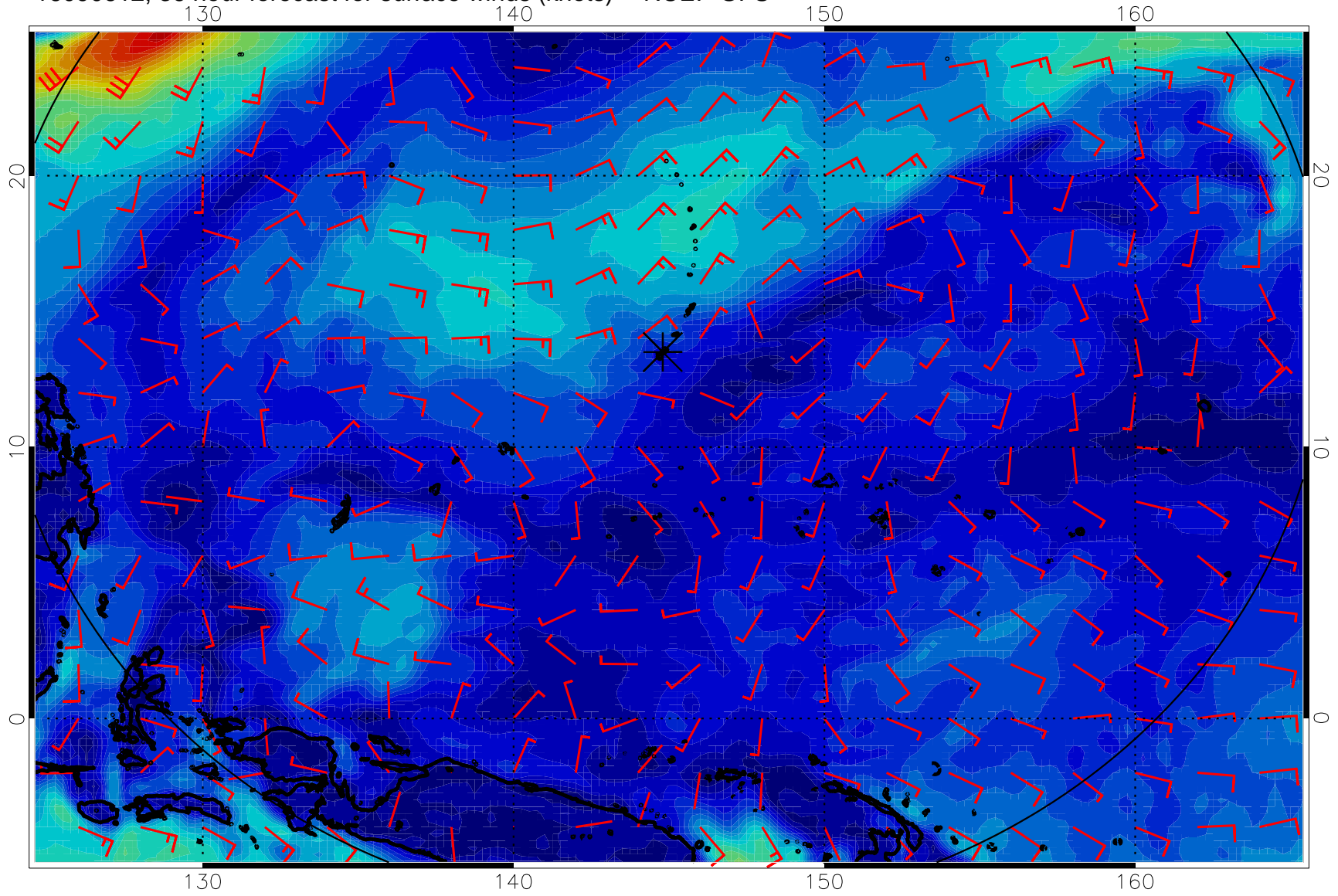
16090612, 36 hour forecast for surface winds (knots) -- NCEP GFS
