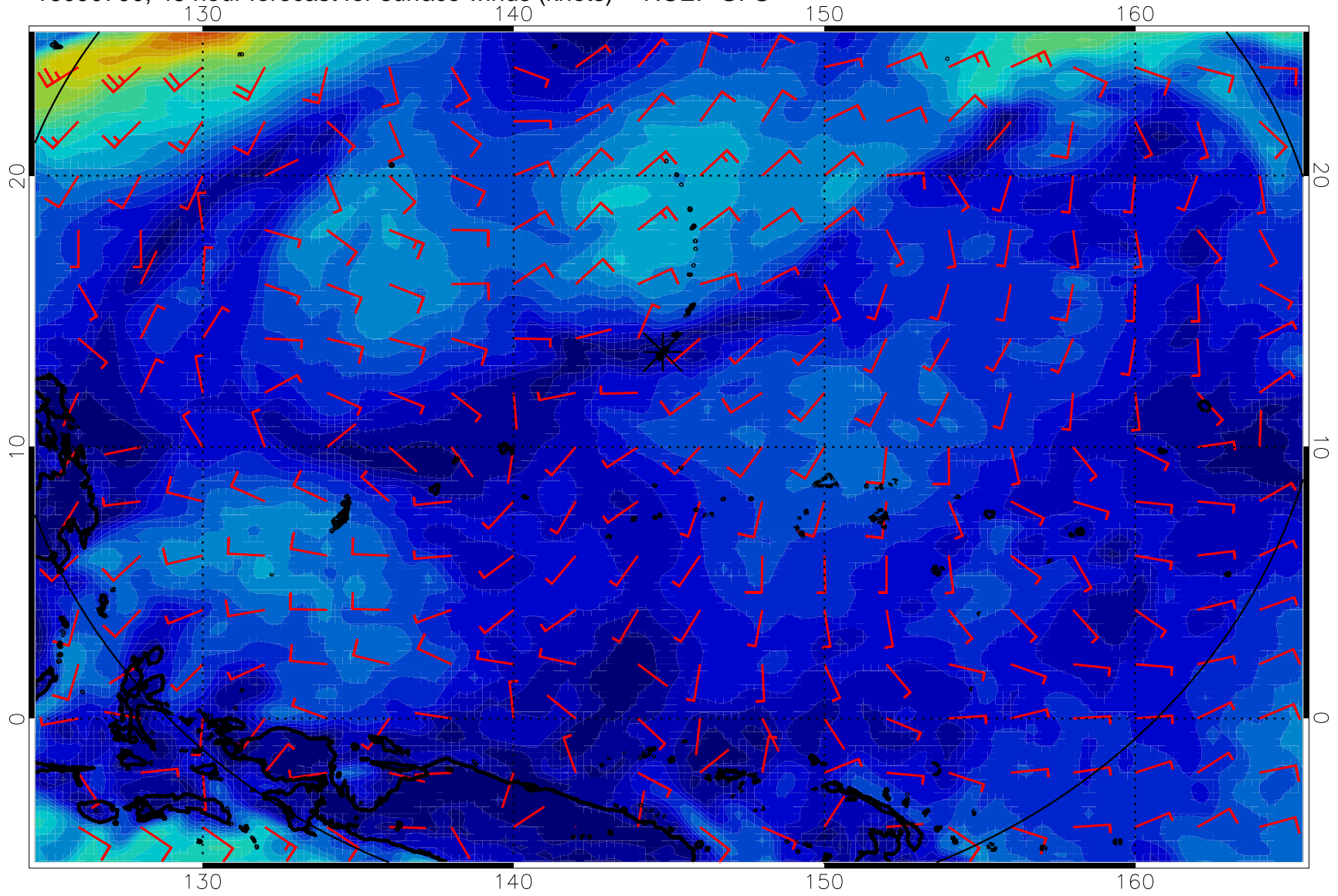
16090700, 48 hour forecast for surface winds (knots) -- NCEP GFS
