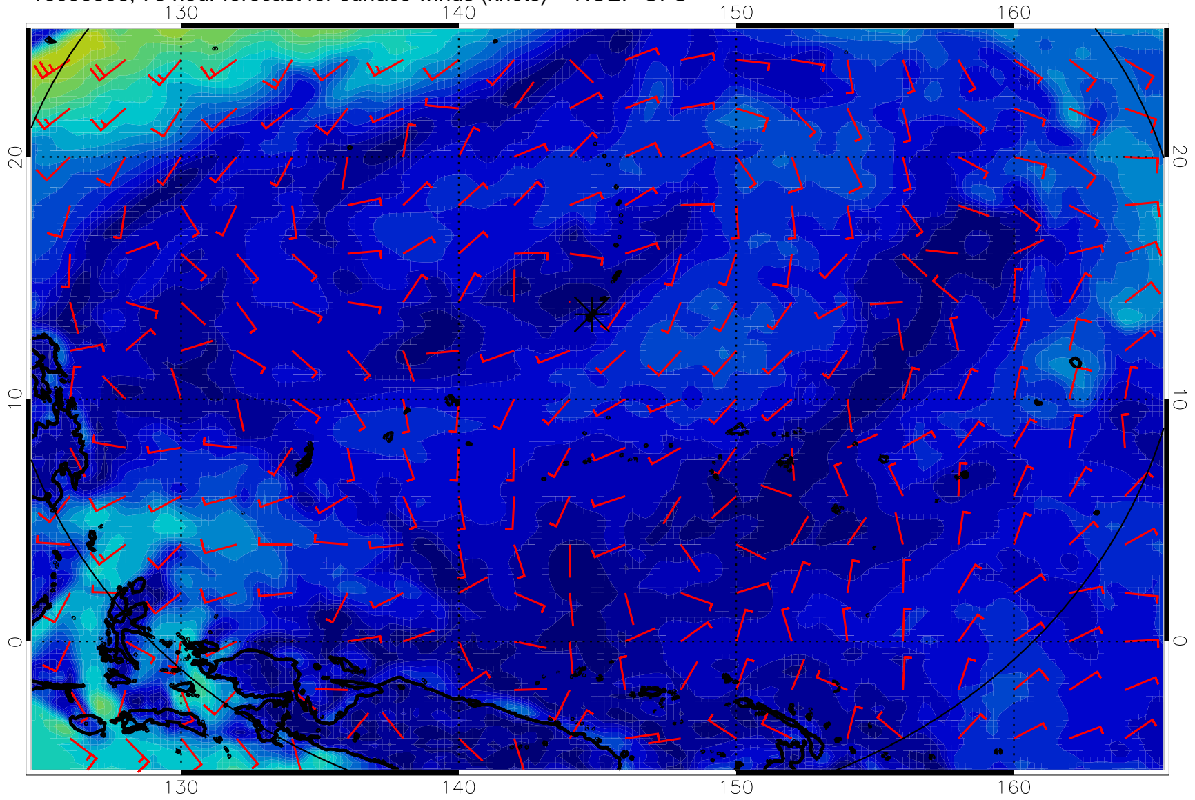
16090806, 78 hour forecast for surface winds (knots) -- NCEP GFS
