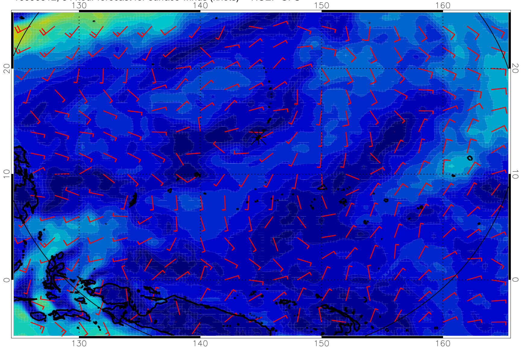
16090812, 84 hour forecast for surface winds (knots) -- NCEP GFS
