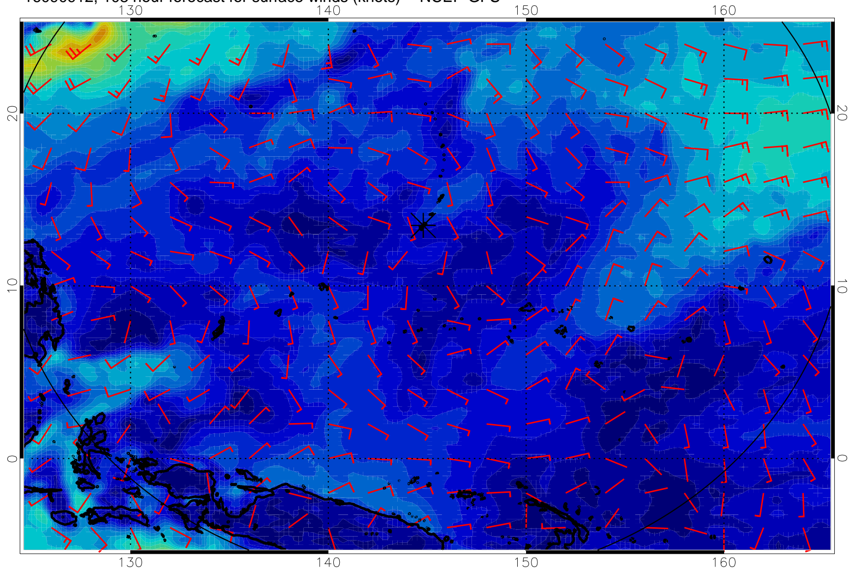
16090912, 108 hour forecast for surface winds (knots) -- NCEP GFS
