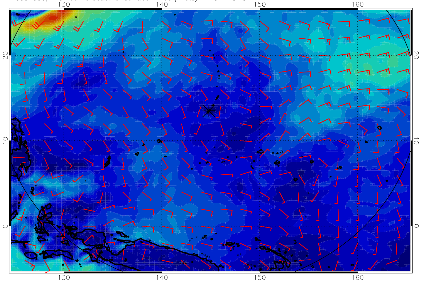
16091000, 120 hour forecast for surface winds (knots) -- NCEP GFS
