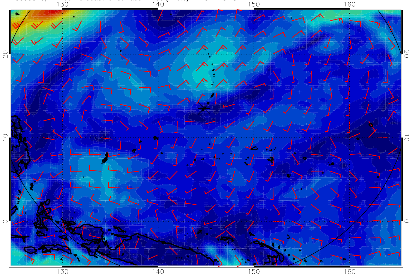
16090618, 42 hour forecast for surface winds (knots) -- NCEP GFS
