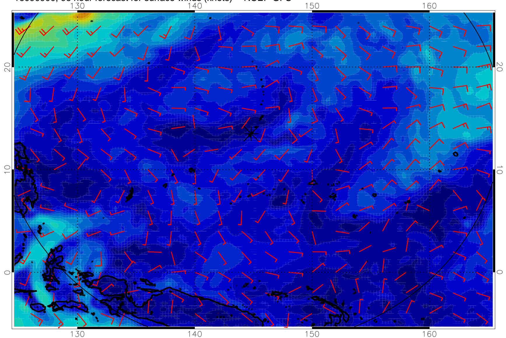
16090900, 96 hour forecast for surface winds (knots) -- NCEP GFS
