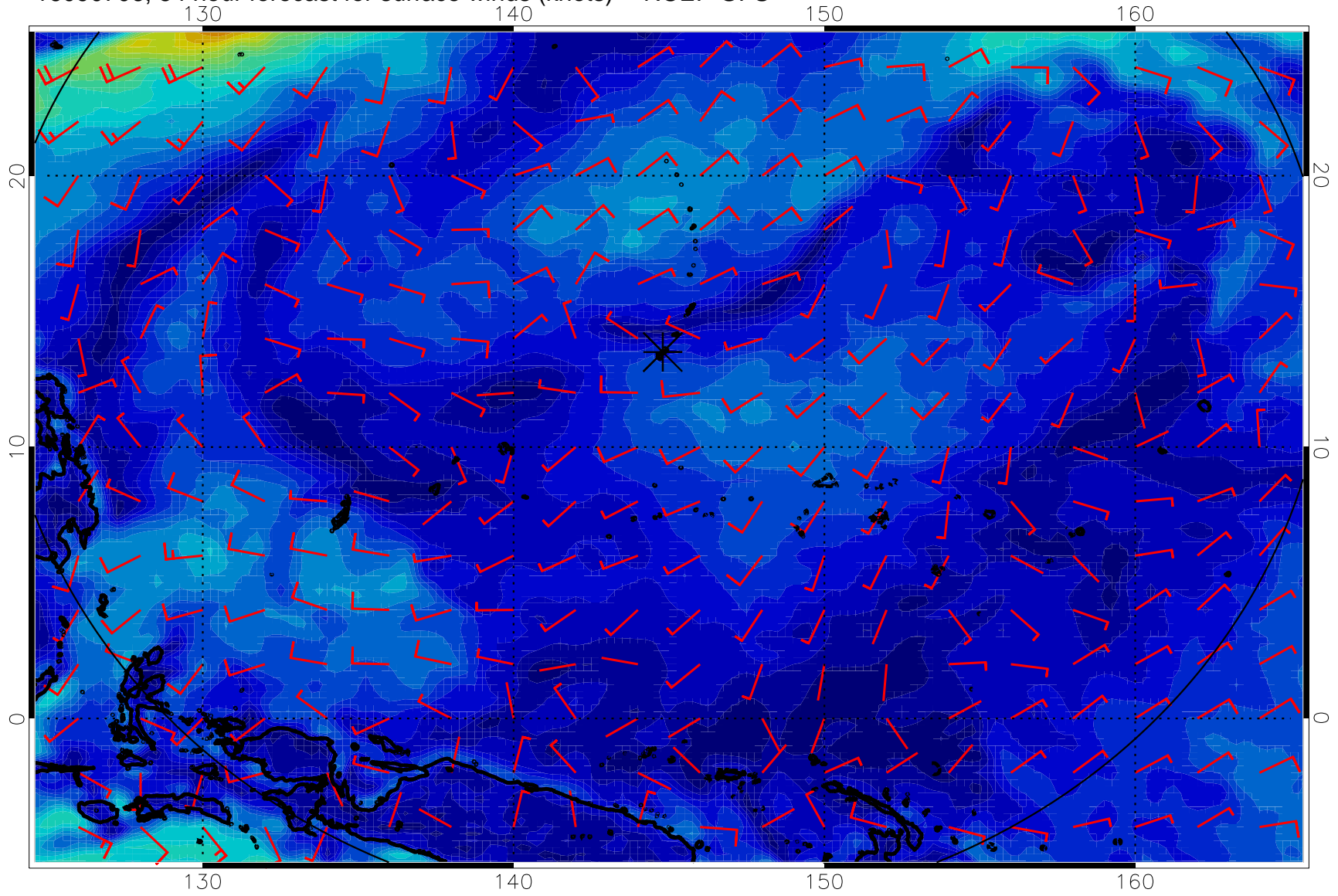
16090706, 54 hour forecast for surface winds (knots) -- NCEP GFS
