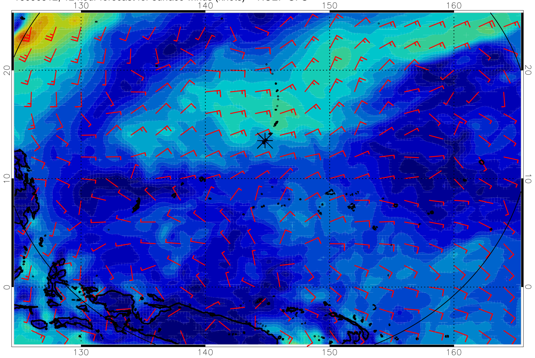
16090512, 12 hour forecast for surface winds (knots) -- NCEP GFS
