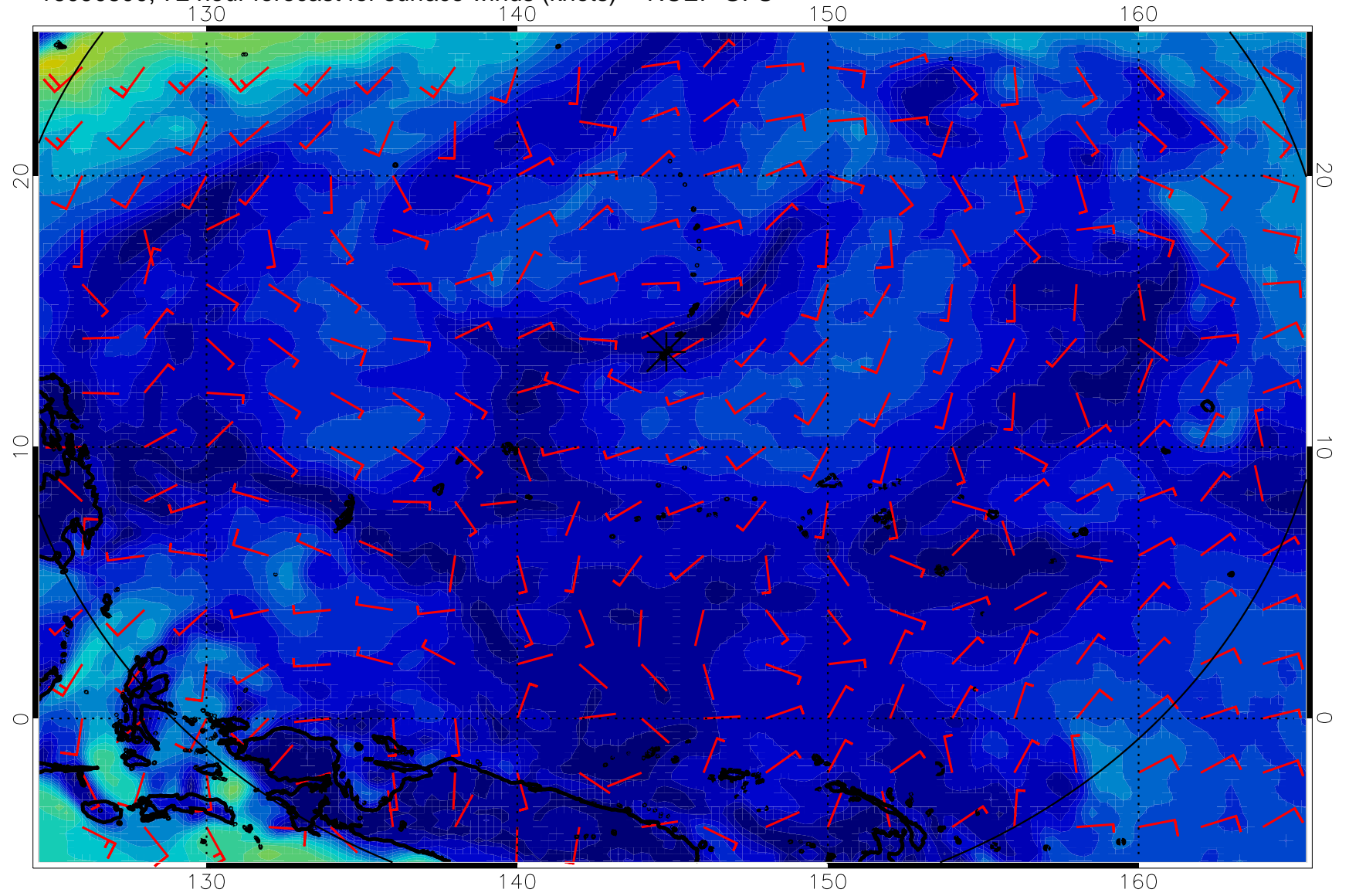
16090800, 72 hour forecast for surface winds (knots) -- NCEP GFS
