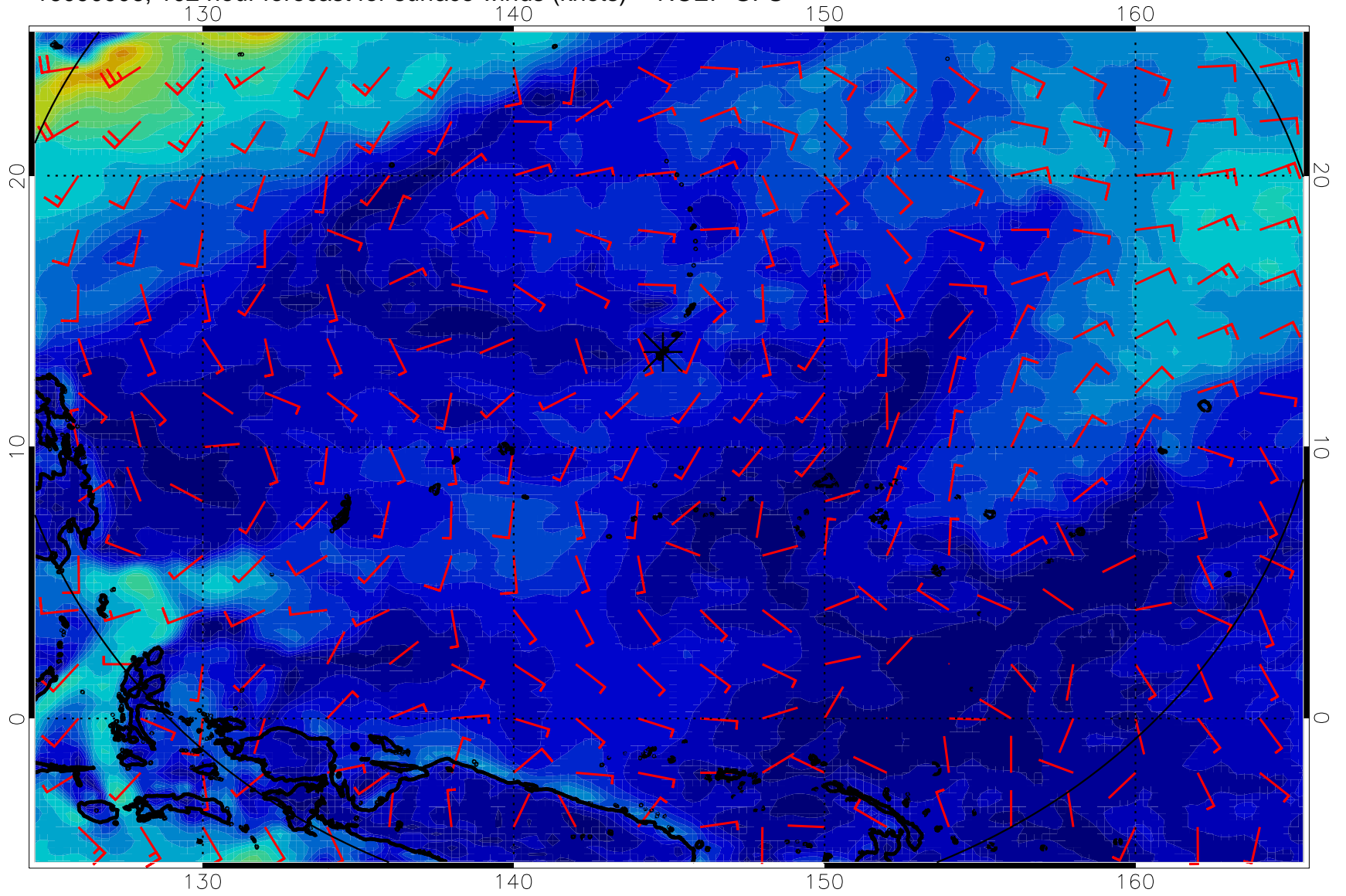
16090906, 102 hour forecast for surface winds (knots) -- NCEP GFS
