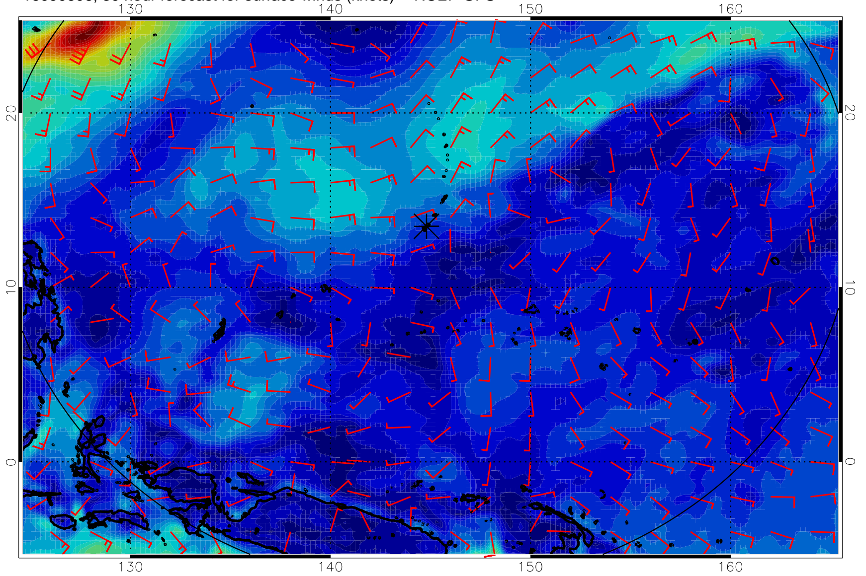
16090606, 30 hour forecast for surface winds (knots) -- NCEP GFS
