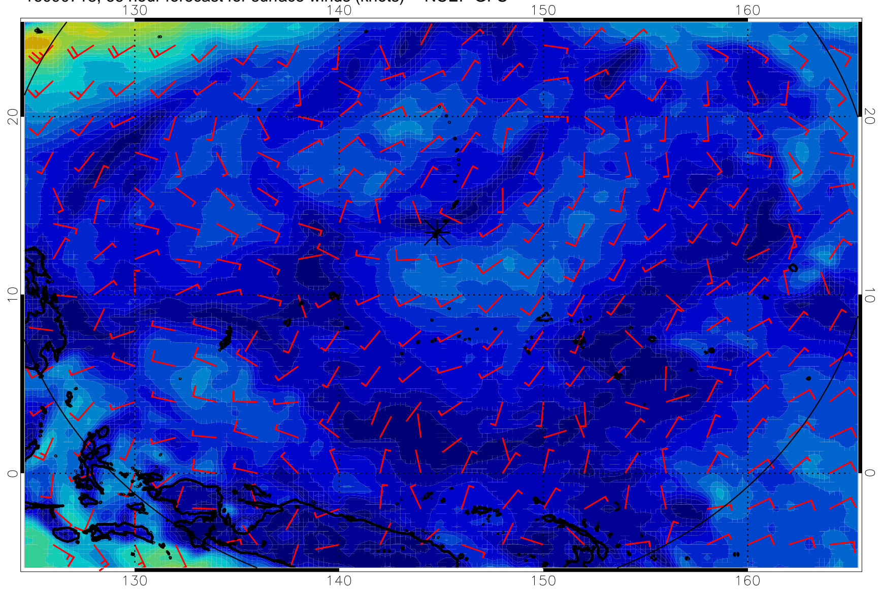
16090718, 66 hour forecast for surface winds (knots) -- NCEP GFS
