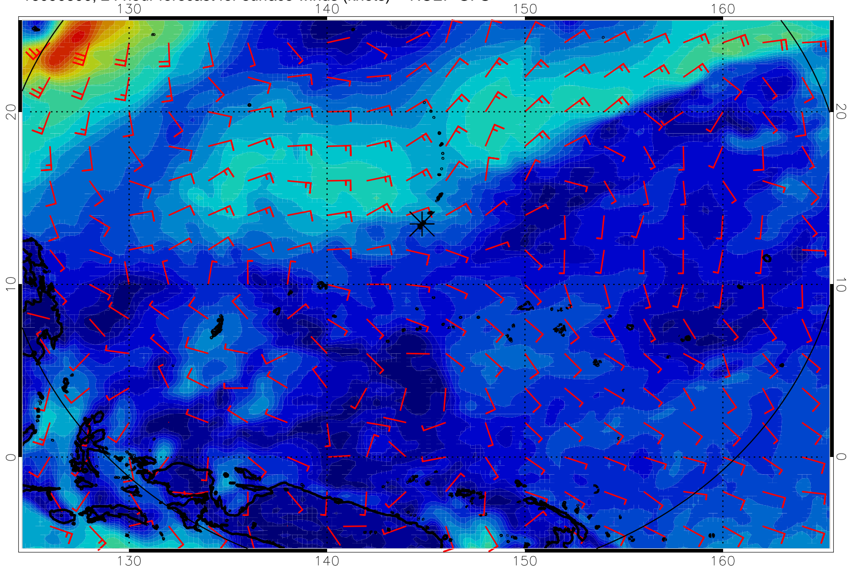
16090600, 24 hour forecast for surface winds (knots) -- NCEP GFS
