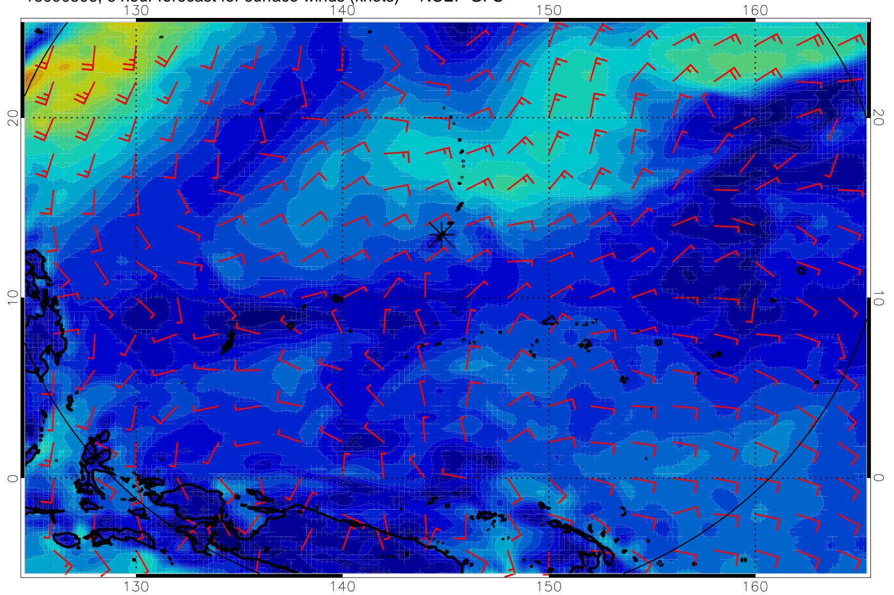
16090506, 6 hour forecast for surface winds (knots) -- NCEP GFS
