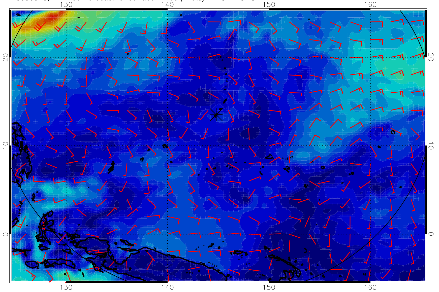
16090918, 114 hour forecast for surface winds (knots) -- NCEP GFS
