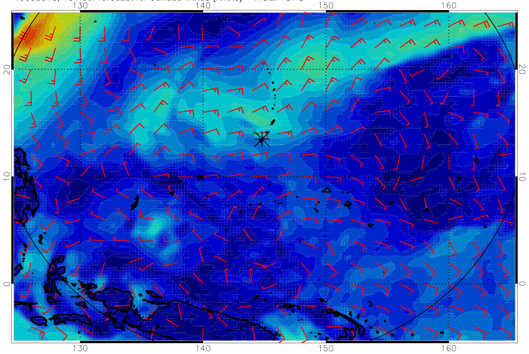
16090518, 18 hour forecast for surface winds (knots) -- NCEP GFS
