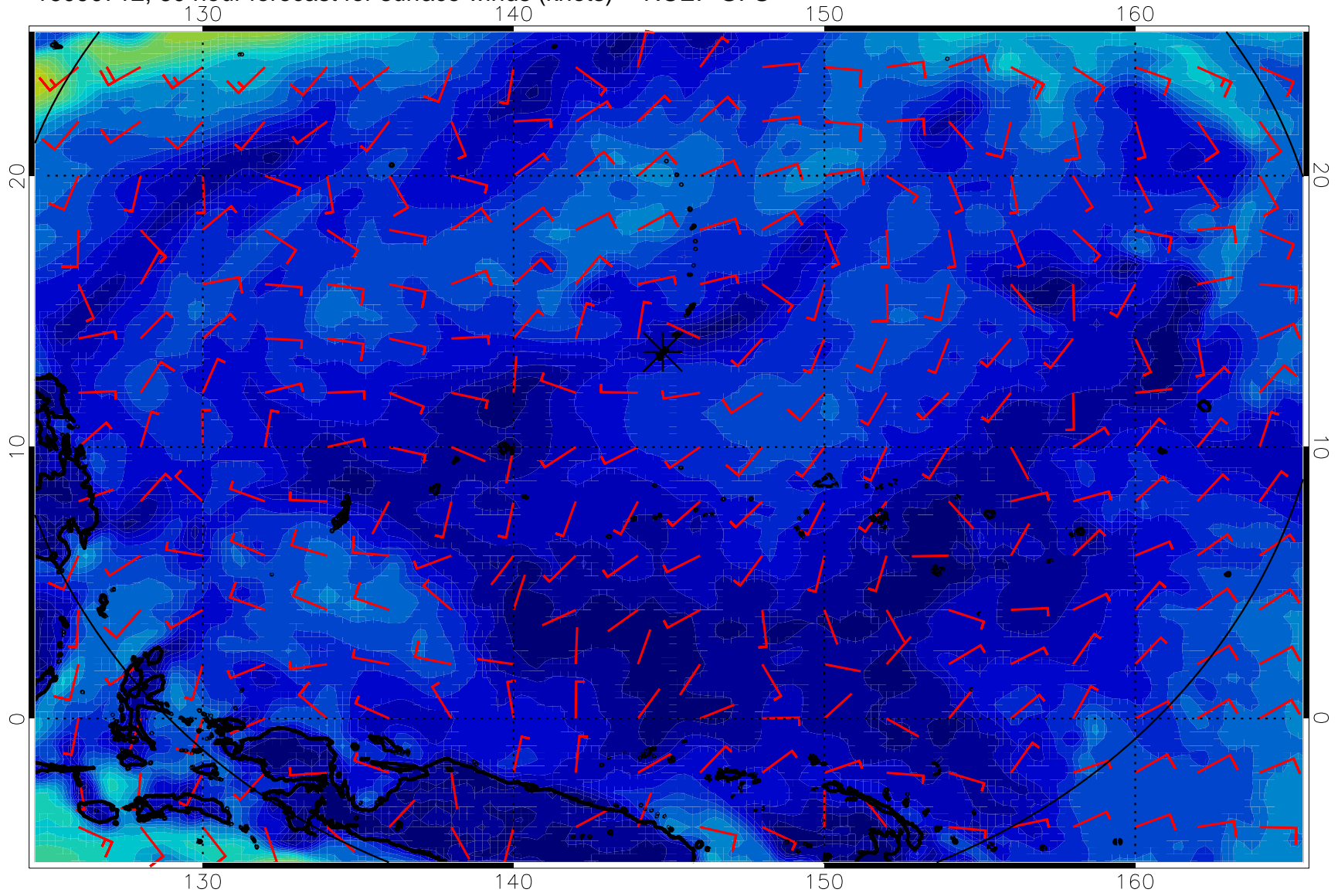
16090712, 60 hour forecast for surface winds (knots) -- NCEP GFS
