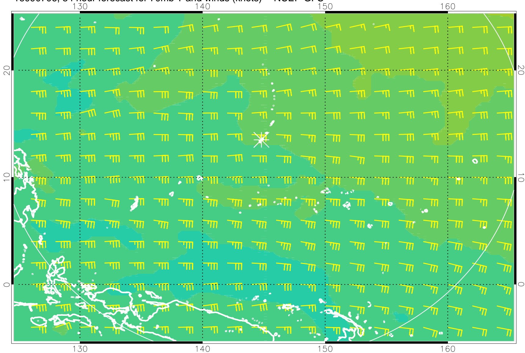
16090706, 54 hour forecast for 70mb T and winds (knots) -- NCEP GFS
