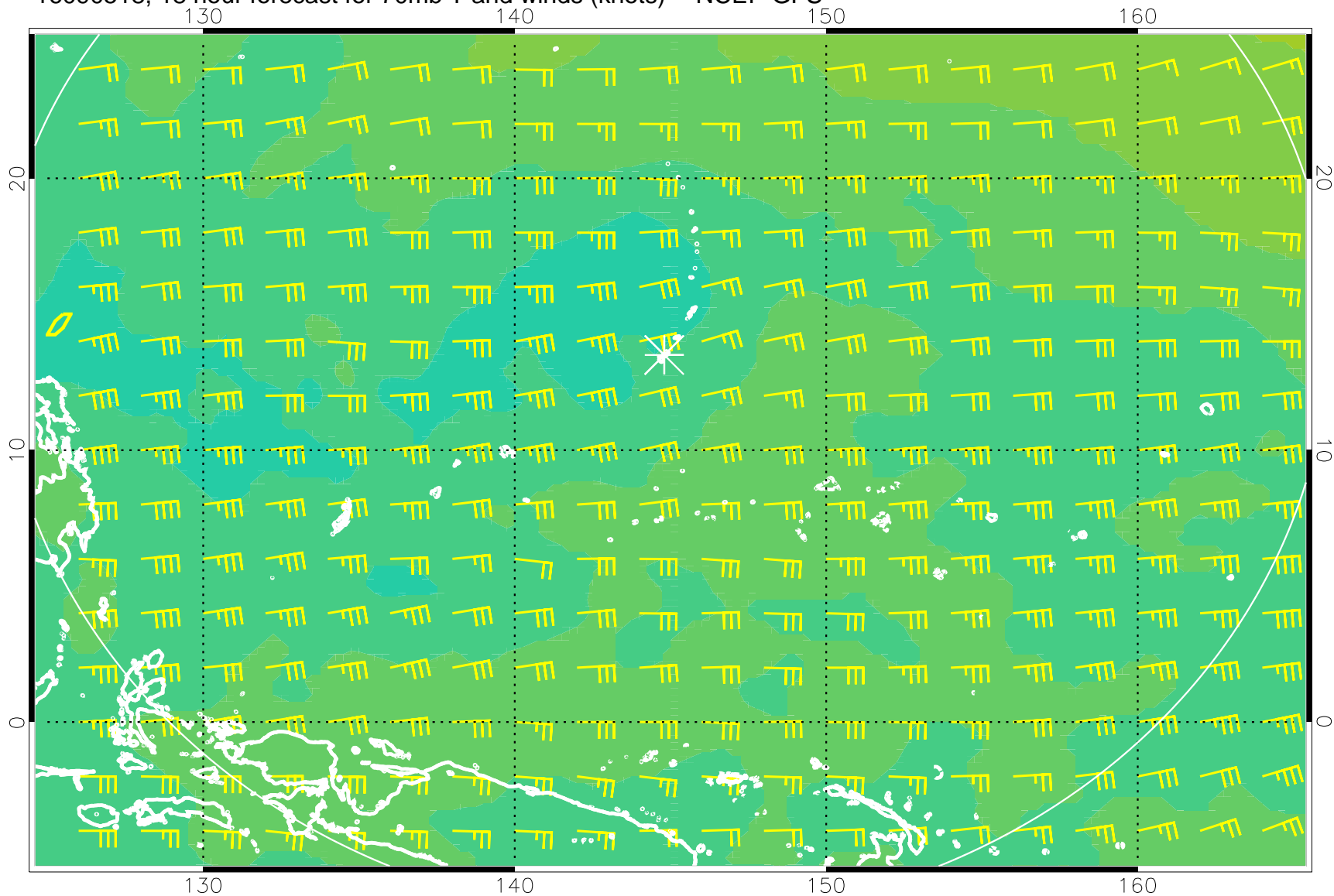
16090518, 18 hour forecast for 70mb T and winds (knots) -- NCEP GFS
