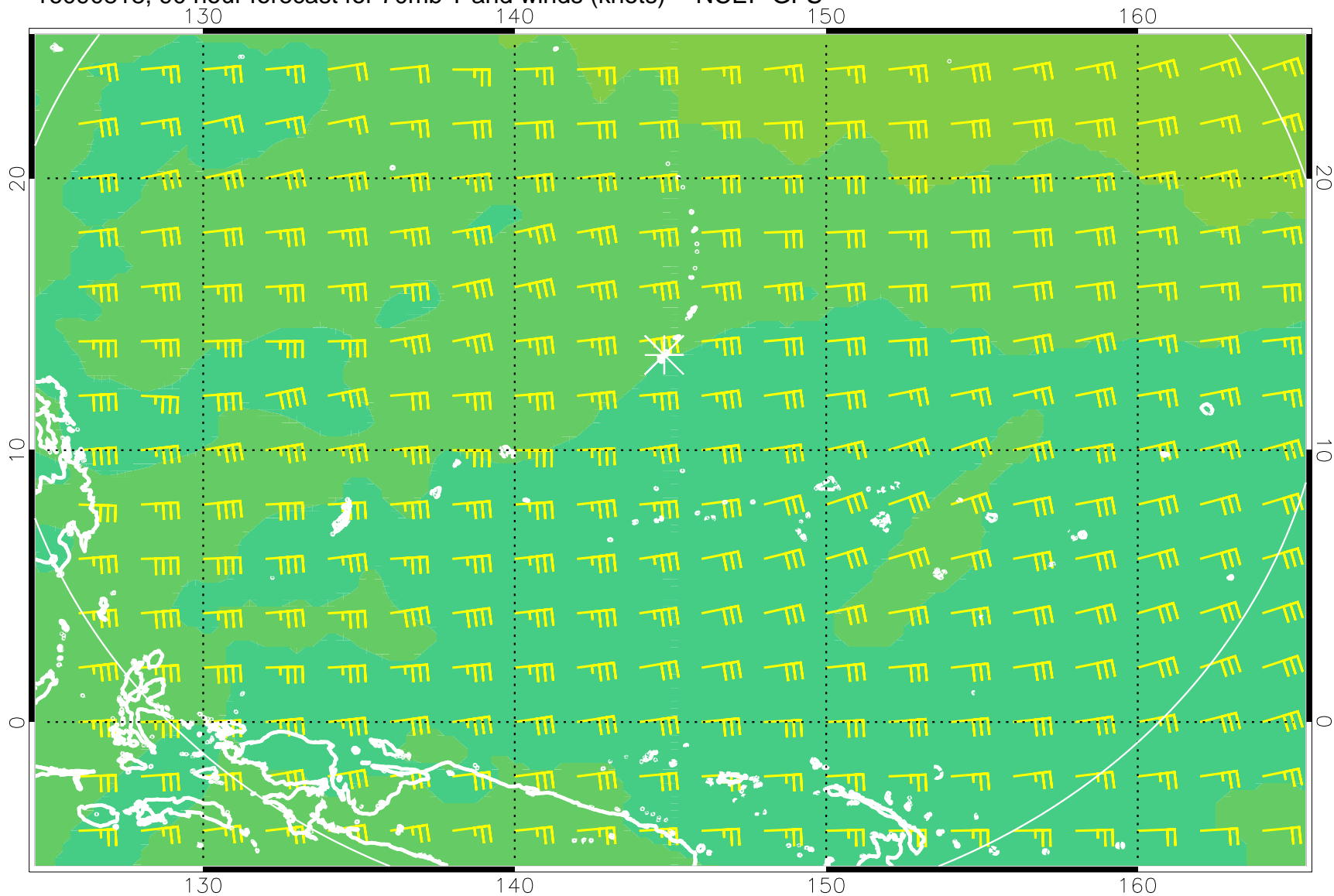
16090818, 90 hour forecast for 70mb T and winds (knots) -- NCEP GFS
