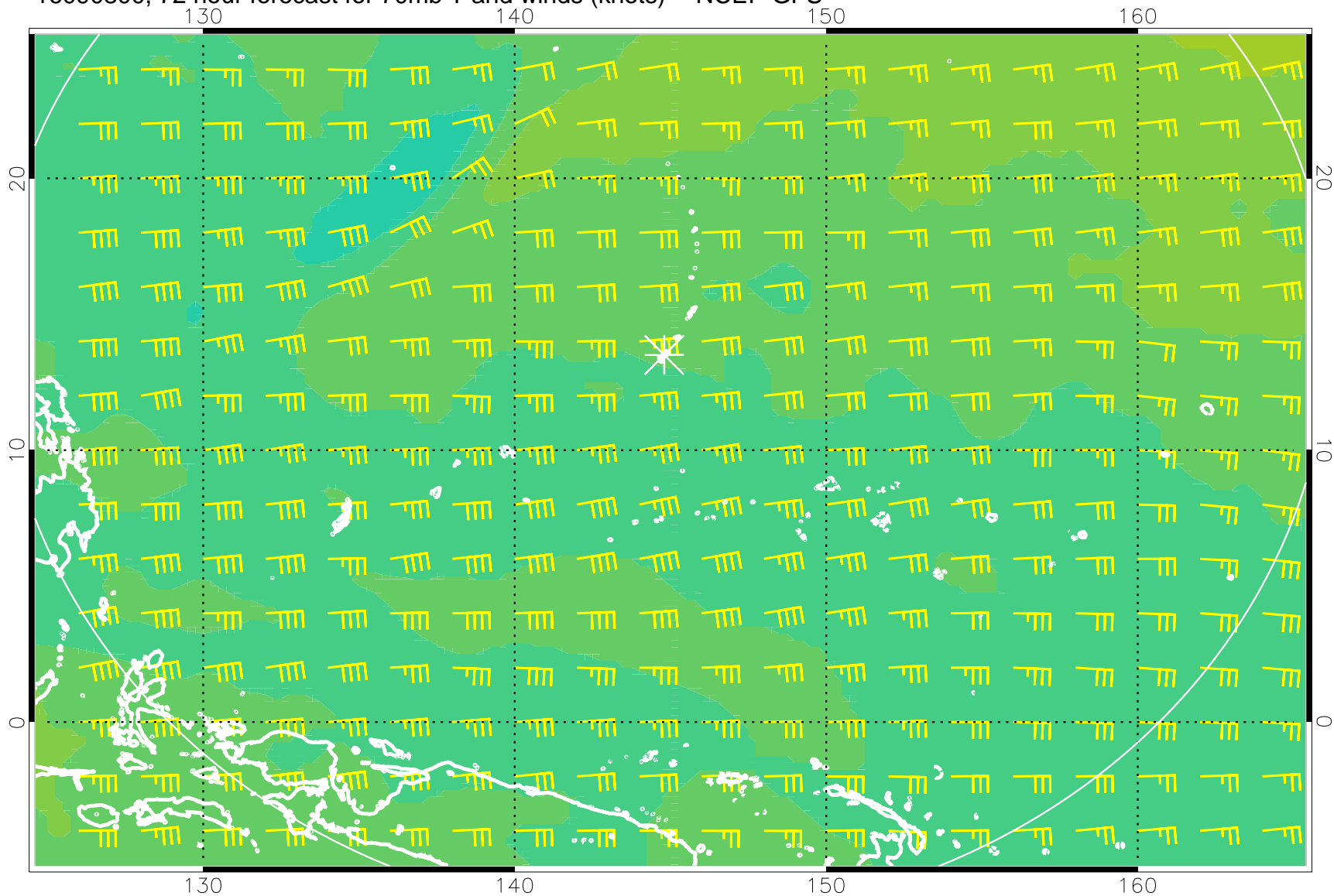
16090800, 72 hour forecast for 70mb T and winds (knots) -- NCEP GFS
