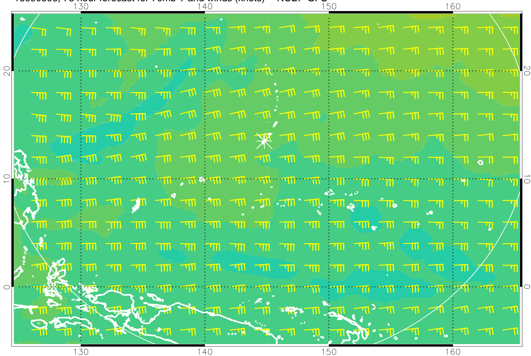
16090806, 78 hour forecast for 70mb T and winds (knots) -- NCEP GFS
