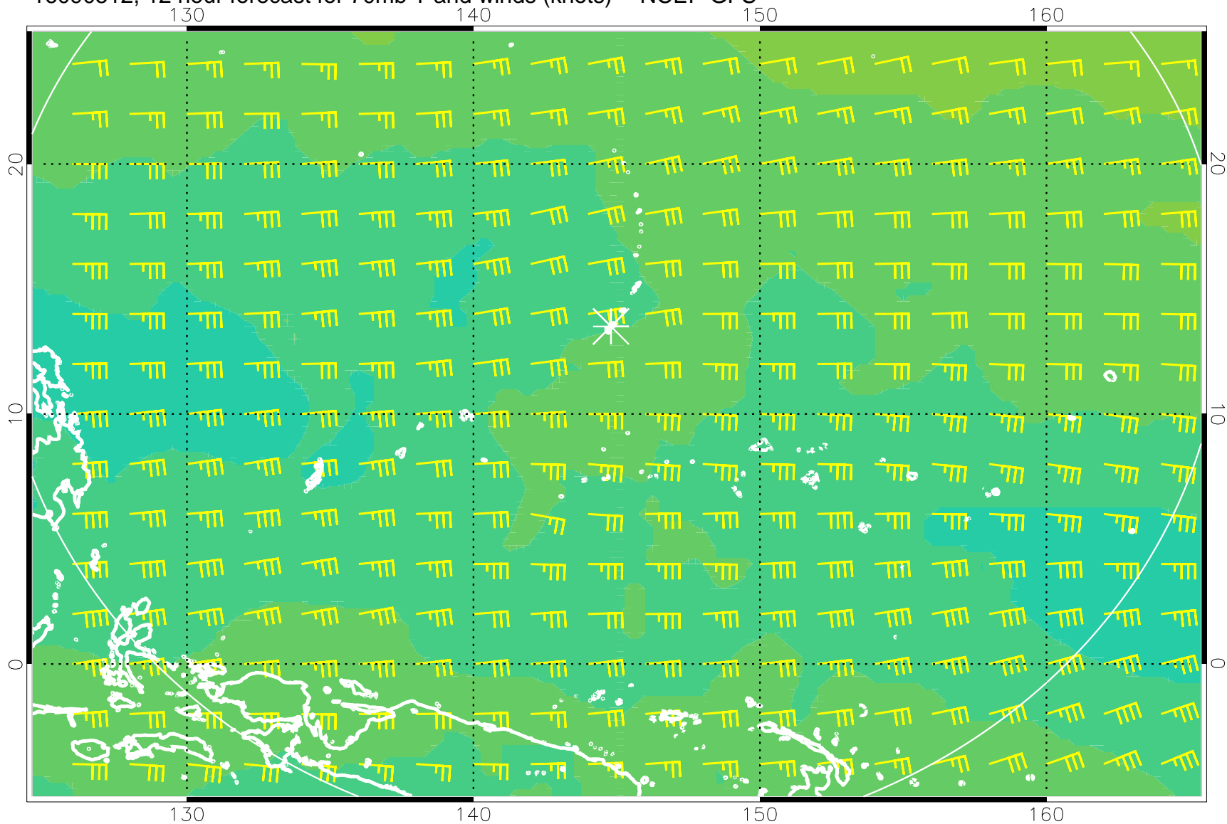
16090512, 12 hour forecast for 70mb T and winds (knots) -- NCEP GFS
