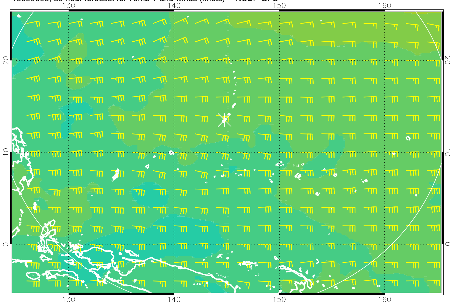
16090606, 30 hour forecast for 70mb T and winds (knots) -- NCEP GFS
