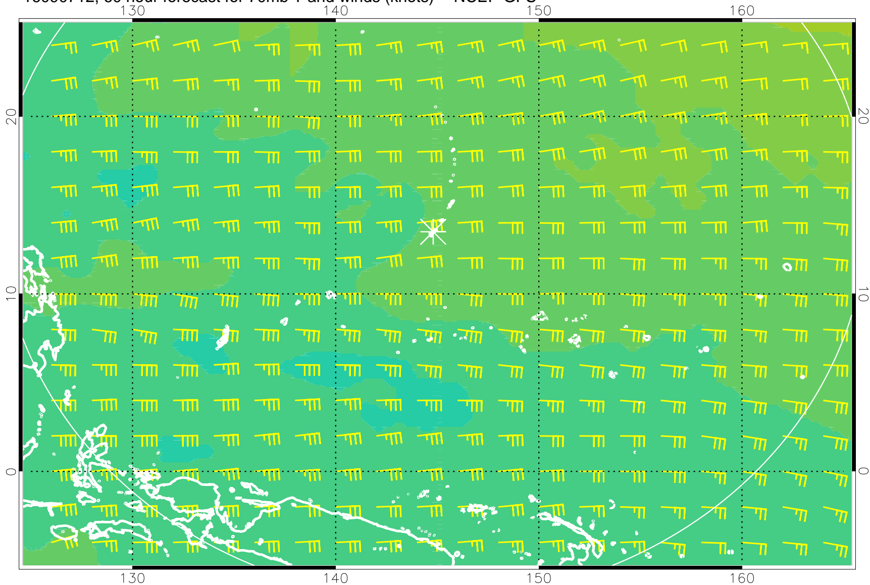
16090712, 60 hour forecast for 70mb T and winds (knots) -- NCEP GFS
