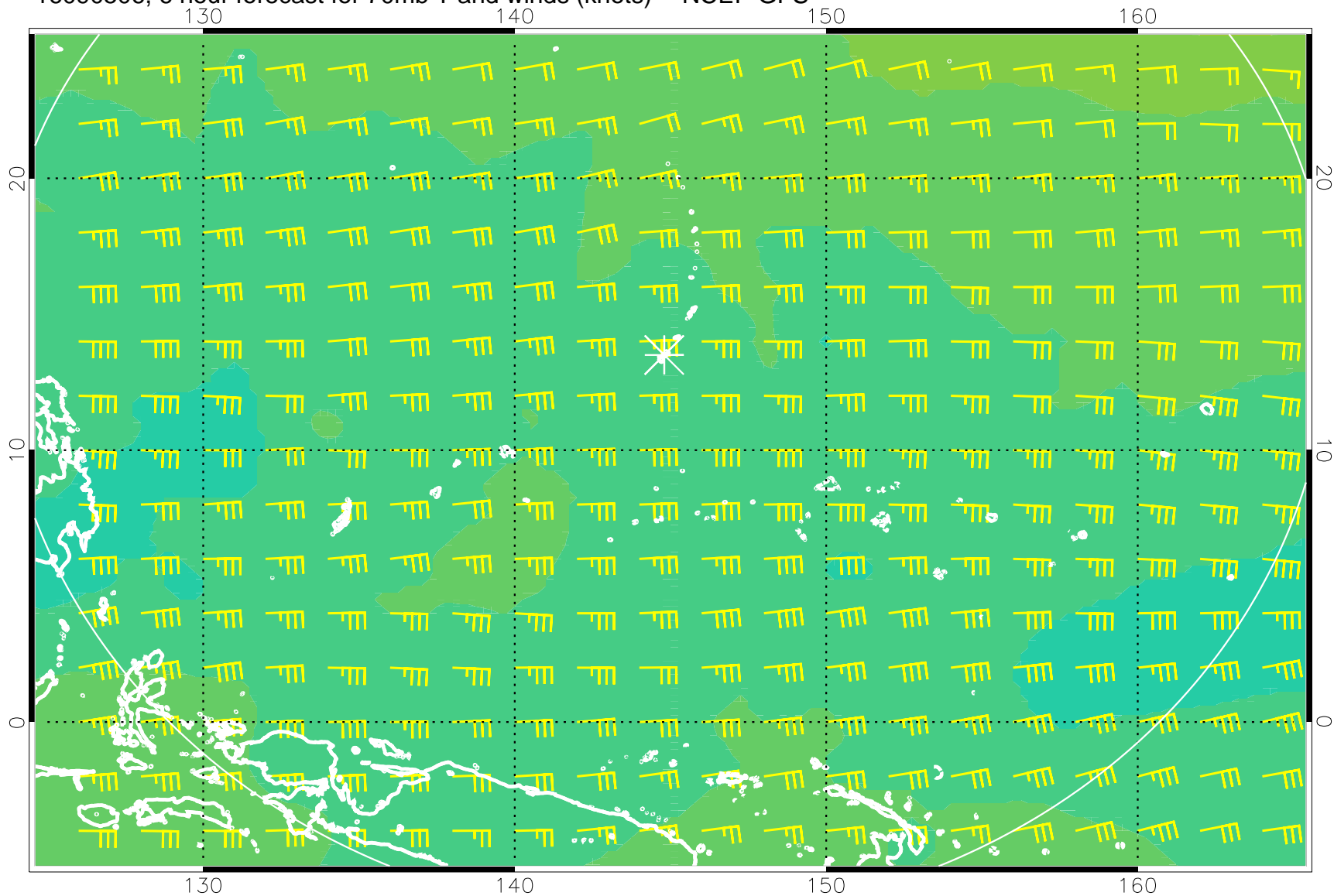
16090506, 6 hour forecast for 70mb T and winds (knots) -- NCEP GFS
