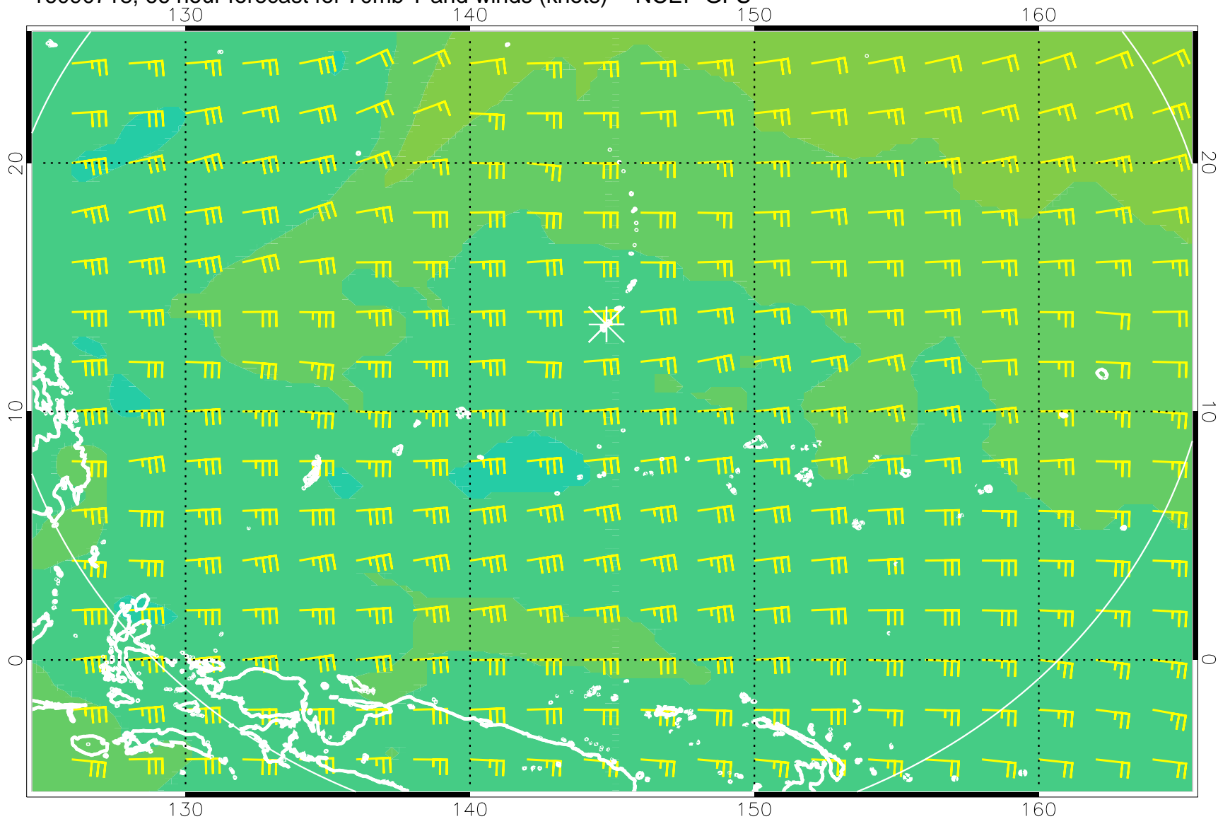
16090718, 66 hour forecast for 70mb T and winds (knots) -- NCEP GFS
