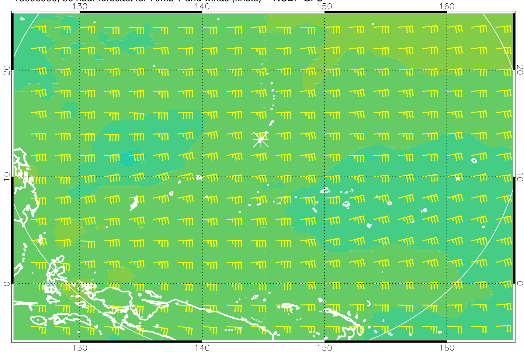
16090900, 96 hour forecast for 70mb T and winds (knots) -- NCEP GFS
