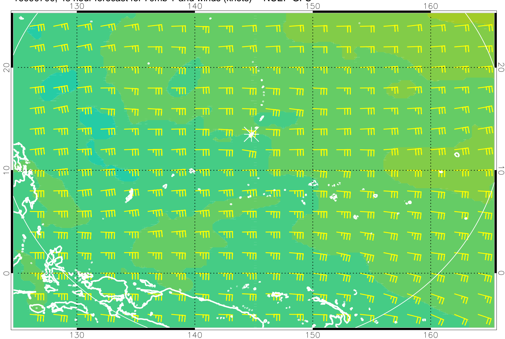
16090700, 48 hour forecast for 70mb T and winds (knots) -- NCEP GFS
