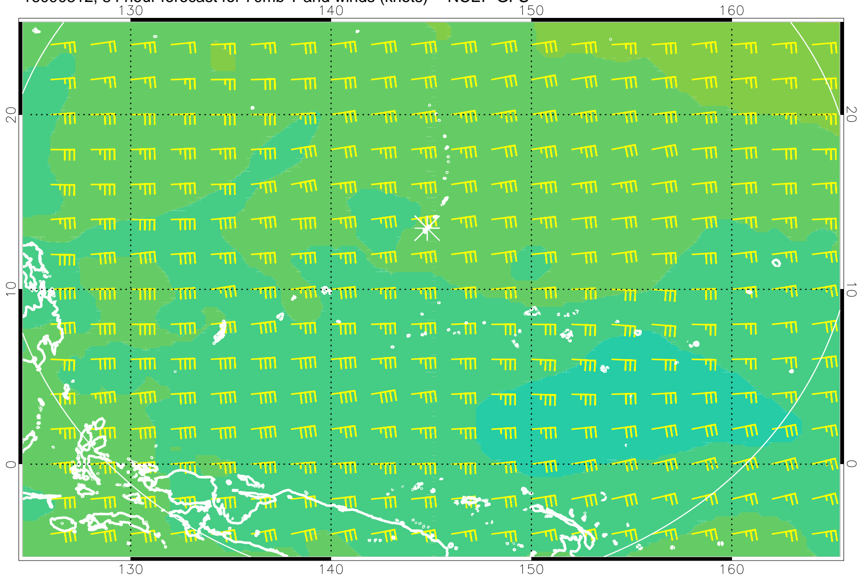
16090812, 84 hour forecast for 70mb T and winds (knots) -- NCEP GFS
