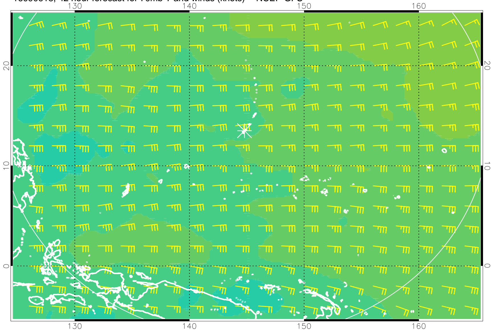
16090618, 42 hour forecast for 70mb T and winds (knots) -- NCEP GFS
