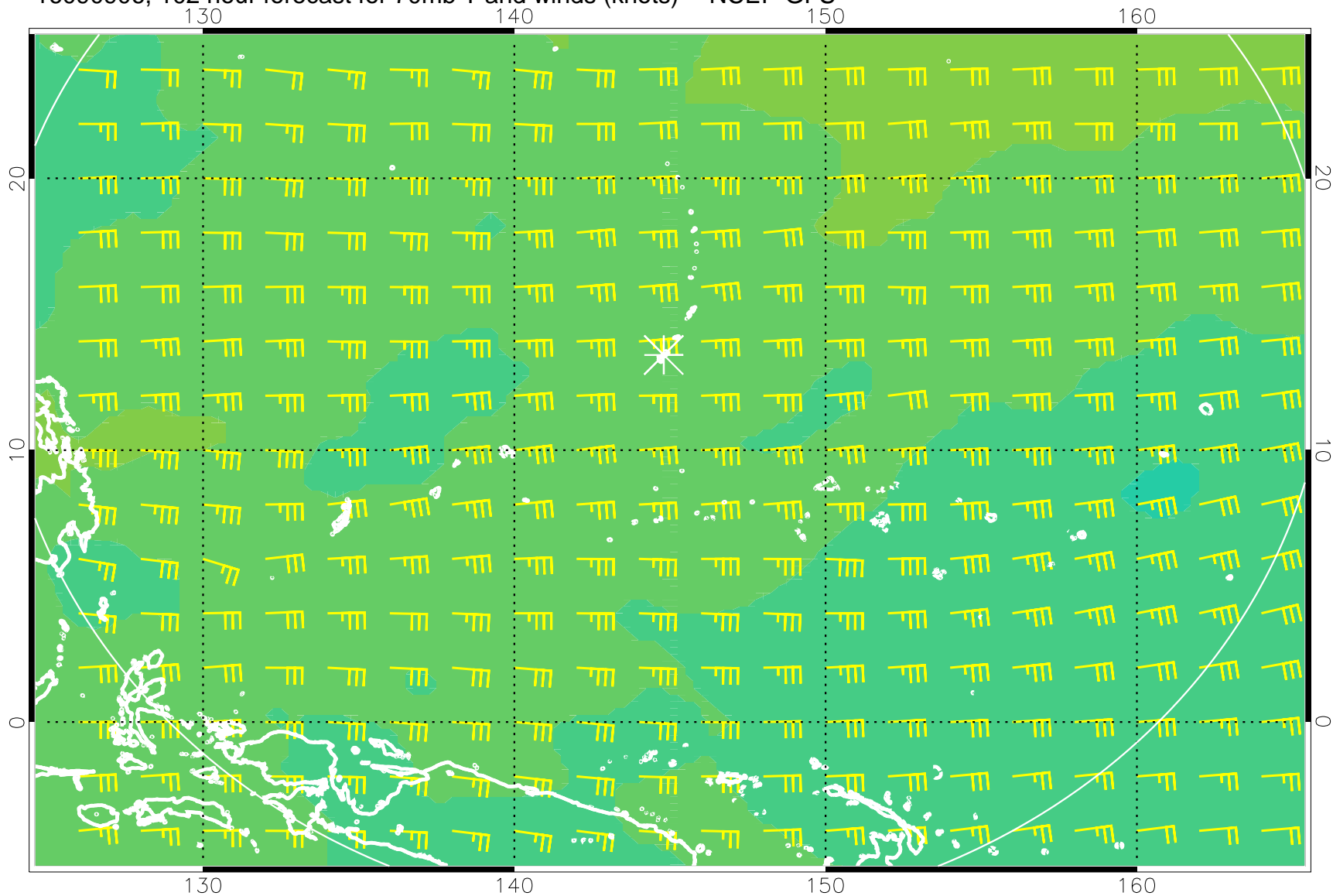
16090906, 102 hour forecast for 70mb T and winds (knots) -- NCEP GFS
