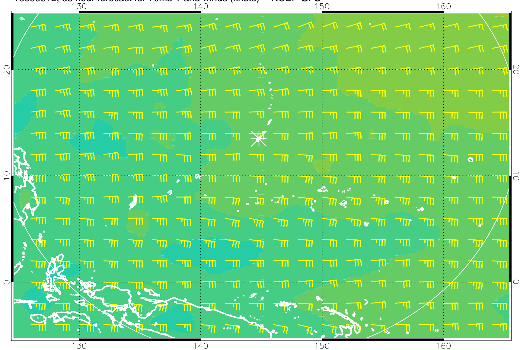
16090612, 36 hour forecast for 70mb T and winds (knots) -- NCEP GFS
