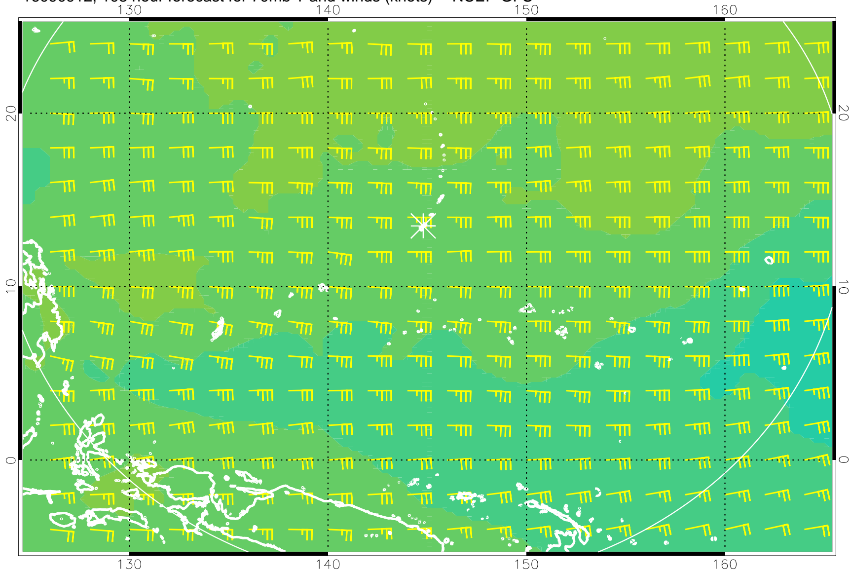
16090912, 108 hour forecast for 70mb T and winds (knots) -- NCEP GFS
