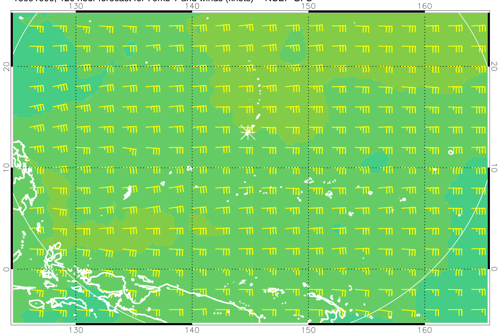
16091000, 120 hour forecast for 70mb T and winds (knots) -- NCEP GFS
