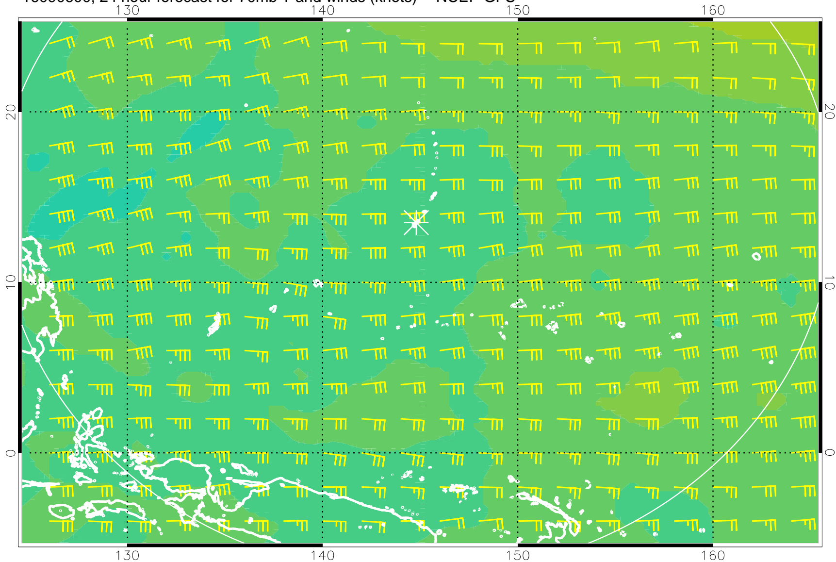
16090600, 24 hour forecast for 70mb T and winds (knots) -- NCEP GFS
