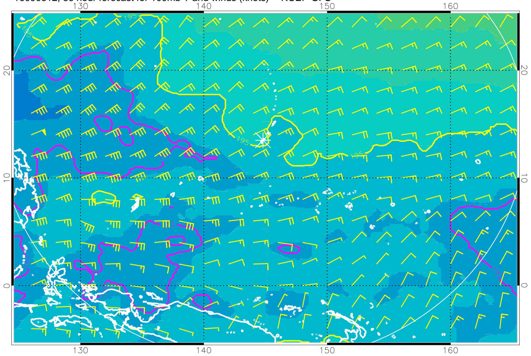
16090612, 36 hour forecast for 100mb T and winds (knots) -- NCEP GFS
