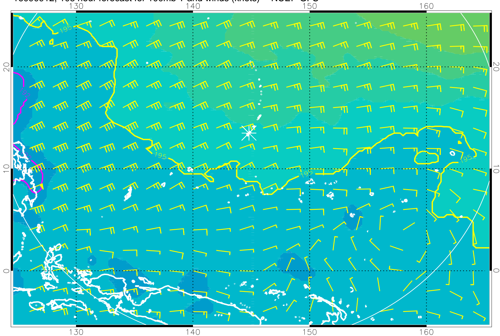
16090912, 108 hour forecast for 100mb T and winds (knots) -- NCEP GFS
