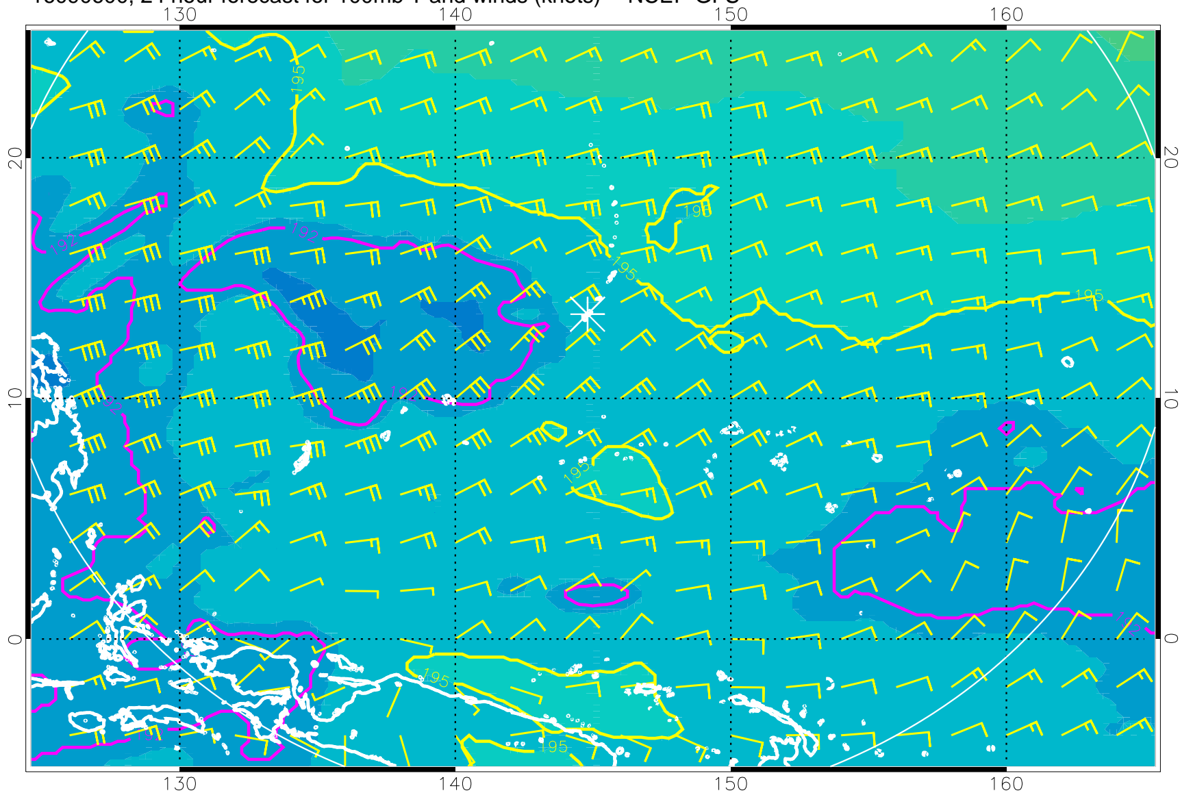
16090600, 24 hour forecast for 100mb T and winds (knots) -- NCEP GFS
