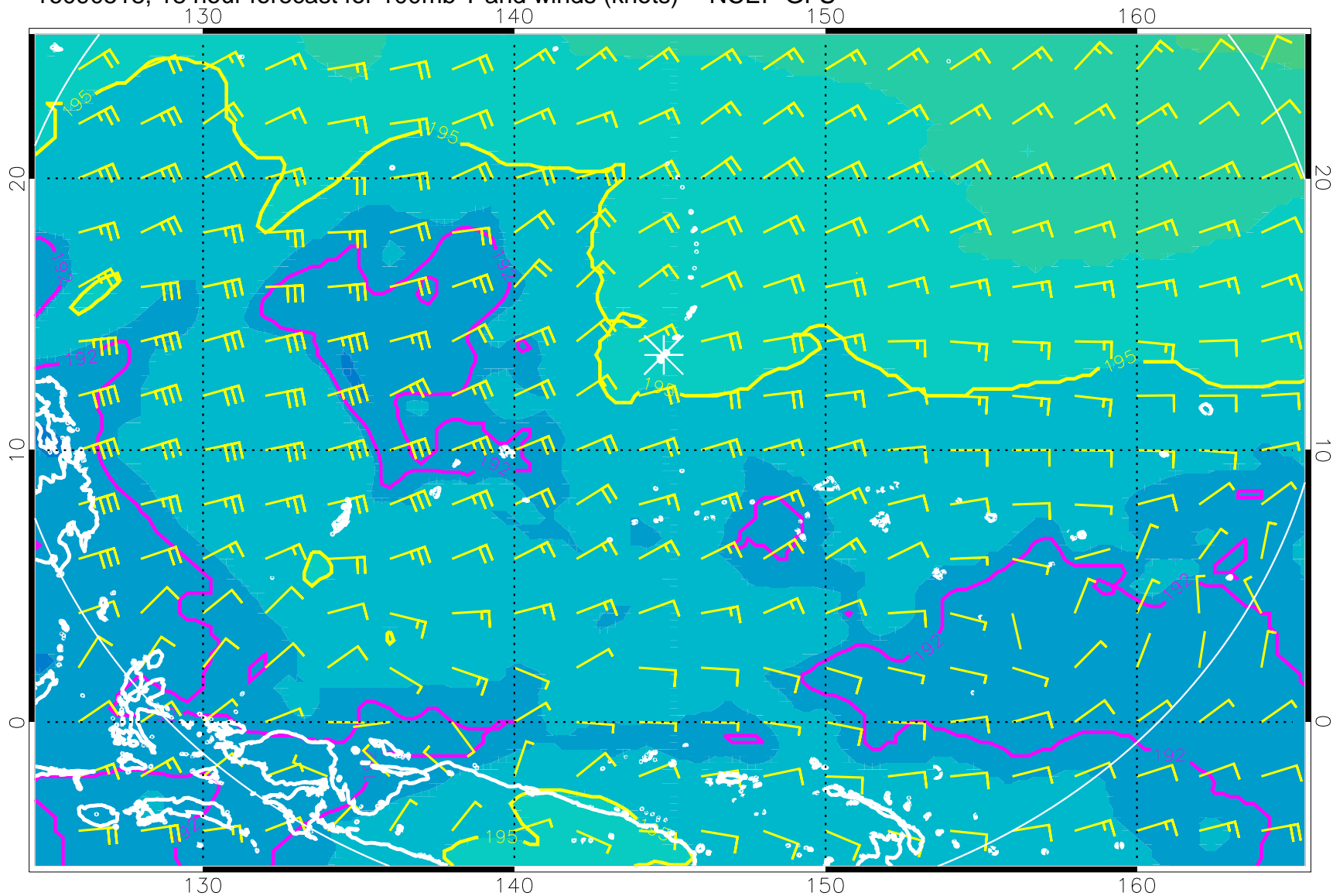
16090518, 18 hour forecast for 100mb T and winds (knots) -- NCEP GFS
