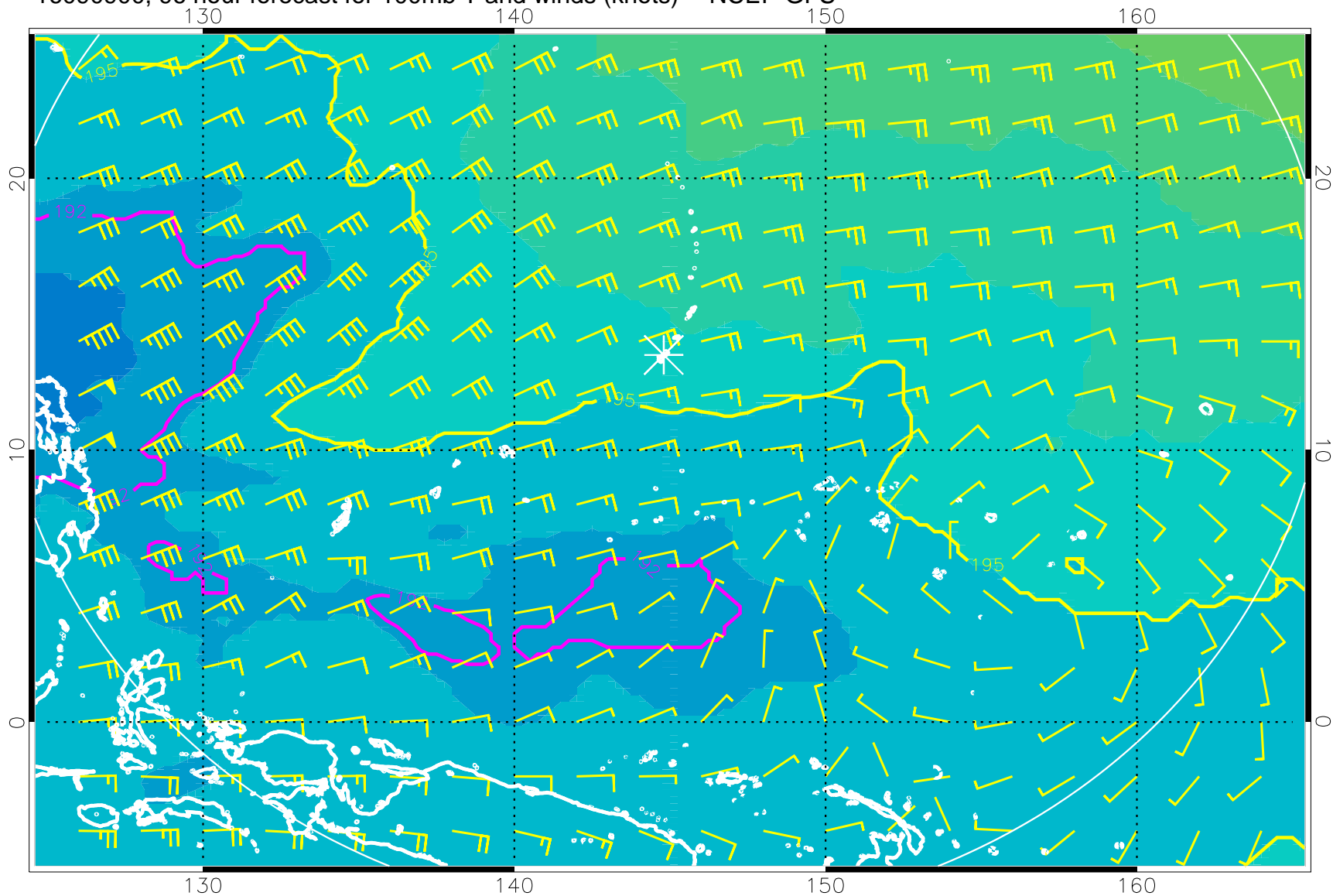
16090900, 96 hour forecast for 100mb T and winds (knots) -- NCEP GFS
