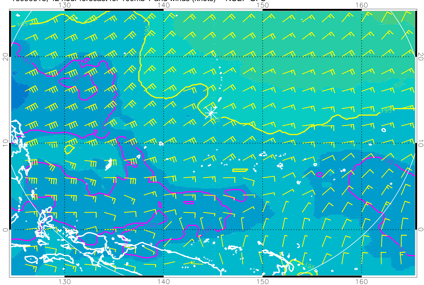
16090618, 42 hour forecast for 100mb T and winds (knots) -- NCEP GFS
