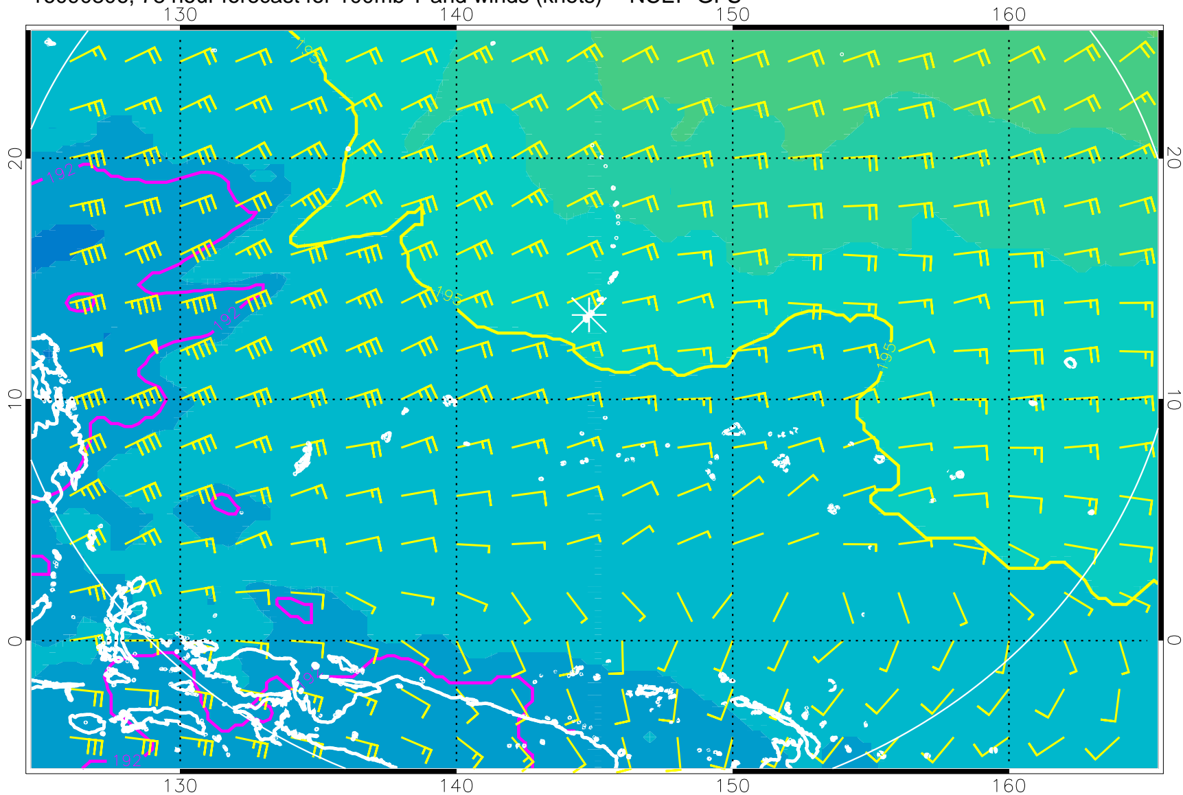
16090806, 78 hour forecast for 100mb T and winds (knots) -- NCEP GFS
