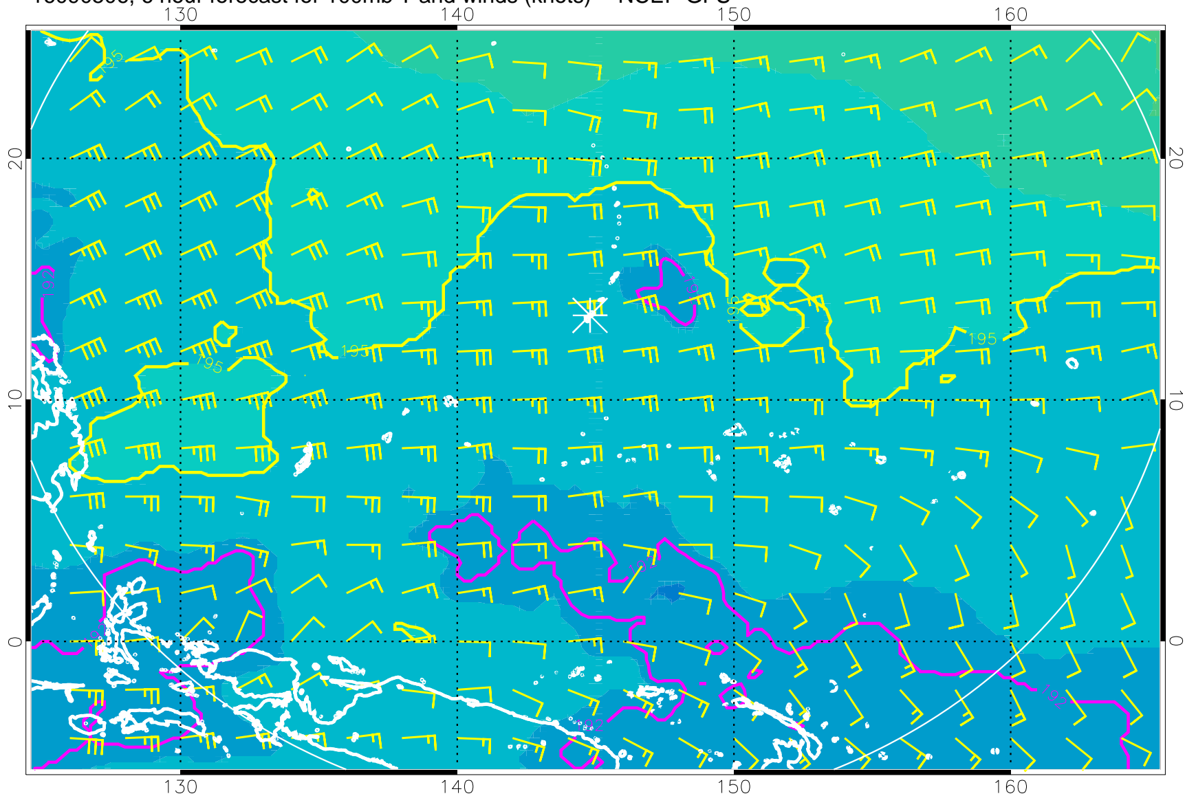
16090506, 6 hour forecast for 100mb T and winds (knots) -- NCEP GFS
