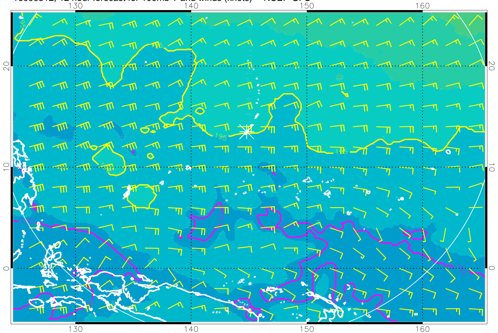
16090512, 12 hour forecast for 100mb T and winds (knots) -- NCEP GFS
