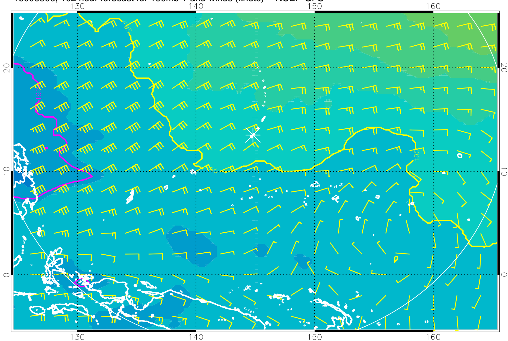
16090906, 102 hour forecast for 100mb T and winds (knots) -- NCEP GFS
