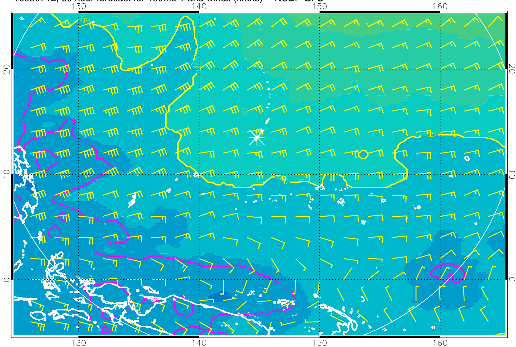
16090712, 60 hour forecast for 100mb T and winds (knots) -- NCEP GFS
