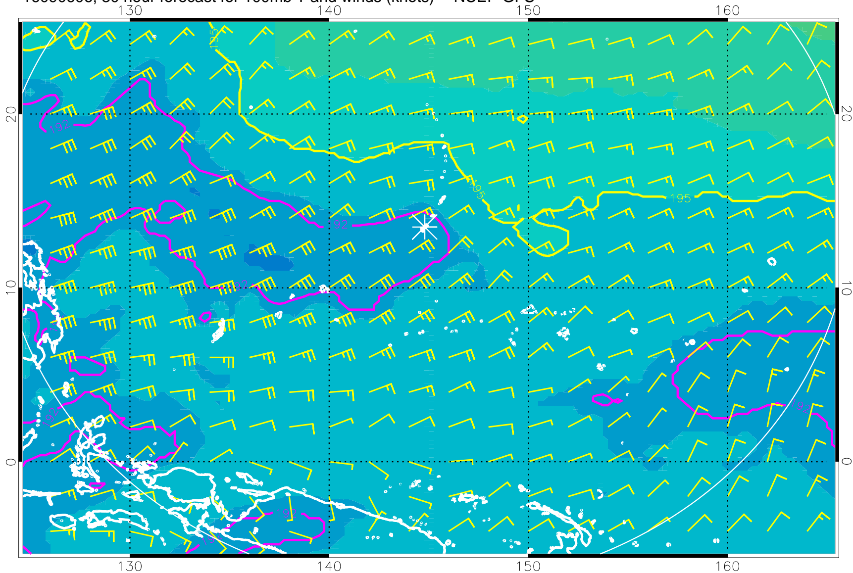
16090606, 30 hour forecast for 100mb T and winds (knots) -- NCEP GFS
