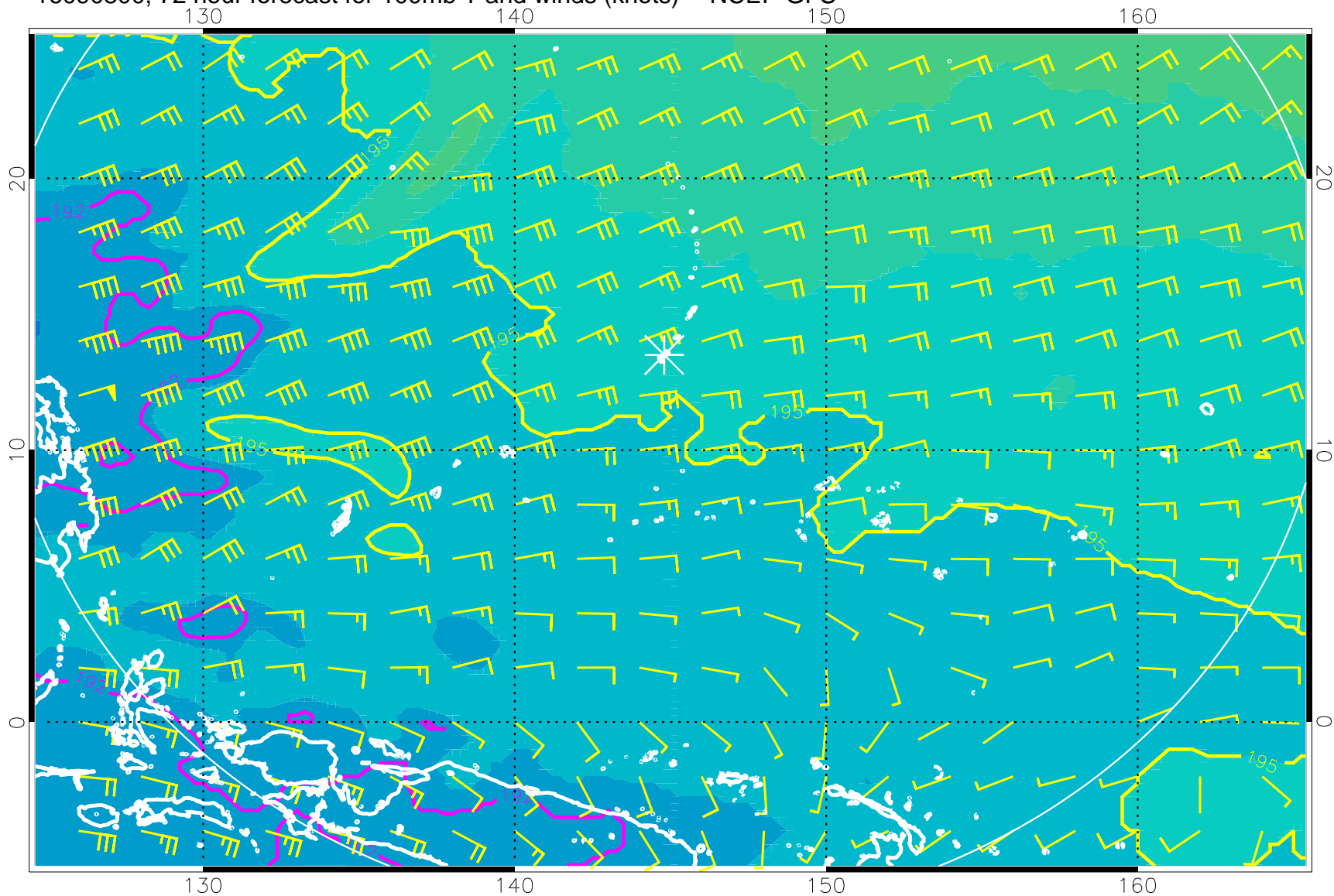
16090800, 72 hour forecast for 100mb T and winds (knots) -- NCEP GFS
