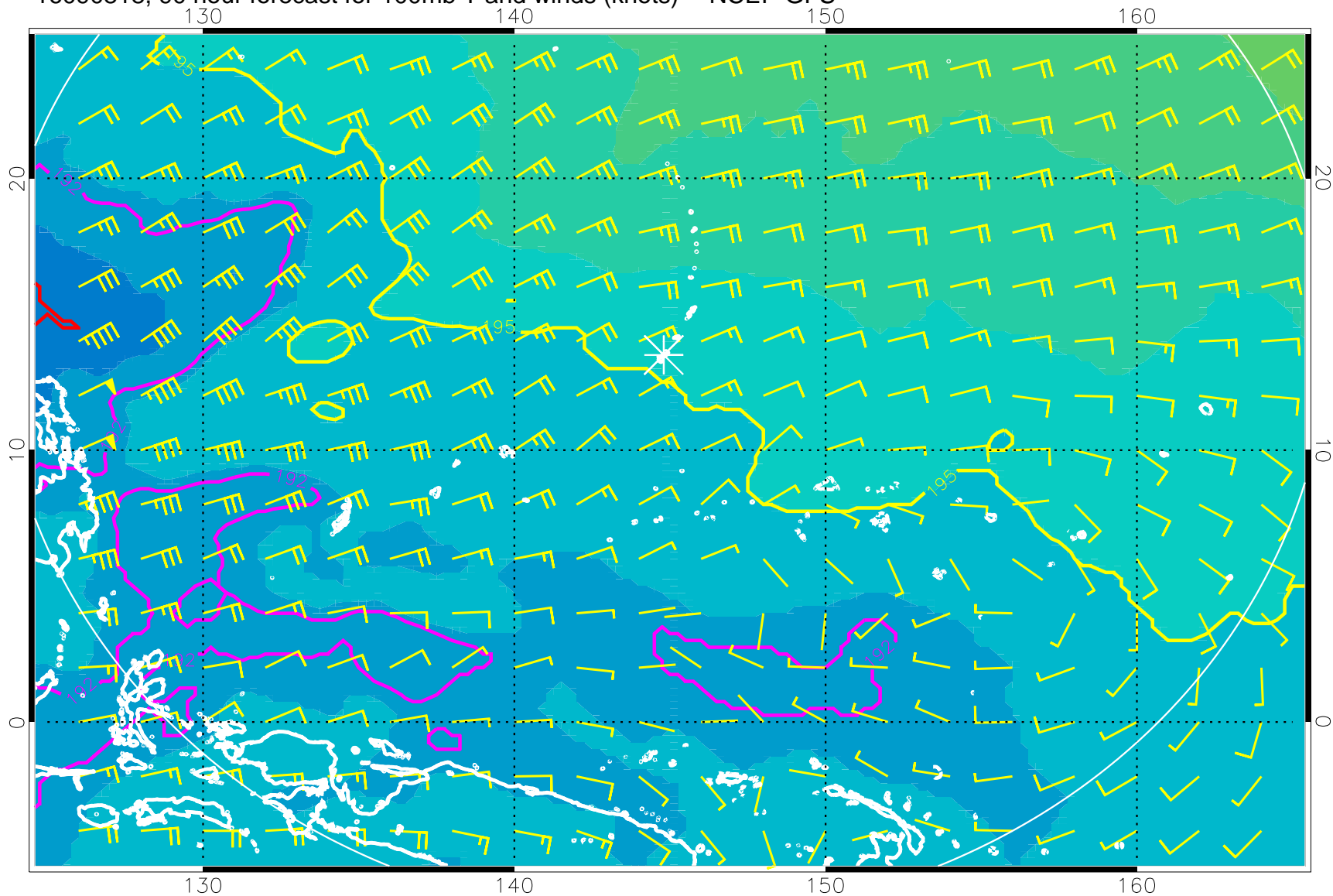
16090818, 90 hour forecast for 100mb T and winds (knots) -- NCEP GFS
