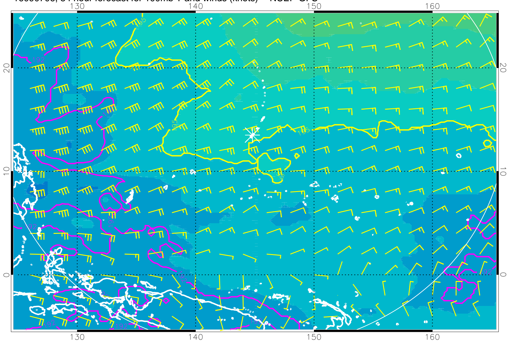
16090706, 54 hour forecast for 100mb T and winds (knots) -- NCEP GFS
