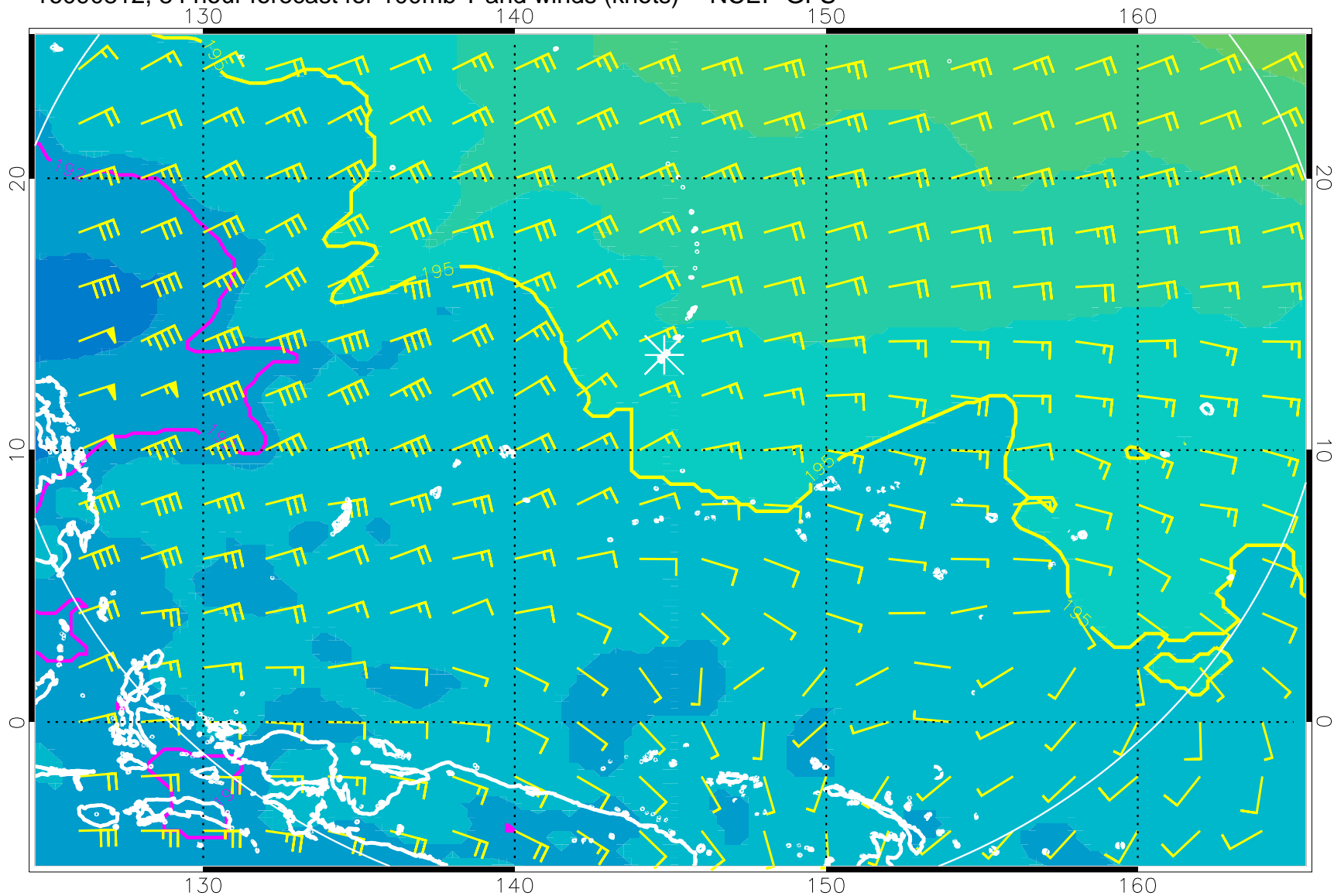
16090812, 84 hour forecast for 100mb T and winds (knots) -- NCEP GFS
