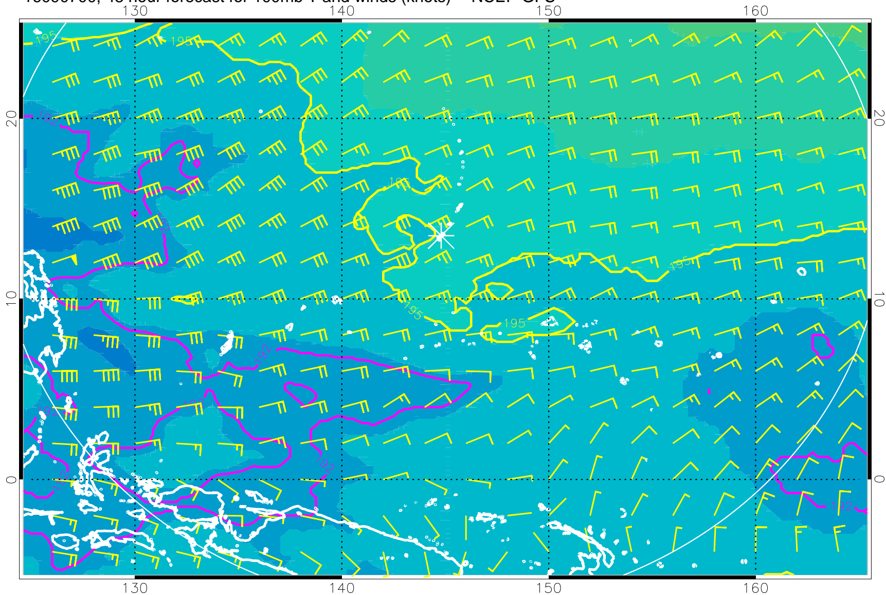
16090700, 48 hour forecast for 100mb T and winds (knots) -- NCEP GFS
