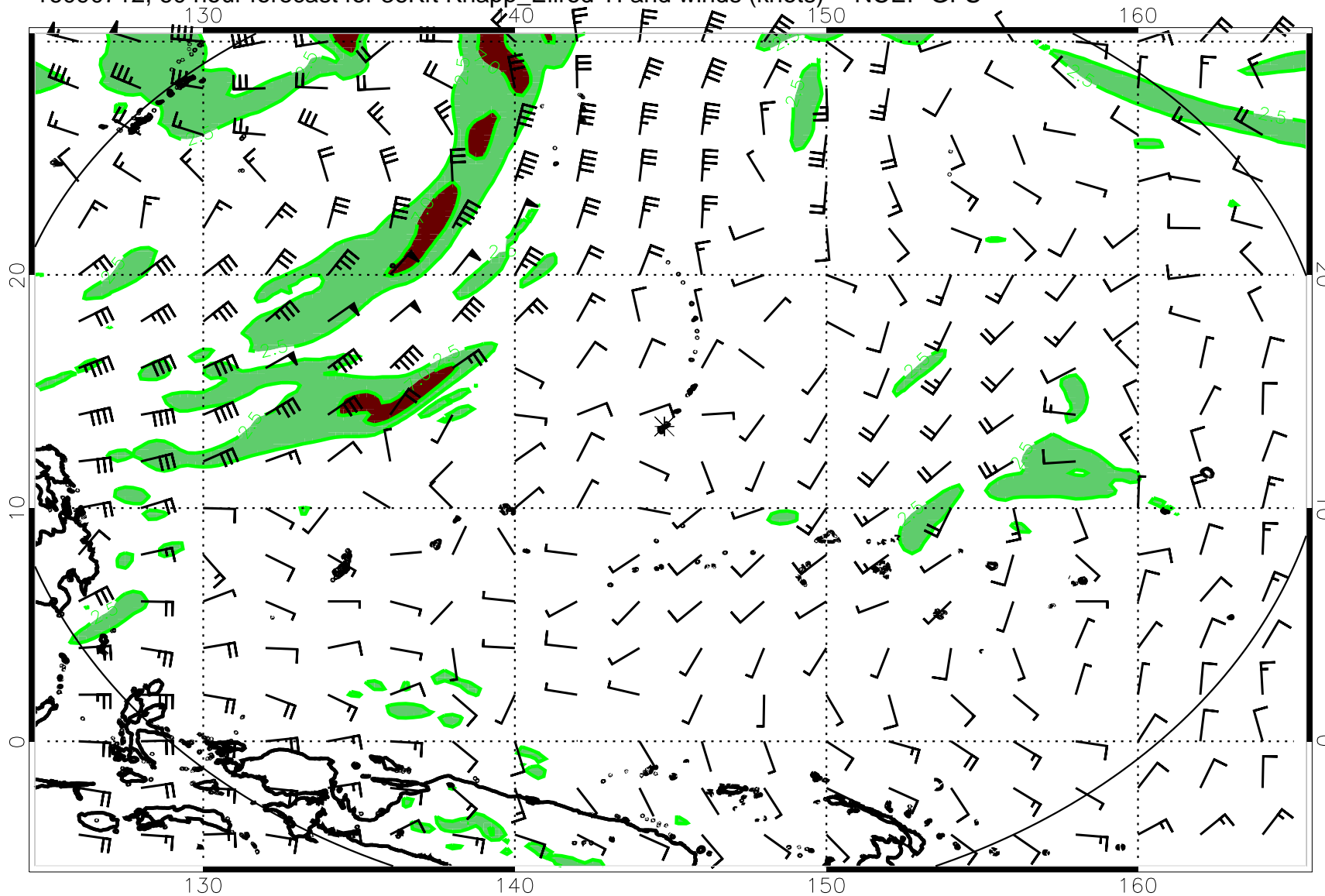
16090712, 60 hour forecast for 36Kft Knapp_Ellrod TI and winds (knots) -- NCEP GFS
