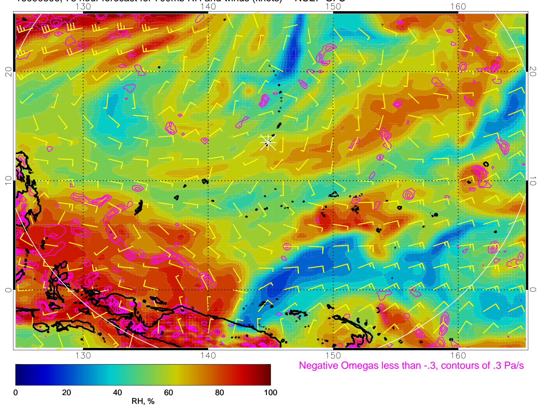
16090806, 78 hour forecast for 700mb RH and winds (knots) -- NCEP GFS
