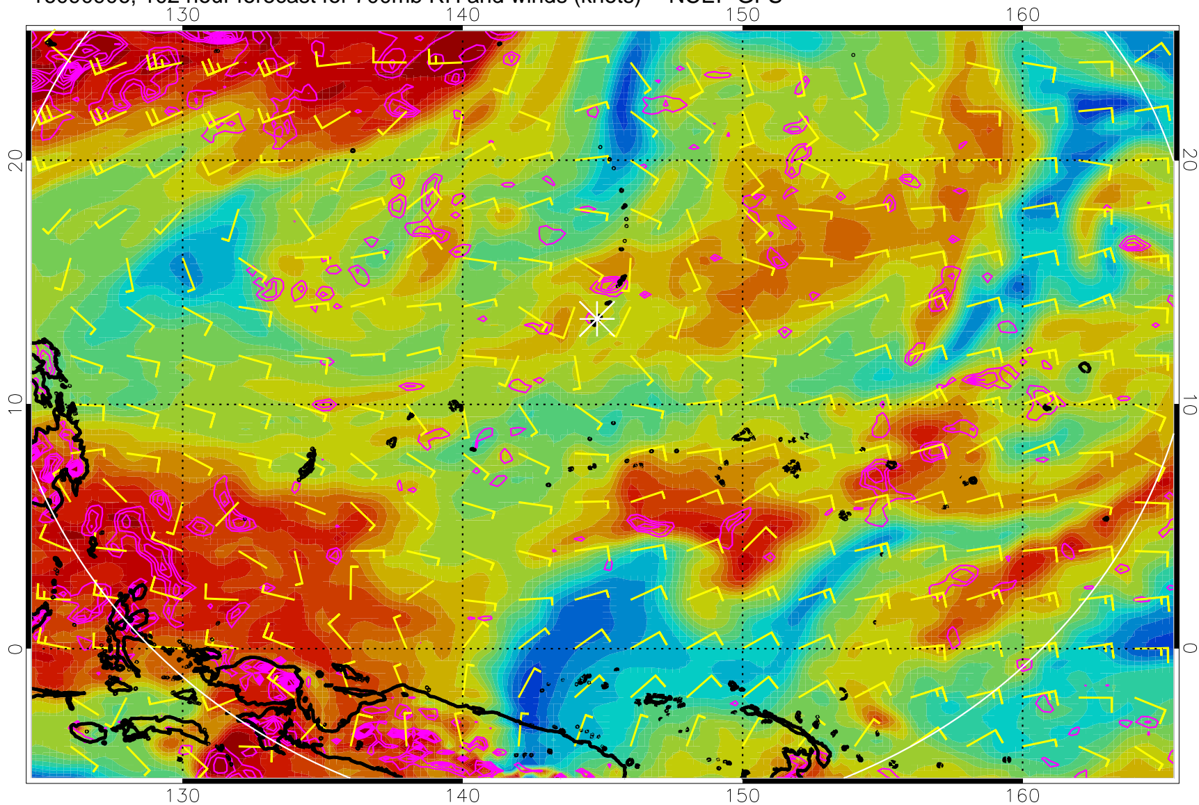
16090906, 102 hour forecast for 700mb RH and winds (knots) -- NCEP GFS
