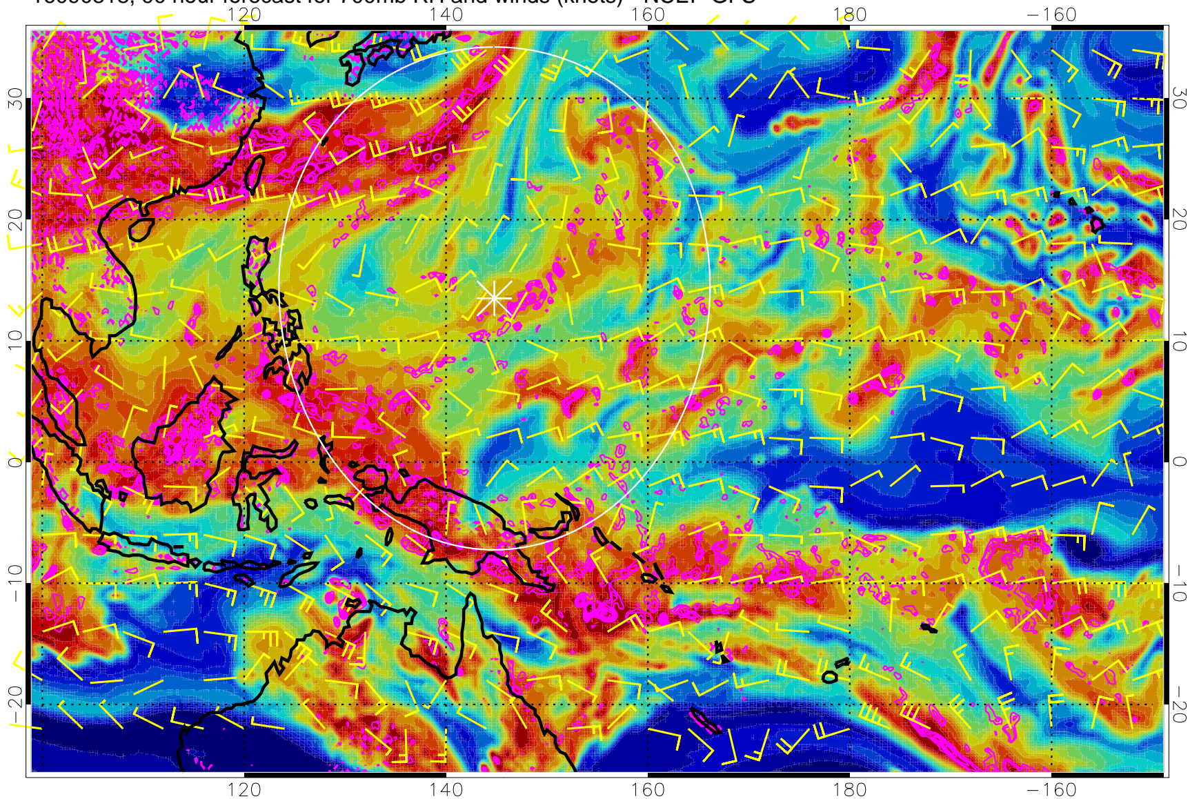
16090818, 90 hour forecast for 700mb RH and winds (knots) - NCEP GFS
