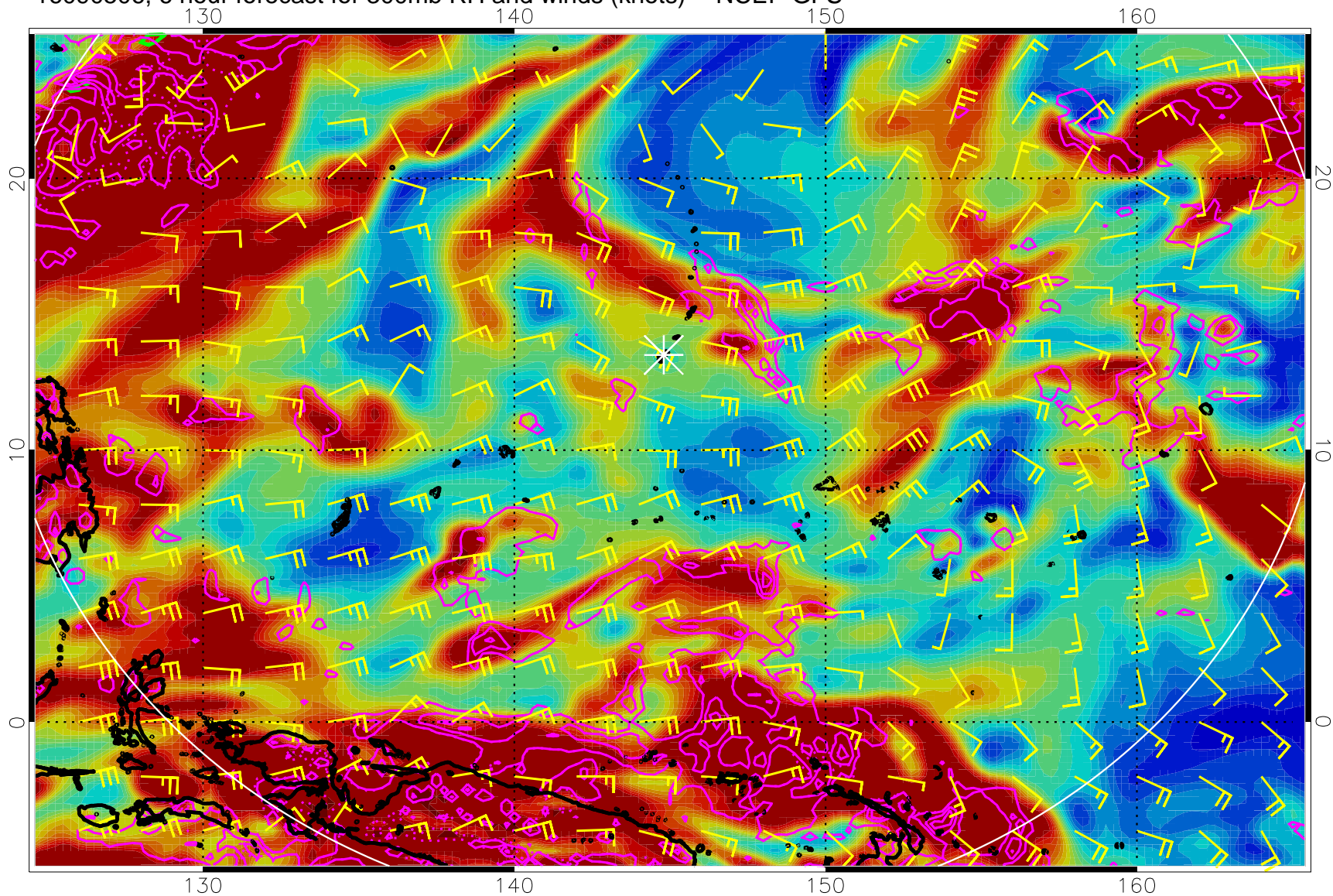
16090506, 6 hour forecast for 300mb RH and winds (knots) -- NCEP GFS
