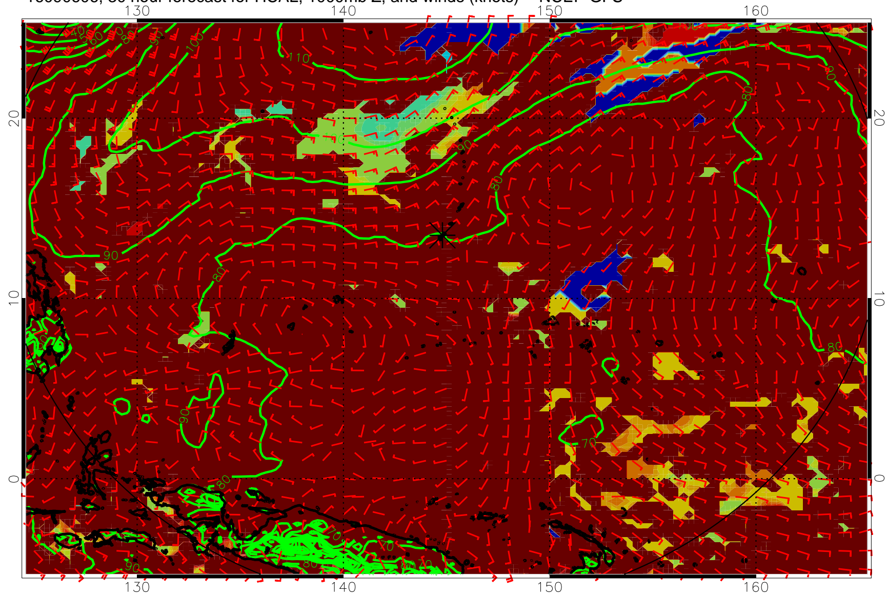
16090606, 30 hour forecast for HCAL, 1000mb Z, and winds (knots) -- NCEP GFS
