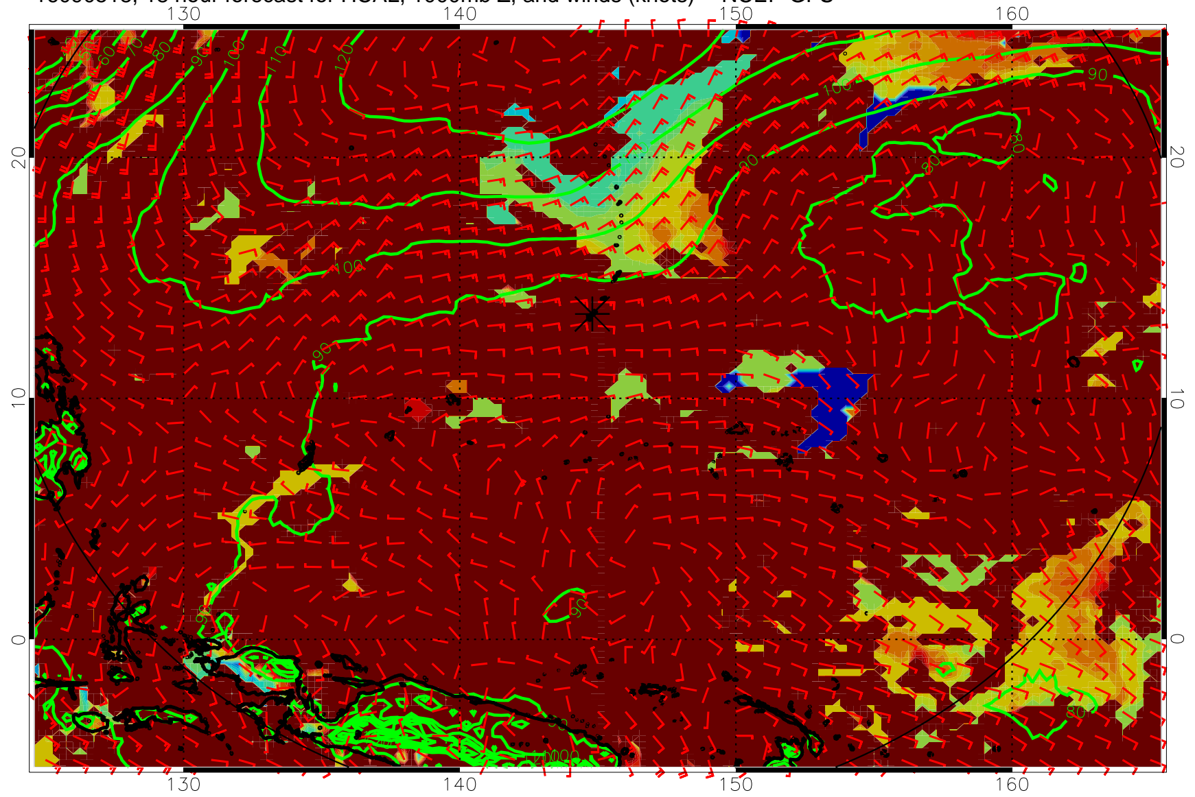
16090518, 18 hour forecast for HCAL, 1000mb Z, and winds (knots) -- NCEP GFS
