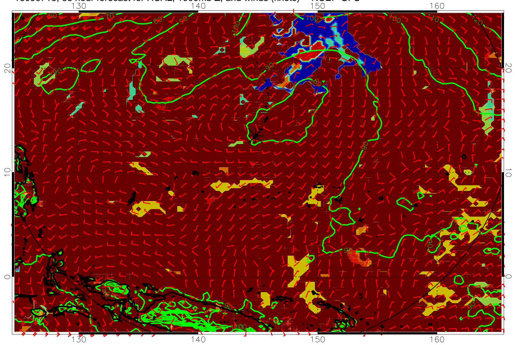
16090718, 66 hour forecast for HCAL, 1000mb Z, and winds (knots) -- NCEP GFS
