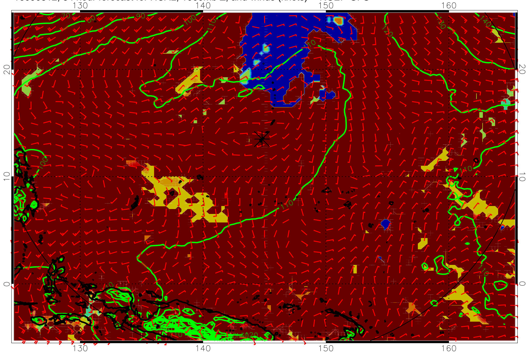
16090812, 84 hour forecast for HCAL, 1000mb Z, and winds (knots) -- NCEP GFS
