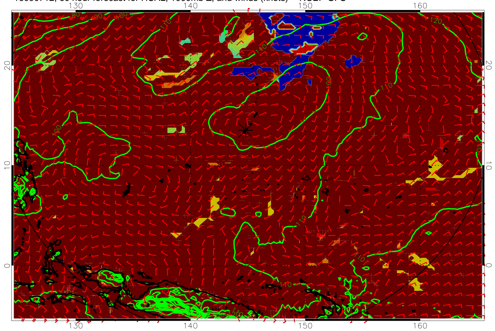
16090712, 60 hour forecast for HCAL, 1000mb Z, and winds (knots) -- NCEP GFS
