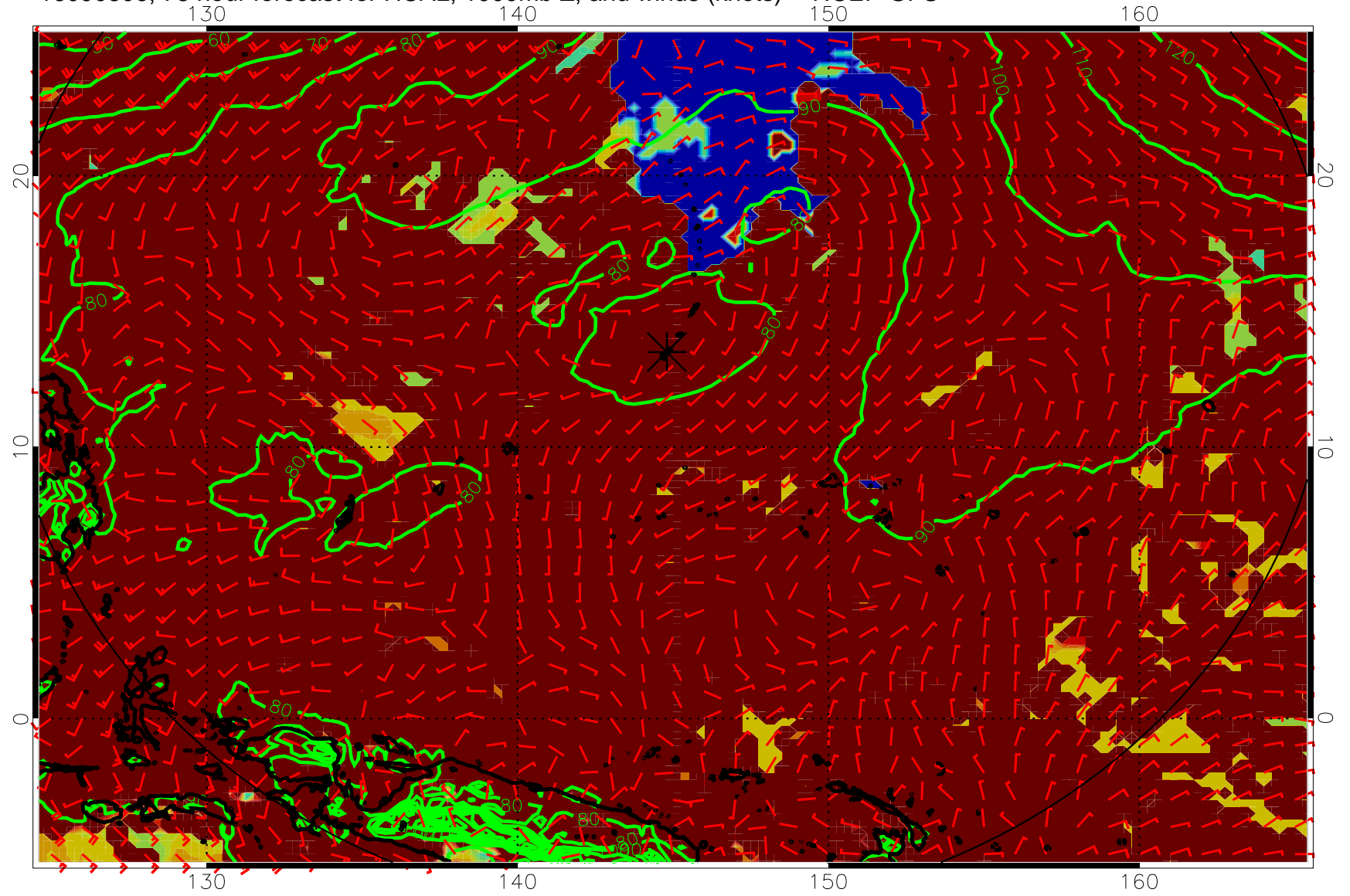
16090806, 78 hour forecast for HCAL, 1000mb Z, and winds (knots) -- NCEP GFS
