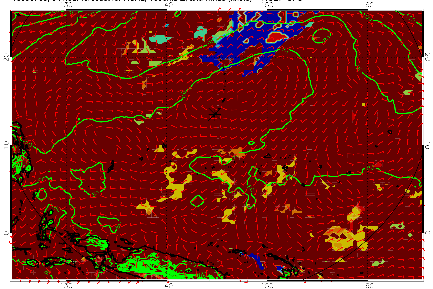
16090706, 54 hour forecast for HCAL, 1000mb Z, and winds (knots) -- NCEP GFS
