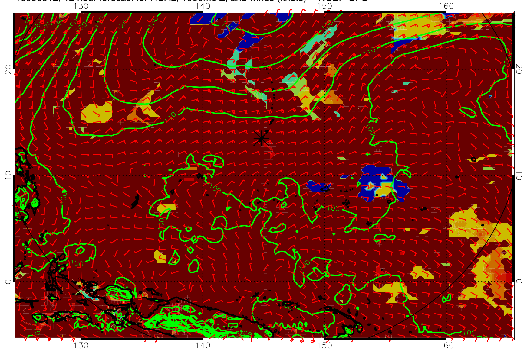
16090512, 12 hour forecast for HCAL, 1000mb Z, and winds (knots) -- NCEP GFS
