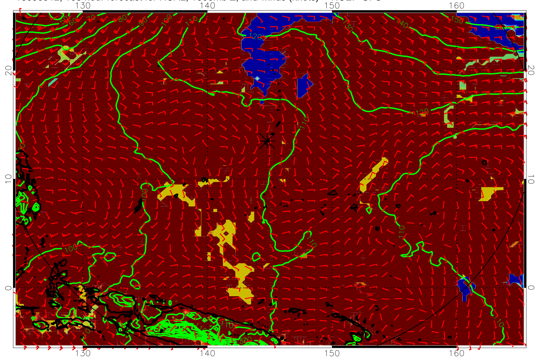
16090912, 108 hour forecast for HCAL, 1000mb Z, and winds (knots) -- NCEP GFS
