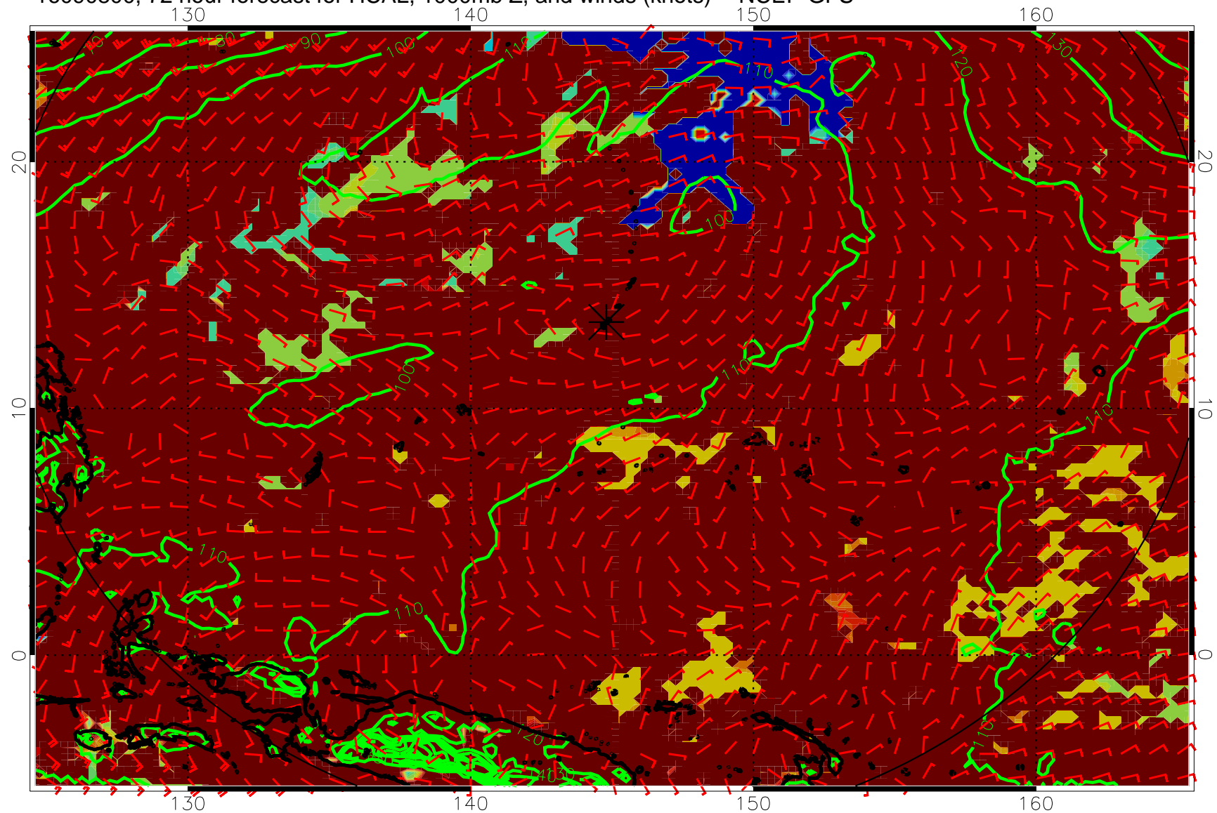
16090800, 72 hour forecast for HCAL, 1000mb Z, and winds (knots) -- NCEP GFS
