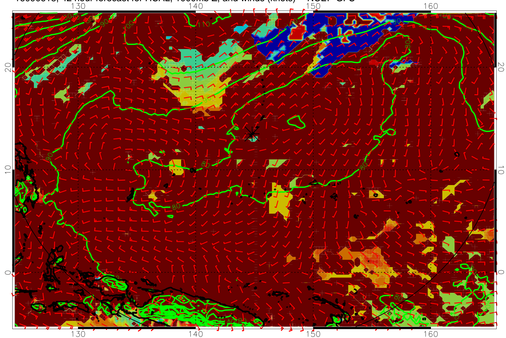
16090618, 42 hour forecast for HCAL, 1000mb Z, and winds (knots) -- NCEP GFS
