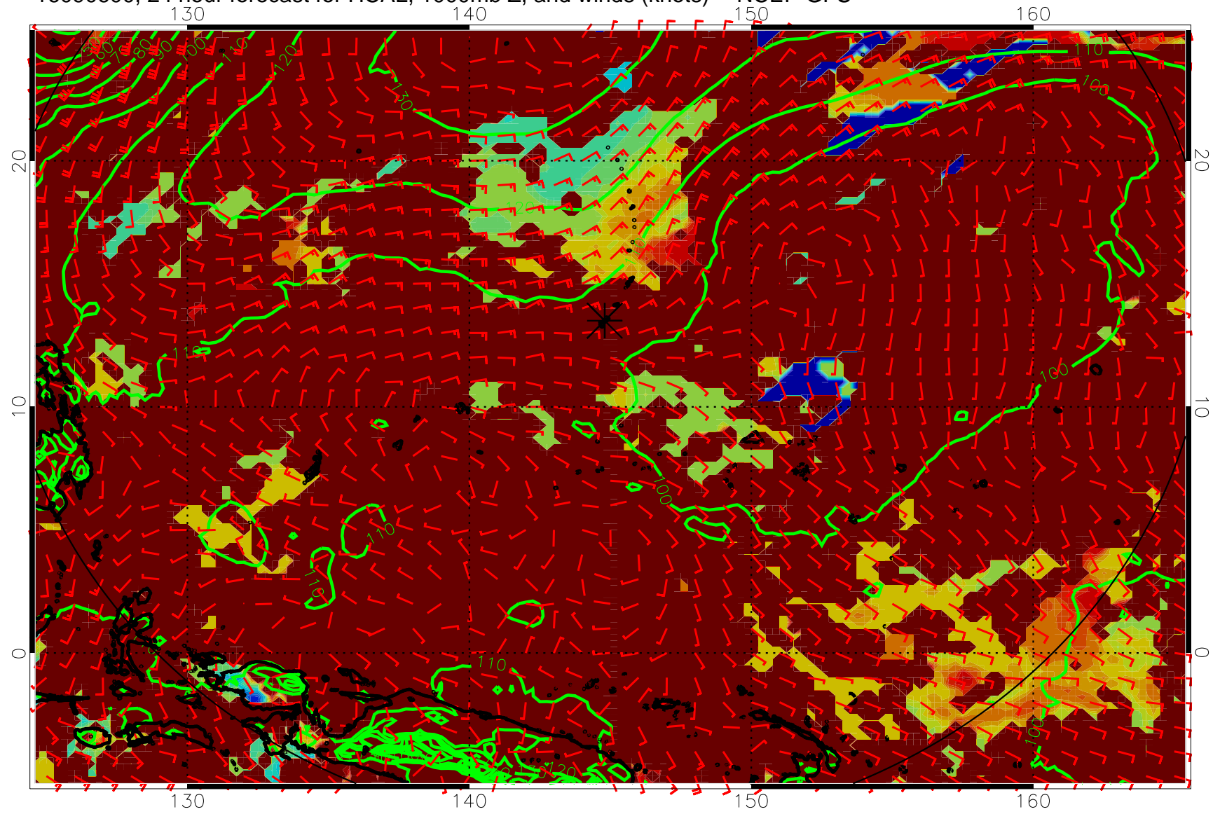
16090600, 24 hour forecast for HCAL, 1000mb Z, and winds (knots) -- NCEP GFS
