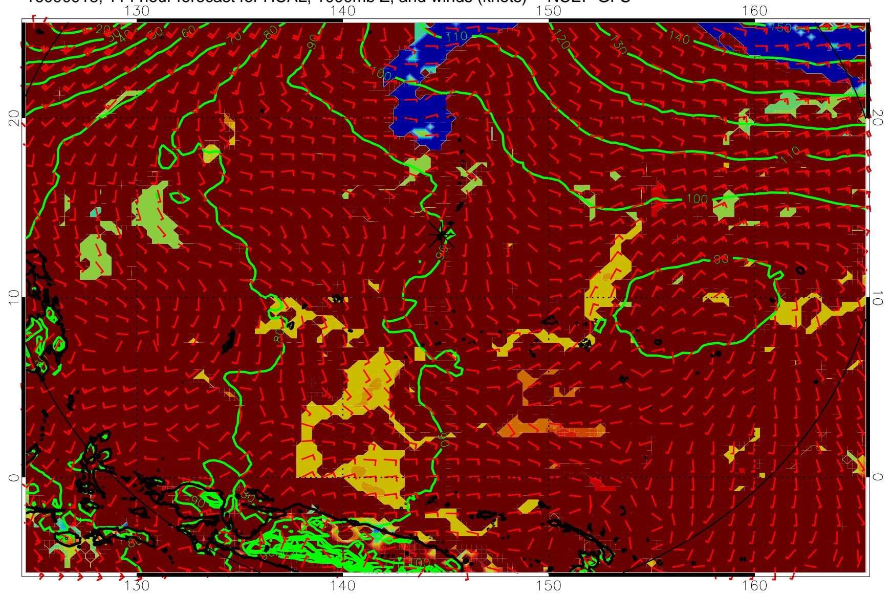
16090918, 114 hour forecast for HCAL, 1000mb Z, and winds (knots) -- NCEP GFS
