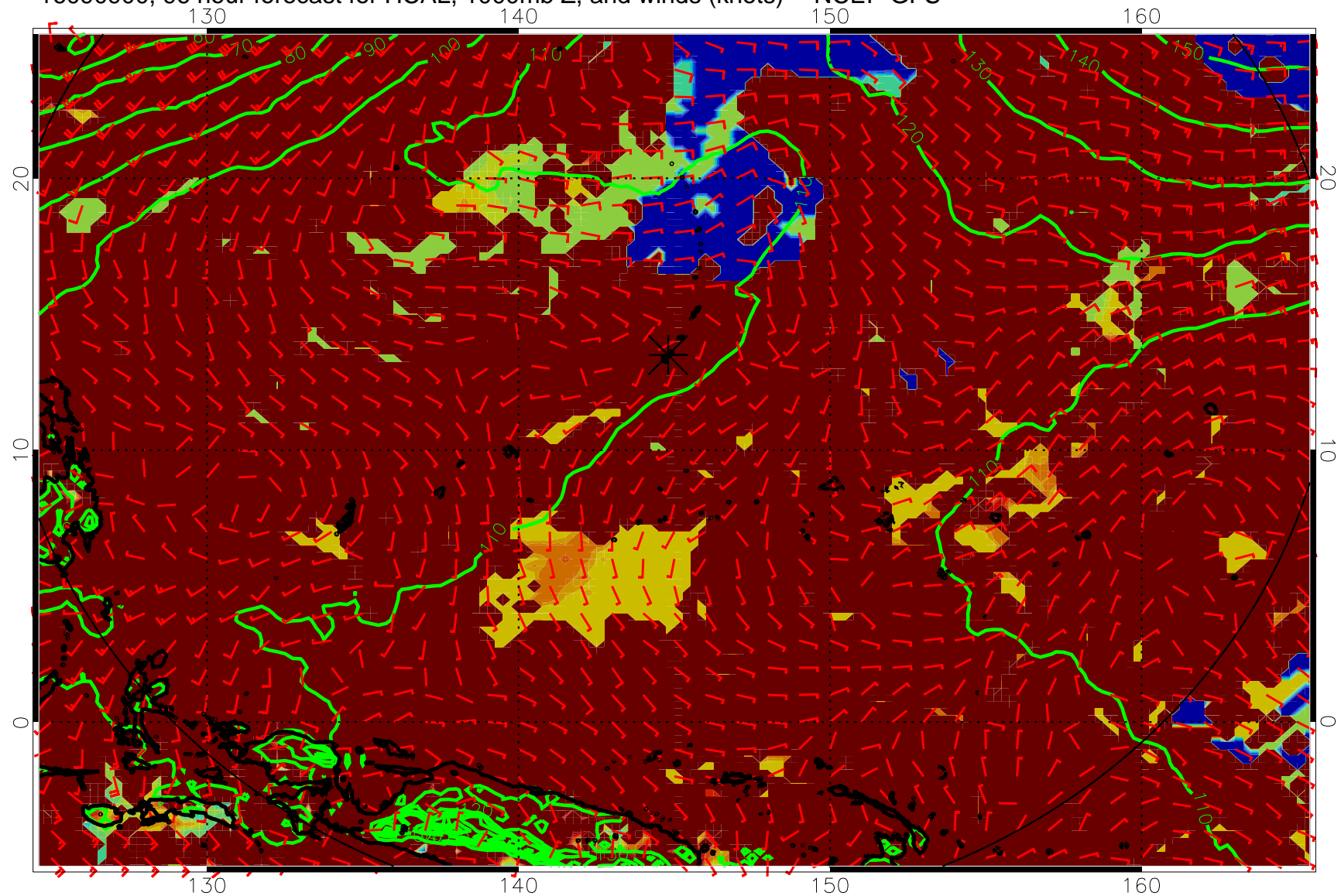
16090900, 96 hour forecast for HCAL, 1000mb Z, and winds (knots) -- NCEP GFS
