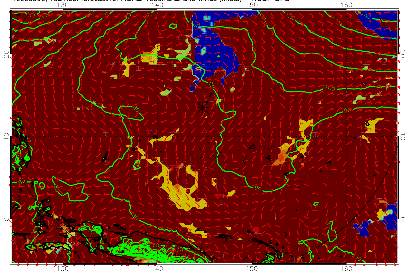
16090906, 102 hour forecast for HCAL, 1000mb Z, and winds (knots) -- NCEP GFS
