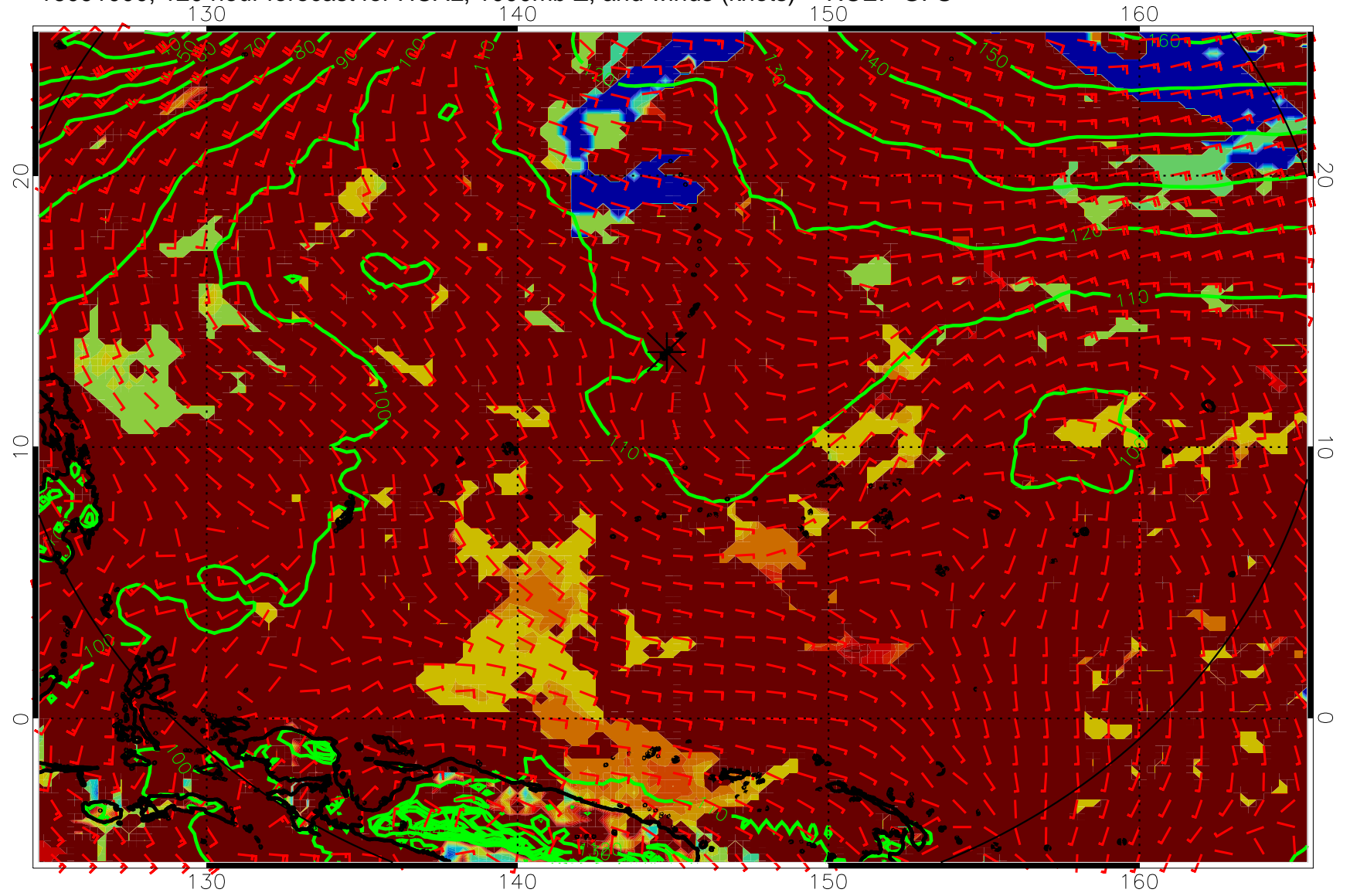
16091000, 120 hour forecast for HCAL, 1000mb Z, and winds (knots) -- NCEP GFS
