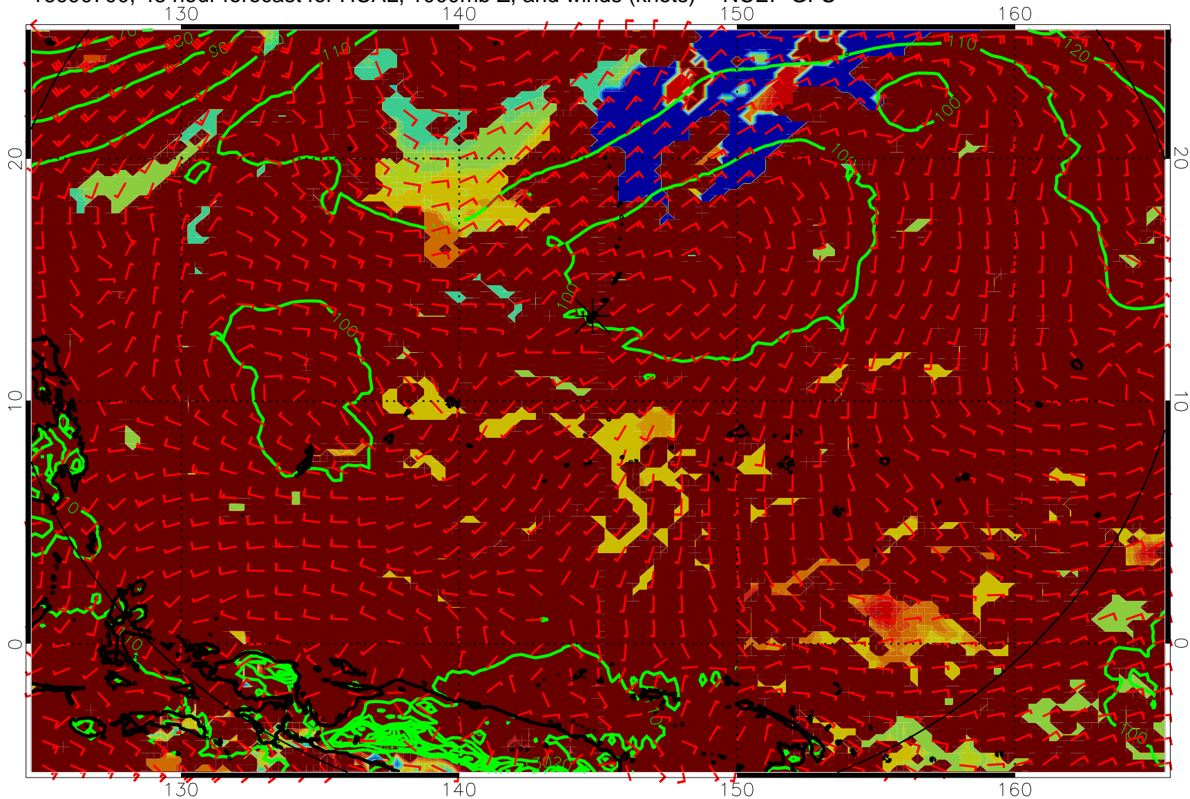
16090700, 48 hour forecast for HCAL, 1000mb Z, and winds (knots) -- NCEP GFS
