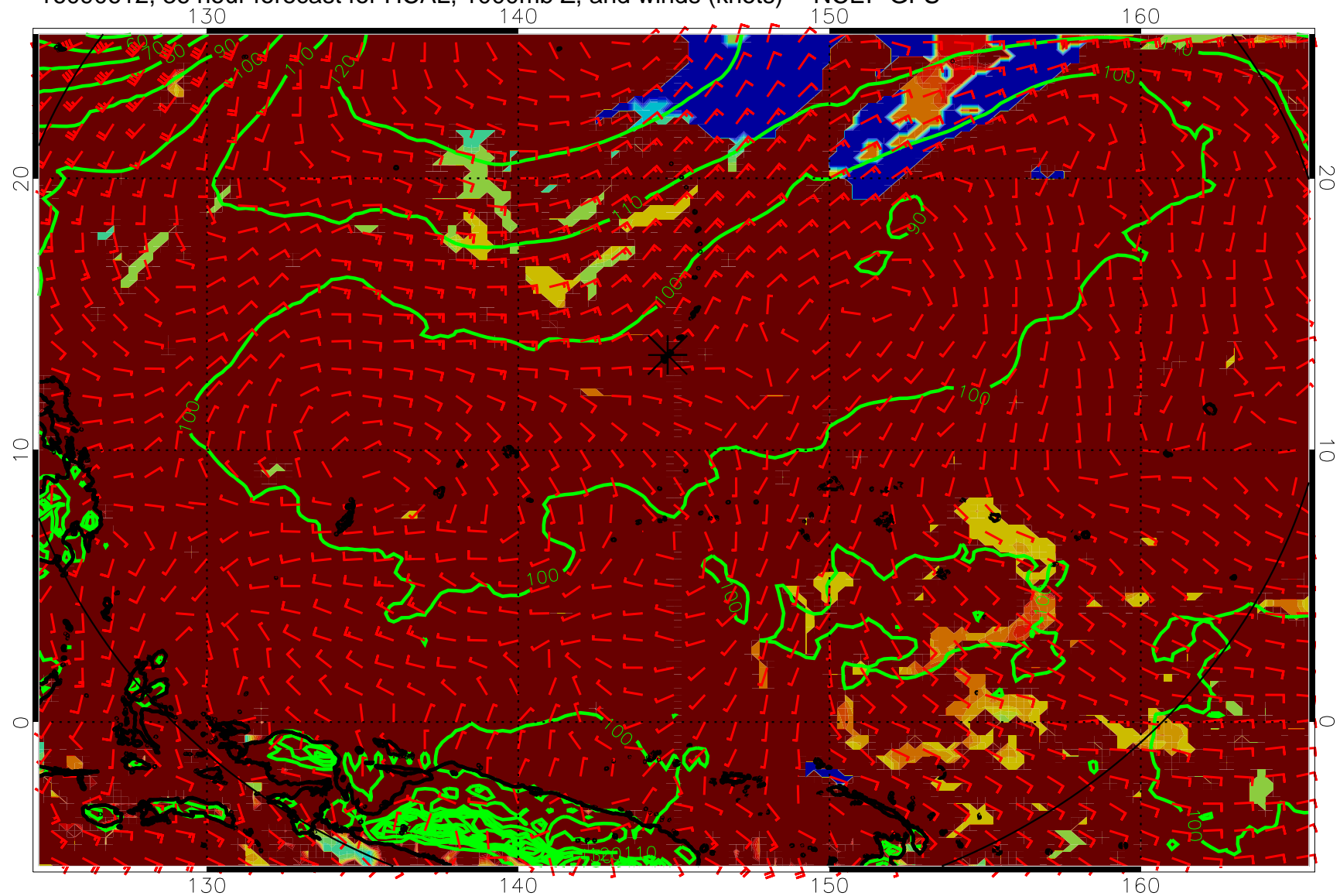
16090612, 36 hour forecast for HCAL, 1000mb Z, and winds (knots) -- NCEP GFS
