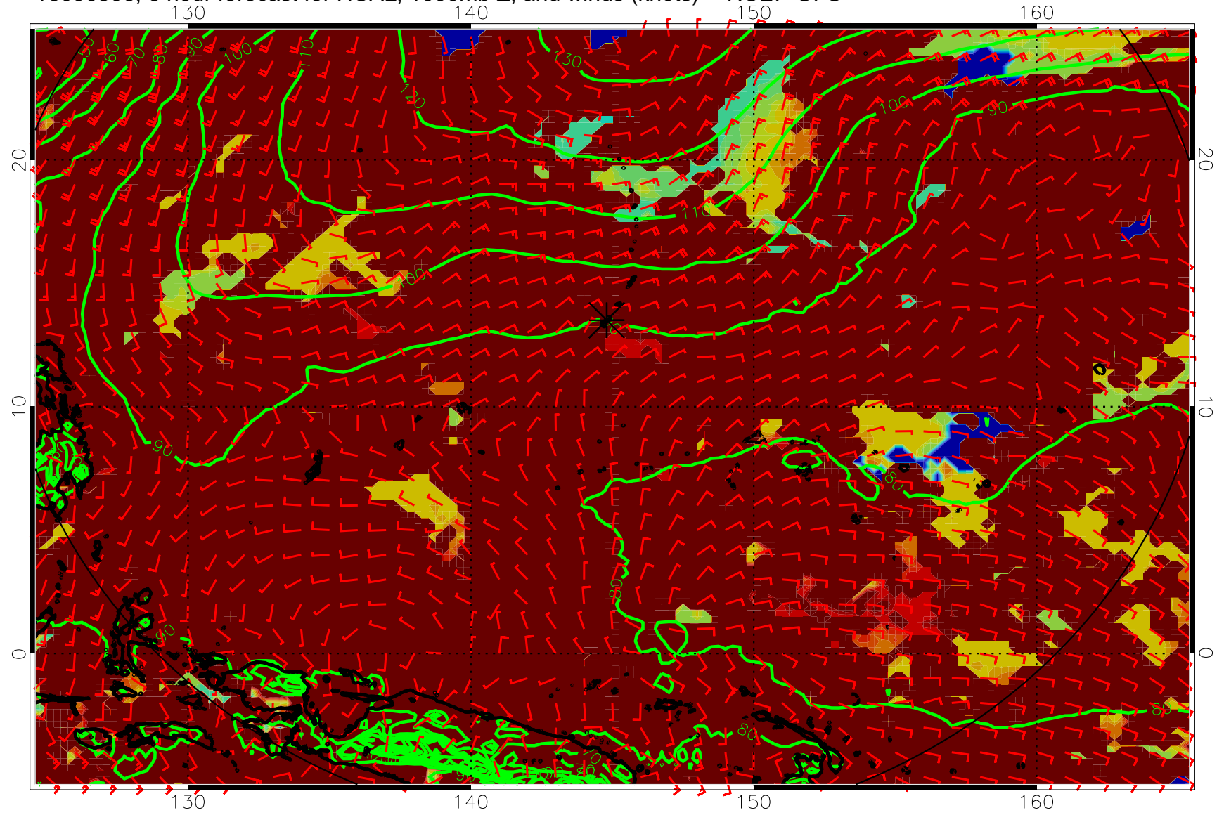
16090506, 6 hour forecast for HCAL, 1000mb Z, and winds (knots) -- NCEP GFS
