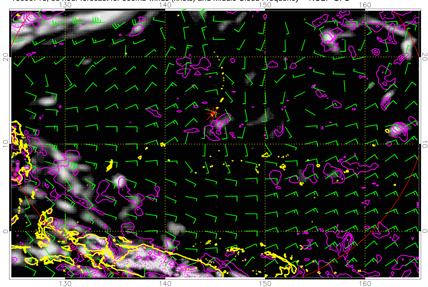
16090718, 66 hour forecast for 500mb winds (knots) and Middle Cloud Frequency -- NCEP GFS
